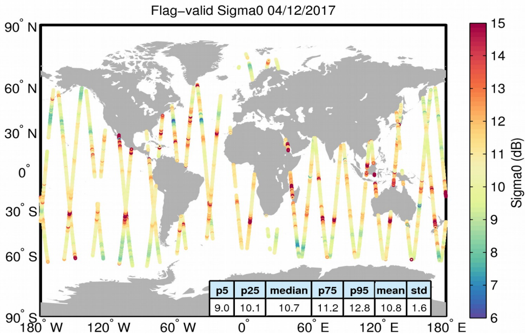
Figure 23. Geographical distribution of flag-valid sigma0 data over oceans and lakes for 04/12/2017. The statistical values shown in the table refer to the sigma0 in dB and are calculated over all measurements shown in the figure.
