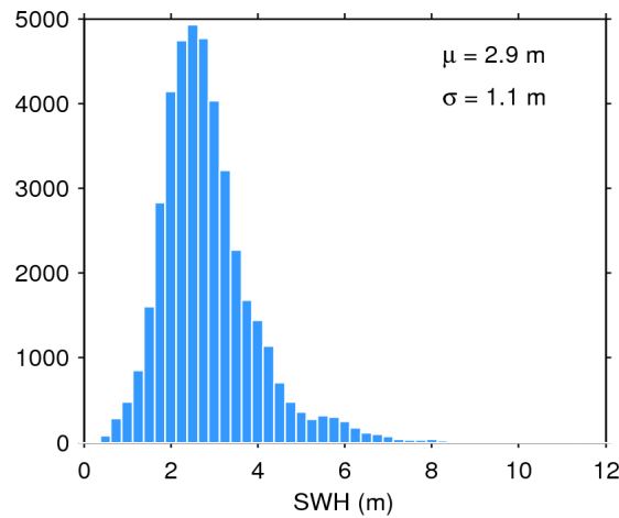
Figure 17. Histogram of flag-valid SWH over oceans and lakes for 04/12/2017. The mean ( \mu ) and standard deviation ( \sigma ) are also shown. Note that values larger than 12 m are excluded from the histogram for the sake of readability but not from the computation of \mu and \sigma .
