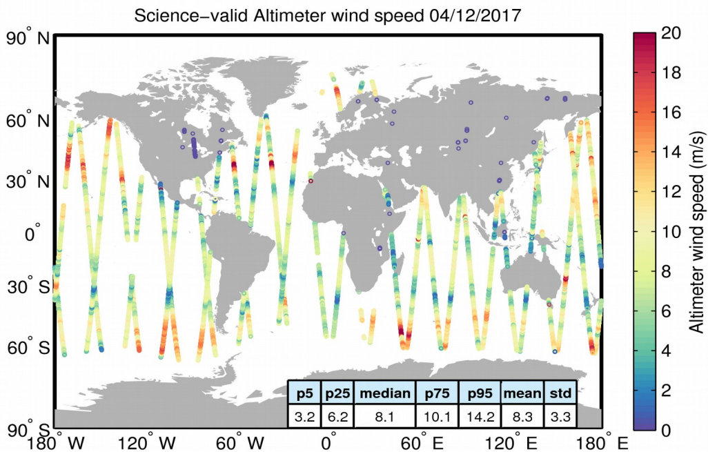
Figure 34. Geographical distribution of science-valid wind data over oceans and lakes for 04/12/2017. The statistical values shown in the table refer to the wind in m/s and are calculated over all measurements shown in the figure. Gray circles denote records that have been rejected based on the editing criteria described in Table 5.
