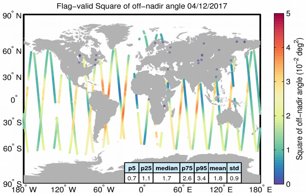
Figure 37. Geographical distribution of flag-valid mispointing data over oceans and lakes for 04/12/2017. The statistical values shown in the table refer to the mispointing in 10^{-2} deg 2 and are calculated over all measurements shown in the figure.
