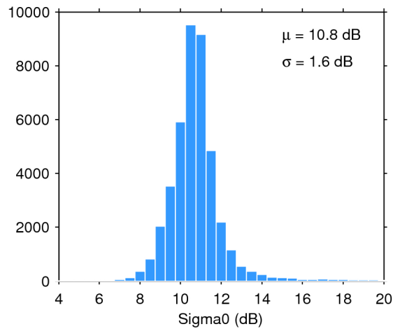
Figure 25. Histogram of flag-valid sigma0 over oceans and lakes for 04/12/2017. The mean ( \mu ) and standard deviation ( \sigma ) are also shown. Note that values outside [4 20] dB are excluded from the histogram for the sake of readability but not from the computation of \mu and \sigma .
