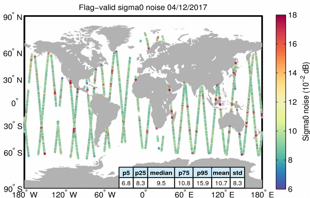
Figure 26. Geographical distribution of flag-valid 20-Hz sigma0 measurement noise over oceans and lakes for 04/12/2017. The statistical values shown in the table refer to the sigma0 noise and are calculated over all measurements shown in the figure.
