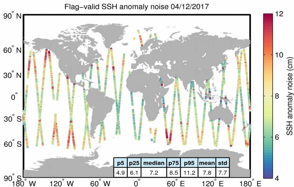
Figure 8. Geographical distribution of flag-valid 20-Hz SSH anomaly measurement noise over oceans and lakes for 04/12/2017. The statistical values shown in the table refer to the SSH anomaly noise and are calculated over all measurements shown in the figure.
