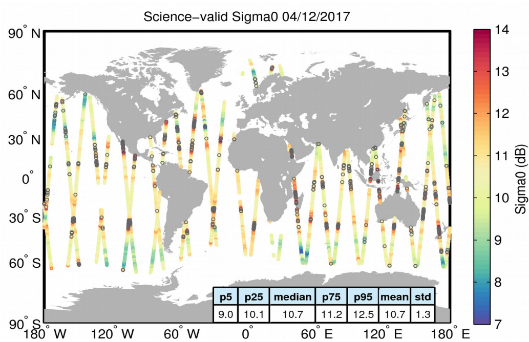
Figure 27. Geographical distribution of science-valid sigma0 data over oceans and lakes for 04/12/2017. The statistical values shown in the table refer to the sigma0 in dB and are calculated over all measurements shown in the figure. Gray circles denote records that have been rejected based on the editing criteria described in Table 4.
