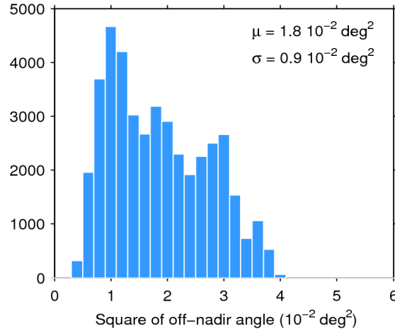
Figure 39. Histogram of flag-valid mispointing over oceans and lakes for 04/12/2017. The mean ( \mu ) and standard deviation ( \sigma ) are also shown. Note that values larger than 6 \cdot 10^{-2} \text{ deg}^2 are excluded from the histogram for the sake of readability but not from the computation of \mu and \sigma .
