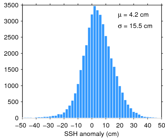
Figure 7. Histogram of flag-valid SSH anomaly over oceans and lakes for 04/12/2017. The mean ( \mu ) and standard deviation ( \sigma ) are also shown. Note that values outside [-50\ 50] cm are excluded from the histogram for the sake of readability but not from the computation of \mu and \sigma .
