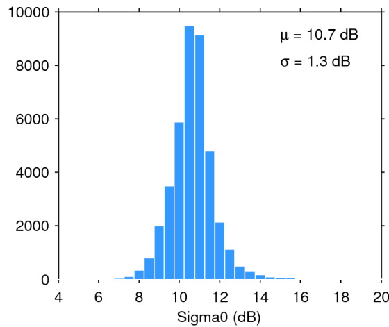
Figure 28. Histogram of science-valid sigma0 over oceans and lakes for 04/12/2017. The mean ( \mu ) and standard deviation ( \sigma ) are also shown. Note that values outside [4 20] dB are excluded from the histogram for the sake of readability but not from the computation of \mu and \sigma .
