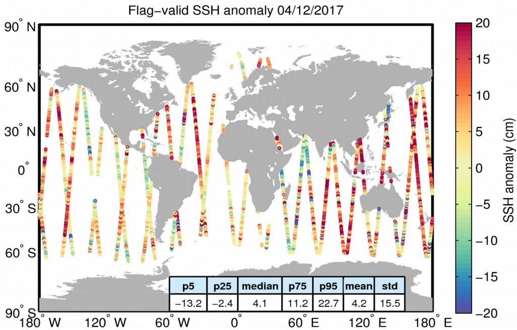
Figure 5. Geographical distribution of flag-valid 1-Hz SSH anomaly data over oceans and lakes for 04/12/2017. The statistical values shown in the table refer to the SSH anomaly in cm and are calculated over all measurements shown in the figure.
