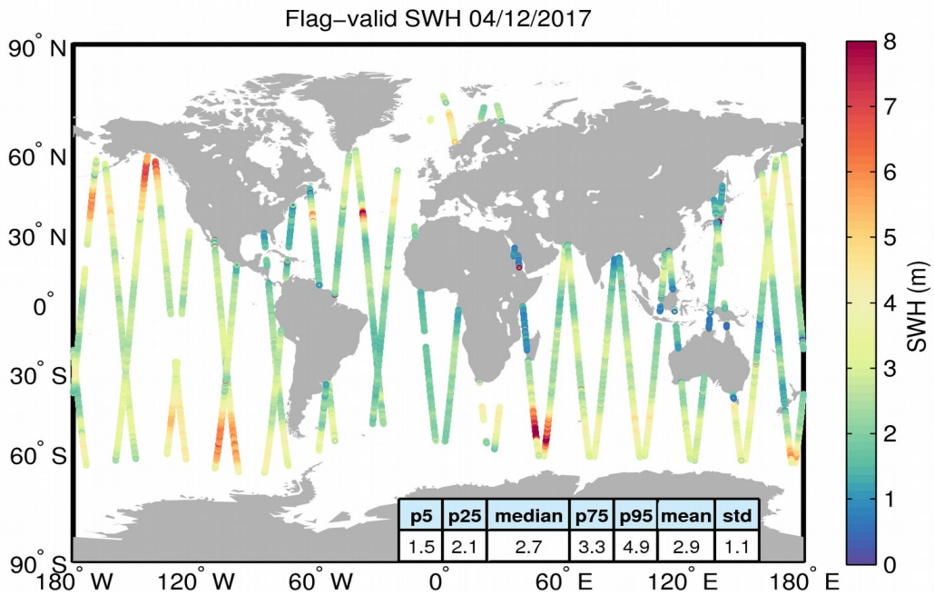
Figure 15. Geographical distribution of flag-valid SWH data over oceans and lakes for 04/12/2017. The statistical values shown in the table refer to the SWH in m and are calculated over all measurements shown in the figure.
