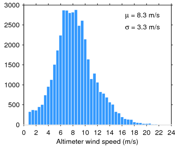
Figure 33. Histogram of flag-valid wind over oceans and lakes for 04/12/2017. The mean ( \mu ) and standard deviation ( \sigma ) are also shown. Note that values larger than 24 m/s are excluded from the histogram for the sake of readability but not from the computation of \mu and \sigma .
