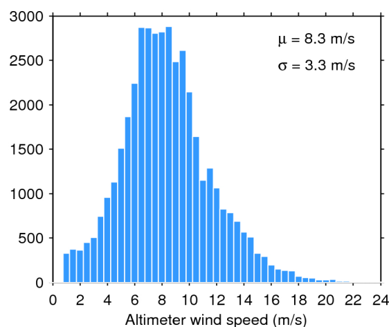
Figure 35. Histogram of science-valid wind over oceans and lakes for 04/12/2017. The mean ( \mu ) and standard deviation ( \sigma ) are also shown. Note that values larger than 24 m/s are excluded from the histogram for the sake of readability but not from the computation of \mu and \sigma .
