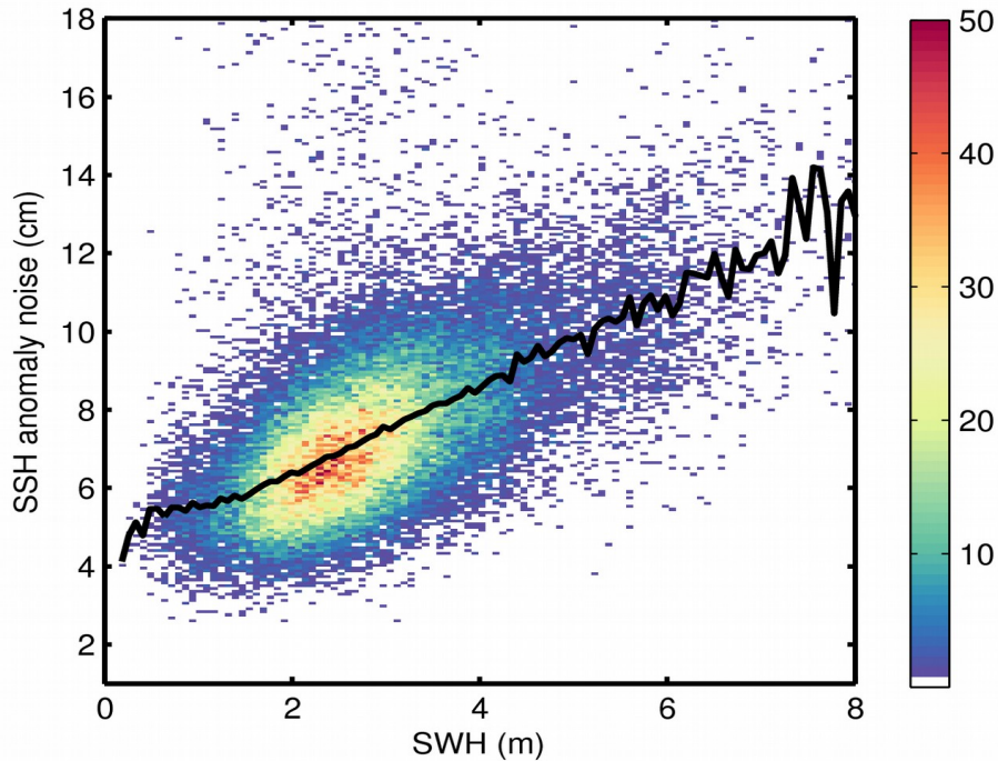
Figure 9. 2D histogram showing flag-valid SSH anomaly noise as a function of SWH for 04/12/2017. The black line denotes the median SSH anomaly noise as a function of SWH.
