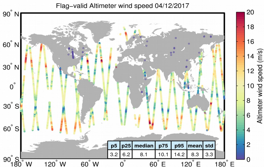
Figure 31. Geographical distribution of flag-valid wind data over oceans and lakes for 04/12/2017. The statistical values shown in the table refer to the wind in m/s and are calculated over all measurements shown in the figure.
