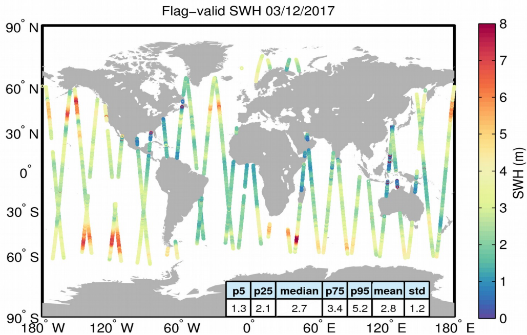
Figure 15. Geographical distribution of flag-valid SWH data over oceans and lakes for 03/12/2017. The statistical values shown in the table refer to the SWH in m and are calculated over all measurements shown in the figure.
