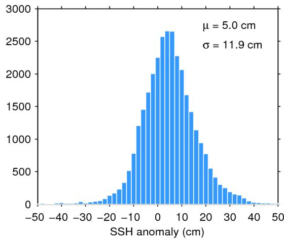
Figure 11. Histogram of science-valid SSH anomaly over oceans and lakes for 03/12/2017. The mean ( \mu ) and standard deviation ( \sigma ) are also shown. Note that values outside [-50 50] cm are excluded from the histogram for the sake of readability but not from the computation of \mu and \sigma .
