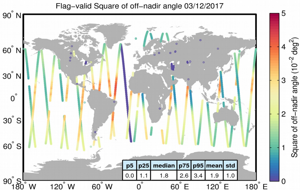
Figure 37. Geographical distribution of flag-valid mispointing data over oceans and lakes for 03/12/2017. The statistical values shown in the table refer to the mispointing in 10^{-2} deg 2 and are calculated over all measurements shown in the figure.
