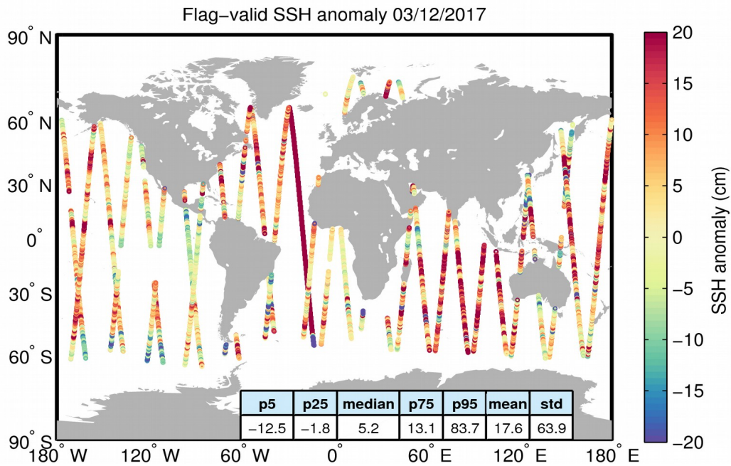
Figure 5. Geographical distribution of flag-valid 1-Hz SSH anomaly data over oceans and lakes for 03/12/2017. The statistical values shown in the table refer to the SSH anomaly in cm and are calculated over all measurements shown in the figure.
