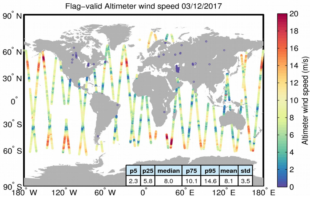
Figure 31. Geographical distribution of flag-valid wind data over oceans and lakes for 03/12/2017. The statistical values shown in the table refer to the wind in m/s and are calculated over all measurements shown in the figure.
