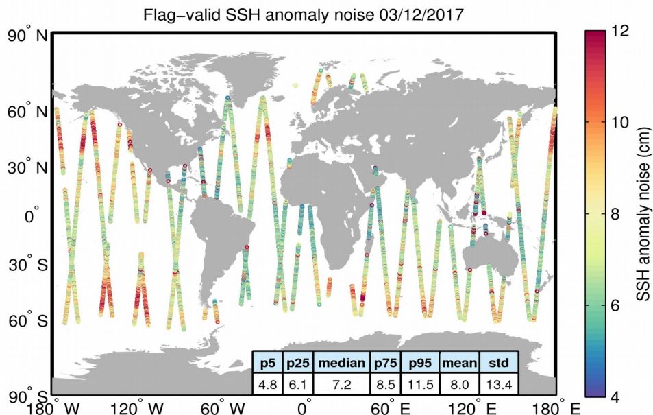
Figure 8. Geographical distribution of flag-valid 20-Hz SSH anomaly measurement noise over oceans and lakes for 03/12/2017. The statistical values shown in the table refer to the SSH anomaly noise and are calculated over all measurements shown in the figure.
