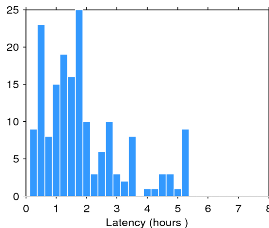
Figure 2. Histogram of the data latency for 03/12/2017. The y-axis denotes the number of files that are made available with a delay of x-hours with respect to the mean time of the records stored in the file.
