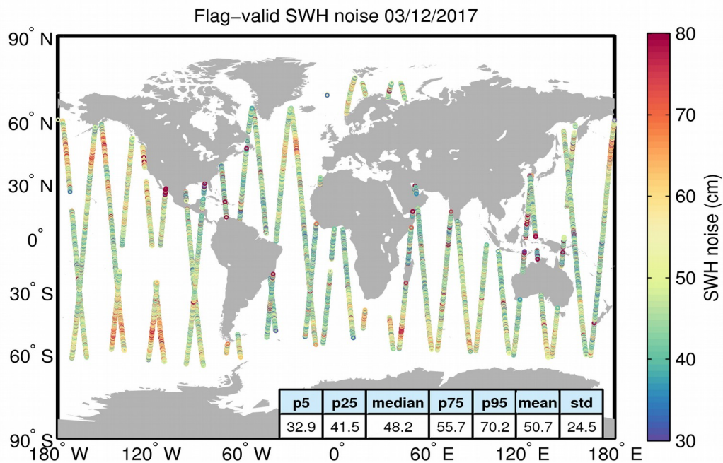
Figure 18. Geographical distribution of flag-valid 20-Hz SWH measurement noise over oceans and lakes for 03/12/2017. The statistical values shown in the table refer to the SWH noise and are calculated over all measurements shown in the figure.
