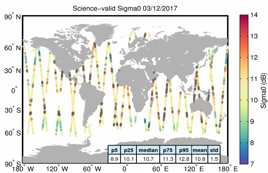
Figure 27. Geographical distribution of science-valid sigma0 data over oceans and lakes for 03/12/2017. The statistical values shown in the table refer to the sigma0 in dB and are calculated over all measurements shown in the figure. Gray circles denote records that have been rejected based on the editing criteria described in Table 4.
