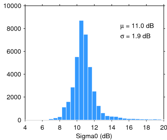
Figure 25. Histogram of flag-valid sigma0 over oceans and lakes for 03/12/2017. The mean ( \mu ) and standard deviation ( \sigma ) are also shown. Note that values outside [4 20] dB are excluded from the histogram for the sake of readability but not from the computation of \mu and \sigma .
