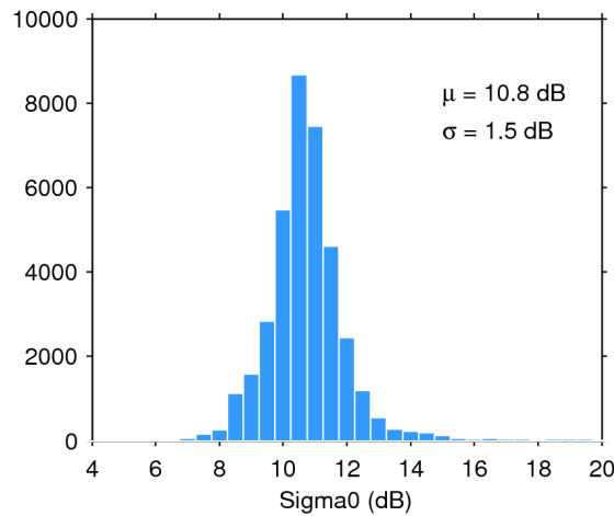
Figure 28. Histogram of science-valid sigma0 over oceans and lakes for 03/12/2017. The mean ( \mu ) and standard deviation ( \sigma ) are also shown. Note that values outside [4 20] dB are excluded from the histogram for the sake of readability but not from the computation of \mu and \sigma .
