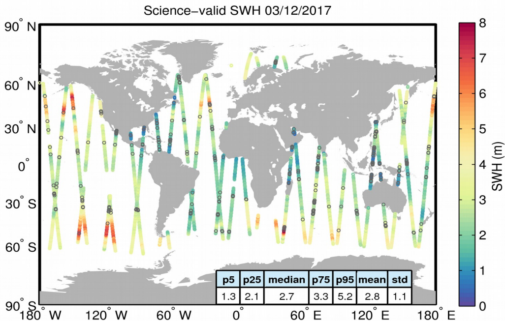
Figure 19. Geographical distribution of science-valid SWH data over oceans and lakes for 03/12/2017. The statistical values shown in the table refer to the SWH in m and are calculated over all measurements shown in the figure. Gray circles denote records that have been rejected based on the editing criteria described in Table 3.
