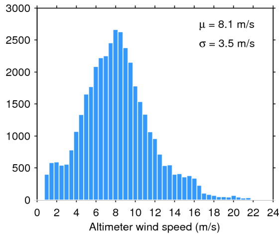
Figure 33. Histogram of flag-valid wind over oceans and lakes for 03/12/2017. The mean ( \mu ) and standard deviation ( \sigma ) are also shown. Note that values larger than 24 m/s are excluded from the histogram for the sake of readability but not from the computation of \mu and \sigma .
