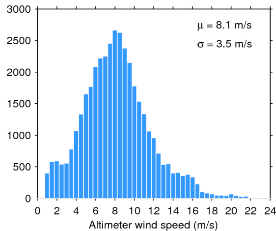
Figure 35. Histogram of science-valid wind over oceans and lakes for 03/12/2017. The mean ( \mu ) and standard deviation ( \sigma ) are also shown. Note that values larger than 24 m/s are excluded from the histogram for the sake of readability but not from the computation of \mu and \sigma .
