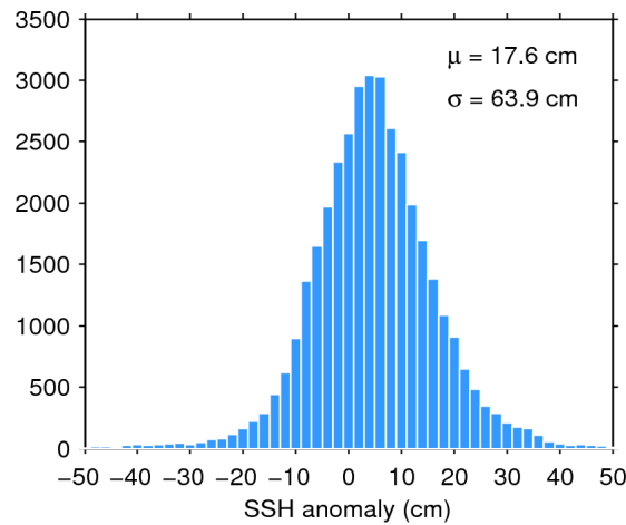
Figure 7. Histogram of flag-valid SSH anomaly over oceans and lakes for 03/12/2017. The mean ( \mu ) and standard deviation ( \sigma ) are also shown. Note that values outside [-50 50] cm are excluded from the histogram for the sake of readability but not from the computation of \mu and \sigma .
