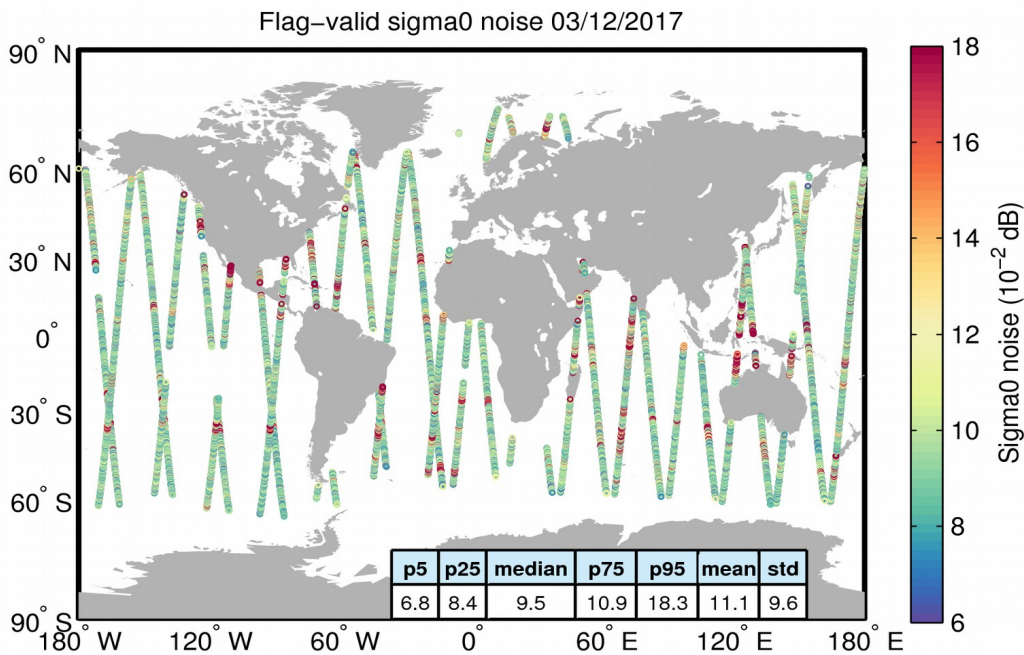
Figure 26. Geographical distribution of flag-valid 20-Hz sigma0 measurement noise over oceans and lakes for 03/12/2017. The statistical values shown in the table refer to the sigma0 noise and are calculated over all measurements shown in the figure.
