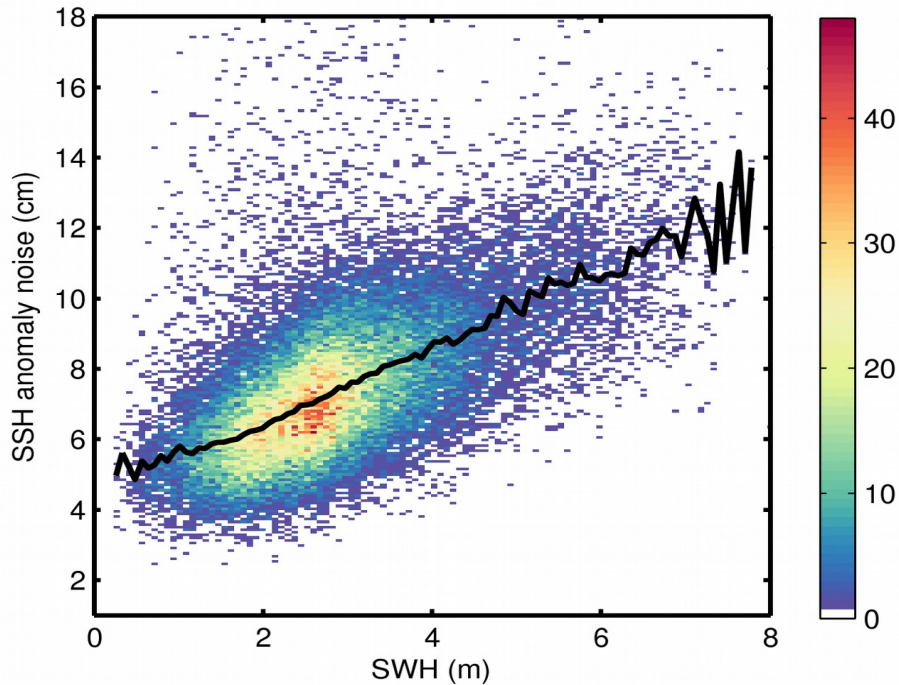
Figure 9. 2D histogram showing flag-valid SSH anomaly noise as a function of SWH for 03/12/2017. The black line denotes the median SSH anomaly noise as a function of SWH.
