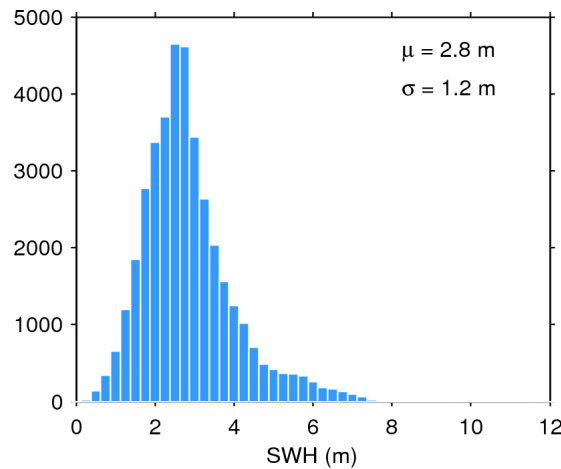
Figure 17. Histogram of flag-valid SWH over oceans and lakes for 03/12/2017. The mean ( \mu ) and standard deviation ( \sigma ) are also shown. Note that values larger than 12 m are excluded from the histogram for the sake of readability but not from the computation of \mu and \sigma .
