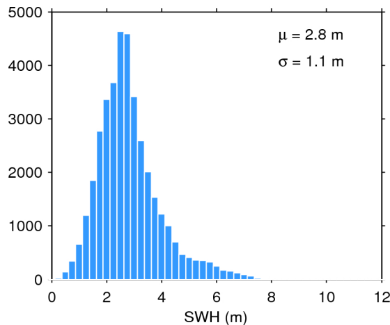
Figure 20. Histogram of science-valid SWH over oceans and lakes for 03/12/2017. The mean ( \mu ) and standard deviation ( \sigma ) are also shown. Note that values larger than 12 m are excluded from the histogram for the sake of readability but not from the computation of \mu and \sigma .
