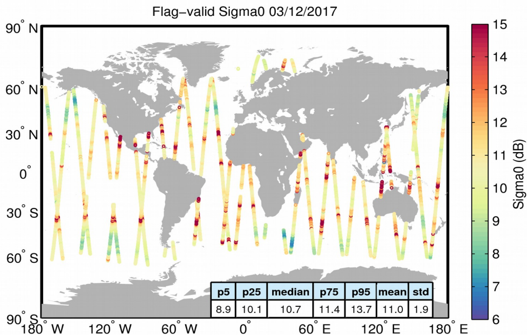
Figure 23. Geographical distribution of flag-valid sigma0 data over oceans and lakes for 03/12/2017. The statistical values shown in the table refer to the sigma0 in dB and are calculated over all measurements shown in the figure.
