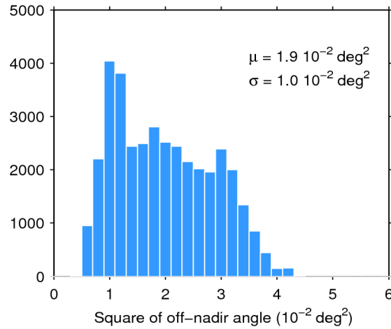
Figure 39. Histogram of flag-valid mispointing over oceans and lakes for 03/12/2017. The mean ( \mu ) and standard deviation ( \sigma ) are also shown. Note that values larger than 6 \cdot 10^{-2} \text{ deg}^2 are excluded from the histogram for the sake of readability but not from the computation of \mu and \sigma .
