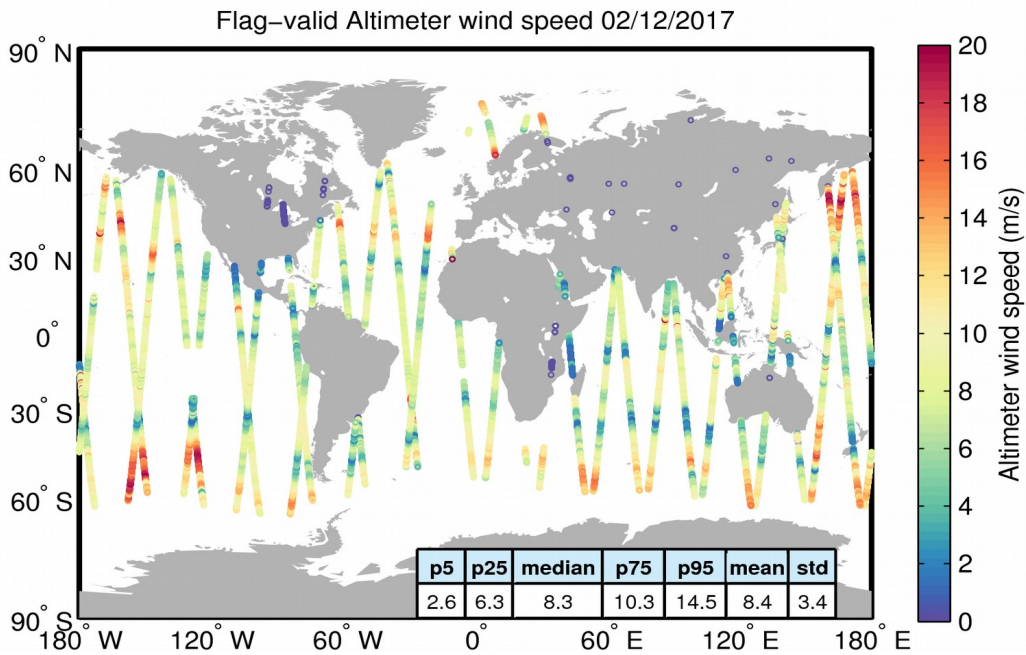
Figure 31. Geographical distribution of flag-valid wind data over oceans and lakes for 02/12/2017. The statistical values shown in the table refer to the wind in m/s and are calculated over all measurements shown in the figure.
