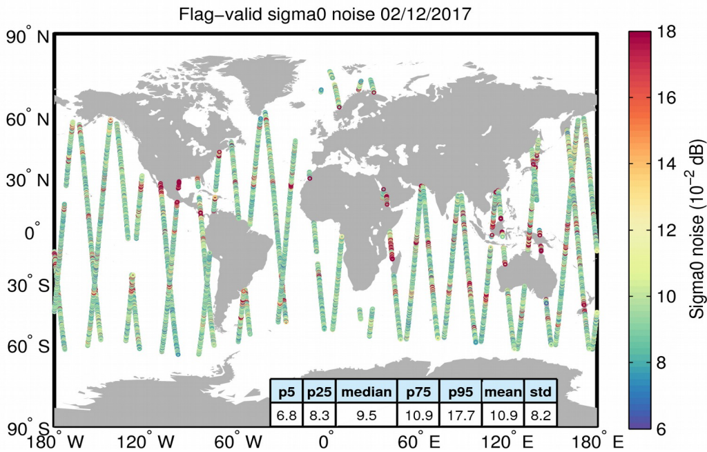
Figure 26. Geographical distribution of flag-valid 20-Hz sigma0 measurement noise over oceans and lakes for 02/12/2017. The statistical values shown in the table refer to the sigma0 noise and are calculated over all measurements shown in the figure.
