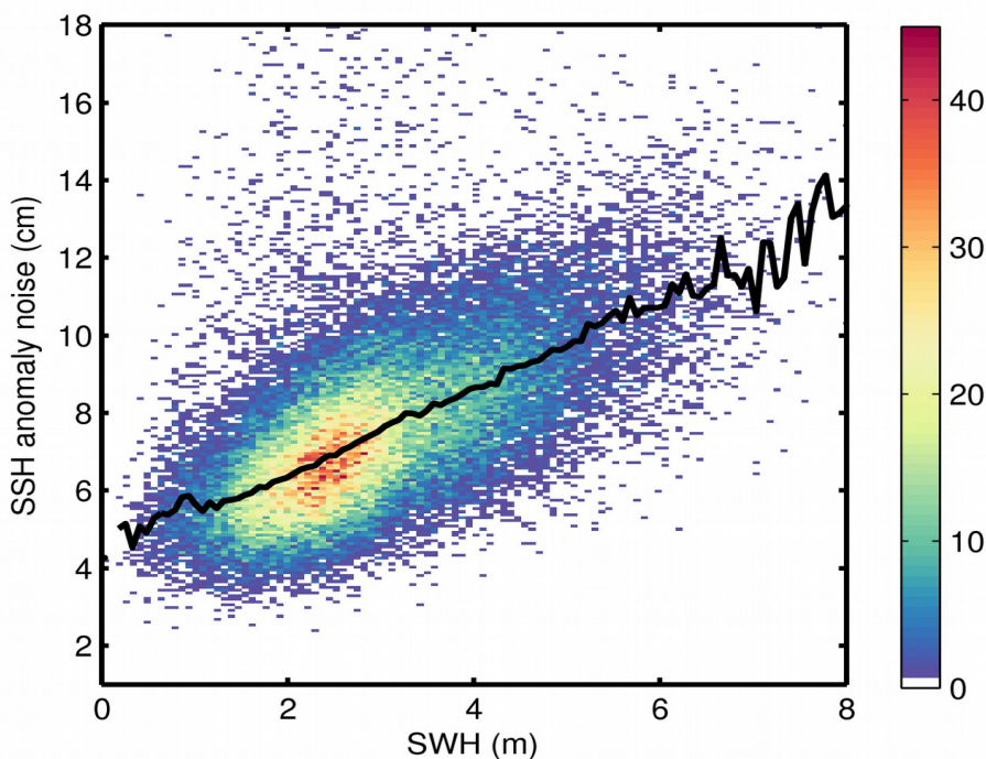
Figure 9. 2D histogram showing flag-valid SSH anomaly noise as a function of SWH for 02/12/2017. The black line denotes the median SSH anomaly noise as a function of SWH.
