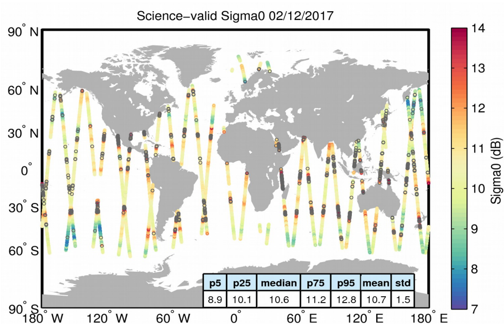
Figure 27. Geographical distribution of science-valid sigma0 data over oceans and lakes for 02/12/2017. The statistical values shown in the table refer to the sigma0 in dB and are calculated over all measurements shown in the figure. Gray circles denote records that have been rejected based on the editing criteria described in Table 4.
