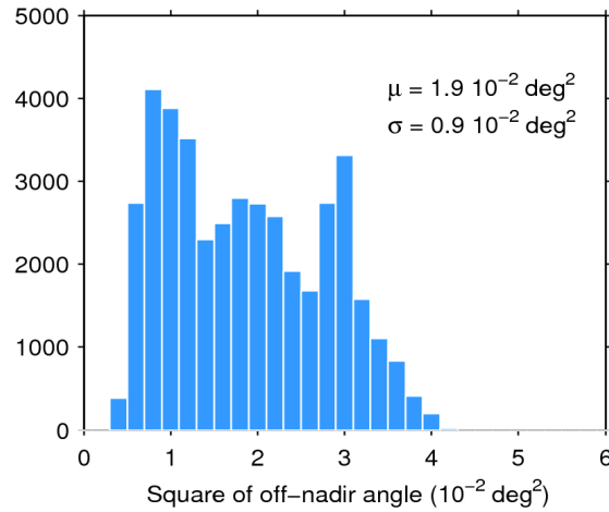
Figure 39. Histogram of flag-valid mispointing over oceans and lakes for 02/12/2017. The mean ( \mu ) and standard deviation ( \sigma ) are also shown. Note that values larger than 6 \cdot 10^{-2} \text{ deg}^2 are excluded from the histogram for the sake of readability but not from the computation of \mu and \sigma .
