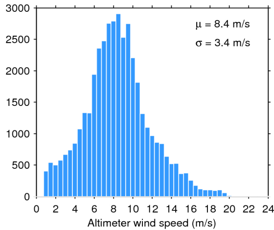
Figure 33. Histogram of flag-valid wind over oceans and lakes for 02/12/2017. The mean ( \mu ) and standard deviation ( \sigma ) are also shown. Note that values larger than 24 m/s are excluded from the histogram for the sake of readability but not from the computation of \mu and \sigma .
