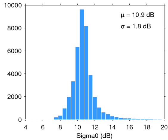
Figure 25. Histogram of flag-valid sigma0 over oceans and lakes for 02/12/2017. The mean ( \mu ) and standard deviation ( \sigma ) are also shown. Note that values outside [4 20] dB are excluded from the histogram for the sake of readability but not from the computation of \mu and \sigma .
