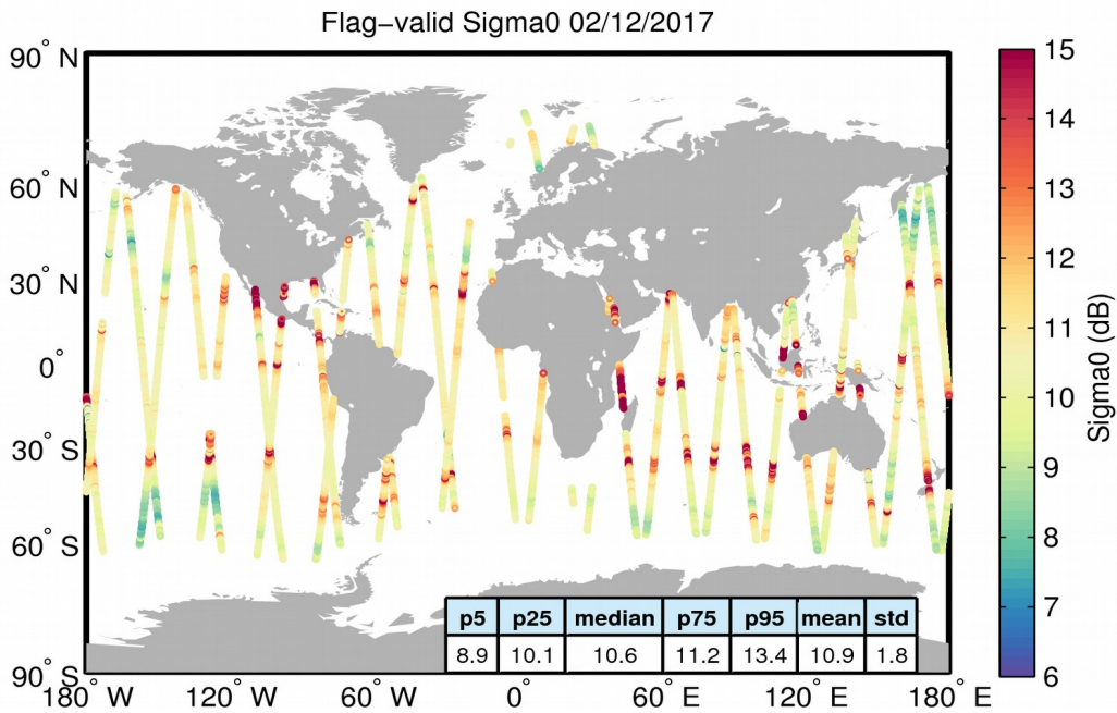
Figure 23. Geographical distribution of flag-valid sigma0 data over oceans and lakes for 02/12/2017. The statistical values shown in the table refer to the sigma0 in dB and are calculated over all measurements shown in the figure.
