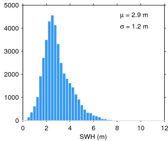
Figure 17. Histogram of flag-valid SWH over oceans and lakes for 02/12/2017. The mean ( \mu ) and standard deviation ( \sigma ) are also shown. Note that values larger than 12 m are excluded from the histogram for the sake of readability but not from the computation of \mu and \sigma .
