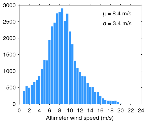
Figure 35. Histogram of science-valid wind over oceans and lakes for 02/12/2017. The mean ( \mu ) and standard deviation ( \sigma ) are also shown. Note that values larger than 24 m/s are excluded from the histogram for the sake of readability but not from the computation of \mu and \sigma .
