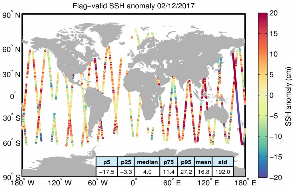
Figure 5. Geographical distribution of flag-valid 1-Hz SSH anomaly data over oceans and lakes for 02/12/2017. The statistical values shown in the table refer to the SSH anomaly in cm and are calculated over all measurements shown in the figure.
