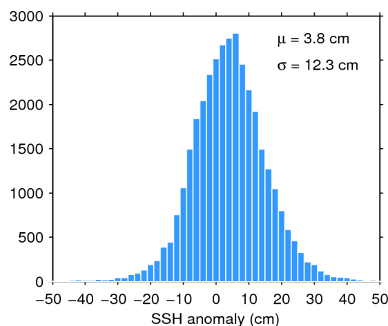
Figure 11. Histogram of science-valid SSH anomaly over oceans and lakes for 02/12/2017. The mean ( \mu ) and standard deviation ( \sigma ) are also shown. Note that values outside [-50 50] cm are excluded from the histogram for the sake of readability but not from the computation of \mu and \sigma .
