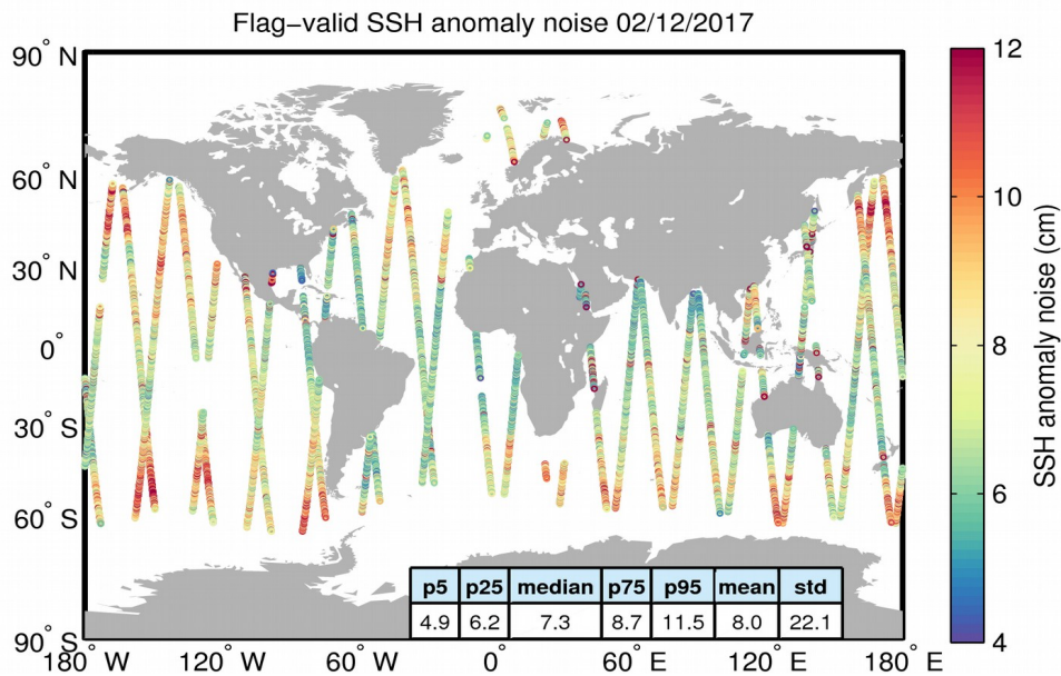
Figure 8. Geographical distribution of flag-valid 20-Hz SSH anomaly measurement noise over oceans and lakes for 02/12/2017. The statistical values shown in the table refer to the SSH anomaly noise and are calculated over all measurements shown in the figure.
