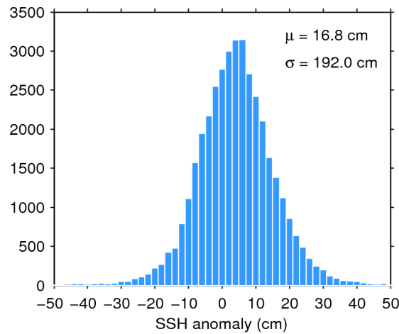
Figure 7. Histogram of flag-valid SSH anomaly over oceans and lakes for 02/12/2017. The mean ( \mu ) and standard deviation ( \sigma ) are also shown. Note that values outside [-50 50] cm are excluded from the histogram for the sake of readability but not from the computation of \mu and \sigma .
