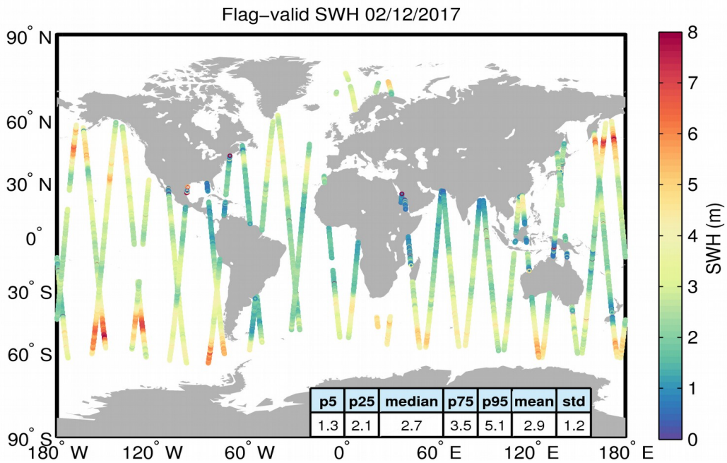
Figure 15. Geographical distribution of flag-valid SWH data over oceans and lakes for 02/12/2017. The statistical values shown in the table refer to the SWH in m and are calculated over all measurements shown in the figure.
