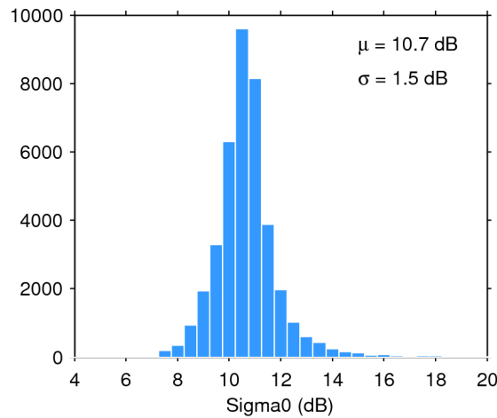
Figure 28. Histogram of science-valid sigma0 over oceans and lakes for 02/12/2017. The mean ( \mu ) and standard deviation ( \sigma ) are also shown. Note that values outside [4 20] dB are excluded from the histogram for the sake of readability but not from the computation of \mu and \sigma .
