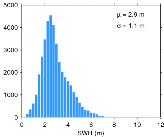
Figure 20. Histogram of science-valid SWH over oceans and lakes for 02/12/2017. The mean ( \mu ) and standard deviation ( \sigma ) are also shown. Note that values larger than 12 m are excluded from the histogram for the sake of readability but not from the computation of \mu and \sigma .
