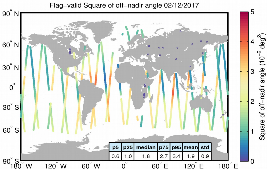
Figure 37. Geographical distribution of flag-valid mispointing data over oceans and lakes for 02/12/2017. The statistical values shown in the table refer to the mispointing in 10^{-2} deg 2 and are calculated over all measurements shown in the figure.
