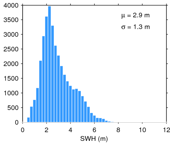
Figure 17. Histogram of flag-valid SWH over oceans and lakes for 30/11/2017. The mean ( \mu ) and standard deviation ( \sigma ) are also shown. Note that values larger than 12 m are excluded from the histogram for the sake of readability but not from the computation of \mu and \sigma .
