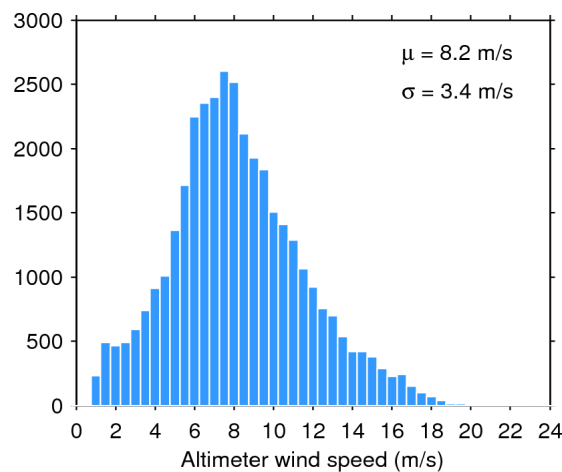
Figure 35. Histogram of science-valid wind over oceans and lakes for 30/11/2017. The mean ( \mu ) and standard deviation ( \sigma ) are also shown. Note that values larger than 24 m/s are excluded from the histogram for the sake of readability but not from the computation of \mu and \sigma .
