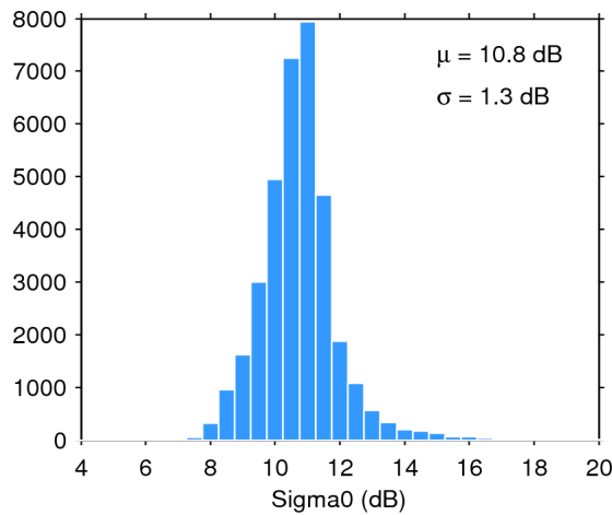
Figure 28. Histogram of science-valid sigma0 over oceans and lakes for 30/11/2017. The mean ( \mu ) and standard deviation ( \sigma ) are also shown. Note that values outside [4 20] dB are excluded from the histogram for the sake of readability but not from the computation of \mu and \sigma .
