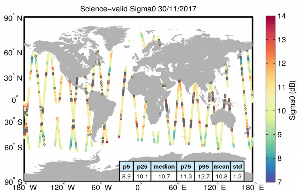
Figure 27. Geographical distribution of science-valid sigma0 data over oceans and lakes for 30/11/2017. The statistical values shown in the table refer to the sigma0 in dB and are calculated over all measurements shown in the figure. Gray circles denote records that have been rejected based on the editing criteria described in Table 4.
