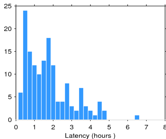
Figure 2. Histogram of the data latency for 30/11/2017. The y-axis denotes the number of files that are made available with a delay of x-hours with respect to the mean time of the records stored in the file.
