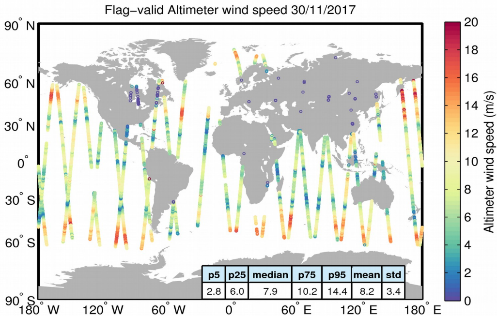
Figure 31. Geographical distribution of flag-valid wind data over oceans and lakes for 30/11/2017. The statistical values shown in the table refer to the wind in m/s and are calculated over all measurements shown in the figure.
