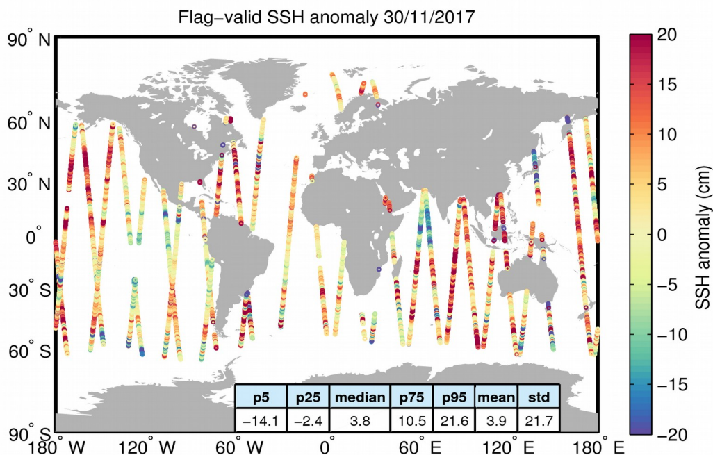
Figure 5. Geographical distribution of flag-valid 1-Hz SSH anomaly data over oceans and lakes for 30/11/2017. The statistical values shown in the table refer to the SSH anomaly in cm and are calculated over all measurements shown in the figure.
