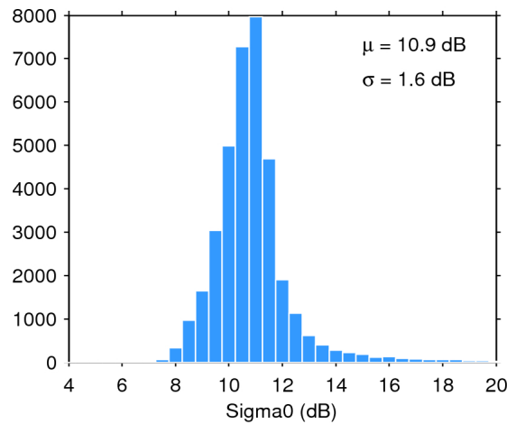
Figure 25. Histogram of flag-valid sigma0 over oceans and lakes for 30/11/2017. The mean ( \mu ) and standard deviation ( \sigma ) are also shown. Note that values outside [4 20] dB are excluded from the histogram for the sake of readability but not from the computation of \mu and \sigma .
