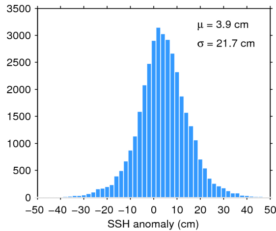
Figure 7. Histogram of flag-valid SSH anomaly over oceans and lakes for 30/11/2017. The mean ( \mu ) and standard deviation ( \sigma ) are also shown. Note that values outside [-50 50] cm are excluded from the histogram for the sake of readability but not from the computation of \mu and \sigma .
