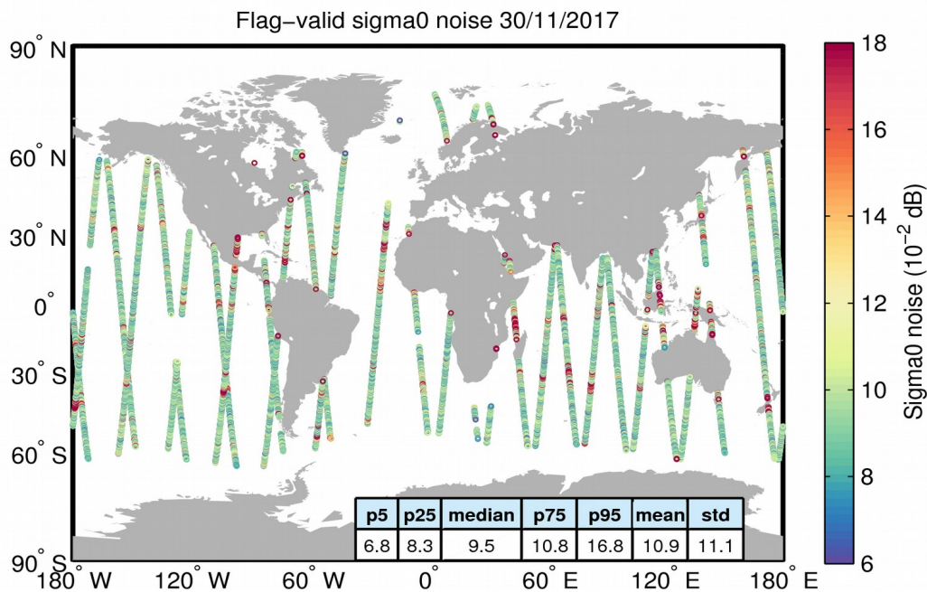
Figure 26. Geographical distribution of flag-valid 20-Hz sigma0 measurement noise over oceans and lakes for 30/11/2017. The statistical values shown in the table refer to the sigma0 noise and are calculated over all measurements shown in the figure.
