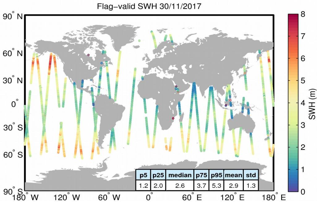
Figure 15. Geographical distribution of flag-valid SWH data over oceans and lakes for 30/11/2017. The statistical values shown in the table refer to the SWH in m and are calculated over all measurements shown in the figure.
