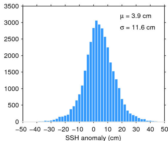
Figure 11. Histogram of science-valid SSH anomaly over oceans and lakes for 30/11/2017. The mean ( \mu ) and standard deviation ( \sigma ) are also shown. Note that values outside [-50 50] cm are excluded from the histogram for the sake of readability but not from the computation of \mu and \sigma .
