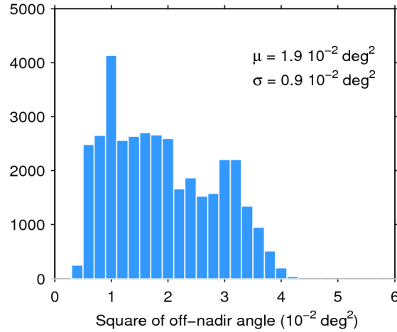
Figure 39. Histogram of flag-valid mispointing over oceans and lakes for 30/11/2017. The mean ( \mu ) and standard deviation ( \sigma ) are also shown. Note that values larger than 6 \cdot 10^{-2} \text{ deg}^2 are excluded from the histogram for the sake of readability but not from the computation of \mu and \sigma .
