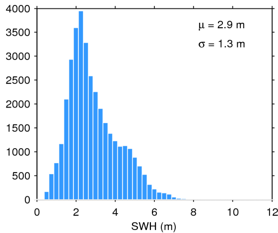
Figure 20. Histogram of science-valid SWH over oceans and lakes for 30/11/2017. The mean ( \mu ) and standard deviation ( \sigma ) are also shown. Note that values larger than 12 m are excluded from the histogram for the sake of readability but not from the computation of \mu and \sigma .
