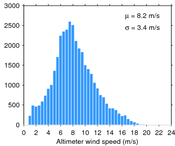
Figure 33. Histogram of flag-valid wind over oceans and lakes for 30/11/2017. The mean ( \mu ) and standard deviation ( \sigma ) are also shown. Note that values larger than 24 m/s are excluded from the histogram for the sake of readability but not from the computation of \mu and \sigma .
