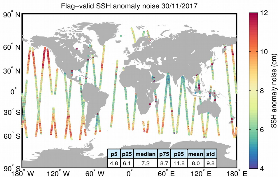
Figure 8. Geographical distribution of flag-valid 20-Hz SSH anomaly measurement noise over oceans and lakes for 30/11/2017. The statistical values shown in the table refer to the SSH anomaly noise and are calculated over all measurements shown in the figure.
