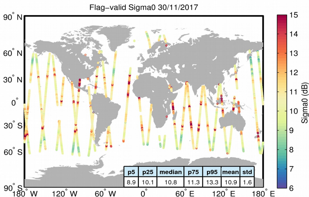
Figure 23. Geographical distribution of flag-valid sigma0 data over oceans and lakes for 30/11/2017. The statistical values shown in the table refer to the sigma0 in dB and are calculated over all measurements shown in the figure.
