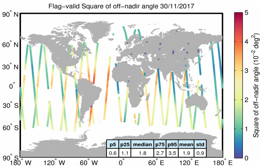
Figure 37. Geographical distribution of flag-valid mispointing data over oceans and lakes for 30/11/2017. The statistical values shown in the table refer to the mispointing in 10^{-2} deg 2 and are calculated over all measurements shown in the figure.
