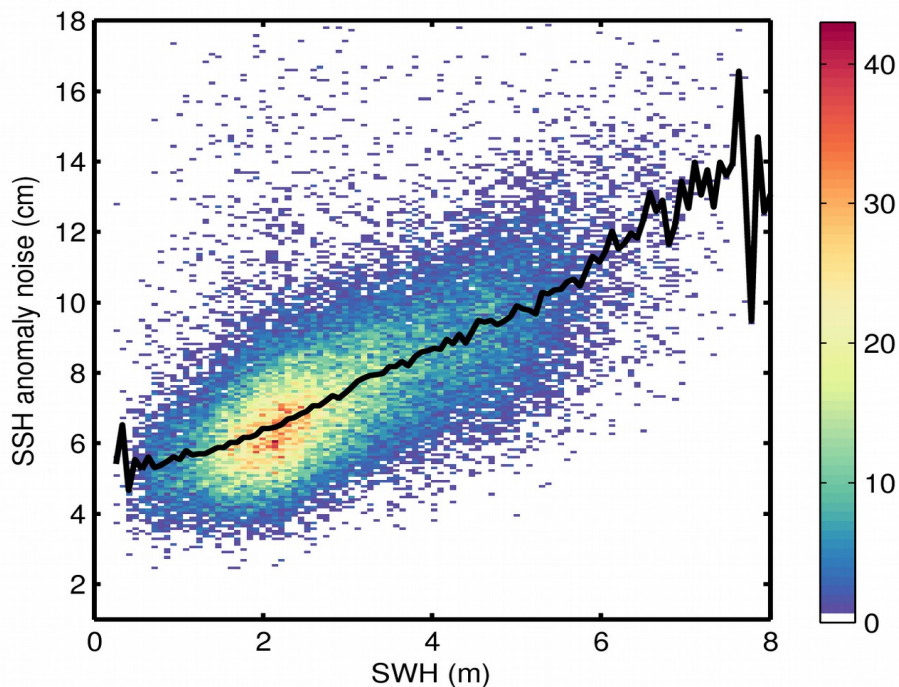
Figure 9. 2D histogram showing flag-valid SSH anomaly noise as a function of SWH for 30/11/2017. The black line denotes the median SSH anomaly noise as a function of SWH.
