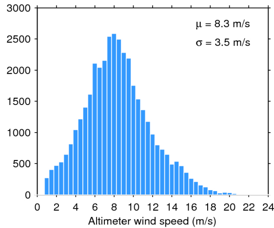
Figure 33. Histogram of flag-valid wind over oceans and lakes for 29/11/2017. The mean ( \mu ) and standard deviation ( \sigma ) are also shown. Note that values larger than 24 m/s are excluded from the histogram for the sake of readability but not from the computation of \mu and \sigma .
