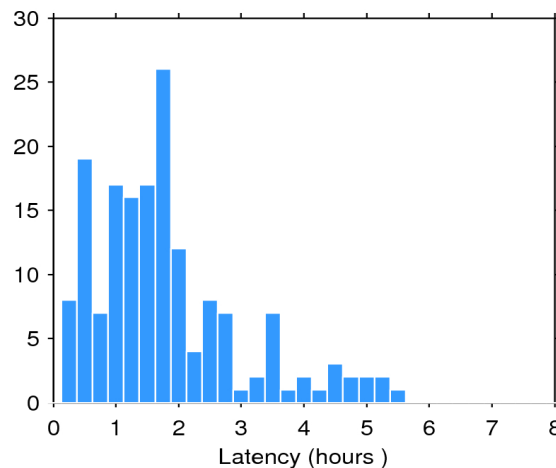
Figure 2. Histogram of the data latency for 29/11/2017. The y-axis denotes the number of files that are made available with a delay of x-hours with respect to the mean time of the records stored in the file.
