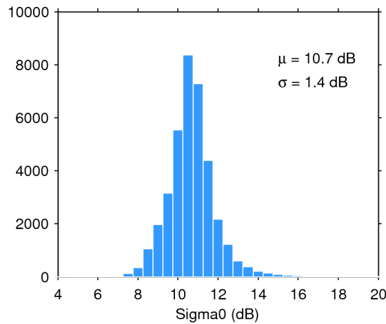
Figure 28. Histogram of science-valid sigma0 over oceans and lakes for 29/11/2017. The mean ( \mu ) and standard deviation ( \sigma ) are also shown. Note that values outside [4 20] dB are excluded from the histogram for the sake of readability but not from the computation of \mu and \sigma .
