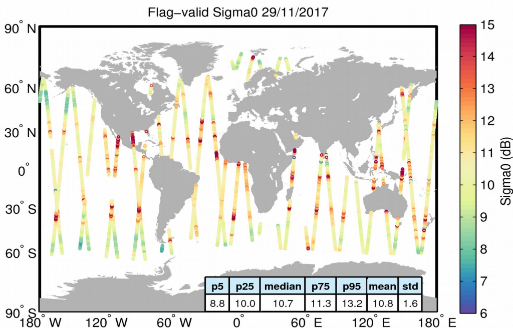
Figure 23. Geographical distribution of flag-valid sigma0 data over oceans and lakes for 29/11/2017. The statistical values shown in the table refer to the sigma0 in dB and are calculated over all measurements shown in the figure.
