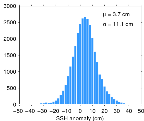
Figure 11. Histogram of science-valid SSH anomaly over oceans and lakes for 29/11/2017. The mean ( \mu ) and standard deviation ( \sigma ) are also shown. Note that values outside [-50 50] cm are excluded from the histogram for the sake of readability but not from the computation of \mu and \sigma .
