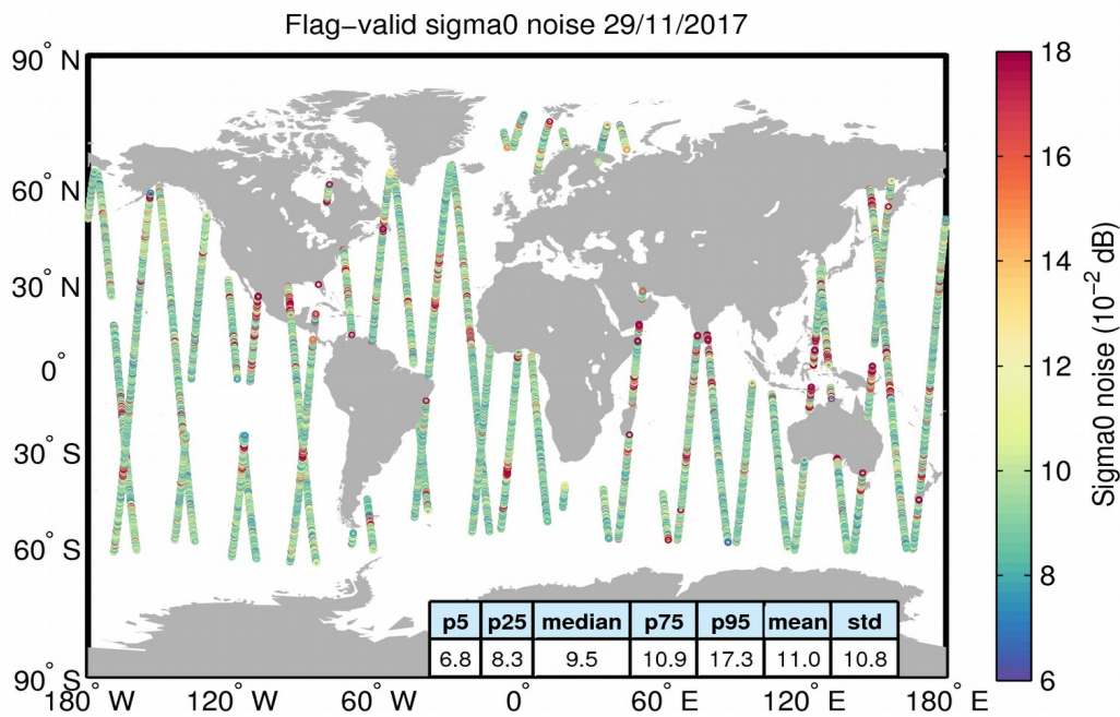
Figure 26. Geographical distribution of flag-valid 20-Hz sigma0 measurement noise over oceans and lakes for 29/11/2017. The statistical values shown in the table refer to the sigma0 noise and are calculated over all measurements shown in the figure.
