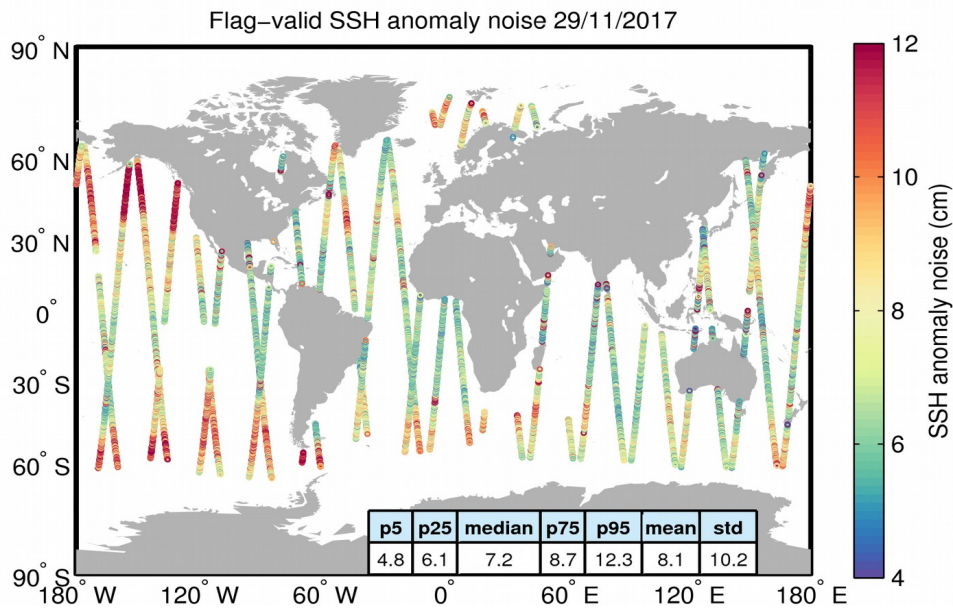
Figure 8. Geographical distribution of flag-valid 20-Hz SSH anomaly measurement noise over oceans and lakes for 29/11/2017. The statistical values shown in the table refer to the SSH anomaly noise and are calculated over all measurements shown in the figure.
