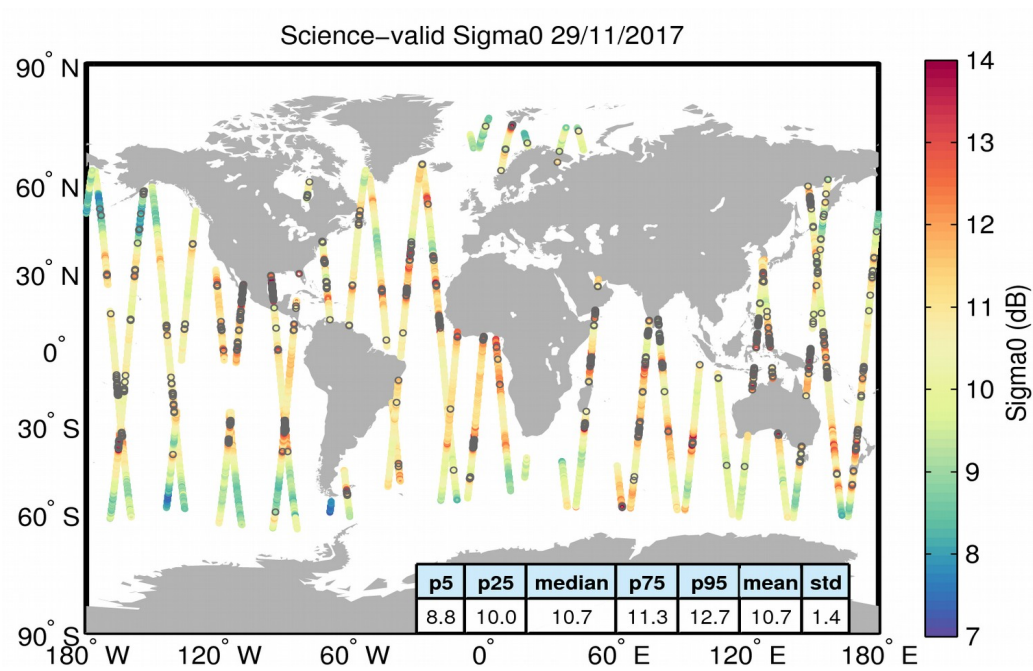
Figure 27. Geographical distribution of science-valid sigma0 data over oceans and lakes for 29/11/2017. The statistical values shown in the table refer to the sigma0 in dB and are calculated over all measurements shown in the figure. Gray circles denote records that have been rejected based on the editing criteria described in Table 4.
