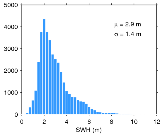
Figure 17. Histogram of flag-valid SWH over oceans and lakes for 29/11/2017. The mean ( \mu ) and standard deviation ( \sigma ) are also shown. Note that values larger than 12 m are excluded from the histogram for the sake of readability but not from the computation of \mu and \sigma .
