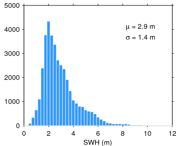
Figure 20. Histogram of science-valid SWH over oceans and lakes for 29/11/2017. The mean ( \mu ) and standard deviation ( \sigma ) are also shown. Note that values larger than 12 m are excluded from the histogram for the sake of readability but not from the computation of \mu and \sigma .
