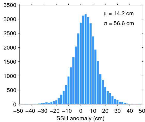
Figure 7. Histogram of flag-valid SSH anomaly over oceans and lakes for 29/11/2017. The mean ( \mu ) and standard deviation ( \sigma ) are also shown. Note that values outside [-50 50] cm are excluded from the histogram for the sake of readability but not from the computation of \mu and \sigma .
