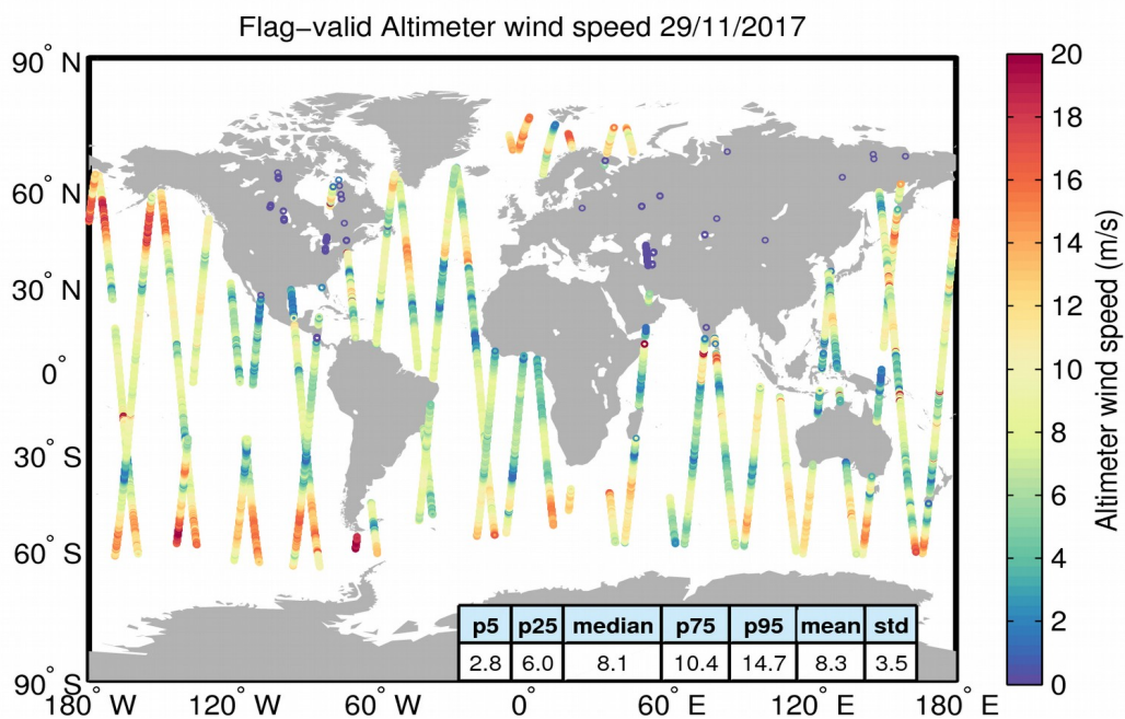
Figure 31. Geographical distribution of flag-valid wind data over oceans and lakes for 29/11/2017. The statistical values shown in the table refer to the wind in m/s and are calculated over all measurements shown in the figure.
