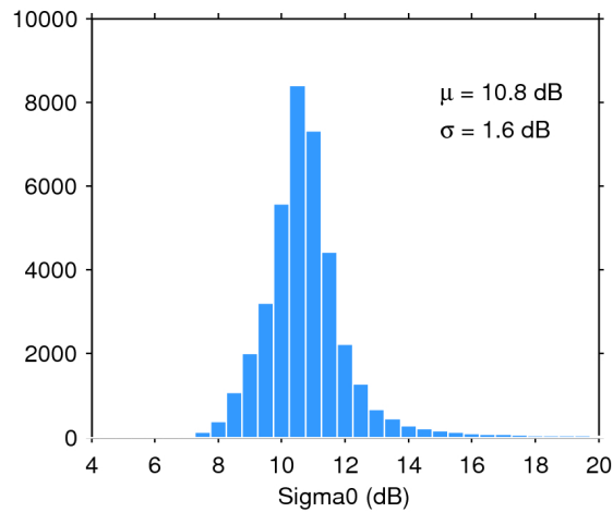
Figure 25. Histogram of flag-valid sigma0 over oceans and lakes for 29/11/2017. The mean ( \mu ) and standard deviation ( \sigma ) are also shown. Note that values outside [4 20] dB are excluded from the histogram for the sake of readability but not from the computation of \mu and \sigma .
