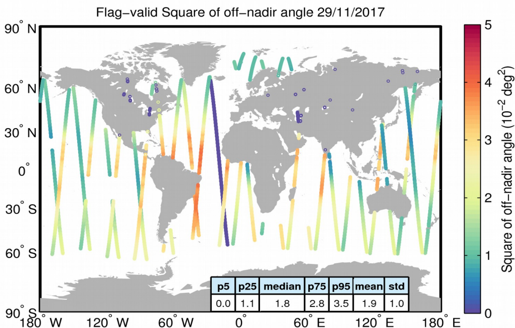
Figure 37. Geographical distribution of flag-valid mispointing data over oceans and lakes for 29/11/2017. The statistical values shown in the table refer to the mispointing in 10^{-2} deg 2 and are calculated over all measurements shown in the figure.
