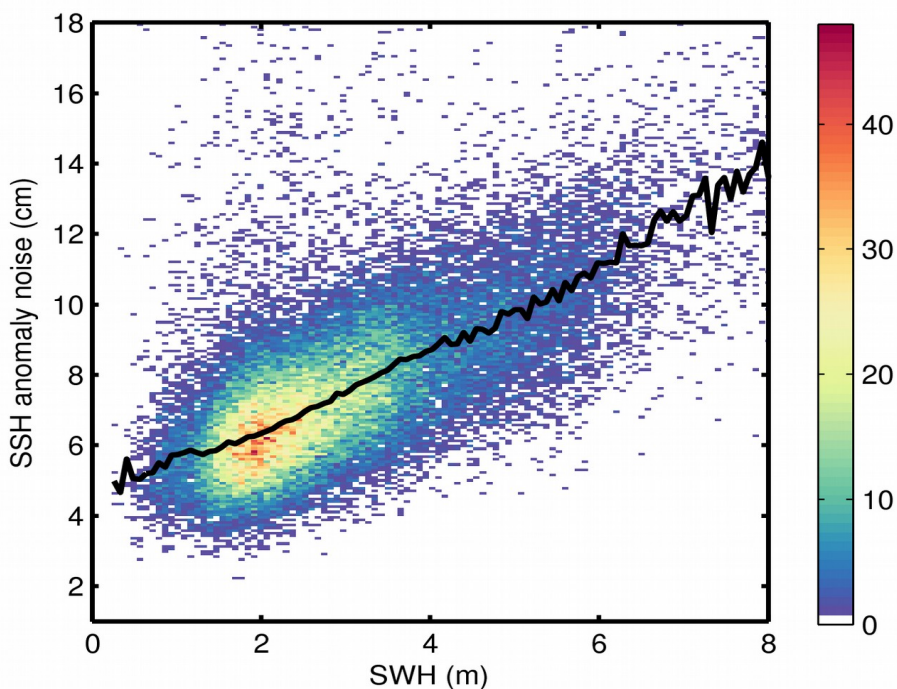
Figure 9. 2D histogram showing flag-valid SSH anomaly noise as a function of SWH for 29/11/2017. The black line denotes the median SSH anomaly noise as a function of SWH.
