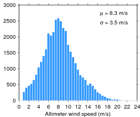
Figure 35. Histogram of science-valid wind over oceans and lakes for 29/11/2017. The mean ( \mu ) and standard deviation ( \sigma ) are also shown. Note that values larger than 24 m/s are excluded from the histogram for the sake of readability but not from the computation of \mu and \sigma .
