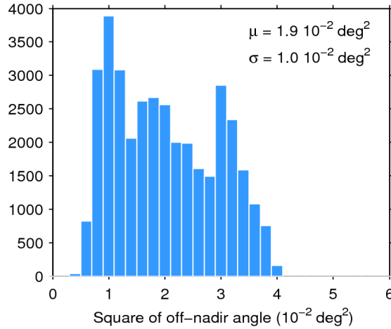
Figure 39. Histogram of flag-valid mispointing over oceans and lakes for 29/11/2017. The mean ( \mu ) and standard deviation ( \sigma ) are also shown. Note that values larger than 6 \cdot 10^{-2} \text{ deg}^2 are excluded from the histogram for the sake of readability but not from the computation of \mu and \sigma .
