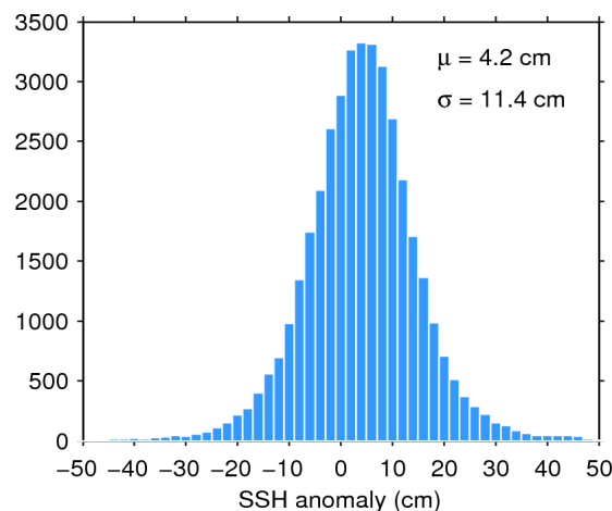
Figure 11. Histogram of science-valid SSH anomaly over oceans and lakes for 28/11/2017. The mean ( \mu ) and standard deviation ( \sigma ) are also shown. Note that values outside [-50 50] cm are excluded from the histogram for the sake of readability but not from the computation of \mu and \sigma .
