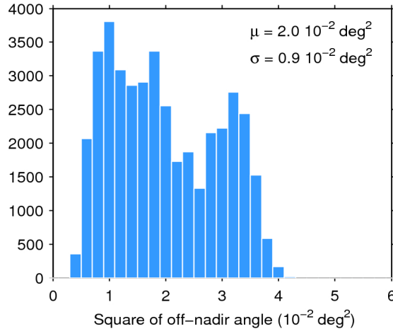
Figure 39. Histogram of flag-valid mispointing over oceans and lakes for 28/11/2017. The mean ( \mu ) and standard deviation ( \sigma ) are also shown. Note that values larger than 6 \cdot 10^{-2} \text{ deg}^2 are excluded from the histogram for the sake of readability but not from the computation of \mu and \sigma .
