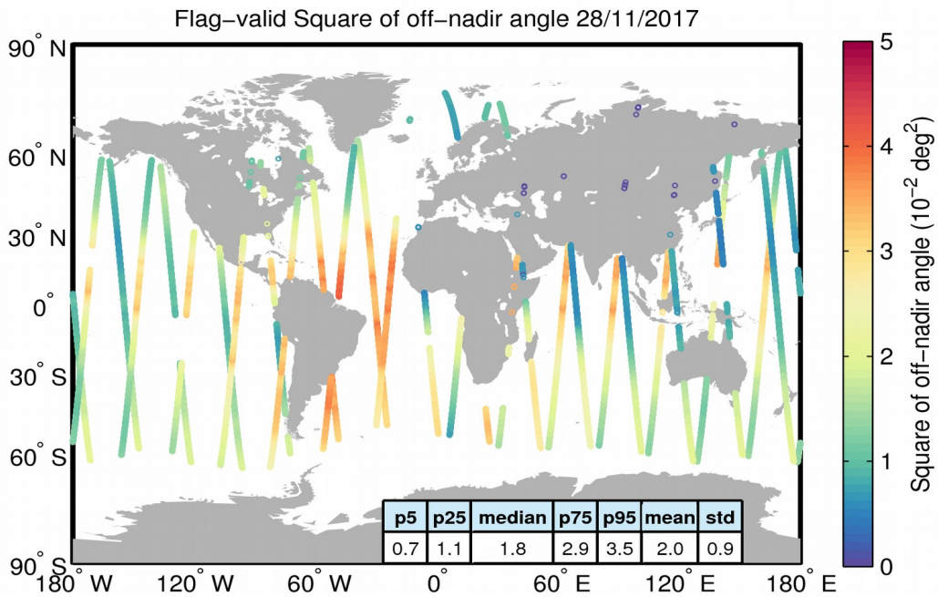
Figure 37. Geographical distribution of flag-valid mispointing data over oceans and lakes for 28/11/2017. The statistical values shown in the table refer to the mispointing in 10^{-2} deg 2 and are calculated over all measurements shown in the figure.
