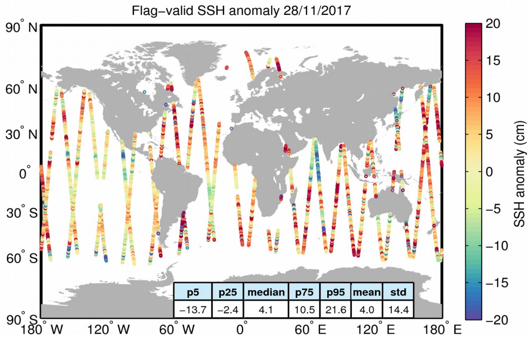
Figure 5. Geographical distribution of flag-valid 1-Hz SSH anomaly data over oceans and lakes for 28/11/2017. The statistical values shown in the table refer to the SSH anomaly in cm and are calculated over all measurements shown in the figure.
