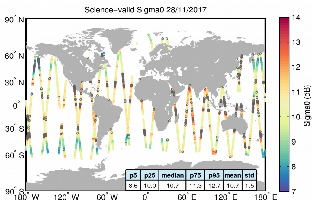
Figure 27. Geographical distribution of science-valid sigma0 data over oceans and lakes for 28/11/2017. The statistical values shown in the table refer to the sigma0 in dB and are calculated over all measurements shown in the figure. Gray circles denote records that have been rejected based on the editing criteria described in Table 4.
