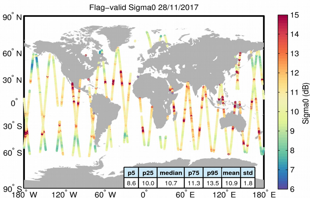
Figure 23. Geographical distribution of flag-valid sigma0 data over oceans and lakes for 28/11/2017. The statistical values shown in the table refer to the sigma0 in dB and are calculated over all measurements shown in the figure.
