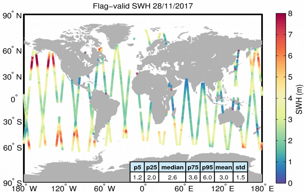
Figure 15. Geographical distribution of flag-valid SWH data over oceans and lakes for 28/11/2017. The statistical values shown in the table refer to the SWH in m and are calculated over all measurements shown in the figure.
