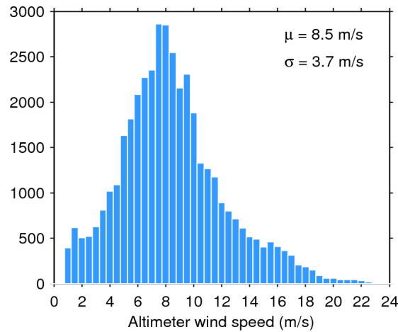
Figure 33. Histogram of flag-valid wind over oceans and lakes for 28/11/2017. The mean ( \mu ) and standard deviation ( \sigma ) are also shown. Note that values larger than 24 m/s are excluded from the histogram for the sake of readability but not from the computation of \mu and \sigma .
