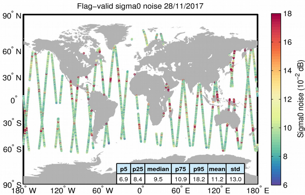
Figure 26. Geographical distribution of flag-valid 20-Hz sigma0 measurement noise over oceans and lakes for 28/11/2017. The statistical values shown in the table refer to the sigma0 noise and are calculated over all measurements shown in the figure.
