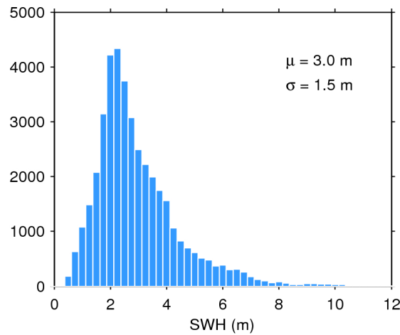
Figure 17. Histogram of flag-valid SWH over oceans and lakes for 28/11/2017. The mean ( \mu ) and standard deviation ( \sigma ) are also shown. Note that values larger than 12 m are excluded from the histogram for the sake of readability but not from the computation of \mu and \sigma .
