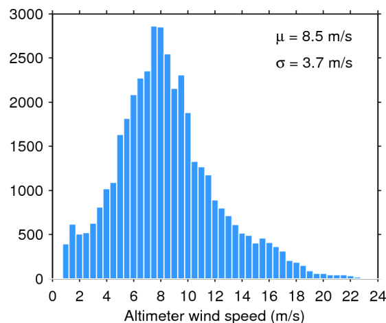
Figure 35. Histogram of science-valid wind over oceans and lakes for 28/11/2017. The mean ( \mu ) and standard deviation ( \sigma ) are also shown. Note that values larger than 24 m/s are excluded from the histogram for the sake of readability but not from the computation of \mu and \sigma .
