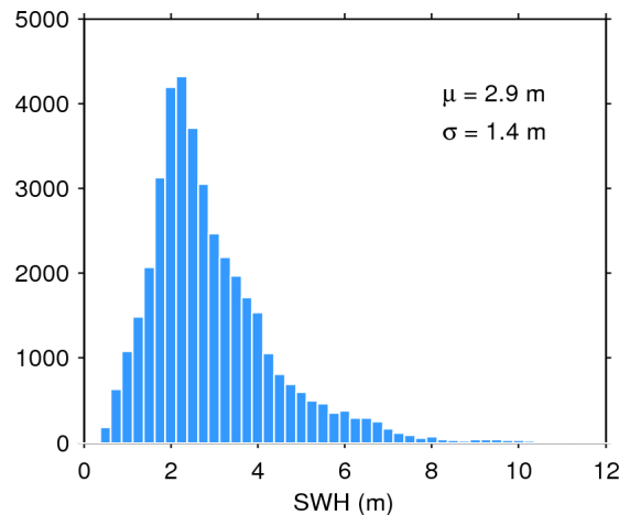
Figure 20. Histogram of science-valid SWH over oceans and lakes for 28/11/2017. The mean ( \mu ) and standard deviation ( \sigma ) are also shown. Note that values larger than 12 m are excluded from the histogram for the sake of readability but not from the computation of \mu and \sigma .
