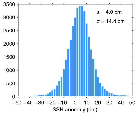
Figure 7. Histogram of flag-valid SSH anomaly over oceans and lakes for 28/11/2017. The mean ( \mu ) and standard deviation ( \sigma ) are also shown. Note that values outside [-50\ 50] cm are excluded from the histogram for the sake of readability but not from the computation of \mu and \sigma .
