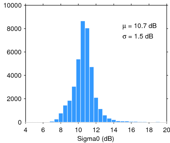
Figure 28. Histogram of science-valid sigma0 over oceans and lakes for 28/11/2017. The mean ( \mu ) and standard deviation ( \sigma ) are also shown. Note that values outside [4 20] dB are excluded from the histogram for the sake of readability but not from the computation of \mu and \sigma .
