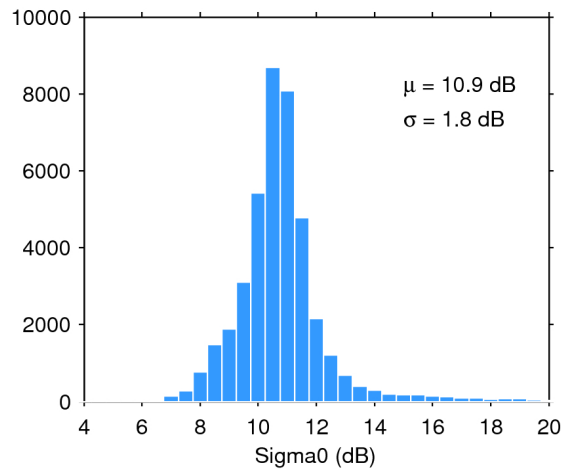
Figure 25. Histogram of flag-valid sigma0 over oceans and lakes for 28/11/2017. The mean ( \mu ) and standard deviation ( \sigma ) are also shown. Note that values outside [4 20] dB are excluded from the histogram for the sake of readability but not from the computation of \mu and \sigma .
