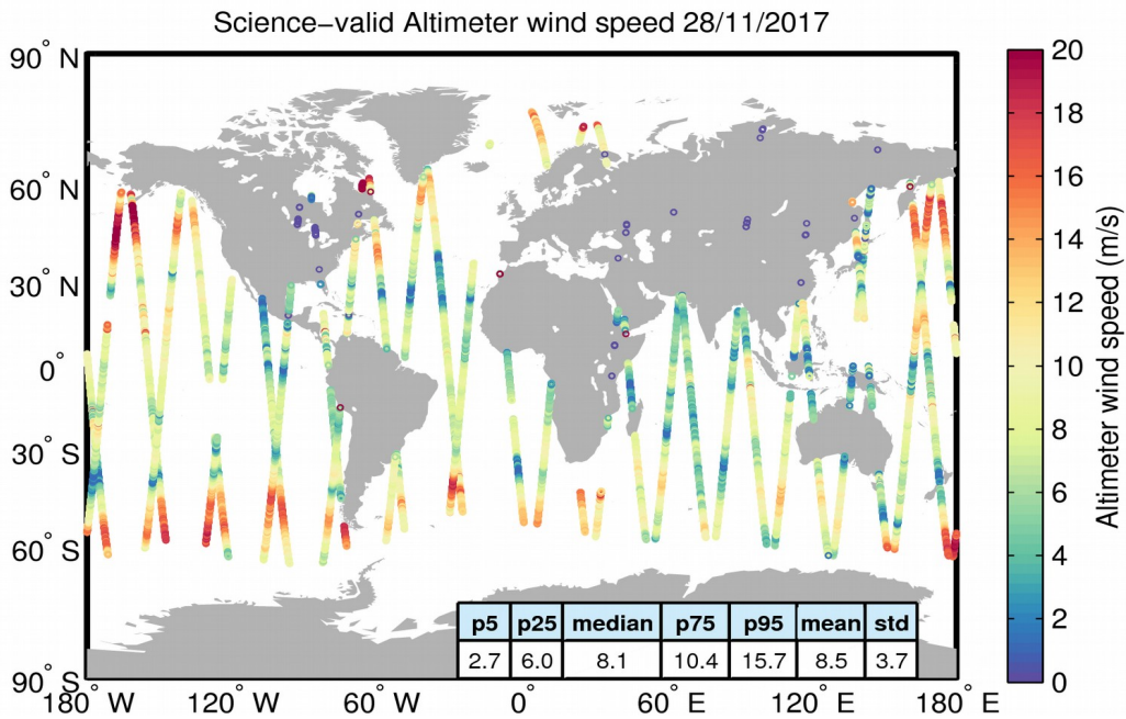
Figure 34. Geographical distribution of science-valid wind data over oceans and lakes for 28/11/2017. The statistical values shown in the table refer to the wind in m/s and are calculated over all measurements shown in the figure. Gray circles denote records that have been rejected based on the editing criteria described in Table 5.
