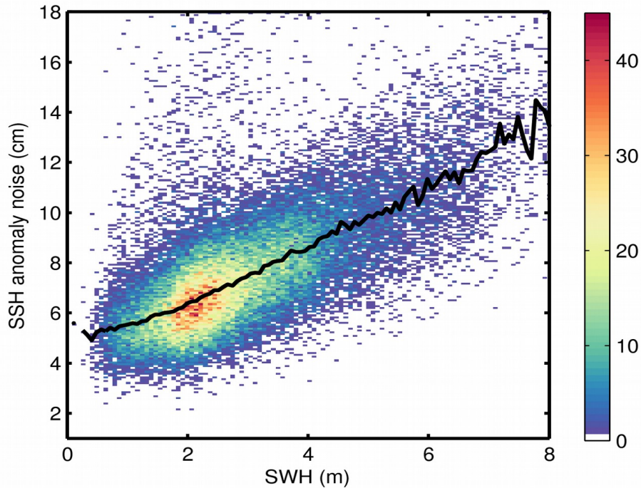
Figure 9. 2D histogram showing flag-valid SSH anomaly noise as a function of SWH for 28/11/2017. The black line denotes the median SSH anomaly noise as a function of SWH.
