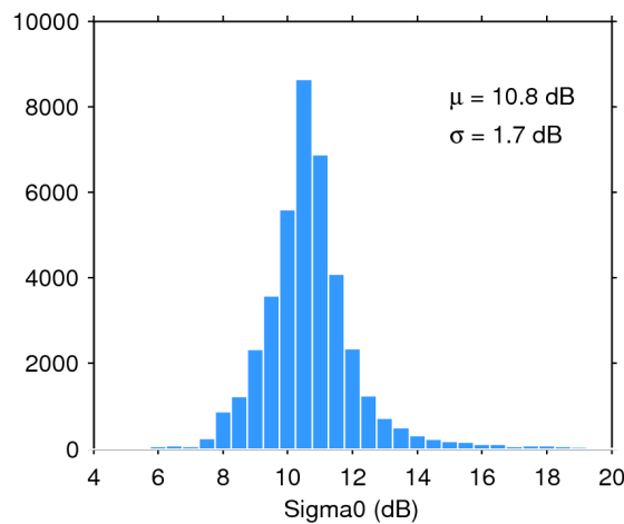
Figure 25. Histogram of flag-valid sigma0 over oceans and lakes for 27/11/2017. The mean ( \mu ) and standard deviation ( \sigma ) are also shown. Note that values outside [4 20] dB are excluded from the histogram for the sake of readability but not from the computation of \mu and \sigma .
