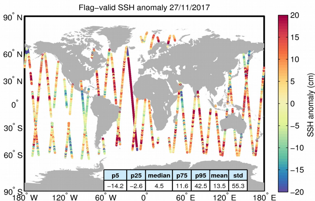
Figure 5. Geographical distribution of flag-valid 1-Hz SSH anomaly data over oceans and lakes for 27/11/2017. The statistical values shown in the table refer to the SSH anomaly in cm and are calculated over all measurements shown in the figure.
