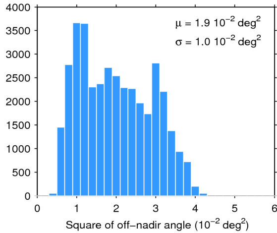
Figure 39. Histogram of flag-valid mispointing over oceans and lakes for 27/11/2017. The mean ( \mu ) and standard deviation ( \sigma ) are also shown. Note that values larger than 6 \cdot 10^{-2} \text{ deg}^2 are excluded from the histogram for the sake of readability but not from the computation of \mu and \sigma .
