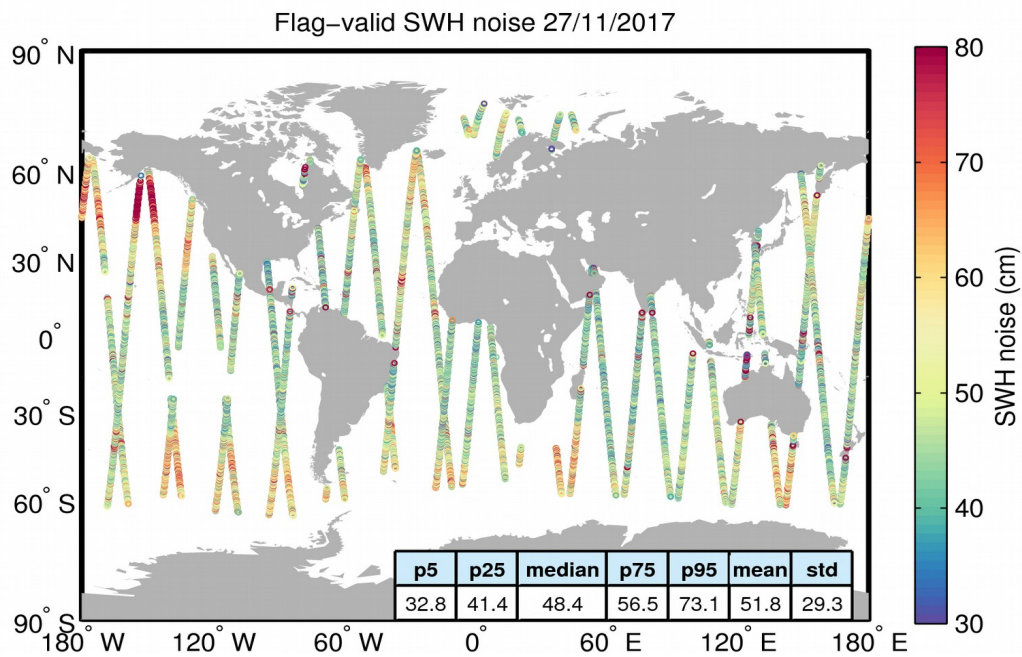
Figure 18. Geographical distribution of flag-valid 20-Hz SWH measurement noise over oceans and lakes for 27/11/2017. The statistical values shown in the table refer to the SWH noise and are calculated over all measurements shown in the figure.
