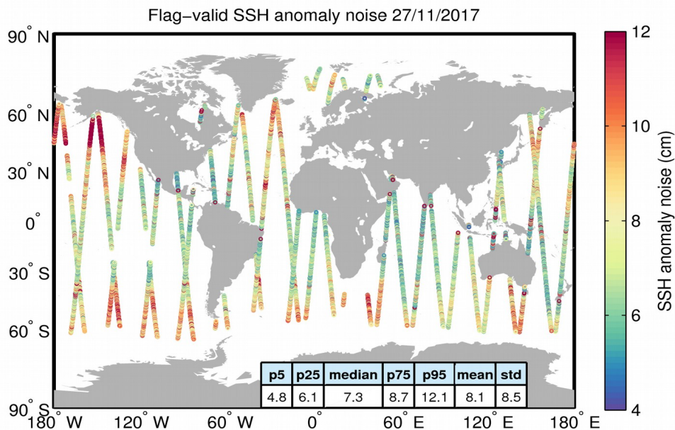
Figure 8. Geographical distribution of flag-valid 20-Hz SSH anomaly measurement noise over oceans and lakes for 27/11/2017. The statistical values shown in the table refer to the SSH anomaly noise and are calculated over all measurements shown in the figure.
