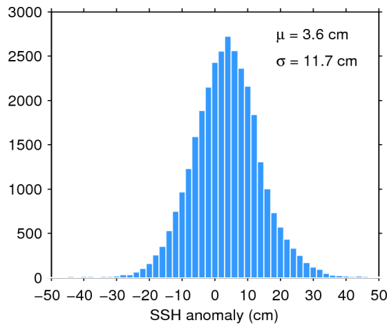
Figure 11. Histogram of science-valid SSH anomaly over oceans and lakes for 27/11/2017. The mean ( \mu ) and standard deviation ( \sigma ) are also shown. Note that values outside [-50 50] cm are excluded from the histogram for the sake of readability but not from the computation of \mu and \sigma .
