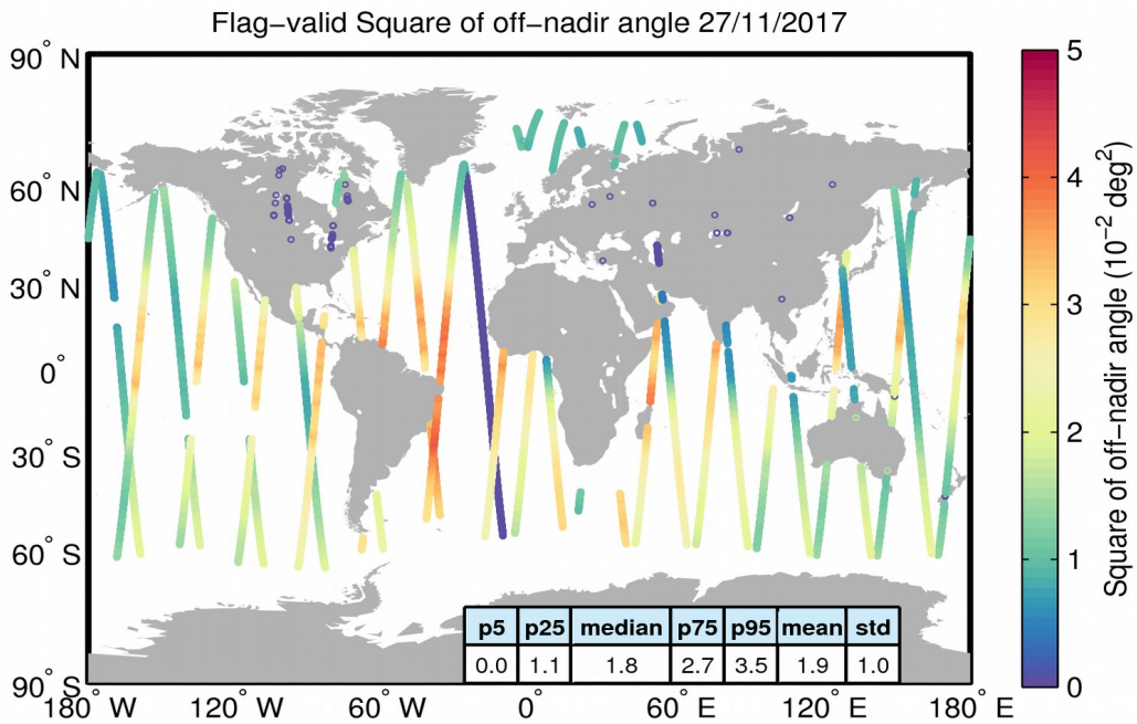
Figure 37. Geographical distribution of flag-valid mispointing data over oceans and lakes for 27/11/2017. The statistical values shown in the table refer to the mispointing in 10^{-2} \text{deg}^2 and are calculated over all measurements shown in the figure.
