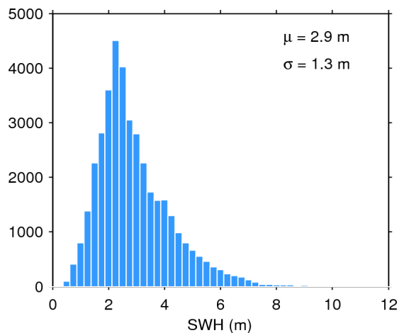
Figure 20. Histogram of science-valid SWH over oceans and lakes for 27/11/2017. The mean ( \mu ) and standard deviation ( \sigma ) are also shown. Note that values larger than 12 m are excluded from the histogram for the sake of readability but not from the computation of \mu and \sigma .
