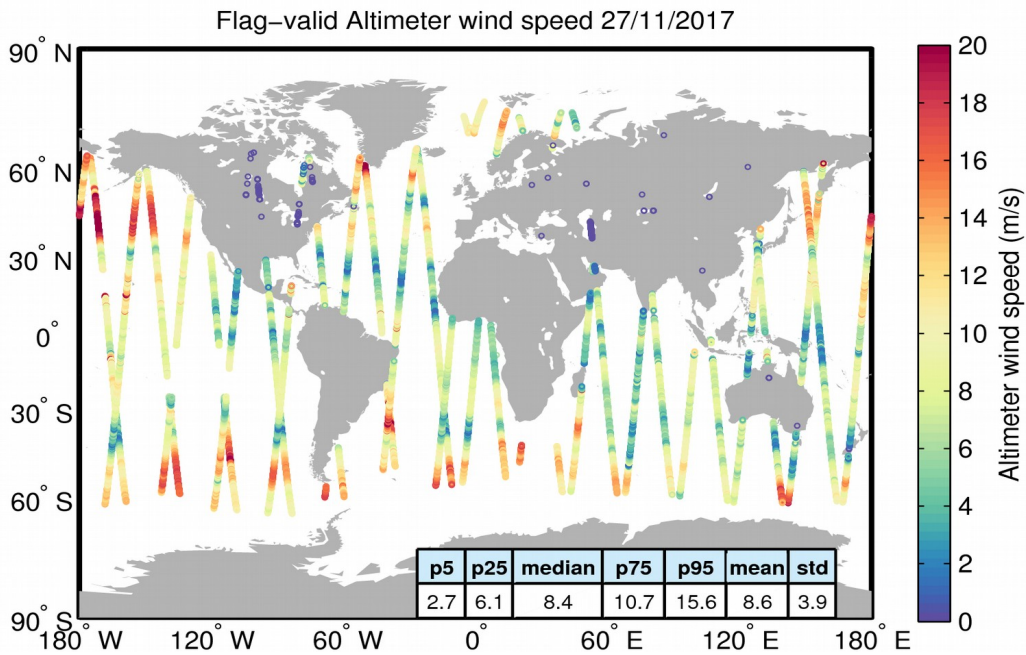
Figure 31. Geographical distribution of flag-valid wind data over oceans and lakes for 27/11/2017. The statistical values shown in the table refer to the wind in m/s and are calculated over all measurements shown in the figure.
