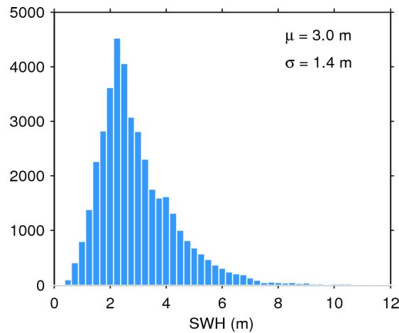
Figure 17. Histogram of flag-valid SWH over oceans and lakes for 27/11/2017. The mean ( \mu ) and standard deviation ( \sigma ) are also shown. Note that values larger than 12 m are excluded from the histogram for the sake of readability but not from the computation of \mu and \sigma .
