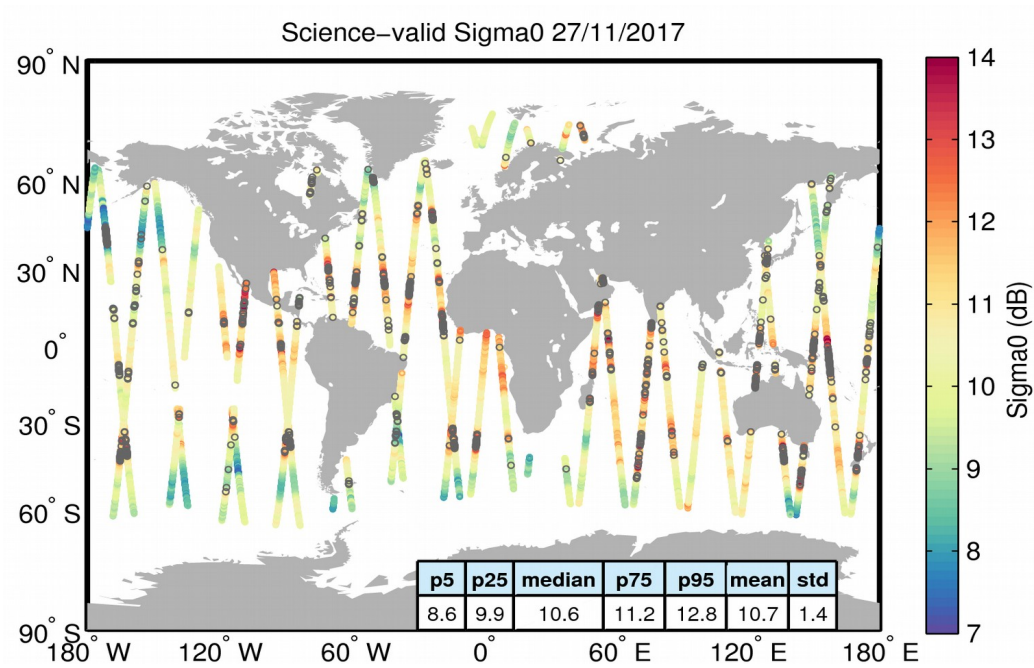
Figure 27. Geographical distribution of science-valid sigma0 data over oceans and lakes for 27/11/2017. The statistical values shown in the table refer to the sigma0 in dB and are calculated over all measurements shown in the figure. Gray circles denote records that have been rejected based on the editing criteria described in Table 4.
