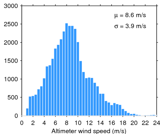
Figure 35. Histogram of science-valid wind over oceans and lakes for 27/11/2017. The mean ( \mu ) and standard deviation ( \sigma ) are also shown. Note that values larger than 24 m/s are excluded from the histogram for the sake of readability but not from the computation of \mu and \sigma .
