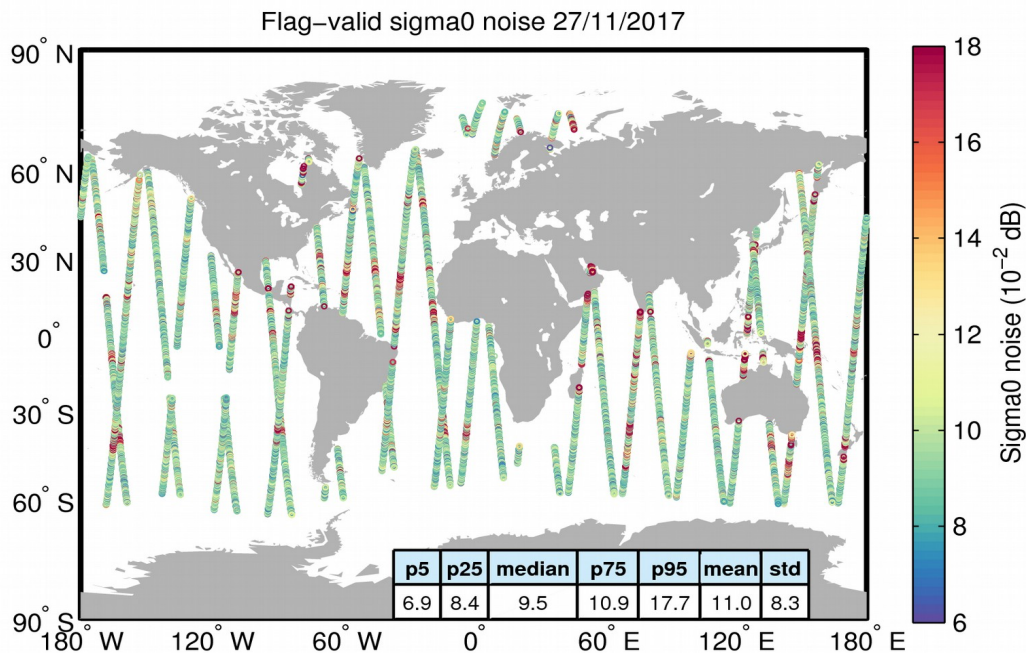
Figure 26. Geographical distribution of flag-valid 20-Hz sigma0 measurement noise over oceans and lakes for 27/11/2017. The statistical values shown in the table refer to the sigma0 noise and are calculated over all measurements shown in the figure.
