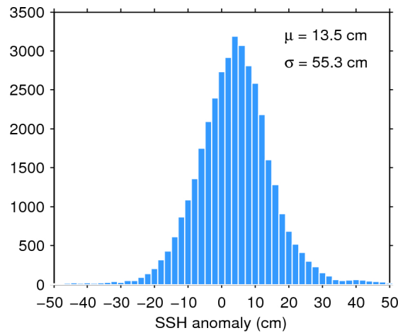
Figure 7. Histogram of flag-valid SSH anomaly over oceans and lakes for 27/11/2017. The mean ( \mu ) and standard deviation ( \sigma ) are also shown. Note that values outside [-50 50] cm are excluded from the histogram for the sake of readability but not from the computation of \mu and \sigma .
