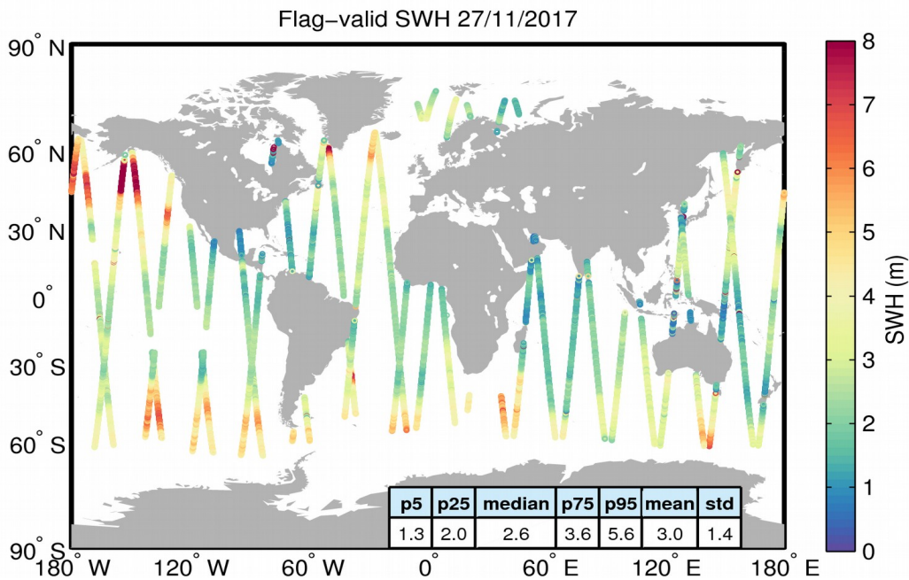
Figure 15. Geographical distribution of flag-valid SWH data over oceans and lakes for 27/11/2017. The statistical values shown in the table refer to the SWH in m and are calculated over all measurements shown in the figure.
