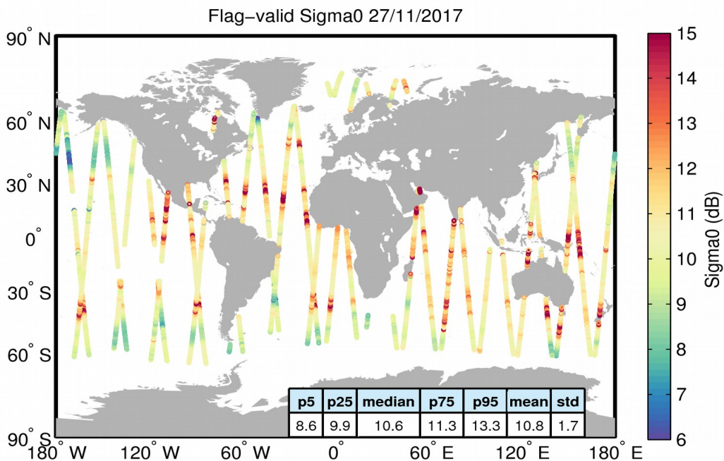
Figure 23. Geographical distribution of flag-valid sigma0 data over oceans and lakes for 27/11/2017. The statistical values shown in the table refer to the sigma0 in dB and are calculated over all measurements shown in the figure.
