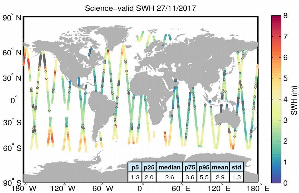
Figure 19. Geographical distribution of science-valid SWH data over oceans and lakes for 27/11/2017. The statistical values shown in the table refer to the SWH in m and are calculated over all measurements shown in the figure. Gray circles denote records that have been rejected based on the editing criteria described in Table 3.
