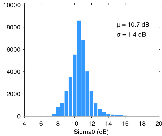
Figure 28. Histogram of science-valid sigma0 over oceans and lakes for 27/11/2017. The mean ( \mu ) and standard deviation ( \sigma ) are also shown. Note that values outside [4 20] dB are excluded from the histogram for the sake of readability but not from the computation of \mu and \sigma .
