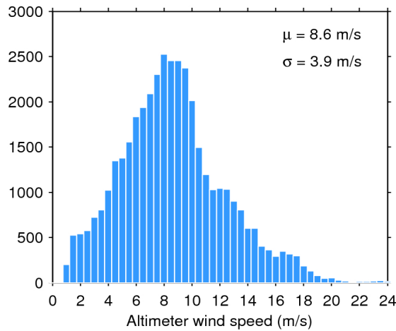
Figure 33. Histogram of flag-valid wind over oceans and lakes for 27/11/2017. The mean ( \mu ) and standard deviation ( \sigma ) are also shown. Note that values larger than 24 m/s are excluded from the histogram for the sake of readability but not from the computation of \mu and \sigma .
