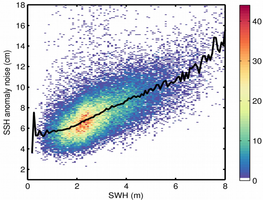
Figure 9. 2D histogram showing flag-valid SSH anomaly noise as a function of SWH for 27/11/2017. The black line denotes the median SSH anomaly noise as a function of SWH.
