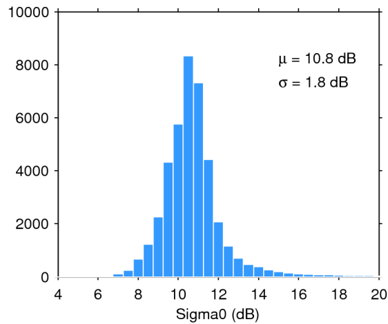
Figure 25. Histogram of flag-valid sigma0 over oceans and lakes for 26/11/2017. The mean ( \mu ) and standard deviation ( \sigma ) are also shown. Note that values outside [4 20] dB are excluded from the histogram for the sake of readability but not from the computation of \mu and \sigma .
