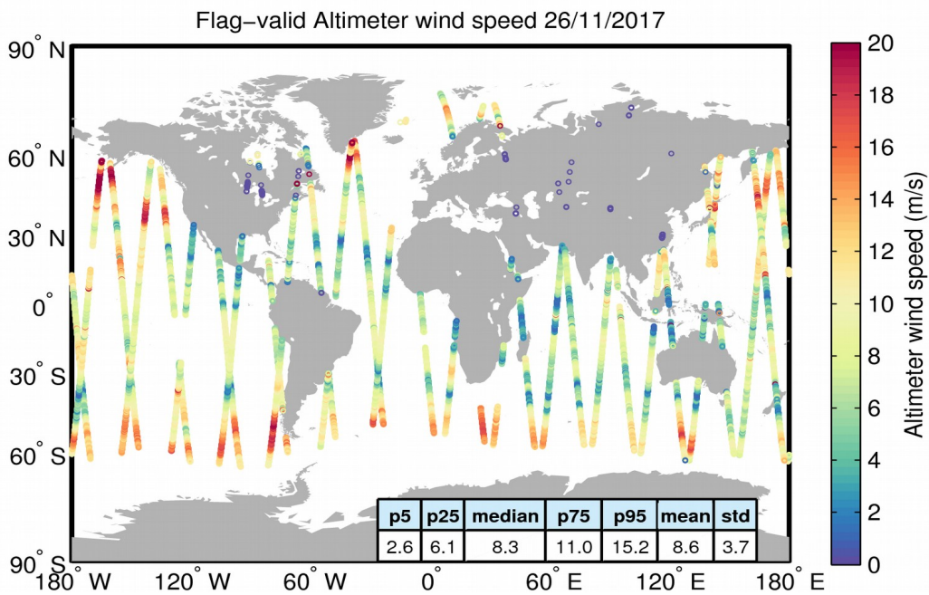
Figure 31. Geographical distribution of flag-valid wind data over oceans and lakes for 26/11/2017. The statistical values shown in the table refer to the wind in m/s and are calculated over all measurements shown in the figure.
