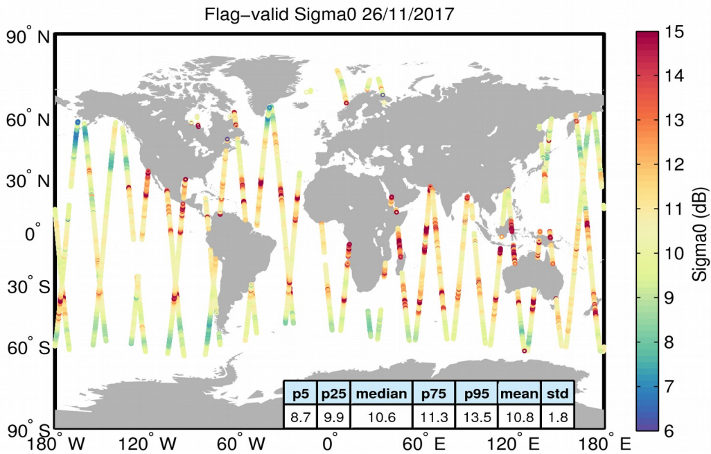
Figure 23. Geographical distribution of flag-valid sigma0 data over oceans and lakes for 26/11/2017. The statistical values shown in the table refer to the sigma0 in dB and are calculated over all measurements shown in the figure.
