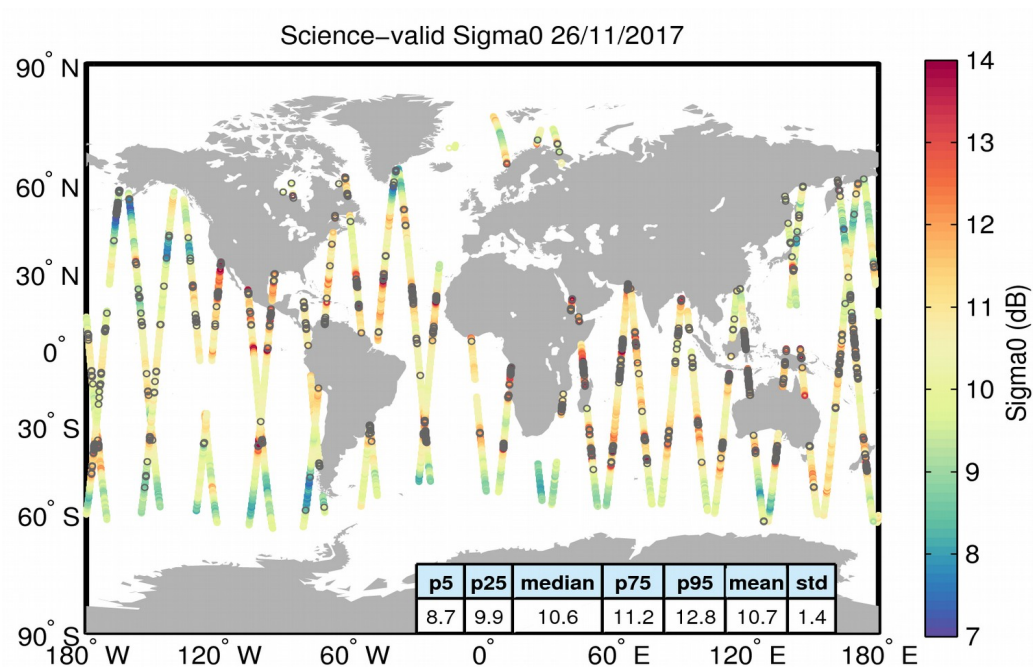
Figure 27. Geographical distribution of science-valid sigma0 data over oceans and lakes for 26/11/2017. The statistical values shown in the table refer to the sigma0 in dB and are calculated over all measurements shown in the figure. Gray circles denote records that have been rejected based on the editing criteria described in Table 4.
