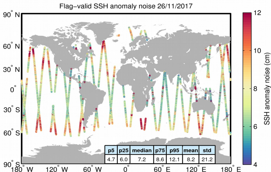
Figure 8. Geographical distribution of flag-valid 20-Hz SSH anomaly measurement noise over oceans and lakes for 26/11/2017. The statistical values shown in the table refer to the SSH anomaly noise and are calculated over all measurements shown in the figure.
