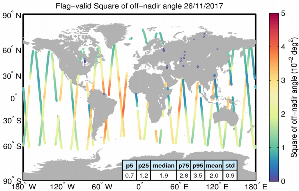
Figure 37. Geographical distribution of flag-valid mispointing data over oceans and lakes for 26/11/2017. The statistical values shown in the table refer to the mispointing in 10^{-2} deg 2 and are calculated over all measurements shown in the figure.
