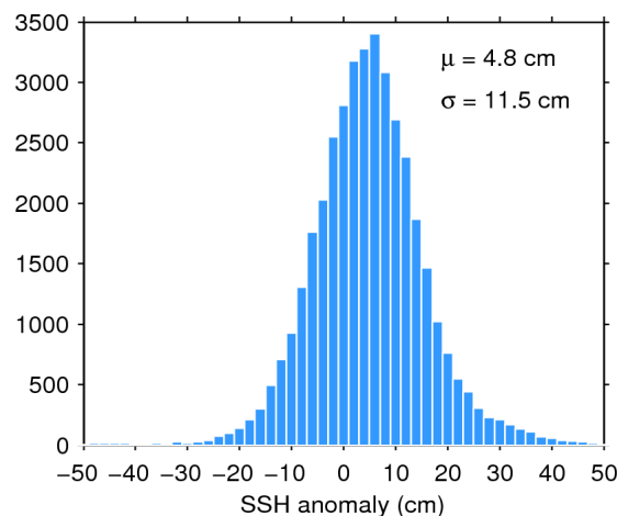
Figure 11. Histogram of science-valid SSH anomaly over oceans and lakes for 26/11/2017. The mean ( \mu ) and standard deviation ( \sigma ) are also shown. Note that values outside [-50 50] cm are excluded from the histogram for the sake of readability but not from the computation of \mu and \sigma .
