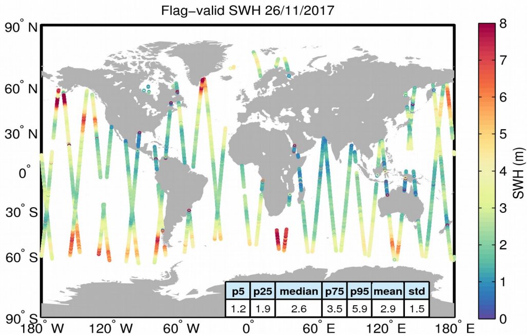
Figure 15. Geographical distribution of flag-valid SWH data over oceans and lakes for 26/11/2017. The statistical values shown in the table refer to the SWH in m and are calculated over all measurements shown in the figure.
