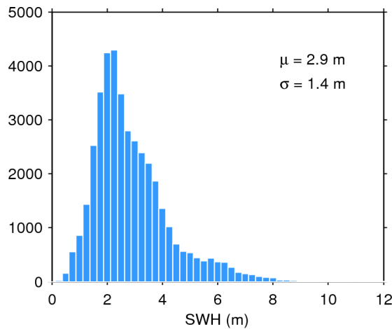
Figure 20. Histogram of science-valid SWH over oceans and lakes for 26/11/2017. The mean ( \mu ) and standard deviation ( \sigma ) are also shown. Note that values larger than 12 m are excluded from the histogram for the sake of readability but not from the computation of \mu and \sigma .
