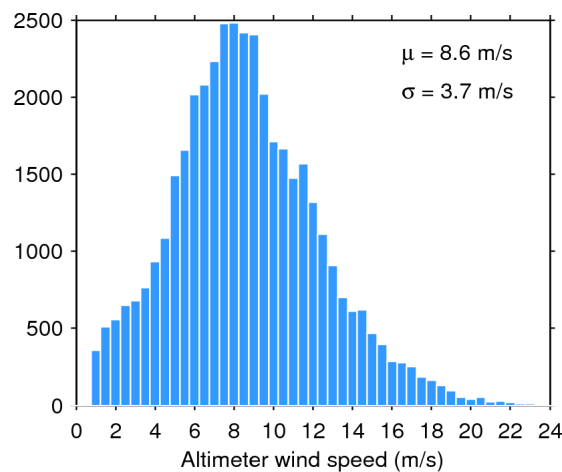
Figure 35. Histogram of science-valid wind over oceans and lakes for 26/11/2017. The mean ( \mu ) and standard deviation ( \sigma ) are also shown. Note that values larger than 24 m/s are excluded from the histogram for the sake of readability but not from the computation of \mu and \sigma .
