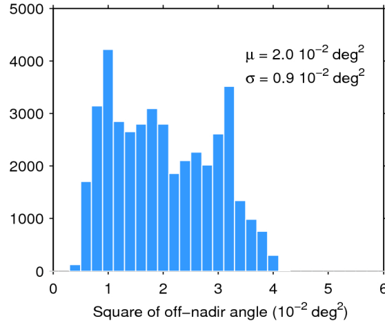
Figure 39. Histogram of flag-valid mispointing over oceans and lakes for 26/11/2017. The mean ( \mu ) and standard deviation ( \sigma ) are also shown. Note that values larger than 6 \cdot 10^{-2} \text{ deg}^2 are excluded from the histogram for the sake of readability but not from the computation of \mu and \sigma .
