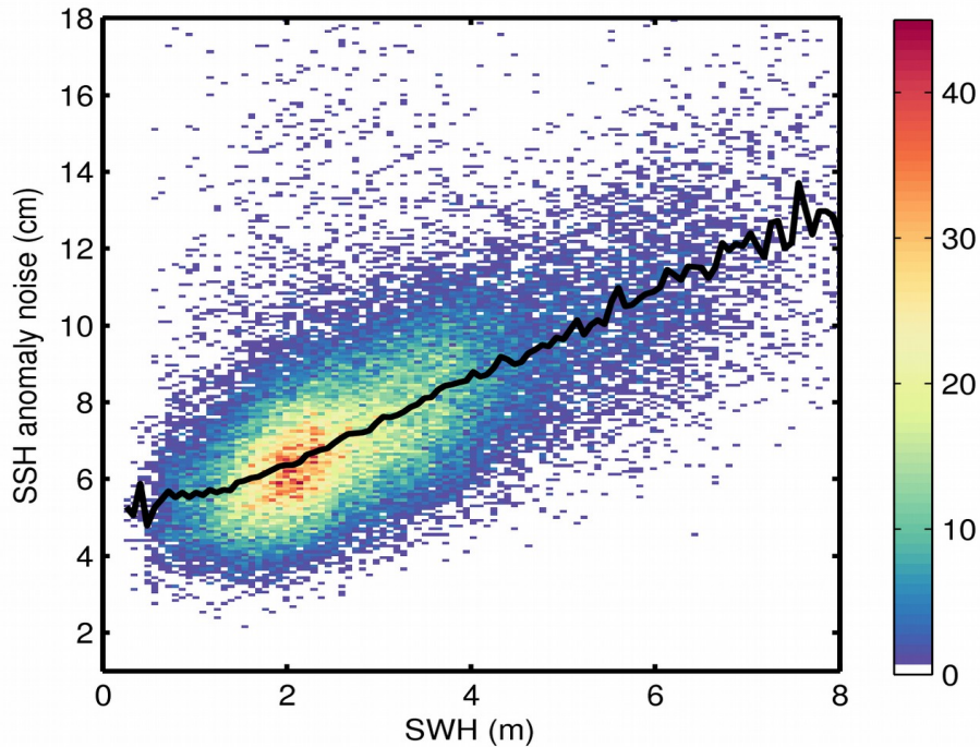
Figure 9. 2D histogram showing flag-valid SSH anomaly noise as a function of SWH for 26/11/2017. The black line denotes the median SSH anomaly noise as a function of SWH.
