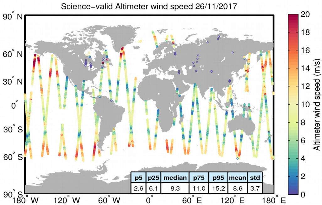
Figure 34. Geographical distribution of science-valid wind data over oceans and lakes for 26/11/2017. The statistical values shown in the table refer to the wind in m/s and are calculated over all measurements shown in the figure. Gray circles denote records that have been rejected based on the editing criteria described in Table 5.
