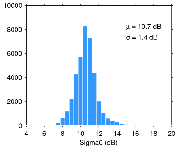
Figure 28. Histogram of science-valid sigma0 over oceans and lakes for 26/11/2017. The mean ( \mu ) and standard deviation ( \sigma ) are also shown. Note that values outside [4 20] dB are excluded from the histogram for the sake of readability but not from the computation of \mu and \sigma .
