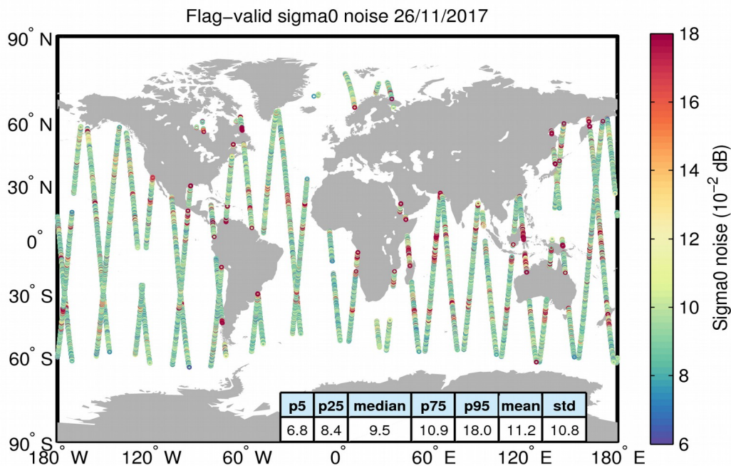
Figure 26. Geographical distribution of flag-valid 20-Hz sigma0 measurement noise over oceans and lakes for 26/11/2017. The statistical values shown in the table refer to the sigma0 noise and are calculated over all measurements shown in the figure.
