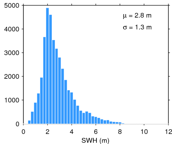
Figure 20. Histogram of science-valid SWH over oceans and lakes for 24/11/2017. The mean ( \mu ) and standard deviation ( \sigma ) are also shown. Note that values larger than 12 m are excluded from the histogram for the sake of readability but not from the computation of \mu and \sigma .
