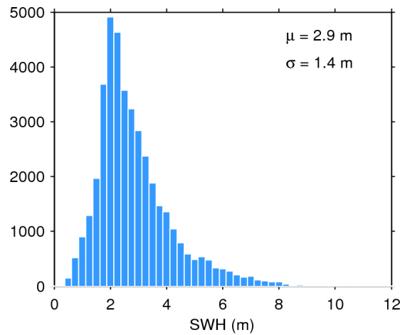
Figure 17. Histogram of flag-valid SWH over oceans and lakes for 24/11/2017. The mean ( \mu ) and standard deviation ( \sigma ) are also shown. Note that values larger than 12 m are excluded from the histogram for the sake of readability but not from the computation of \mu and \sigma .
