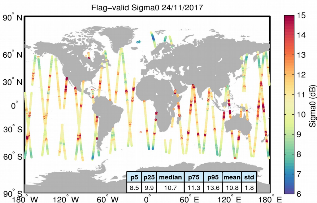
Figure 23. Geographical distribution of flag-valid sigma0 data over oceans and lakes for 24/11/2017. The statistical values shown in the table refer to the sigma0 in dB and are calculated over all measurements shown in the figure.
