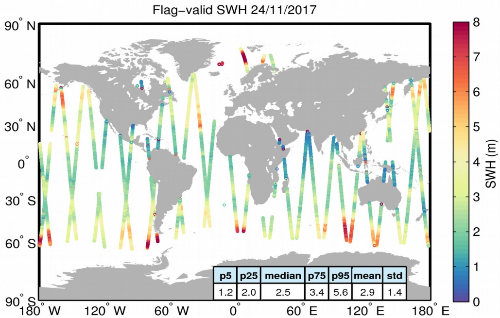
Figure 15. Geographical distribution of flag-valid SWH data over oceans and lakes for 24/11/2017. The statistical values shown in the table refer to the SWH in m and are calculated over all measurements shown in the figure.
