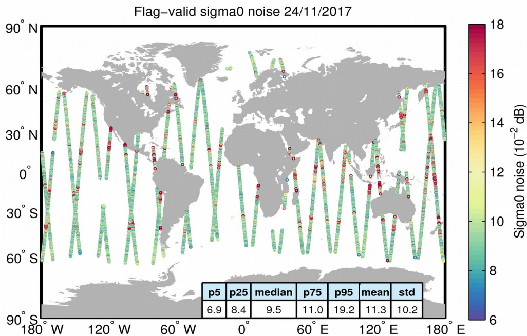
Figure 26. Geographical distribution of flag-valid 20-Hz sigma0 measurement noise over oceans and lakes for 24/11/2017. The statistical values shown in the table refer to the sigma0 noise and are calculated over all measurements shown in the figure.
