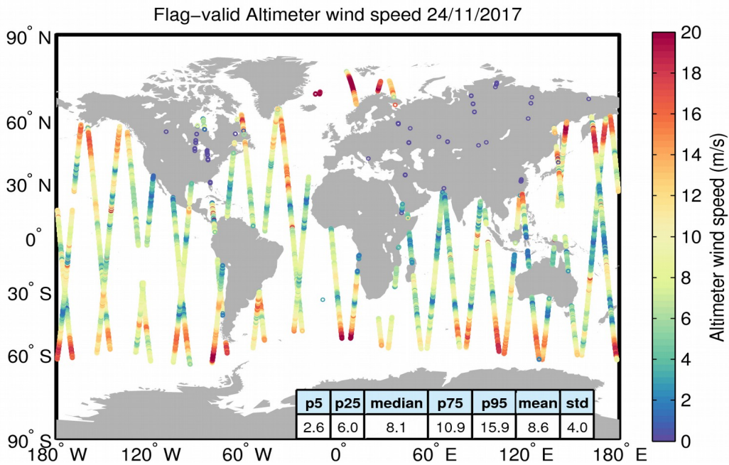
Figure 31. Geographical distribution of flag-valid wind data over oceans and lakes for 24/11/2017. The statistical values shown in the table refer to the wind in m/s and are calculated over all measurements shown in the figure.
