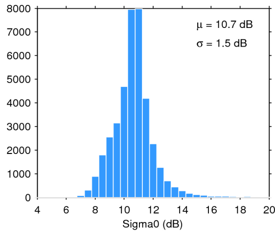
Figure 28. Histogram of science-valid sigma0 over oceans and lakes for 24/11/2017. The mean ( \mu ) and standard deviation ( \sigma ) are also shown. Note that values outside [4 20] dB are excluded from the histogram for the sake of readability but not from the computation of \mu and \sigma .
