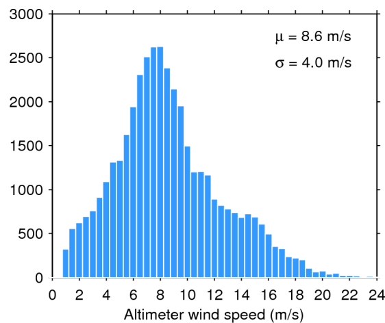
Figure 35. Histogram of science-valid wind over oceans and lakes for 24/11/2017. The mean ( \mu ) and standard deviation ( \sigma ) are also shown. Note that values larger than 24 m/s are excluded from the histogram for the sake of readability but not from the computation of \mu and \sigma .
