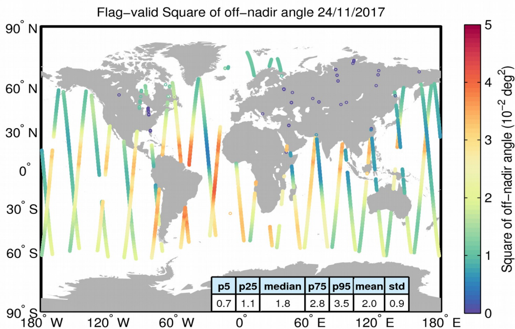
Figure 37. Geographical distribution of flag-valid mispointing data over oceans and lakes for 24/11/2017. The statistical values shown in the table refer to the mispointing in 10^{-2} deg 2 and are calculated over all measurements shown in the figure.
