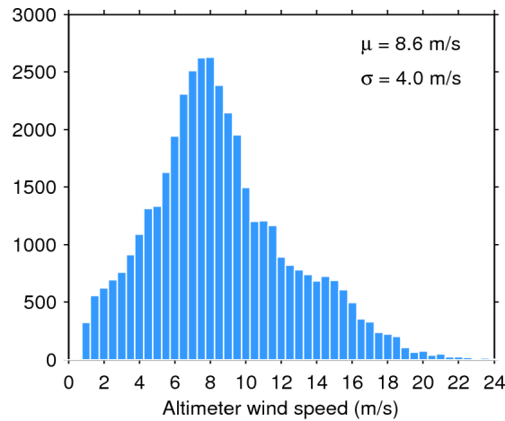
Figure 33. Histogram of flag-valid wind over oceans and lakes for 24/11/2017. The mean ( \mu ) and standard deviation ( \sigma ) are also shown. Note that values larger than 24 m/s are excluded from the histogram for the sake of readability but not from the computation of \mu and \sigma .
