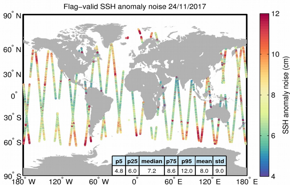
Figure 8. Geographical distribution of flag-valid 20-Hz SSH anomaly measurement noise over oceans and lakes for 24/11/2017. The statistical values shown in the table refer to the SSH anomaly noise and are calculated over all measurements shown in the figure.
