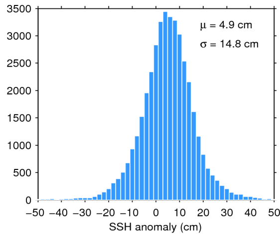
Figure 7. Histogram of flag-valid SSH anomaly over oceans and lakes for 24/11/2017. The mean ( \mu ) and standard deviation ( \sigma ) are also shown. Note that values outside [-50 50] cm are excluded from the histogram for the sake of readability but not from the computation of \mu and \sigma .
