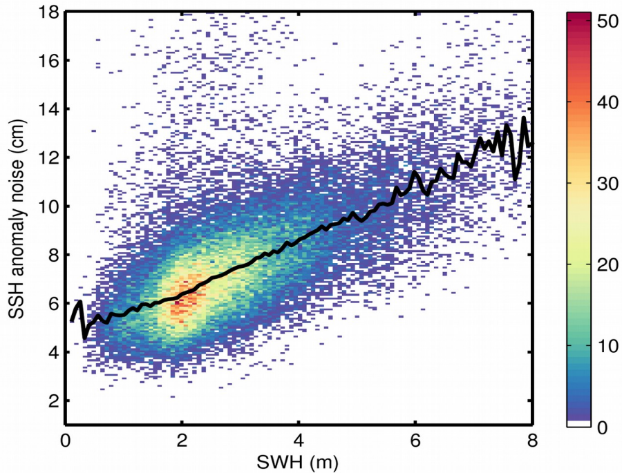
Figure 9. 2D histogram showing flag-valid SSH anomaly noise as a function of SWH for 24/11/2017. The black line denotes the median SSH anomaly noise as a function of SWH.
