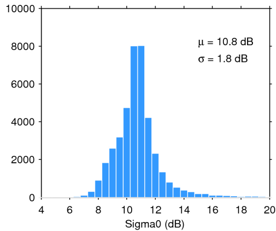
Figure 25. Histogram of flag-valid sigma0 over oceans and lakes for 24/11/2017. The mean ( \mu ) and standard deviation ( \sigma ) are also shown. Note that values outside [4 20] dB are excluded from the histogram for the sake of readability but not from the computation of \mu and \sigma .
