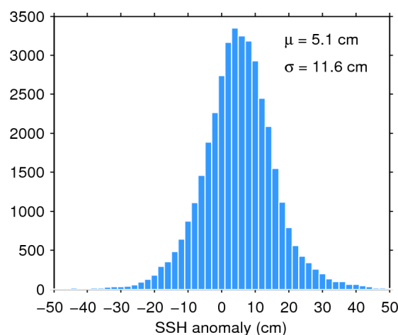
Figure 11. Histogram of science-valid SSH anomaly over oceans and lakes for 24/11/2017. The mean ( \mu ) and standard deviation ( \sigma ) are also shown. Note that values outside [-50 50] cm are excluded from the histogram for the sake of readability but not from the computation of \mu and \sigma .
