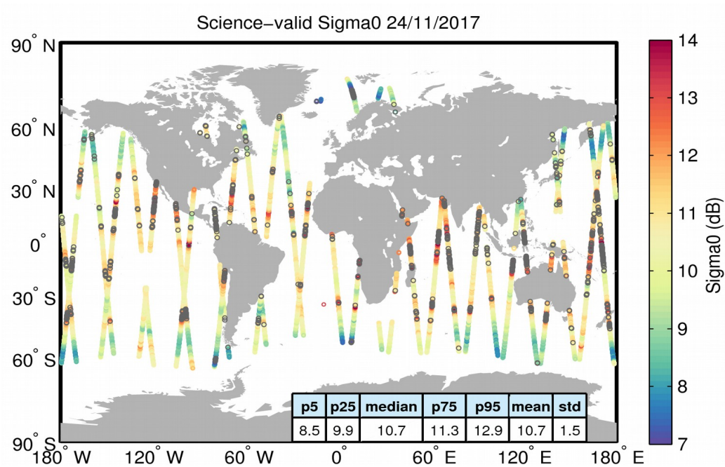
Figure 27. Geographical distribution of science-valid sigma0 data over oceans and lakes for 24/11/2017. The statistical values shown in the table refer to the sigma0 in dB and are calculated over all measurements shown in the figure. Gray circles denote records that have been rejected based on the editing criteria described in Table 4.
