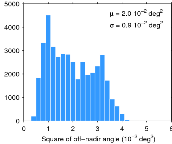
Figure 39. Histogram of flag-valid mispointing over oceans and lakes for 24/11/2017. The mean ( \mu ) and standard deviation ( \sigma ) are also shown. Note that values larger than 6 \cdot 10^{-2} \text{ deg}^2 are excluded from the histogram for the sake of readability but not from the computation of \mu and \sigma .
