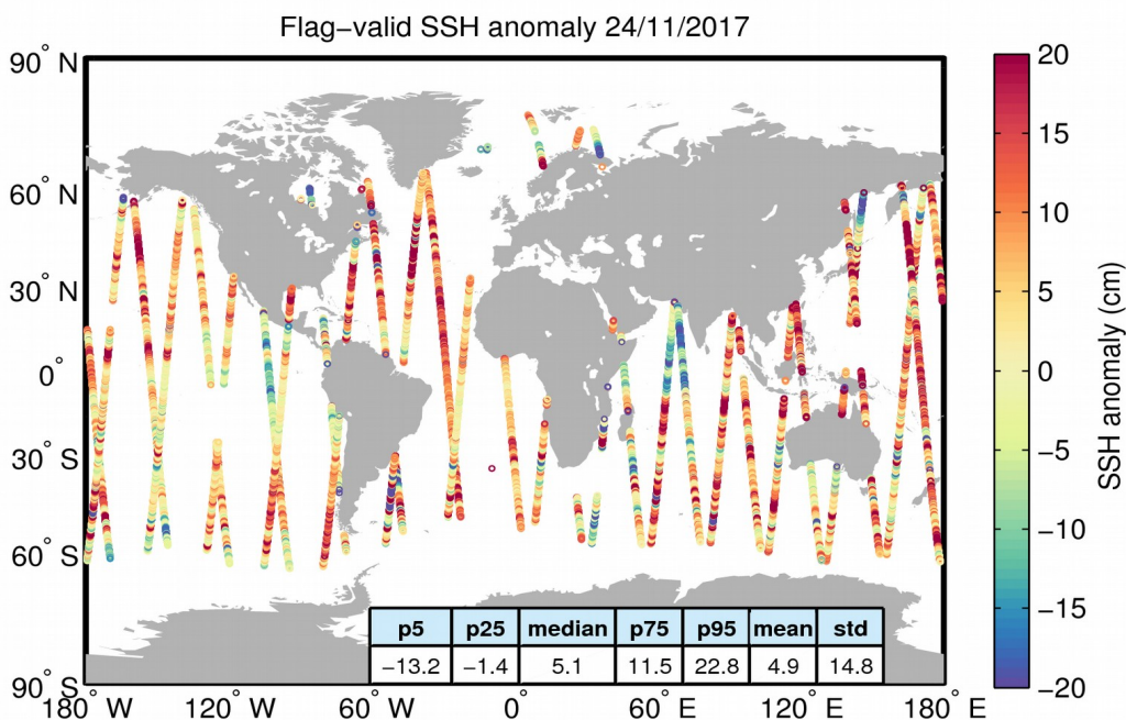
Figure 5. Geographical distribution of flag-valid 1-Hz SSH anomaly data over oceans and lakes for 24/11/2017. The statistical values shown in the table refer to the SSH anomaly in cm and are calculated over all measurements shown in the figure.
