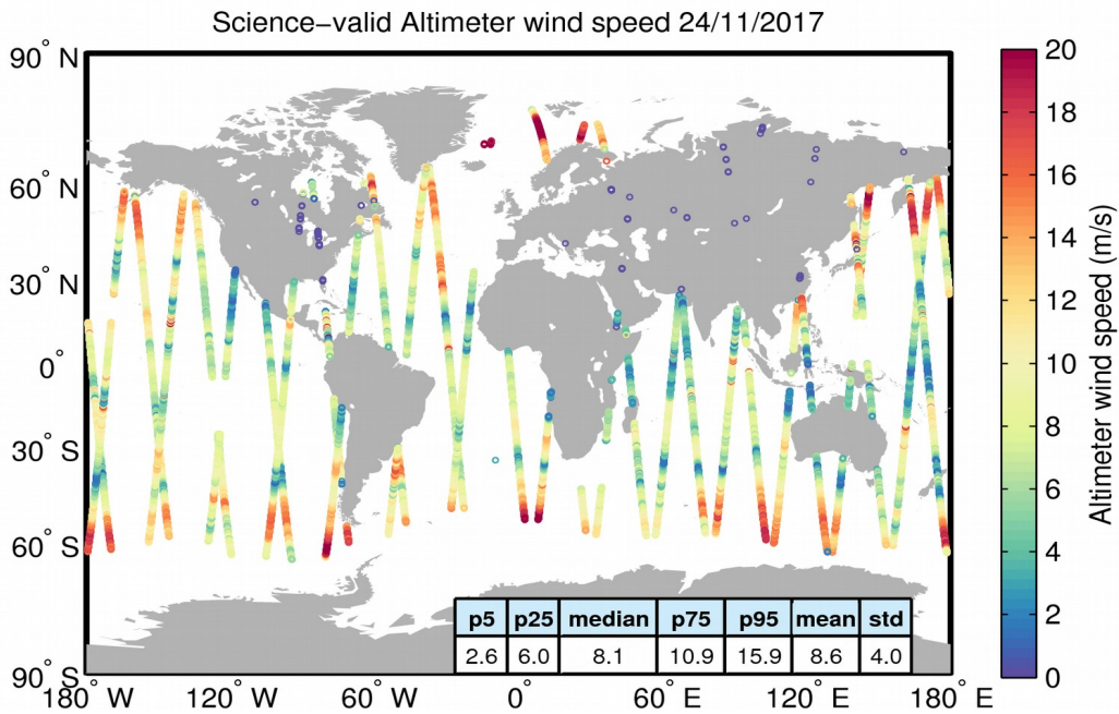
Figure 34. Geographical distribution of science-valid wind data over oceans and lakes for 24/11/2017. The statistical values shown in the table refer to the wind in m/s and are calculated over all measurements shown in the figure. Gray circles denote records that have been rejected based on the editing criteria described in Table 5.
