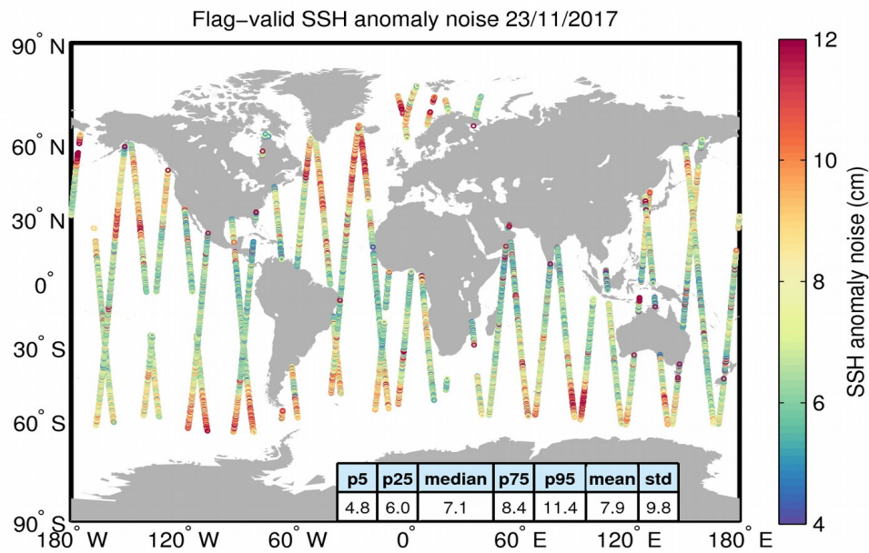
Figure 8. Geographical distribution of flag-valid 20-Hz SSH anomaly measurement noise over oceans and lakes for 23/11/2017. The statistical values shown in the table refer to the SSH anomaly noise and are calculated over all measurements shown in the figure.
