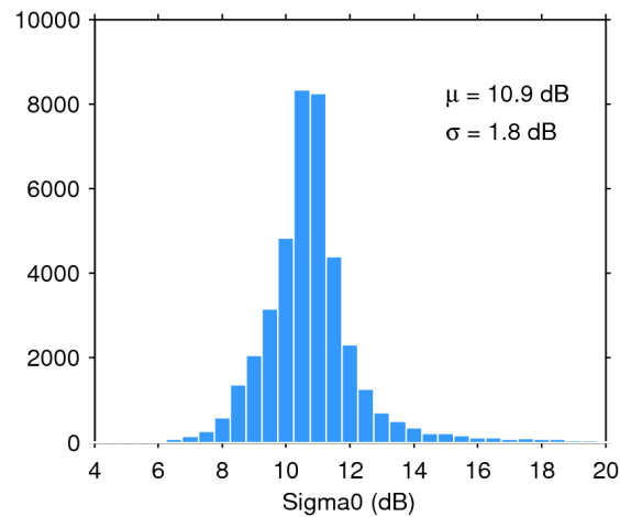
Figure 25. Histogram of flag-valid sigma0 over oceans and lakes for 23/11/2017. The mean ( \mu ) and standard deviation ( \sigma ) are also shown. Note that values outside [4 20] dB are excluded from the histogram for the sake of readability but not from the computation of \mu and \sigma .
