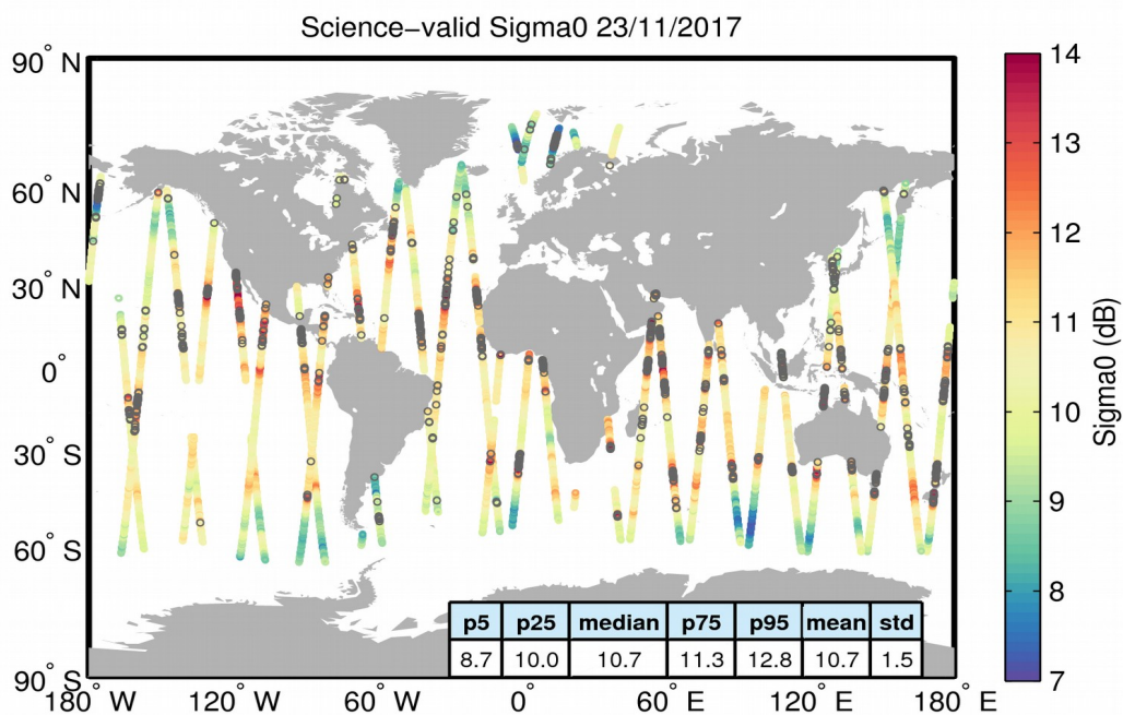
Figure 27. Geographical distribution of science-valid sigma0 data over oceans and lakes for 23/11/2017. The statistical values shown in the table refer to the sigma0 in dB and are calculated over all measurements shown in the figure. Gray circles denote records that have been rejected based on the editing criteria described in Table 4.
