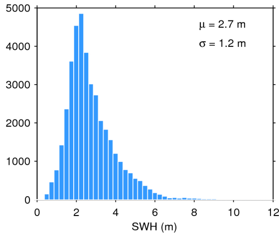
Figure 20. Histogram of science-valid SWH over oceans and lakes for 23/11/2017. The mean ( \mu ) and standard deviation ( \sigma ) are also shown. Note that values larger than 12 m are excluded from the histogram for the sake of readability but not from the computation of \mu and \sigma .
