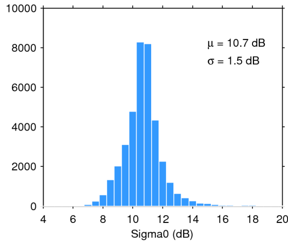
Figure 28. Histogram of science-valid sigma0 over oceans and lakes for 23/11/2017. The mean ( \mu ) and standard deviation ( \sigma ) are also shown. Note that values outside [4 20] dB are excluded from the histogram for the sake of readability but not from the computation of \mu and \sigma .
