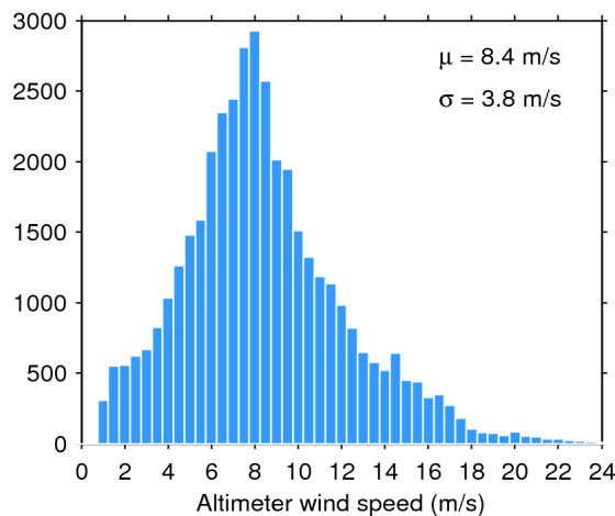
Figure 35. Histogram of science-valid wind over oceans and lakes for 23/11/2017. The mean ( \mu ) and standard deviation ( \sigma ) are also shown. Note that values larger than 24 m/s are excluded from the histogram for the sake of readability but not from the computation of \mu and \sigma .
