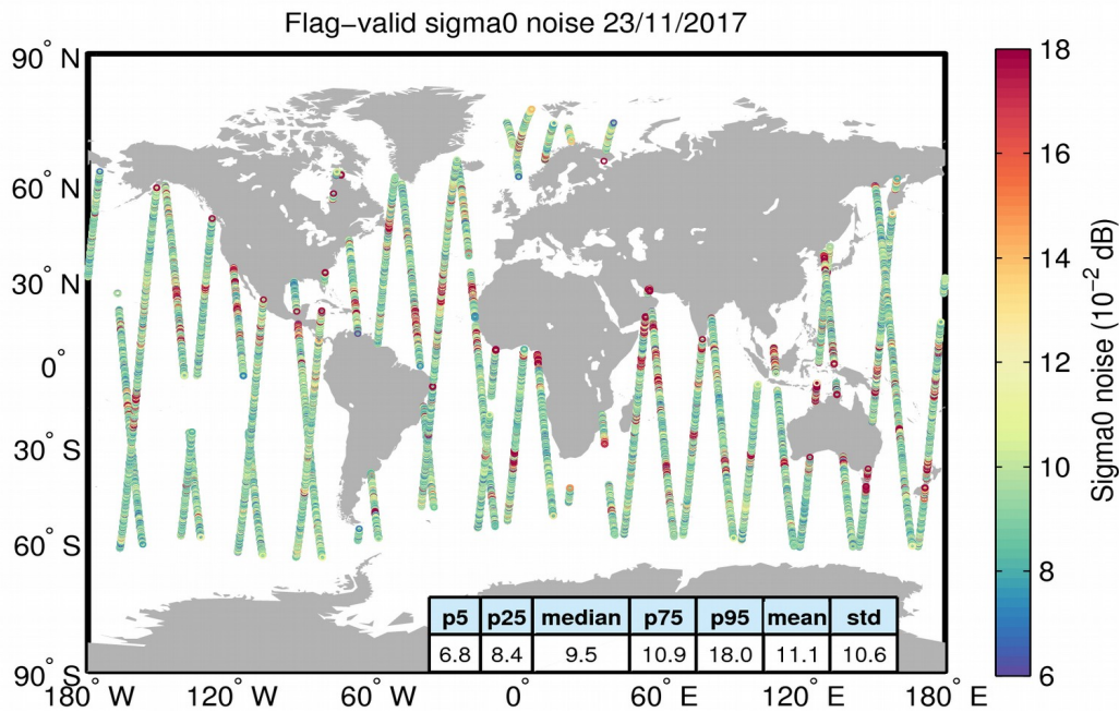
Figure 26. Geographical distribution of flag-valid 20-Hz sigma0 measurement noise over oceans and lakes for 23/11/2017. The statistical values shown in the table refer to the sigma0 noise and are calculated over all measurements shown in the figure.
