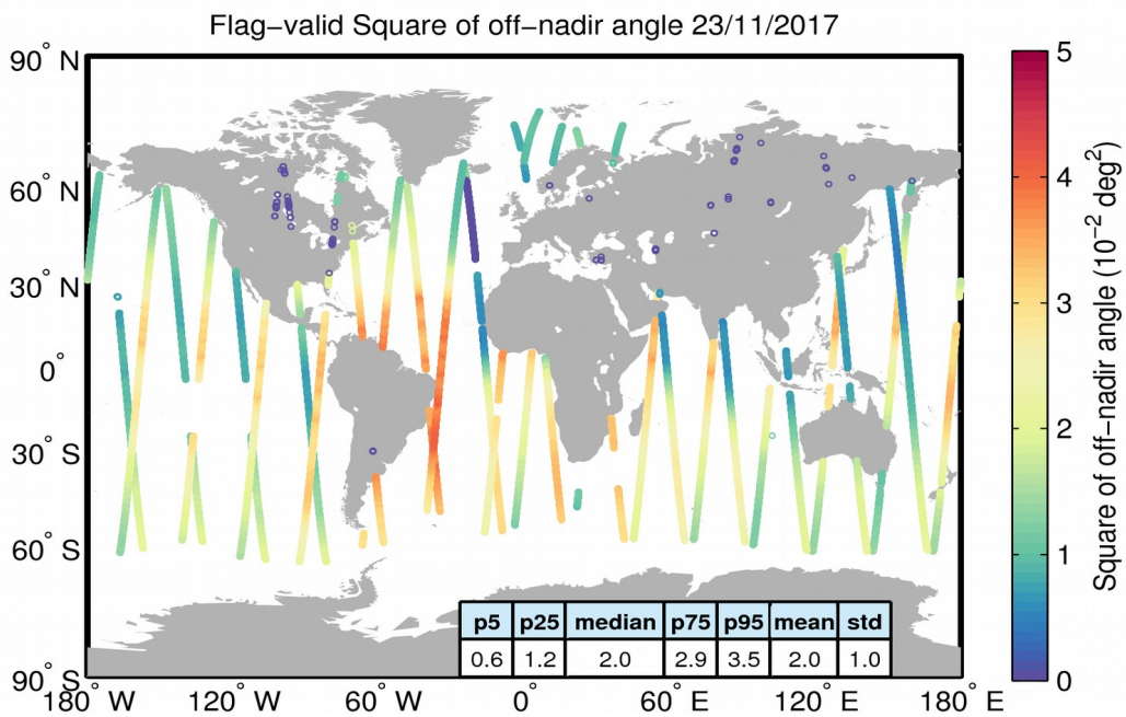
Figure 37. Geographical distribution of flag-valid mispointing data over oceans and lakes for 23/11/2017. The statistical values shown in the table refer to the mispointing in 10^{-2} deg 2 and are calculated over all measurements shown in the figure.
