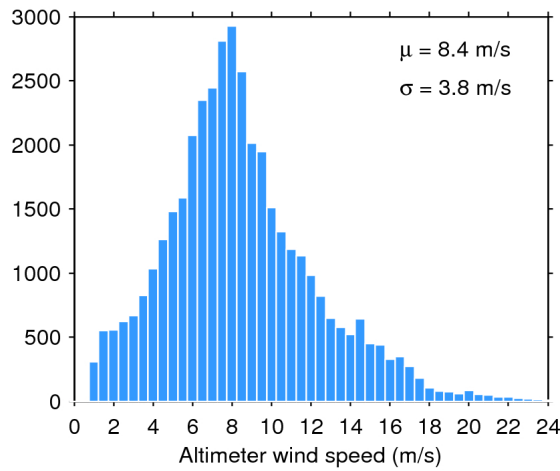
Figure 33. Histogram of flag-valid wind over oceans and lakes for 23/11/2017. The mean ( \mu ) and standard deviation ( \sigma ) are also shown. Note that values larger than 24 m/s are excluded from the histogram for the sake of readability but not from the computation of \mu and \sigma .
