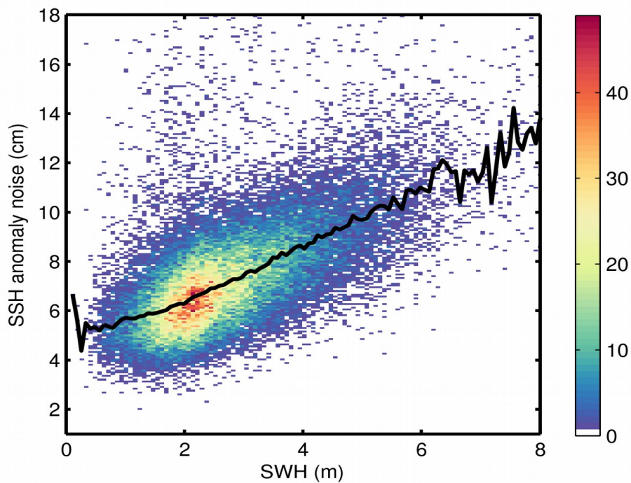
Figure 9. 2D histogram showing flag-valid SSH anomaly noise as a function of SWH for 23/11/2017. The black line denotes the median SSH anomaly noise as a function of SWH.
