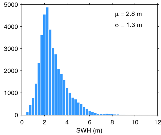
Figure 17. Histogram of flag-valid SWH over oceans and lakes for 23/11/2017. The mean ( \mu ) and standard deviation ( \sigma ) are also shown. Note that values larger than 12 m are excluded from the histogram for the sake of readability but not from the computation of \mu and \sigma .
