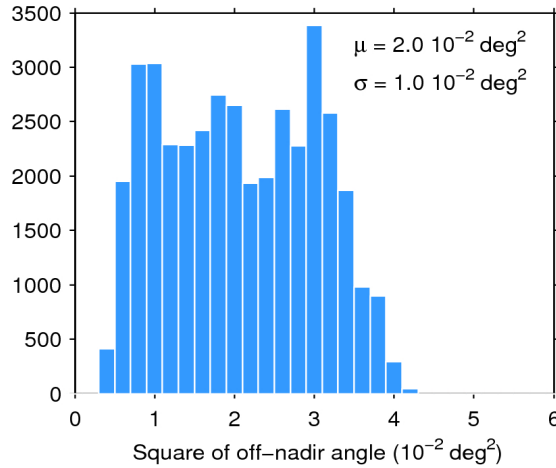
Figure 39. Histogram of flag-valid mispointing over oceans and lakes for 23/11/2017. The mean ( \mu ) and standard deviation ( \sigma ) are also shown. Note that values larger than 6 \cdot 10^{-2} \text{ deg}^2 are excluded from the histogram for the sake of readability but not from the computation of \mu and \sigma .
