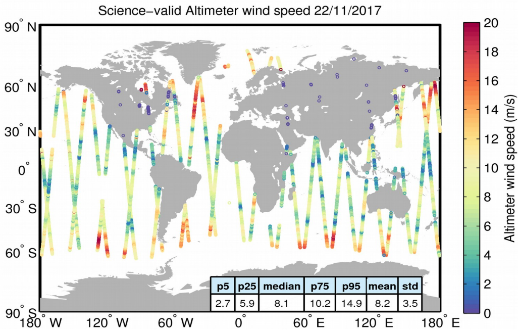
Figure 34. Geographical distribution of science-valid wind data over oceans and lakes for 22/11/2017. The statistical values shown in the table refer to the wind in m/s and are calculated over all measurements shown in the figure. Gray circles denote records that have been rejected based on the editing criteria described in Table 5.
