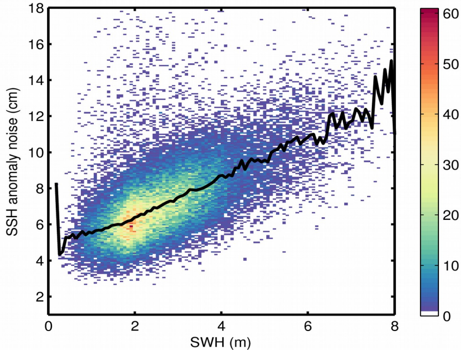
Figure 9. 2D histogram showing flag-valid SSH anomaly noise as a function of SWH for 22/11/2017. The black line denotes the median SSH anomaly noise as a function of SWH.
