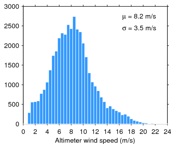
Figure 35. Histogram of science-valid wind over oceans and lakes for 22/11/2017. The mean ( \mu ) and standard deviation ( \sigma ) are also shown. Note that values larger than 24 m/s are excluded from the histogram for the sake of readability but not from the computation of \mu and \sigma .
