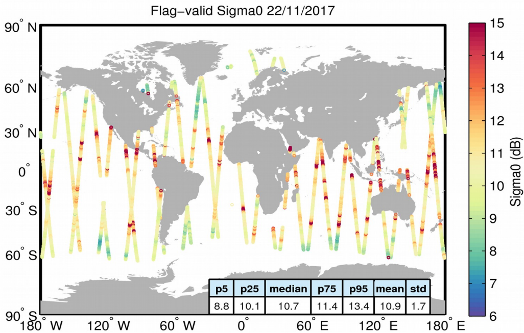
Figure 23. Geographical distribution of flag-valid sigma0 data over oceans and lakes for 22/11/2017. The statistical values shown in the table refer to the sigma0 in dB and are calculated over all measurements shown in the figure.
