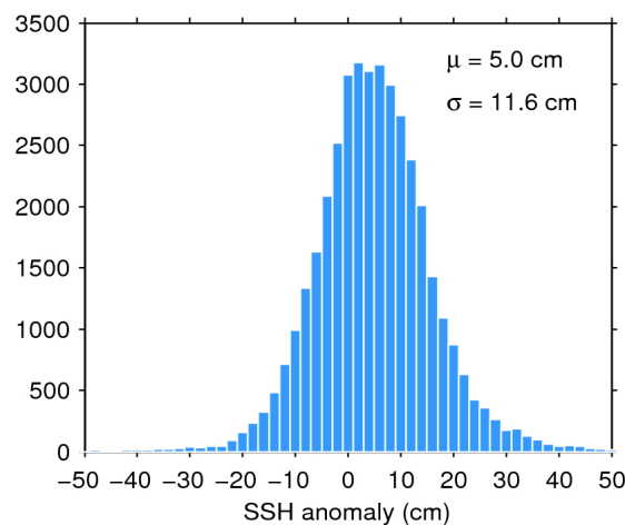
Figure 11. Histogram of science-valid SSH anomaly over oceans and lakes for 22/11/2017. The mean ( \mu ) and standard deviation ( \sigma ) are also shown. Note that values outside [-50 50] cm are excluded from the histogram for the sake of readability but not from the computation of \mu and \sigma .
