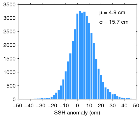
Figure 7. Histogram of flag-valid SSH anomaly over oceans and lakes for 22/11/2017. The mean ( \mu ) and standard deviation ( \sigma ) are also shown. Note that values outside [-50 50] cm are excluded from the histogram for the sake of readability but not from the computation of \mu and \sigma .
