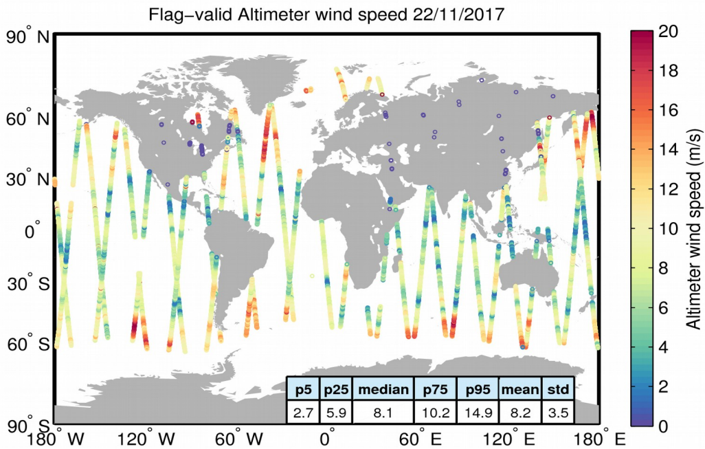
Figure 31. Geographical distribution of flag-valid wind data over oceans and lakes for 22/11/2017. The statistical values shown in the table refer to the wind in m/s and are calculated over all measurements shown in the figure.
