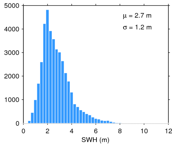
Figure 17. Histogram of flag-valid SWH over oceans and lakes for 22/11/2017. The mean ( \mu ) and standard deviation ( \sigma ) are also shown. Note that values larger than 12 m are excluded from the histogram for the sake of readability but not from the computation of \mu and \sigma .
