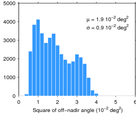
Figure 39. Histogram of flag-valid mispointing over oceans and lakes for 22/11/2017. The mean ( \mu ) and standard deviation ( \sigma ) are also shown. Note that values larger than 6 \cdot 10^{-2} \text{ deg}^2 are excluded from the histogram for the sake of readability but not from the computation of \mu and \sigma .
