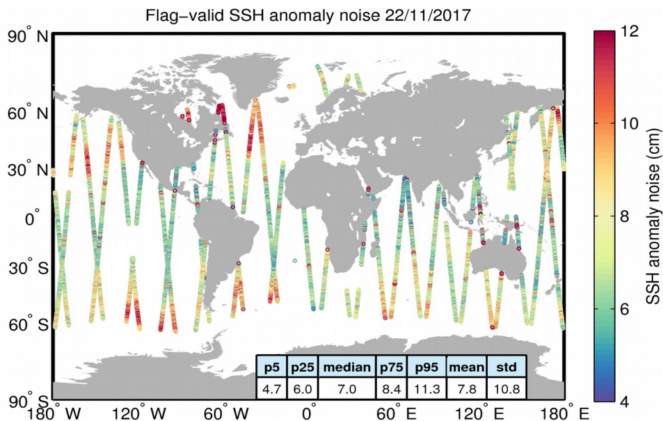
Figure 8. Geographical distribution of flag-valid 20-Hz SSH anomaly measurement noise over oceans and lakes for 22/11/2017. The statistical values shown in the table refer to the SSH anomaly noise and are calculated over all measurements shown in the figure.
