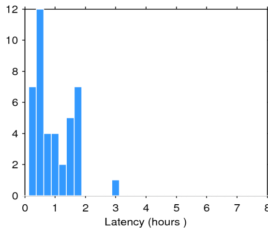
Figure 2. Histogram of the data latency for 22/11/2017. The y-axis denotes the number of files that are made available with a delay of x-hours with respect to the mean time of the records stored in the file.
