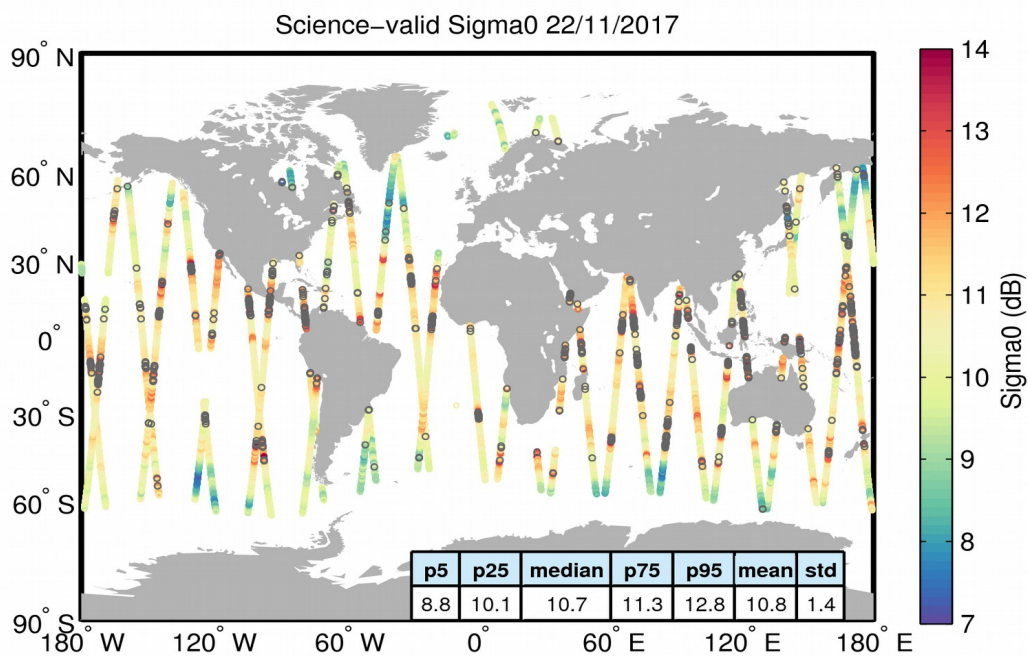
Figure 27. Geographical distribution of science-valid sigma0 data over oceans and lakes for 22/11/2017. The statistical values shown in the table refer to the sigma0 in dB and are calculated over all measurements shown in the figure. Gray circles denote records that have been rejected based on the editing criteria described in Table 4.
