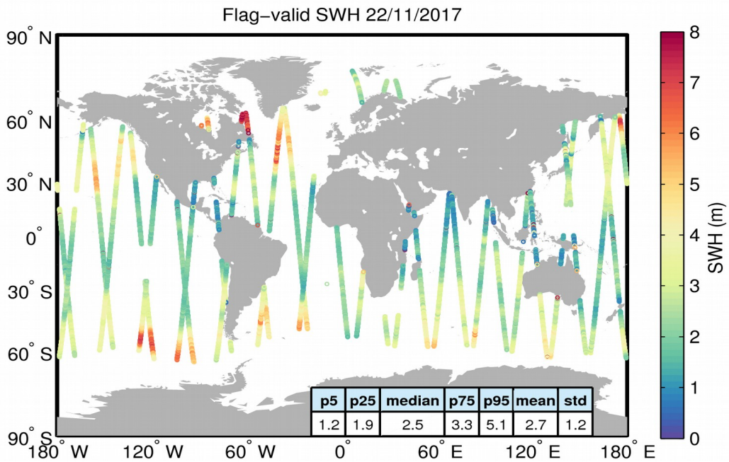
Figure 15. Geographical distribution of flag-valid SWH data over oceans and lakes for 22/11/2017. The statistical values shown in the table refer to the SWH in m and are calculated over all measurements shown in the figure.
