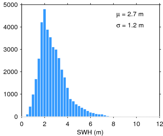
Figure 20. Histogram of science-valid SWH over oceans and lakes for 22/11/2017. The mean ( \mu ) and standard deviation ( \sigma ) are also shown. Note that values larger than 12 m are excluded from the histogram for the sake of readability but not from the computation of \mu and \sigma .
