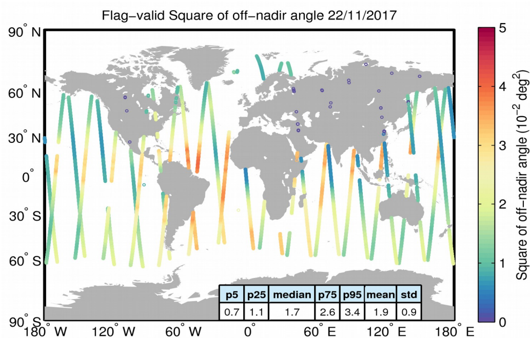
Figure 37. Geographical distribution of flag-valid mispointing data over oceans and lakes for 22/11/2017. The statistical values shown in the table refer to the mispointing in 10^{-2} deg 2 and are calculated over all measurements shown in the figure.
