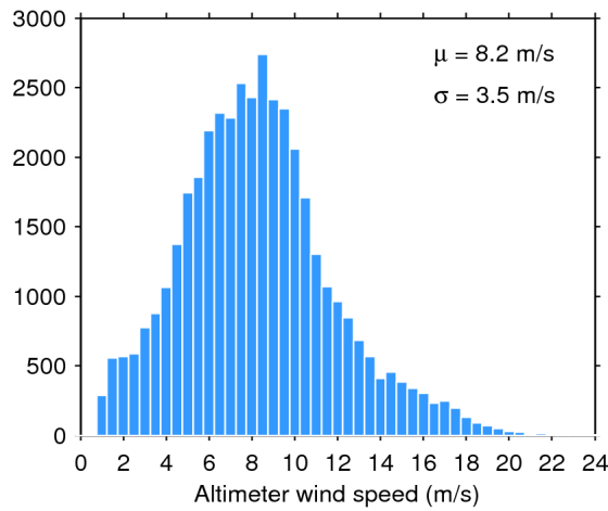
Figure 33. Histogram of flag-valid wind over oceans and lakes for 22/11/2017. The mean ( \mu ) and standard deviation ( \sigma ) are also shown. Note that values larger than 24 m/s are excluded from the histogram for the sake of readability but not from the computation of \mu and \sigma .
