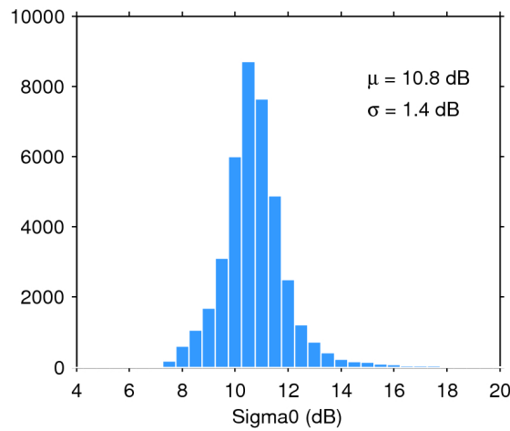
Figure 28. Histogram of science-valid sigma0 over oceans and lakes for 22/11/2017. The mean ( \mu ) and standard deviation ( \sigma ) are also shown. Note that values outside [4 20] dB are excluded from the histogram for the sake of readability but not from the computation of \mu and \sigma .
