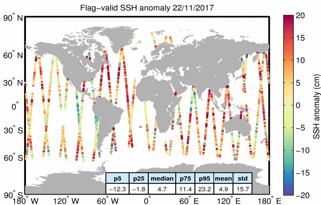
Figure 5. Geographical distribution of flag-valid 1-Hz SSH anomaly data over oceans and lakes for 22/11/2017. The statistical values shown in the table refer to the SSH anomaly in cm and are calculated over all measurements shown in the figure.
