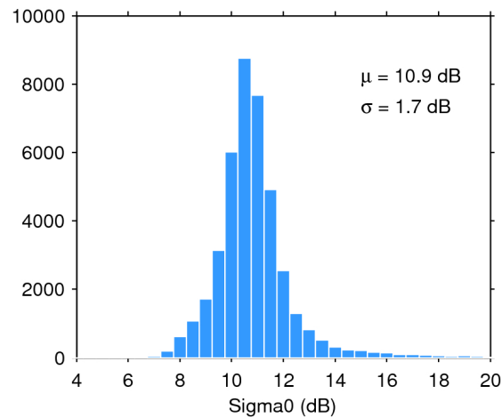
Figure 25. Histogram of flag-valid sigma0 over oceans and lakes for 22/11/2017. The mean ( \mu ) and standard deviation ( \sigma ) are also shown. Note that values outside [4 20] dB are excluded from the histogram for the sake of readability but not from the computation of \mu and \sigma .
