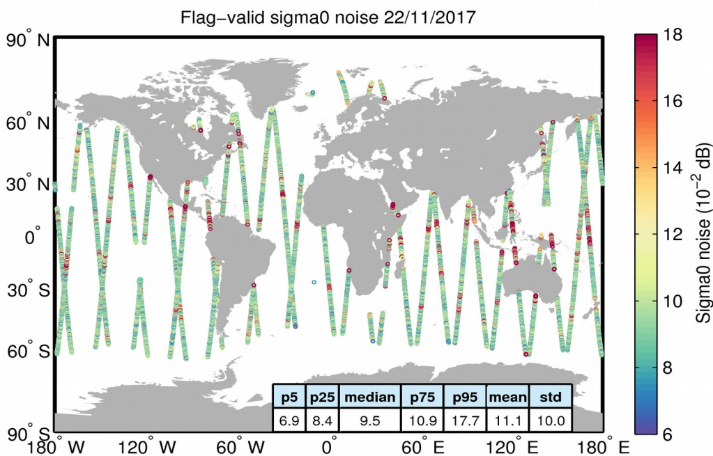
Figure 26. Geographical distribution of flag-valid 20-Hz sigma0 measurement noise over oceans and lakes for 22/11/2017. The statistical values shown in the table refer to the sigma0 noise and are calculated over all measurements shown in the figure.
