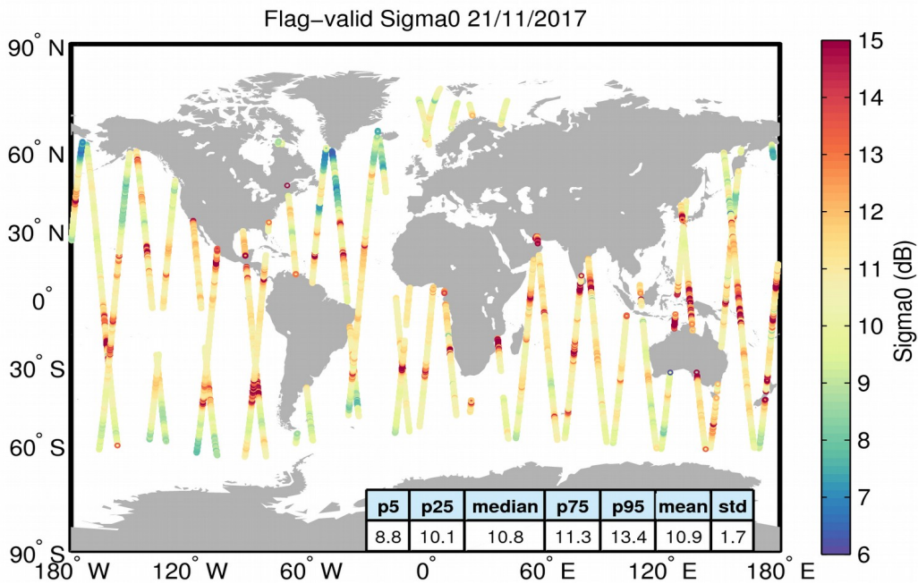
Figure 23. Geographical distribution of flag-valid sigma0 data over oceans and lakes for 21/11/2017. The statistical values shown in the table refer to the sigma0 in dB and are calculated over all measurements shown in the figure.
