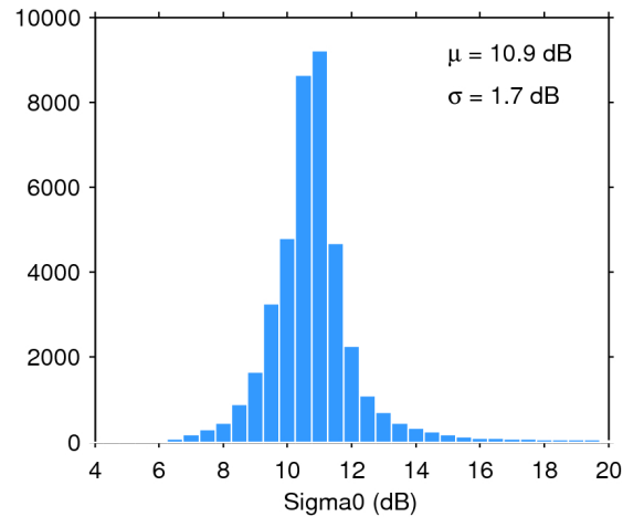
Figure 25. Histogram of flag-valid sigma0 over oceans and lakes for 21/11/2017. The mean ( \mu ) and standard deviation ( \sigma ) are also shown. Note that values outside [4 20] dB are excluded from the histogram for the sake of readability but not from the computation of \mu and \sigma .
