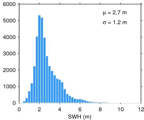
Figure 20. Histogram of science-valid SWH over oceans and lakes for 21/11/2017. The mean ( \mu ) and standard deviation ( \sigma ) are also shown. Note that values larger than 12 m are excluded from the histogram for the sake of readability but not from the computation of \mu and \sigma .
