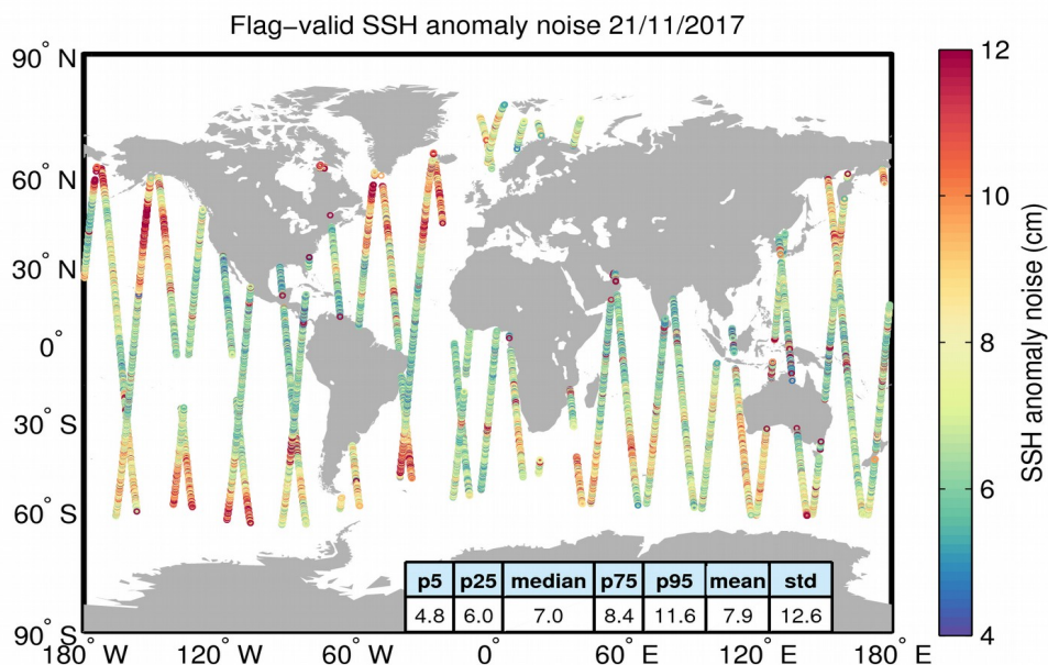
Figure 8. Geographical distribution of flag-valid 20-Hz SSH anomaly measurement noise over oceans and lakes for 21/11/2017. The statistical values shown in the table refer to the SSH anomaly noise and are calculated over all measurements shown in the figure.
