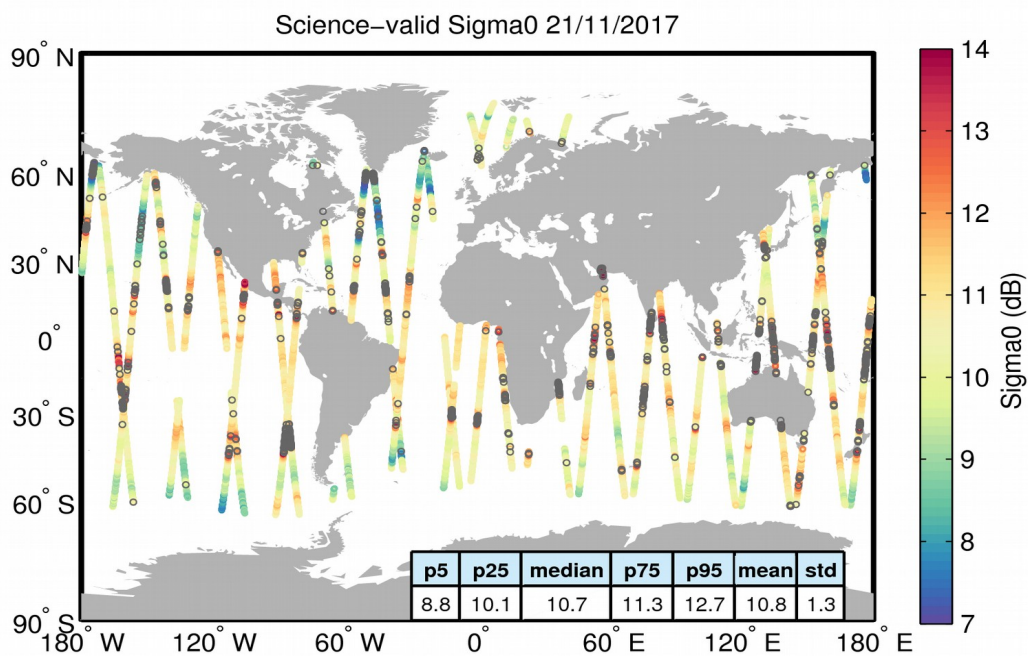
Figure 27. Geographical distribution of science-valid sigma0 data over oceans and lakes for 21/11/2017. The statistical values shown in the table refer to the sigma0 in dB and are calculated over all measurements shown in the figure. Gray circles denote records that have been rejected based on the editing criteria described in Table 4.
