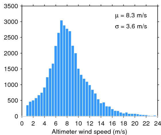
Figure 35. Histogram of science-valid wind over oceans and lakes for 21/11/2017. The mean ( \mu ) and standard deviation ( \sigma ) are also shown. Note that values larger than 24 m/s are excluded from the histogram for the sake of readability but not from the computation of \mu and \sigma .
