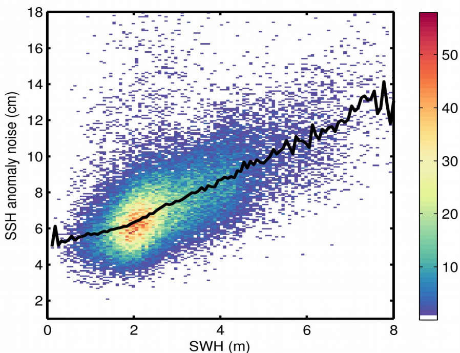
Figure 9. 2D histogram showing flag-valid SSH anomaly noise as a function of SWH for 21/11/2017. The black line denotes the median SSH anomaly noise as a function of SWH.
