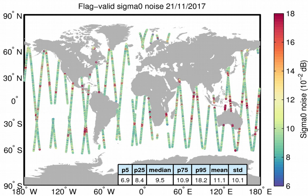
Figure 26. Geographical distribution of flag-valid 20-Hz sigma0 measurement noise over oceans and lakes for 21/11/2017. The statistical values shown in the table refer to the sigma0 noise and are calculated over all measurements shown in the figure.
