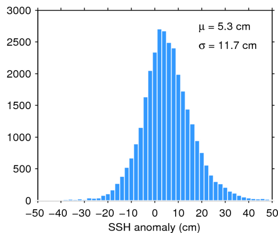
Figure 11. Histogram of science-valid SSH anomaly over oceans and lakes for 21/11/2017. The mean ( \mu ) and standard deviation ( \sigma ) are also shown. Note that values outside [-50 50] cm are excluded from the histogram for the sake of readability but not from the computation of \mu and \sigma .
