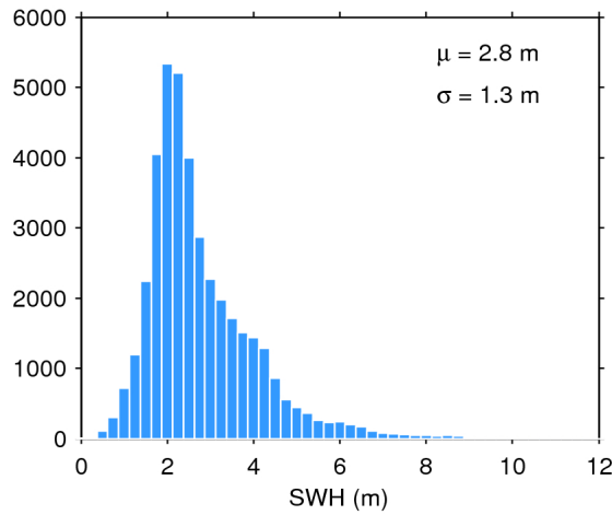
Figure 17. Histogram of flag-valid SWH over oceans and lakes for 21/11/2017. The mean ( \mu ) and standard deviation ( \sigma ) are also shown. Note that values larger than 12 m are excluded from the histogram for the sake of readability but not from the computation of \mu and \sigma .
