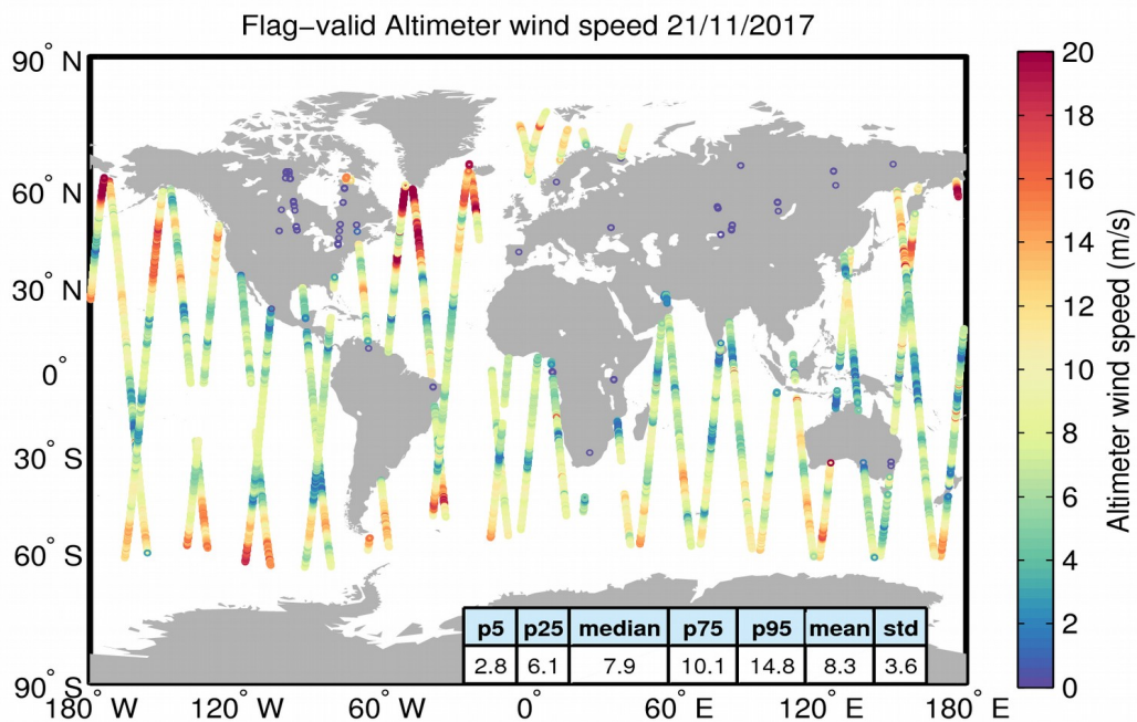
Figure 31. Geographical distribution of flag-valid wind data over oceans and lakes for 21/11/2017. The statistical values shown in the table refer to the wind in m/s and are calculated over all measurements shown in the figure.
