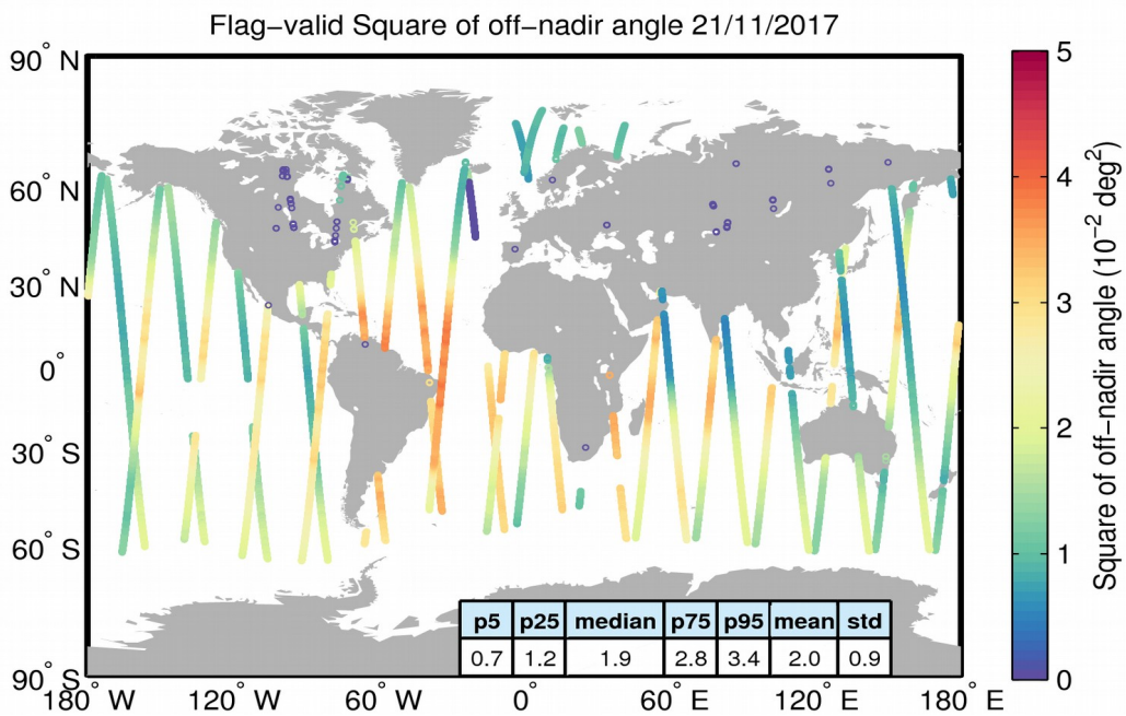
Figure 37. Geographical distribution of flag-valid mispointing data over oceans and lakes for 21/11/2017. The statistical values shown in the table refer to the mispointing in 10^{-2} deg 2 and are calculated over all measurements shown in the figure.
