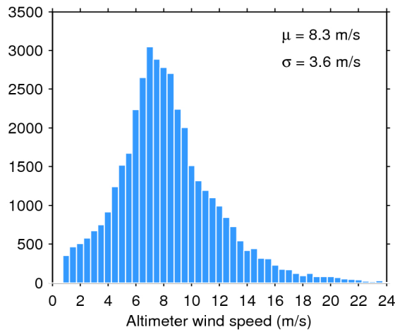
Figure 33. Histogram of flag-valid wind over oceans and lakes for 21/11/2017. The mean ( \mu ) and standard deviation ( \sigma ) are also shown. Note that values larger than 24 m/s are excluded from the histogram for the sake of readability but not from the computation of \mu and \sigma .
