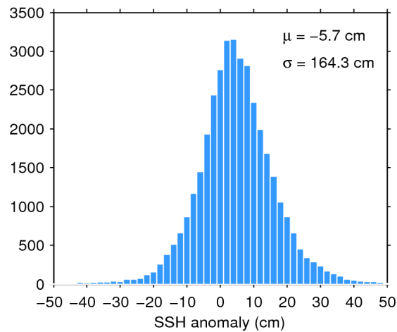
Figure 7. Histogram of flag-valid SSH anomaly over oceans and lakes for 21/11/2017. The mean ( \mu ) and standard deviation ( \sigma ) are also shown. Note that values outside [-50 50] cm are excluded from the histogram for the sake of readability but not from the computation of \mu and \sigma .
