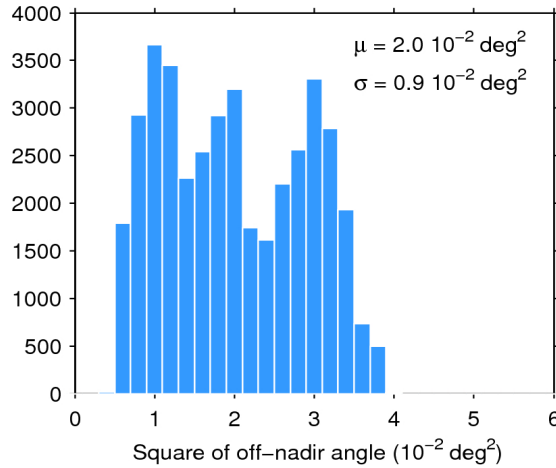
Figure 39. Histogram of flag-valid mispointing over oceans and lakes for 21/11/2017. The mean ( \mu ) and standard deviation ( \sigma ) are also shown. Note that values larger than 6 \cdot 10^{-2} \text{ deg}^2 are excluded from the histogram for the sake of readability but not from the computation of \mu and \sigma .
