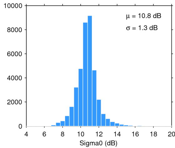
Figure 28. Histogram of science-valid sigma0 over oceans and lakes for 21/11/2017. The mean ( \mu ) and standard deviation ( \sigma ) are also shown. Note that values outside [4 20] dB are excluded from the histogram for the sake of readability but not from the computation of \mu and \sigma .
