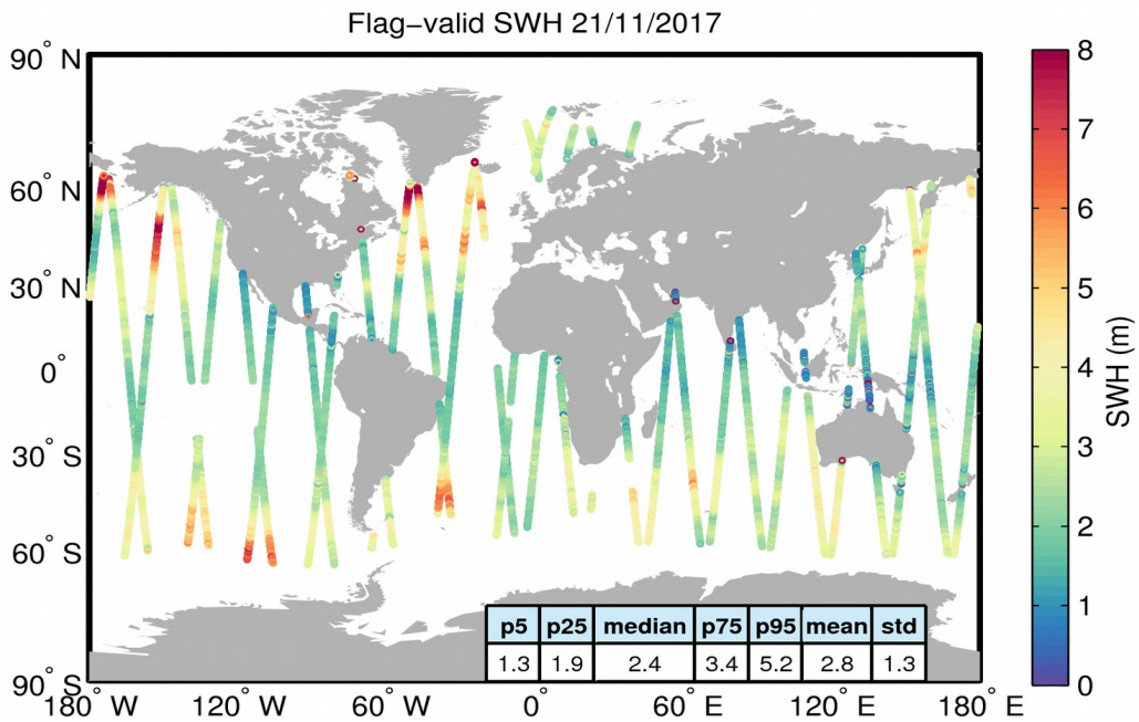
Figure 15. Geographical distribution of flag-valid SWH data over oceans and lakes for 21/11/2017. The statistical values shown in the table refer to the SWH in m and are calculated over all measurements shown in the figure.
