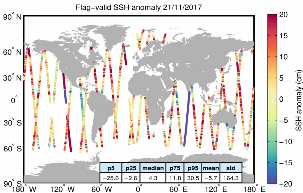
Figure 5. Geographical distribution of flag-valid 1-Hz SSH anomaly data over oceans and lakes for 21/11/2017. The statistical values shown in the table refer to the SSH anomaly in cm and are calculated over all measurements shown in the figure.
