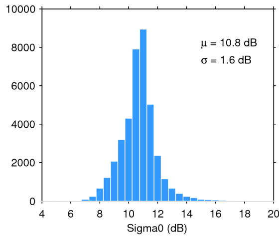
Figure 28. Histogram of science-valid sigma0 over oceans and lakes for 20/11/2017. The mean ( \mu ) and standard deviation ( \sigma ) are also shown. Note that values outside [4 20] dB are excluded from the histogram for the sake of readability but not from the computation of \mu and \sigma .
