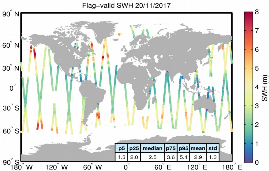
Figure 15. Geographical distribution of flag-valid SWH data over oceans and lakes for 20/11/2017. The statistical values shown in the table refer to the SWH in m and are calculated over all measurements shown in the figure.
