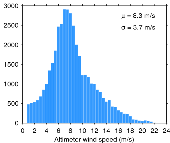
Figure 35. Histogram of science-valid wind over oceans and lakes for 20/11/2017. The mean ( \mu ) and standard deviation ( \sigma ) are also shown. Note that values larger than 24 m/s are excluded from the histogram for the sake of readability but not from the computation of \mu and \sigma .
