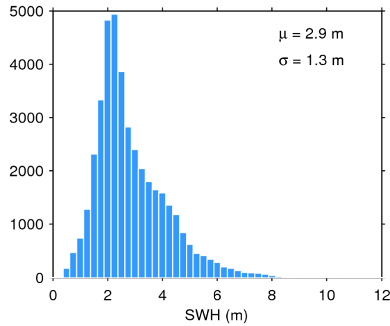
Figure 17. Histogram of flag-valid SWH over oceans and lakes for 20/11/2017. The mean ( \mu ) and standard deviation ( \sigma ) are also shown. Note that values larger than 12 m are excluded from the histogram for the sake of readability but not from the computation of \mu and \sigma .
