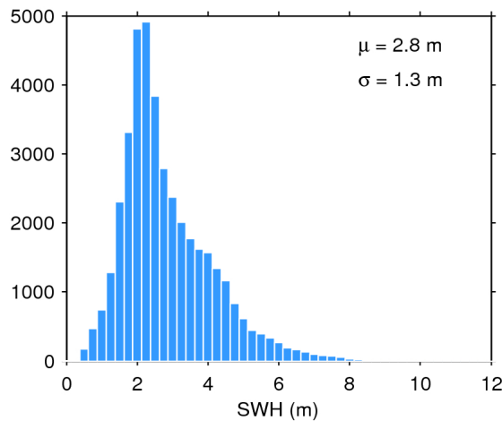
Figure 20. Histogram of science-valid SWH over oceans and lakes for 20/11/2017. The mean ( \mu ) and standard deviation ( \sigma ) are also shown. Note that values larger than 12 m are excluded from the histogram for the sake of readability but not from the computation of \mu and \sigma .
