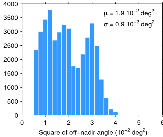
Figure 39. Histogram of flag-valid mispointing over oceans and lakes for 20/11/2017. The mean ( \mu ) and standard deviation ( \sigma ) are also shown. Note that values larger than 6 \cdot 10^{-2} \text{ deg}^2 are excluded from the histogram for the sake of readability but not from the computation of \mu and \sigma .
