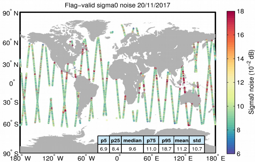
Figure 26. Geographical distribution of flag-valid 20-Hz sigma0 measurement noise over oceans and lakes for 20/11/2017. The statistical values shown in the table refer to the sigma0 noise and are calculated over all measurements shown in the figure.
