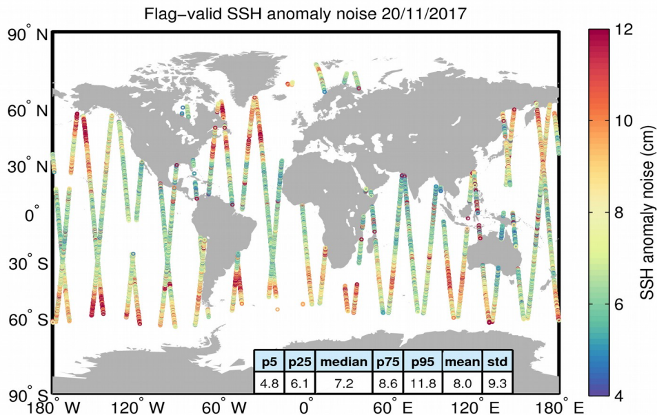
Figure 8. Geographical distribution of flag-valid 20-Hz SSH anomaly measurement noise over oceans and lakes for 20/11/2017. The statistical values shown in the table refer to the SSH anomaly noise and are calculated over all measurements shown in the figure.
