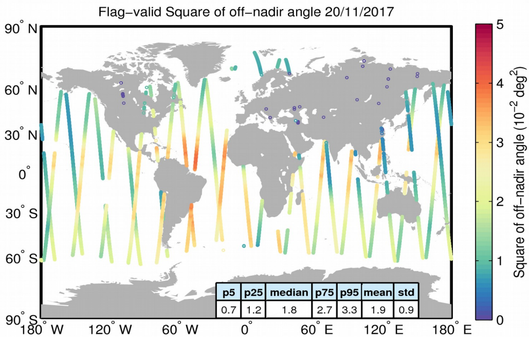
Figure 37. Geographical distribution of flag-valid mispointing data over oceans and lakes for 20/11/2017. The statistical values shown in the table refer to the mispointing in 10^{-2} deg 2 and are calculated over all measurements shown in the figure.
