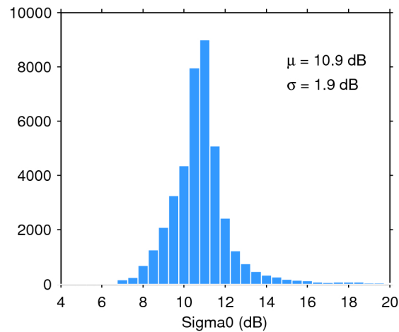
Figure 25. Histogram of flag-valid sigma0 over oceans and lakes for 20/11/2017. The mean ( \mu ) and standard deviation ( \sigma ) are also shown. Note that values outside [4 20] dB are excluded from the histogram for the sake of readability but not from the computation of \mu and \sigma .
