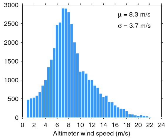
Figure 33. Histogram of flag-valid wind over oceans and lakes for 20/11/2017. The mean ( \mu ) and standard deviation ( \sigma ) are also shown. Note that values larger than 24 m/s are excluded from the histogram for the sake of readability but not from the computation of \mu and \sigma .
