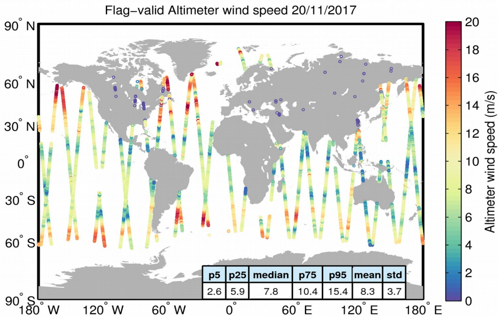
Figure 31. Geographical distribution of flag-valid wind data over oceans and lakes for 20/11/2017. The statistical values shown in the table refer to the wind in m/s and are calculated over all measurements shown in the figure.
