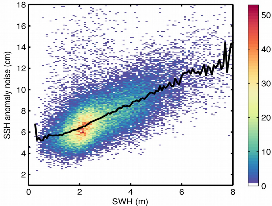
Figure 9. 2D histogram showing flag-valid SSH anomaly noise as a function of SWH for 20/11/2017. The black line denotes the median SSH anomaly noise as a function of SWH.
