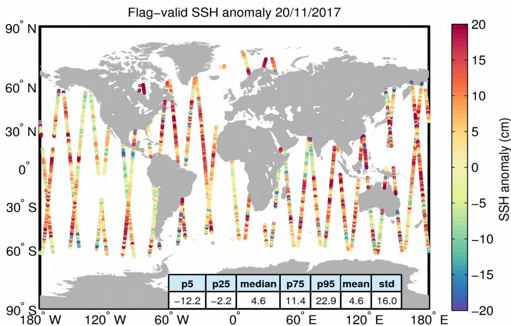
Figure 5. Geographical distribution of flag-valid 1-Hz SSH anomaly data over oceans and lakes for 20/11/2017. The statistical values shown in the table refer to the SSH anomaly in cm and are calculated over all measurements shown in the figure.
