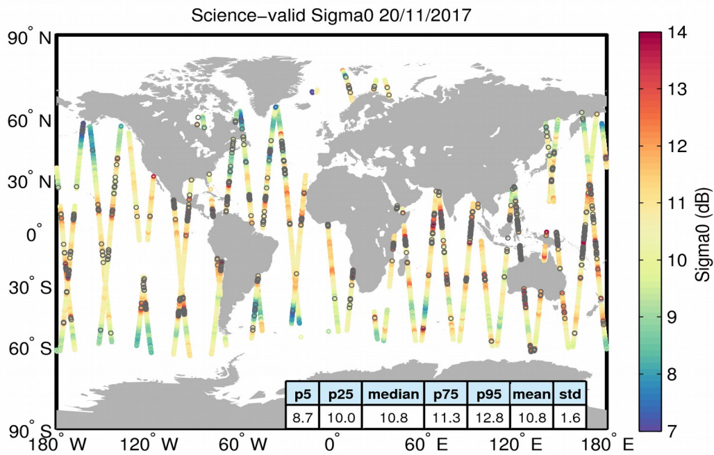
Figure 27. Geographical distribution of science-valid sigma0 data over oceans and lakes for 20/11/2017. The statistical values shown in the table refer to the sigma0 in dB and are calculated over all measurements shown in the figure. Gray circles denote records that have been rejected based on the editing criteria described in Table 4.
