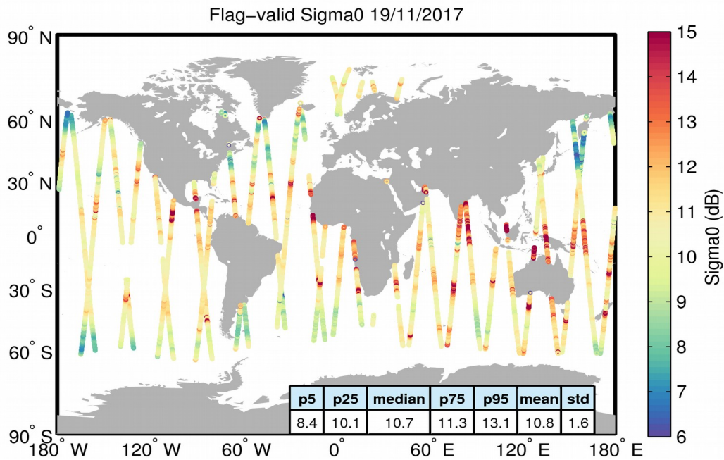
Figure 23. Geographical distribution of flag-valid sigma0 data over oceans and lakes for 19/11/2017. The statistical values shown in the table refer to the sigma0 in dB and are calculated over all measurements shown in the figure.
