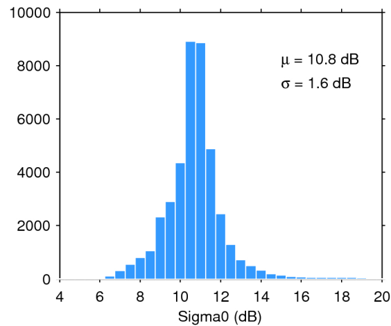
Figure 25. Histogram of flag-valid sigma0 over oceans and lakes for 19/11/2017. The mean ( \mu ) and standard deviation ( \sigma ) are also shown. Note that values outside [4 20] dB are excluded from the histogram for the sake of readability but not from the computation of \mu and \sigma .
