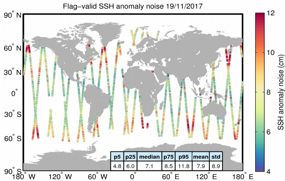
Figure 8. Geographical distribution of flag-valid 20-Hz SSH anomaly measurement noise over oceans and lakes for 19/11/2017. The statistical values shown in the table refer to the SSH anomaly noise and are calculated over all measurements shown in the figure.
