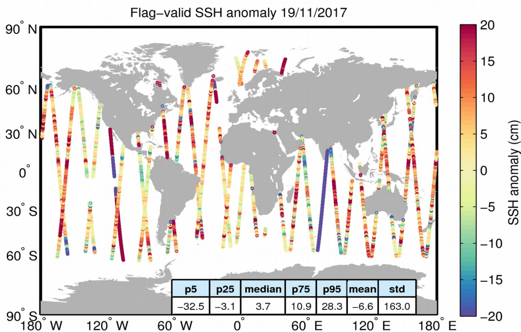
Figure 5. Geographical distribution of flag-valid 1-Hz SSH anomaly data over oceans and lakes for 19/11/2017. The statistical values shown in the table refer to the SSH anomaly in cm and are calculated over all measurements shown in the figure.
