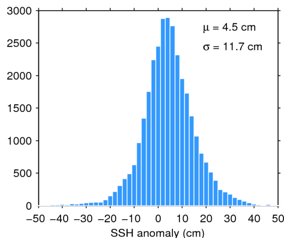
Figure 11. Histogram of science-valid SSH anomaly over oceans and lakes for 19/11/2017. The mean ( \mu ) and standard deviation ( \sigma ) are also shown. Note that values outside [-50 50] cm are excluded from the histogram for the sake of readability but not from the computation of \mu and \sigma .
