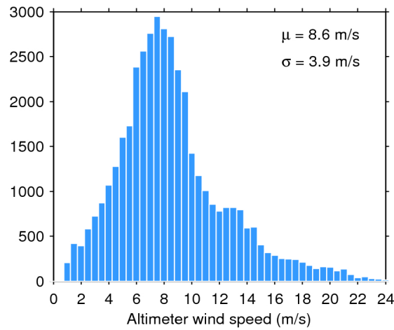
Figure 33. Histogram of flag-valid wind over oceans and lakes for 19/11/2017. The mean ( \mu ) and standard deviation ( \sigma ) are also shown. Note that values larger than 24 m/s are excluded from the histogram for the sake of readability but not from the computation of \mu and \sigma .
