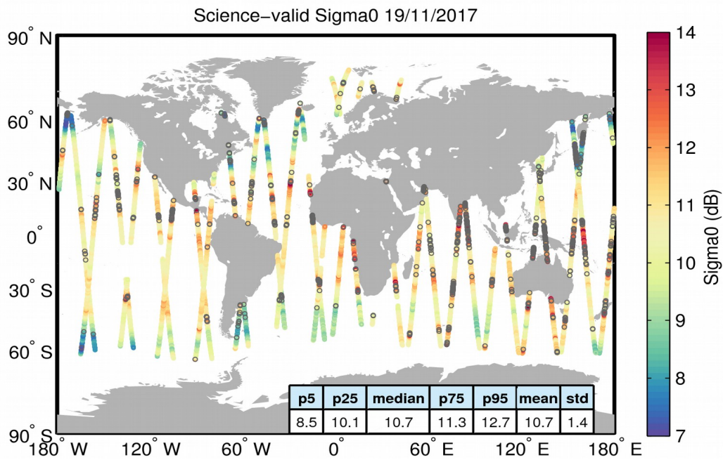
Figure 27. Geographical distribution of science-valid sigma0 data over oceans and lakes for 19/11/2017. The statistical values shown in the table refer to the sigma0 in dB and are calculated over all measurements shown in the figure. Gray circles denote records that have been rejected based on the editing criteria described in Table 4.
