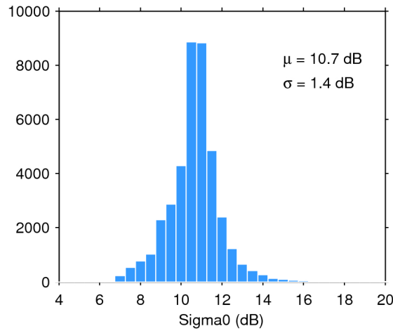
Figure 28. Histogram of science-valid sigma0 over oceans and lakes for 19/11/2017. The mean ( \mu ) and standard deviation ( \sigma ) are also shown. Note that values outside [4 20] dB are excluded from the histogram for the sake of readability but not from the computation of \mu and \sigma .
