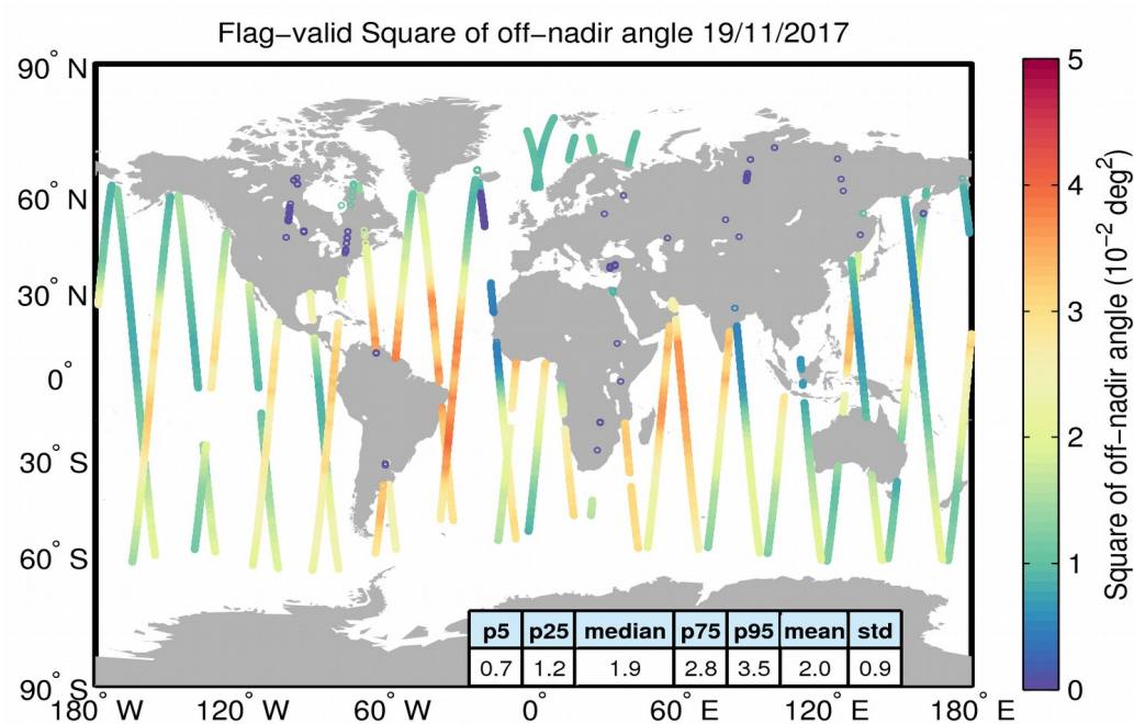
Figure 37. Geographical distribution of flag-valid mispointing data over oceans and lakes for 19/11/2017. The statistical values shown in the table refer to the mispointing in 10^{-2} deg 2 and are calculated over all measurements shown in the figure.
