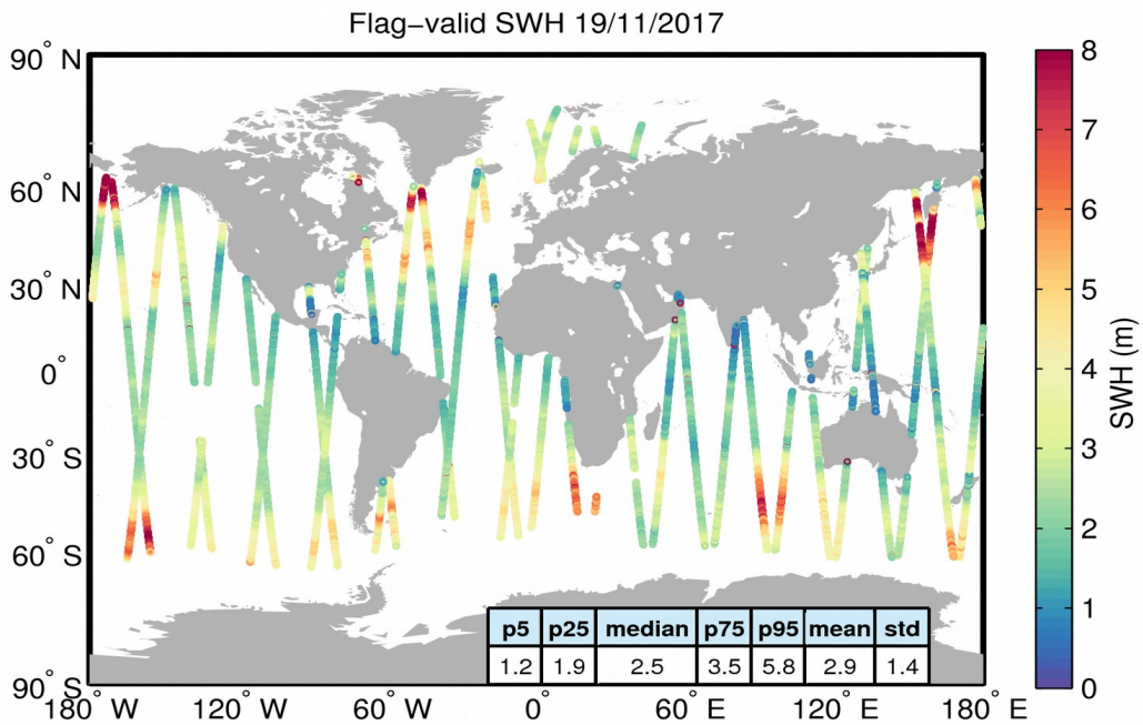
Figure 15. Geographical distribution of flag-valid SWH data over oceans and lakes for 19/11/2017. The statistical values shown in the table refer to the SWH in m and are calculated over all measurements shown in the figure.
