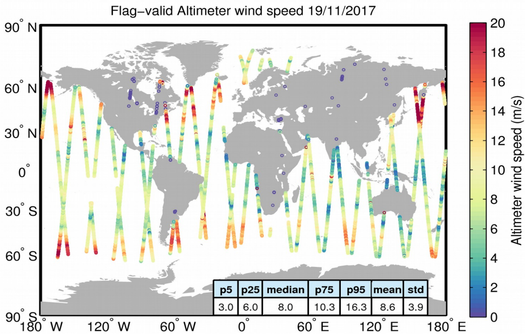
Figure 31. Geographical distribution of flag-valid wind data over oceans and lakes for 19/11/2017. The statistical values shown in the table refer to the wind in m/s and are calculated over all measurements shown in the figure.
