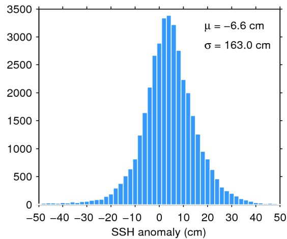
Figure 7. Histogram of flag-valid SSH anomaly over oceans and lakes for 19/11/2017. The mean ( \mu ) and standard deviation ( \sigma ) are also shown. Note that values outside [-50 50] cm are excluded from the histogram for the sake of readability but not from the computation of \mu and \sigma .
