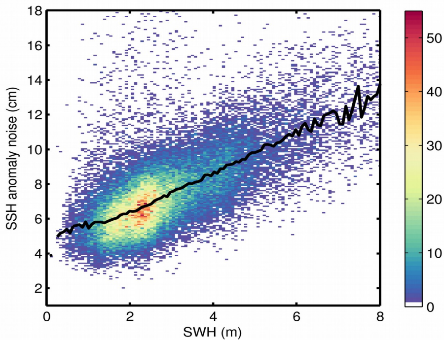
Figure 9. 2D histogram showing flag-valid SSH anomaly noise as a function of SWH for 19/11/2017. The black line denotes the median SSH anomaly noise as a function of SWH.
