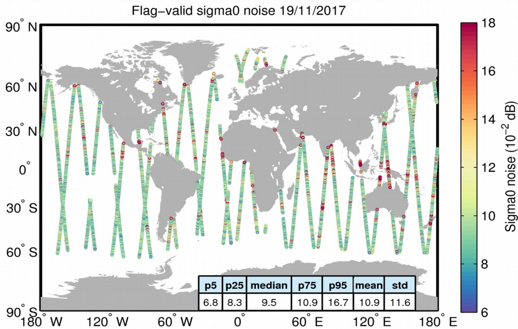
Figure 26. Geographical distribution of flag-valid 20-Hz sigma0 measurement noise over oceans and lakes for 19/11/2017. The statistical values shown in the table refer to the sigma0 noise and are calculated over all measurements shown in the figure.
