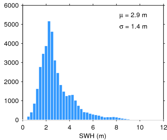
Figure 17. Histogram of flag-valid SWH over oceans and lakes for 19/11/2017. The mean ( \mu ) and standard deviation ( \sigma ) are also shown. Note that values larger than 12 m are excluded from the histogram for the sake of readability but not from the computation of \mu and \sigma .
