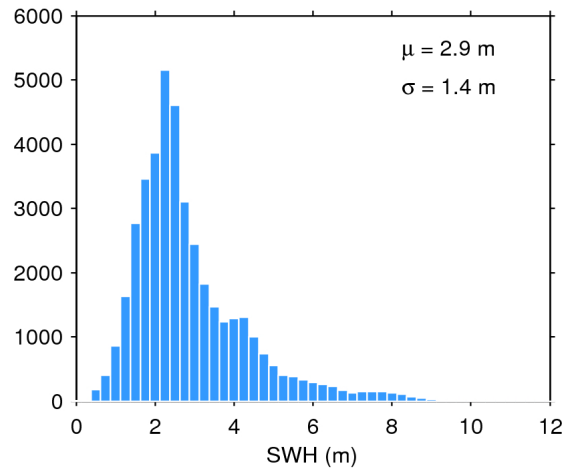
Figure 20. Histogram of science-valid SWH over oceans and lakes for 19/11/2017. The mean ( \mu ) and standard deviation ( \sigma ) are also shown. Note that values larger than 12 m are excluded from the histogram for the sake of readability but not from the computation of \mu and \sigma .
