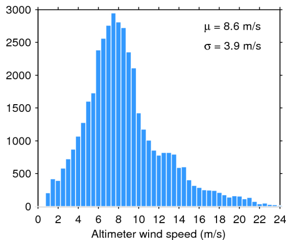
Figure 35. Histogram of science-valid wind over oceans and lakes for 19/11/2017. The mean ( \mu ) and standard deviation ( \sigma ) are also shown. Note that values larger than 24 m/s are excluded from the histogram for the sake of readability but not from the computation of \mu and \sigma .
