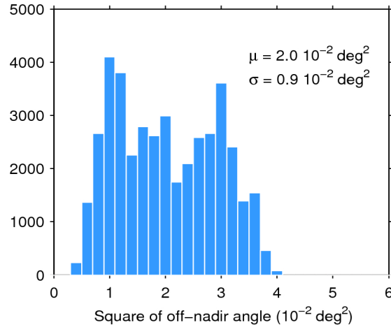
Figure 39. Histogram of flag-valid mispointing over oceans and lakes for 19/11/2017. The mean ( \mu ) and standard deviation ( \sigma ) are also shown. Note that values larger than 6 \cdot 10^{-2} \text{ deg}^2 are excluded from the histogram for the sake of readability but not from the computation of \mu and \sigma .
