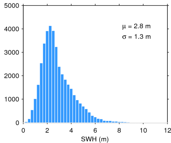
Figure 20. Histogram of science-valid SWH over oceans and lakes for 18/11/2017. The mean ( \mu ) and standard deviation ( \sigma ) are also shown. Note that values larger than 12 m are excluded from the histogram for the sake of readability but not from the computation of \mu and \sigma .
