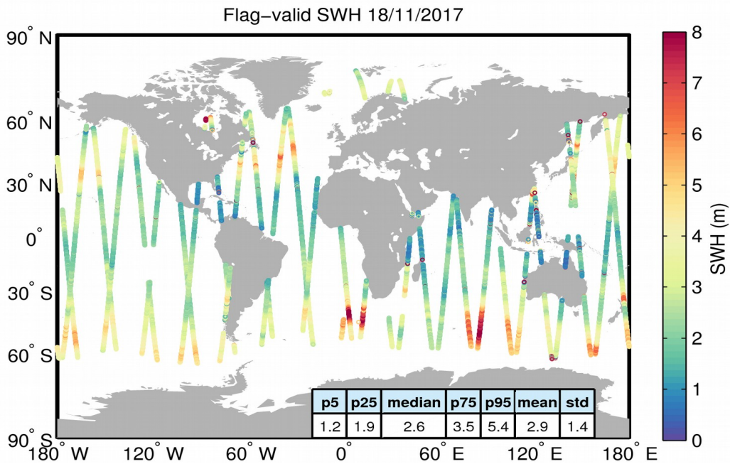
Figure 15. Geographical distribution of flag-valid SWH data over oceans and lakes for 18/11/2017. The statistical values shown in the table refer to the SWH in m and are calculated over all measurements shown in the figure.
