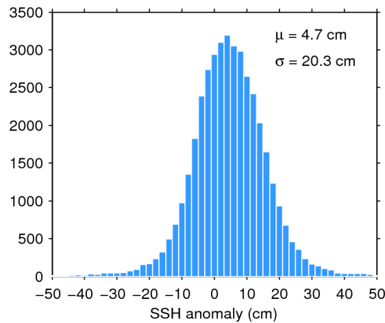
Figure 7. Histogram of flag-valid SSH anomaly over oceans and lakes for 18/11/2017. The mean ( \mu ) and standard deviation ( \sigma ) are also shown. Note that values outside [-50 50] cm are excluded from the histogram for the sake of readability but not from the computation of \mu and \sigma .
