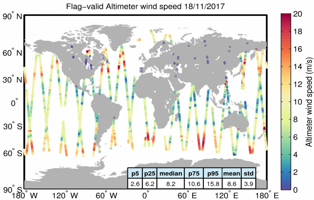
Figure 31. Geographical distribution of flag-valid wind data over oceans and lakes for 18/11/2017. The statistical values shown in the table refer to the wind in m/s and are calculated over all measurements shown in the figure.
