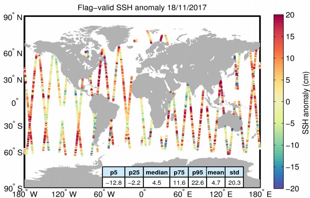
Figure 5. Geographical distribution of flag-valid 1-Hz SSH anomaly data over oceans and lakes for 18/11/2017. The statistical values shown in the table refer to the SSH anomaly in cm and are calculated over all measurements shown in the figure.
