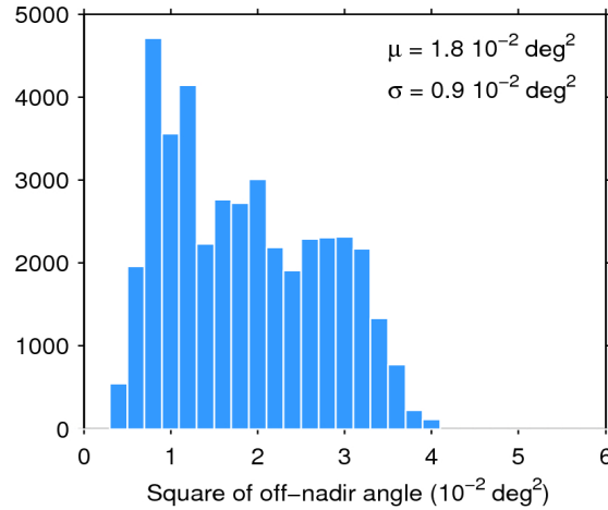
Figure 39. Histogram of flag-valid mispointing over oceans and lakes for 18/11/2017. The mean ( \mu ) and standard deviation ( \sigma ) are also shown. Note that values larger than 6 \cdot 10^{-2} \text{ deg}^2 are excluded from the histogram for the sake of readability but not from the computation of \mu and \sigma .
