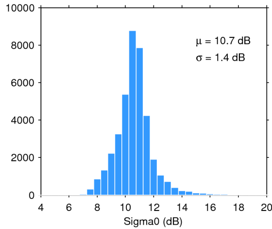
Figure 28. Histogram of science-valid sigma0 over oceans and lakes for 18/11/2017. The mean ( \mu ) and standard deviation ( \sigma ) are also shown. Note that values outside [4 20] dB are excluded from the histogram for the sake of readability but not from the computation of \mu and \sigma .
