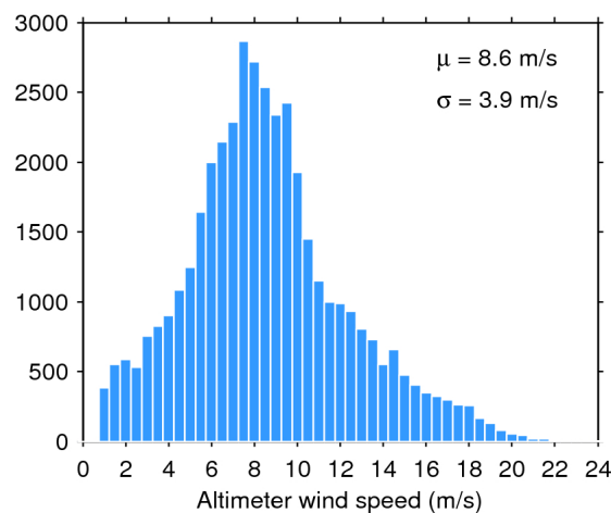
Figure 35. Histogram of science-valid wind over oceans and lakes for 18/11/2017. The mean ( \mu ) and standard deviation ( \sigma ) are also shown. Note that values larger than 24 m/s are excluded from the histogram for the sake of readability but not from the computation of \mu and \sigma .
