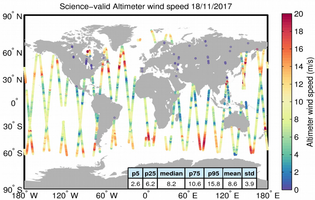
Figure 34. Geographical distribution of science-valid wind data over oceans and lakes for 18/11/2017. The statistical values shown in the table refer to the wind in m/s and are calculated over all measurements shown in the figure. Gray circles denote records that have been rejected based on the editing criteria described in Table 5.
