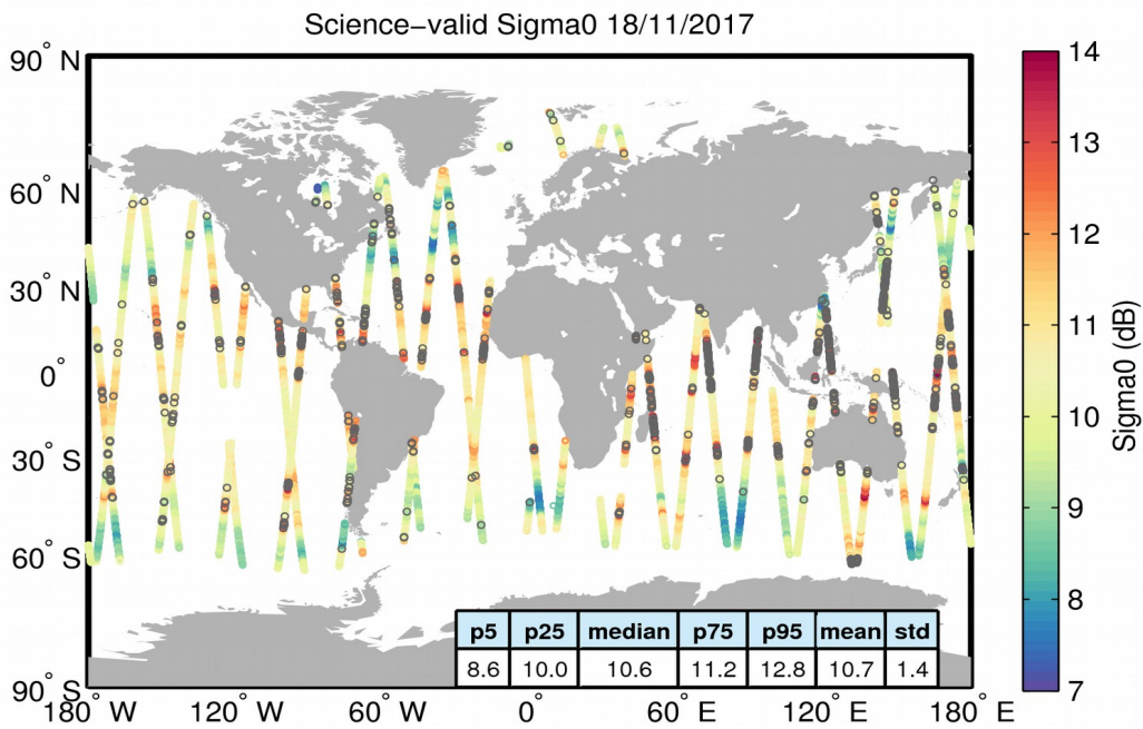
Figure 27. Geographical distribution of science-valid sigma0 data over oceans and lakes for 18/11/2017. The statistical values shown in the table refer to the sigma0 in dB and are calculated over all measurements shown in the figure. Gray circles denote records that have been rejected based on the editing criteria described in Table 4.
