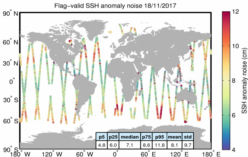
Figure 8. Geographical distribution of flag-valid 20-Hz SSH anomaly measurement noise over oceans and lakes for 18/11/2017. The statistical values shown in the table refer to the SSH anomaly noise and are calculated over all measurements shown in the figure.
