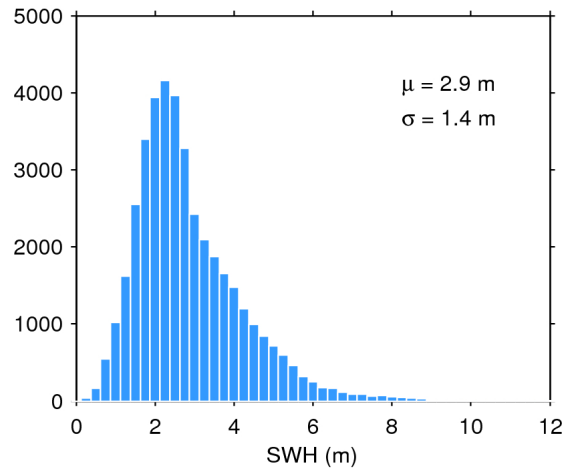
Figure 17. Histogram of flag-valid SWH over oceans and lakes for 18/11/2017. The mean ( \mu ) and standard deviation ( \sigma ) are also shown. Note that values larger than 12 m are excluded from the histogram for the sake of readability but not from the computation of \mu and \sigma .
