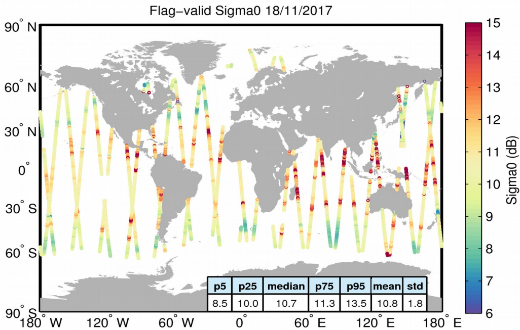
Figure 23. Geographical distribution of flag-valid sigma0 data over oceans and lakes for 18/11/2017. The statistical values shown in the table refer to the sigma0 in dB and are calculated over all measurements shown in the figure.
