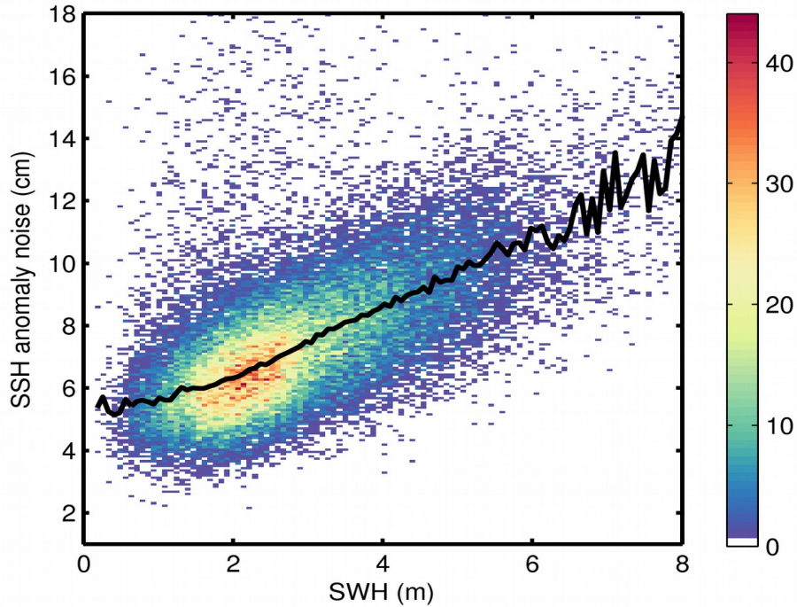
Figure 9. 2D histogram showing flag-valid SSH anomaly noise as a function of SWH for 18/11/2017. The black line denotes the median SSH anomaly noise as a function of SWH.
