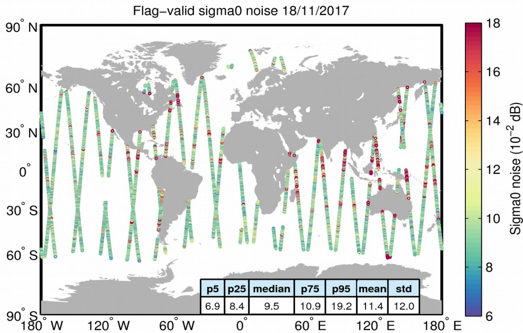
Figure 26. Geographical distribution of flag-valid 20-Hz sigma0 measurement noise over oceans and lakes for 18/11/2017. The statistical values shown in the table refer to the sigma0 noise and are calculated over all measurements shown in the figure.
