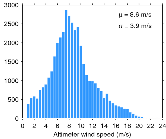
Figure 33. Histogram of flag-valid wind over oceans and lakes for 18/11/2017. The mean ( \mu ) and standard deviation ( \sigma ) are also shown. Note that values larger than 24 m/s are excluded from the histogram for the sake of readability but not from the computation of \mu and \sigma .
