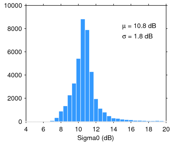
Figure 25. Histogram of flag-valid sigma0 over oceans and lakes for 18/11/2017. The mean ( \mu ) and standard deviation ( \sigma ) are also shown. Note that values outside [4 20] dB are excluded from the histogram for the sake of readability but not from the computation of \mu and \sigma .
