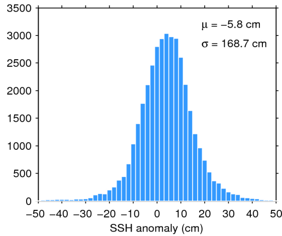
Figure 7. Histogram of flag-valid SSH anomaly over oceans and lakes for 17/11/2017. The mean ( \mu ) and standard deviation ( \sigma ) are also shown. Note that values outside [-50\ 50] cm are excluded from the histogram for the sake of readability but not from the computation of \mu and \sigma .
