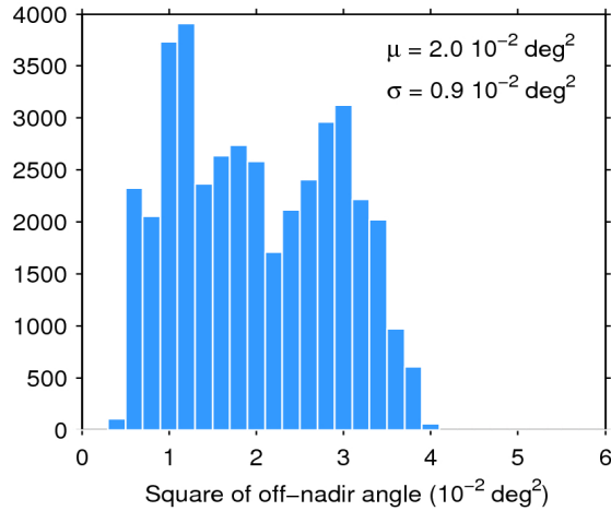
Figure 39. Histogram of flag-valid mispointing over oceans and lakes for 17/11/2017. The mean ( \mu ) and standard deviation ( \sigma ) are also shown. Note that values larger than 6 \cdot 10^{-2} \text{ deg}^2 are excluded from the histogram for the sake of readability but not from the computation of \mu and \sigma .
