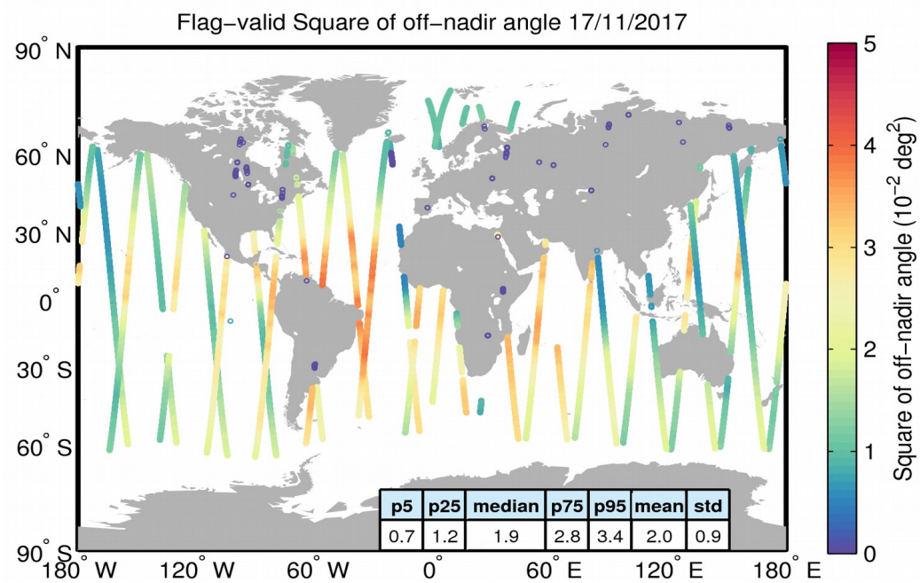
Figure 37. Geographical distribution of flag-valid mispointing data over oceans and lakes for 17/11/2017. The statistical values shown in the table refer to the mispointing in 10^{-2} deg 2 and are calculated over all measurements shown in the figure.
