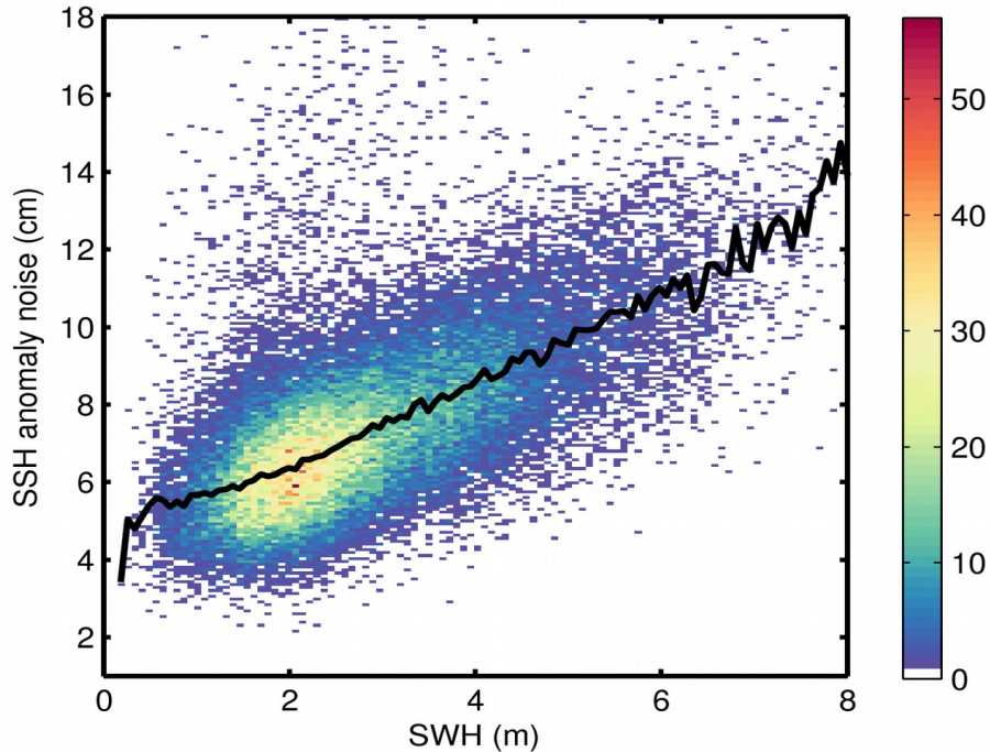
Figure 9. 2D histogram showing flag-valid SSH anomaly noise as a function of SWH for 17/11/2017. The black line denotes the median SSH anomaly noise as a function of SWH.
