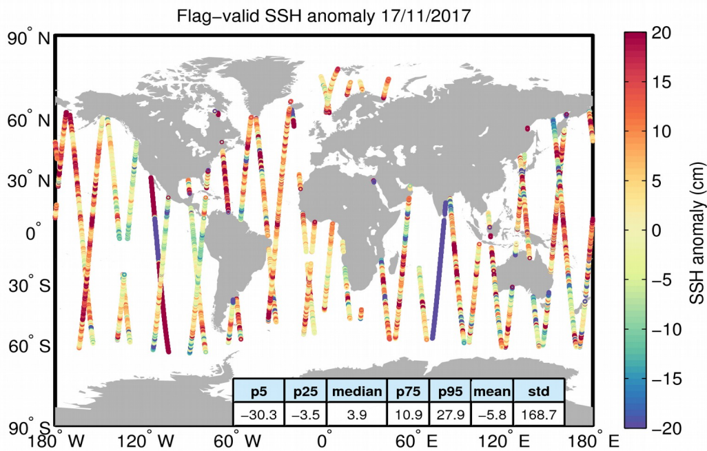
Figure 5. Geographical distribution of flag-valid 1-Hz SSH anomaly data over oceans and lakes for 17/11/2017. The statistical values shown in the table refer to the SSH anomaly in cm and are calculated over all measurements shown in the figure.
