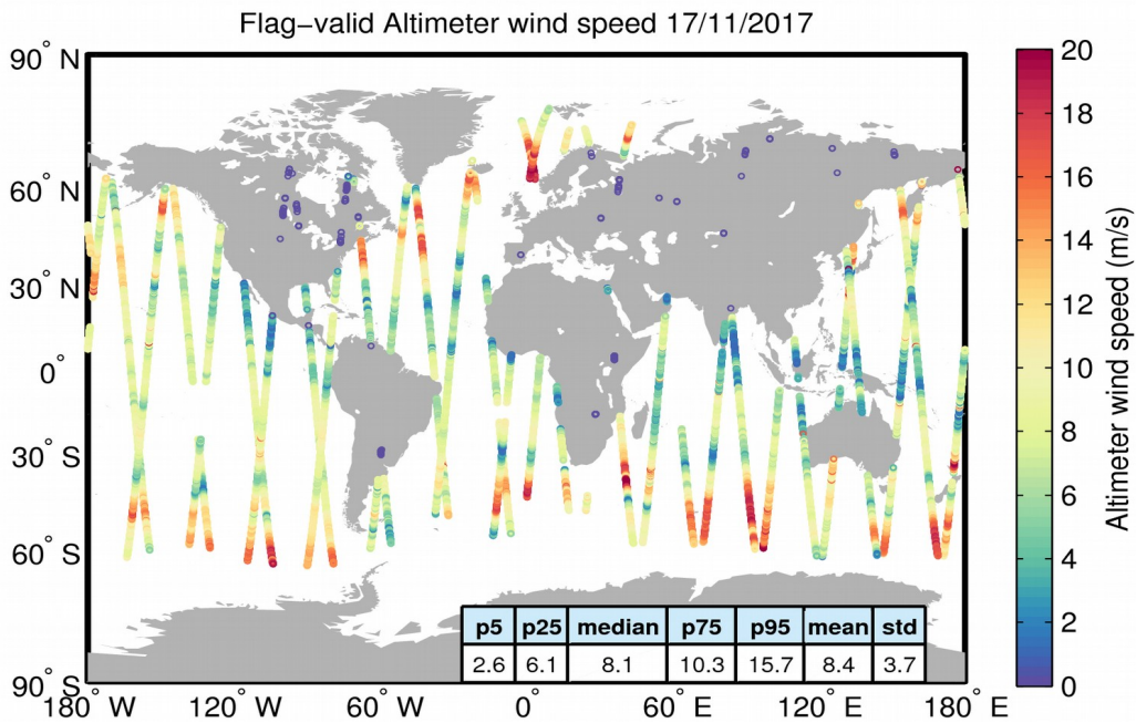
Figure 31. Geographical distribution of flag-valid wind data over oceans and lakes for 17/11/2017. The statistical values shown in the table refer to the wind in m/s and are calculated over all measurements shown in the figure.
