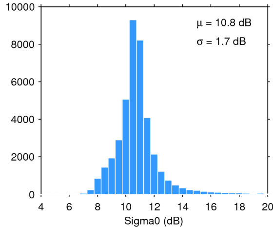
Figure 25. Histogram of flag-valid sigma0 over oceans and lakes for 17/11/2017. The mean ( \mu ) and standard deviation ( \sigma ) are also shown. Note that values outside [4 20] dB are excluded from the histogram for the sake of readability but not from the computation of \mu and \sigma .
