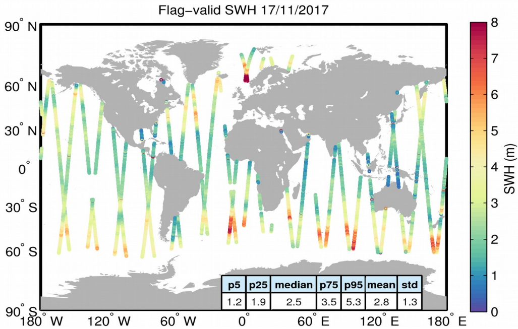
Figure 15. Geographical distribution of flag-valid SWH data over oceans and lakes for 17/11/2017. The statistical values shown in the table refer to the SWH in m and are calculated over all measurements shown in the figure.
