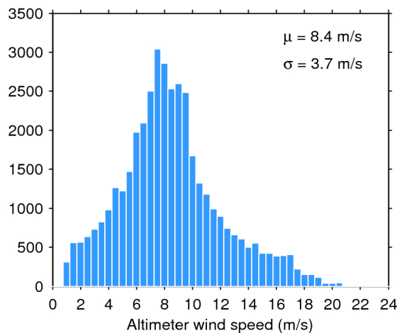
Figure 35. Histogram of science-valid wind over oceans and lakes for 17/11/2017. The mean ( \mu ) and standard deviation ( \sigma ) are also shown. Note that values larger than 24 m/s are excluded from the histogram for the sake of readability but not from the computation of \mu and \sigma .
