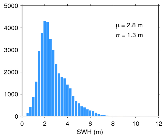
Figure 20. Histogram of science-valid SWH over oceans and lakes for 17/11/2017. The mean ( \mu ) and standard deviation ( \sigma ) are also shown. Note that values larger than 12 m are excluded from the histogram for the sake of readability but not from the computation of \mu and \sigma .
