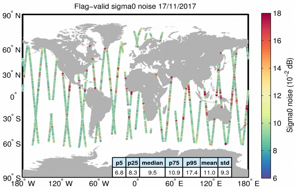
Figure 26. Geographical distribution of flag-valid 20-Hz sigma0 measurement noise over oceans and lakes for 17/11/2017. The statistical values shown in the table refer to the sigma0 noise and are calculated over all measurements shown in the figure.
