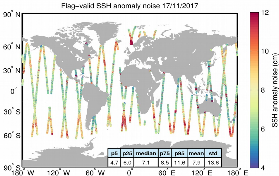
Figure 8. Geographical distribution of flag-valid 20-Hz SSH anomaly measurement noise over oceans and lakes for 17/11/2017. The statistical values shown in the table refer to the SSH anomaly noise and are calculated over all measurements shown in the figure.
