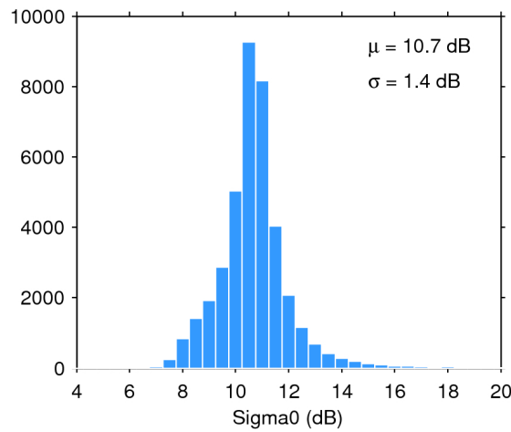
Figure 28. Histogram of science-valid sigma0 over oceans and lakes for 17/11/2017. The mean ( \mu ) and standard deviation ( \sigma ) are also shown. Note that values outside [4 20] dB are excluded from the histogram for the sake of readability but not from the computation of \mu and \sigma .
