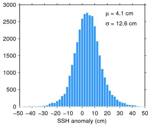
Figure 11. Histogram of science-valid SSH anomaly over oceans and lakes for 17/11/2017. The mean ( \mu ) and standard deviation ( \sigma ) are also shown. Note that values outside [-50 50] cm are excluded from the histogram for the sake of readability but not from the computation of \mu and \sigma .
