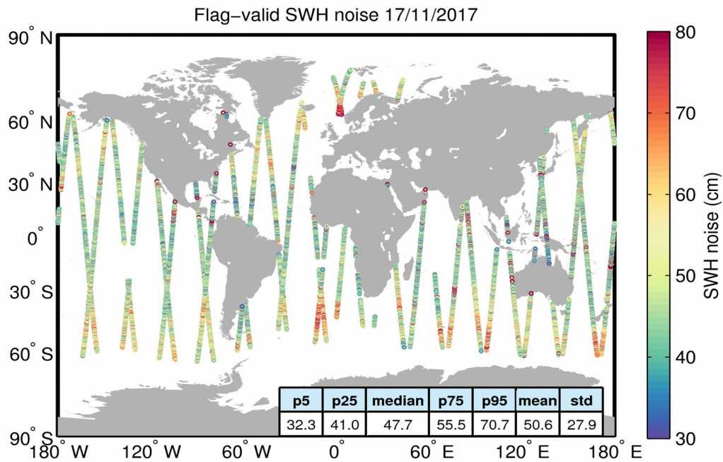
Figure 18. Geographical distribution of flag-valid 20-Hz SWH measurement noise over oceans and lakes for 17/11/2017. The statistical values shown in the table refer to the SWH noise and are calculated over all measurements shown in the figure.
