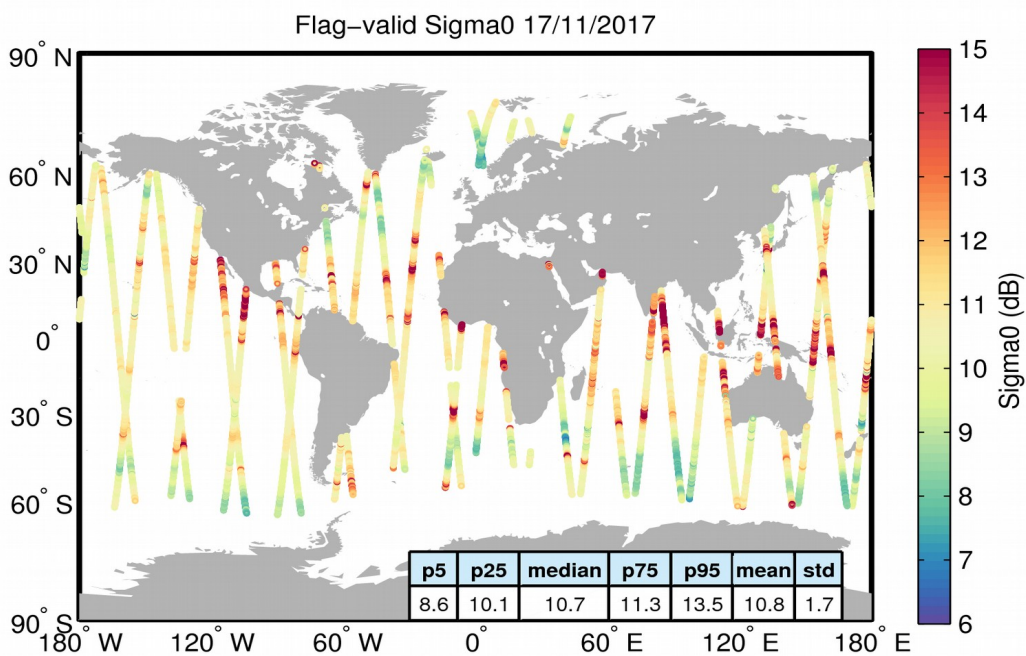
Figure 23. Geographical distribution of flag-valid sigma0 data over oceans and lakes for 17/11/2017. The statistical values shown in the table refer to the sigma0 in dB and are calculated over all measurements shown in the figure.
