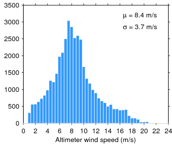
Figure 33. Histogram of flag-valid wind over oceans and lakes for 17/11/2017. The mean ( \mu ) and standard deviation ( \sigma ) are also shown. Note that values larger than 24 m/s are excluded from the histogram for the sake of readability but not from the computation of \mu and \sigma .
