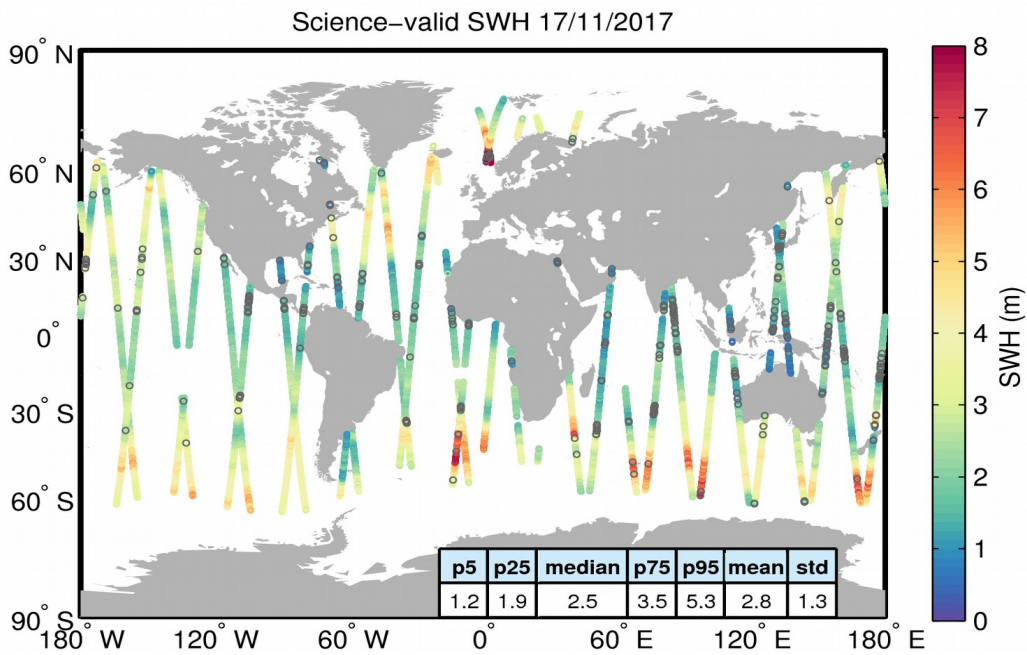
Figure 19. Geographical distribution of science-valid SWH data over oceans and lakes for 17/11/2017. The statistical values shown in the table refer to the SWH in m and are calculated over all measurements shown in the figure. Gray circles denote records that have been rejected based on the editing criteria described in Table 3.
