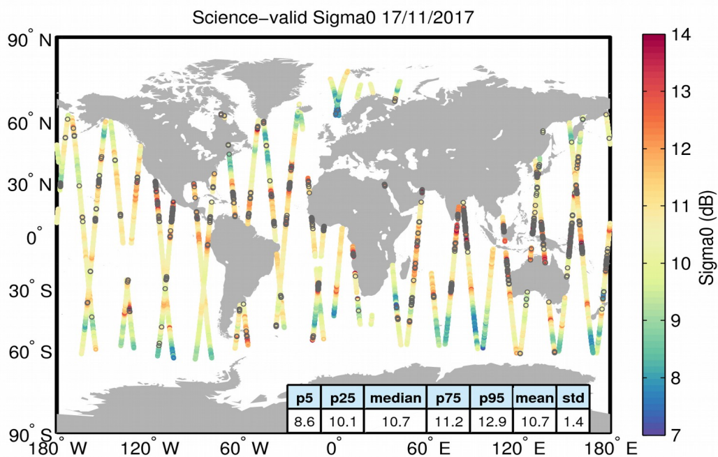
Figure 27. Geographical distribution of science-valid sigma0 data over oceans and lakes for 17/11/2017. The statistical values shown in the table refer to the sigma0 in dB and are calculated over all measurements shown in the figure. Gray circles denote records that have been rejected based on the editing criteria described in Table 4.
