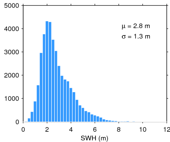
Figure 17. Histogram of flag-valid SWH over oceans and lakes for 17/11/2017. The mean ( \mu ) and standard deviation ( \sigma ) are also shown. Note that values larger than 12 m are excluded from the histogram for the sake of readability but not from the computation of \mu and \sigma .
