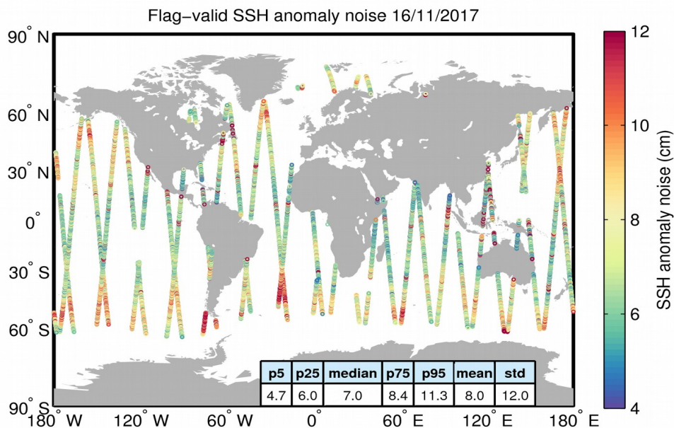
Figure 8. Geographical distribution of flag-valid 20-Hz SSH anomaly measurement noise over oceans and lakes for 16/11/2017. The statistical values shown in the table refer to the SSH anomaly noise and are calculated over all measurements shown in the figure.
