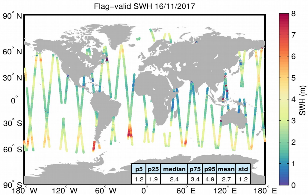
Figure 15. Geographical distribution of flag-valid SWH data over oceans and lakes for 16/11/2017. The statistical values shown in the table refer to the SWH in m and are calculated over all measurements shown in the figure.
