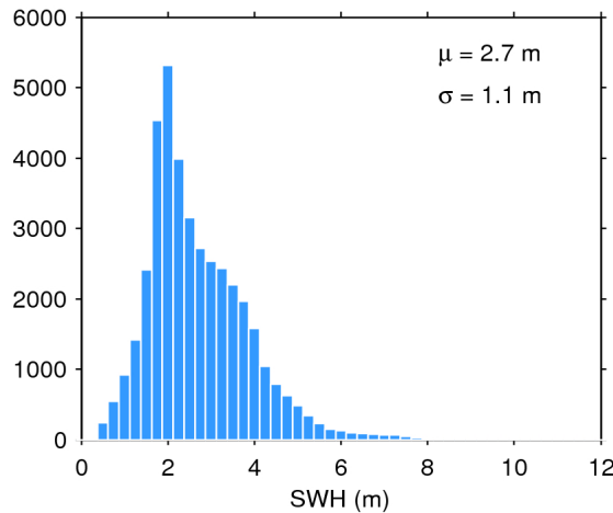
Figure 20. Histogram of science-valid SWH over oceans and lakes for 16/11/2017. The mean ( \mu ) and standard deviation ( \sigma ) are also shown. Note that values larger than 12 m are excluded from the histogram for the sake of readability but not from the computation of \mu and \sigma .
