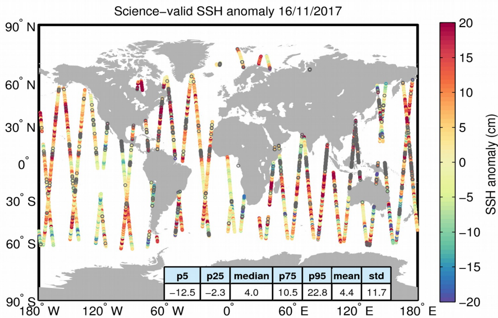
Figure 10. Geographical distribution of science-valid SSH anomaly data over oceans and lakes for 16/11/2017. The statistical values shown in the table refer to the SSH anomaly in cm and are calculated over all measurements shown in the figure. Gray circles denote records that have been rejected based on the editing criteria described in Table 2.
