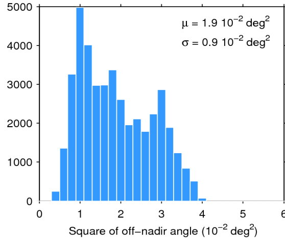
Figure 39. Histogram of flag-valid mispointing over oceans and lakes for 16/11/2017. The mean ( \mu ) and standard deviation ( \sigma ) are also shown. Note that values larger than 6 \cdot 10^{-2} \text{ deg}^2 are excluded from the histogram for the sake of readability but not from the computation of \mu and \sigma .
