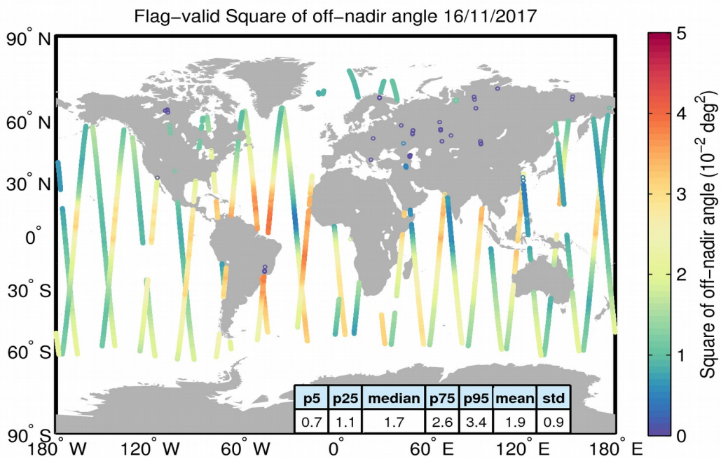
Figure 37. Geographical distribution of flag-valid mispointing data over oceans and lakes for 16/11/2017. The statistical values shown in the table refer to the mispointing in 10^{-2} deg 2 and are calculated over all measurements shown in the figure.
