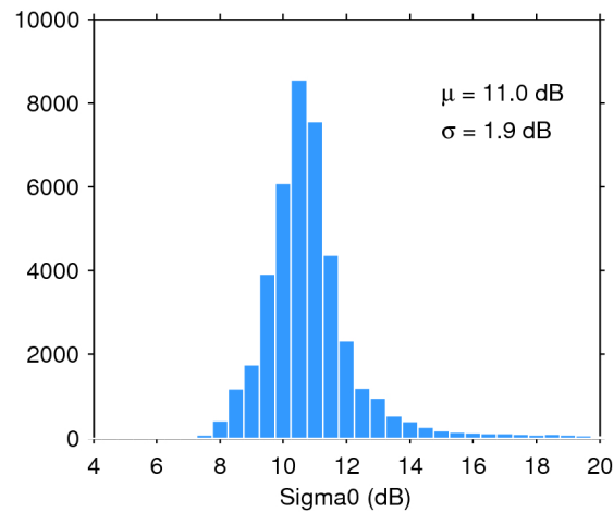
Figure 25. Histogram of flag-valid sigma0 over oceans and lakes for 16/11/2017. The mean ( \mu ) and standard deviation ( \sigma ) are also shown. Note that values outside [4 20] dB are excluded from the histogram for the sake of readability but not from the computation of \mu and \sigma .
