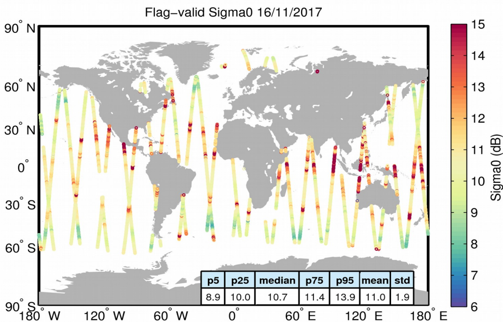
Figure 23. Geographical distribution of flag-valid sigma0 data over oceans and lakes for 16/11/2017. The statistical values shown in the table refer to the sigma0 in dB and are calculated over all measurements shown in the figure.
