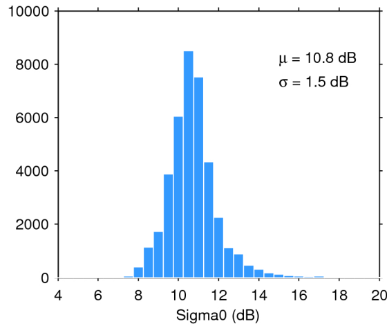
Figure 28. Histogram of science-valid sigma0 over oceans and lakes for 16/11/2017. The mean ( \mu ) and standard deviation ( \sigma ) are also shown. Note that values outside [4 20] dB are excluded from the histogram for the sake of readability but not from the computation of \mu and \sigma .
