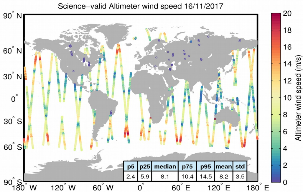
Figure 34. Geographical distribution of science-valid wind data over oceans and lakes for 16/11/2017. The statistical values shown in the table refer to the wind in m/s and are calculated over all measurements shown in the figure. Gray circles denote records that have been rejected based on the editing criteria described in Table 5.
