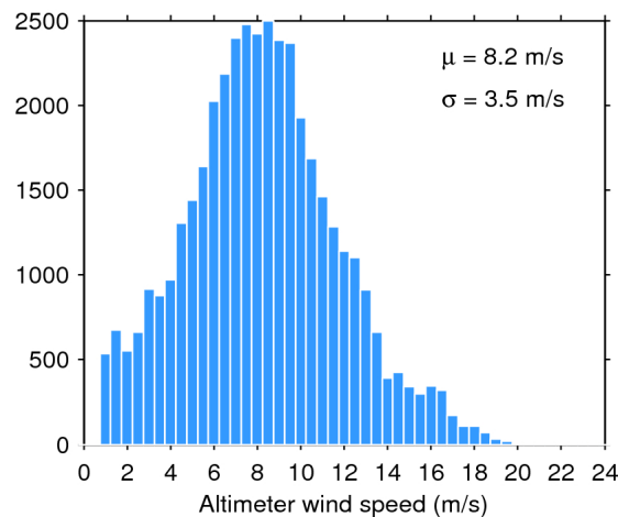
Figure 35. Histogram of science-valid wind over oceans and lakes for 16/11/2017. The mean ( \mu ) and standard deviation ( \sigma ) are also shown. Note that values larger than 24 m/s are excluded from the histogram for the sake of readability but not from the computation of \mu and \sigma .
