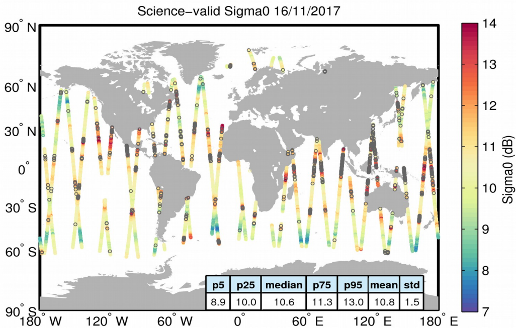
Figure 27. Geographical distribution of science-valid sigma0 data over oceans and lakes for 16/11/2017. The statistical values shown in the table refer to the sigma0 in dB and are calculated over all measurements shown in the figure. Gray circles denote records that have been rejected based on the editing criteria described in Table 4.
