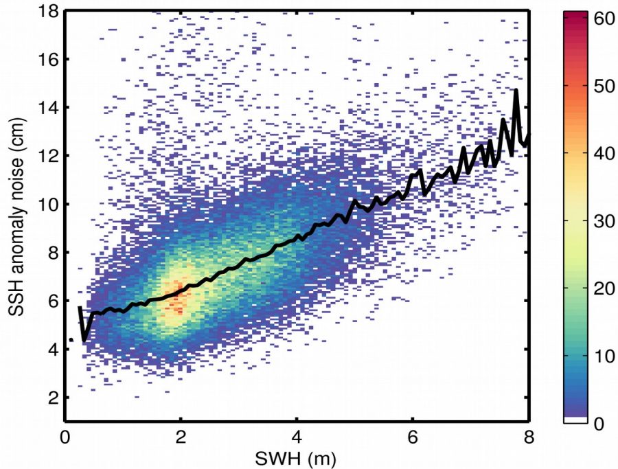
Figure 9. 2D histogram showing flag-valid SSH anomaly noise as a function of SWH for 16/11/2017. The black line denotes the median SSH anomaly noise as a function of SWH.
