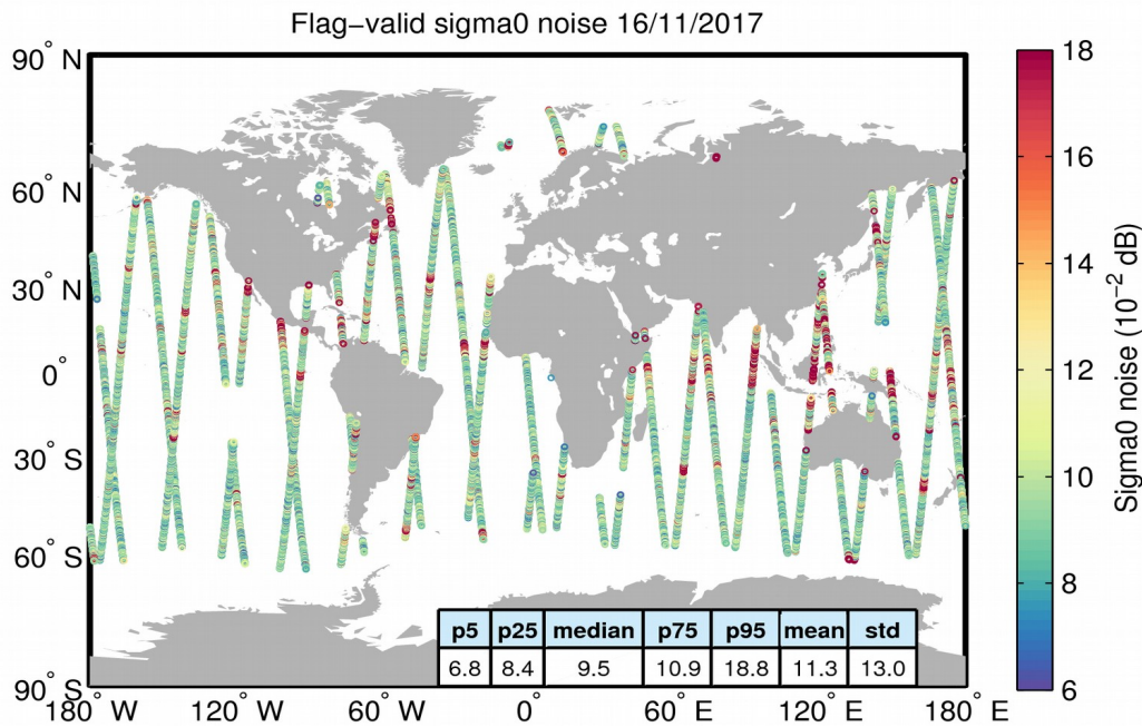
Figure 26. Geographical distribution of flag-valid 20-Hz sigma0 measurement noise over oceans and lakes for 16/11/2017. The statistical values shown in the table refer to the sigma0 noise and are calculated over all measurements shown in the figure.
