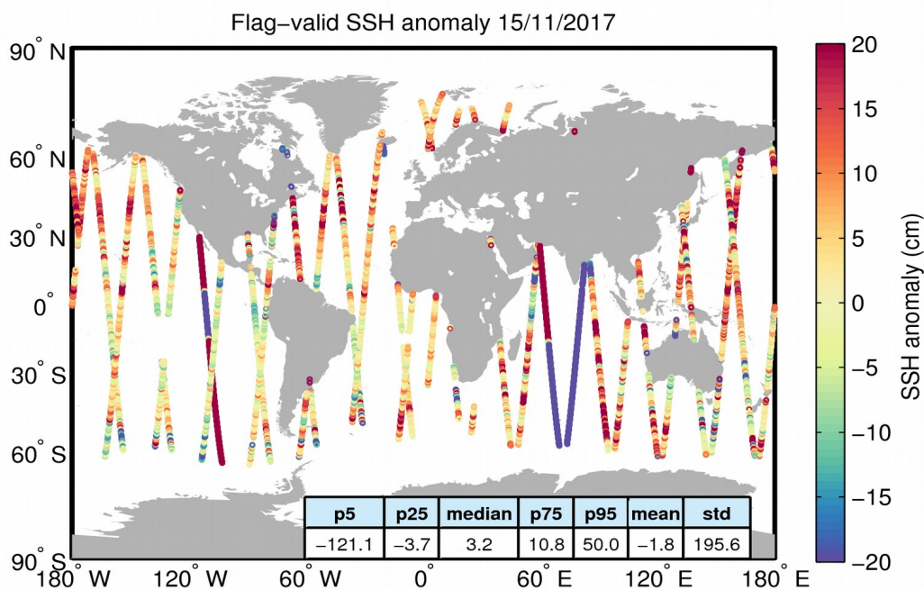
Figure 5. Geographical distribution of flag-valid 1-Hz SSH anomaly data over oceans and lakes for 15/11/2017. The statistical values shown in the table refer to the SSH anomaly in cm and are calculated over all measurements shown in the figure.
