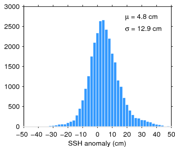
Figure 11. Histogram of science-valid SSH anomaly over oceans and lakes for 15/11/2017. The mean ( \mu ) and standard deviation ( \sigma ) are also shown. Note that values outside [-50 50] cm are excluded from the histogram for the sake of readability but not from the computation of \mu and \sigma .
