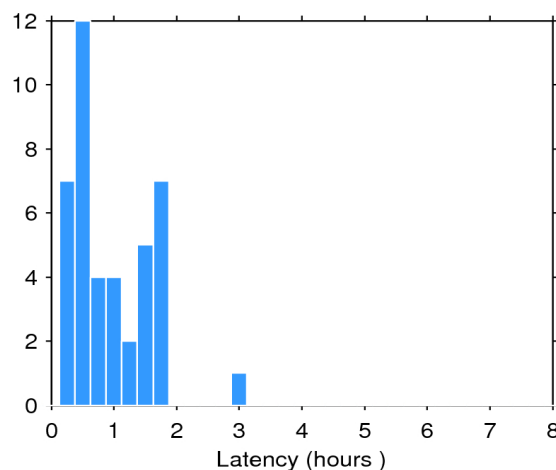
Figure 2. Histogram of the data latency for 15/11/2017. The y-axis denotes the number of files that are made available with a delay of x-hours with respect to the mean time of the records stored in the file.
