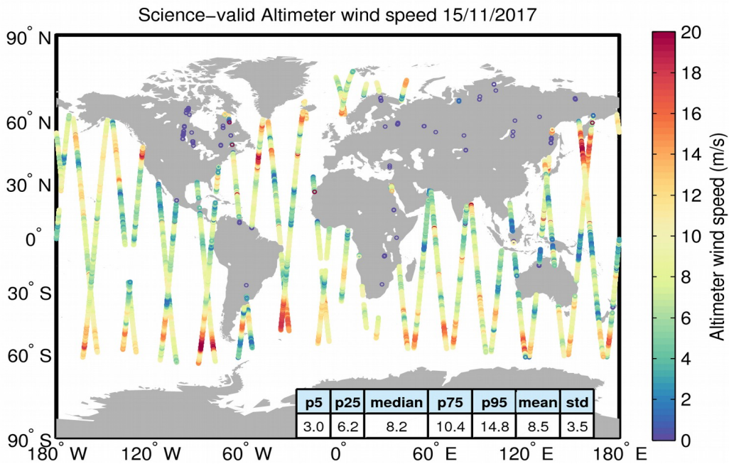
Figure 34. Geographical distribution of science-valid wind data over oceans and lakes for 15/11/2017. The statistical values shown in the table refer to the wind in m/s and are calculated over all measurements shown in the figure. Gray circles denote records that have been rejected based on the editing criteria described in Table 5.
