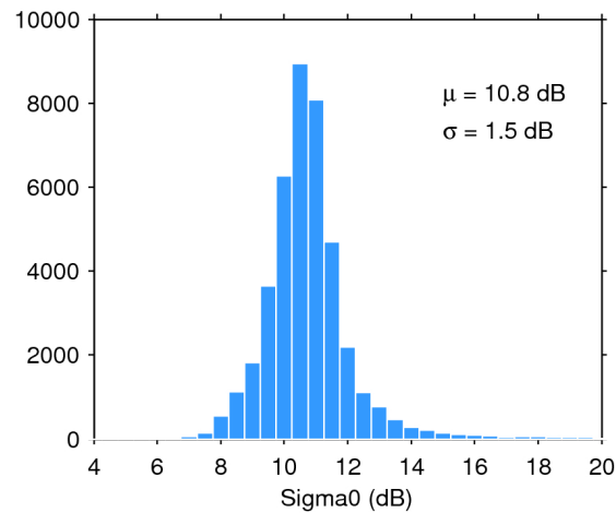
Figure 25. Histogram of flag-valid sigma0 over oceans and lakes for 15/11/2017. The mean ( \mu ) and standard deviation ( \sigma ) are also shown. Note that values outside [4 20] dB are excluded from the histogram for the sake of readability but not from the computation of \mu and \sigma .
