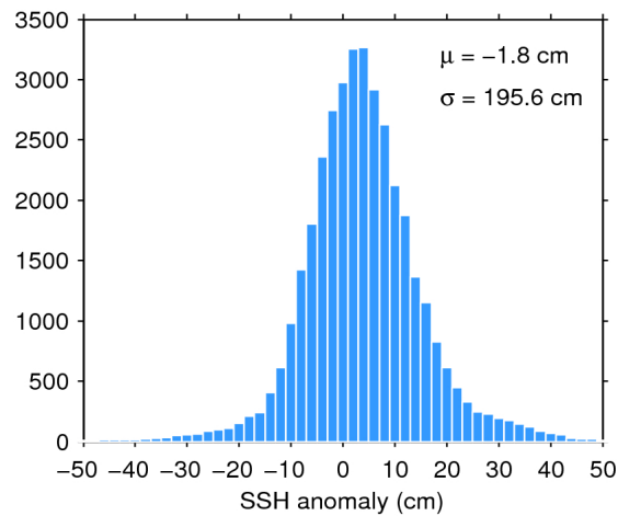
Figure 7. Histogram of flag-valid SSH anomaly over oceans and lakes for 15/11/2017. The mean ( \mu ) and standard deviation ( \sigma ) are also shown. Note that values outside [-50 50] cm are excluded from the histogram for the sake of readability but not from the computation of \mu and \sigma .
