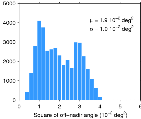
Figure 39. Histogram of flag-valid mispointing over oceans and lakes for 15/11/2017. The mean ( \mu ) and standard deviation ( \sigma ) are also shown. Note that values larger than 6 \cdot 10^{-2} \text{ deg}^2 are excluded from the histogram for the sake of readability but not from the computation of \mu and \sigma .
