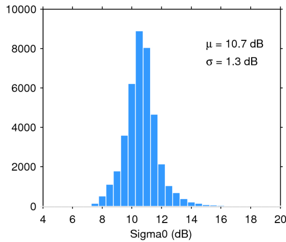
Figure 28. Histogram of science-valid sigma0 over oceans and lakes for 15/11/2017. The mean ( \mu ) and standard deviation ( \sigma ) are also shown. Note that values outside [4 20] dB are excluded from the histogram for the sake of readability but not from the computation of \mu and \sigma .
