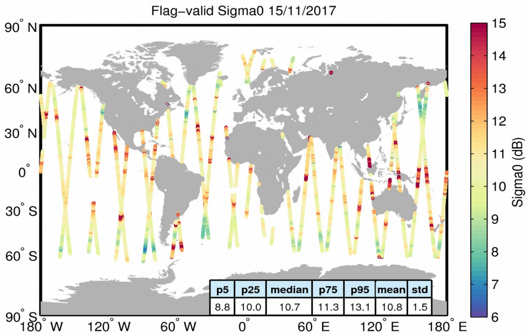
Figure 23. Geographical distribution of flag-valid sigma0 data over oceans and lakes for 15/11/2017. The statistical values shown in the table refer to the sigma0 in dB and are calculated over all measurements shown in the figure.
