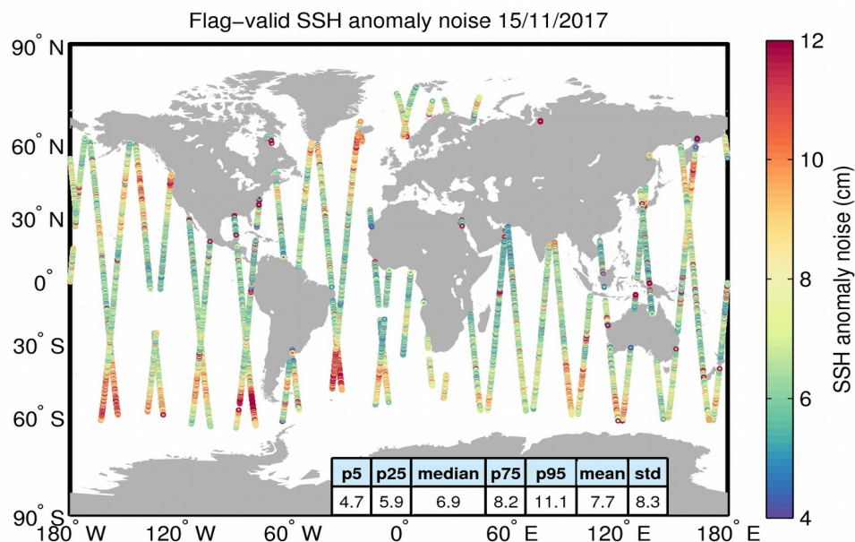
Figure 8. Geographical distribution of flag-valid 20-Hz SSH anomaly measurement noise over oceans and lakes for 15/11/2017. The statistical values shown in the table refer to the SSH anomaly noise and are calculated over all measurements shown in the figure.
