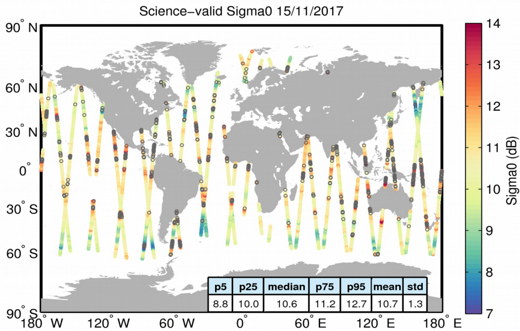
Figure 27. Geographical distribution of science-valid sigma0 data over oceans and lakes for 15/11/2017. The statistical values shown in the table refer to the sigma0 in dB and are calculated over all measurements shown in the figure. Gray circles denote records that have been rejected based on the editing criteria described in Table 4.
