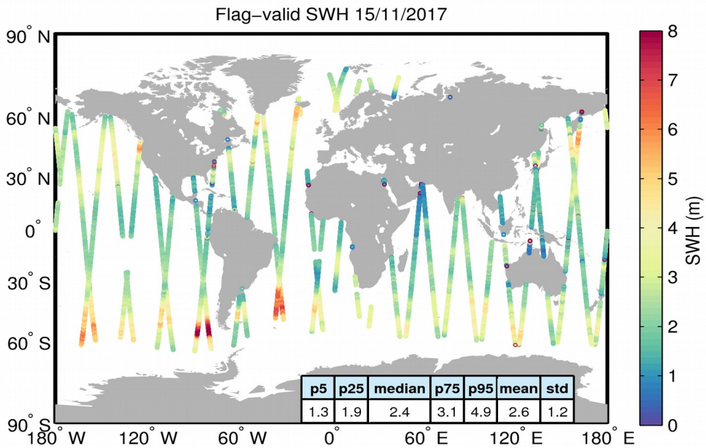
Figure 15. Geographical distribution of flag-valid SWH data over oceans and lakes for 15/11/2017. The statistical values shown in the table refer to the SWH in m and are calculated over all measurements shown in the figure.
