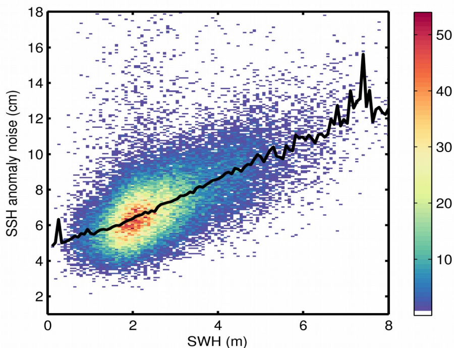
Figure 9. 2D histogram showing flag-valid SSH anomaly noise as a function of SWH for 15/11/2017. The black line denotes the median SSH anomaly noise as a function of SWH.
