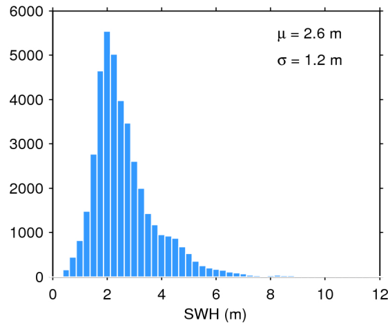
Figure 17. Histogram of flag-valid SWH over oceans and lakes for 15/11/2017. The mean ( \mu ) and standard deviation ( \sigma ) are also shown. Note that values larger than 12 m are excluded from the histogram for the sake of readability but not from the computation of \mu and \sigma .
