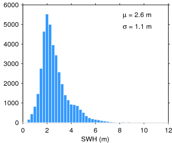
Figure 20. Histogram of science-valid SWH over oceans and lakes for 15/11/2017. The mean ( \mu ) and standard deviation ( \sigma ) are also shown. Note that values larger than 12 m are excluded from the histogram for the sake of readability but not from the computation of \mu and \sigma .
