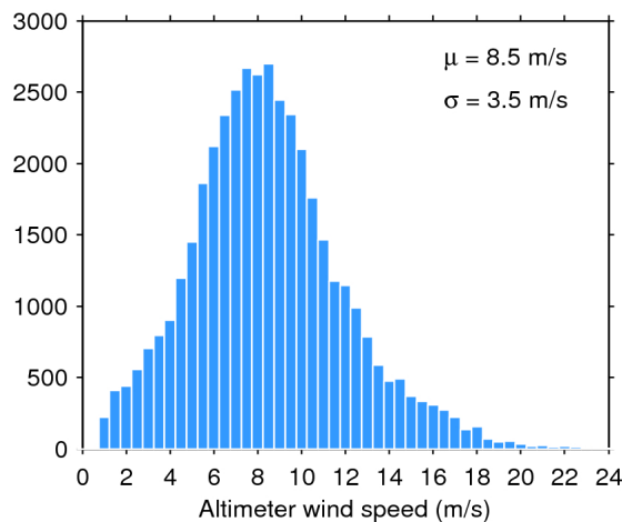
Figure 35. Histogram of science-valid wind over oceans and lakes for 15/11/2017. The mean ( \mu ) and standard deviation ( \sigma ) are also shown. Note that values larger than 24 m/s are excluded from the histogram for the sake of readability but not from the computation of \mu and \sigma .
