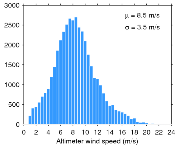
Figure 33. Histogram of flag-valid wind over oceans and lakes for 15/11/2017. The mean ( \mu ) and standard deviation ( \sigma ) are also shown. Note that values larger than 24 m/s are excluded from the histogram for the sake of readability but not from the computation of \mu and \sigma .
