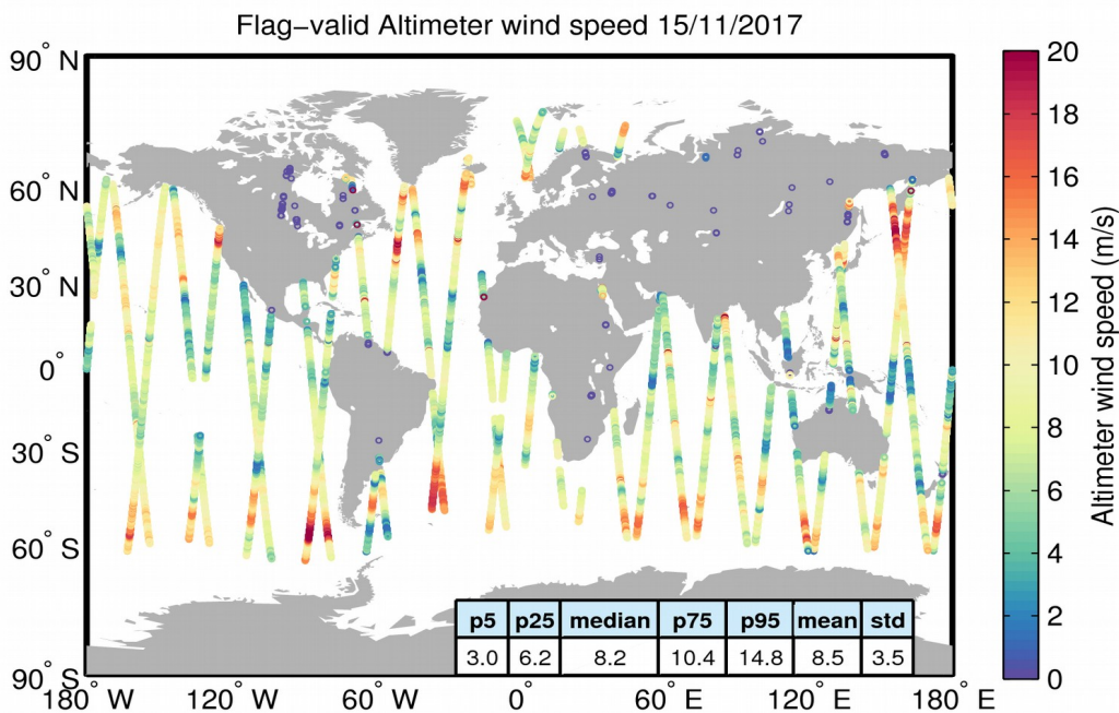
Figure 31. Geographical distribution of flag-valid wind data over oceans and lakes for 15/11/2017. The statistical values shown in the table refer to the wind in m/s and are calculated over all measurements shown in the figure.
