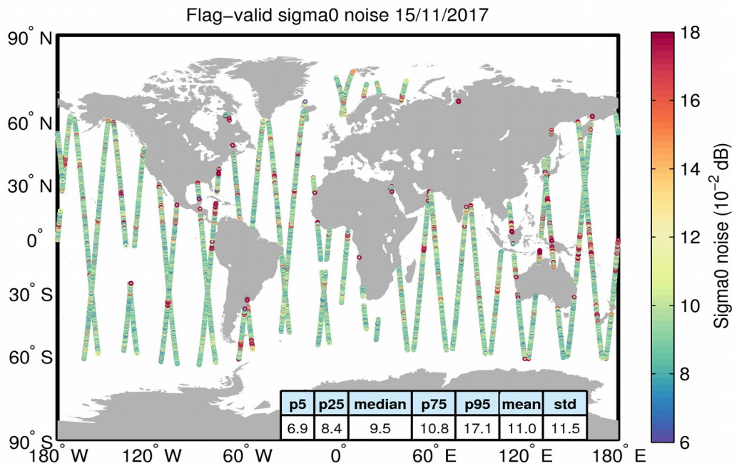
Figure 26. Geographical distribution of flag-valid 20-Hz sigma0 measurement noise over oceans and lakes for 15/11/2017. The statistical values shown in the table refer to the sigma0 noise and are calculated over all measurements shown in the figure.
