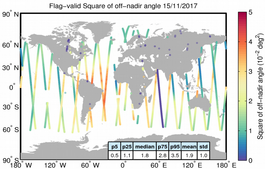
Figure 37. Geographical distribution of flag-valid mispointing data over oceans and lakes for 15/11/2017. The statistical values shown in the table refer to the mispointing in 10^{-2} deg 2 and are calculated over all measurements shown in the figure.
