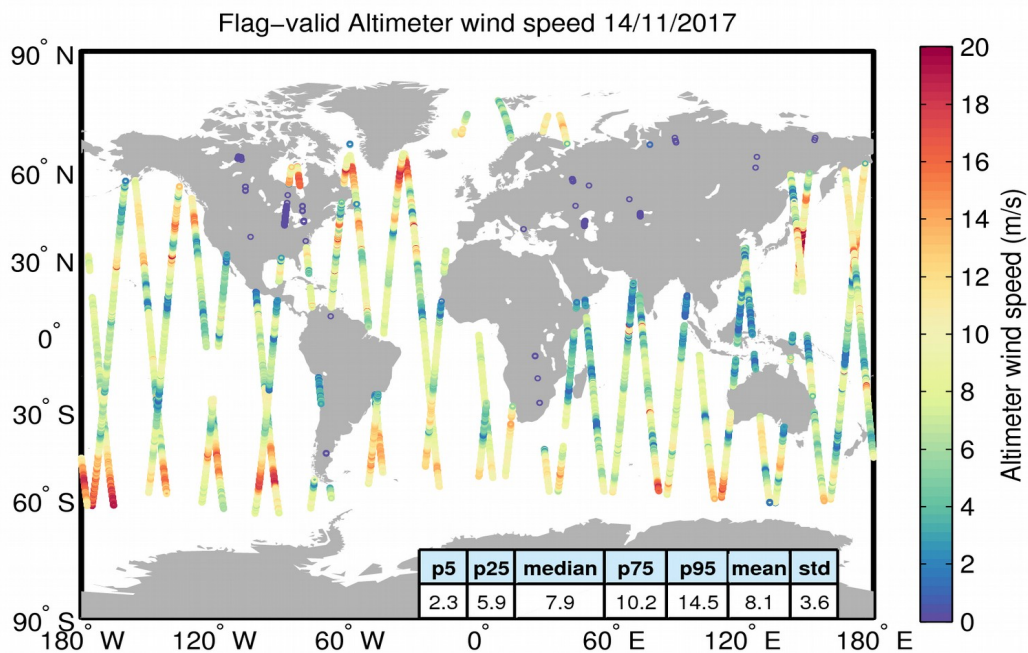
Figure 31. Geographical distribution of flag-valid wind data over oceans and lakes for 14/11/2017. The statistical values shown in the table refer to the wind in m/s and are calculated over all measurements shown in the figure.
