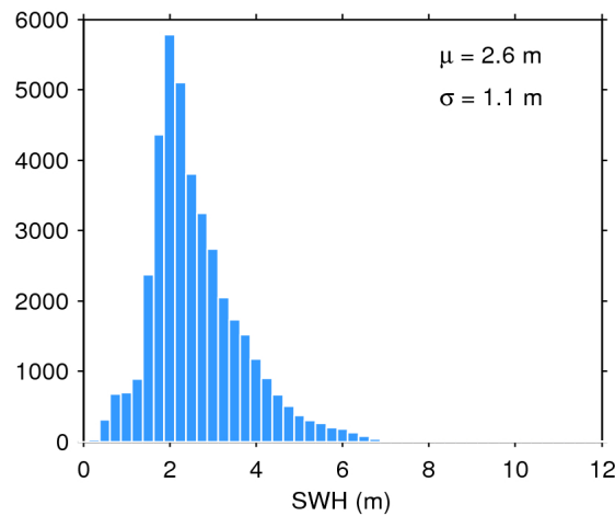
Figure 17. Histogram of flag-valid SWH over oceans and lakes for 14/11/2017. The mean ( \mu ) and standard deviation ( \sigma ) are also shown. Note that values larger than 12 m are excluded from the histogram for the sake of readability but not from the computation of \mu and \sigma .
