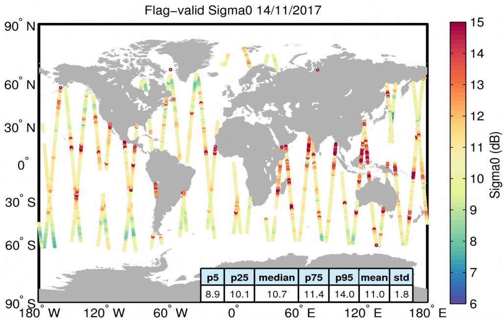
Figure 23. Geographical distribution of flag-valid sigma0 data over oceans and lakes for 14/11/2017. The statistical values shown in the table refer to the sigma0 in dB and are calculated over all measurements shown in the figure.
