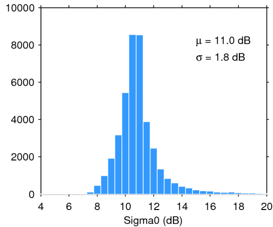
Figure 25. Histogram of flag-valid sigma0 over oceans and lakes for 14/11/2017. The mean ( \mu ) and standard deviation ( \sigma ) are also shown. Note that values outside [4 20] dB are excluded from the histogram for the sake of readability but not from the computation of \mu and \sigma .
