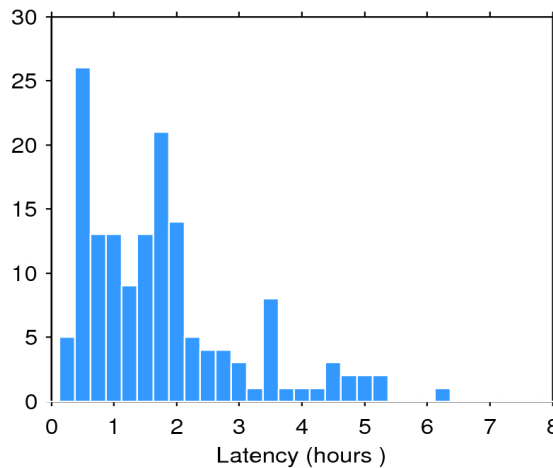
Figure 2. Histogram of the data latency for 14/11/2017. The y-axis denotes the number of files that are made available with a delay of x-hours with respect to the mean time of the records stored in the file.
