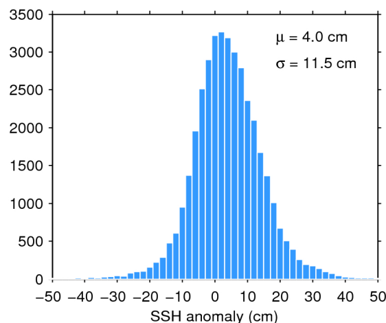
Figure 11. Histogram of science-valid SSH anomaly over oceans and lakes for 14/11/2017. The mean ( \mu ) and standard deviation ( \sigma ) are also shown. Note that values outside [-50 50] cm are excluded from the histogram for the sake of readability but not from the computation of \mu and \sigma .
