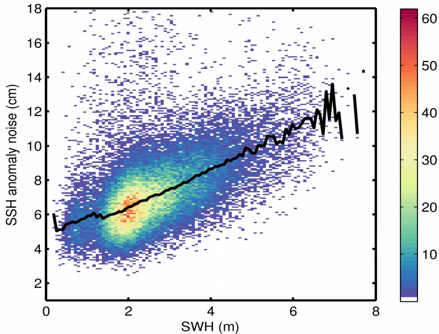
Figure 9. 2D histogram showing flag-valid SSH anomaly noise as a function of SWH for 14/11/2017. The black line denotes the median SSH anomaly noise as a function of SWH.
