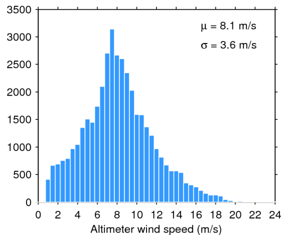
Figure 35. Histogram of science-valid wind over oceans and lakes for 14/11/2017. The mean ( \mu ) and standard deviation ( \sigma ) are also shown. Note that values larger than 24 m/s are excluded from the histogram for the sake of readability but not from the computation of \mu and \sigma .
