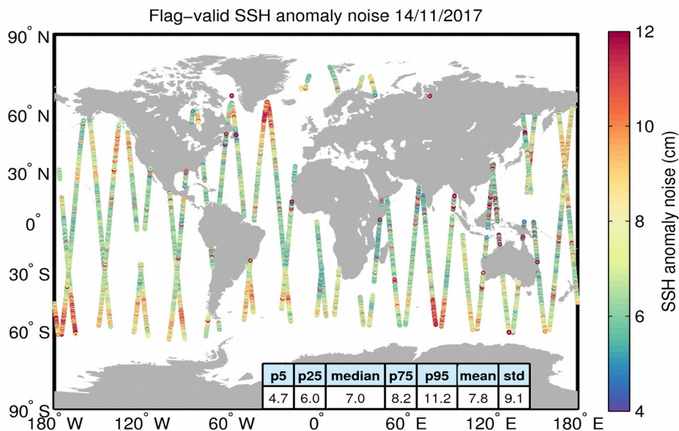
Figure 8. Geographical distribution of flag-valid 20-Hz SSH anomaly measurement noise over oceans and lakes for 14/11/2017. The statistical values shown in the table refer to the SSH anomaly noise and are calculated over all measurements shown in the figure.
