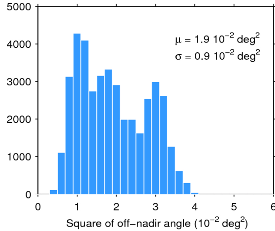
Figure 39. Histogram of flag-valid mispointing over oceans and lakes for 14/11/2017. The mean ( \mu ) and standard deviation ( \sigma ) are also shown. Note that values larger than 6 \cdot 10^{-2} \text{ deg}^2 are excluded from the histogram for the sake of readability but not from the computation of \mu and \sigma .
