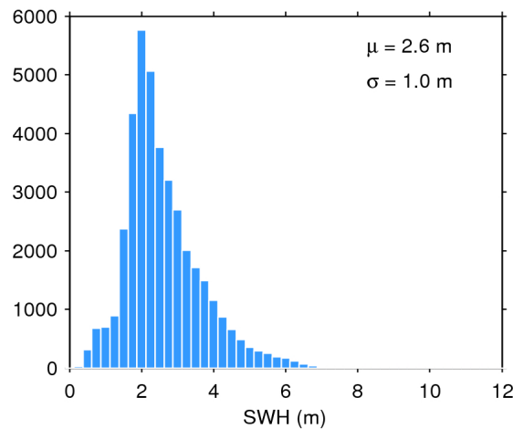
Figure 20. Histogram of science-valid SWH over oceans and lakes for 14/11/2017. The mean ( \mu ) and standard deviation ( \sigma ) are also shown. Note that values larger than 12 m are excluded from the histogram for the sake of readability but not from the computation of \mu and \sigma .
