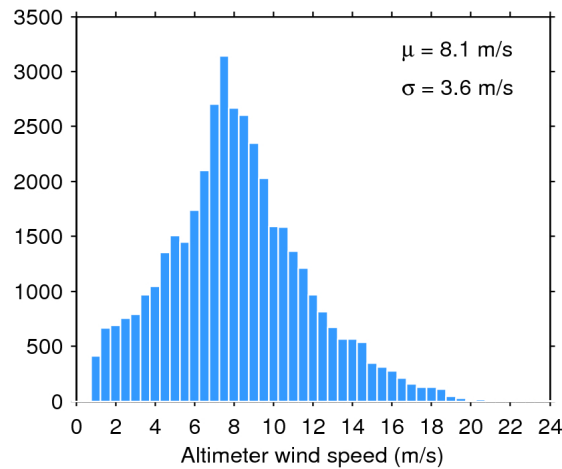
Figure 33. Histogram of flag-valid wind over oceans and lakes for 14/11/2017. The mean ( \mu ) and standard deviation ( \sigma ) are also shown. Note that values larger than 24 m/s are excluded from the histogram for the sake of readability but not from the computation of \mu and \sigma .
