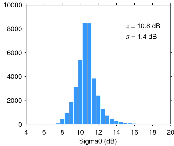
Figure 28. Histogram of science-valid sigma0 over oceans and lakes for 14/11/2017. The mean ( \mu ) and standard deviation ( \sigma ) are also shown. Note that values outside [4 20] dB are excluded from the histogram for the sake of readability but not from the computation of \mu and \sigma .
