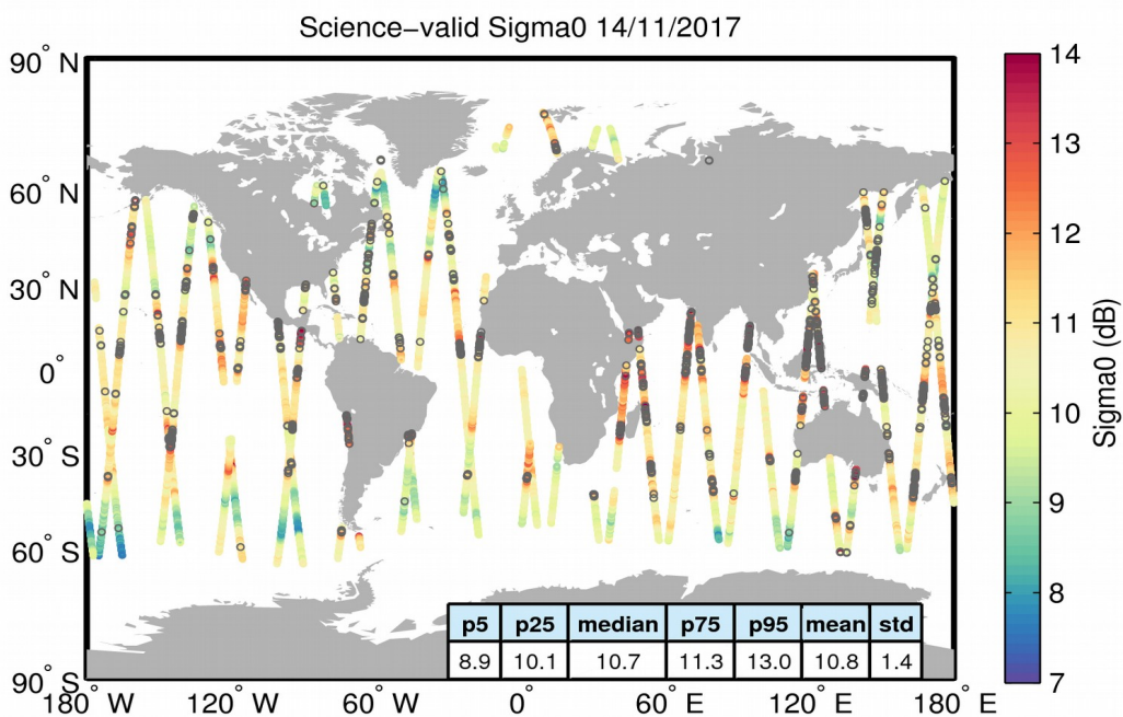
Figure 27. Geographical distribution of science-valid sigma0 data over oceans and lakes for 14/11/2017. The statistical values shown in the table refer to the sigma0 in dB and are calculated over all measurements shown in the figure. Gray circles denote records that have been rejected based on the editing criteria described in Table 4.
