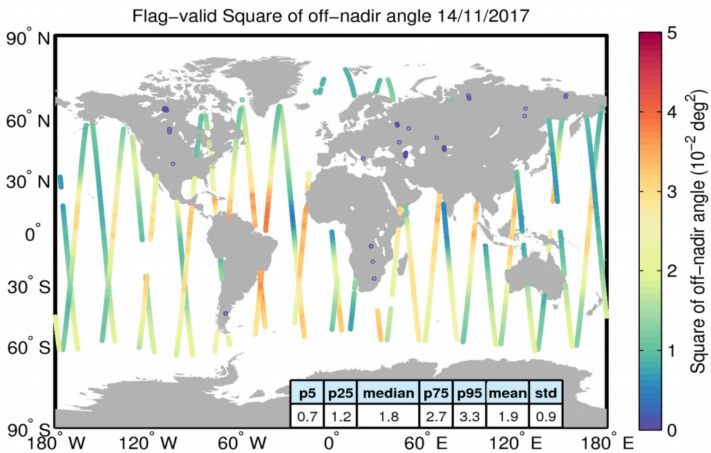
Figure 37. Geographical distribution of flag-valid mispointing data over oceans and lakes for 14/11/2017. The statistical values shown in the table refer to the mispointing in 10^{-2} deg 2 and are calculated over all measurements shown in the figure.
