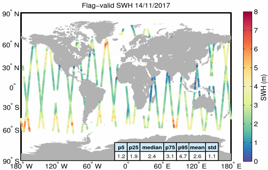
Figure 15. Geographical distribution of flag-valid SWH data over oceans and lakes for 14/11/2017. The statistical values shown in the table refer to the SWH in m and are calculated over all measurements shown in the figure.
