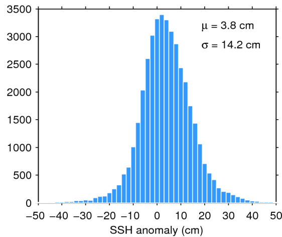
Figure 7. Histogram of flag-valid SSH anomaly over oceans and lakes for 14/11/2017. The mean ( \mu ) and standard deviation ( \sigma ) are also shown. Note that values outside [-50 50] cm are excluded from the histogram for the sake of readability but not from the computation of \mu and \sigma .
