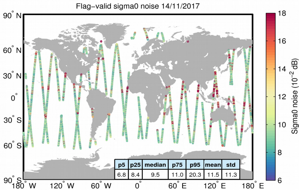
Figure 26. Geographical distribution of flag-valid 20-Hz sigma0 measurement noise over oceans and lakes for 14/11/2017. The statistical values shown in the table refer to the sigma0 noise and are calculated over all measurements shown in the figure.
