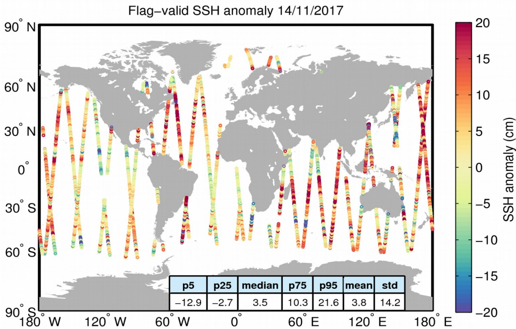
Figure 5. Geographical distribution of flag-valid 1-Hz SSH anomaly data over oceans and lakes for 14/11/2017. The statistical values shown in the table refer to the SSH anomaly in cm and are calculated over all measurements shown in the figure.
