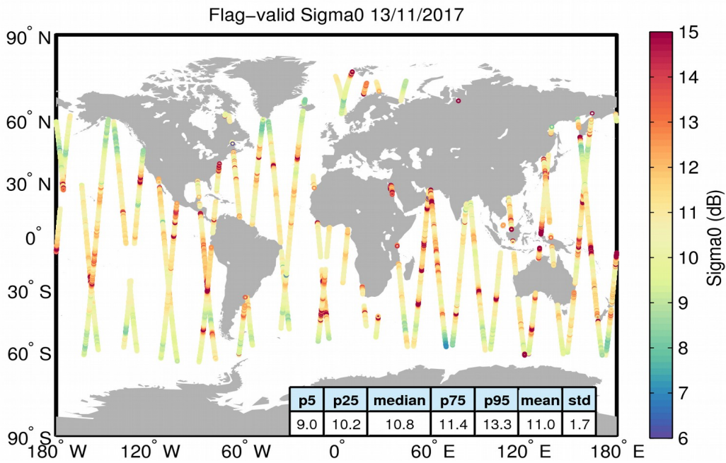
Figure 23. Geographical distribution of flag-valid sigma0 data over oceans and lakes for 13/11/2017. The statistical values shown in the table refer to the sigma0 in dB and are calculated over all measurements shown in the figure.
