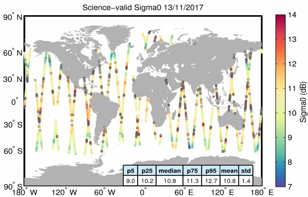
Figure 27. Geographical distribution of science-valid sigma0 data over oceans and lakes for 13/11/2017. The statistical values shown in the table refer to the sigma0 in dB and are calculated over all measurements shown in the figure. Gray circles denote records that have been rejected based on the editing criteria described in Table 4.
