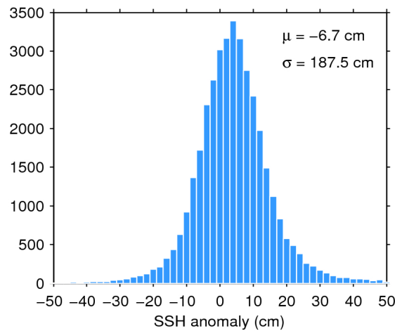
Figure 7. Histogram of flag-valid SSH anomaly over oceans and lakes for 13/11/2017. The mean ( \mu ) and standard deviation ( \sigma ) are also shown. Note that values outside [-50 50] cm are excluded from the histogram for the sake of readability but not from the computation of \mu and \sigma .
