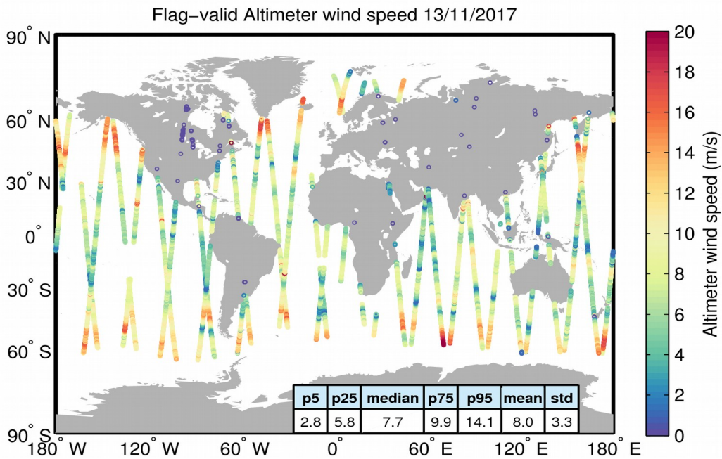
Figure 31. Geographical distribution of flag-valid wind data over oceans and lakes for 13/11/2017. The statistical values shown in the table refer to the wind in m/s and are calculated over all measurements shown in the figure.
