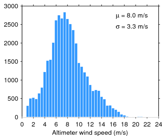
Figure 35. Histogram of science-valid wind over oceans and lakes for 13/11/2017. The mean ( \mu ) and standard deviation ( \sigma ) are also shown. Note that values larger than 24 m/s are excluded from the histogram for the sake of readability but not from the computation of \mu and \sigma .
