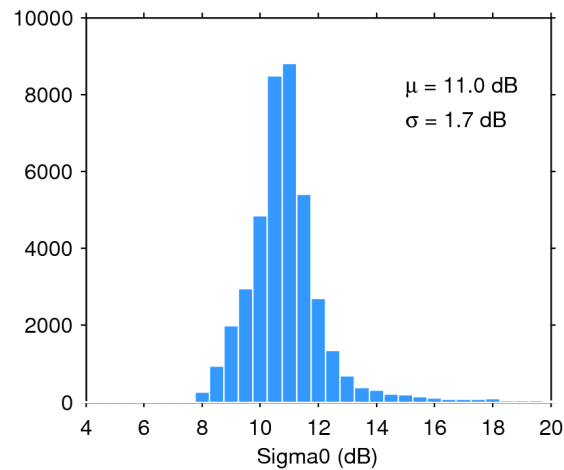
Figure 25. Histogram of flag-valid sigma0 over oceans and lakes for 13/11/2017. The mean ( \mu ) and standard deviation ( \sigma ) are also shown. Note that values outside [4 20] dB are excluded from the histogram for the sake of readability but not from the computation of \mu and \sigma .
