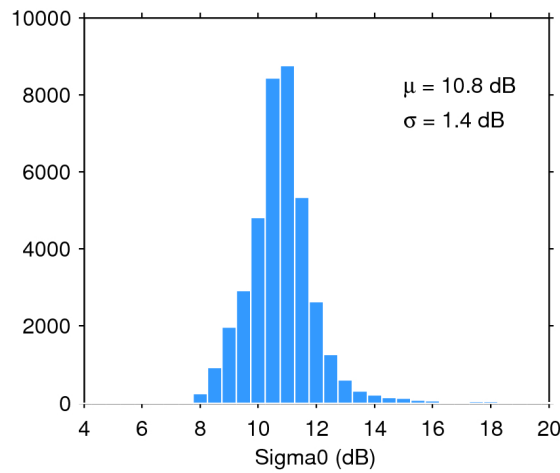
Figure 28. Histogram of science-valid sigma0 over oceans and lakes for 13/11/2017. The mean ( \mu ) and standard deviation ( \sigma ) are also shown. Note that values outside [4 20] dB are excluded from the histogram for the sake of readability but not from the computation of \mu and \sigma .
