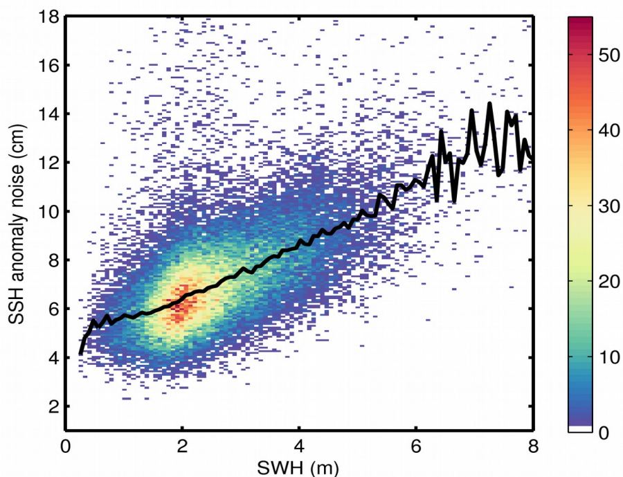
Figure 9. 2D histogram showing flag-valid SSH anomaly noise as a function of SWH for 13/11/2017. The black line denotes the median SSH anomaly noise as a function of SWH.
