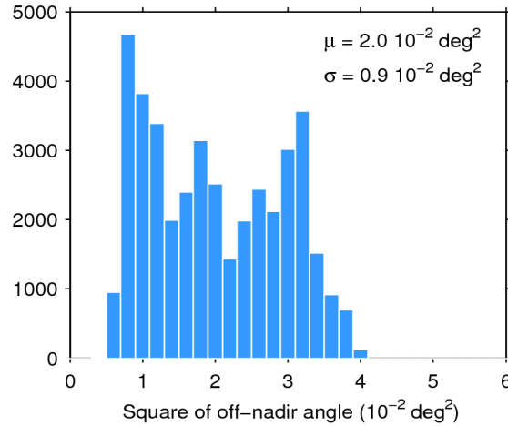
Figure 39. Histogram of flag-valid mispointing over oceans and lakes for 13/11/2017. The mean ( \mu ) and standard deviation ( \sigma ) are also shown. Note that values larger than 6 \cdot 10^{-2} \text{ deg}^2 are excluded from the histogram for the sake of readability but not from the computation of \mu and \sigma .
