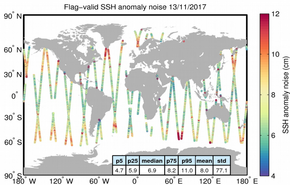
Figure 8. Geographical distribution of flag-valid 20-Hz SSH anomaly measurement noise over oceans and lakes for 13/11/2017. The statistical values shown in the table refer to the SSH anomaly noise and are calculated over all measurements shown in the figure.
