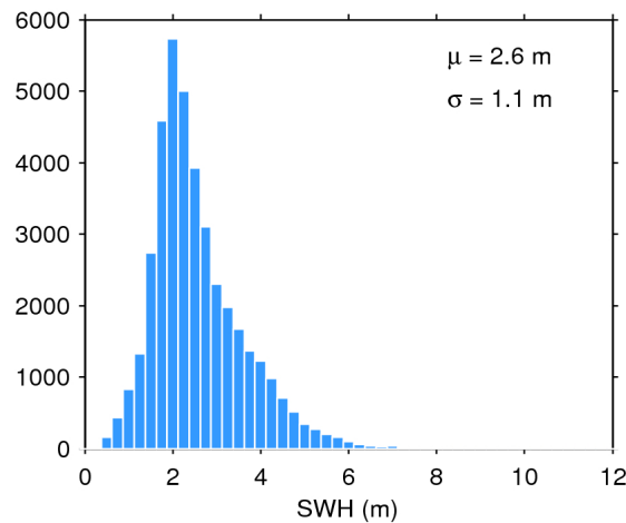
Figure 20. Histogram of science-valid SWH over oceans and lakes for 13/11/2017. The mean ( \mu ) and standard deviation ( \sigma ) are also shown. Note that values larger than 12 m are excluded from the histogram for the sake of readability but not from the computation of \mu and \sigma .
