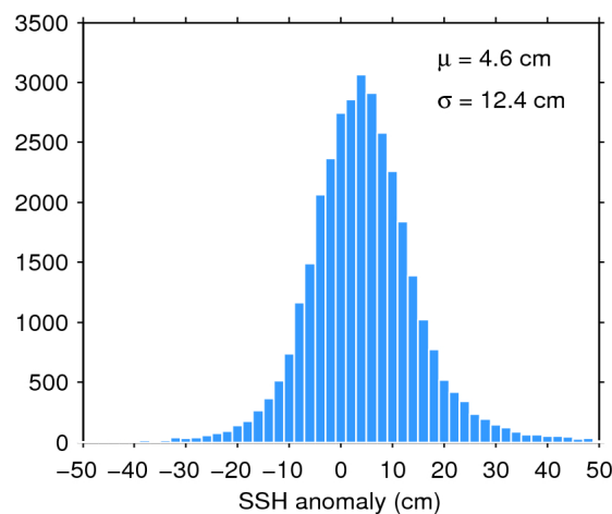
Figure 11. Histogram of science-valid SSH anomaly over oceans and lakes for 13/11/2017. The mean ( \mu ) and standard deviation ( \sigma ) are also shown. Note that values outside [-50 50] cm are excluded from the histogram for the sake of readability but not from the computation of \mu and \sigma .
