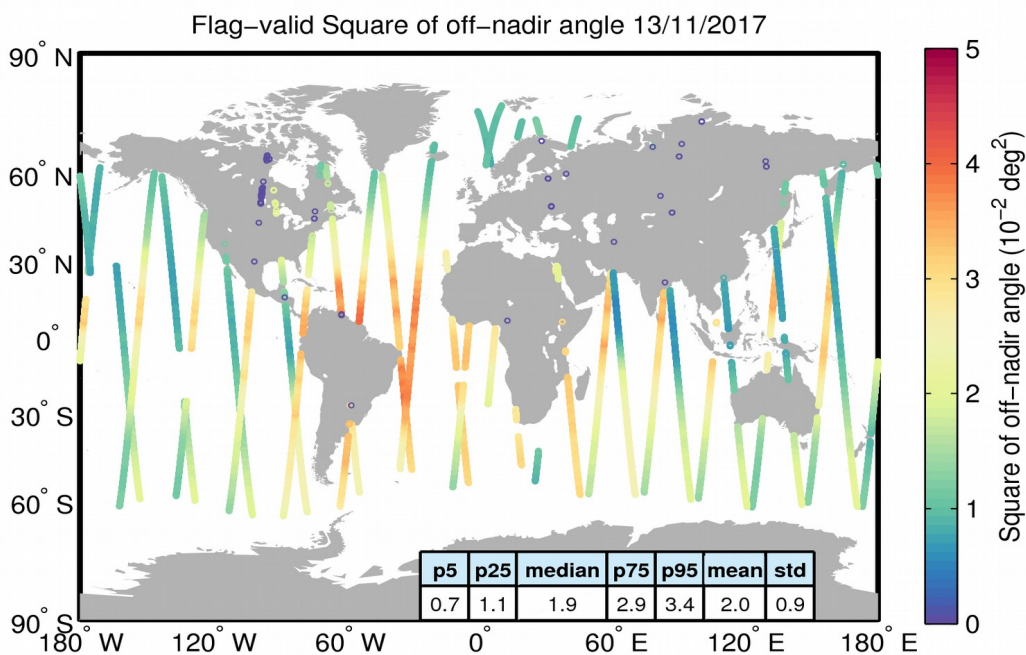
Figure 37. Geographical distribution of flag-valid mispointing data over oceans and lakes for 13/11/2017. The statistical values shown in the table refer to the mispointing in 10^{-2} deg 2 and are calculated over all measurements shown in the figure.
