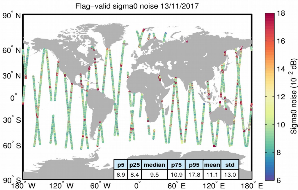
Figure 26. Geographical distribution of flag-valid 20-Hz sigma0 measurement noise over oceans and lakes for 13/11/2017. The statistical values shown in the table refer to the sigma0 noise and are calculated over all measurements shown in the figure.
