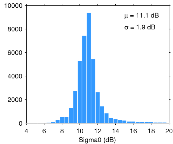
Figure 25. Histogram of flag-valid sigma0 over oceans and lakes for 12/11/2017. The mean ( \mu ) and standard deviation ( \sigma ) are also shown. Note that values outside [4 20] dB are excluded from the histogram for the sake of readability but not from the computation of \mu and \sigma .
