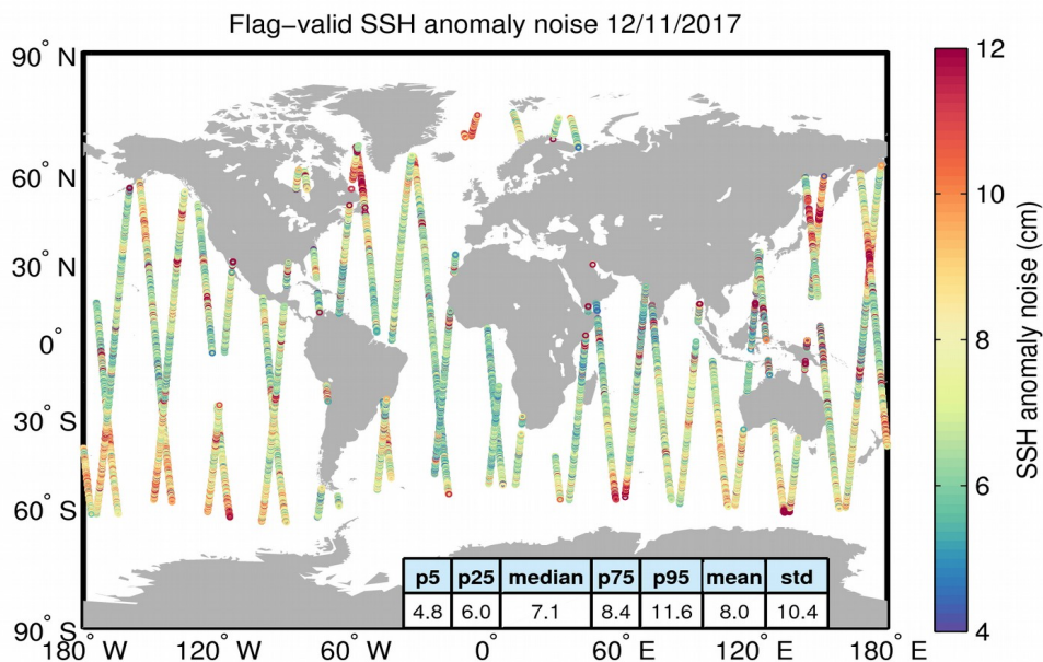
Figure 8. Geographical distribution of flag-valid 20-Hz SSH anomaly measurement noise over oceans and lakes for 12/11/2017. The statistical values shown in the table refer to the SSH anomaly noise and are calculated over all measurements shown in the figure.
