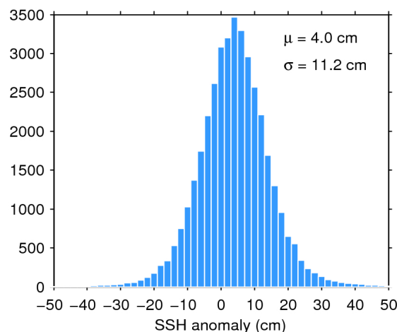
Figure 11. Histogram of science-valid SSH anomaly over oceans and lakes for 12/11/2017. The mean ( \mu ) and standard deviation ( \sigma ) are also shown. Note that values outside [-50 50] cm are excluded from the histogram for the sake of readability but not from the computation of \mu and \sigma .
