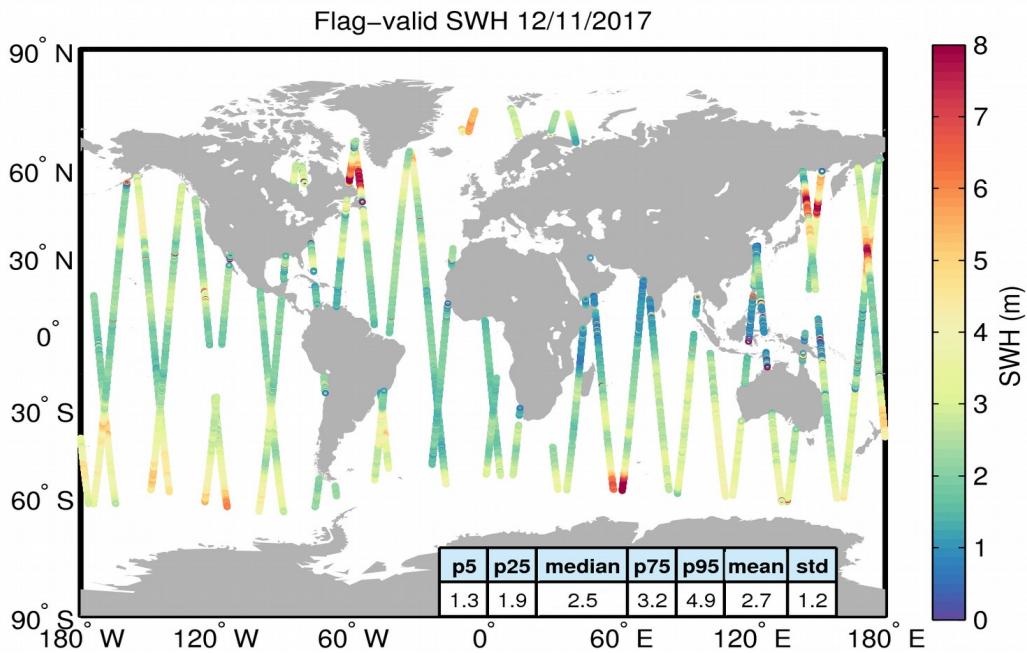
Figure 15. Geographical distribution of flag-valid SWH data over oceans and lakes for 12/11/2017. The statistical values shown in the table refer to the SWH in m and are calculated over all measurements shown in the figure.
