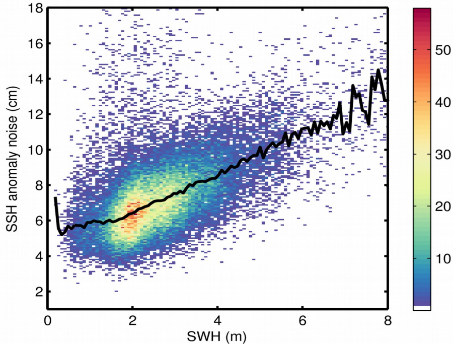
Figure 9. 2D histogram showing flag-valid SSH anomaly noise as a function of SWH for 12/11/2017. The black line denotes the median SSH anomaly noise as a function of SWH.
