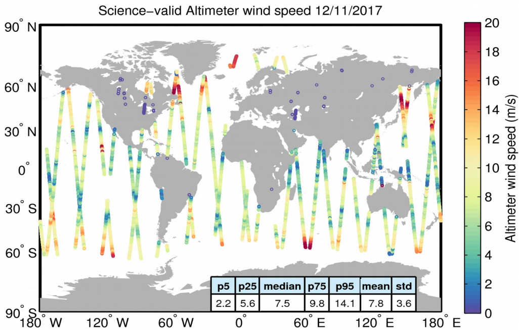
Figure 34. Geographical distribution of science-valid wind data over oceans and lakes for 12/11/2017. The statistical values shown in the table refer to the wind in m/s and are calculated over all measurements shown in the figure. Gray circles denote records that have been rejected based on the editing criteria described in Table 5.
