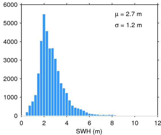
Figure 20. Histogram of science-valid SWH over oceans and lakes for 12/11/2017. The mean ( \mu ) and standard deviation ( \sigma ) are also shown. Note that values larger than 12 m are excluded from the histogram for the sake of readability but not from the computation of \mu and \sigma .
