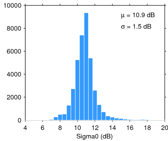
Figure 28. Histogram of science-valid sigma0 over oceans and lakes for 12/11/2017. The mean ( \mu ) and standard deviation ( \sigma ) are also shown. Note that values outside [4 20] dB are excluded from the histogram for the sake of readability but not from the computation of \mu and \sigma .
