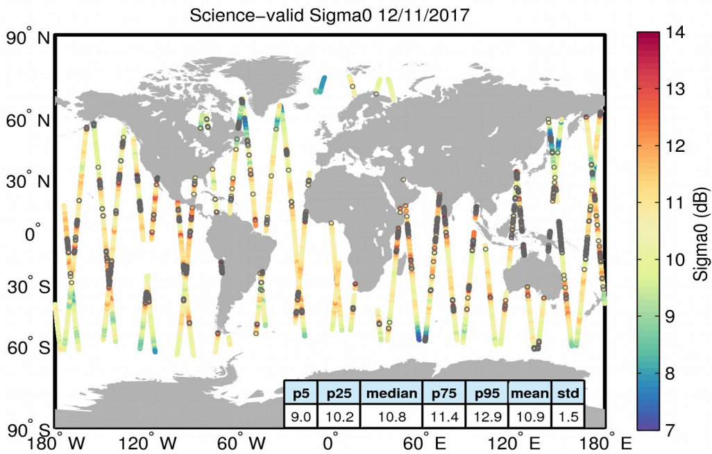
Figure 27. Geographical distribution of science-valid sigma0 data over oceans and lakes for 12/11/2017. The statistical values shown in the table refer to the sigma0 in dB and are calculated over all measurements shown in the figure. Gray circles denote records that have been rejected based on the editing criteria described in Table 4.
