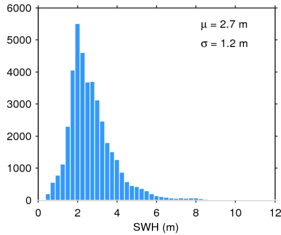
Figure 17. Histogram of flag-valid SWH over oceans and lakes for 12/11/2017. The mean ( \mu ) and standard deviation ( \sigma ) are also shown. Note that values larger than 12 m are excluded from the histogram for the sake of readability but not from the computation of \mu and \sigma .
