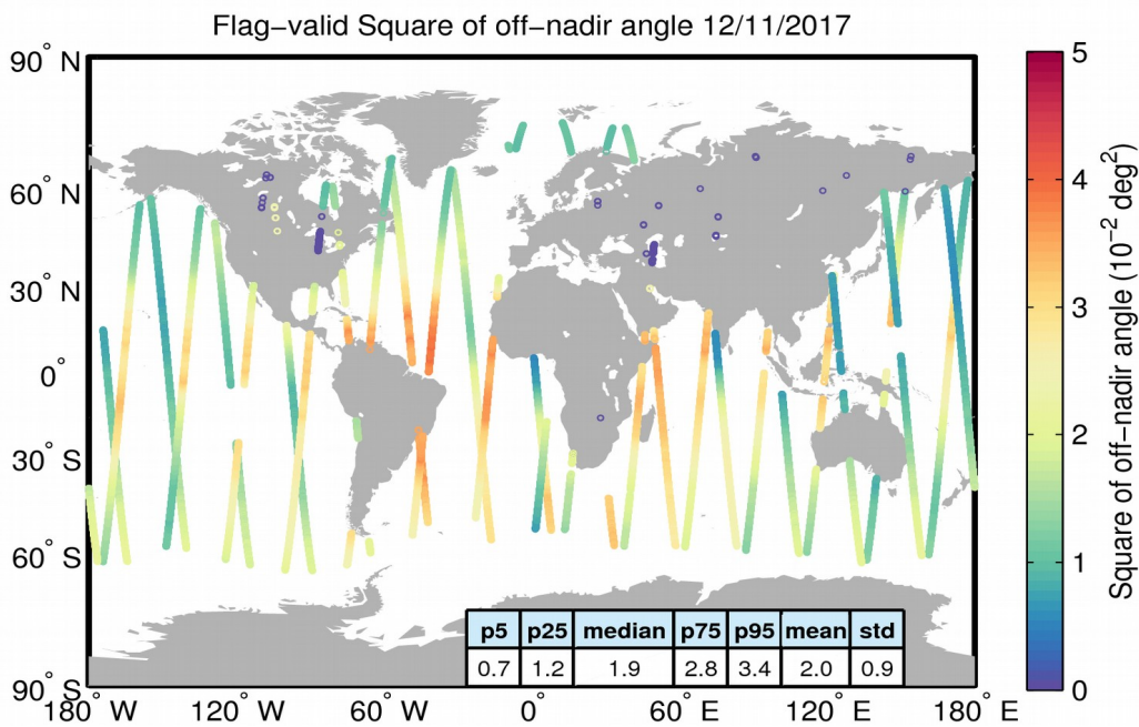
Figure 37. Geographical distribution of flag-valid mispointing data over oceans and lakes for 12/11/2017. The statistical values shown in the table refer to the mispointing in 10^{-2} deg 2 and are calculated over all measurements shown in the figure.
