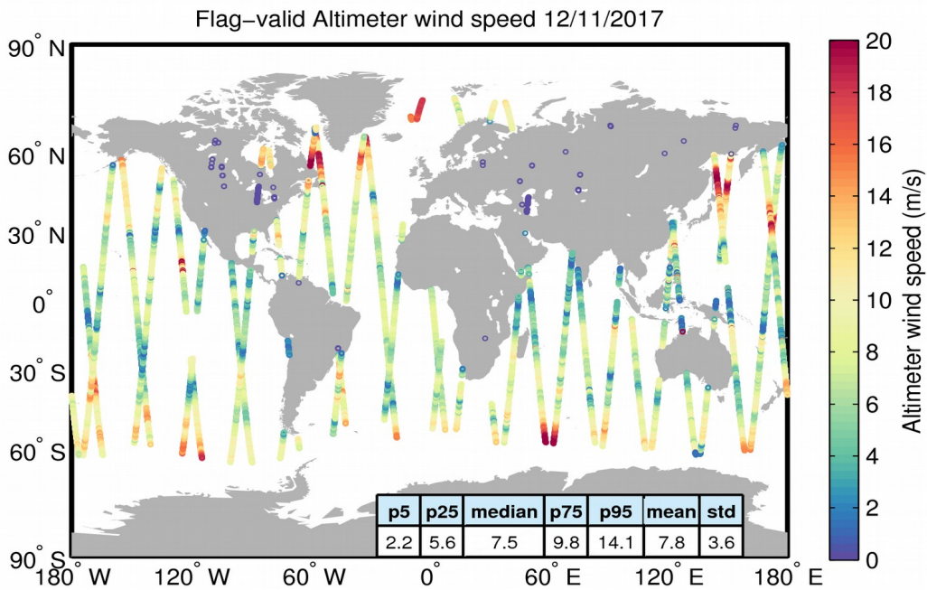
Figure 31. Geographical distribution of flag-valid wind data over oceans and lakes for 12/11/2017. The statistical values shown in the table refer to the wind in m/s and are calculated over all measurements shown in the figure.
