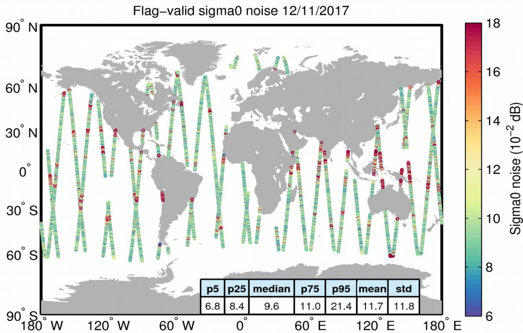
Figure 26. Geographical distribution of flag-valid 20-Hz sigma0 measurement noise over oceans and lakes for 12/11/2017. The statistical values shown in the table refer to the sigma0 noise and are calculated over all measurements shown in the figure.
