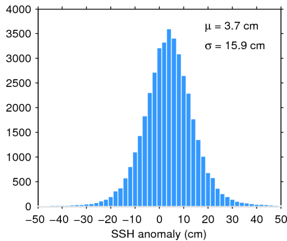
Figure 7. Histogram of flag-valid SSH anomaly over oceans and lakes for 12/11/2017. The mean ( \mu ) and standard deviation ( \sigma ) are also shown. Note that values outside [-50 50] cm are excluded from the histogram for the sake of readability but not from the computation of \mu and \sigma .
