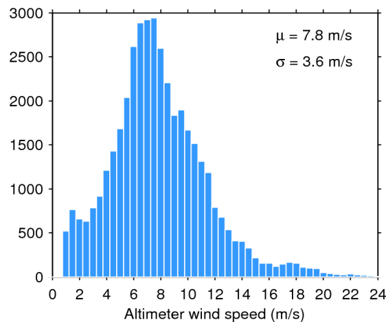
Figure 35. Histogram of science-valid wind over oceans and lakes for 12/11/2017. The mean ( \mu ) and standard deviation ( \sigma ) are also shown. Note that values larger than 24 m/s are excluded from the histogram for the sake of readability but not from the computation of \mu and \sigma .
