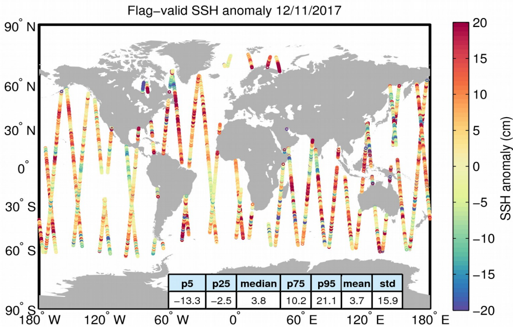
Figure 5. Geographical distribution of flag-valid 1-Hz SSH anomaly data over oceans and lakes for 12/11/2017. The statistical values shown in the table refer to the SSH anomaly in cm and are calculated over all measurements shown in the figure.
