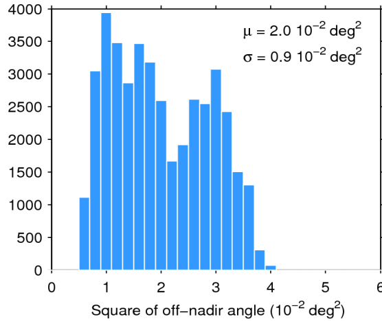
Figure 39. Histogram of flag-valid mispointing over oceans and lakes for 12/11/2017. The mean ( \mu ) and standard deviation ( \sigma ) are also shown. Note that values larger than 6 \cdot 10^{-2} \text{ deg}^2 are excluded from the histogram for the sake of readability but not from the computation of \mu and \sigma .
