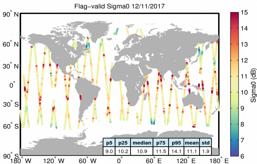
Figure 23. Geographical distribution of flag-valid sigma0 data over oceans and lakes for 12/11/2017. The statistical values shown in the table refer to the sigma0 in dB and are calculated over all measurements shown in the figure.
