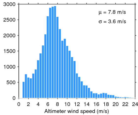
Figure 33. Histogram of flag-valid wind over oceans and lakes for 12/11/2017. The mean ( \mu ) and standard deviation ( \sigma ) are also shown. Note that values larger than 24 m/s are excluded from the histogram for the sake of readability but not from the computation of \mu and \sigma .
