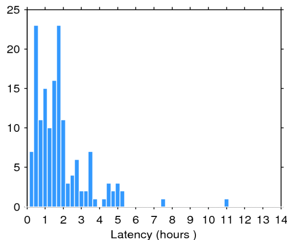
Figure 2. Histogram of the data latency for 12/11/2017. The y-axis denotes the number of files that are made available with a delay of x-hours with respect to the mean time of the records stored in the file.
