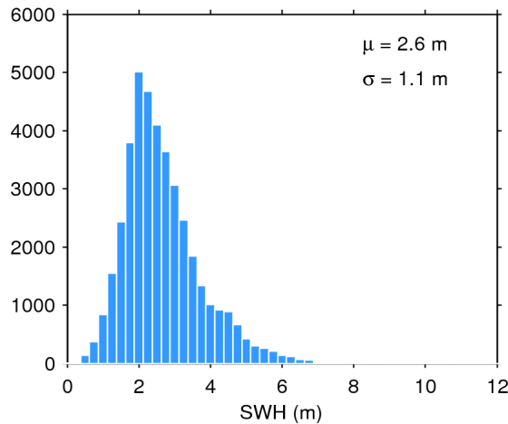
Figure 20. Histogram of science-valid SWH over oceans and lakes for 11/11/2017. The mean ( \mu ) and standard deviation ( \sigma ) are also shown. Note that values larger than 12 m are excluded from the histogram for the sake of readability but not from the computation of \mu and \sigma .
