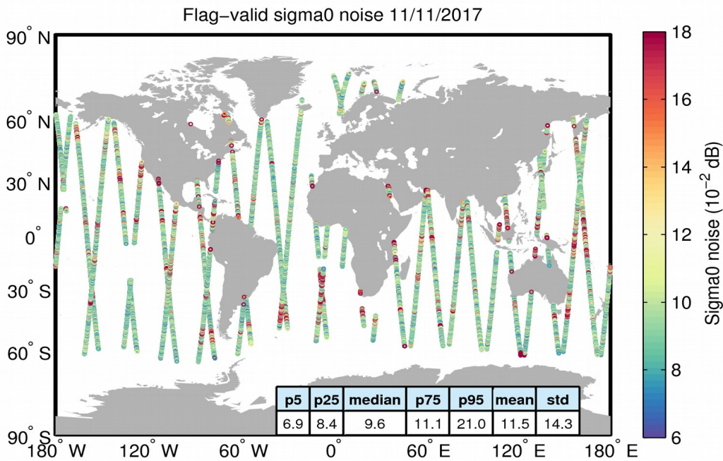
Figure 26. Geographical distribution of flag-valid 20-Hz sigma0 measurement noise over oceans and lakes for 11/11/2017. The statistical values shown in the table refer to the sigma0 noise and are calculated over all measurements shown in the figure.
