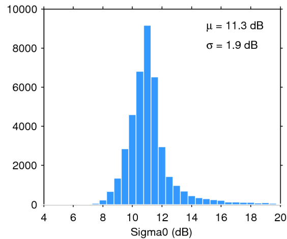
Figure 25. Histogram of flag-valid sigma0 over oceans and lakes for 11/11/2017. The mean ( \mu ) and standard deviation ( \sigma ) are also shown. Note that values outside [4 20] dB are excluded from the histogram for the sake of readability but not from the computation of \mu and \sigma .
