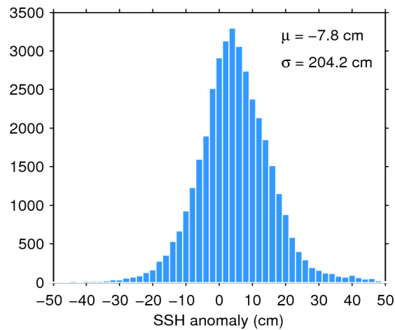
Figure 7. Histogram of flag-valid SSH anomaly over oceans and lakes for 11/11/2017. The mean ( \mu ) and standard deviation ( \sigma ) are also shown. Note that values outside [-50 50] cm are excluded from the histogram for the sake of readability but not from the computation of \mu and \sigma .
