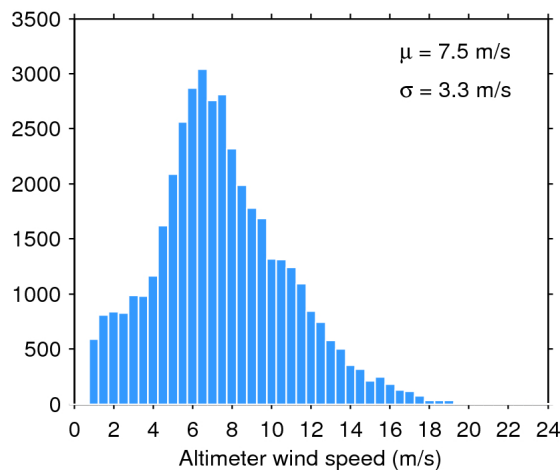
Figure 35. Histogram of science-valid wind over oceans and lakes for 11/11/2017. The mean ( \mu ) and standard deviation ( \sigma ) are also shown. Note that values larger than 24 m/s are excluded from the histogram for the sake of readability but not from the computation of \mu and \sigma .
