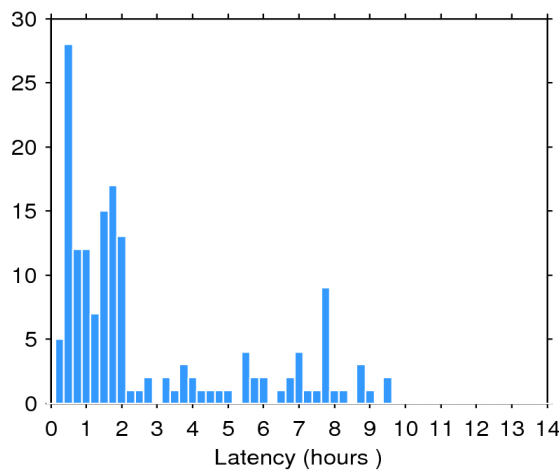
Figure 2. Histogram of the data latency for 11/11/2017. The y-axis denotes the number of files that are made available with a delay of x-hours with respect to the mean time of the records stored in the file.
