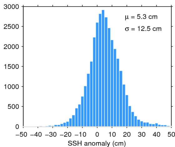
Figure 11. Histogram of science-valid SSH anomaly over oceans and lakes for 11/11/2017. The mean ( \mu ) and standard deviation ( \sigma ) are also shown. Note that values outside [-50 50] cm are excluded from the histogram for the sake of readability but not from the computation of \mu and \sigma .
