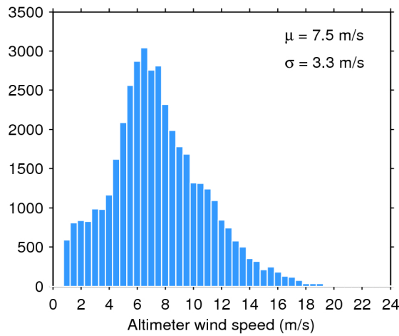
Figure 33. Histogram of flag-valid wind over oceans and lakes for 11/11/2017. The mean ( \mu ) and standard deviation ( \sigma ) are also shown. Note that values larger than 24 m/s are excluded from the histogram for the sake of readability but not from the computation of \mu and \sigma .
