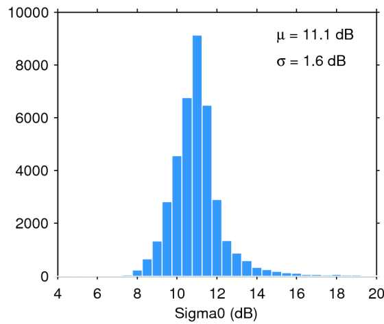
Figure 28. Histogram of science-valid sigma0 over oceans and lakes for 11/11/2017. The mean ( \mu ) and standard deviation ( \sigma ) are also shown. Note that values outside [4 20] dB are excluded from the histogram for the sake of readability but not from the computation of \mu and \sigma .
