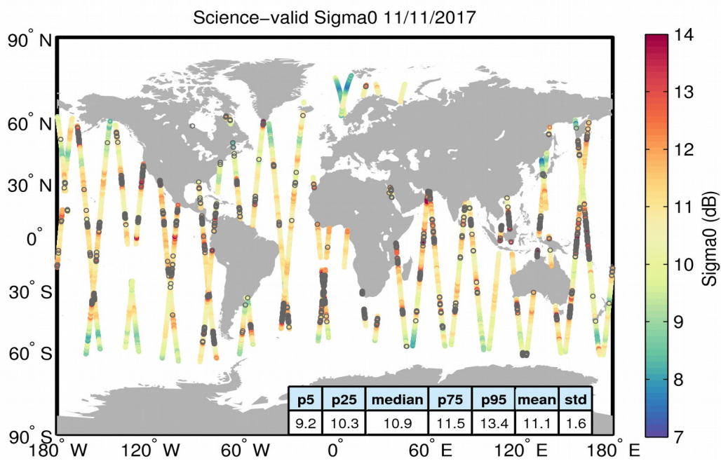
Figure 27. Geographical distribution of science-valid sigma0 data over oceans and lakes for 11/11/2017. The statistical values shown in the table refer to the sigma0 in dB and are calculated over all measurements shown in the figure. Gray circles denote records that have been rejected based on the editing criteria described in Table 4.
