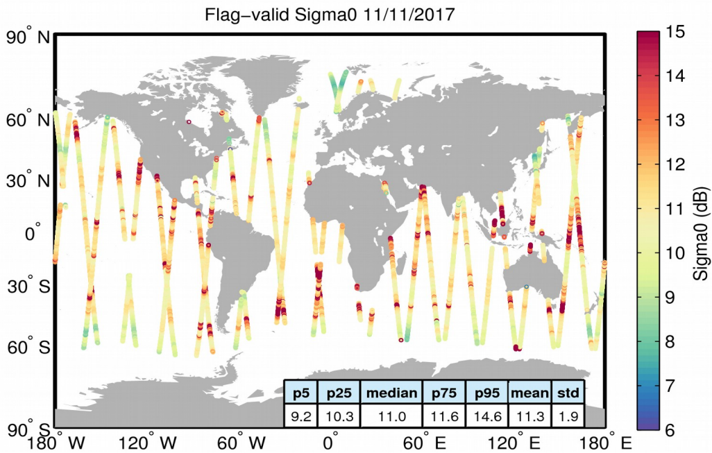
Figure 23. Geographical distribution of flag-valid sigma0 data over oceans and lakes for 11/11/2017. The statistical values shown in the table refer to the sigma0 in dB and are calculated over all measurements shown in the figure.
