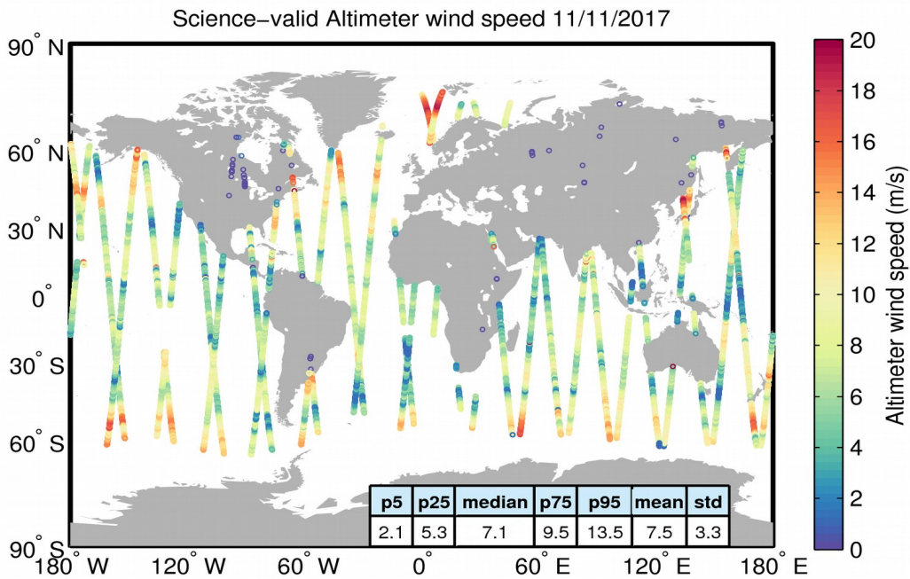
Figure 34. Geographical distribution of science-valid wind data over oceans and lakes for 11/11/2017. The statistical values shown in the table refer to the wind in m/s and are calculated over all measurements shown in the figure. Gray circles denote records that have been rejected based on the editing criteria described in Table 5.
