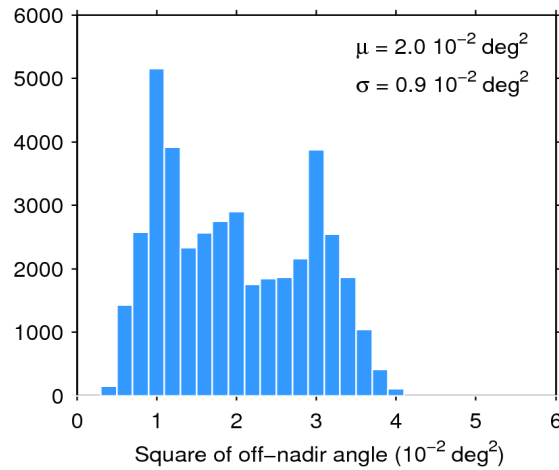
Figure 39. Histogram of flag-valid mispointing over oceans and lakes for 11/11/2017. The mean ( \mu ) and standard deviation ( \sigma ) are also shown. Note that values larger than 6 \cdot 10^{-2} \text{ deg}^2 are excluded from the histogram for the sake of readability but not from the computation of \mu and \sigma .
