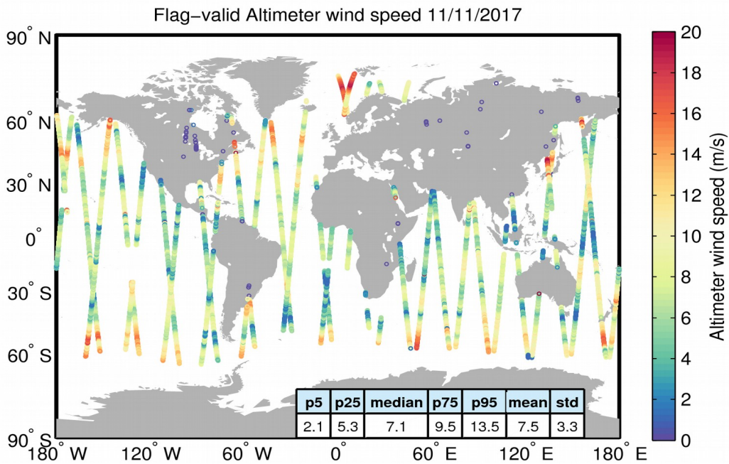
Figure 31. Geographical distribution of flag-valid wind data over oceans and lakes for 11/11/2017. The statistical values shown in the table refer to the wind in m/s and are calculated over all measurements shown in the figure.
