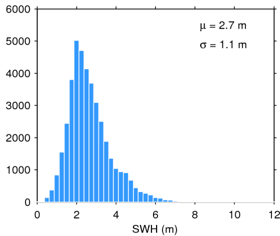
Figure 17. Histogram of flag-valid SWH over oceans and lakes for 11/11/2017. The mean ( \mu ) and standard deviation ( \sigma ) are also shown. Note that values larger than 12 m are excluded from the histogram for the sake of readability but not from the computation of \mu and \sigma .
