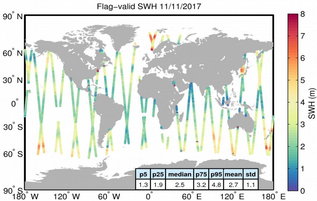
Figure 15. Geographical distribution of flag-valid SWH data over oceans and lakes for 11/11/2017. The statistical values shown in the table refer to the SWH in m and are calculated over all measurements shown in the figure.
