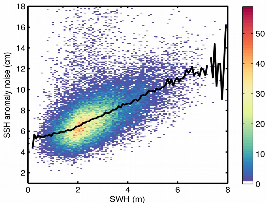
Figure 9. 2D histogram showing flag-valid SSH anomaly noise as a function of SWH for 11/11/2017. The black line denotes the median SSH anomaly noise as a function of SWH.
