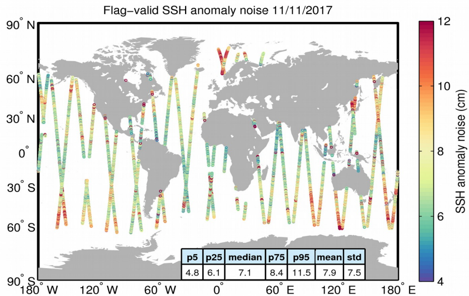
Figure 8. Geographical distribution of flag-valid 20-Hz SSH anomaly measurement noise over oceans and lakes for 11/11/2017. The statistical values shown in the table refer to the SSH anomaly noise and are calculated over all measurements shown in the figure.
