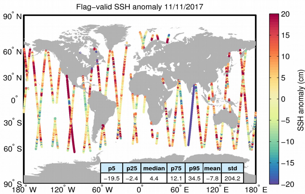
Figure 5. Geographical distribution of flag-valid 1-Hz SSH anomaly data over oceans and lakes for 11/11/2017. The statistical values shown in the table refer to the SSH anomaly in cm and are calculated over all measurements shown in the figure.
