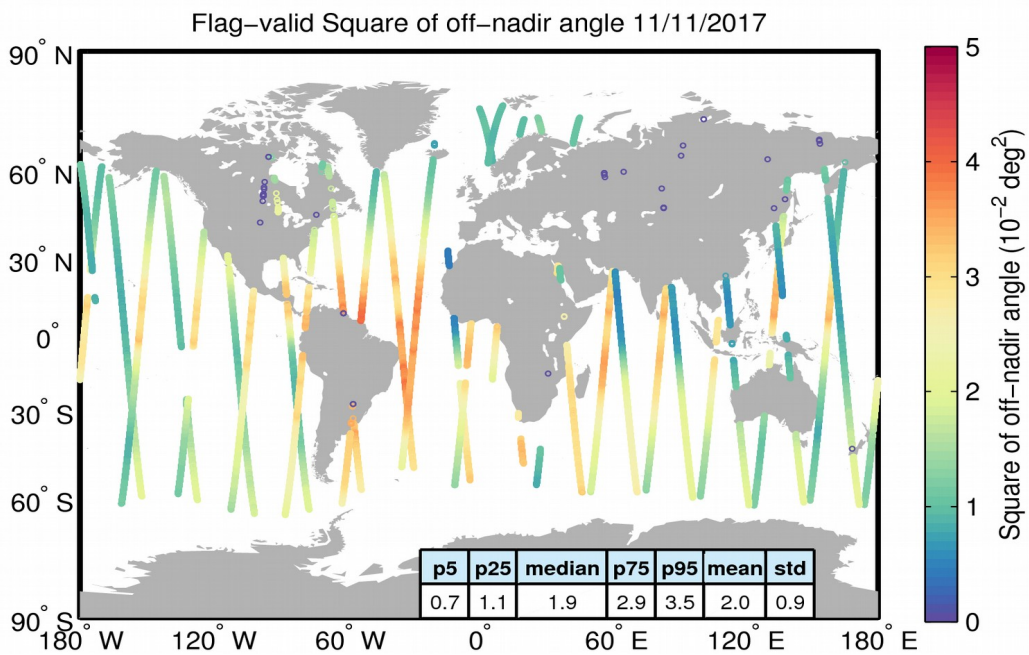
Figure 37. Geographical distribution of flag-valid mispointing data over oceans and lakes for 11/11/2017. The statistical values shown in the table refer to the mispointing in 10^{-2} \text{ deg}^2 and are calculated over all measurements shown in the figure.
