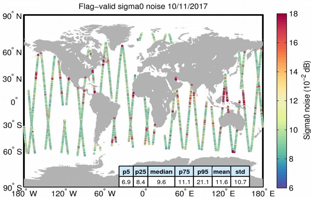
Figure 26. Geographical distribution of flag-valid 20-Hz sigma0 measurement noise over oceans and lakes for 10/11/2017. The statistical values shown in the table refer to the sigma0 noise and are calculated over all measurements shown in the figure.
