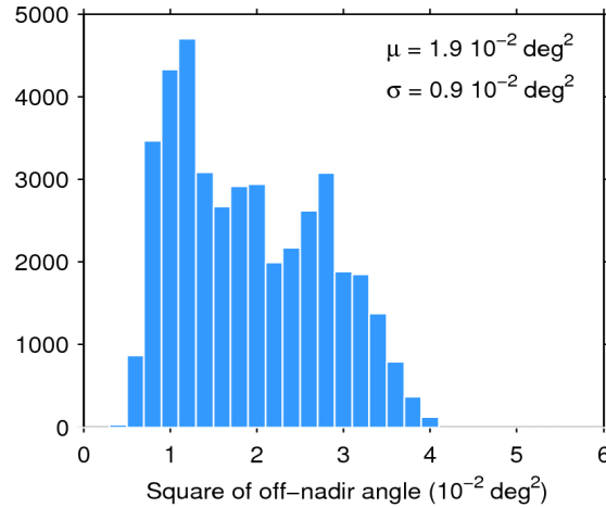
Figure 39. Histogram of flag-valid mispointing over oceans and lakes for 10/11/2017. The mean ( \mu ) and standard deviation ( \sigma ) are also shown. Note that values larger than 6 \cdot 10^{-2} \text{ deg}^2 are excluded from the histogram for the sake of readability but not from the computation of \mu and \sigma .
