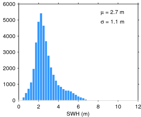
Figure 20. Histogram of science-valid SWH over oceans and lakes for 10/11/2017. The mean ( \mu ) and standard deviation ( \sigma ) are also shown. Note that values larger than 12 m are excluded from the histogram for the sake of readability but not from the computation of \mu and \sigma .
