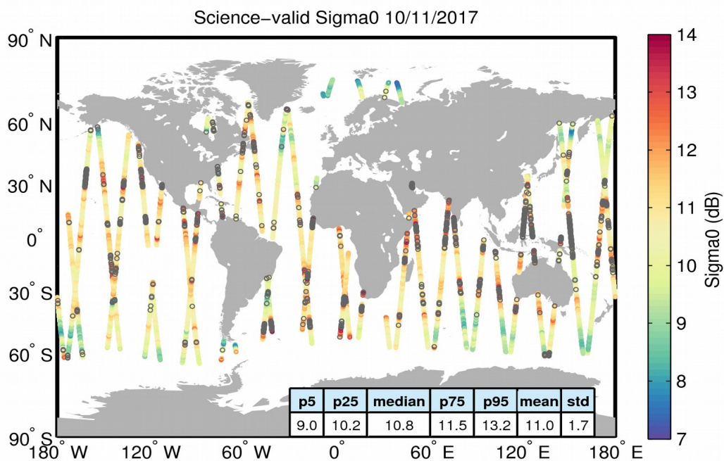
Figure 27. Geographical distribution of science-valid sigma0 data over oceans and lakes for 10/11/2017. The statistical values shown in the table refer to the sigma0 in dB and are calculated over all measurements shown in the figure. Gray circles denote records that have been rejected based on the editing criteria described in Table 4.
