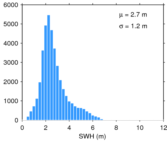
Figure 17. Histogram of flag-valid SWH over oceans and lakes for 10/11/2017. The mean ( \mu ) and standard deviation ( \sigma ) are also shown. Note that values larger than 12 m are excluded from the histogram for the sake of readability but not from the computation of \mu and \sigma .
