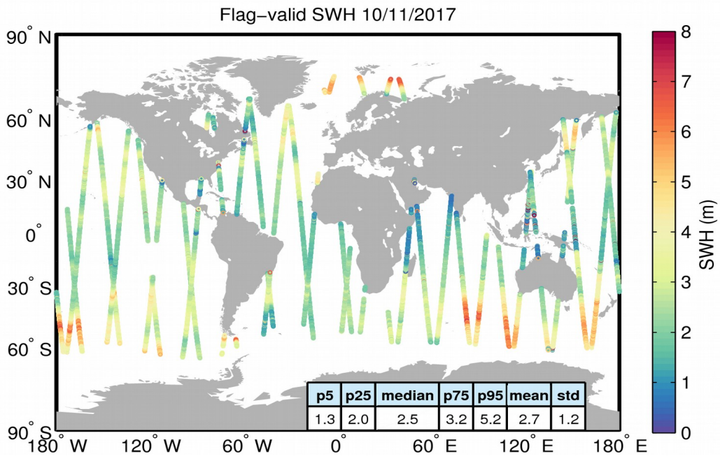
Figure 15. Geographical distribution of flag-valid SWH data over oceans and lakes for 10/11/2017. The statistical values shown in the table refer to the SWH in m and are calculated over all measurements shown in the figure.
