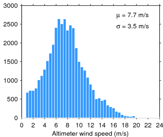
Figure 35. Histogram of science-valid wind over oceans and lakes for 10/11/2017. The mean ( \mu ) and standard deviation ( \sigma ) are also shown. Note that values larger than 24 m/s are excluded from the histogram for the sake of readability but not from the computation of \mu and \sigma .
