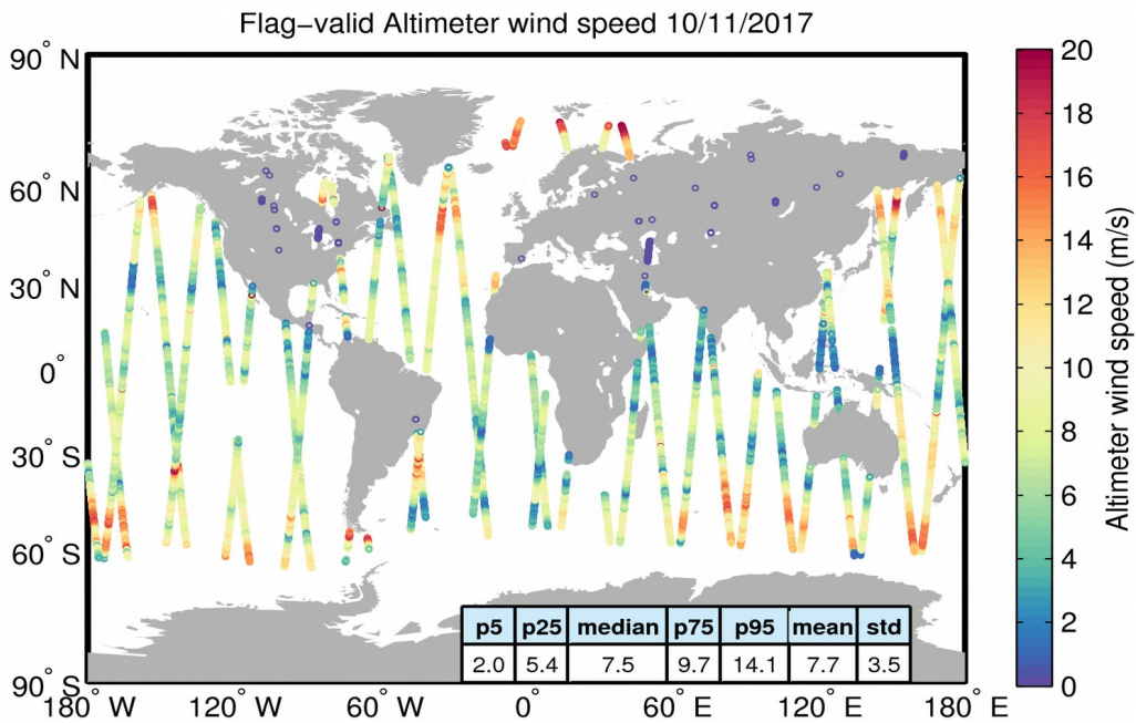
Figure 31. Geographical distribution of flag-valid wind data over oceans and lakes for 10/11/2017. The statistical values shown in the table refer to the wind in m/s and are calculated over all measurements shown in the figure.
