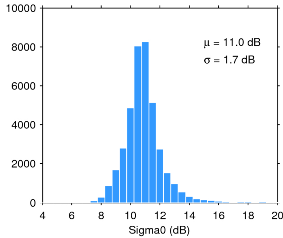
Figure 28. Histogram of science-valid sigma0 over oceans and lakes for 10/11/2017. The mean ( \mu ) and standard deviation ( \sigma ) are also shown. Note that values outside [4 20] dB are excluded from the histogram for the sake of readability but not from the computation of \mu and \sigma .
