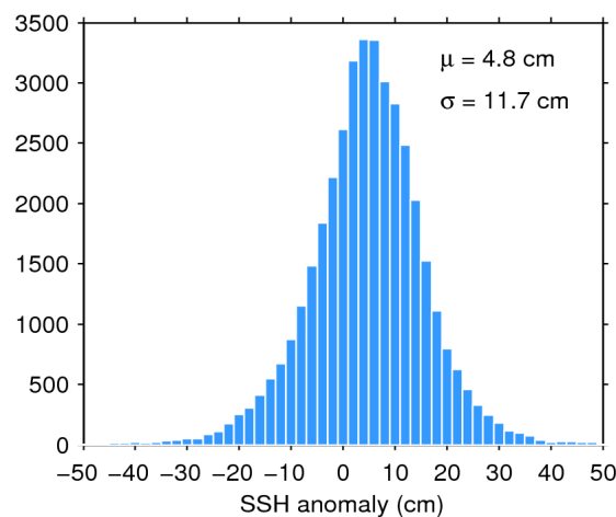
Figure 11. Histogram of science-valid SSH anomaly over oceans and lakes for 10/11/2017. The mean ( \mu ) and standard deviation ( \sigma ) are also shown. Note that values outside [-50 50] cm are excluded from the histogram for the sake of readability but not from the computation of \mu and \sigma .
