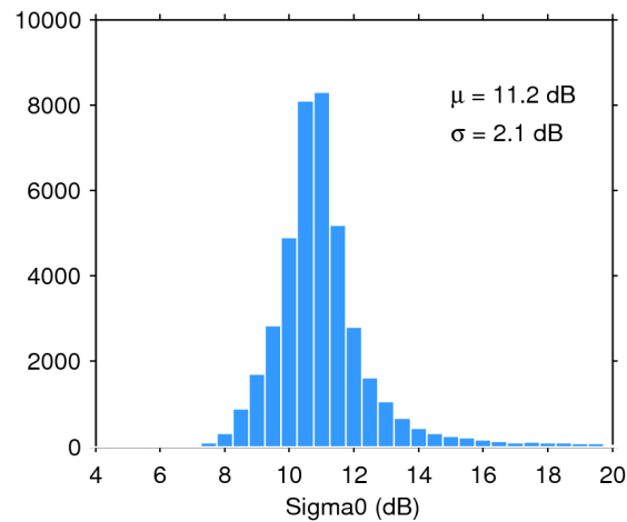
Figure 25. Histogram of flag-valid sigma0 over oceans and lakes for 10/11/2017. The mean ( \mu ) and standard deviation ( \sigma ) are also shown. Note that values outside [4 20] dB are excluded from the histogram for the sake of readability but not from the computation of \mu and \sigma .
