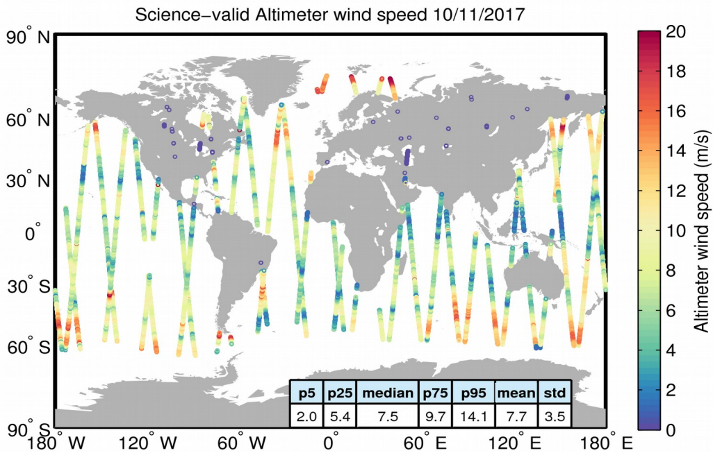
Figure 34. Geographical distribution of science-valid wind data over oceans and lakes for 10/11/2017. The statistical values shown in the table refer to the wind in m/s and are calculated over all measurements shown in the figure. Gray circles denote records that have been rejected based on the editing criteria described in Table 5.
