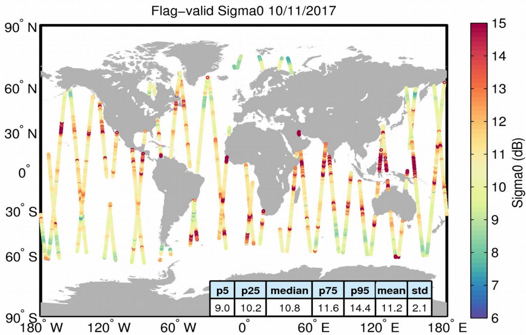
Figure 23. Geographical distribution of flag-valid sigma0 data over oceans and lakes for 10/11/2017. The statistical values shown in the table refer to the sigma0 in dB and are calculated over all measurements shown in the figure.
