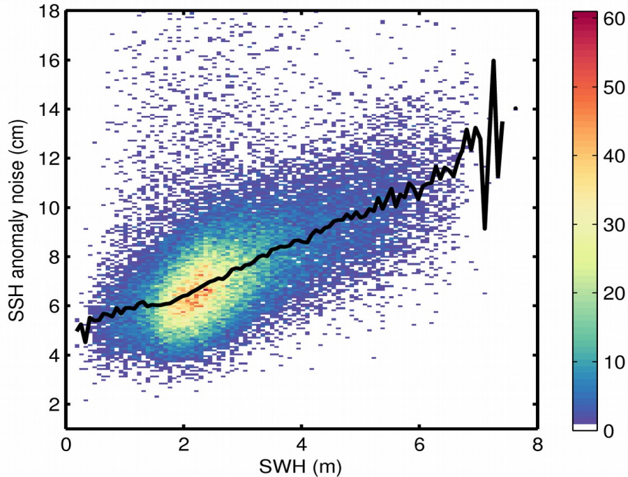
Figure 9. 2D histogram showing flag-valid SSH anomaly noise as a function of SWH for 10/11/2017. The black line denotes the median SSH anomaly noise as a function of SWH.
