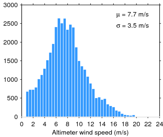
Figure 33. Histogram of flag-valid wind over oceans and lakes for 10/11/2017. The mean ( \mu ) and standard deviation ( \sigma ) are also shown. Note that values larger than 24 m/s are excluded from the histogram for the sake of readability but not from the computation of \mu and \sigma .
