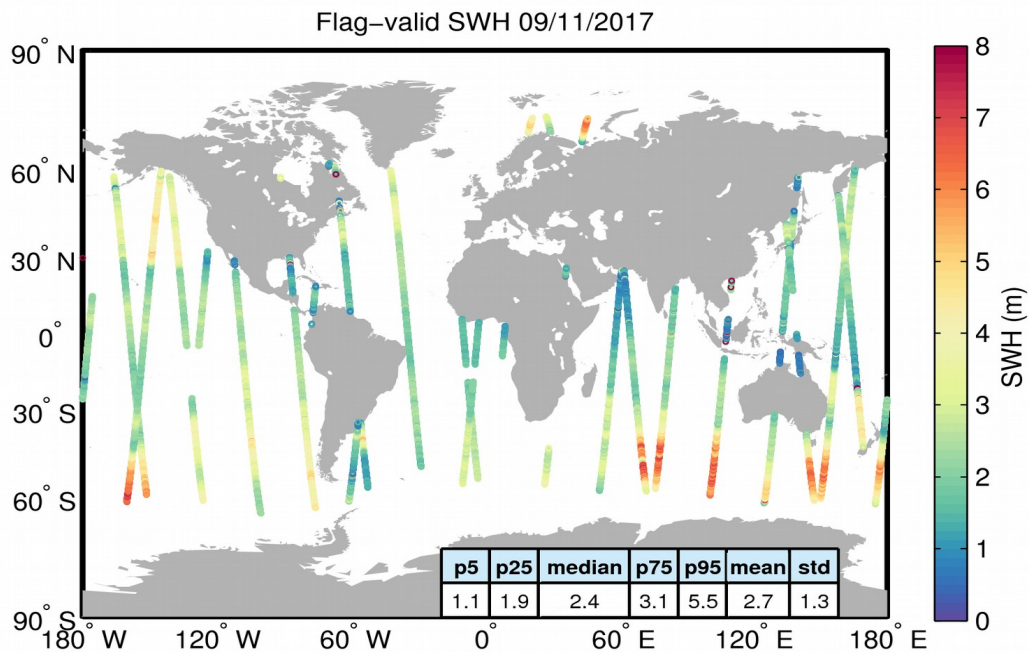
Figure 15. Geographical distribution of flag-valid SWH data over oceans and lakes for 09/11/2017. The statistical values shown in the table refer to the SWH in m and are calculated over all measurements shown in the figure.
