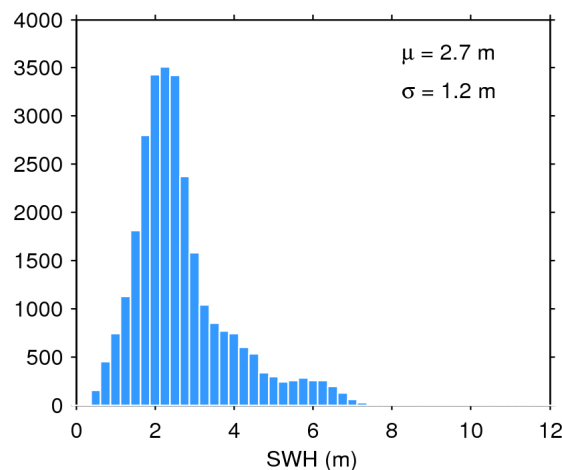
Figure 20. Histogram of science-valid SWH over oceans and lakes for 09/11/2017. The mean ( \mu ) and standard deviation ( \sigma ) are also shown. Note that values larger than 12 m are excluded from the histogram for the sake of readability but not from the computation of \mu and \sigma .
