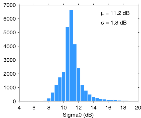
Figure 25. Histogram of flag-valid sigma0 over oceans and lakes for 09/11/2017. The mean ( \mu ) and standard deviation ( \sigma ) are also shown. Note that values outside [4 20] dB are excluded from the histogram for the sake of readability but not from the computation of \mu and \sigma .
