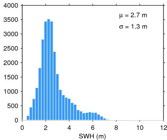
Figure 17. Histogram of flag-valid SWH over oceans and lakes for 09/11/2017. The mean ( \mu ) and standard deviation ( \sigma ) are also shown. Note that values larger than 12 m are excluded from the histogram for the sake of readability but not from the computation of \mu and \sigma .
