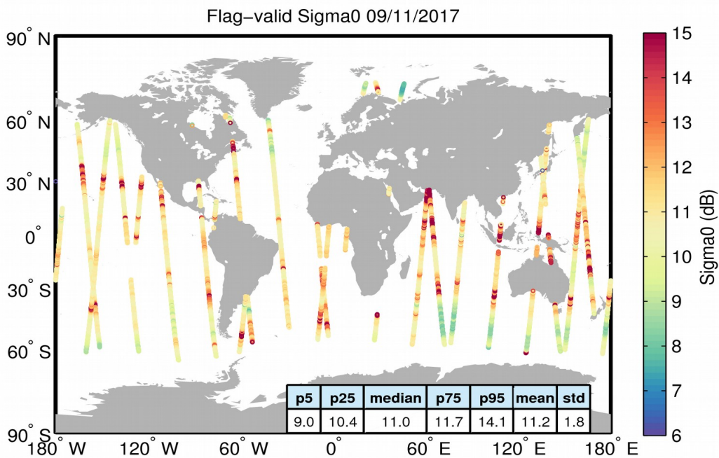
Figure 23. Geographical distribution of flag-valid sigma0 data over oceans and lakes for 09/11/2017. The statistical values shown in the table refer to the sigma0 in dB and are calculated over all measurements shown in the figure.
