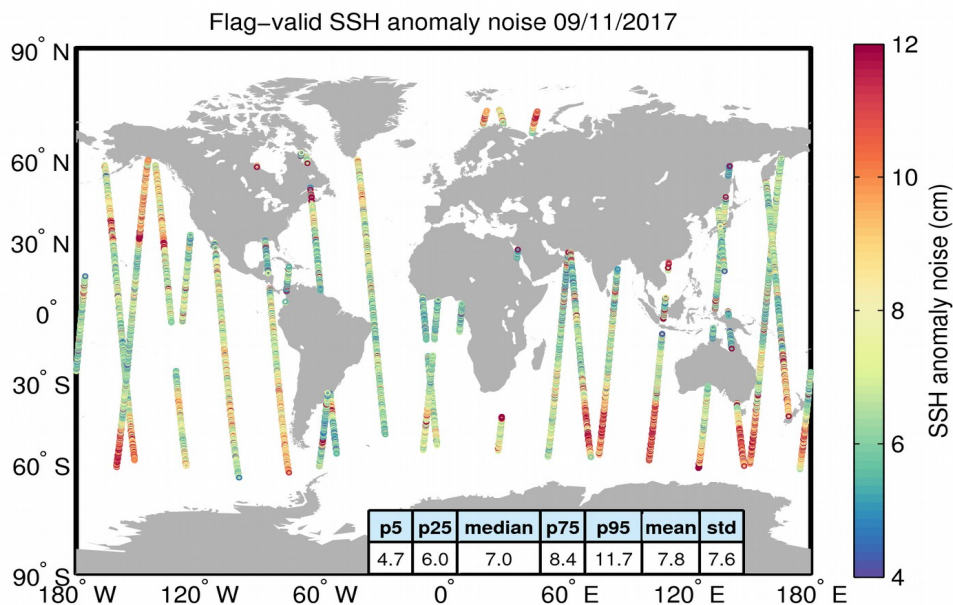
Figure 8. Geographical distribution of flag-valid 20-Hz SSH anomaly measurement noise over oceans and lakes for 09/11/2017. The statistical values shown in the table refer to the SSH anomaly noise and are calculated over all measurements shown in the figure.
