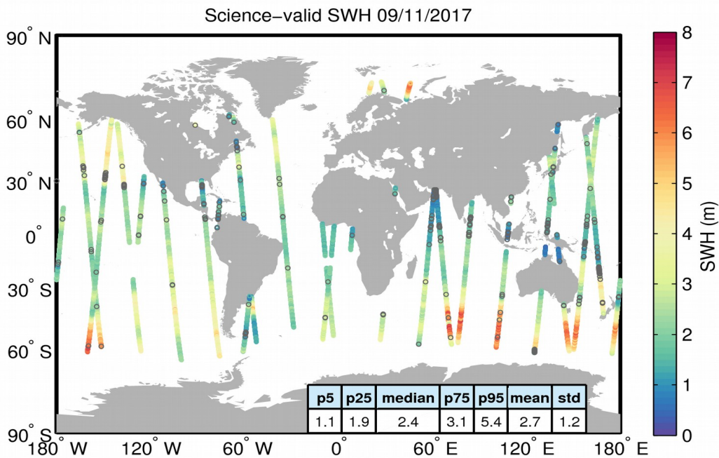
Figure 19. Geographical distribution of science-valid SWH data over oceans and lakes for 09/11/2017. The statistical values shown in the table refer to the SWH in m and are calculated over all measurements shown in the figure. Gray circles denote records that have been rejected based on the editing criteria described in Table 3.
