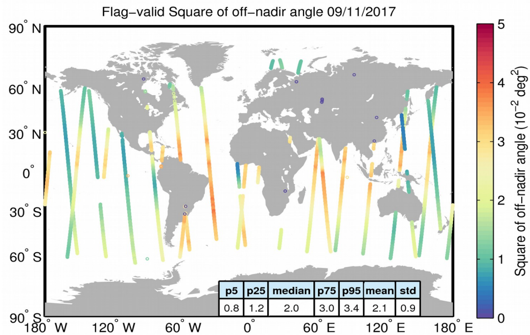
Figure 37. Geographical distribution of flag-valid mispointing data over oceans and lakes for 09/11/2017. The statistical values shown in the table refer to the mispointing in 10^{-2} deg 2 and are calculated over all measurements shown in the figure.
