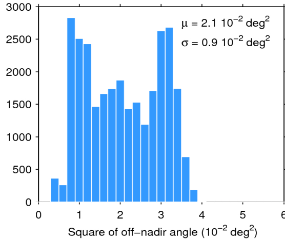
Figure 39. Histogram of flag-valid mispointing over oceans and lakes for 09/11/2017. The mean ( \mu ) and standard deviation ( \sigma ) are also shown. Note that values larger than 6 \cdot 10^{-2} \text{ deg}^2 are excluded from the histogram for the sake of readability but not from the computation of \mu and \sigma .
