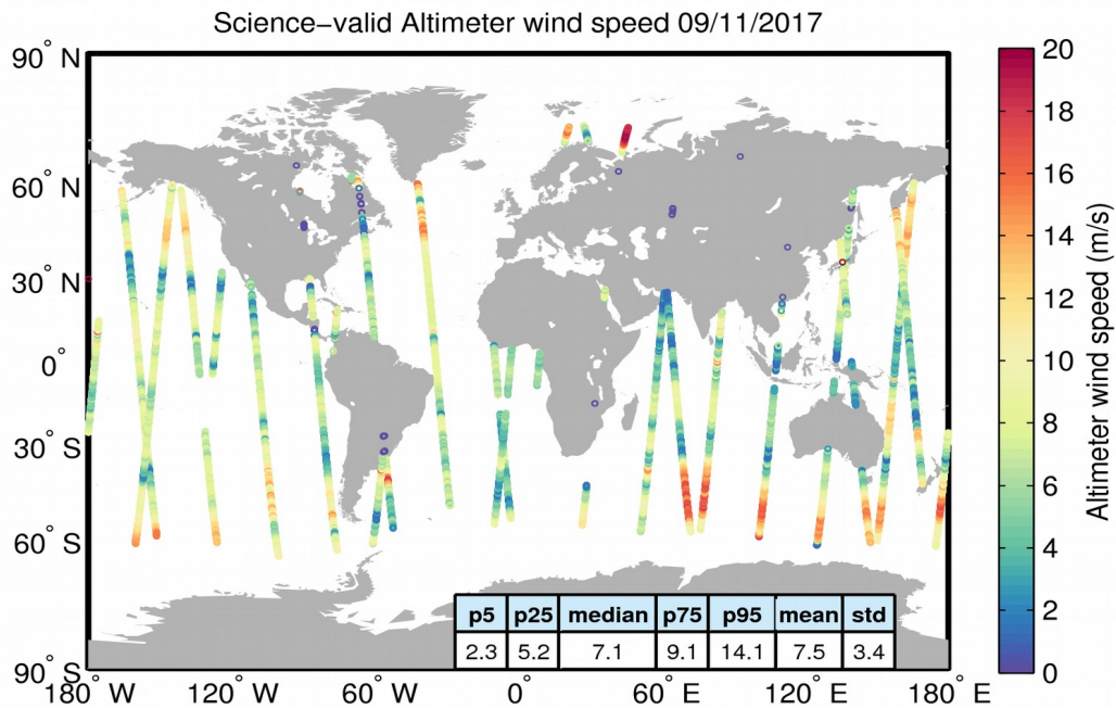
Figure 34. Geographical distribution of science-valid wind data over oceans and lakes for 09/11/2017. The statistical values shown in the table refer to the wind in m/s and are calculated over all measurements shown in the figure. Gray circles denote records that have been rejected based on the editing criteria described in Table 5.
