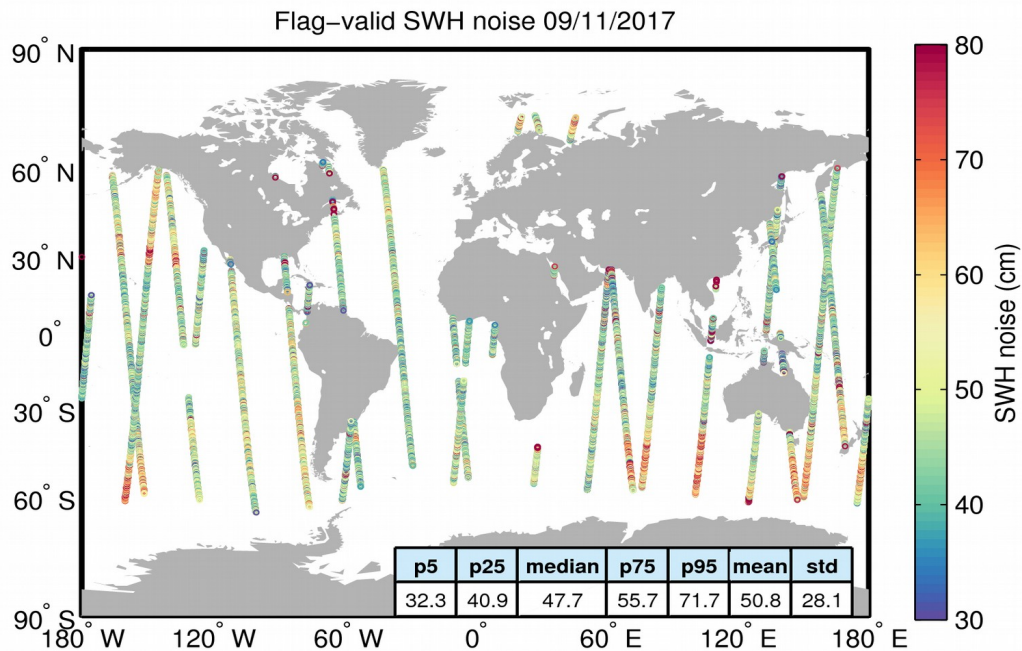
Figure 18. Geographical distribution of flag-valid 20-Hz SWH measurement noise over oceans and lakes for 09/11/2017. The statistical values shown in the table refer to the SWH noise and are calculated over all measurements shown in the figure.
