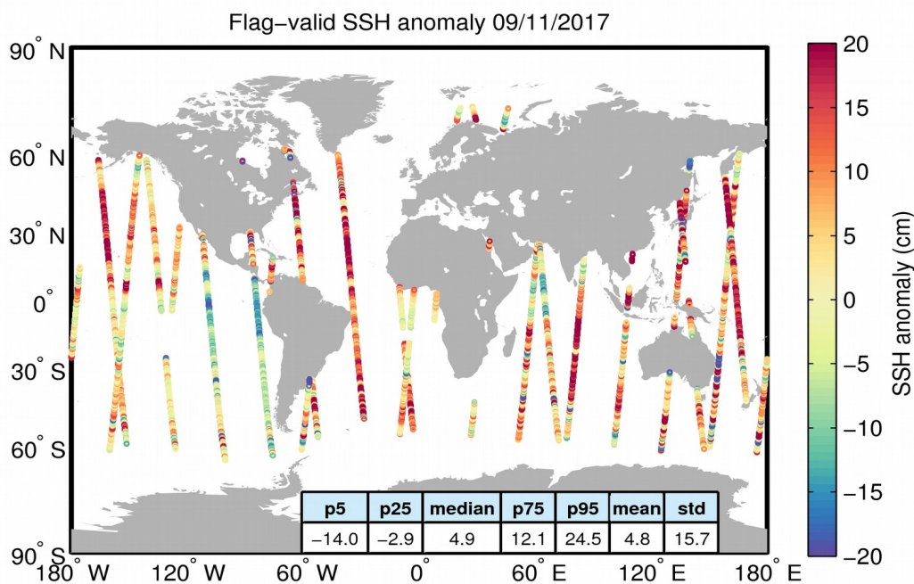
Figure 5. Geographical distribution of flag-valid 1-Hz SSH anomaly data over oceans and lakes for 09/11/2017. The statistical values shown in the table refer to the SSH anomaly in cm and are calculated over all measurements shown in the figure.
