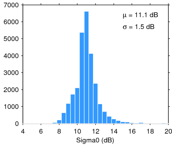
Figure 28. Histogram of science-valid sigma0 over oceans and lakes for 09/11/2017. The mean ( \mu ) and standard deviation ( \sigma ) are also shown. Note that values outside [4 20] dB are excluded from the histogram for the sake of readability but not from the computation of \mu and \sigma .
