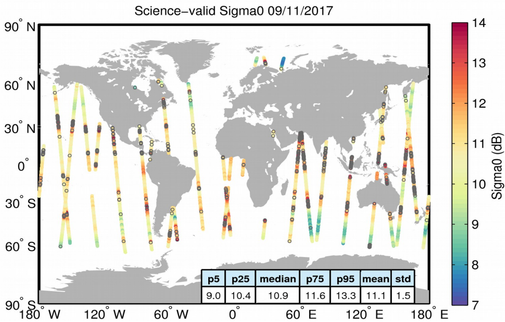
Figure 27. Geographical distribution of science-valid sigma0 data over oceans and lakes for 09/11/2017. The statistical values shown in the table refer to the sigma0 in dB and are calculated over all measurements shown in the figure. Gray circles denote records that have been rejected based on the editing criteria described in Table 4.
