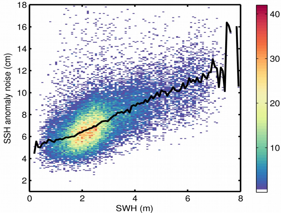
Figure 9. 2D histogram showing flag-valid SSH anomaly noise as a function of SWH for 09/11/2017. The black line denotes the median SSH anomaly noise as a function of SWH.
