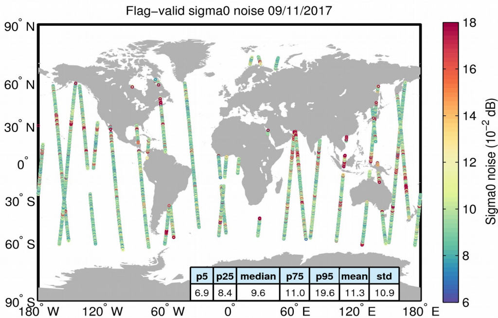
Figure 26. Geographical distribution of flag-valid 20-Hz sigma0 measurement noise over oceans and lakes for 09/11/2017. The statistical values shown in the table refer to the sigma0 noise and are calculated over all measurements shown in the figure.
