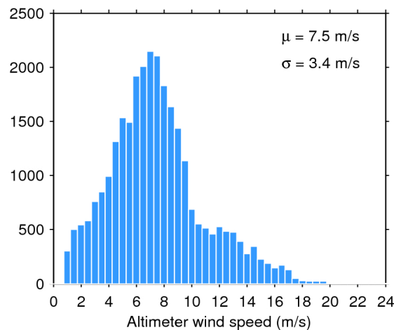
Figure 35. Histogram of science-valid wind over oceans and lakes for 09/11/2017. The mean ( \mu ) and standard deviation ( \sigma ) are also shown. Note that values larger than 24 m/s are excluded from the histogram for the sake of readability but not from the computation of \mu and \sigma .
