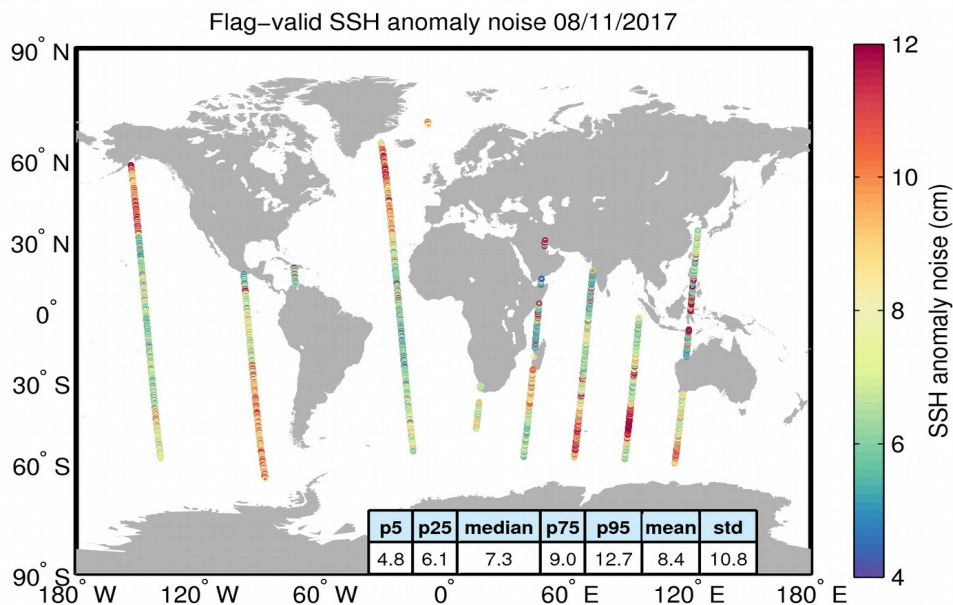
Figure 8. Geographical distribution of flag-valid 20-Hz SSH anomaly measurement noise over oceans and lakes for 08/11/2017. The statistical values shown in the table refer to the SSH anomaly noise and are calculated over all measurements shown in the figure.
