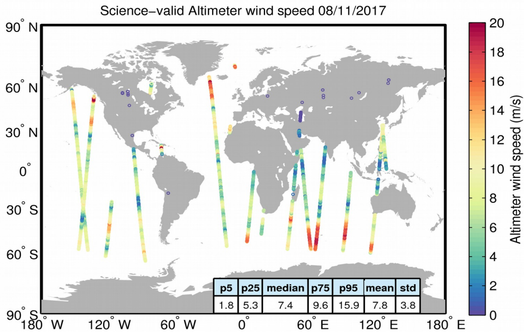
Figure 34. Geographical distribution of science-valid wind data over oceans and lakes for 08/11/2017. The statistical values shown in the table refer to the wind in m/s and are calculated over all measurements shown in the figure. Gray circles denote records that have been rejected based on the editing criteria described in Table 5.
