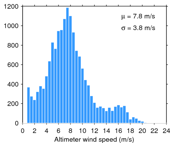
Figure 35. Histogram of science-valid wind over oceans and lakes for 08/11/2017. The mean ( \mu ) and standard deviation ( \sigma ) are also shown. Note that values larger than 24 m/s are excluded from the histogram for the sake of readability but not from the computation of \mu and \sigma .
