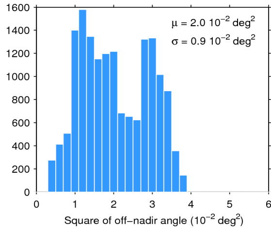
Figure 39. Histogram of flag-valid mispointing over oceans and lakes for 08/11/2017. The mean ( \mu ) and standard deviation ( \sigma ) are also shown. Note that values larger than 6 \cdot 10^{-2} \text{ deg}^2 are excluded from the histogram for the sake of readability but not from the computation of \mu and \sigma .
