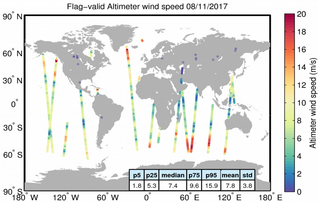
Figure 31. Geographical distribution of flag-valid wind data over oceans and lakes for 08/11/2017. The statistical values shown in the table refer to the wind in m/s and are calculated over all measurements shown in the figure.
