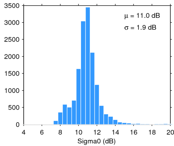
Figure 28. Histogram of science-valid sigma0 over oceans and lakes for 08/11/2017. The mean ( \mu ) and standard deviation ( \sigma ) are also shown. Note that values outside [4 20] dB are excluded from the histogram for the sake of readability but not from the computation of \mu and \sigma .
