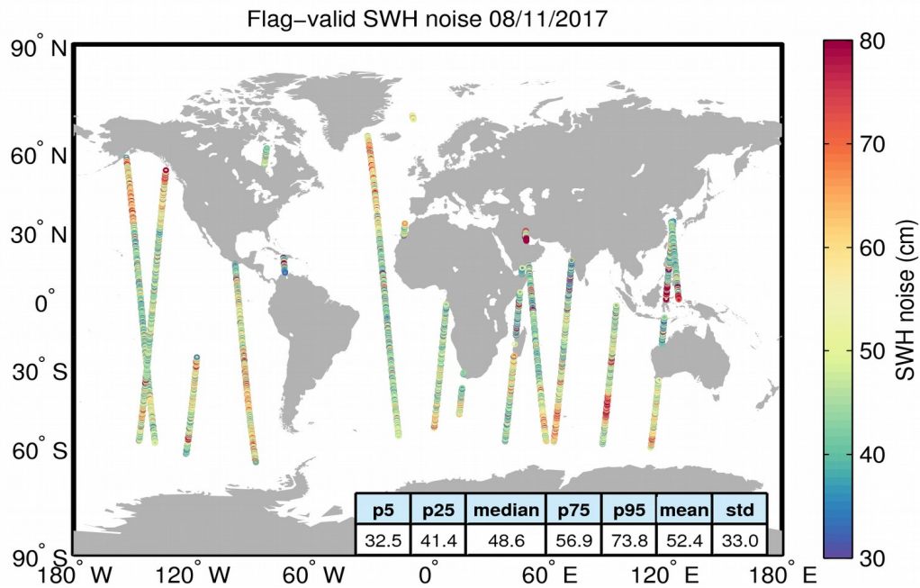
Figure 18. Geographical distribution of flag-valid 20-Hz SWH measurement noise over oceans and lakes for 08/11/2017. The statistical values shown in the table refer to the SWH noise and are calculated over all measurements shown in the figure.
