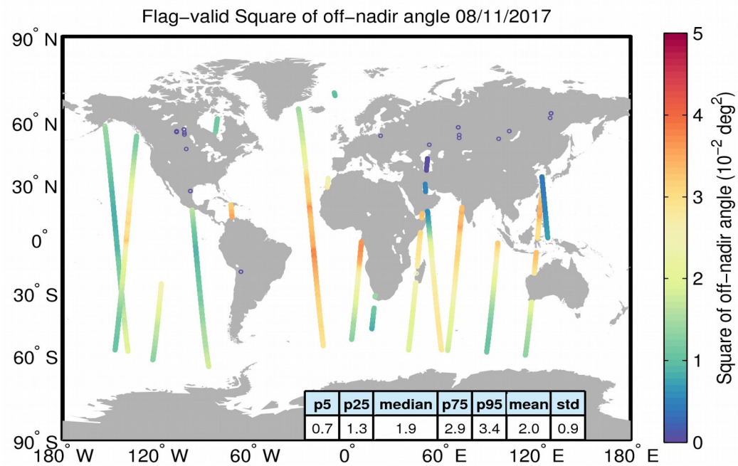
Figure 37. Geographical distribution of flag-valid mispointing data over oceans and lakes for 08/11/2017. The statistical values shown in the table refer to the mispointing in 10^{-2} deg 2 and are calculated over all measurements shown in the figure.
