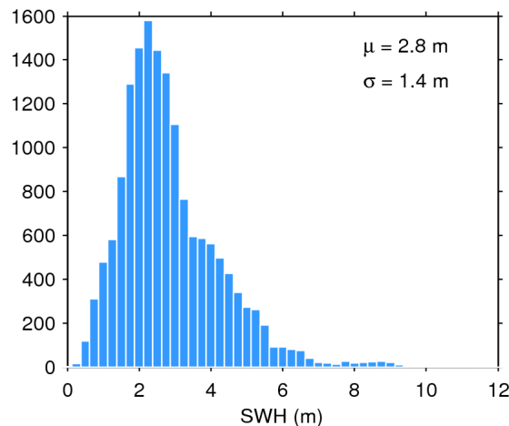
Figure 20. Histogram of science-valid SWH over oceans and lakes for 08/11/2017. The mean ( \mu ) and standard deviation ( \sigma ) are also shown. Note that values larger than 12 m are excluded from the histogram for the sake of readability but not from the computation of \mu and \sigma .
