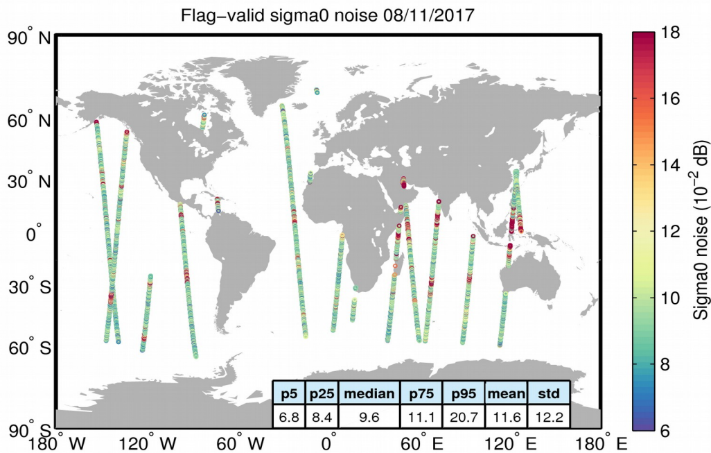
Figure 26. Geographical distribution of flag-valid 20-Hz sigma0 measurement noise over oceans and lakes for 08/11/2017. The statistical values shown in the table refer to the sigma0 noise and are calculated over all measurements shown in the figure.
