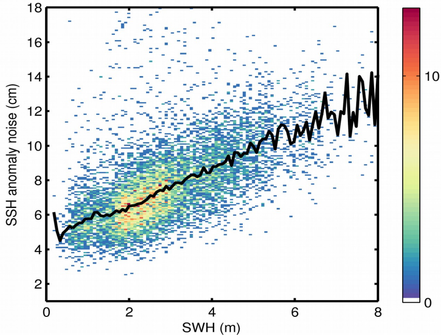
Figure 9. 2D histogram showing flag-valid SSH anomaly noise as a function of SWH for 08/11/2017. The black line denotes the median SSH anomaly noise as a function of SWH.
