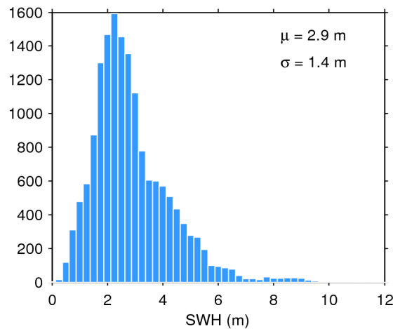
Figure 17. Histogram of flag-valid SWH over oceans and lakes for 08/11/2017. The mean ( \mu ) and standard deviation ( \sigma ) are also shown. Note that values larger than 12 m are excluded from the histogram for the sake of readability but not from the computation of \mu and \sigma .
