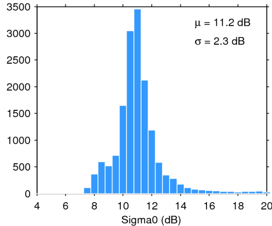
Figure 25. Histogram of flag-valid sigma0 over oceans and lakes for 08/11/2017. The mean ( \mu ) and standard deviation ( \sigma ) are also shown. Note that values outside [4 20] dB are excluded from the histogram for the sake of readability but not from the computation of \mu and \sigma .
