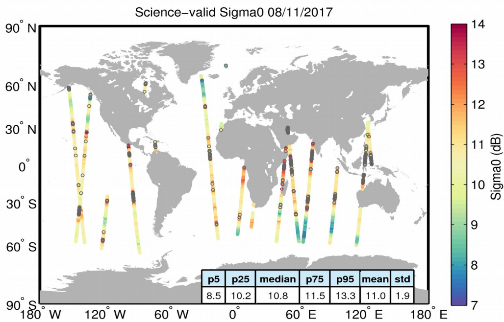
Figure 27. Geographical distribution of science-valid sigma0 data over oceans and lakes for 08/11/2017. The statistical values shown in the table refer to the sigma0 in dB and are calculated over all measurements shown in the figure. Gray circles denote records that have been rejected based on the editing criteria described in Table 4.
