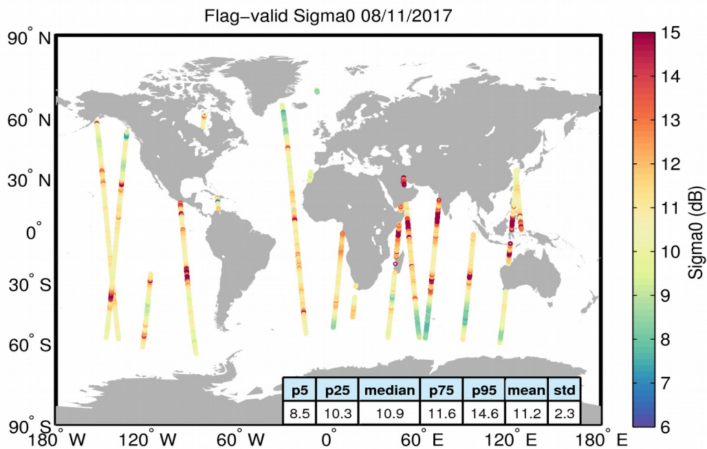
Figure 23. Geographical distribution of flag-valid sigma0 data over oceans and lakes for 08/11/2017. The statistical values shown in the table refer to the sigma0 in dB and are calculated over all measurements shown in the figure.
