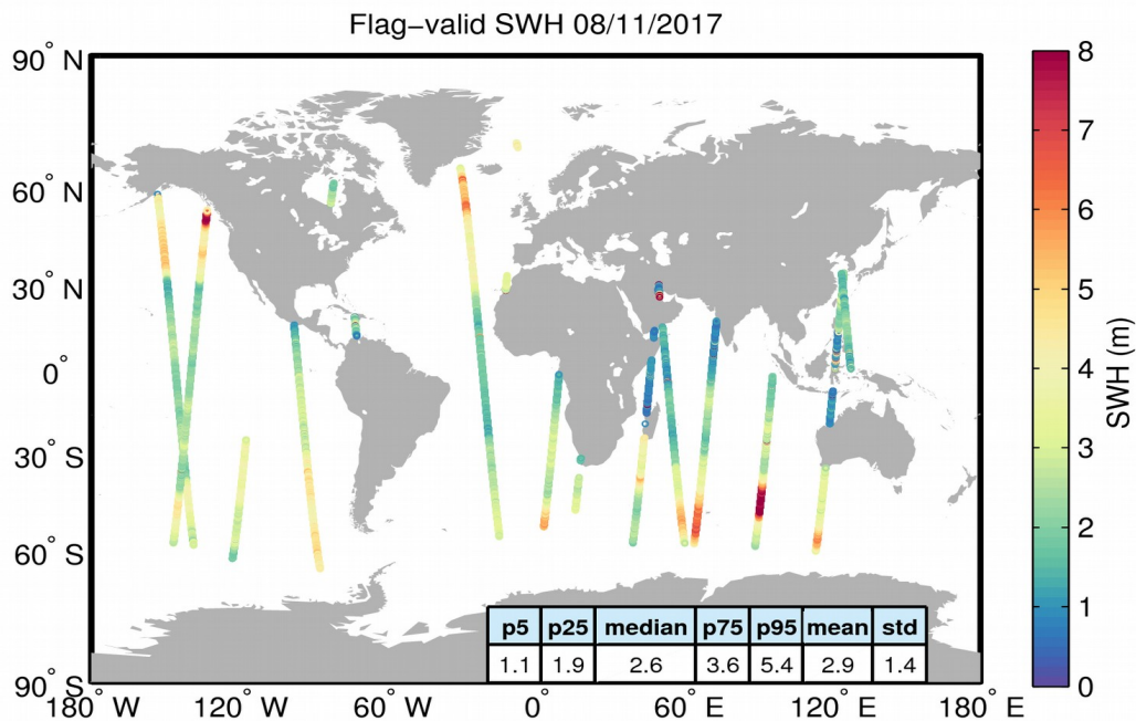
Figure 15. Geographical distribution of flag-valid SWH data over oceans and lakes for 08/11/2017. The statistical values shown in the table refer to the SWH in m and are calculated over all measurements shown in the figure.
