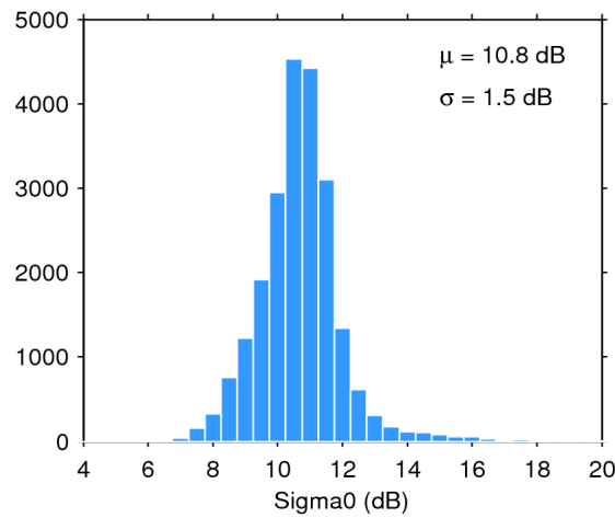
Figure 28. Histogram of science-valid sigma0 over oceans and lakes for 06/11/2017. The mean ( \mu ) and standard deviation ( \sigma ) are also shown. Note that values outside [4 20] dB are excluded from the histogram for the sake of readability but not from the computation of \mu and \sigma .
