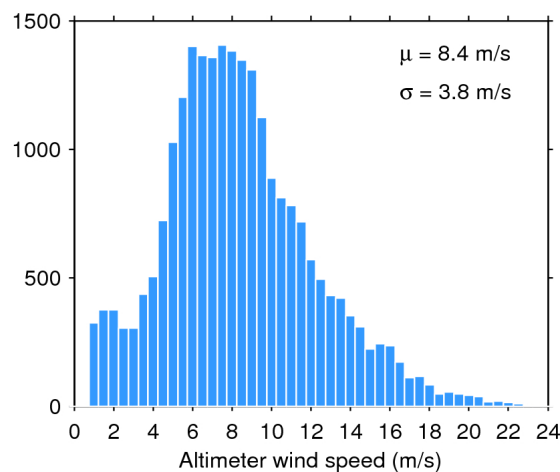
Figure 35. Histogram of science-valid wind over oceans and lakes for 06/11/2017. The mean ( \mu ) and standard deviation ( \sigma ) are also shown. Note that values larger than 24 m/s are excluded from the histogram for the sake of readability but not from the computation of \mu and \sigma .
