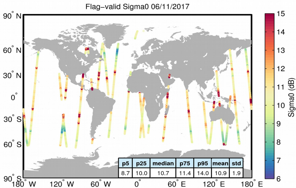
Figure 23. Geographical distribution of flag-valid sigma0 data over oceans and lakes for 06/11/2017. The statistical values shown in the table refer to the sigma0 in dB and are calculated over all measurements shown in the figure.
