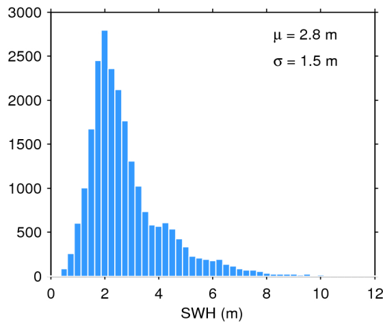
Figure 20. Histogram of science-valid SWH over oceans and lakes for 06/11/2017. The mean ( \mu ) and standard deviation ( \sigma ) are also shown. Note that values larger than 12 m are excluded from the histogram for the sake of readability but not from the computation of \mu and \sigma .
