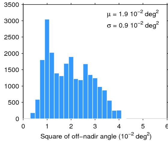
Figure 39. Histogram of flag-valid mispointing over oceans and lakes for 06/11/2017. The mean ( \mu ) and standard deviation ( \sigma ) are also shown. Note that values larger than 6 \cdot 10^{-2} \text{ deg}^2 are excluded from the histogram for the sake of readability but not from the computation of \mu and \sigma .
