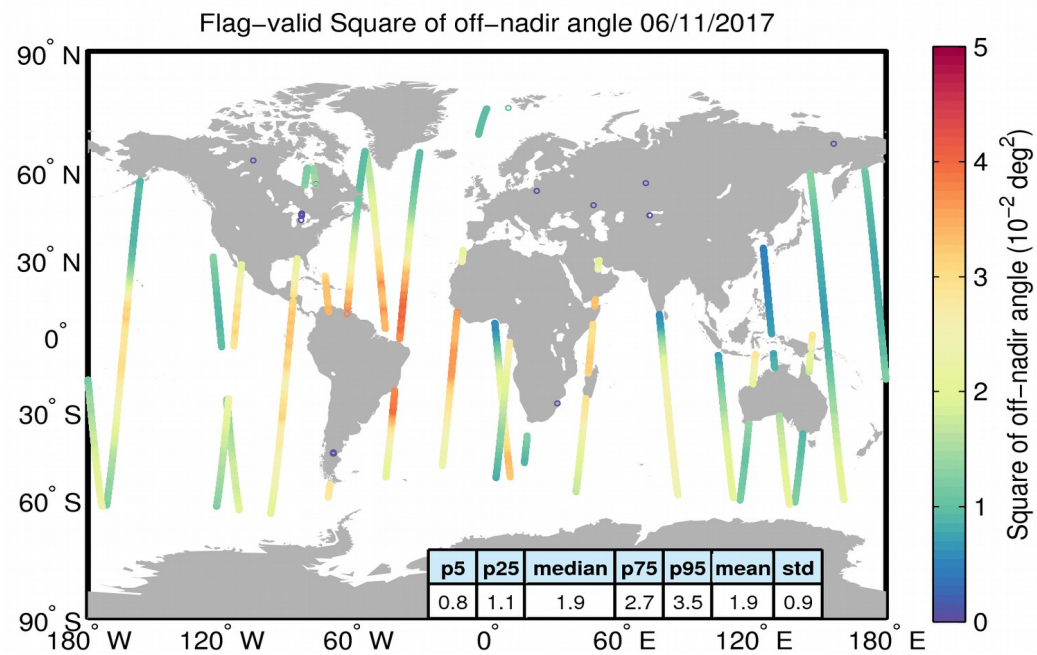
Figure 37. Geographical distribution of flag-valid mispointing data over oceans and lakes for 06/11/2017. The statistical values shown in the table refer to the mispointing in 10^{-2} deg 2 and are calculated over all measurements shown in the figure.
