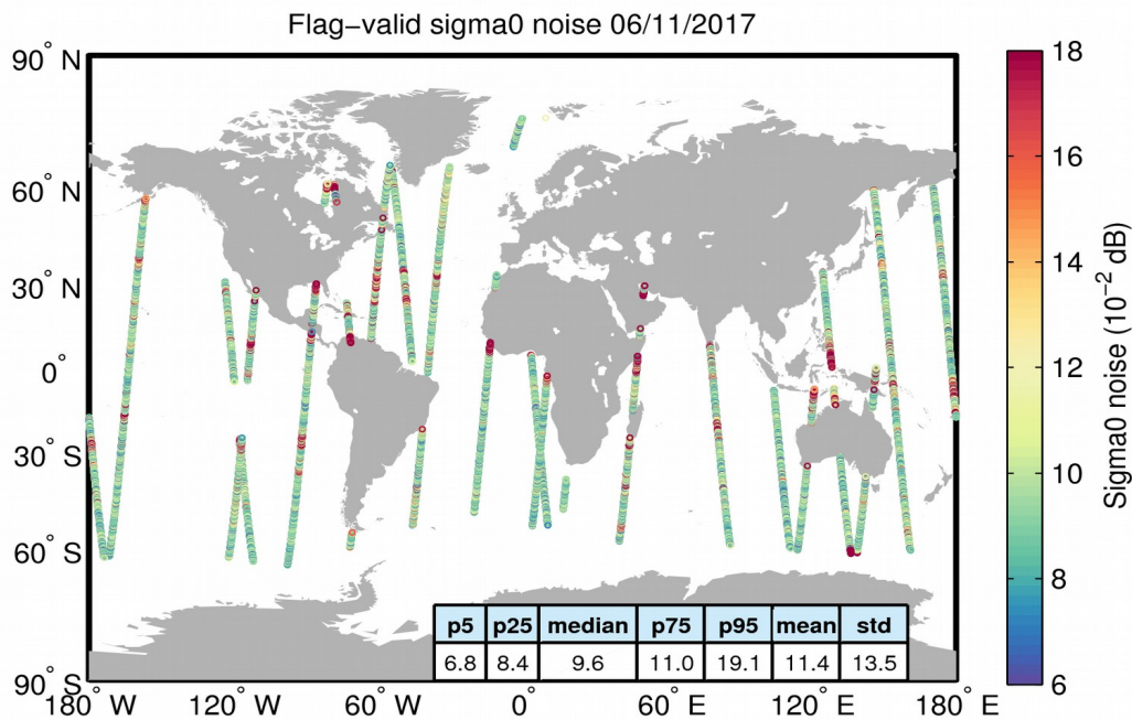
Figure 26. Geographical distribution of flag-valid 20-Hz sigma0 measurement noise over oceans and lakes for 06/11/2017. The statistical values shown in the table refer to the sigma0 noise and are calculated over all measurements shown in the figure.
