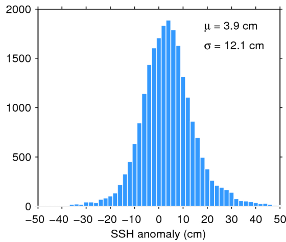
Figure 11. Histogram of science-valid SSH anomaly over oceans and lakes for 06/11/2017. The mean ( \mu ) and standard deviation ( \sigma ) are also shown. Note that values outside [-50 50] cm are excluded from the histogram for the sake of readability but not from the computation of \mu and \sigma .
