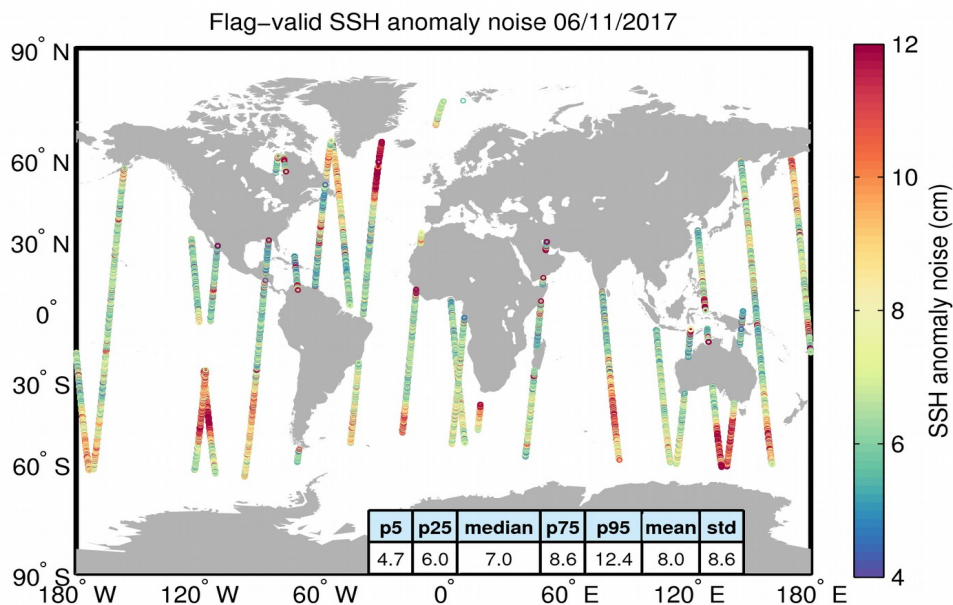
Figure 8. Geographical distribution of flag-valid 20-Hz SSH anomaly measurement noise over oceans and lakes for 06/11/2017. The statistical values shown in the table refer to the SSH anomaly noise and are calculated over all measurements shown in the figure.
