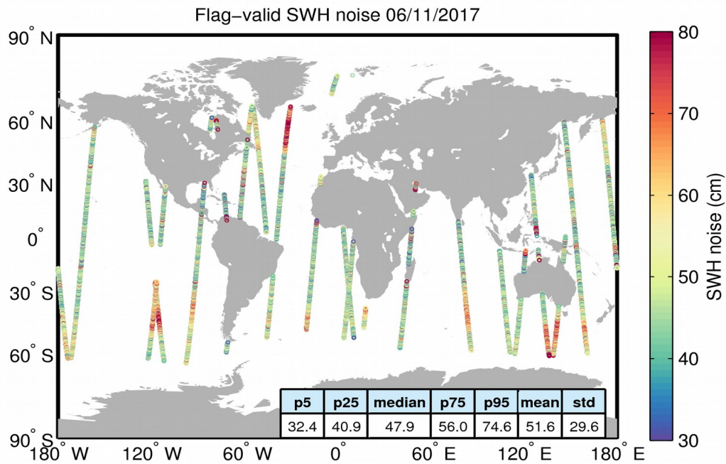
Figure 18. Geographical distribution of flag-valid 20-Hz SWH measurement noise over oceans and lakes for 06/11/2017. The statistical values shown in the table refer to the SWH noise and are calculated over all measurements shown in the figure.
