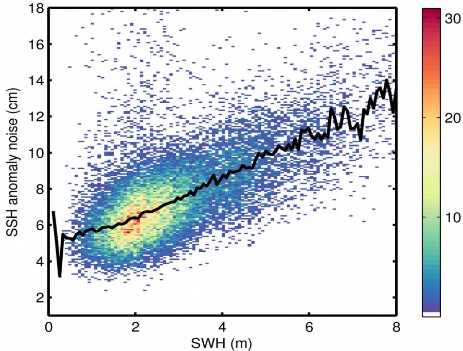
Figure 9. 2D histogram showing flag-valid SSH anomaly noise as a function of SWH for 06/11/2017. The black line denotes the median SSH anomaly noise as a function of SWH.
