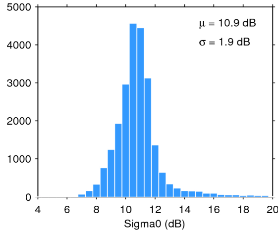
Figure 25. Histogram of flag-valid sigma0 over oceans and lakes for 06/11/2017. The mean ( \mu ) and standard deviation ( \sigma ) are also shown. Note that values outside [4 20] dB are excluded from the histogram for the sake of readability but not from the computation of \mu and \sigma .
