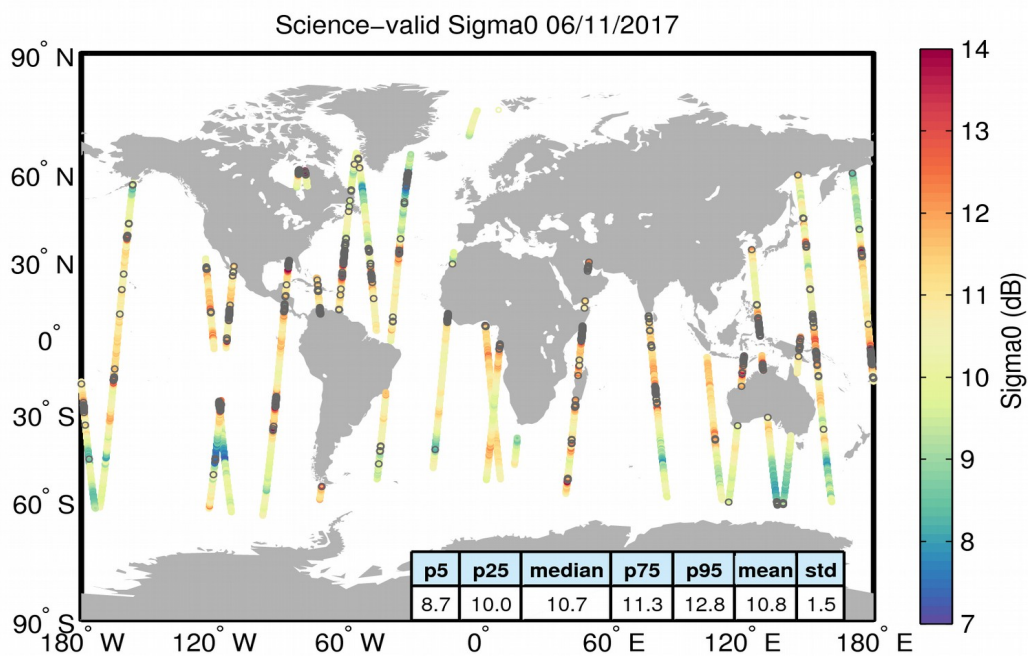
Figure 27. Geographical distribution of science-valid sigma0 data over oceans and lakes for 06/11/2017. The statistical values shown in the table refer to the sigma0 in dB and are calculated over all measurements shown in the figure. Gray circles denote records that have been rejected based on the editing criteria described in Table 4.
