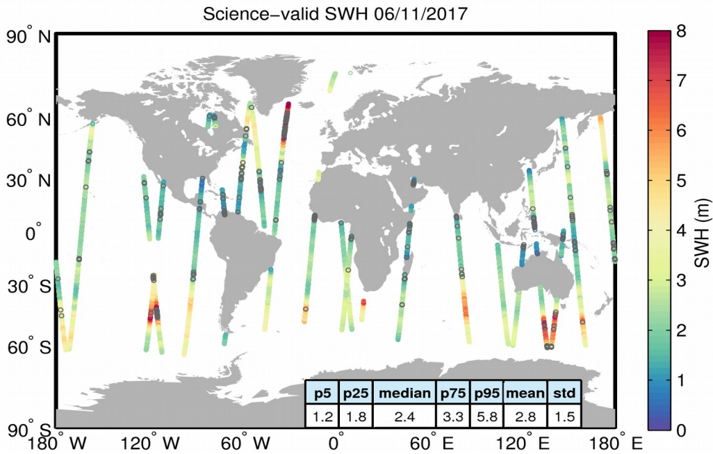
Figure 19. Geographical distribution of science-valid SWH data over oceans and lakes for 06/11/2017. The statistical values shown in the table refer to the SWH in m and are calculated over all measurements shown in the figure. Gray circles denote records that have been rejected based on the editing criteria described in Table 3.
