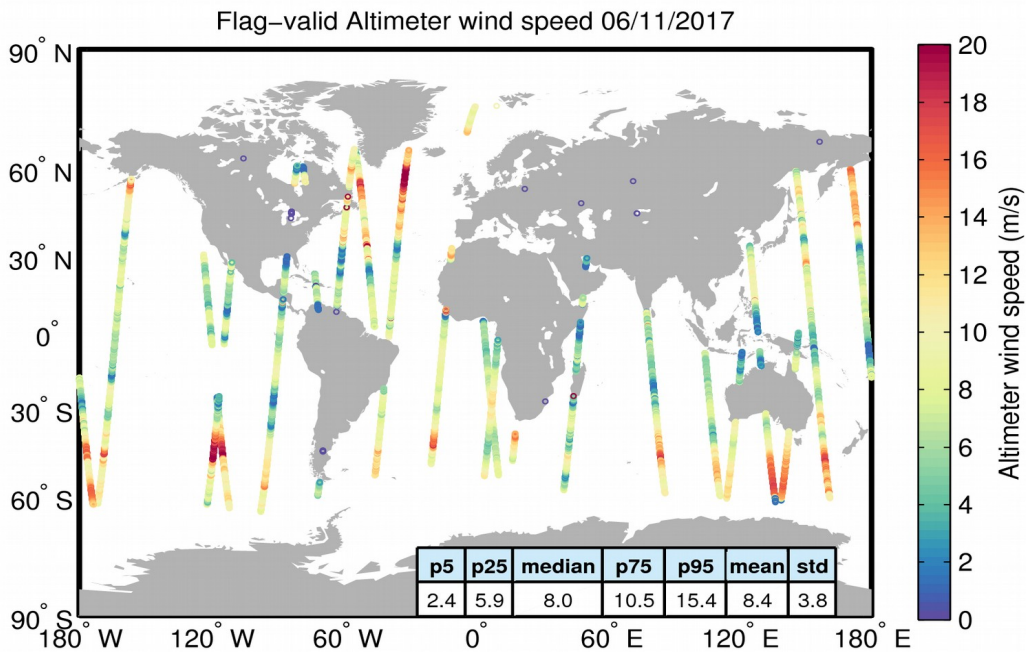
Figure 31. Geographical distribution of flag-valid wind data over oceans and lakes for 06/11/2017. The statistical values shown in the table refer to the wind in m/s and are calculated over all measurements shown in the figure.
