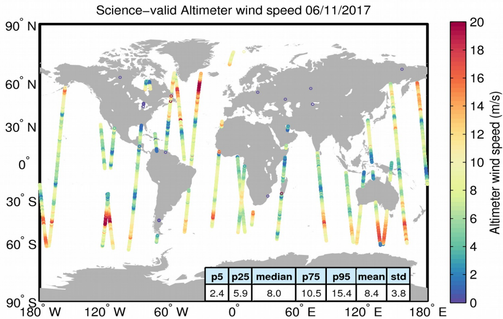
Figure 34. Geographical distribution of science-valid wind data over oceans and lakes for 06/11/2017. The statistical values shown in the table refer to the wind in m/s and are calculated over all measurements shown in the figure. Gray circles denote records that have been rejected based on the editing criteria described in Table 5.
