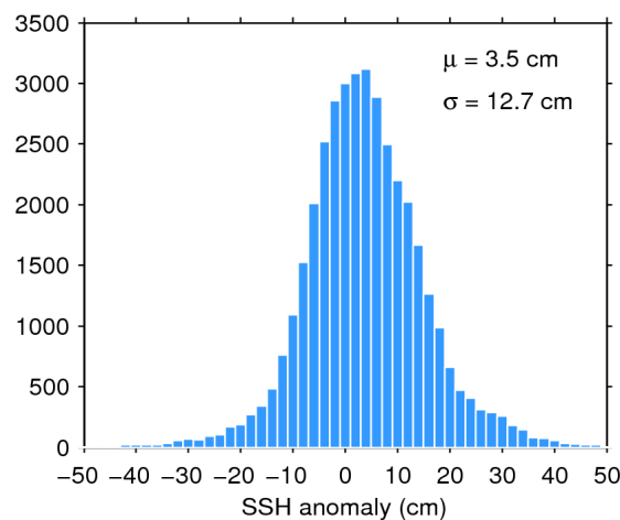
Figure 11. Histogram of science-valid SSH anomaly over oceans and lakes for 05/11/2017. The mean ( \mu ) and standard deviation ( \sigma ) are also shown. Note that values outside [-50 50] cm are excluded from the histogram for the sake of readability but not from the computation of \mu and \sigma .
