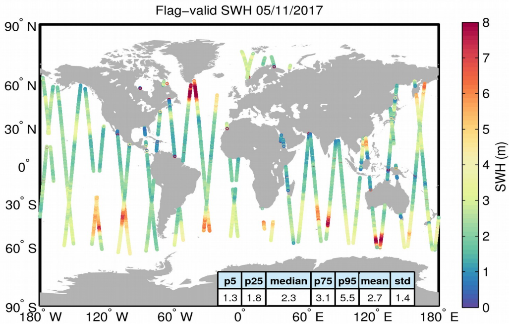
Figure 15. Geographical distribution of flag-valid SWH data over oceans and lakes for 05/11/2017. The statistical values shown in the table refer to the SWH in m and are calculated over all measurements shown in the figure.
