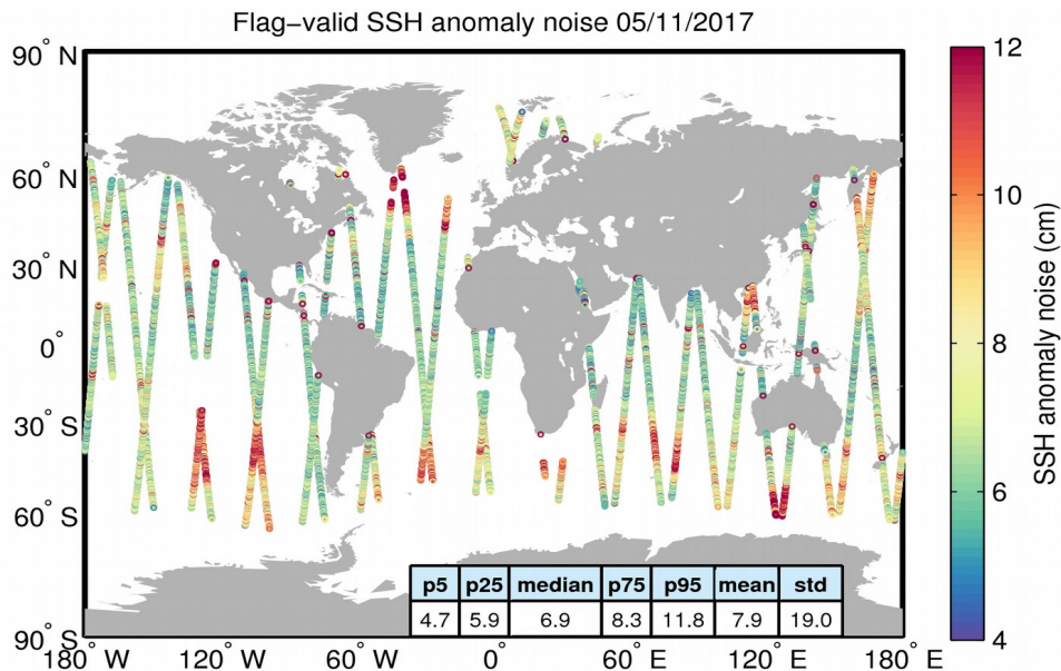
Figure 8. Geographical distribution of flag-valid 20-Hz SSH anomaly measurement noise over oceans and lakes for 05/11/2017. The statistical values shown in the table refer to the SSH anomaly noise and are calculated over all measurements shown in the figure.
