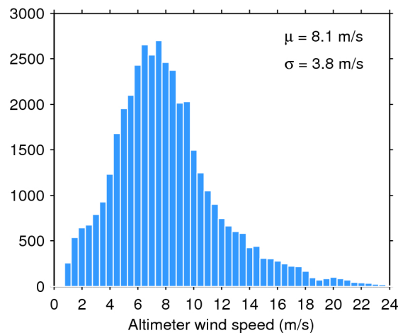
Figure 35. Histogram of science-valid wind over oceans and lakes for 05/11/2017. The mean ( \mu ) and standard deviation ( \sigma ) are also shown. Note that values larger than 24 m/s are excluded from the histogram for the sake of readability but not from the computation of \mu and \sigma .
