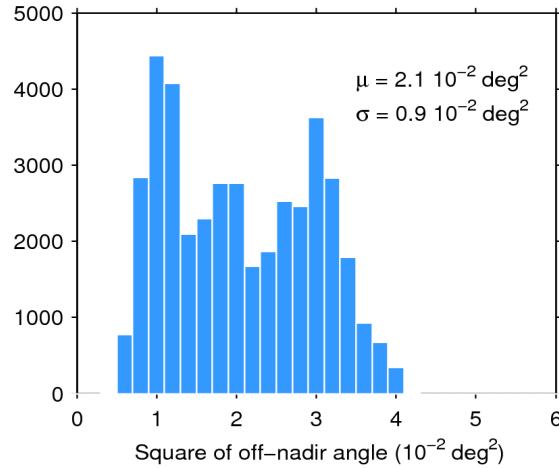
Figure 39. Histogram of flag-valid mispointing over oceans and lakes for 05/11/2017. The mean ( \mu ) and standard deviation ( \sigma ) are also shown. Note that values larger than 6 \cdot 10^{-2} \text{ deg}^2 are excluded from the histogram for the sake of readability but not from the computation of \mu and \sigma .
