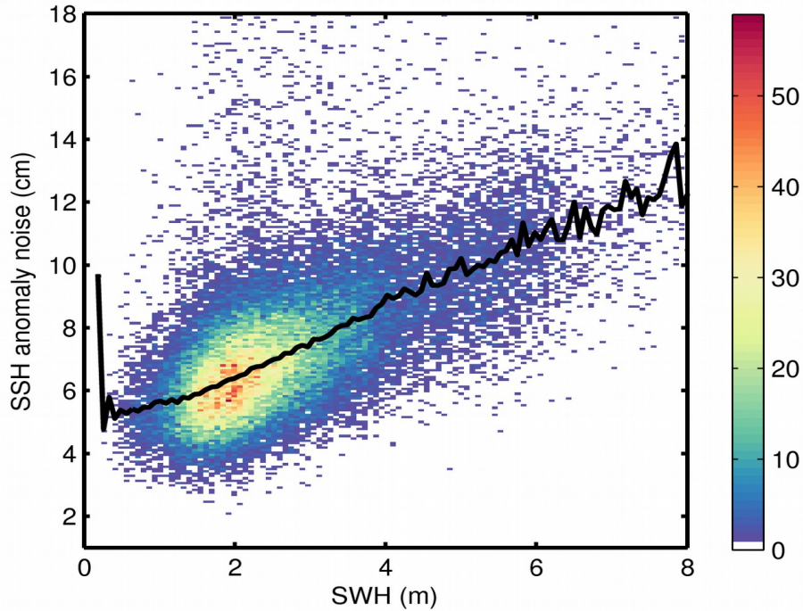
Figure 9. 2D histogram showing flag-valid SSH anomaly noise as a function of SWH for 05/11/2017. The black line denotes the median SSH anomaly noise as a function of SWH.
