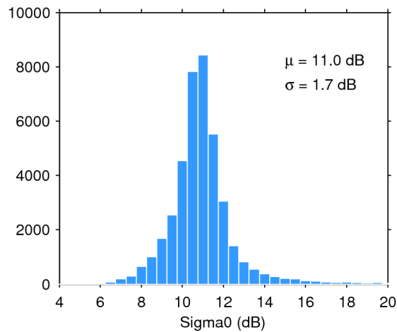
Figure 25. Histogram of flag-valid sigma0 over oceans and lakes for 05/11/2017. The mean ( \mu ) and standard deviation ( \sigma ) are also shown. Note that values outside [4 20] dB are excluded from the histogram for the sake of readability but not from the computation of \mu and \sigma .
