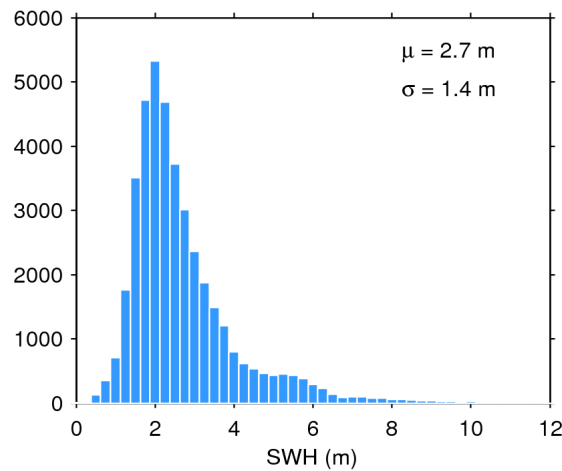
Figure 17. Histogram of flag-valid SWH over oceans and lakes for 05/11/2017. The mean ( \mu ) and standard deviation ( \sigma ) are also shown. Note that values larger than 12 m are excluded from the histogram for the sake of readability but not from the computation of \mu and \sigma .
