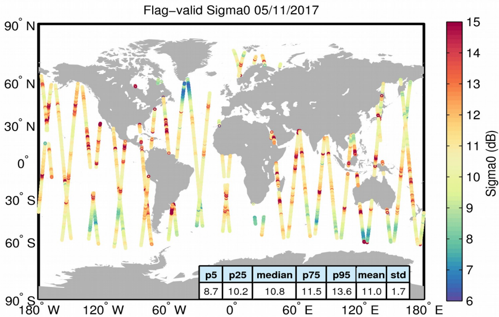
Figure 23. Geographical distribution of flag-valid sigma0 data over oceans and lakes for 05/11/2017. The statistical values shown in the table refer to the sigma0 in dB and are calculated over all measurements shown in the figure.
