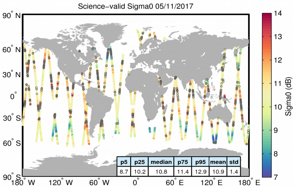
Figure 27. Geographical distribution of science-valid sigma0 data over oceans and lakes for 05/11/2017. The statistical values shown in the table refer to the sigma0 in dB and are calculated over all measurements shown in the figure. Gray circles denote records that have been rejected based on the editing criteria described in Table 4.
