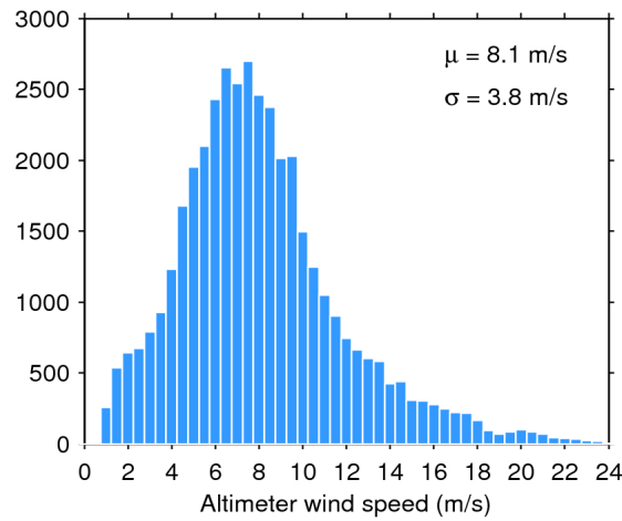
Figure 33. Histogram of flag-valid wind over oceans and lakes for 05/11/2017. The mean ( \mu ) and standard deviation ( \sigma ) are also shown. Note that values larger than 24 m/s are excluded from the histogram for the sake of readability but not from the computation of \mu and \sigma .
