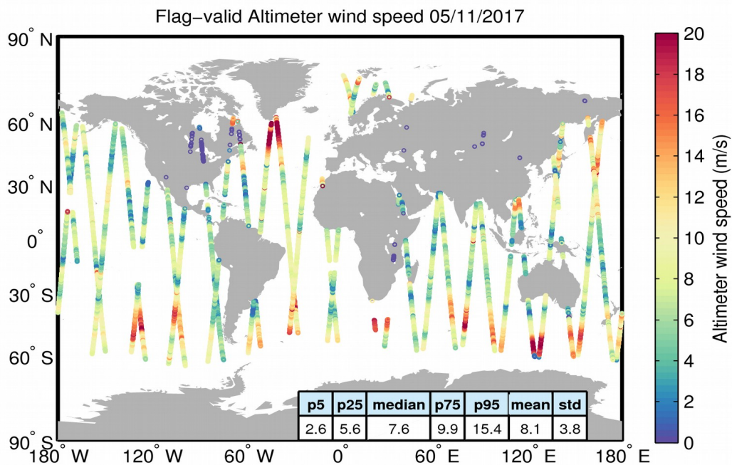
Figure 31. Geographical distribution of flag-valid wind data over oceans and lakes for 05/11/2017. The statistical values shown in the table refer to the wind in m/s and are calculated over all measurements shown in the figure.
