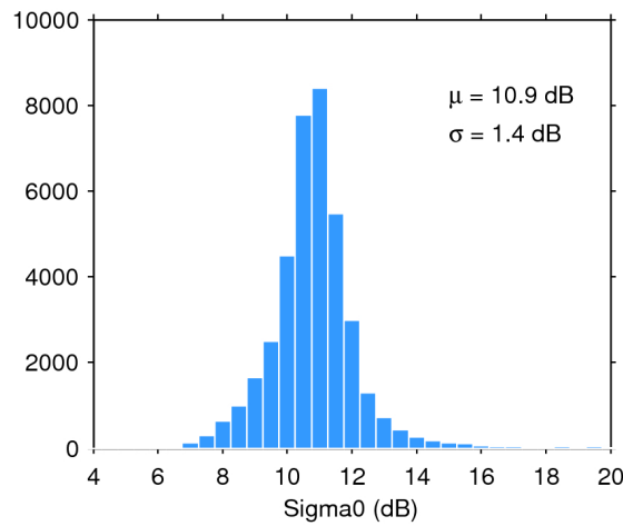
Figure 28. Histogram of science-valid sigma0 over oceans and lakes for 05/11/2017. The mean ( \mu ) and standard deviation ( \sigma ) are also shown. Note that values outside [4 20] dB are excluded from the histogram for the sake of readability but not from the computation of \mu and \sigma .
