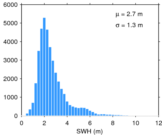
Figure 20. Histogram of science-valid SWH over oceans and lakes for 05/11/2017. The mean ( \mu ) and standard deviation ( \sigma ) are also shown. Note that values larger than 12 m are excluded from the histogram for the sake of readability but not from the computation of \mu and \sigma .
