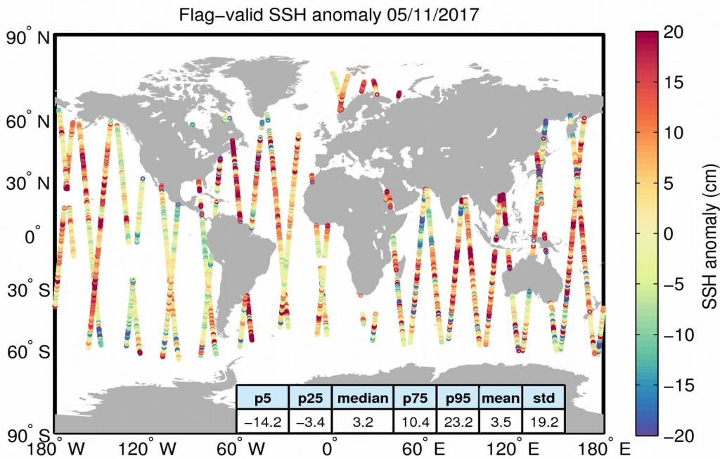
Figure 5. Geographical distribution of flag-valid 1-Hz SSH anomaly data over oceans and lakes for 05/11/2017. The statistical values shown in the table refer to the SSH anomaly in cm and are calculated over all measurements shown in the figure.
