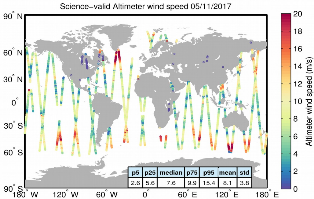
Figure 34. Geographical distribution of science-valid wind data over oceans and lakes for 05/11/2017. The statistical values shown in the table refer to the wind in m/s and are calculated over all measurements shown in the figure. Gray circles denote records that have been rejected based on the editing criteria described in Table 5.
