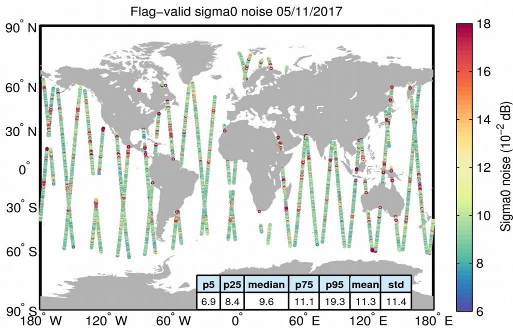
Figure 26. Geographical distribution of flag-valid 20-Hz sigma0 measurement noise over oceans and lakes for 05/11/2017. The statistical values shown in the table refer to the sigma0 noise and are calculated over all measurements shown in the figure.
