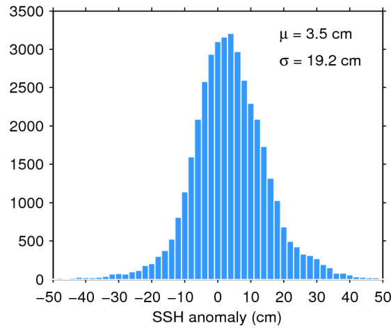
Figure 7. Histogram of flag-valid SSH anomaly over oceans and lakes for 05/11/2017. The mean ( \mu ) and standard deviation ( \sigma ) are also shown. Note that values outside [-50 50] cm are excluded from the histogram for the sake of readability but not from the computation of \mu and \sigma .
