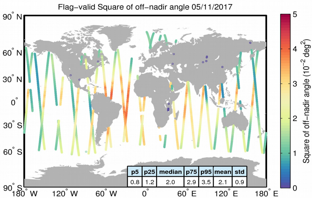
Figure 37. Geographical distribution of flag-valid mispointing data over oceans and lakes for 05/11/2017. The statistical values shown in the table refer to the mispointing in 10^{-2} deg 2 and are calculated over all measurements shown in the figure.
