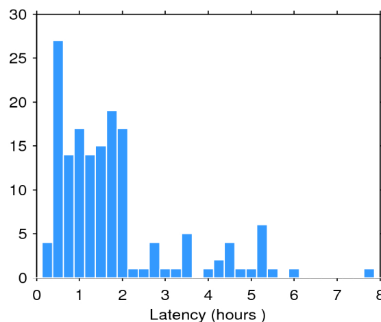
Figure 2. Histogram of the data latency for 05/11/2017. The y-axis denotes the number of files that are made available with a delay of x-hours with respect to the mean time of the records stored in the file.
