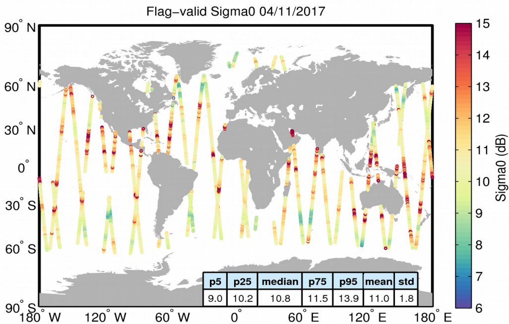
Figure 23. Geographical distribution of flag-valid sigma0 data over oceans and lakes for 04/11/2017. The statistical values shown in the table refer to the sigma0 in dB and are calculated over all measurements shown in the figure.
