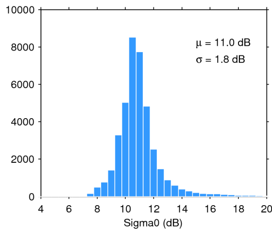
Figure 25. Histogram of flag-valid sigma0 over oceans and lakes for 04/11/2017. The mean ( \mu ) and standard deviation ( \sigma ) are also shown. Note that values outside [4 20] dB are excluded from the histogram for the sake of readability but not from the computation of \mu and \sigma .
