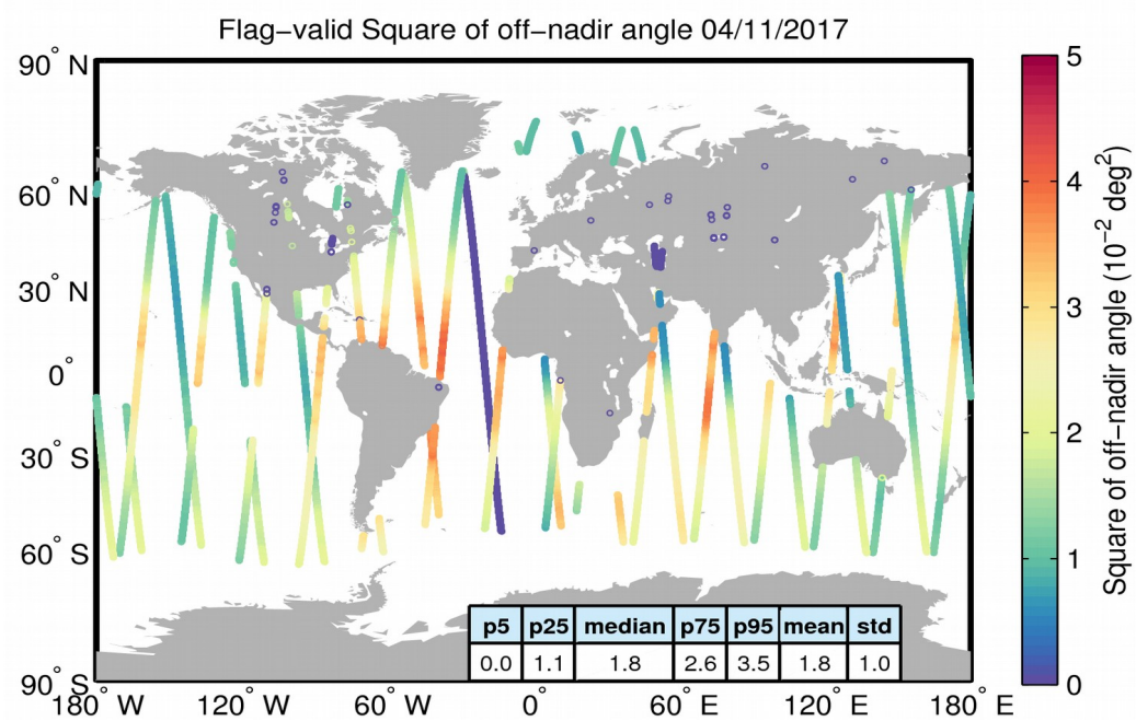
Figure 37. Geographical distribution of flag-valid mispointing data over oceans and lakes for 04/11/2017. The statistical values shown in the table refer to the mispointing in 10^{-2} \text{ deg}^2 and are calculated over all measurements shown in the figure.
