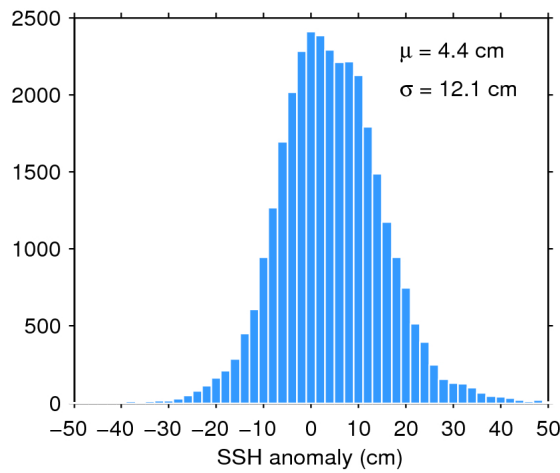
Figure 11. Histogram of science-valid SSH anomaly over oceans and lakes for 04/11/2017. The mean ( \mu ) and standard deviation ( \sigma ) are also shown. Note that values outside [-50 50] cm are excluded from the histogram for the sake of readability but not from the computation of \mu and \sigma .
