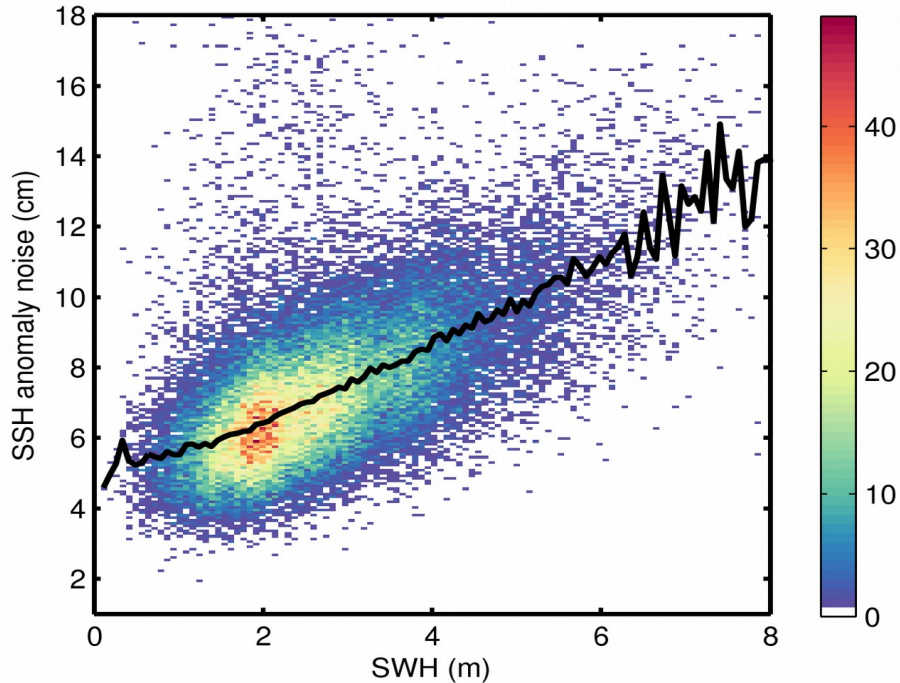
Figure 9. 2D histogram showing flag-valid SSH anomaly noise as a function of SWH for 04/11/2017. The black line denotes the median SSH anomaly noise as a function of SWH.
