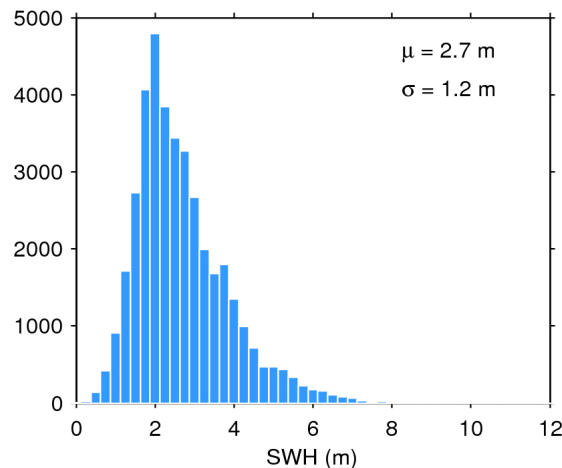
Figure 20. Histogram of science-valid SWH over oceans and lakes for 04/11/2017. The mean ( \mu ) and standard deviation ( \sigma ) are also shown. Note that values larger than 12 m are excluded from the histogram for the sake of readability but not from the computation of \mu and \sigma .
