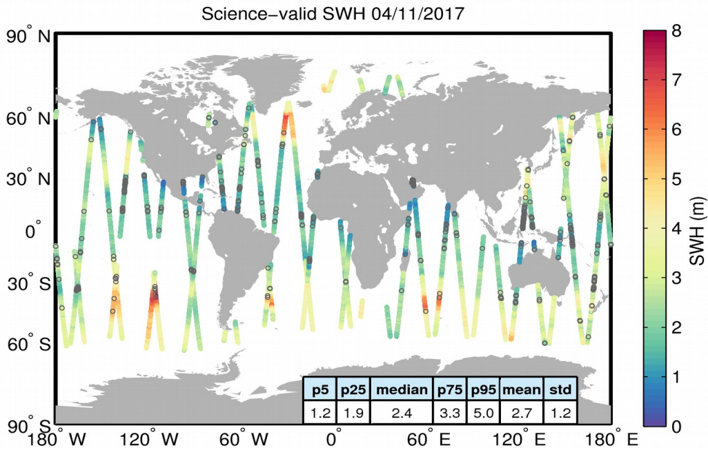
Figure 19. Geographical distribution of science-valid SWH data over oceans and lakes for 04/11/2017. The statistical values shown in the table refer to the SWH in m and are calculated over all measurements shown in the figure. Gray circles denote records that have been rejected based on the editing criteria described in Table 3.
