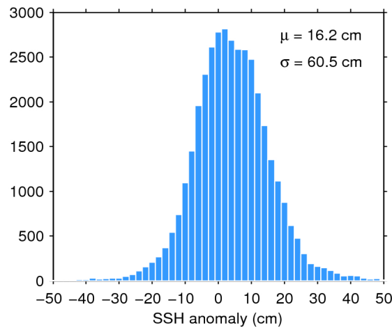
Figure 7. Histogram of flag-valid SSH anomaly over oceans and lakes for 04/11/2017. The mean ( \mu ) and standard deviation ( \sigma ) are also shown. Note that values outside [-50 50] cm are excluded from the histogram for the sake of readability but not from the computation of \mu and \sigma .
