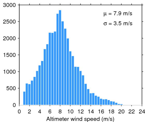
Figure 35. Histogram of science-valid wind over oceans and lakes for 04/11/2017. The mean ( \mu ) and standard deviation ( \sigma ) are also shown. Note that values larger than 24 m/s are excluded from the histogram for the sake of readability but not from the computation of \mu and \sigma .
