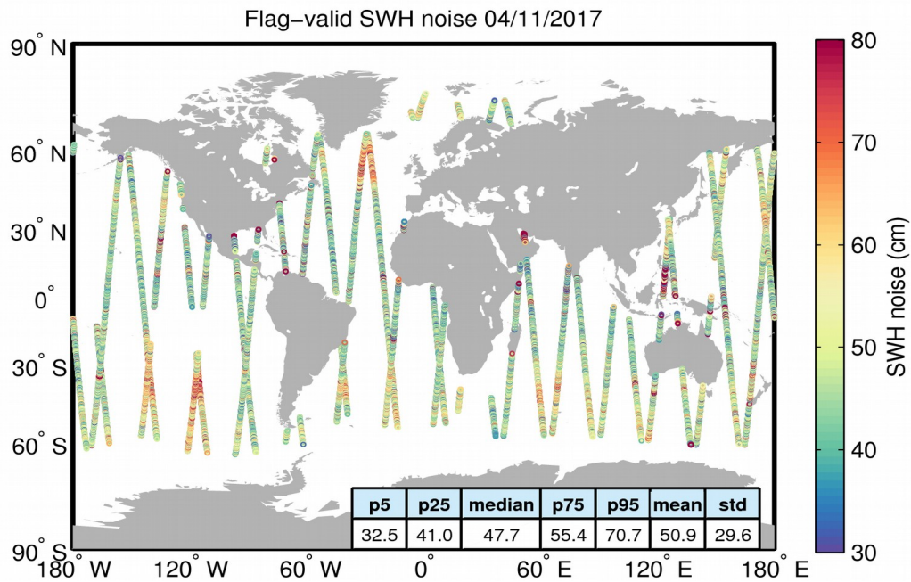
Figure 18. Geographical distribution of flag-valid 20-Hz SWH measurement noise over oceans and lakes for 04/11/2017. The statistical values shown in the table refer to the SWH noise and are calculated over all measurements shown in the figure.
