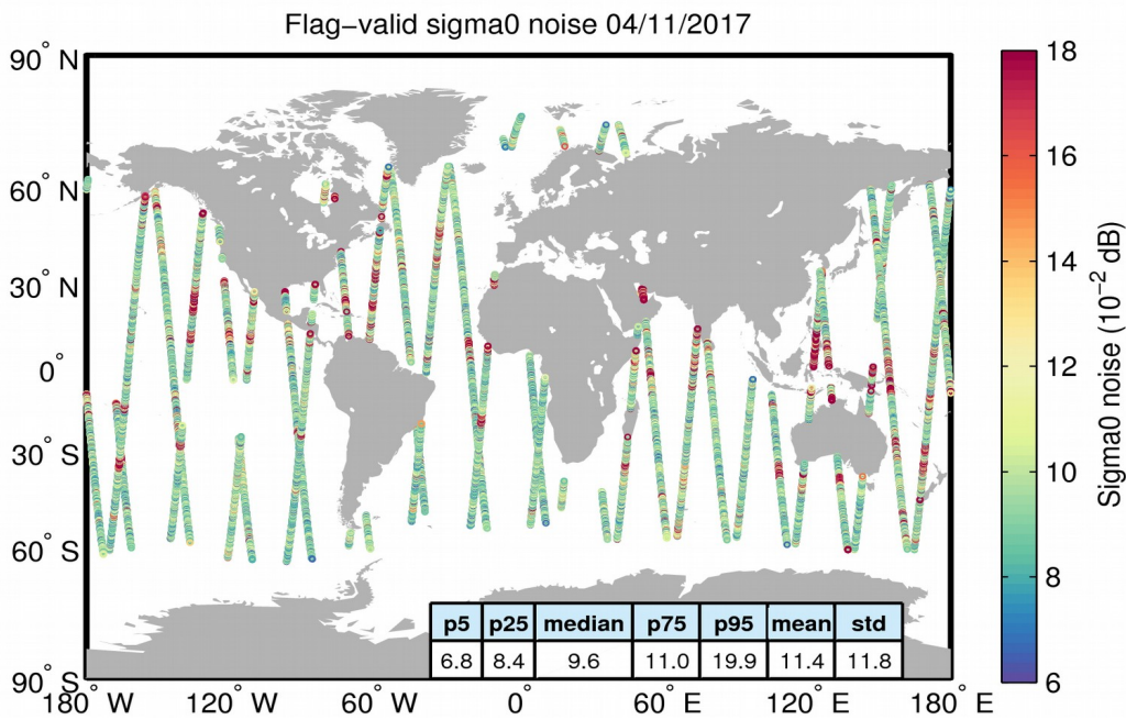
Figure 26. Geographical distribution of flag-valid 20-Hz sigma0 measurement noise over oceans and lakes for 04/11/2017. The statistical values shown in the table refer to the sigma0 noise and are calculated over all measurements shown in the figure.
