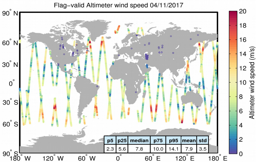
Figure 31. Geographical distribution of flag-valid wind data over oceans and lakes for 04/11/2017. The statistical values shown in the table refer to the wind in m/s and are calculated over all measurements shown in the figure.
