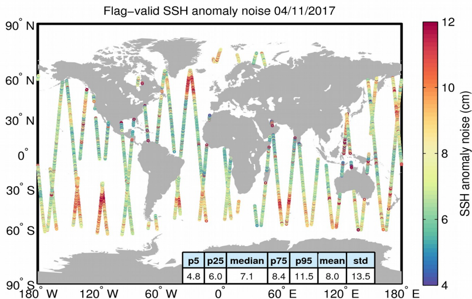
Figure 8. Geographical distribution of flag-valid 20-Hz SSH anomaly measurement noise over oceans and lakes for 04/11/2017. The statistical values shown in the table refer to the SSH anomaly noise and are calculated over all measurements shown in the figure.
