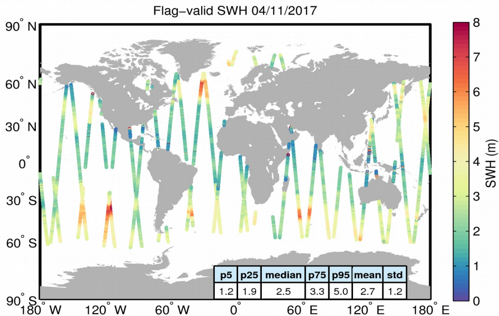
Figure 15. Geographical distribution of flag-valid SWH data over oceans and lakes for 04/11/2017. The statistical values shown in the table refer to the SWH in m and are calculated over all measurements shown in the figure.
