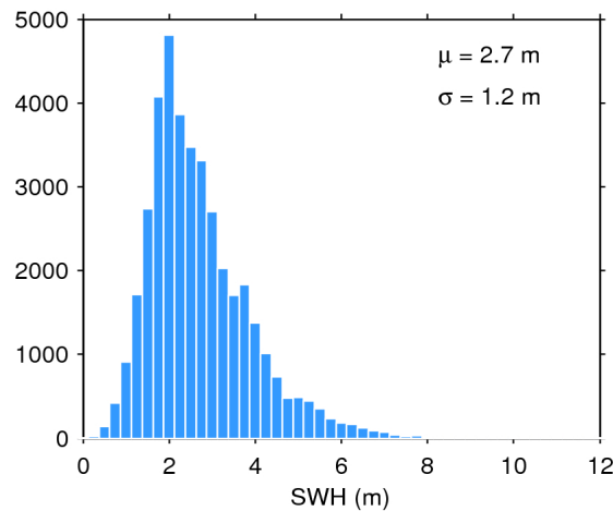
Figure 17. Histogram of flag-valid SWH over oceans and lakes for 04/11/2017. The mean ( \mu ) and standard deviation ( \sigma ) are also shown. Note that values larger than 12 m are excluded from the histogram for the sake of readability but not from the computation of \mu and \sigma .
