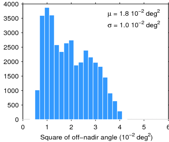
Figure 39. Histogram of flag-valid mispointing over oceans and lakes for 04/11/2017. The mean ( \mu ) and standard deviation ( \sigma ) are also shown. Note that values larger than 6 \cdot 10^{-2} \text{ deg}^2 are excluded from the histogram for the sake of readability but not from the computation of \mu and \sigma .
