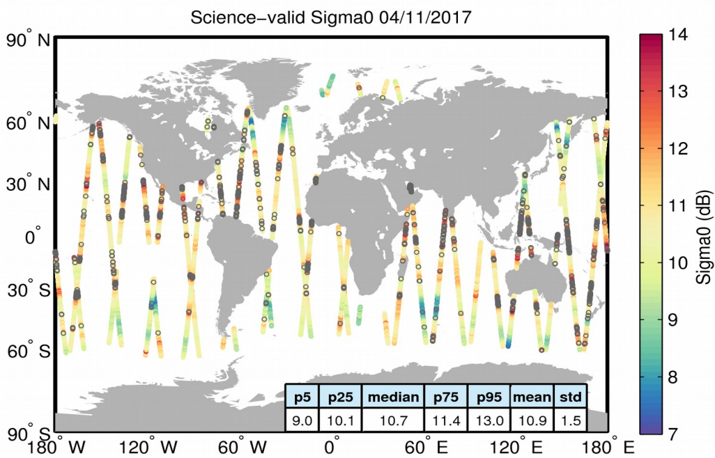
Figure 27. Geographical distribution of science-valid sigma0 data over oceans and lakes for 04/11/2017. The statistical values shown in the table refer to the sigma0 in dB and are calculated over all measurements shown in the figure. Gray circles denote records that have been rejected based on the editing criteria described in Table 4.
