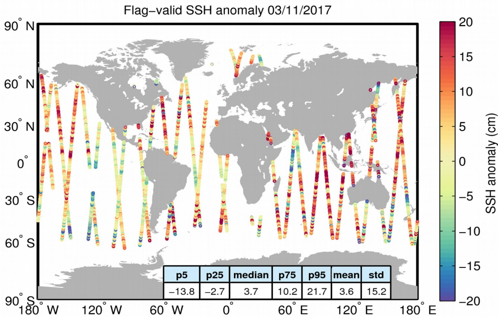
Figure 5. Geographical distribution of flag-valid 1-Hz SSH anomaly data over oceans and lakes for 03/11/2017. The statistical values shown in the table refer to the SSH anomaly in cm and are calculated over all measurements shown in the figure.
