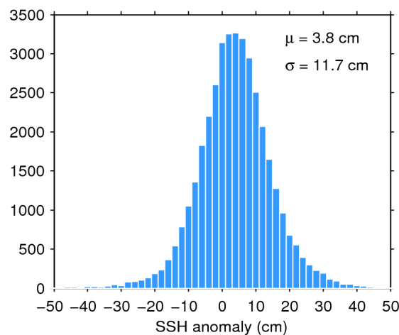
Figure 11. Histogram of science-valid SSH anomaly over oceans and lakes for 03/11/2017. The mean ( \mu ) and standard deviation ( \sigma ) are also shown. Note that values outside [-50 50] cm are excluded from the histogram for the sake of readability but not from the computation of \mu and \sigma .
