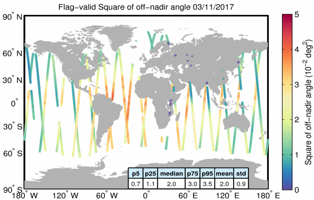
Figure 37. Geographical distribution of flag-valid mispointing data over oceans and lakes for 03/11/2017. The statistical values shown in the table refer to the mispointing in 10^{-2} deg 2 and are calculated over all measurements shown in the figure.
