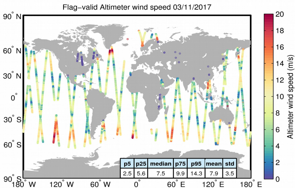
Figure 31. Geographical distribution of flag-valid wind data over oceans and lakes for 03/11/2017. The statistical values shown in the table refer to the wind in m/s and are calculated over all measurements shown in the figure.
