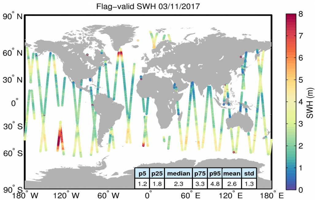
Figure 15. Geographical distribution of flag-valid SWH data over oceans and lakes for 03/11/2017. The statistical values shown in the table refer to the SWH in m and are calculated over all measurements shown in the figure.
