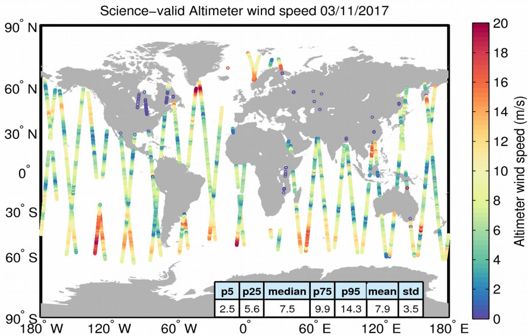
Figure 34. Geographical distribution of science-valid wind data over oceans and lakes for 03/11/2017. The statistical values shown in the table refer to the wind in m/s and are calculated over all measurements shown in the figure. Gray circles denote records that have been rejected based on the editing criteria described in Table 5.
