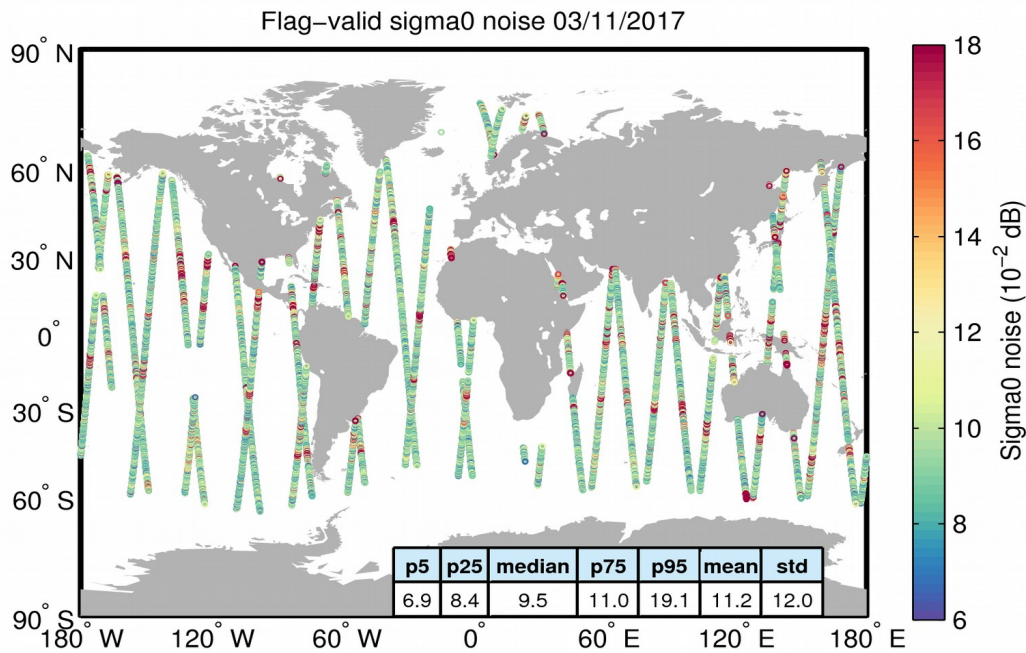
Figure 26. Geographical distribution of flag-valid 20-Hz sigma0 measurement noise over oceans and lakes for 03/11/2017. The statistical values shown in the table refer to the sigma0 noise and are calculated over all measurements shown in the figure.
