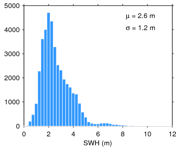
Figure 20. Histogram of science-valid SWH over oceans and lakes for 03/11/2017. The mean ( \mu ) and standard deviation ( \sigma ) are also shown. Note that values larger than 12 m are excluded from the histogram for the sake of readability but not from the computation of \mu and \sigma .
