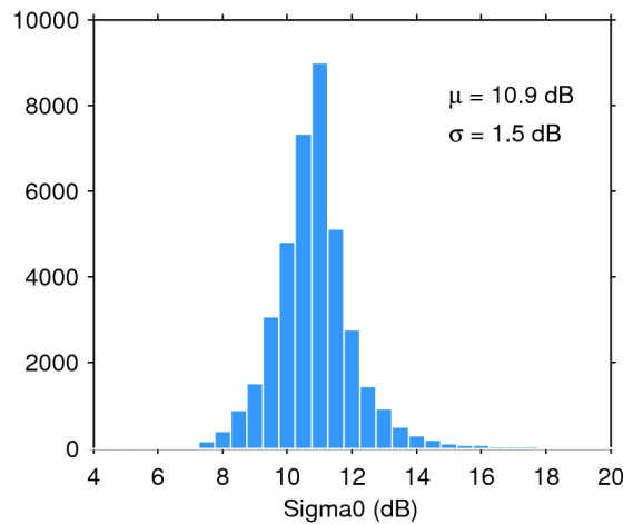
Figure 28. Histogram of science-valid sigma0 over oceans and lakes for 03/11/2017. The mean ( \mu ) and standard deviation ( \sigma ) are also shown. Note that values outside [4 20] dB are excluded from the histogram for the sake of readability but not from the computation of \mu and \sigma .
