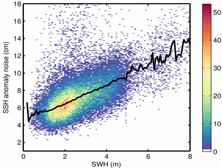
Figure 9. 2D histogram showing flag-valid SSH anomaly noise as a function of SWH for 03/11/2017. The black line denotes the median SSH anomaly noise as a function of SWH.
