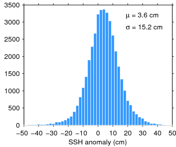
Figure 7. Histogram of flag-valid SSH anomaly over oceans and lakes for 03/11/2017. The mean ( \mu ) and standard deviation ( \sigma ) are also shown. Note that values outside [-50\ 50] cm are excluded from the histogram for the sake of readability but not from the computation of \mu and \sigma .
