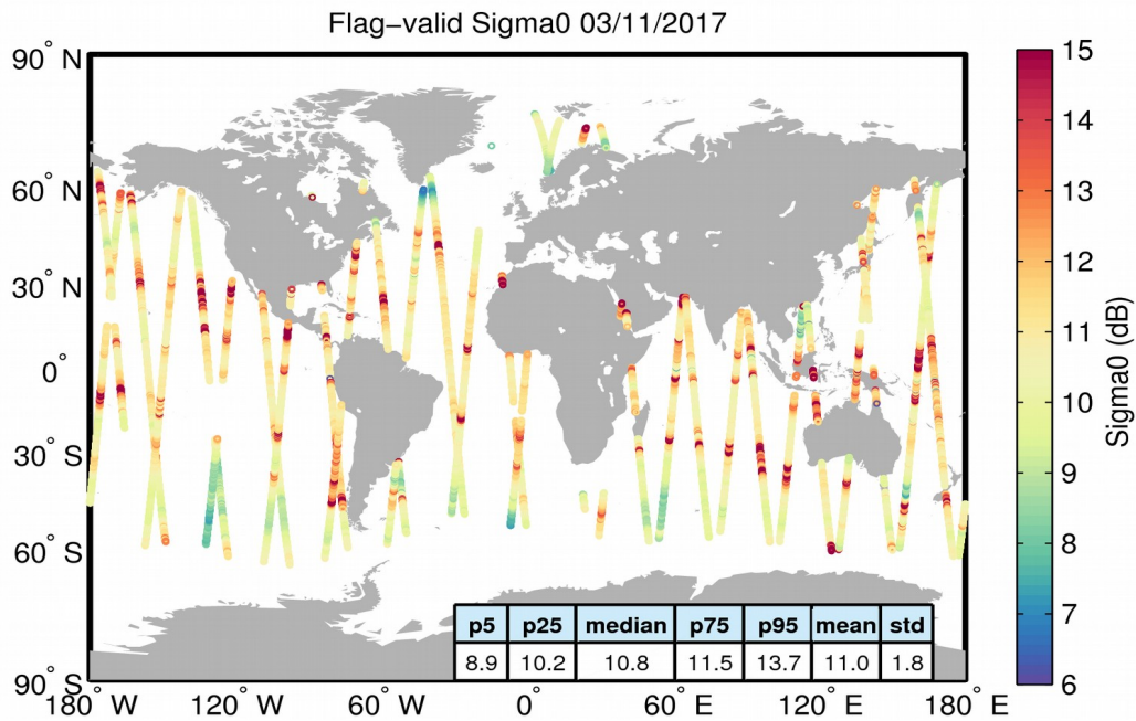
Figure 23. Geographical distribution of flag-valid sigma0 data over oceans and lakes for 03/11/2017. The statistical values shown in the table refer to the sigma0 in dB and are calculated over all measurements shown in the figure.
