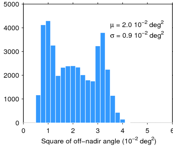
Figure 39. Histogram of flag-valid mispointing over oceans and lakes for 03/11/2017. The mean ( \mu ) and standard deviation ( \sigma ) are also shown. Note that values larger than 6 \cdot 10^{-2} \text{ deg}^2 are excluded from the histogram for the sake of readability but not from the computation of \mu and \sigma .
