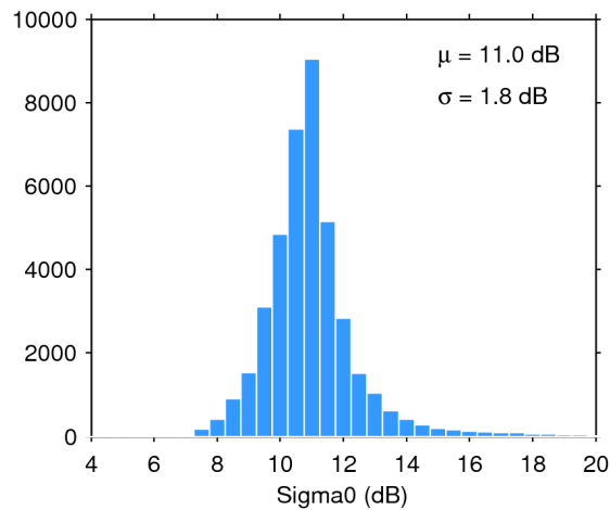
Figure 25. Histogram of flag-valid sigma0 over oceans and lakes for 03/11/2017. The mean ( \mu ) and standard deviation ( \sigma ) are also shown. Note that values outside [4 20] dB are excluded from the histogram for the sake of readability but not from the computation of \mu and \sigma .
