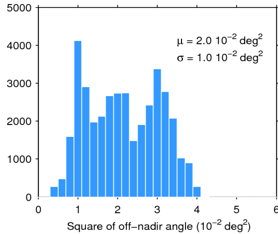
Figure 39. Histogram of flag-valid mispointing over oceans and lakes for 31/10/2017. The mean ( \mu ) and standard deviation ( \sigma ) are also shown. Note that values larger than 6 \cdot 10^{-2} \text{ deg}^2 are excluded from the histogram for the sake of readability but not from the computation of \mu and \sigma .
