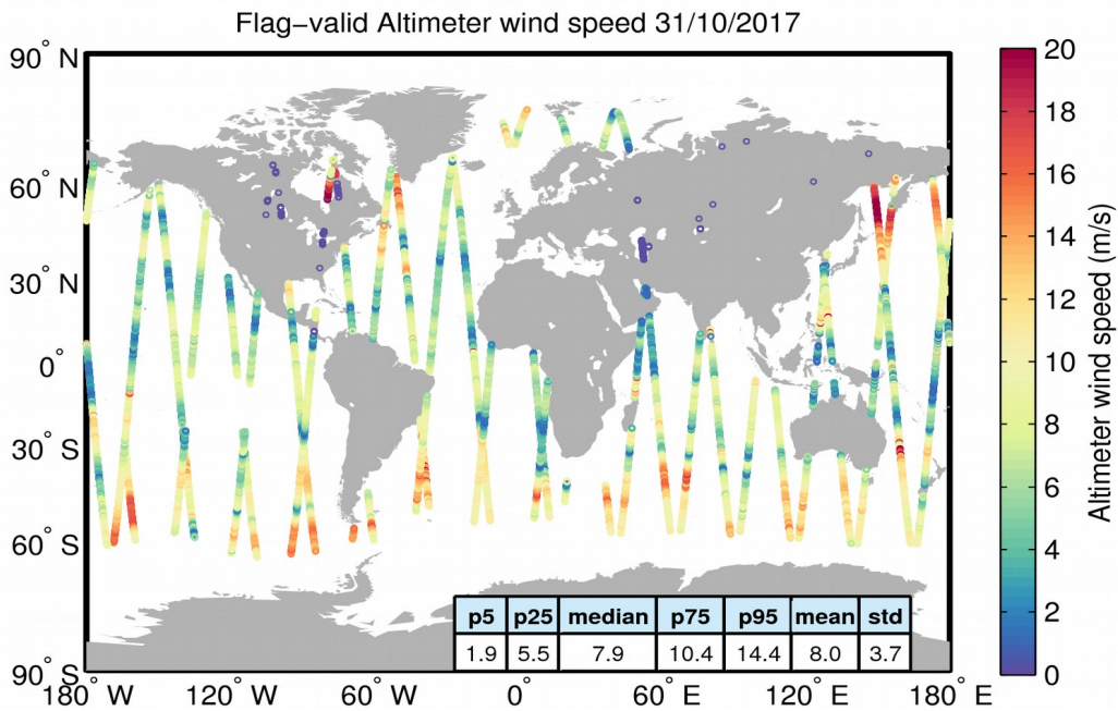
Figure 31. Geographical distribution of flag-valid wind data over oceans and lakes for 31/10/2017. The statistical values shown in the table refer to the wind in m/s and are calculated over all measurements shown in the figure.
