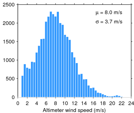
Figure 35. Histogram of science-valid wind over oceans and lakes for 31/10/2017. The mean ( \mu ) and standard deviation ( \sigma ) are also shown. Note that values larger than 24 m/s are excluded from the histogram for the sake of readability but not from the computation of \mu and \sigma .
