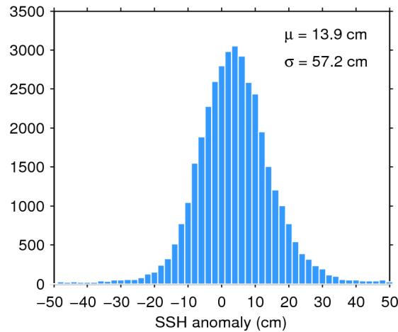
Figure 7. Histogram of flag-valid SSH anomaly over oceans and lakes for 31/10/2017. The mean ( \mu ) and standard deviation ( \sigma ) are also shown. Note that values outside [-50 50] cm are excluded from the histogram for the sake of readability but not from the computation of \mu and \sigma .
