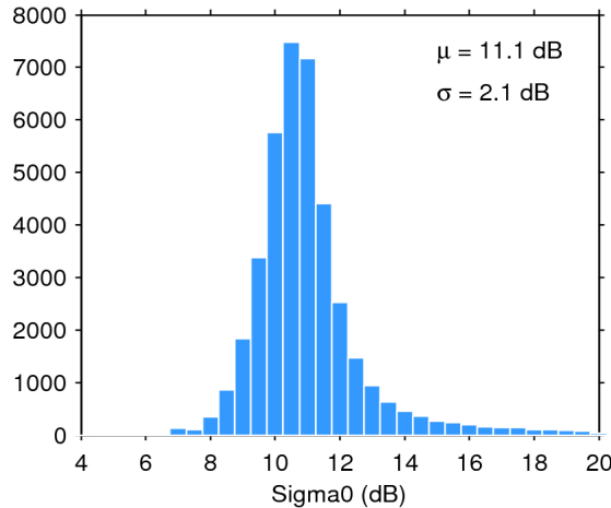
Figure 25. Histogram of flag-valid sigma0 over oceans and lakes for 31/10/2017. The mean ( \mu ) and standard deviation ( \sigma ) are also shown. Note that values outside [4 20] dB are excluded from the histogram for the sake of readability but not from the computation of \mu and \sigma .
