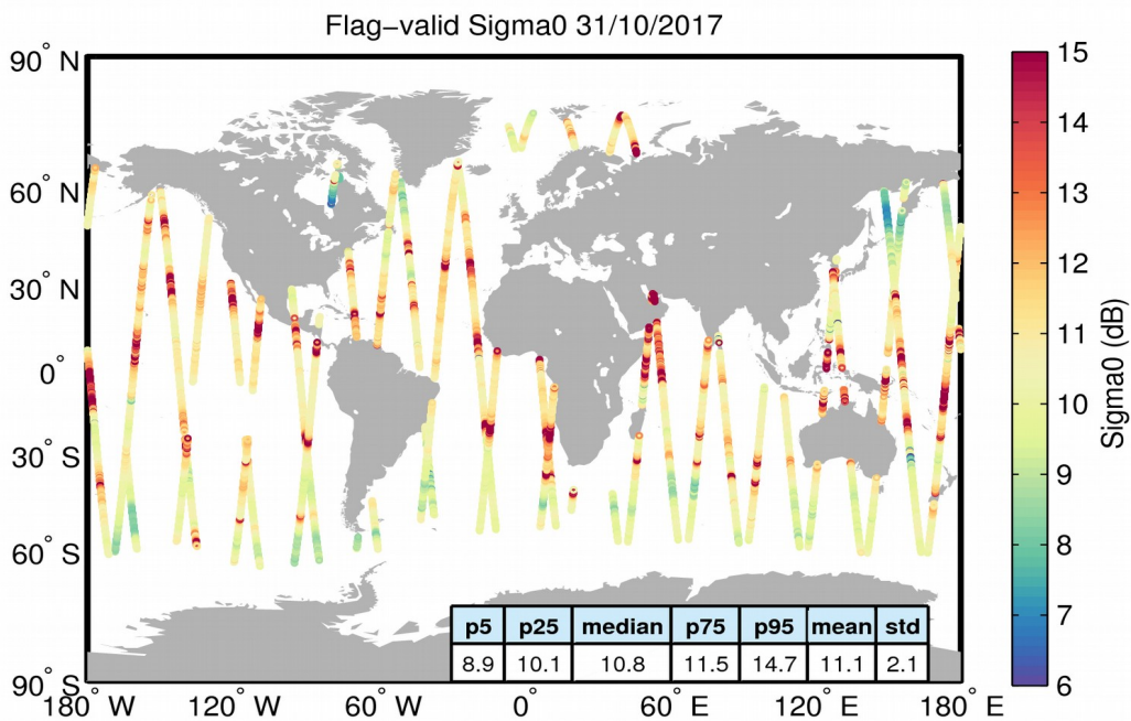
Figure 23. Geographical distribution of flag-valid sigma0 data over oceans and lakes for 31/10/2017. The statistical values shown in the table refer to the sigma0 in dB and are calculated over all measurements shown in the figure.
