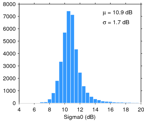
Figure 28. Histogram of science-valid sigma0 over oceans and lakes for 31/10/2017. The mean ( \mu ) and standard deviation ( \sigma ) are also shown. Note that values outside [4 20] dB are excluded from the histogram for the sake of readability but not from the computation of \mu and \sigma .
