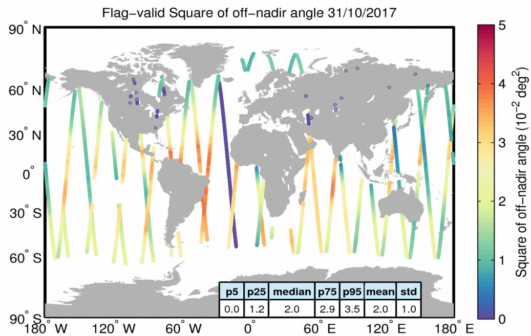
Figure 37. Geographical distribution of flag-valid mispointing data over oceans and lakes for 31/10/2017. The statistical values shown in the table refer to the mispointing in 10^{-2} deg 2 and are calculated over all measurements shown in the figure.
