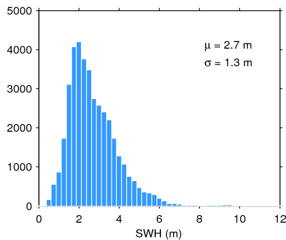
Figure 17. Histogram of flag-valid SWH over oceans and lakes for 31/10/2017. The mean ( \mu ) and standard deviation ( \sigma ) are also shown. Note that values larger than 12 m are excluded from the histogram for the sake of readability but not from the computation of \mu and \sigma .
