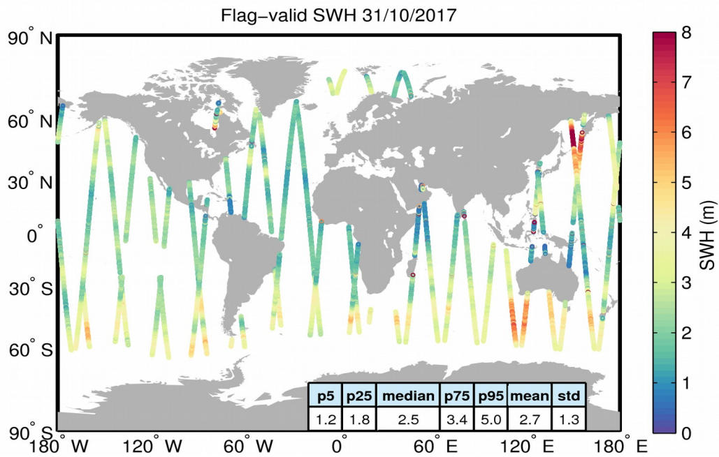
Figure 15. Geographical distribution of flag-valid SWH data over oceans and lakes for 31/10/2017. The statistical values shown in the table refer to the SWH in m and are calculated over all measurements shown in the figure.
