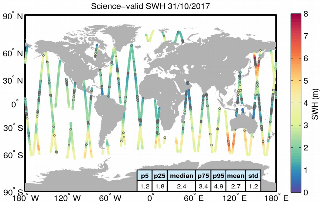
Figure 19. Geographical distribution of science-valid SWH data over oceans and lakes for 31/10/2017. The statistical values shown in the table refer to the SWH in m and are calculated over all measurements shown in the figure. Gray circles denote records that have been rejected based on the editing criteria described in Table 3.
