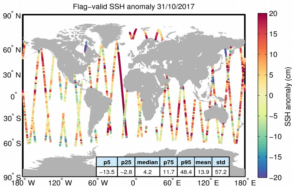
Figure 5. Geographical distribution of flag-valid 1-Hz SSH anomaly data over oceans and lakes for 31/10/2017. The statistical values shown in the table refer to the SSH anomaly in cm and are calculated over all measurements shown in the figure.
