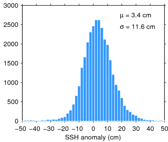
Figure 11. Histogram of science-valid SSH anomaly over oceans and lakes for 31/10/2017. The mean ( \mu ) and standard deviation ( \sigma ) are also shown. Note that values outside [-50 50] cm are excluded from the histogram for the sake of readability but not from the computation of \mu and \sigma .
