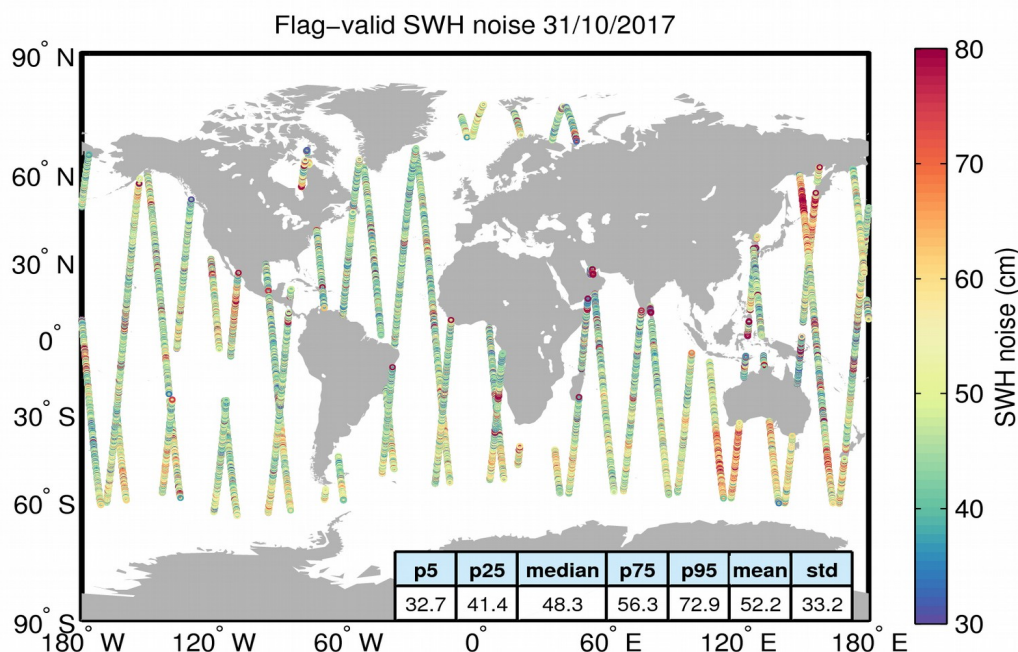
Figure 18. Geographical distribution of flag-valid 20-Hz SWH measurement noise over oceans and lakes for 31/10/2017. The statistical values shown in the table refer to the SWH noise and are calculated over all measurements shown in the figure.
