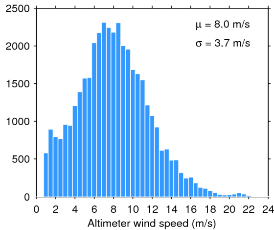
Figure 33. Histogram of flag-valid wind over oceans and lakes for 31/10/2017. The mean ( \mu ) and standard deviation ( \sigma ) are also shown. Note that values larger than 24 m/s are excluded from the histogram for the sake of readability but not from the computation of \mu and \sigma .
