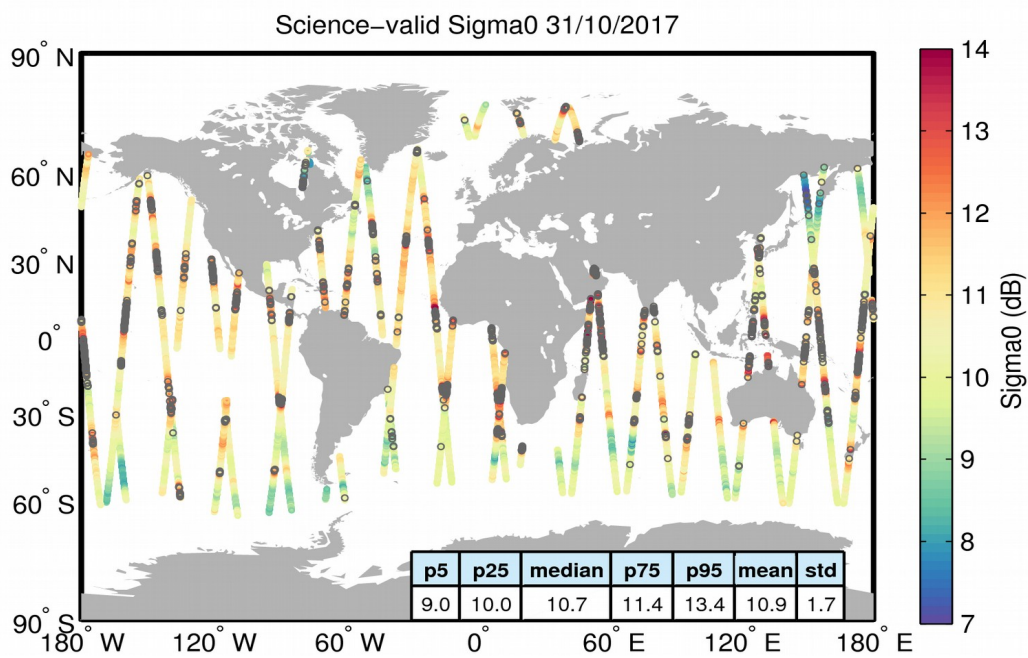
Figure 27. Geographical distribution of science-valid sigma0 data over oceans and lakes for 31/10/2017. The statistical values shown in the table refer to the sigma0 in dB and are calculated over all measurements shown in the figure. Gray circles denote records that have been rejected based on the editing criteria described in Table 4.
