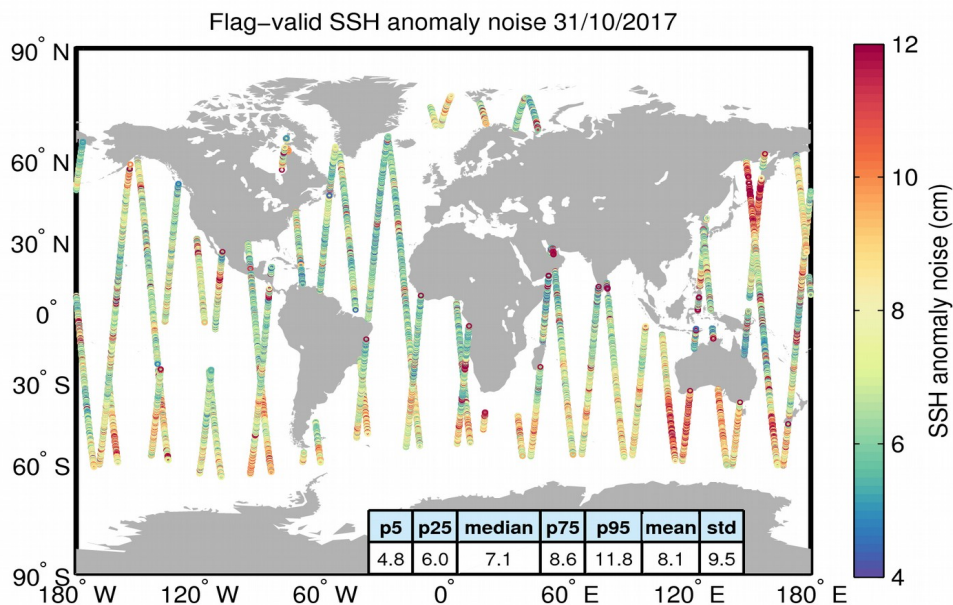
Figure 8. Geographical distribution of flag-valid 20-Hz SSH anomaly measurement noise over oceans and lakes for 31/10/2017. The statistical values shown in the table refer to the SSH anomaly noise and are calculated over all measurements shown in the figure.
