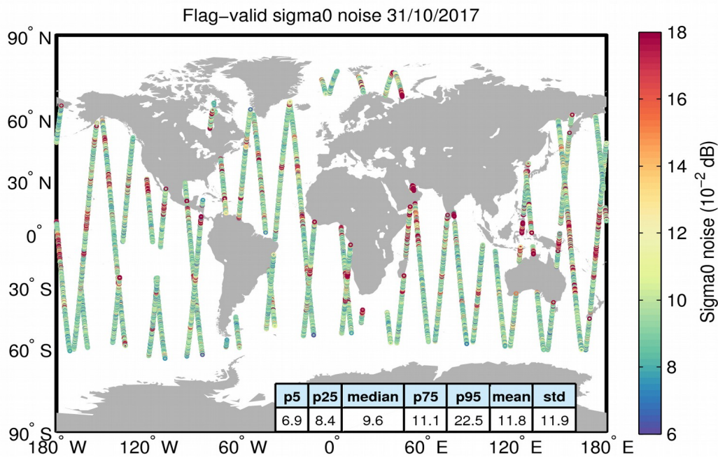
Figure 26. Geographical distribution of flag-valid 20-Hz sigma0 measurement noise over oceans and lakes for 31/10/2017. The statistical values shown in the table refer to the sigma0 noise and are calculated over all measurements shown in the figure.
