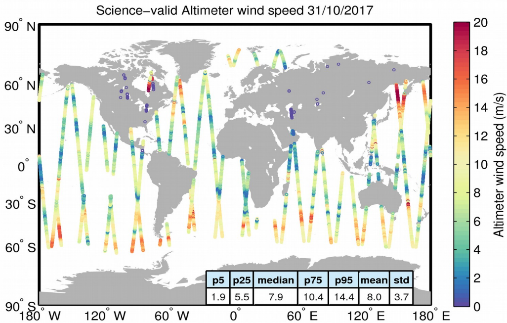
Figure 34. Geographical distribution of science-valid wind data over oceans and lakes for 31/10/2017. The statistical values shown in the table refer to the wind in m/s and are calculated over all measurements shown in the figure. Gray circles denote records that have been rejected based on the editing criteria described in Table 5.
