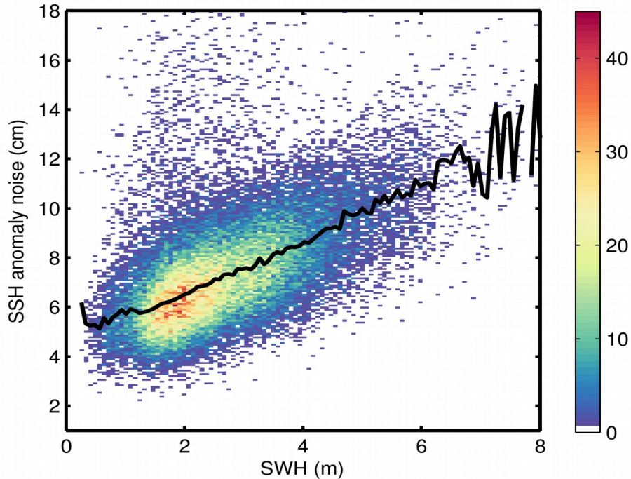
Figure 9. 2D histogram showing flag-valid SSH anomaly noise as a function of SWH for 31/10/2017. The black line denotes the median SSH anomaly noise as a function of SWH.
