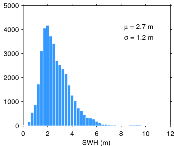
Figure 20. Histogram of science-valid SWH over oceans and lakes for 31/10/2017. The mean ( \mu ) and standard deviation ( \sigma ) are also shown. Note that values larger than 12 m are excluded from the histogram for the sake of readability but not from the computation of \mu and \sigma .
