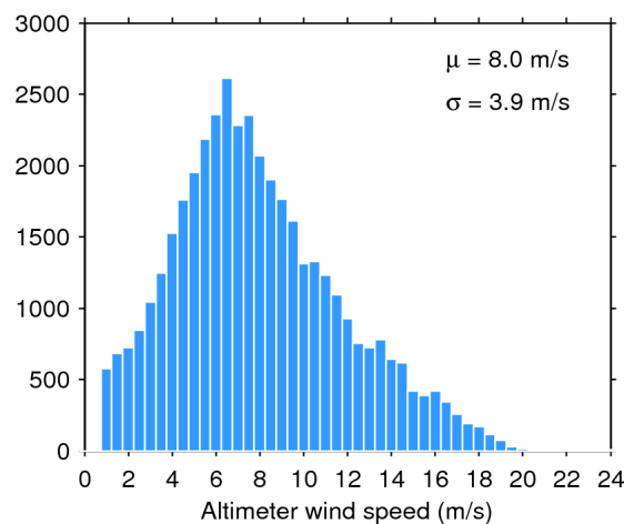
Figure 35. Histogram of science-valid wind over oceans and lakes for 30/10/2017. The mean ( \mu ) and standard deviation ( \sigma ) are also shown. Note that values larger than 24 m/s are excluded from the histogram for the sake of readability but not from the computation of \mu and \sigma .
