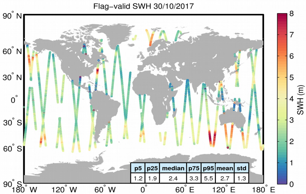
Figure 15. Geographical distribution of flag-valid SWH data over oceans and lakes for 30/10/2017. The statistical values shown in the table refer to the SWH in m and are calculated over all measurements shown in the figure.
