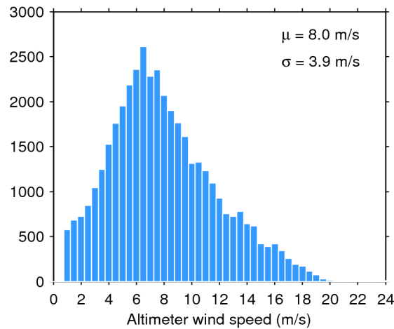
Figure 33. Histogram of flag-valid wind over oceans and lakes for 30/10/2017. The mean ( \mu ) and standard deviation ( \sigma ) are also shown. Note that values larger than 24 m/s are excluded from the histogram for the sake of readability but not from the computation of \mu and \sigma .
