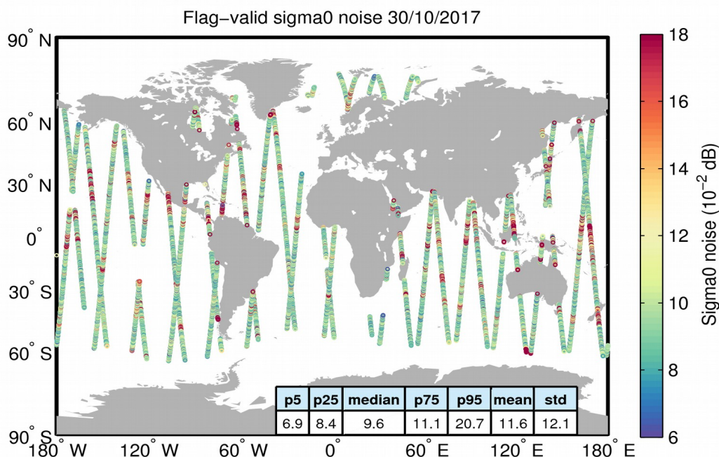
Figure 26. Geographical distribution of flag-valid 20-Hz sigma0 measurement noise over oceans and lakes for 30/10/2017. The statistical values shown in the table refer to the sigma0 noise and are calculated over all measurements shown in the figure.
