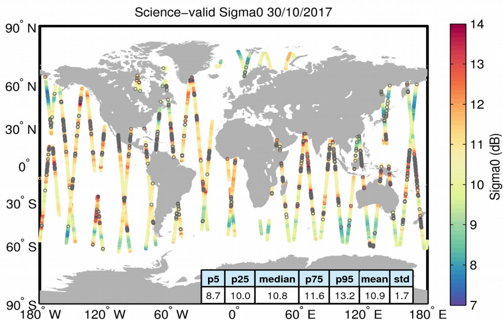
Figure 27. Geographical distribution of science-valid sigma0 data over oceans and lakes for 30/10/2017. The statistical values shown in the table refer to the sigma0 in dB and are calculated over all measurements shown in the figure. Gray circles denote records that have been rejected based on the editing criteria described in Table 4.
