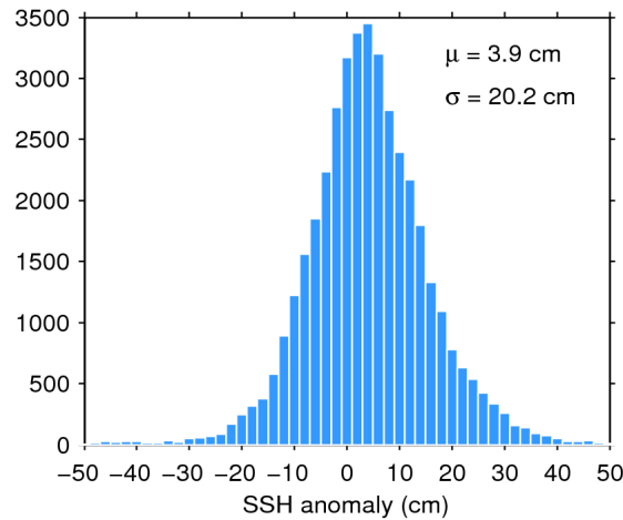
Figure 7. Histogram of flag-valid SSH anomaly over oceans and lakes for 30/10/2017. The mean ( \mu ) and standard deviation ( \sigma ) are also shown. Note that values outside [-50 50] cm are excluded from the histogram for the sake of readability but not from the computation of \mu and \sigma .
