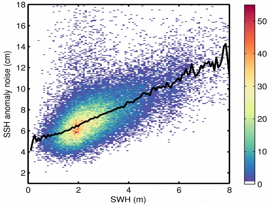
Figure 9. 2D histogram showing flag-valid SSH anomaly noise as a function of SWH for 30/10/2017. The black line denotes the median SSH anomaly noise as a function of SWH.
