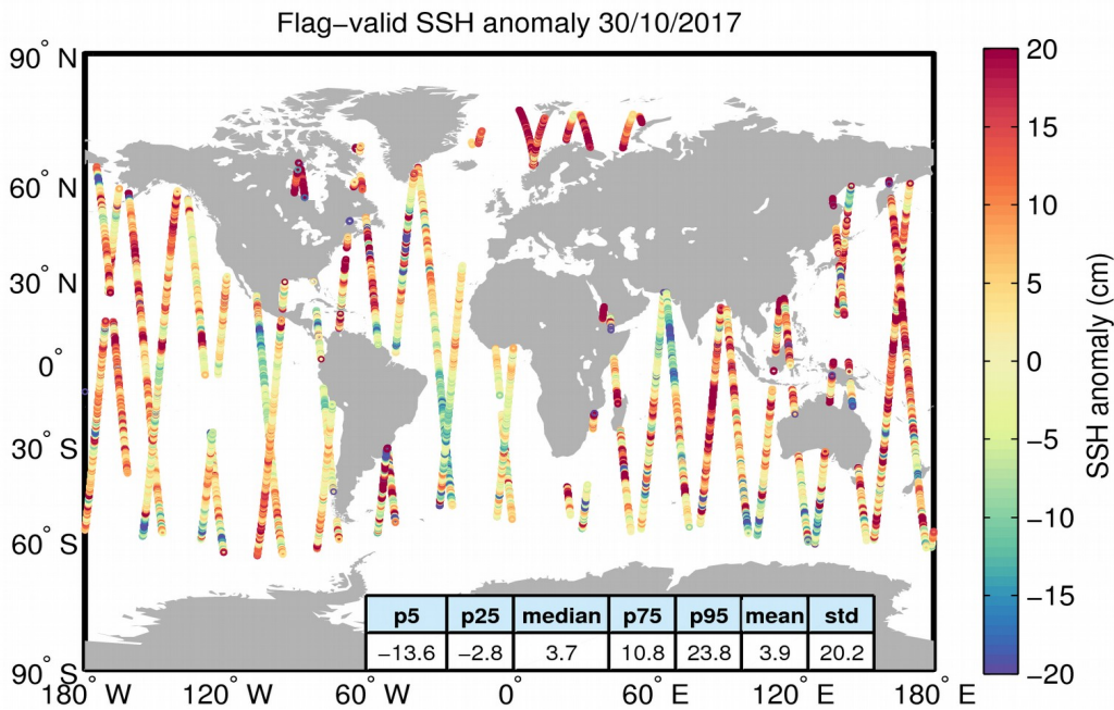
Figure 5. Geographical distribution of flag-valid 1-Hz SSH anomaly data over oceans and lakes for 30/10/2017. The statistical values shown in the table refer to the SSH anomaly in cm and are calculated over all measurements shown in the figure.
