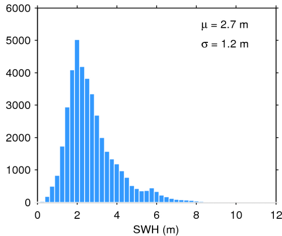
Figure 20. Histogram of science-valid SWH over oceans and lakes for 30/10/2017. The mean ( \mu ) and standard deviation ( \sigma ) are also shown. Note that values larger than 12 m are excluded from the histogram for the sake of readability but not from the computation of \mu and \sigma .
