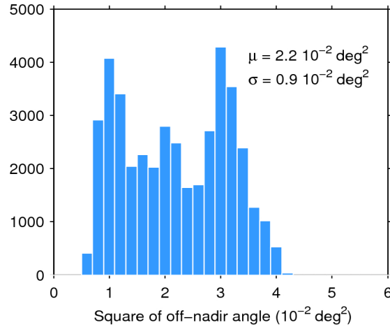
Figure 39. Histogram of flag-valid mispointing over oceans and lakes for 30/10/2017. The mean ( \mu ) and standard deviation ( \sigma ) are also shown. Note that values larger than 6 \cdot 10^{-2} \text{ deg}^2 are excluded from the histogram for the sake of readability but not from the computation of \mu and \sigma .
