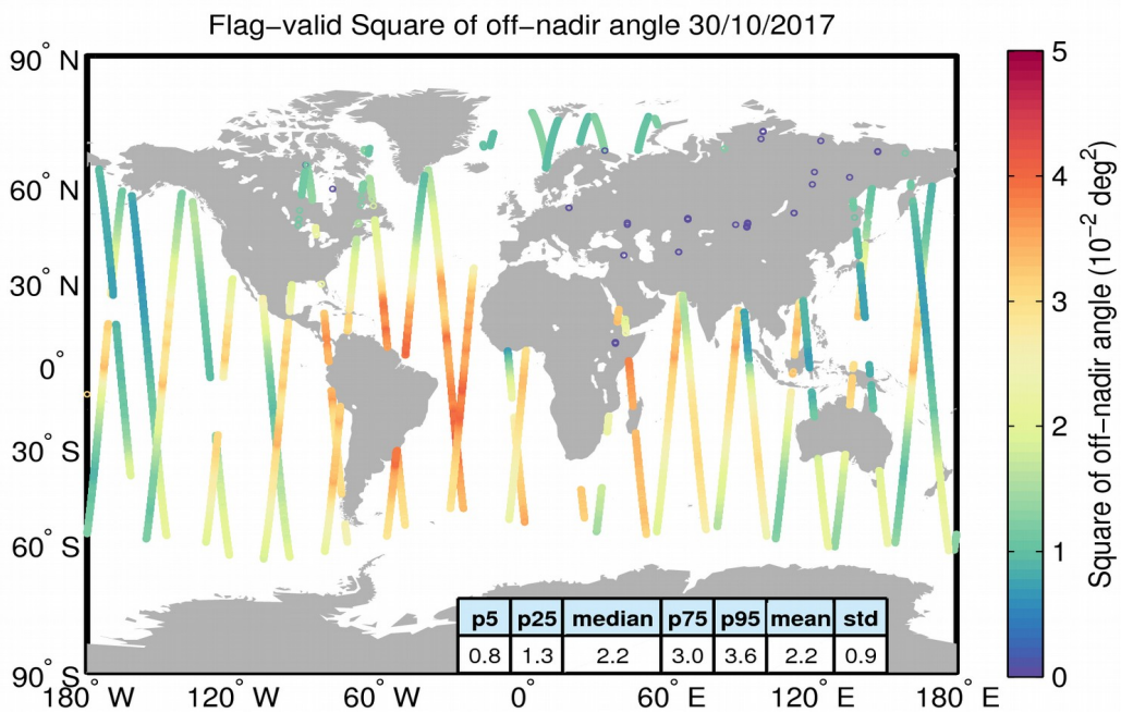
Figure 37. Geographical distribution of flag-valid mispointing data over oceans and lakes for 30/10/2017. The statistical values shown in the table refer to the mispointing in 10^{-2} deg 2 and are calculated over all measurements shown in the figure.
