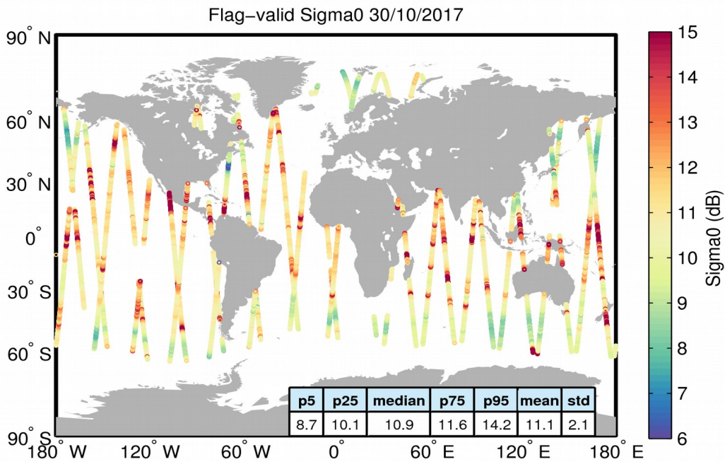
Figure 23. Geographical distribution of flag-valid sigma0 data over oceans and lakes for 30/10/2017. The statistical values shown in the table refer to the sigma0 in dB and are calculated over all measurements shown in the figure.
