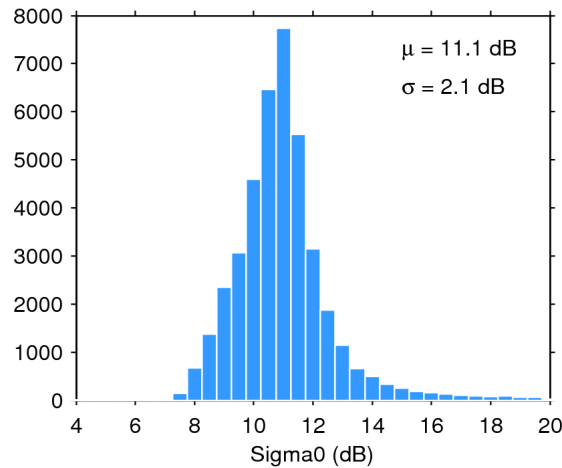
Figure 25. Histogram of flag-valid sigma0 over oceans and lakes for 30/10/2017. The mean ( \mu ) and standard deviation ( \sigma ) are also shown. Note that values outside [4 20] dB are excluded from the histogram for the sake of readability but not from the computation of \mu and \sigma .
