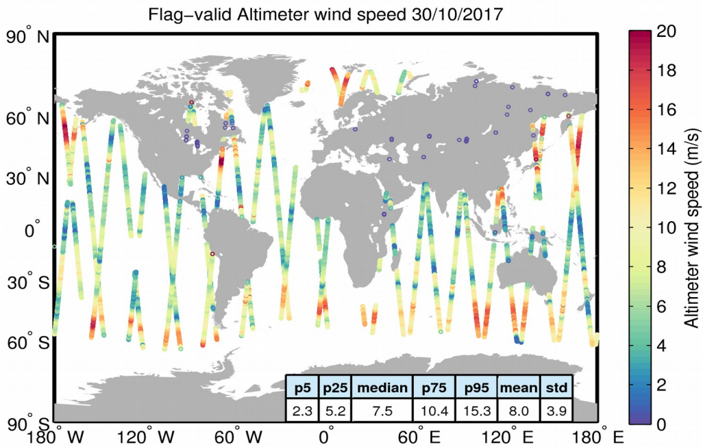
Figure 31. Geographical distribution of flag-valid wind data over oceans and lakes for 30/10/2017. The statistical values shown in the table refer to the wind in m/s and are calculated over all measurements shown in the figure.
