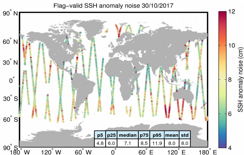
Figure 8. Geographical distribution of flag-valid 20-Hz SSH anomaly measurement noise over oceans and lakes for 30/10/2017. The statistical values shown in the table refer to the SSH anomaly noise and are calculated over all measurements shown in the figure.
