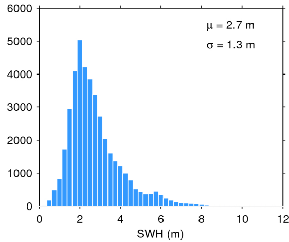
Figure 17. Histogram of flag-valid SWH over oceans and lakes for 30/10/2017. The mean ( \mu ) and standard deviation ( \sigma ) are also shown. Note that values larger than 12 m are excluded from the histogram for the sake of readability but not from the computation of \mu and \sigma .
