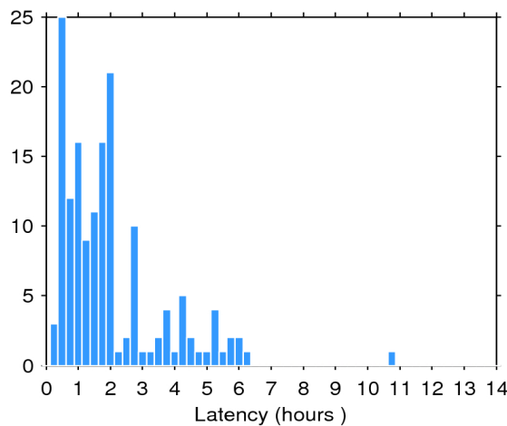
Figure 2. Histogram of the data latency for 30/10/2017. The y-axis denotes the number of files that are made available with a delay of x-hours with respect to the mean time of the records stored in the file.
