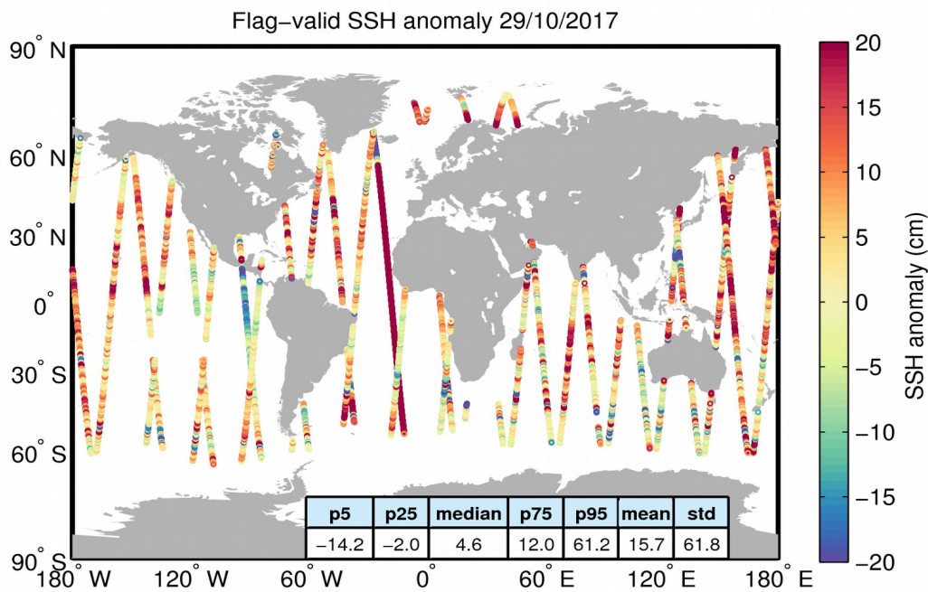
Figure 5. Geographical distribution of flag-valid 1-Hz SSH anomaly data over oceans and lakes for 29/10/2017. The statistical values shown in the table refer to the SSH anomaly in cm and are calculated over all measurements shown in the figure.
