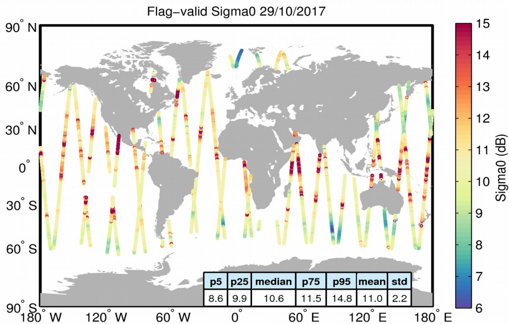
Figure 23. Geographical distribution of flag-valid sigma0 data over oceans and lakes for 29/10/2017. The statistical values shown in the table refer to the sigma0 in dB and are calculated over all measurements shown in the figure.
