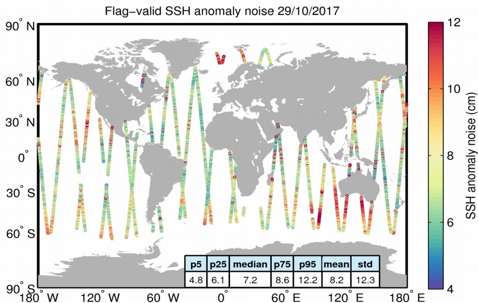
Figure 8. Geographical distribution of flag-valid 20-Hz SSH anomaly measurement noise over oceans and lakes for 29/10/2017. The statistical values shown in the table refer to the SSH anomaly noise and are calculated over all measurements shown in the figure.
