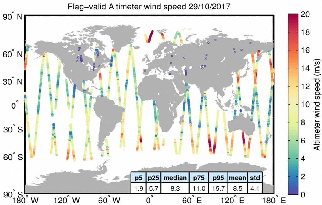
Figure 31. Geographical distribution of flag-valid wind data over oceans and lakes for 29/10/2017. The statistical values shown in the table refer to the wind in m/s and are calculated over all measurements shown in the figure.
