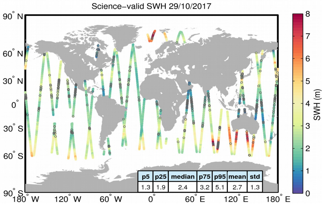
Figure 19. Geographical distribution of science-valid SWH data over oceans and lakes for 29/10/2017. The statistical values shown in the table refer to the SWH in m and are calculated over all measurements shown in the figure. Gray circles denote records that have been rejected based on the editing criteria described in Table 3.
