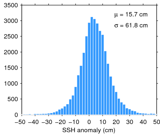
Figure 7. Histogram of flag-valid SSH anomaly over oceans and lakes for 29/10/2017. The mean ( \mu ) and standard deviation ( \sigma ) are also shown. Note that values outside [-50 50] cm are excluded from the histogram for the sake of readability but not from the computation of \mu and \sigma .
