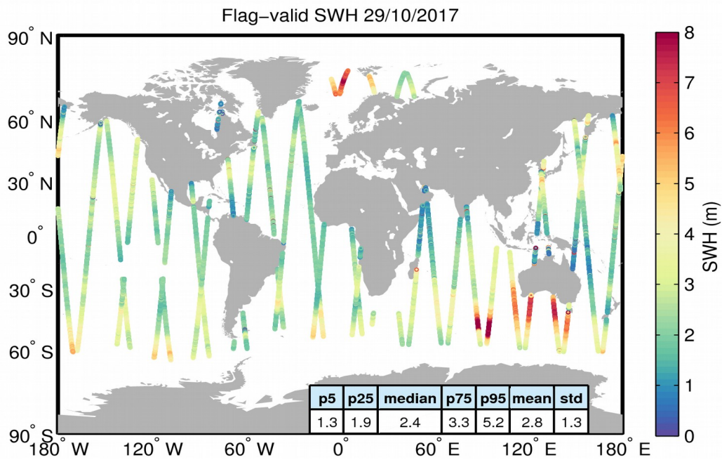
Figure 15. Geographical distribution of flag-valid SWH data over oceans and lakes for 29/10/2017. The statistical values shown in the table refer to the SWH in m and are calculated over all measurements shown in the figure.
