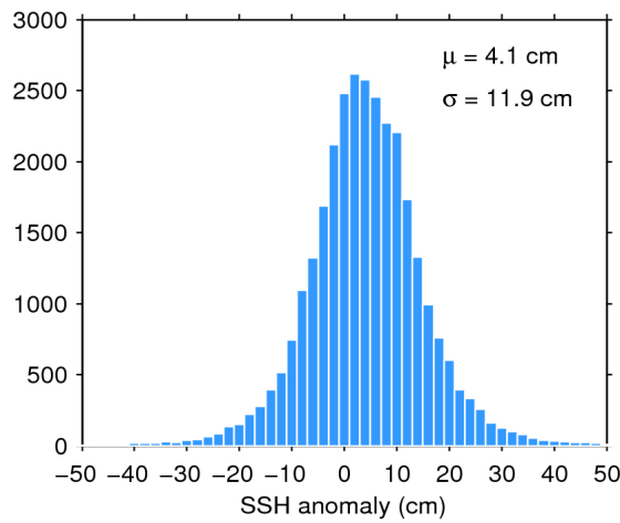
Figure 11. Histogram of science-valid SSH anomaly over oceans and lakes for 29/10/2017. The mean ( \mu ) and standard deviation ( \sigma ) are also shown. Note that values outside [-50 50] cm are excluded from the histogram for the sake of readability but not from the computation of \mu and \sigma .
