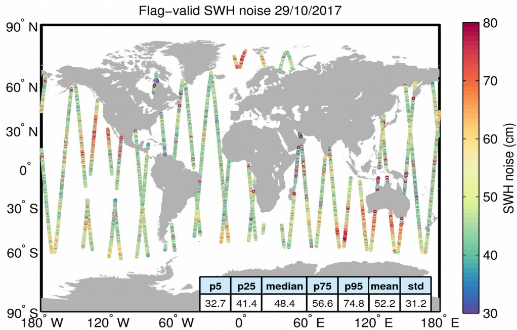
Figure 18. Geographical distribution of flag-valid 20-Hz SWH measurement noise over oceans and lakes for 29/10/2017. The statistical values shown in the table refer to the SWH noise and are calculated over all measurements shown in the figure.
