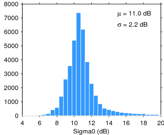
Figure 25. Histogram of flag-valid sigma0 over oceans and lakes for 29/10/2017. The mean ( \mu ) and standard deviation ( \sigma ) are also shown. Note that values outside [4 20] dB are excluded from the histogram for the sake of readability but not from the computation of \mu and \sigma .
