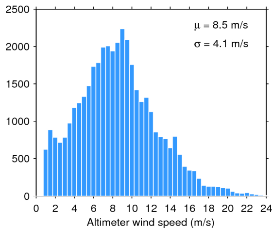
Figure 35. Histogram of science-valid wind over oceans and lakes for 29/10/2017. The mean ( \mu ) and standard deviation ( \sigma ) are also shown. Note that values larger than 24 m/s are excluded from the histogram for the sake of readability but not from the computation of \mu and \sigma .
