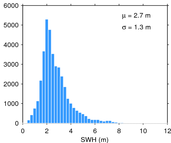
Figure 20. Histogram of science-valid SWH over oceans and lakes for 29/10/2017. The mean ( \mu ) and standard deviation ( \sigma ) are also shown. Note that values larger than 12 m are excluded from the histogram for the sake of readability but not from the computation of \mu and \sigma .
