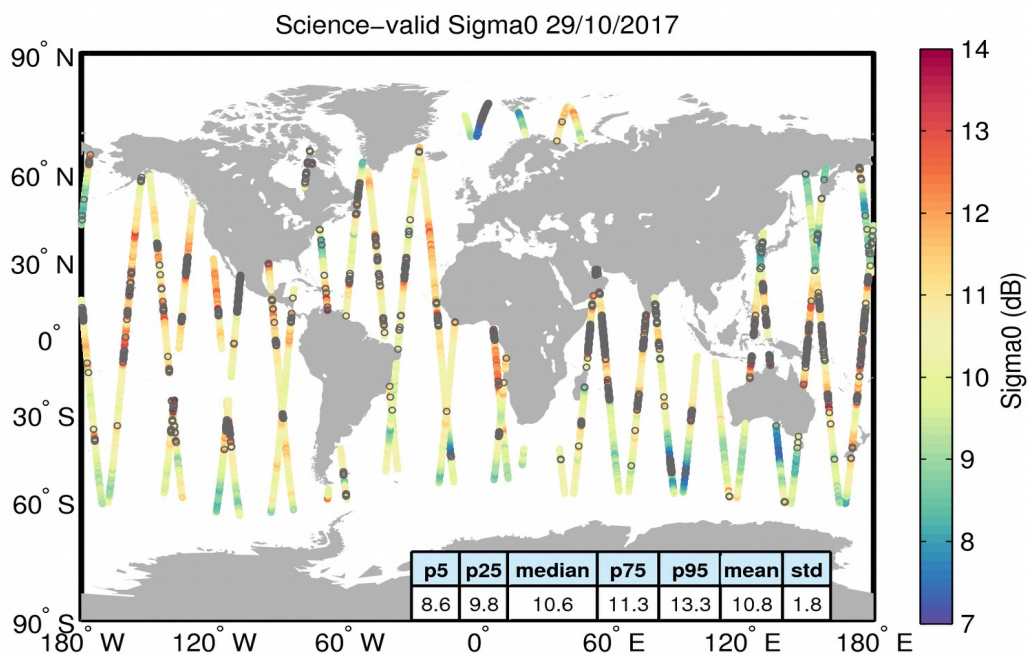
Figure 27. Geographical distribution of science-valid sigma0 data over oceans and lakes for 29/10/2017. The statistical values shown in the table refer to the sigma0 in dB and are calculated over all measurements shown in the figure. Gray circles denote records that have been rejected based on the editing criteria described in Table 4.
