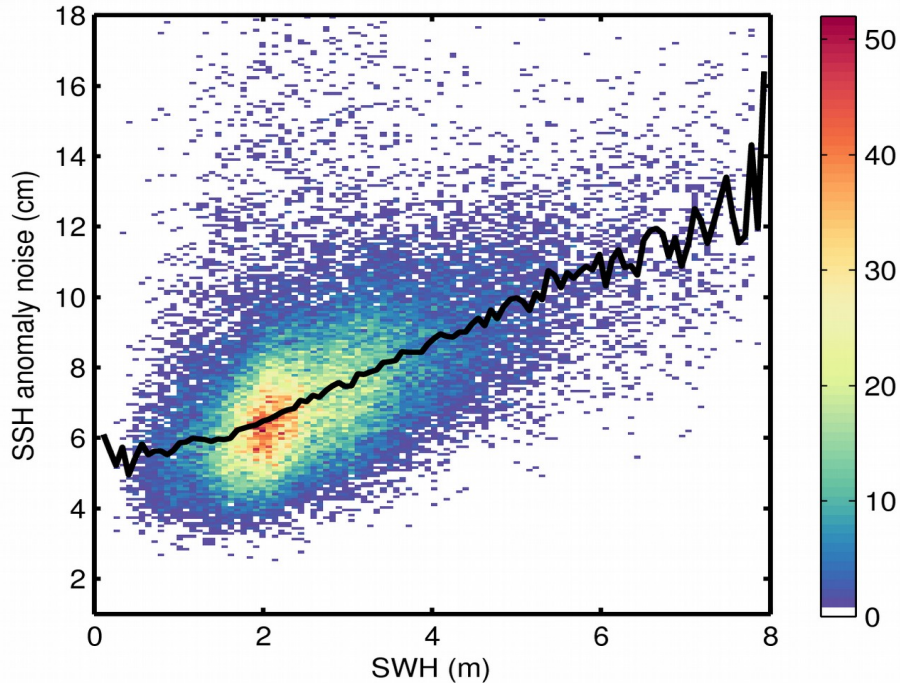
Figure 9. 2D histogram showing flag-valid SSH anomaly noise as a function of SWH for 29/10/2017. The black line denotes the median SSH anomaly noise as a function of SWH.
