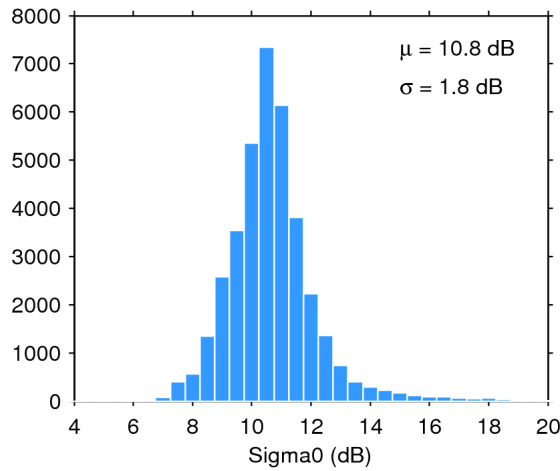
Figure 28. Histogram of science-valid sigma0 over oceans and lakes for 29/10/2017. The mean ( \mu ) and standard deviation ( \sigma ) are also shown. Note that values outside [4 20] dB are excluded from the histogram for the sake of readability but not from the computation of \mu and \sigma .
