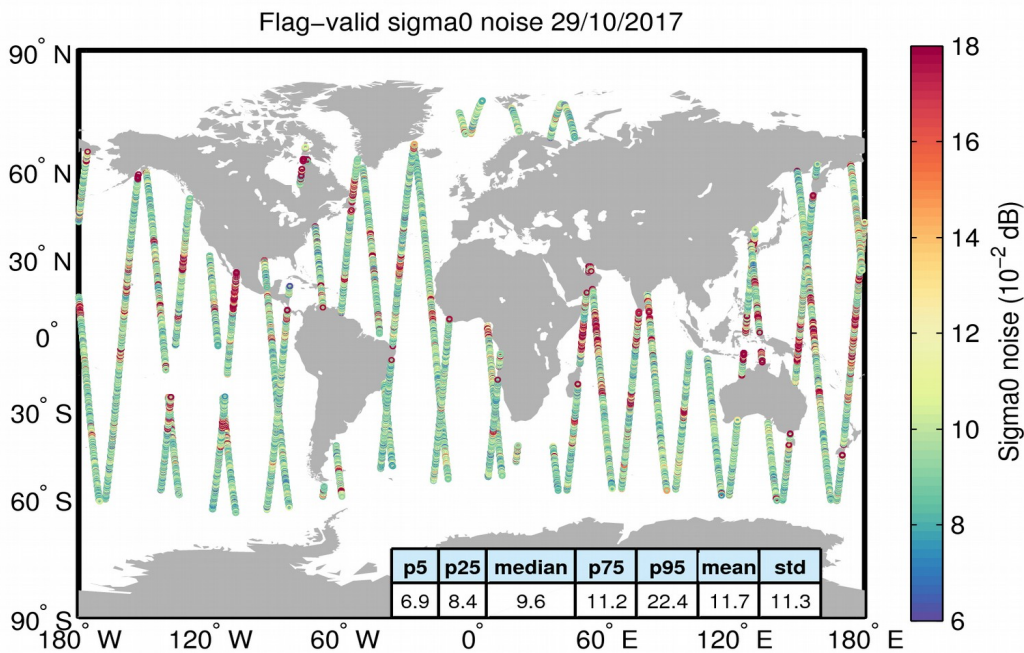
Figure 26. Geographical distribution of flag-valid 20-Hz sigma0 measurement noise over oceans and lakes for 29/10/2017. The statistical values shown in the table refer to the sigma0 noise and are calculated over all measurements shown in the figure.
