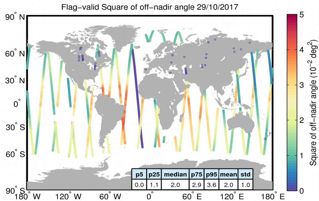
Figure 37. Geographical distribution of flag-valid mispointing data over oceans and lakes for 29/10/2017. The statistical values shown in the table refer to the mispointing in 10^{-2} deg 2 and are calculated over all measurements shown in the figure.
