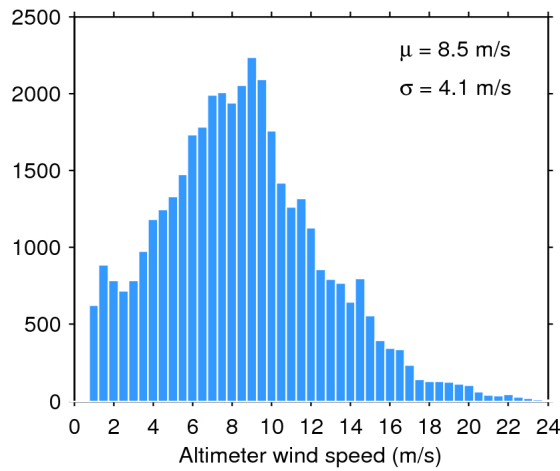
Figure 33. Histogram of flag-valid wind over oceans and lakes for 29/10/2017. The mean ( \mu ) and standard deviation ( \sigma ) are also shown. Note that values larger than 24 m/s are excluded from the histogram for the sake of readability but not from the computation of \mu and \sigma .
