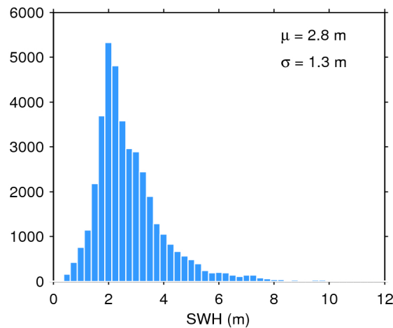
Figure 17. Histogram of flag-valid SWH over oceans and lakes for 29/10/2017. The mean ( \mu ) and standard deviation ( \sigma ) are also shown. Note that values larger than 12 m are excluded from the histogram for the sake of readability but not from the computation of \mu and \sigma .
