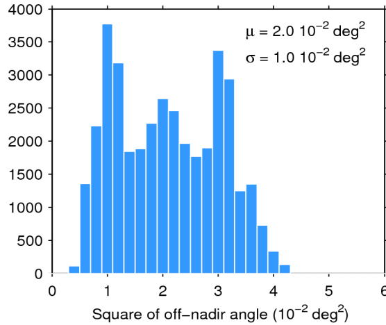
Figure 39. Histogram of flag-valid mispointing over oceans and lakes for 29/10/2017. The mean ( \mu ) and standard deviation ( \sigma ) are also shown. Note that values larger than 6 \cdot 10^{-2} \text{ deg}^2 are excluded from the histogram for the sake of readability but not from the computation of \mu and \sigma .
