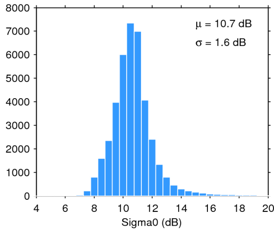
Figure 28. Histogram of science-valid sigma0 over oceans and lakes for 28/10/2017. The mean ( \mu ) and standard deviation ( \sigma ) are also shown. Note that values outside [4 20] dB are excluded from the histogram for the sake of readability but not from the computation of \mu and \sigma .
