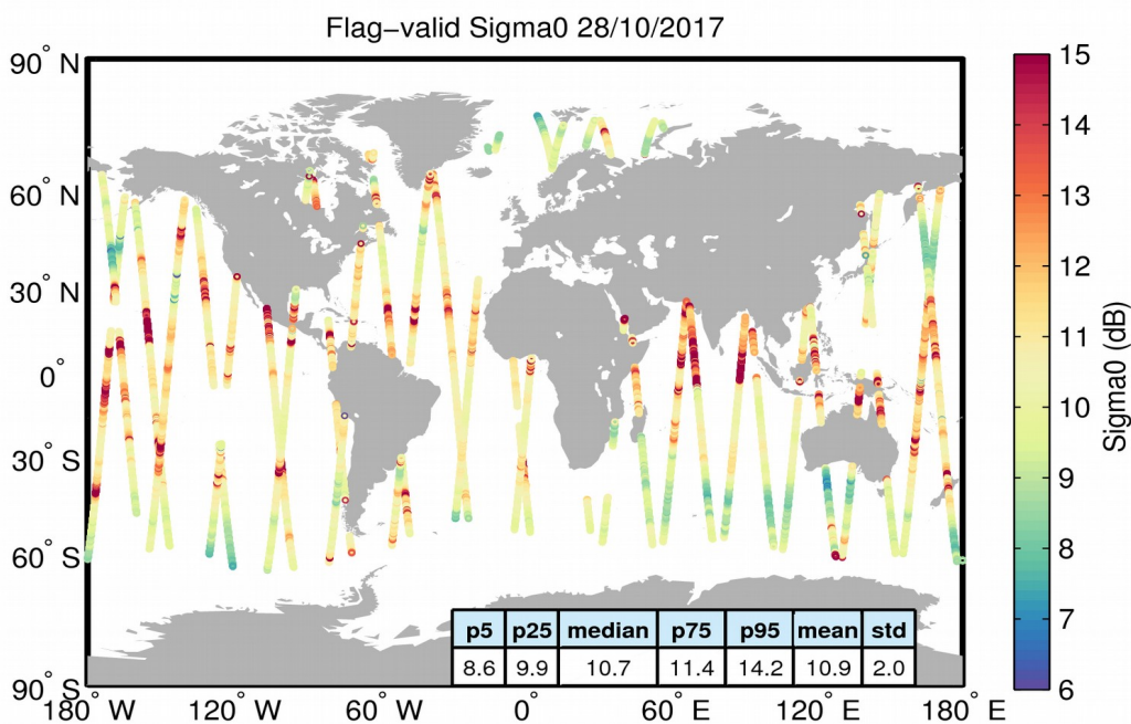
Figure 23. Geographical distribution of flag-valid sigma0 data over oceans and lakes for 28/10/2017. The statistical values shown in the table refer to the sigma0 in dB and are calculated over all measurements shown in the figure.
