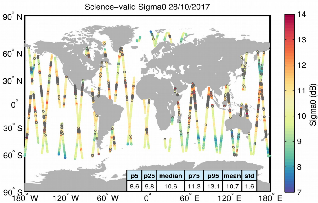
Figure 27. Geographical distribution of science-valid sigma0 data over oceans and lakes for 28/10/2017. The statistical values shown in the table refer to the sigma0 in dB and are calculated over all measurements shown in the figure. Gray circles denote records that have been rejected based on the editing criteria described in Table 4.
