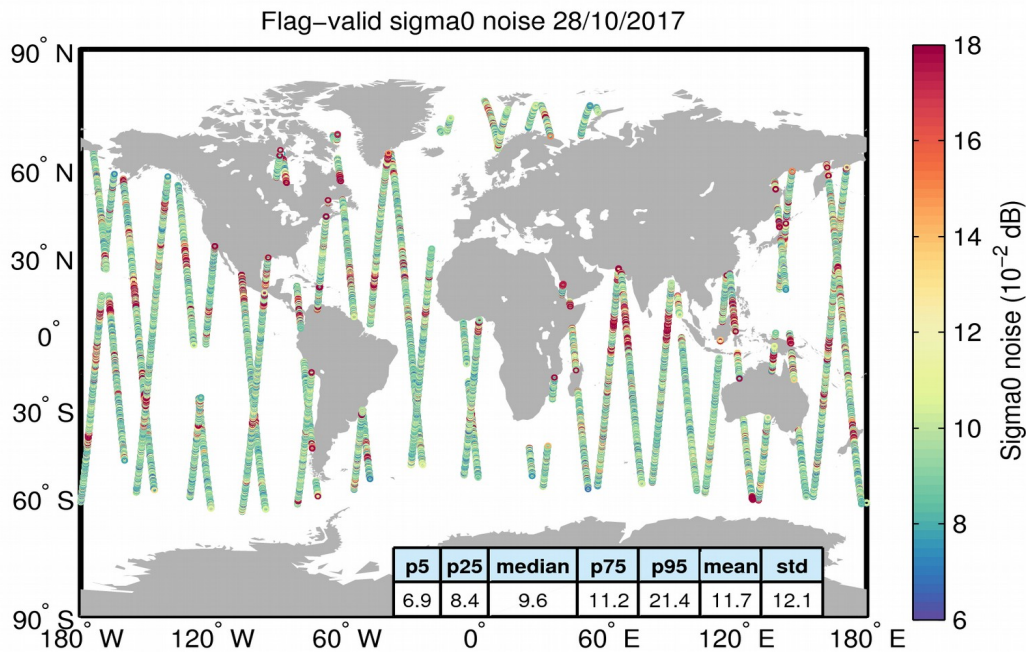
Figure 26. Geographical distribution of flag-valid 20-Hz sigma0 measurement noise over oceans and lakes for 28/10/2017. The statistical values shown in the table refer to the sigma0 noise and are calculated over all measurements shown in the figure.
