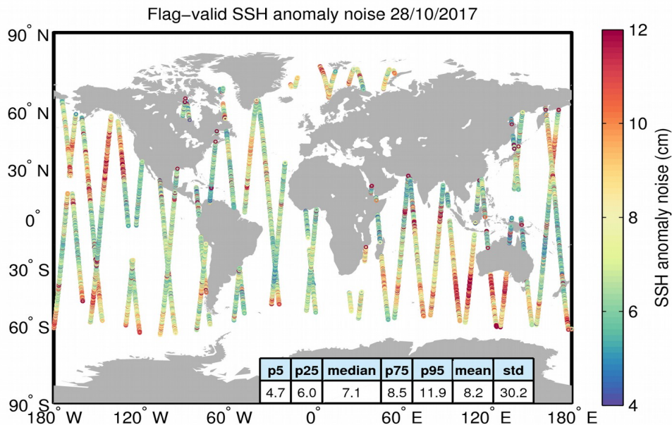
Figure 8. Geographical distribution of flag-valid 20-Hz SSH anomaly measurement noise over oceans and lakes for 28/10/2017. The statistical values shown in the table refer to the SSH anomaly noise and are calculated over all measurements shown in the figure.
