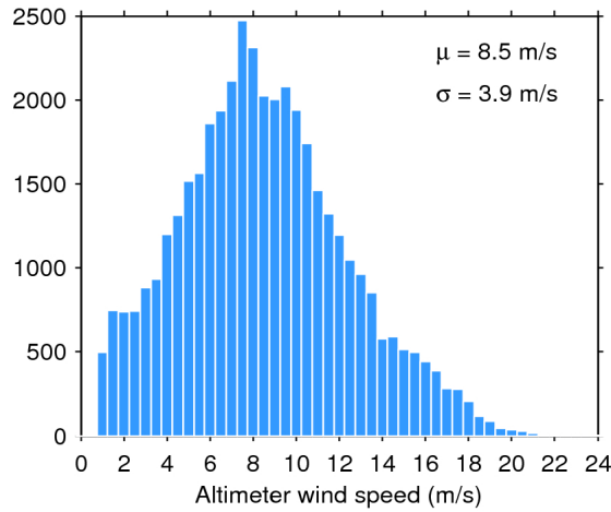
Figure 33. Histogram of flag-valid wind over oceans and lakes for 28/10/2017. The mean ( \mu ) and standard deviation ( \sigma ) are also shown. Note that values larger than 24 m/s are excluded from the histogram for the sake of readability but not from the computation of \mu and \sigma .
