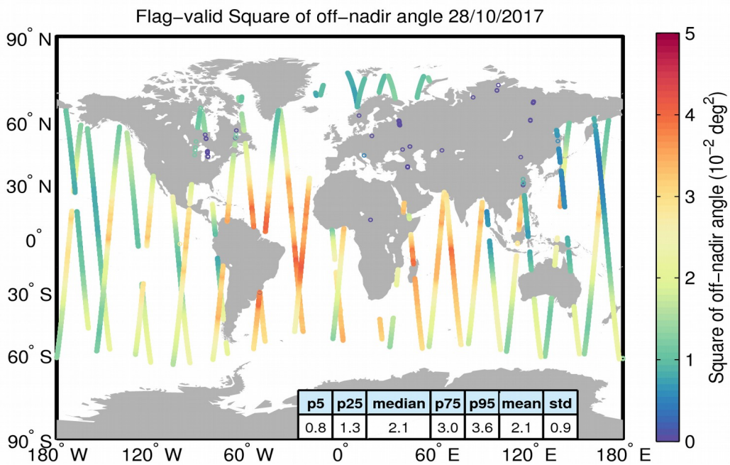
Figure 37. Geographical distribution of flag-valid mispointing data over oceans and lakes for 28/10/2017. The statistical values shown in the table refer to the mispointing in 10^{-2} deg 2 and are calculated over all measurements shown in the figure.
