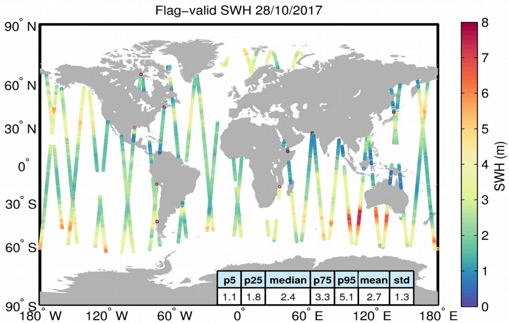
Figure 15. Geographical distribution of flag-valid SWH data over oceans and lakes for 28/10/2017. The statistical values shown in the table refer to the SWH in m and are calculated over all measurements shown in the figure.
