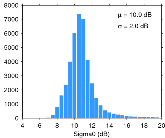
Figure 25. Histogram of flag-valid sigma0 over oceans and lakes for 28/10/2017. The mean ( \mu ) and standard deviation ( \sigma ) are also shown. Note that values outside [4 20] dB are excluded from the histogram for the sake of readability but not from the computation of \mu and \sigma .
