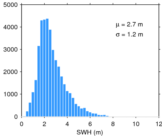
Figure 20. Histogram of science-valid SWH over oceans and lakes for 28/10/2017. The mean ( \mu ) and standard deviation ( \sigma ) are also shown. Note that values larger than 12 m are excluded from the histogram for the sake of readability but not from the computation of \mu and \sigma .
