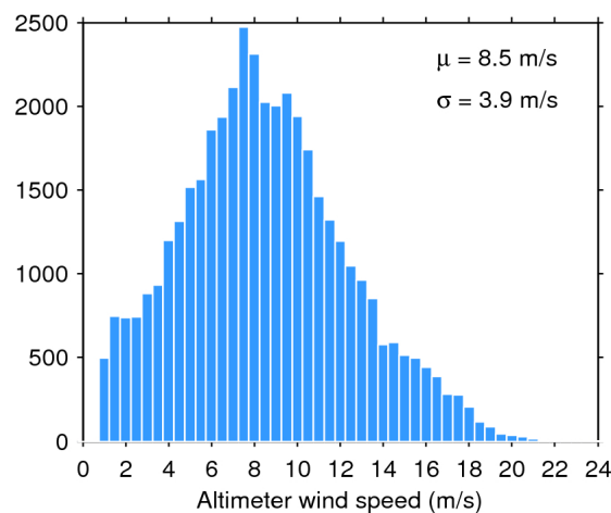
Figure 35. Histogram of science-valid wind over oceans and lakes for 28/10/2017. The mean ( \mu ) and standard deviation ( \sigma ) are also shown. Note that values larger than 24 m/s are excluded from the histogram for the sake of readability but not from the computation of \mu and \sigma .
