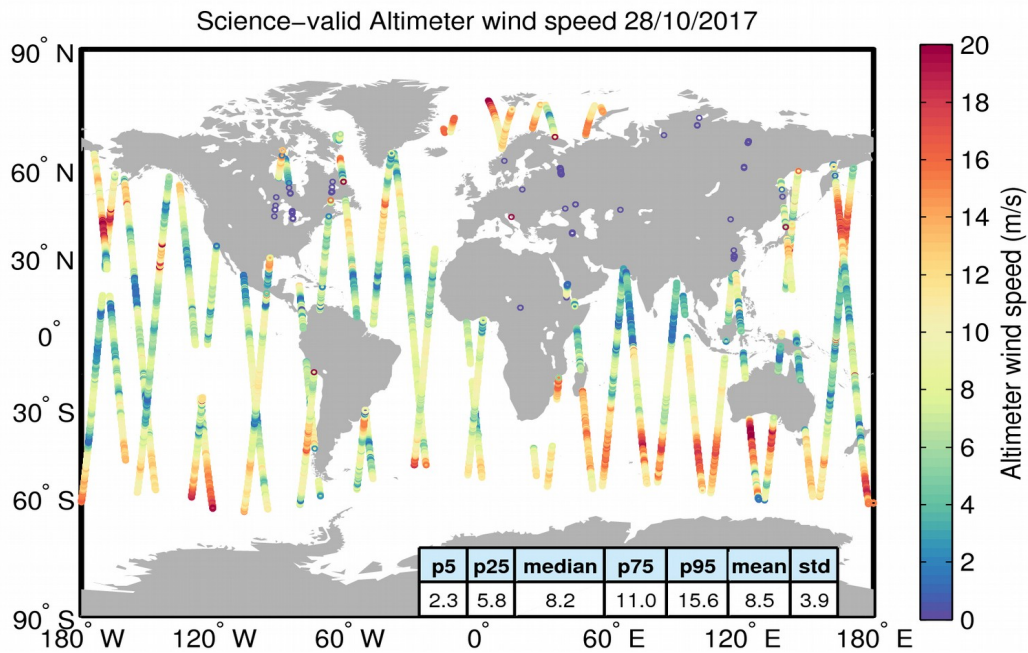
Figure 34. Geographical distribution of science-valid wind data over oceans and lakes for 28/10/2017. The statistical values shown in the table refer to the wind in m/s and are calculated over all measurements shown in the figure. Gray circles denote records that have been rejected based on the editing criteria described in Table 5.
