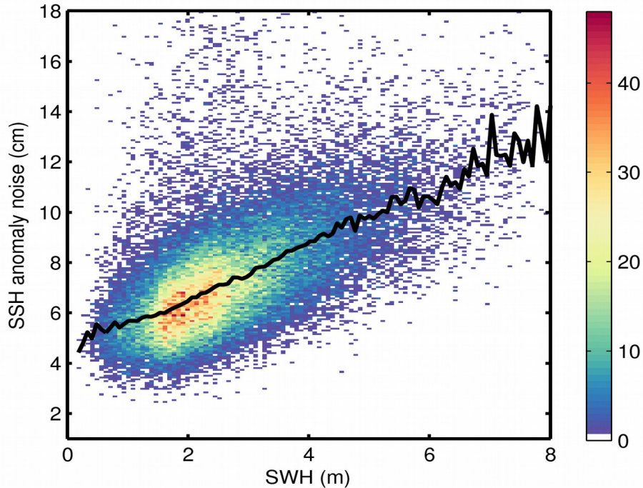
Figure 9. 2D histogram showing flag-valid SSH anomaly noise as a function of SWH for 28/10/2017. The black line denotes the median SSH anomaly noise as a function of SWH.
