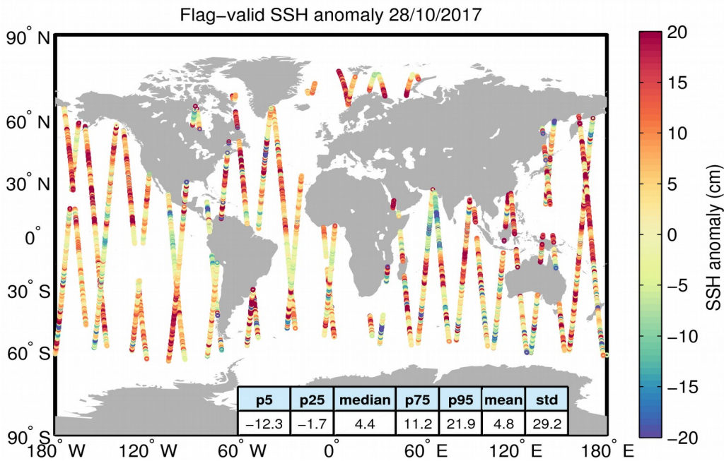
Figure 5. Geographical distribution of flag-valid 1-Hz SSH anomaly data over oceans and lakes for 28/10/2017. The statistical values shown in the table refer to the SSH anomaly in cm and are calculated over all measurements shown in the figure.
