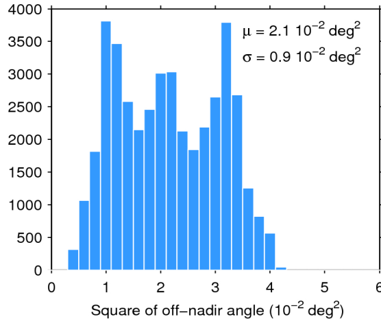
Figure 39. Histogram of flag-valid mispointing over oceans and lakes for 28/10/2017. The mean ( \mu ) and standard deviation ( \sigma ) are also shown. Note that values larger than 6 \cdot 10^{-2} \text{ deg}^2 are excluded from the histogram for the sake of readability but not from the computation of \mu and \sigma .
