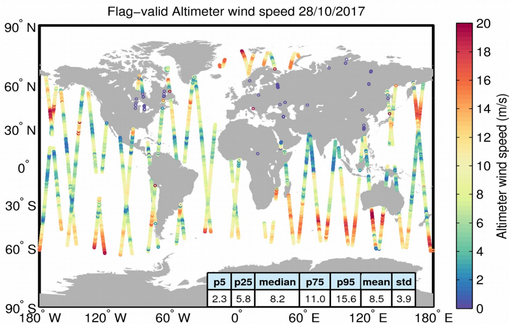
Figure 31. Geographical distribution of flag-valid wind data over oceans and lakes for 28/10/2017. The statistical values shown in the table refer to the wind in m/s and are calculated over all measurements shown in the figure.
