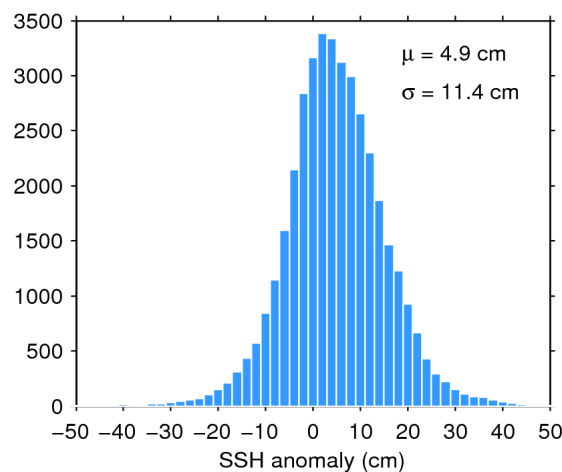
Figure 11. Histogram of science-valid SSH anomaly over oceans and lakes for 28/10/2017. The mean ( \mu ) and standard deviation ( \sigma ) are also shown. Note that values outside [-50 50] cm are excluded from the histogram for the sake of readability but not from the computation of \mu and \sigma .
