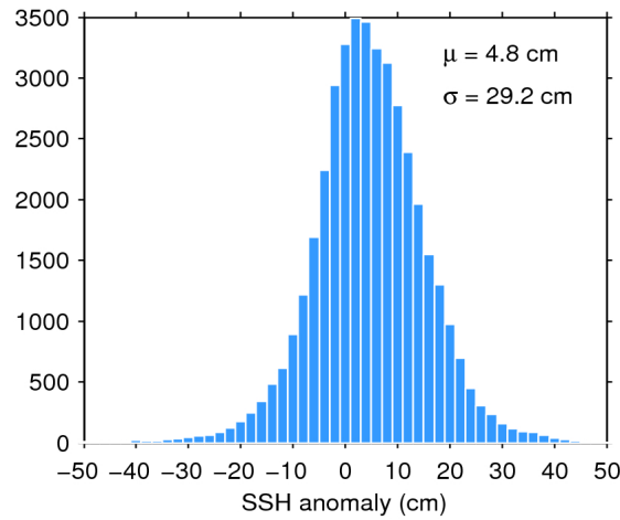
Figure 7. Histogram of flag-valid SSH anomaly over oceans and lakes for 28/10/2017. The mean ( \mu ) and standard deviation ( \sigma ) are also shown. Note that values outside [-50 50] cm are excluded from the histogram for the sake of readability but not from the computation of \mu and \sigma .
