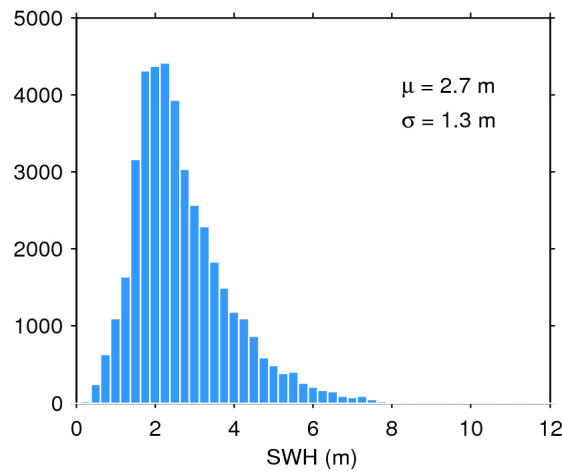
Figure 17. Histogram of flag-valid SWH over oceans and lakes for 28/10/2017. The mean ( \mu ) and standard deviation ( \sigma ) are also shown. Note that values larger than 12 m are excluded from the histogram for the sake of readability but not from the computation of \mu and \sigma .
