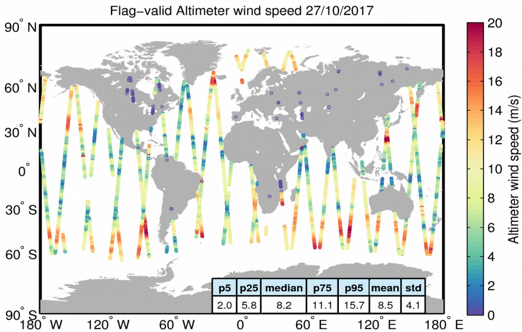
Figure 31. Geographical distribution of flag-valid wind data over oceans and lakes for 27/10/2017. The statistical values shown in the table refer to the wind in m/s and are calculated over all measurements shown in the figure.
