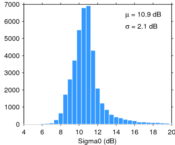
Figure 25. Histogram of flag-valid sigma0 over oceans and lakes for 27/10/2017. The mean ( \mu ) and standard deviation ( \sigma ) are also shown. Note that values outside [4 20] dB are excluded from the histogram for the sake of readability but not from the computation of \mu and \sigma .
