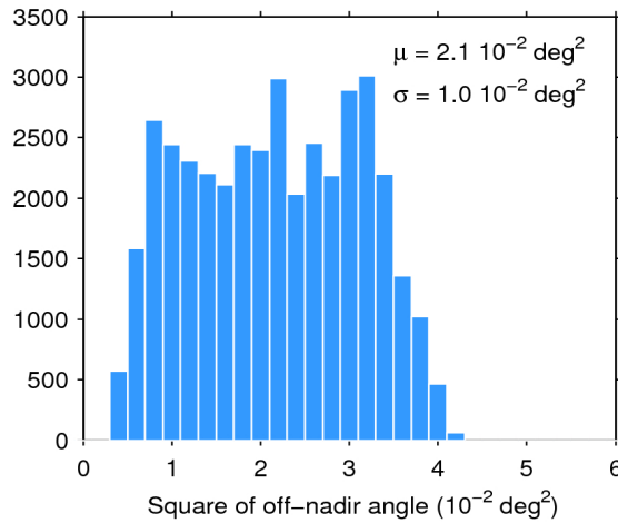
Figure 39. Histogram of flag-valid mispointing over oceans and lakes for 27/10/2017. The mean ( \mu ) and standard deviation ( \sigma ) are also shown. Note that values larger than 6 \cdot 10^{-2} \text{ deg}^2 are excluded from the histogram for the sake of readability but not from the computation of \mu and \sigma .
