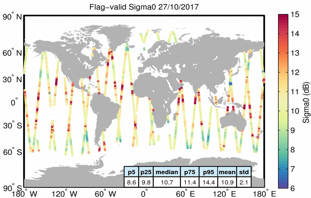
Figure 23. Geographical distribution of flag-valid sigma0 data over oceans and lakes for 27/10/2017. The statistical values shown in the table refer to the sigma0 in dB and are calculated over all measurements shown in the figure.
