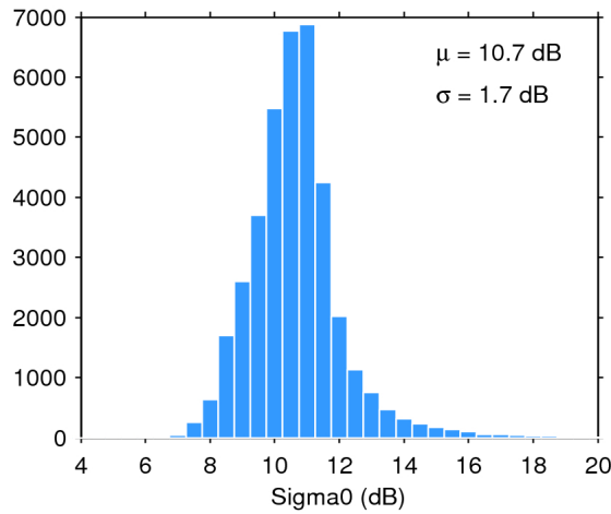
Figure 28. Histogram of science-valid sigma0 over oceans and lakes for 27/10/2017. The mean ( \mu ) and standard deviation ( \sigma ) are also shown. Note that values outside [4 20] dB are excluded from the histogram for the sake of readability but not from the computation of \mu and \sigma .
