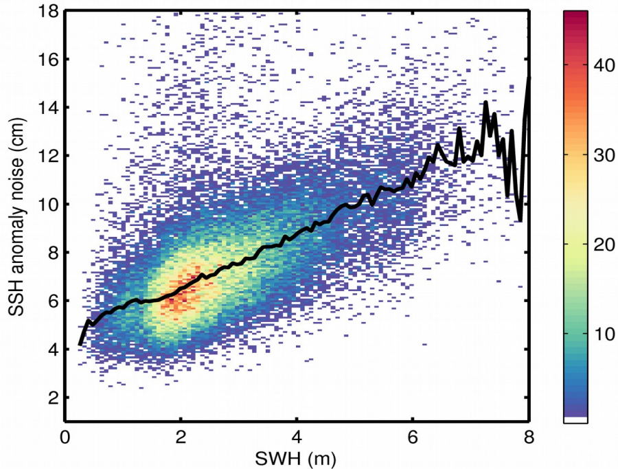
Figure 9. 2D histogram showing flag-valid SSH anomaly noise as a function of SWH for 27/10/2017. The black line denotes the median SSH anomaly noise as a function of SWH.
