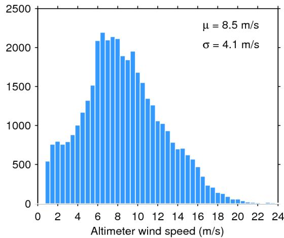
Figure 33. Histogram of flag-valid wind over oceans and lakes for 27/10/2017. The mean ( \mu ) and standard deviation ( \sigma ) are also shown. Note that values larger than 24 m/s are excluded from the histogram for the sake of readability but not from the computation of \mu and \sigma .
