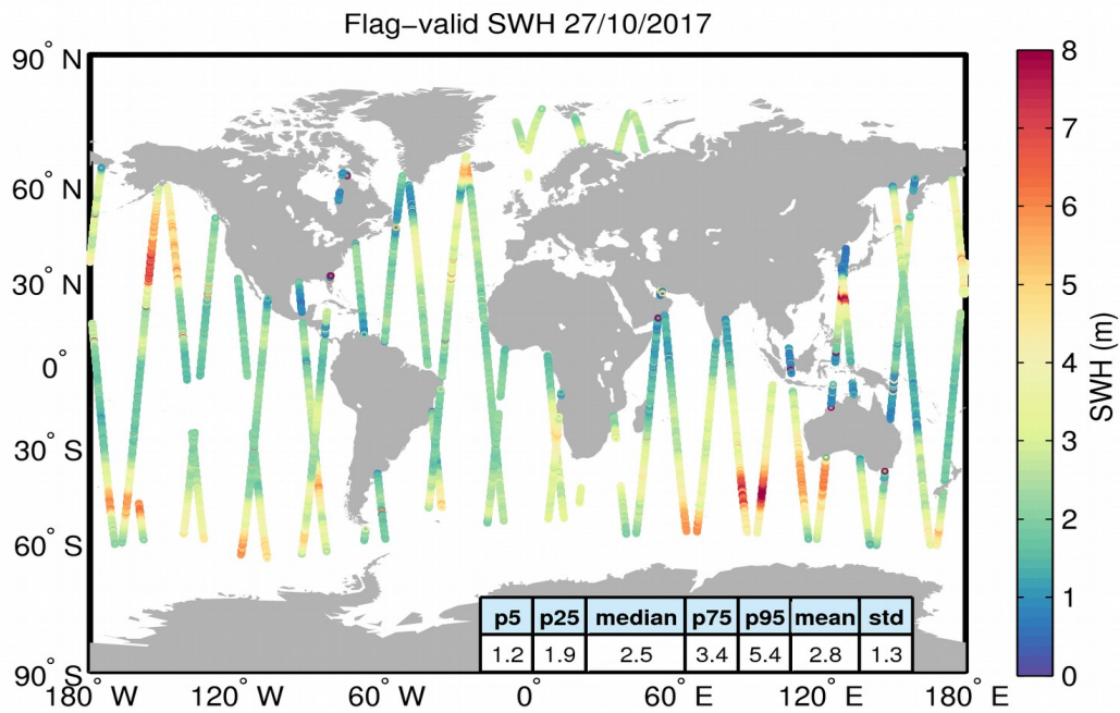
Figure 15. Geographical distribution of flag-valid SWH data over oceans and lakes for 27/10/2017. The statistical values shown in the table refer to the SWH in m and are calculated over all measurements shown in the figure.
