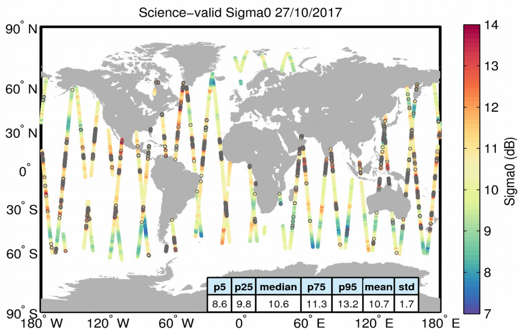
Figure 27. Geographical distribution of science-valid sigma0 data over oceans and lakes for 27/10/2017. The statistical values shown in the table refer to the sigma0 in dB and are calculated over all measurements shown in the figure. Gray circles denote records that have been rejected based on the editing criteria described in Table 4.
