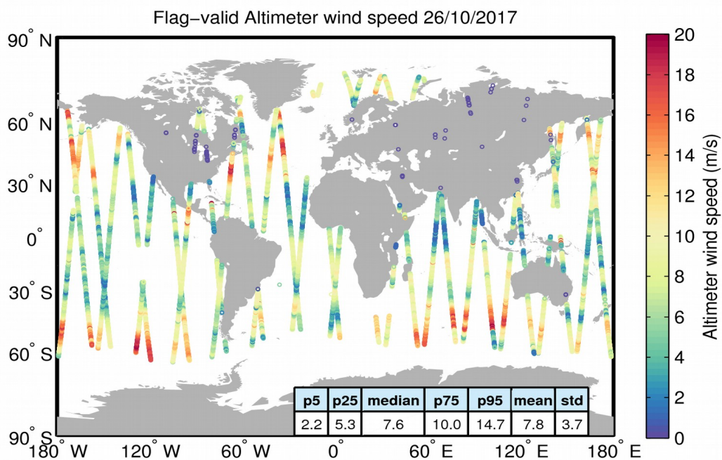
Figure 31. Geographical distribution of flag-valid wind data over oceans and lakes for 26/10/2017. The statistical values shown in the table refer to the wind in m/s and are calculated over all measurements shown in the figure.
