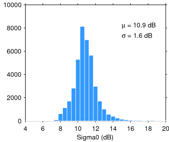
Figure 28. Histogram of science-valid sigma0 over oceans and lakes for 26/10/2017. The mean ( \mu ) and standard deviation ( \sigma ) are also shown. Note that values outside [4 20] dB are excluded from the histogram for the sake of readability but not from the computation of \mu and \sigma .
