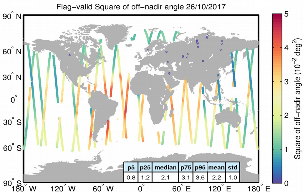
Figure 37. Geographical distribution of flag-valid mispointing data over oceans and lakes for 26/10/2017. The statistical values shown in the table refer to the mispointing in 10^{-2} deg 2 and are calculated over all measurements shown in the figure.
