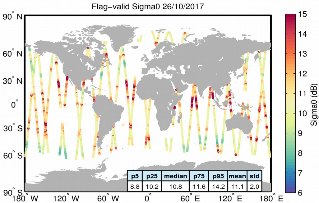
Figure 23. Geographical distribution of flag-valid sigma0 data over oceans and lakes for 26/10/2017. The statistical values shown in the table refer to the sigma0 in dB and are calculated over all measurements shown in the figure.
