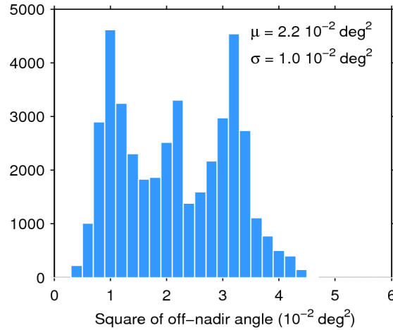
Figure 39. Histogram of flag-valid mispointing over oceans and lakes for 26/10/2017. The mean ( \mu ) and standard deviation ( \sigma ) are also shown. Note that values larger than 6 \cdot 10^{-2} \text{ deg}^2 are excluded from the histogram for the sake of readability but not from the computation of \mu and \sigma .
