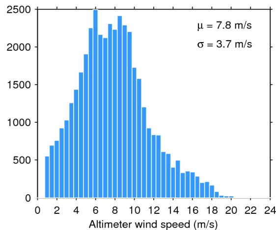
Figure 35. Histogram of science-valid wind over oceans and lakes for 26/10/2017. The mean ( \mu ) and standard deviation ( \sigma ) are also shown. Note that values larger than 24 m/s are excluded from the histogram for the sake of readability but not from the computation of \mu and \sigma .
