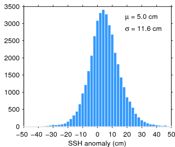
Figure 11. Histogram of science-valid SSH anomaly over oceans and lakes for 26/10/2017. The mean ( \mu ) and standard deviation ( \sigma ) are also shown. Note that values outside [-50 50] cm are excluded from the histogram for the sake of readability but not from the computation of \mu and \sigma .
