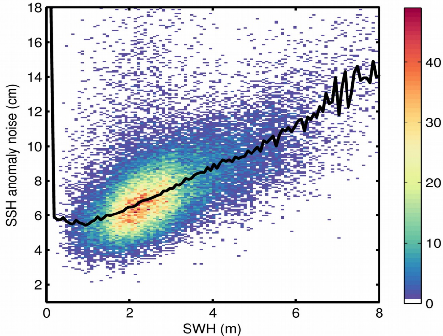
Figure 9. 2D histogram showing flag-valid SSH anomaly noise as a function of SWH for 26/10/2017. The black line denotes the median SSH anomaly noise as a function of SWH.
