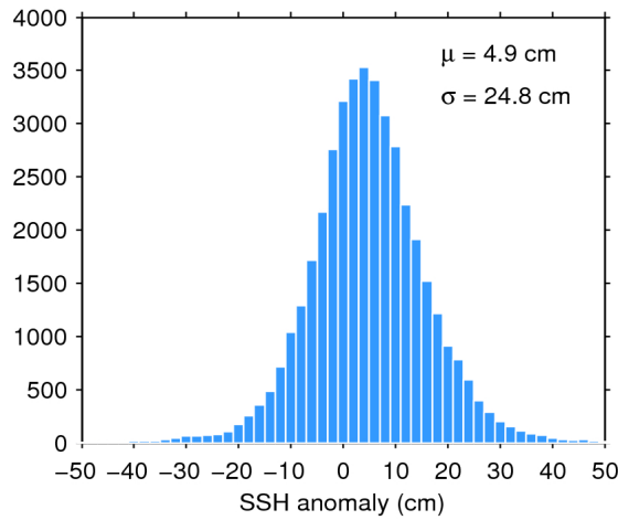
Figure 7. Histogram of flag-valid SSH anomaly over oceans and lakes for 26/10/2017. The mean ( \mu ) and standard deviation ( \sigma ) are also shown. Note that values outside [-50 50] cm are excluded from the histogram for the sake of readability but not from the computation of \mu and \sigma .
