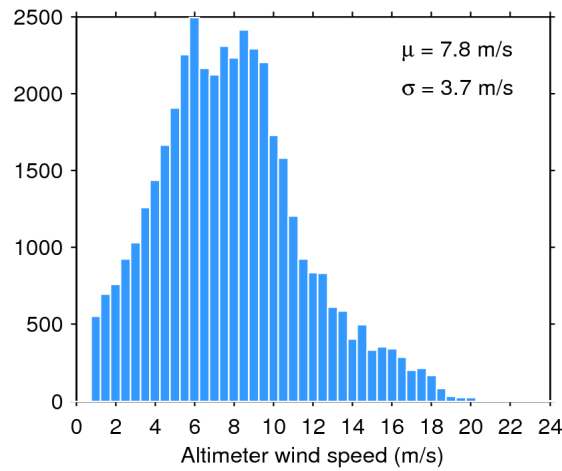
Figure 33. Histogram of flag-valid wind over oceans and lakes for 26/10/2017. The mean ( \mu ) and standard deviation ( \sigma ) are also shown. Note that values larger than 24 m/s are excluded from the histogram for the sake of readability but not from the computation of \mu and \sigma .
