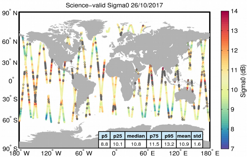
Figure 27. Geographical distribution of science-valid sigma0 data over oceans and lakes for 26/10/2017. The statistical values shown in the table refer to the sigma0 in dB and are calculated over all measurements shown in the figure. Gray circles denote records that have been rejected based on the editing criteria described in Table 4.
