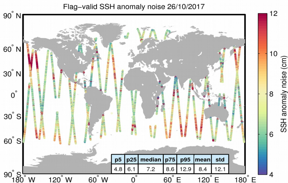
Figure 8. Geographical distribution of flag-valid 20-Hz SSH anomaly measurement noise over oceans and lakes for 26/10/2017. The statistical values shown in the table refer to the SSH anomaly noise and are calculated over all measurements shown in the figure.
