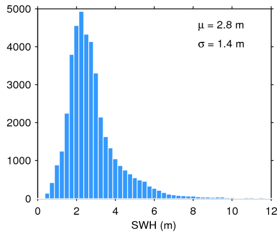
Figure 17. Histogram of flag-valid SWH over oceans and lakes for 26/10/2017. The mean ( \mu ) and standard deviation ( \sigma ) are also shown. Note that values larger than 12 m are excluded from the histogram for the sake of readability but not from the computation of \mu and \sigma .
