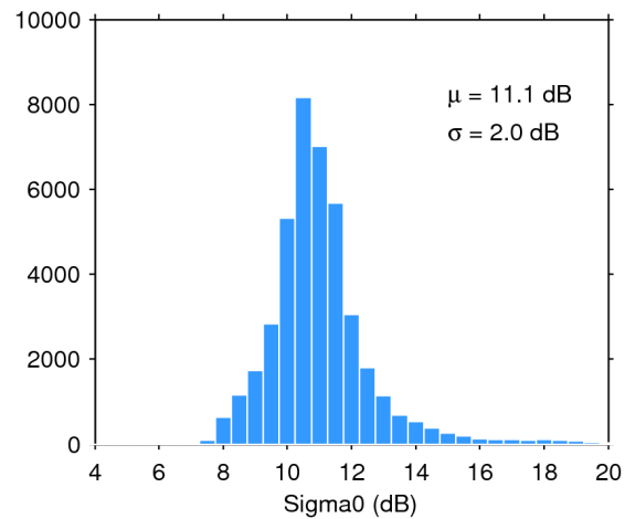
Figure 25. Histogram of flag-valid sigma0 over oceans and lakes for 26/10/2017. The mean ( \mu ) and standard deviation ( \sigma ) are also shown. Note that values outside [4 20] dB are excluded from the histogram for the sake of readability but not from the computation of \mu and \sigma .
