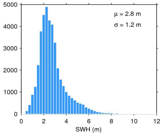
Figure 20. Histogram of science-valid SWH over oceans and lakes for 26/10/2017. The mean ( \mu ) and standard deviation ( \sigma ) are also shown. Note that values larger than 12 m are excluded from the histogram for the sake of readability but not from the computation of \mu and \sigma .
