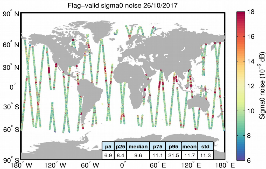
Figure 26. Geographical distribution of flag-valid 20-Hz sigma0 measurement noise over oceans and lakes for 26/10/2017. The statistical values shown in the table refer to the sigma0 noise and are calculated over all measurements shown in the figure.
