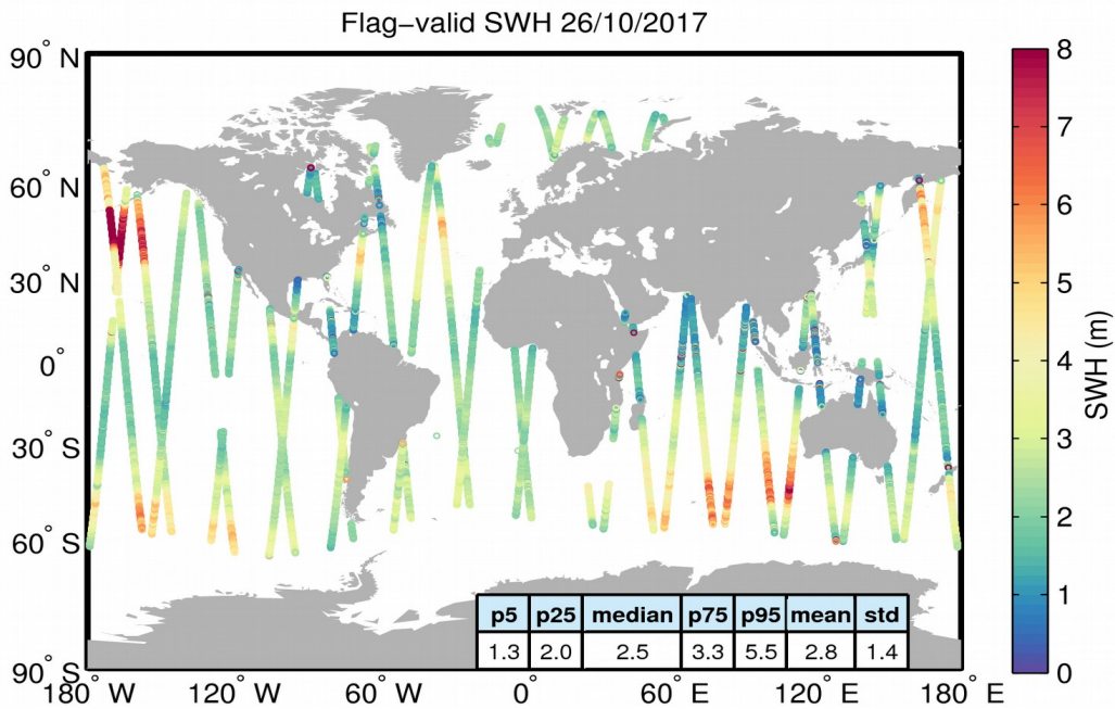
Figure 15. Geographical distribution of flag-valid SWH data over oceans and lakes for 26/10/2017. The statistical values shown in the table refer to the SWH in m and are calculated over all measurements shown in the figure.
