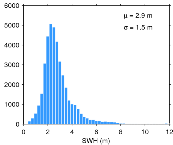
Figure 17. Histogram of flag-valid SWH over oceans and lakes for 25/10/2017. The mean ( \mu ) and standard deviation ( \sigma ) are also shown. Note that values larger than 12 m are excluded from the histogram for the sake of readability but not from the computation of \mu and \sigma .
