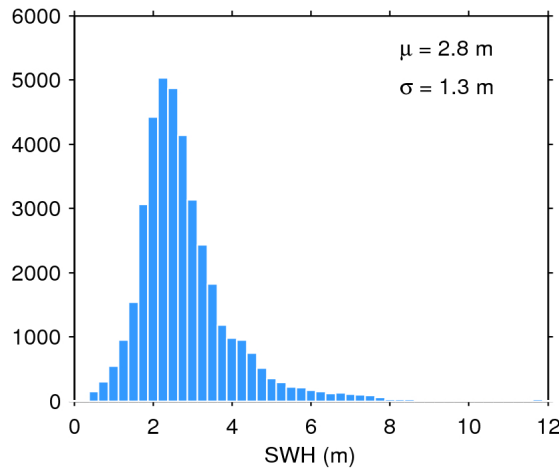
Figure 20. Histogram of science-valid SWH over oceans and lakes for 25/10/2017. The mean ( \mu ) and standard deviation ( \sigma ) are also shown. Note that values larger than 12 m are excluded from the histogram for the sake of readability but not from the computation of \mu and \sigma .
