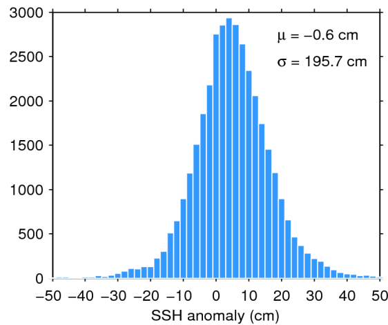
Figure 7. Histogram of flag-valid SSH anomaly over oceans and lakes for 25/10/2017. The mean ( \mu ) and standard deviation ( \sigma ) are also shown. Note that values outside [-50 50] cm are excluded from the histogram for the sake of readability but not from the computation of \mu and \sigma .
