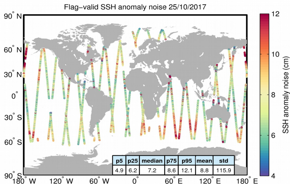
Figure 8. Geographical distribution of flag-valid 20-Hz SSH anomaly measurement noise over oceans and lakes for 25/10/2017. The statistical values shown in the table refer to the SSH anomaly noise and are calculated over all measurements shown in the figure.
