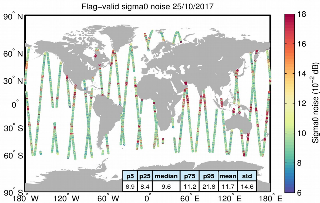
Figure 26. Geographical distribution of flag-valid 20-Hz sigma0 measurement noise over oceans and lakes for 25/10/2017. The statistical values shown in the table refer to the sigma0 noise and are calculated over all measurements shown in the figure.
