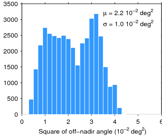
Figure 39. Histogram of flag-valid mispointing over oceans and lakes for 25/10/2017. The mean ( \mu ) and standard deviation ( \sigma ) are also shown. Note that values larger than 6 \cdot 10^{-2} \text{ deg}^2 are excluded from the histogram for the sake of readability but not from the computation of \mu and \sigma .
