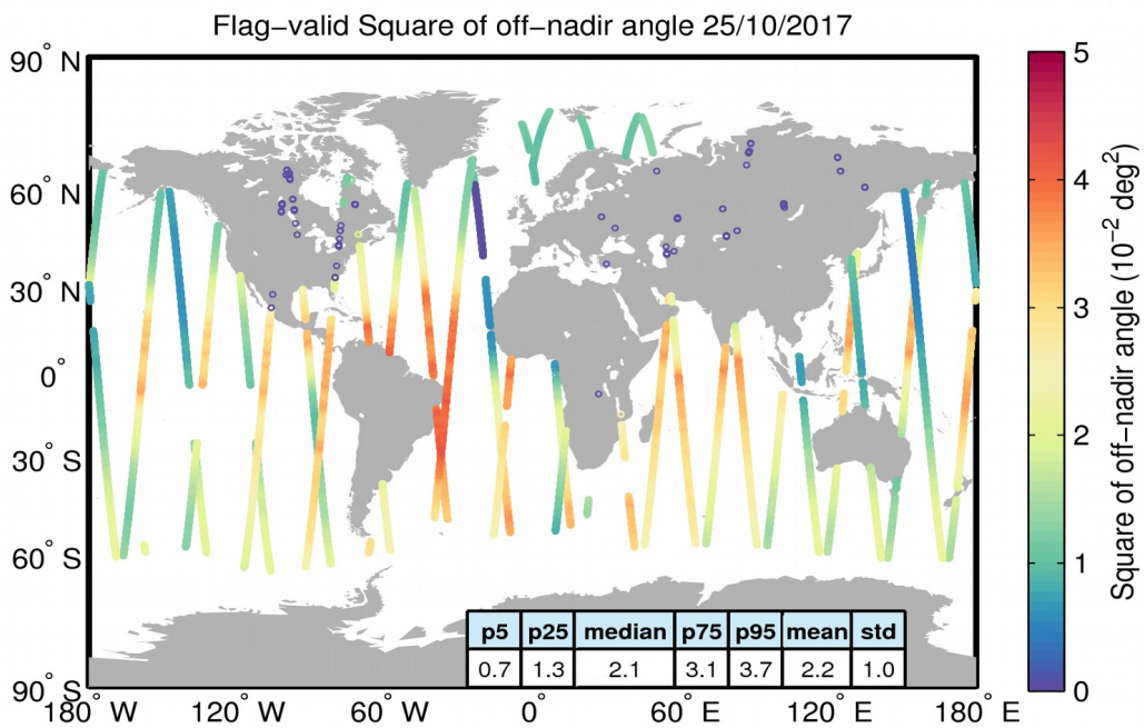
Figure 37. Geographical distribution of flag-valid mispointing data over oceans and lakes for 25/10/2017. The statistical values shown in the table refer to the mispointing in 10^{-2} deg 2 and are calculated over all measurements shown in the figure.
