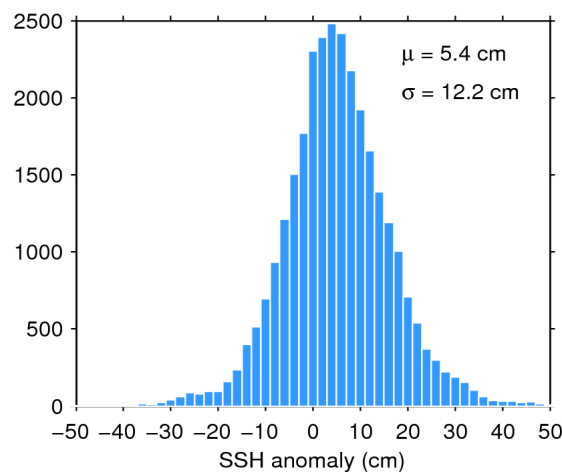
Figure 11. Histogram of science-valid SSH anomaly over oceans and lakes for 25/10/2017. The mean ( \mu ) and standard deviation ( \sigma ) are also shown. Note that values outside [-50 50] cm are excluded from the histogram for the sake of readability but not from the computation of \mu and \sigma .
