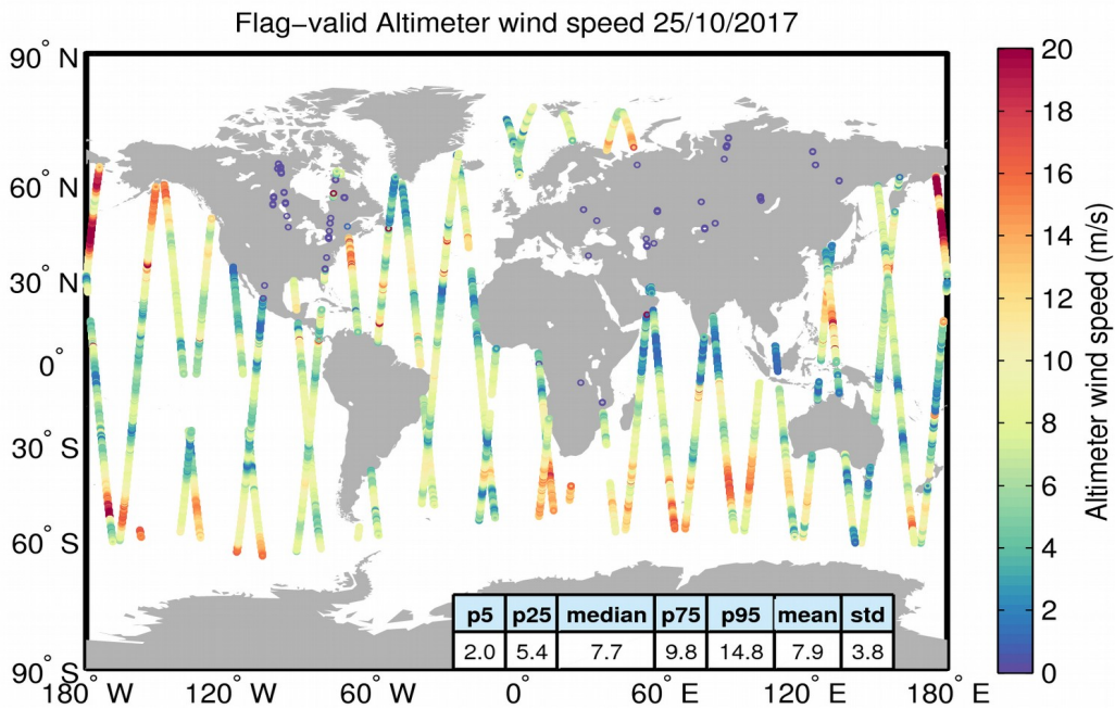
Figure 31. Geographical distribution of flag-valid wind data over oceans and lakes for 25/10/2017. The statistical values shown in the table refer to the wind in m/s and are calculated over all measurements shown in the figure.
