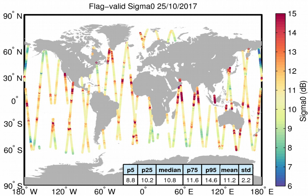
Figure 23. Geographical distribution of flag-valid sigma0 data over oceans and lakes for 25/10/2017. The statistical values shown in the table refer to the sigma0 in dB and are calculated over all measurements shown in the figure.
