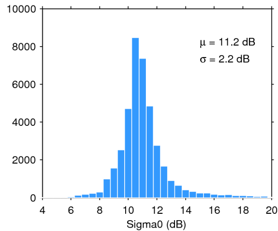
Figure 25. Histogram of flag-valid sigma0 over oceans and lakes for 25/10/2017. The mean ( \mu ) and standard deviation ( \sigma ) are also shown. Note that values outside [4 20] dB are excluded from the histogram for the sake of readability but not from the computation of \mu and \sigma .
