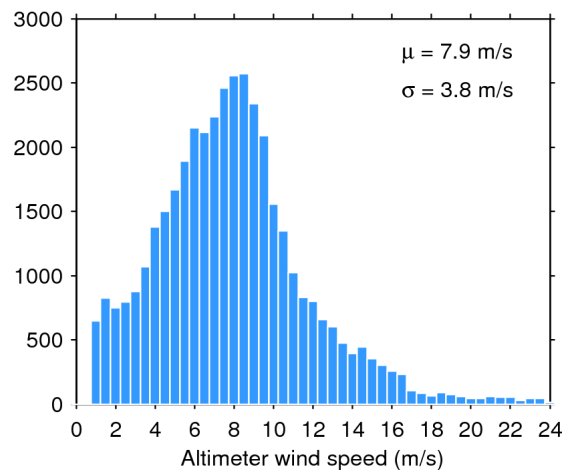
Figure 35. Histogram of science-valid wind over oceans and lakes for 25/10/2017. The mean ( \mu ) and standard deviation ( \sigma ) are also shown. Note that values larger than 24 m/s are excluded from the histogram for the sake of readability but not from the computation of \mu and \sigma .
