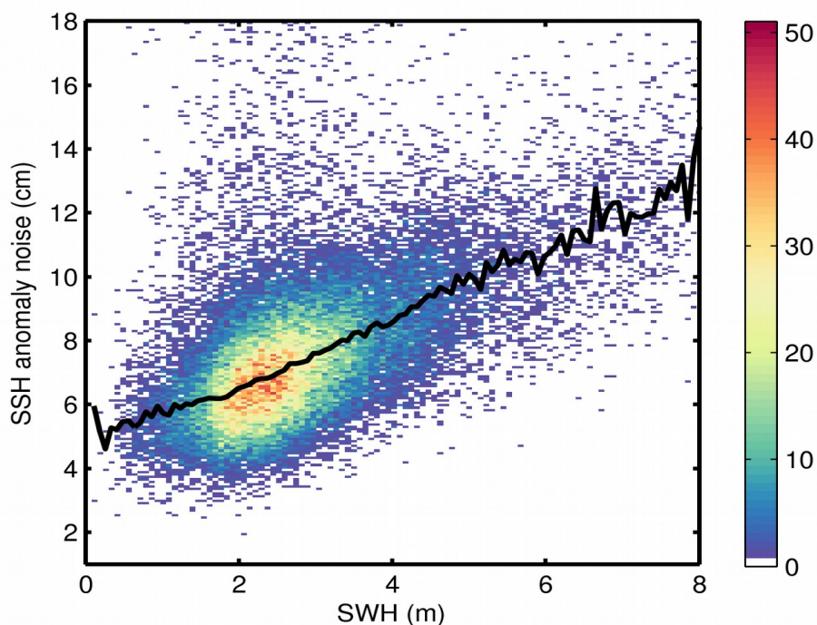
Figure 9. 2D histogram showing flag-valid SSH anomaly noise as a function of SWH for 25/10/2017. The black line denotes the median SSH anomaly noise as a function of SWH.
