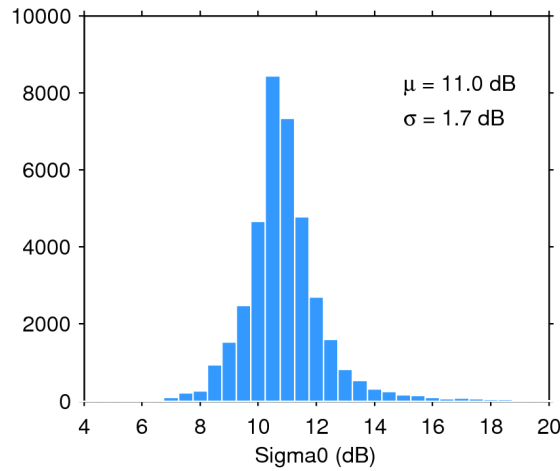
Figure 28. Histogram of science-valid sigma0 over oceans and lakes for 25/10/2017. The mean ( \mu ) and standard deviation ( \sigma ) are also shown. Note that values outside [4 20] dB are excluded from the histogram for the sake of readability but not from the computation of \mu and \sigma .
