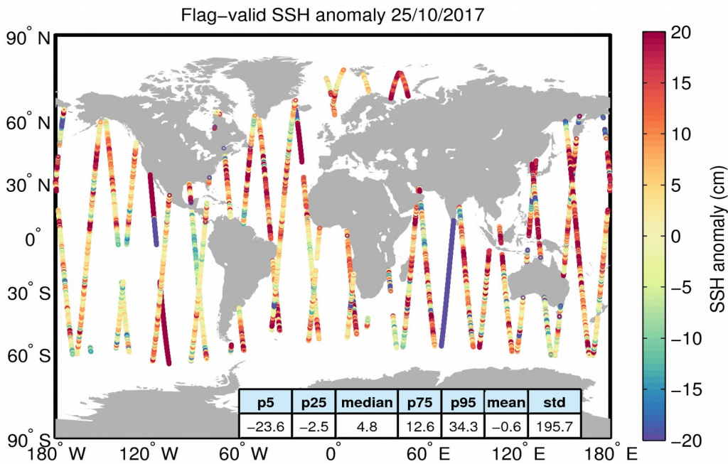
Figure 5. Geographical distribution of flag-valid 1-Hz SSH anomaly data over oceans and lakes for 25/10/2017. The statistical values shown in the table refer to the SSH anomaly in cm and are calculated over all measurements shown in the figure.
