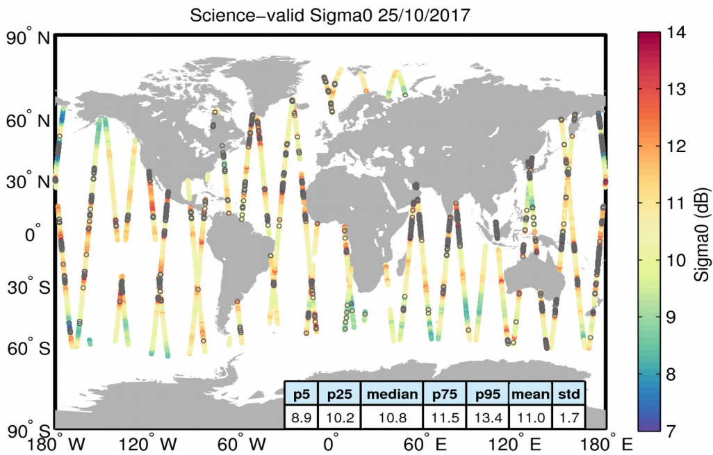
Figure 27. Geographical distribution of science-valid sigma0 data over oceans and lakes for 25/10/2017. The statistical values shown in the table refer to the sigma0 in dB and are calculated over all measurements shown in the figure. Gray circles denote records that have been rejected based on the editing criteria described in Table 4.
