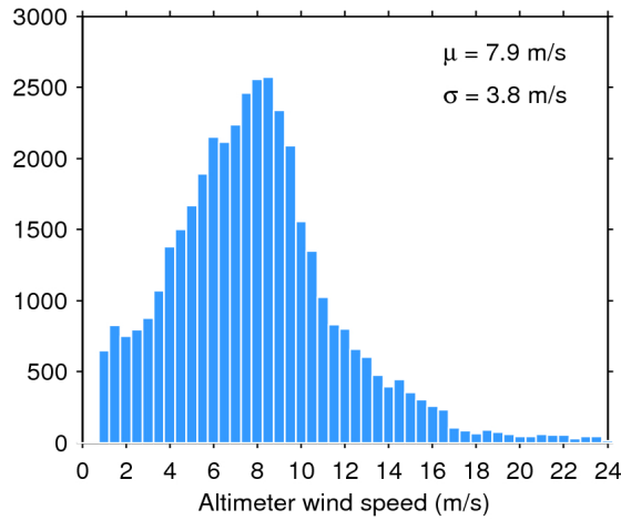
Figure 33. Histogram of flag-valid wind over oceans and lakes for 25/10/2017. The mean ( \mu ) and standard deviation ( \sigma ) are also shown. Note that values larger than 24 m/s are excluded from the histogram for the sake of readability but not from the computation of \mu and \sigma .
