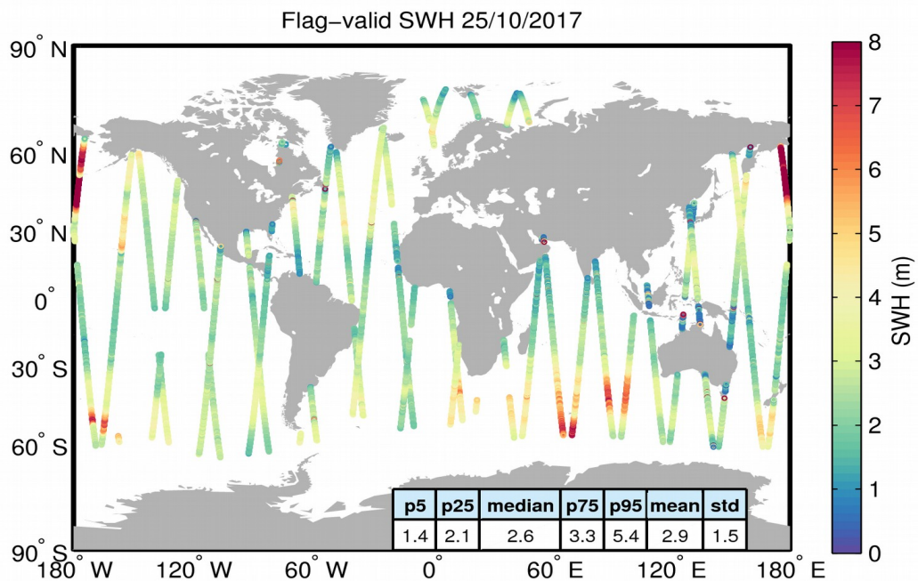
Figure 15. Geographical distribution of flag-valid SWH data over oceans and lakes for 25/10/2017. The statistical values shown in the table refer to the SWH in m and are calculated over all measurements shown in the figure.
