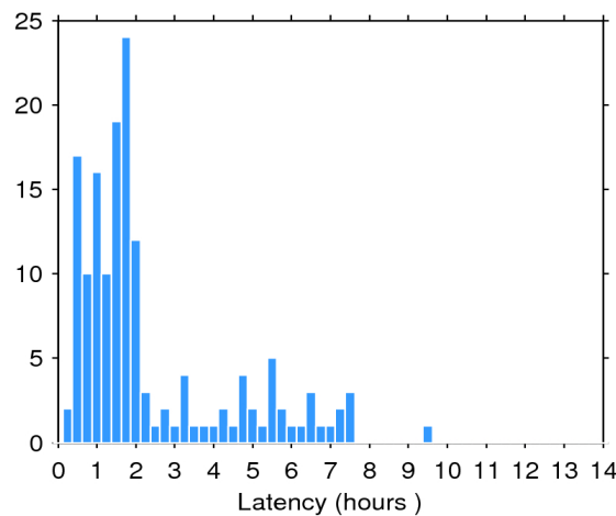
Figure 2. Histogram of the data latency for 23/10/2017. The y-axis denotes the number of files that are made available with a delay of x-hours with respect to the mean time of the records stored in the file.
