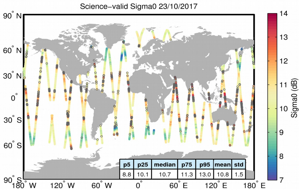
Figure 27. Geographical distribution of science-valid sigma0 data over oceans and lakes for 23/10/2017. The statistical values shown in the table refer to the sigma0 in dB and are calculated over all measurements shown in the figure. Gray circles denote records that have been rejected based on the editing criteria described in Table 4.
