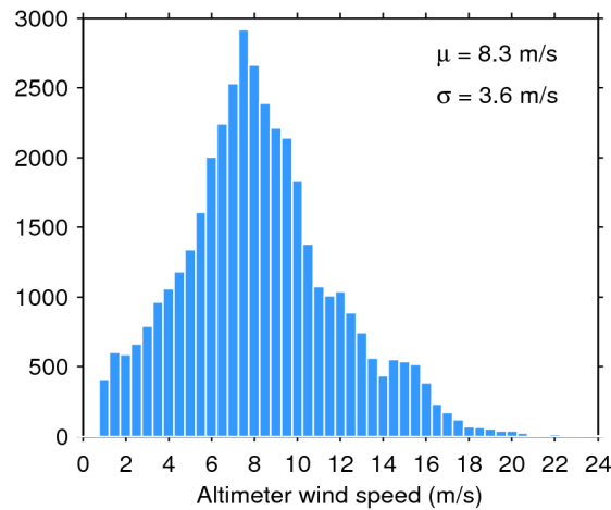
Figure 33. Histogram of flag-valid wind over oceans and lakes for 23/10/2017. The mean ( \mu ) and standard deviation ( \sigma ) are also shown. Note that values larger than 24 m/s are excluded from the histogram for the sake of readability but not from the computation of \mu and \sigma .
