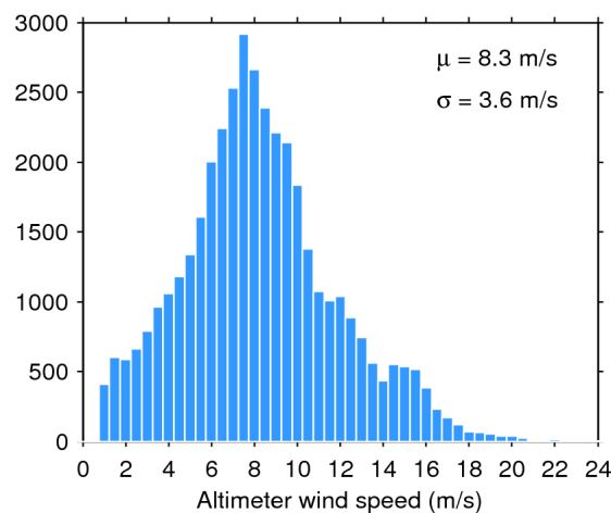
Figure 35. Histogram of science-valid wind over oceans and lakes for 23/10/2017. The mean ( \mu ) and standard deviation ( \sigma ) are also shown. Note that values larger than 24 m/s are excluded from the histogram for the sake of readability but not from the computation of \mu and \sigma .
