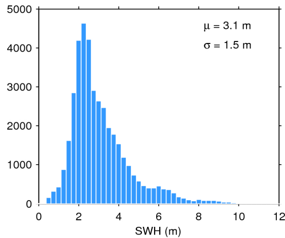
Figure 17. Histogram of flag-valid SWH over oceans and lakes for 23/10/2017. The mean ( \mu ) and standard deviation ( \sigma ) are also shown. Note that values larger than 12 m are excluded from the histogram for the sake of readability but not from the computation of \mu and \sigma .
