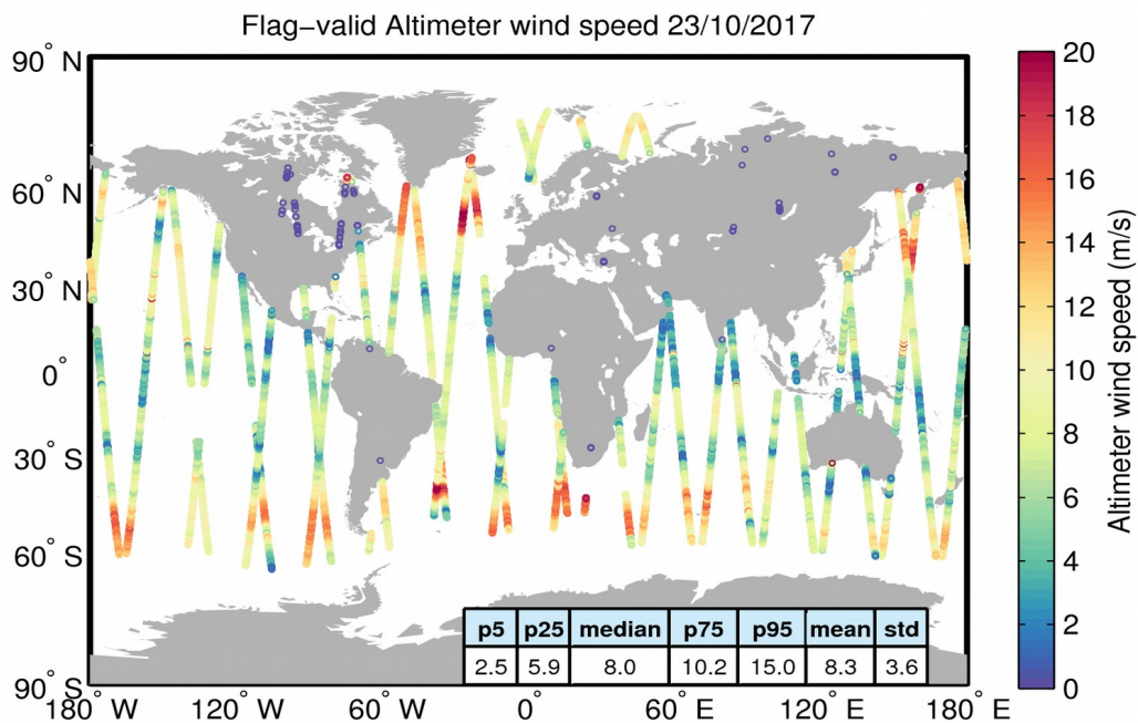
Figure 31. Geographical distribution of flag-valid wind data over oceans and lakes for 23/10/2017. The statistical values shown in the table refer to the wind in m/s and are calculated over all measurements shown in the figure.
