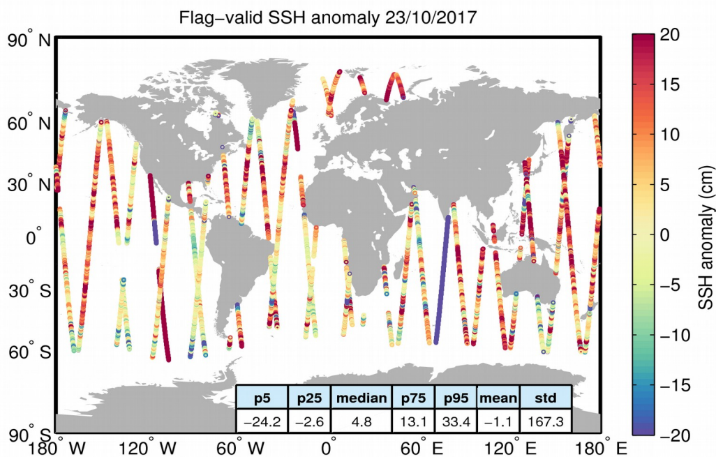
Figure 5. Geographical distribution of flag-valid 1-Hz SSH anomaly data over oceans and lakes for 23/10/2017. The statistical values shown in the table refer to the SSH anomaly in cm and are calculated over all measurements shown in the figure.
