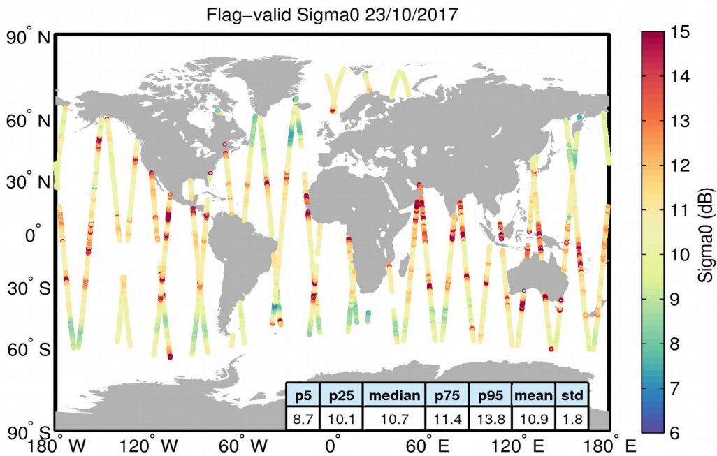
Figure 23. Geographical distribution of flag-valid sigma0 data over oceans and lakes for 23/10/2017. The statistical values shown in the table refer to the sigma0 in dB and are calculated over all measurements shown in the figure.
