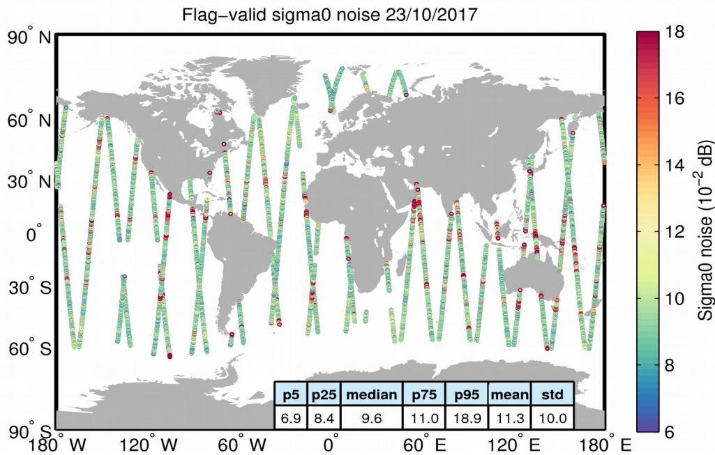
Figure 26. Geographical distribution of flag-valid 20-Hz sigma0 measurement noise over oceans and lakes for 23/10/2017. The statistical values shown in the table refer to the sigma0 noise and are calculated over all measurements shown in the figure.
