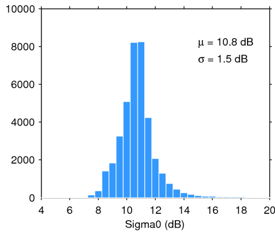
Figure 28. Histogram of science-valid sigma0 over oceans and lakes for 23/10/2017. The mean ( \mu ) and standard deviation ( \sigma ) are also shown. Note that values outside [4 20] dB are excluded from the histogram for the sake of readability but not from the computation of \mu and \sigma .
