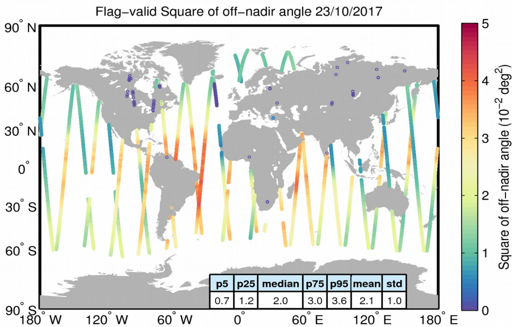
Figure 37. Geographical distribution of flag-valid mispointing data over oceans and lakes for 23/10/2017. The statistical values shown in the table refer to the mispointing in 10^{-2} deg 2 and are calculated over all measurements shown in the figure.
