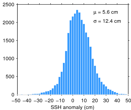
Figure 11. Histogram of science-valid SSH anomaly over oceans and lakes for 23/10/2017. The mean ( \mu ) and standard deviation ( \sigma ) are also shown. Note that values outside [-50 50] cm are excluded from the histogram for the sake of readability but not from the computation of \mu and \sigma .
