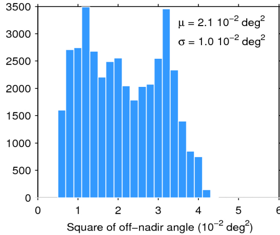
Figure 39. Histogram of flag-valid mispointing over oceans and lakes for 23/10/2017. The mean ( \mu ) and standard deviation ( \sigma ) are also shown. Note that values larger than 6 \cdot 10^{-2} \text{ deg}^2 are excluded from the histogram for the sake of readability but not from the computation of \mu and \sigma .
