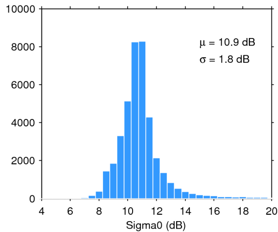
Figure 25. Histogram of flag-valid sigma0 over oceans and lakes for 23/10/2017. The mean ( \mu ) and standard deviation ( \sigma ) are also shown. Note that values outside [4 20] dB are excluded from the histogram for the sake of readability but not from the computation of \mu and \sigma .
