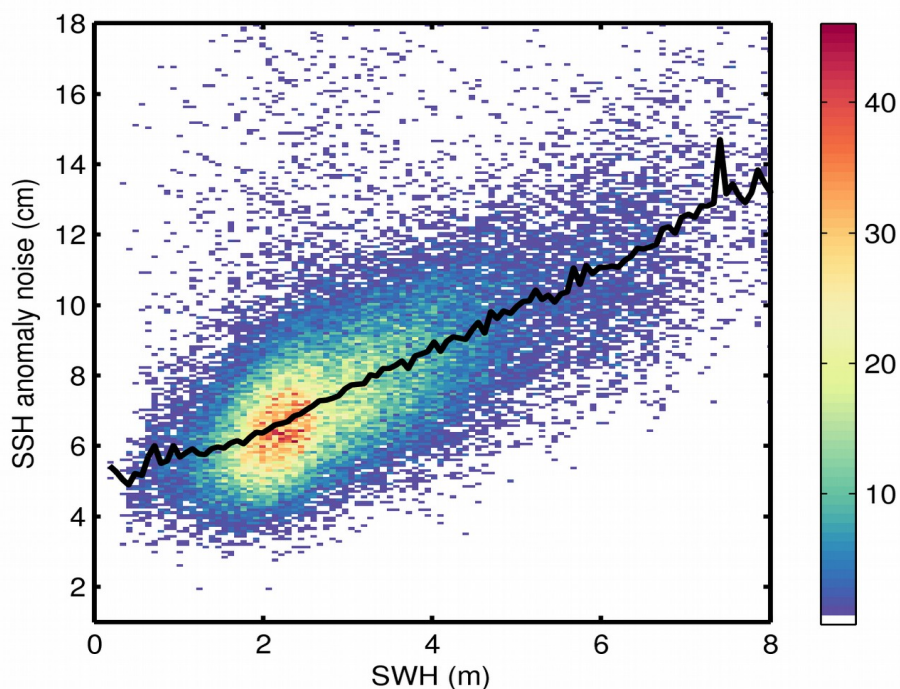
Figure 9. 2D histogram showing flag-valid SSH anomaly noise as a function of SWH for 23/10/2017. The black line denotes the median SSH anomaly noise as a function of SWH.
