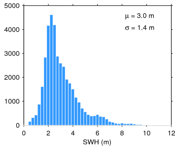
Figure 20. Histogram of science-valid SWH over oceans and lakes for 23/10/2017. The mean ( \mu ) and standard deviation ( \sigma ) are also shown. Note that values larger than 12 m are excluded from the histogram for the sake of readability but not from the computation of \mu and \sigma .
