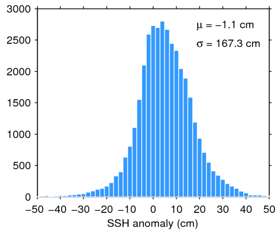
Figure 7. Histogram of flag-valid SSH anomaly over oceans and lakes for 23/10/2017. The mean ( \mu ) and standard deviation ( \sigma ) are also shown. Note that values outside [-50 50] cm are excluded from the histogram for the sake of readability but not from the computation of \mu and \sigma .
