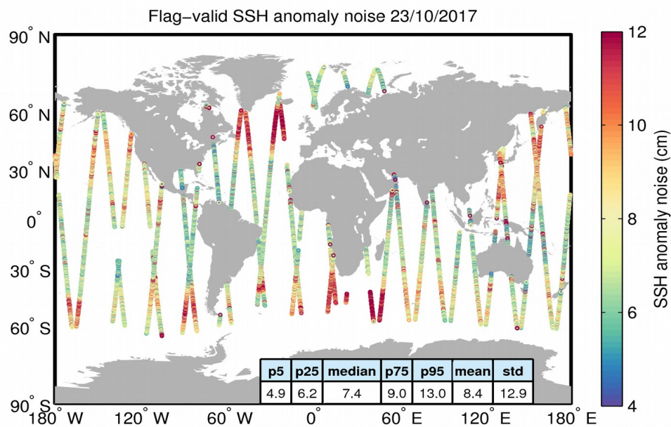
Figure 8. Geographical distribution of flag-valid 20-Hz SSH anomaly measurement noise over oceans and lakes for 23/10/2017. The statistical values shown in the table refer to the SSH anomaly noise and are calculated over all measurements shown in the figure.
