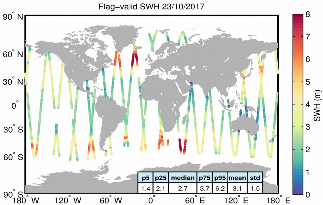
Figure 15. Geographical distribution of flag-valid SWH data over oceans and lakes for 23/10/2017. The statistical values shown in the table refer to the SWH in m and are calculated over all measurements shown in the figure.
