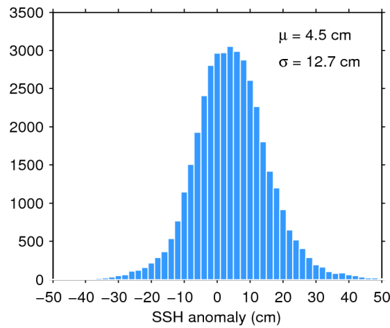
Figure 11. Histogram of science-valid SSH anomaly over oceans and lakes for 22/10/2017. The mean ( \mu ) and standard deviation ( \sigma ) are also shown. Note that values outside [-50 50] cm are excluded from the histogram for the sake of readability but not from the computation of \mu and \sigma .
