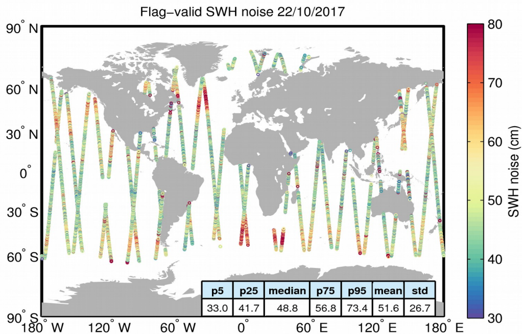
Figure 18. Geographical distribution of flag-valid 20-Hz SWH measurement noise over oceans and lakes for 22/10/2017. The statistical values shown in the table refer to the SWH noise and are calculated over all measurements shown in the figure.
