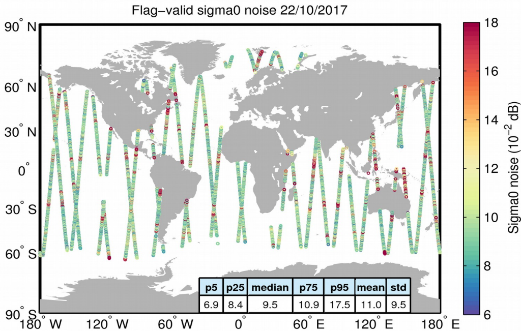
Figure 26. Geographical distribution of flag-valid 20-Hz sigma0 measurement noise over oceans and lakes for 22/10/2017. The statistical values shown in the table refer to the sigma0 noise and are calculated over all measurements shown in the figure.
