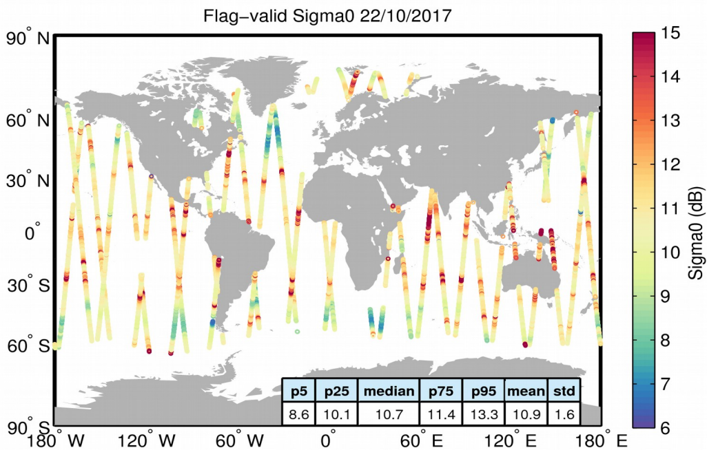
Figure 23. Geographical distribution of flag-valid sigma0 data over oceans and lakes for 22/10/2017. The statistical values shown in the table refer to the sigma0 in dB and are calculated over all measurements shown in the figure.
