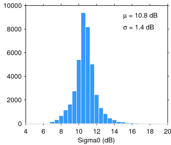
Figure 28. Histogram of science-valid sigma0 over oceans and lakes for 22/10/2017. The mean ( \mu ) and standard deviation ( \sigma ) are also shown. Note that values outside [4 20] dB are excluded from the histogram for the sake of readability but not from the computation of \mu and \sigma .
