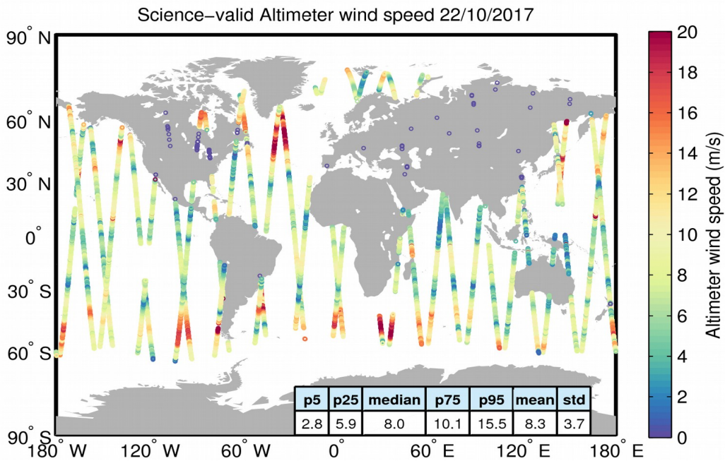
Figure 34. Geographical distribution of science-valid wind data over oceans and lakes for 22/10/2017. The statistical values shown in the table refer to the wind in m/s and are calculated over all measurements shown in the figure. Gray circles denote records that have been rejected based on the editing criteria described in Table 5.
