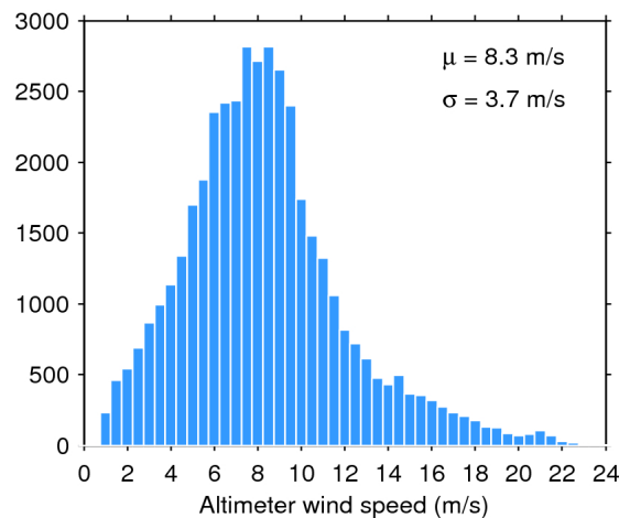
Figure 35. Histogram of science-valid wind over oceans and lakes for 22/10/2017. The mean ( \mu ) and standard deviation ( \sigma ) are also shown. Note that values larger than 24 m/s are excluded from the histogram for the sake of readability but not from the computation of \mu and \sigma .
