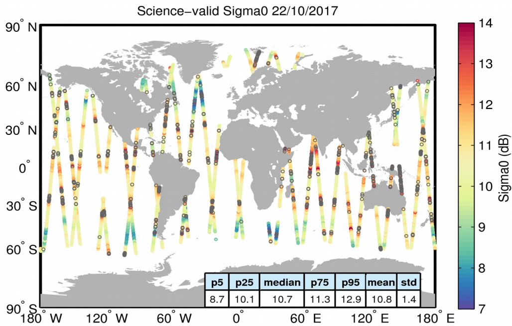
Figure 27. Geographical distribution of science-valid sigma0 data over oceans and lakes for 22/10/2017. The statistical values shown in the table refer to the sigma0 in dB and are calculated over all measurements shown in the figure. Gray circles denote records that have been rejected based on the editing criteria described in Table 4.
