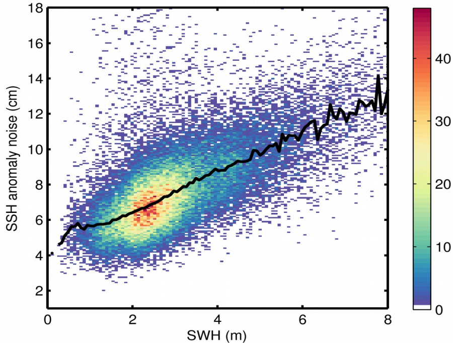
Figure 9. 2D histogram showing flag-valid SSH anomaly noise as a function of SWH for 22/10/2017. The black line denotes the median SSH anomaly noise as a function of SWH.
