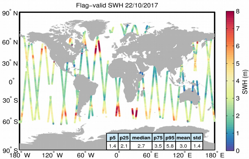
Figure 15. Geographical distribution of flag-valid SWH data over oceans and lakes for 22/10/2017. The statistical values shown in the table refer to the SWH in m and are calculated over all measurements shown in the figure.
