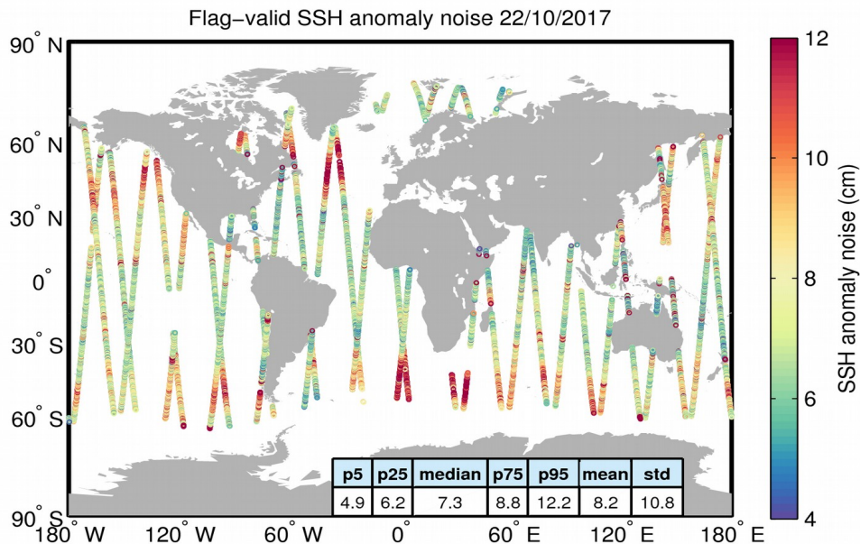
Figure 8. Geographical distribution of flag-valid 20-Hz SSH anomaly measurement noise over oceans and lakes for 22/10/2017. The statistical values shown in the table refer to the SSH anomaly noise and are calculated over all measurements shown in the figure.
