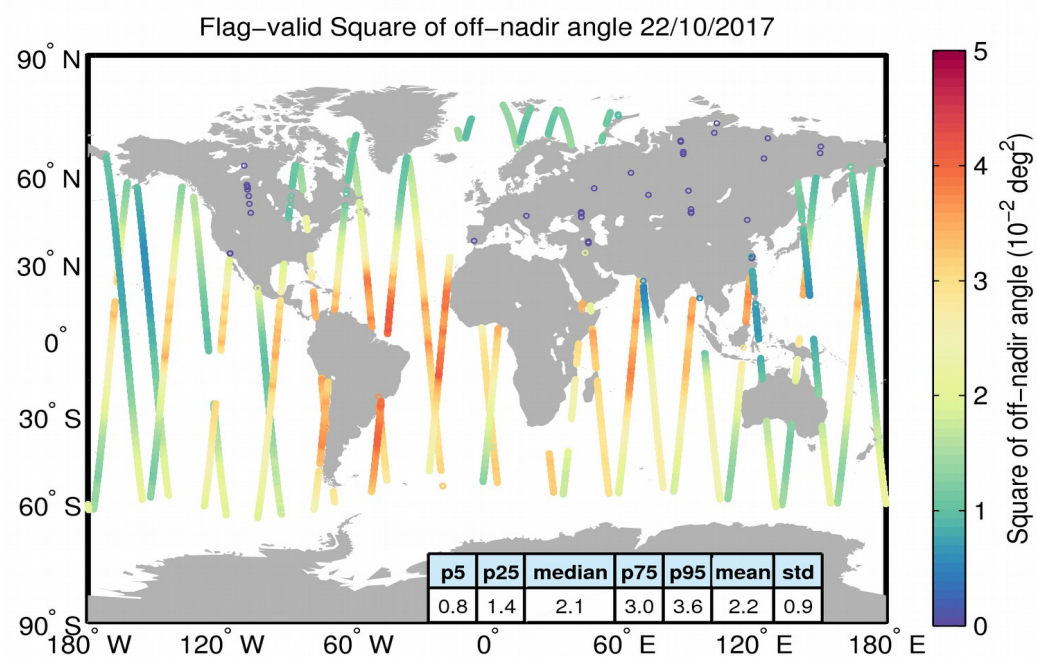
Figure 37. Geographical distribution of flag-valid mispointing data over oceans and lakes for 22/10/2017. The statistical values shown in the table refer to the mispointing in 10^{-2} deg 2 and are calculated over all measurements shown in the figure.
