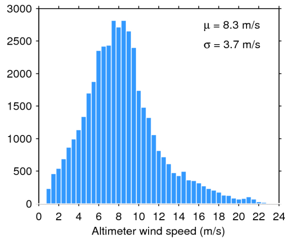
Figure 33. Histogram of flag-valid wind over oceans and lakes for 22/10/2017. The mean ( \mu ) and standard deviation ( \sigma ) are also shown. Note that values larger than 24 m/s are excluded from the histogram for the sake of readability but not from the computation of \mu and \sigma .
