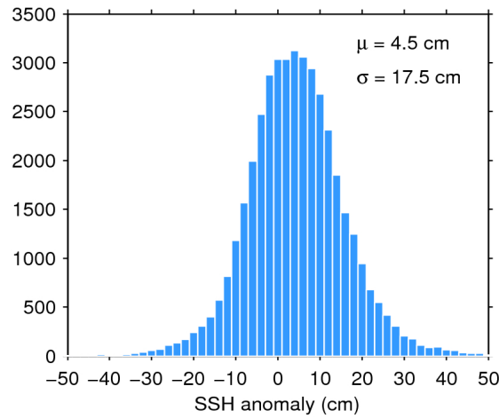
Figure 7. Histogram of flag-valid SSH anomaly over oceans and lakes for 22/10/2017. The mean ( \mu ) and standard deviation ( \sigma ) are also shown. Note that values outside [-50 50] cm are excluded from the histogram for the sake of readability but not from the computation of \mu and \sigma .
