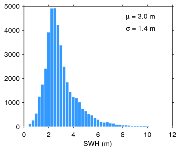
Figure 20. Histogram of science-valid SWH over oceans and lakes for 22/10/2017. The mean ( \mu ) and standard deviation ( \sigma ) are also shown. Note that values larger than 12 m are excluded from the histogram for the sake of readability but not from the computation of \mu and \sigma .
