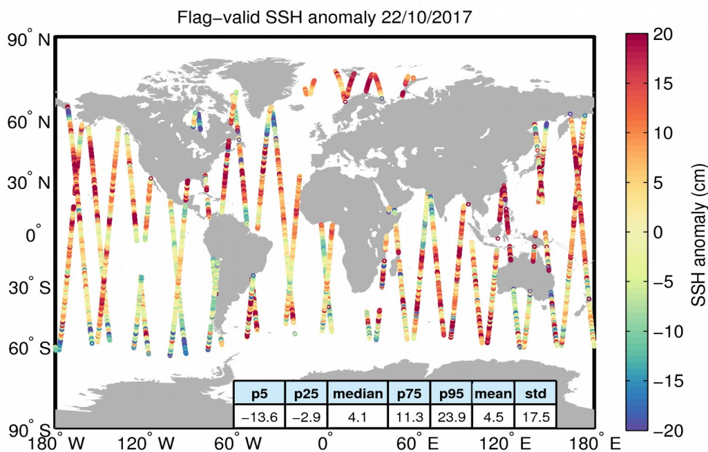
Figure 5. Geographical distribution of flag-valid 1-Hz SSH anomaly data over oceans and lakes for 22/10/2017. The statistical values shown in the table refer to the SSH anomaly in cm and are calculated over all measurements shown in the figure.
