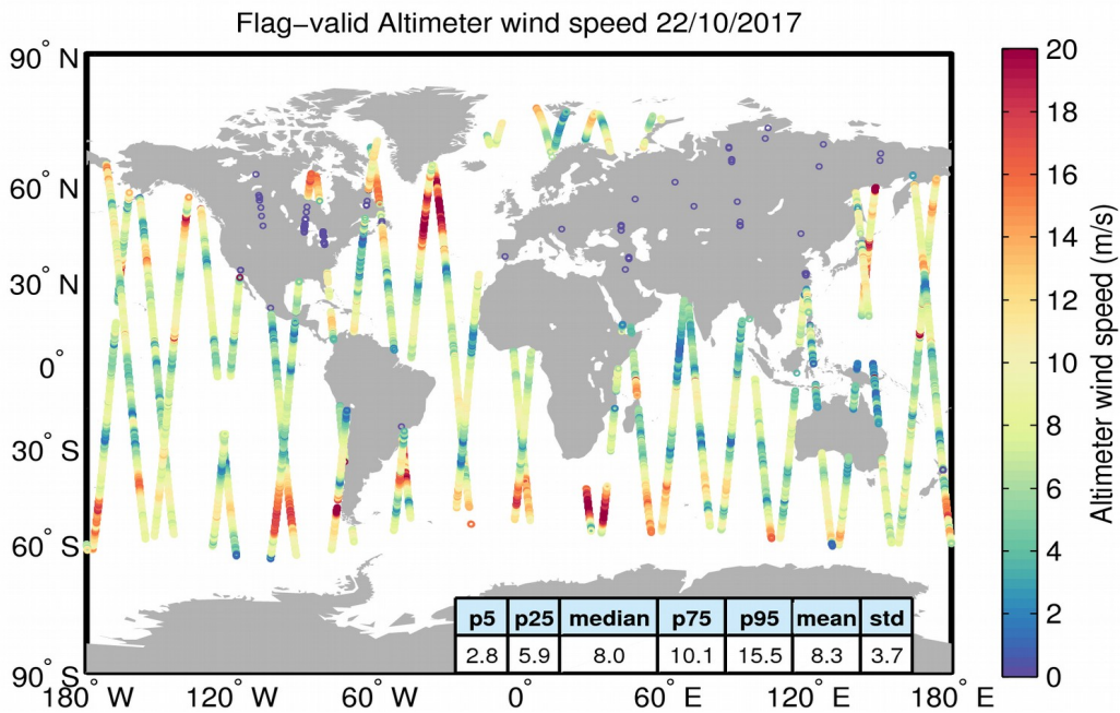
Figure 31. Geographical distribution of flag-valid wind data over oceans and lakes for 22/10/2017. The statistical values shown in the table refer to the wind in m/s and are calculated over all measurements shown in the figure.
