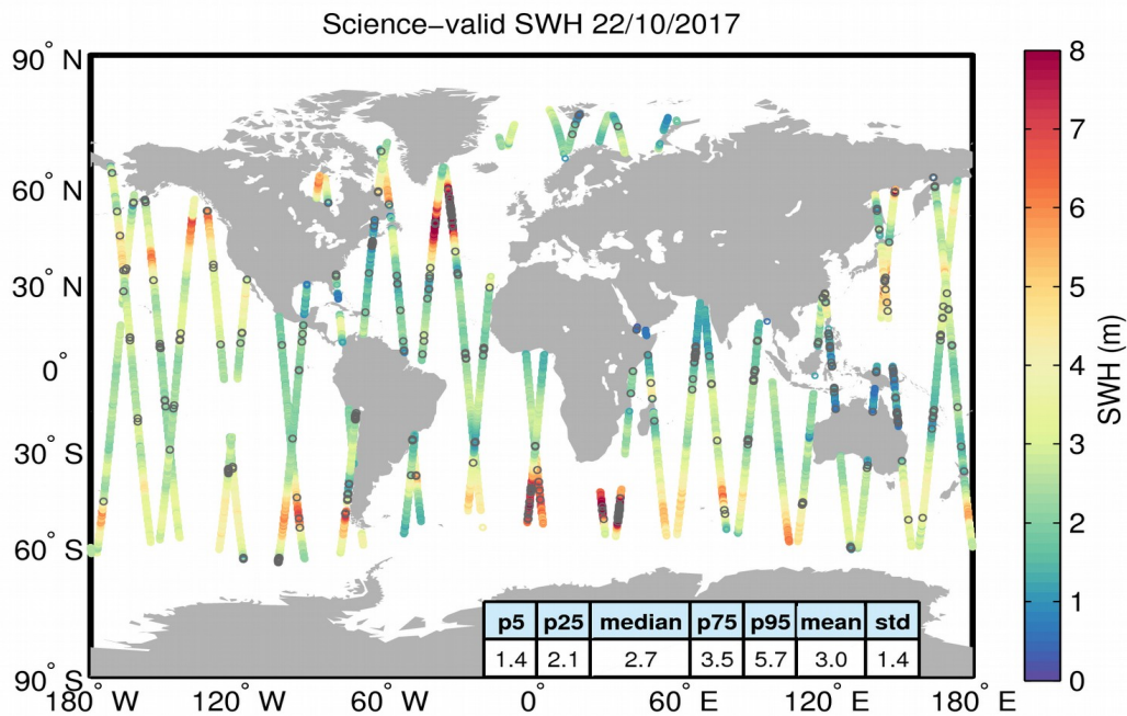
Figure 19. Geographical distribution of science-valid SWH data over oceans and lakes for 22/10/2017. The statistical values shown in the table refer to the SWH in m and are calculated over all measurements shown in the figure. Gray circles denote records that have been rejected based on the editing criteria described in Table 3.
