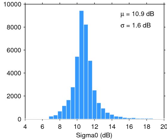
Figure 25. Histogram of flag-valid sigma0 over oceans and lakes for 22/10/2017. The mean ( \mu ) and standard deviation ( \sigma ) are also shown. Note that values outside [4 20] dB are excluded from the histogram for the sake of readability but not from the computation of \mu and \sigma .
