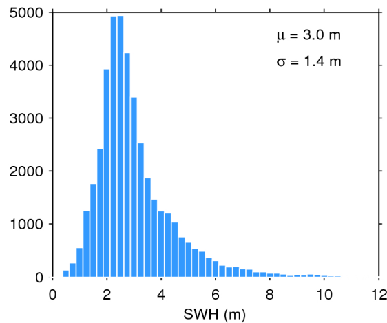
Figure 17. Histogram of flag-valid SWH over oceans and lakes for 22/10/2017. The mean ( \mu ) and standard deviation ( \sigma ) are also shown. Note that values larger than 12 m are excluded from the histogram for the sake of readability but not from the computation of \mu and \sigma .
