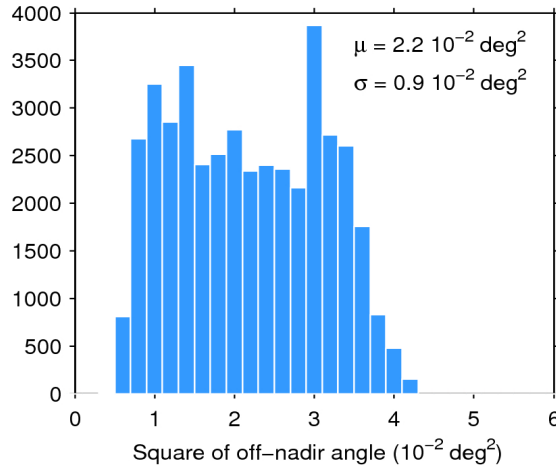
Figure 39. Histogram of flag-valid mispointing over oceans and lakes for 22/10/2017. The mean ( \mu ) and standard deviation ( \sigma ) are also shown. Note that values larger than 6 \cdot 10^{-2} \text{ deg}^2 are excluded from the histogram for the sake of readability but not from the computation of \mu and \sigma .
