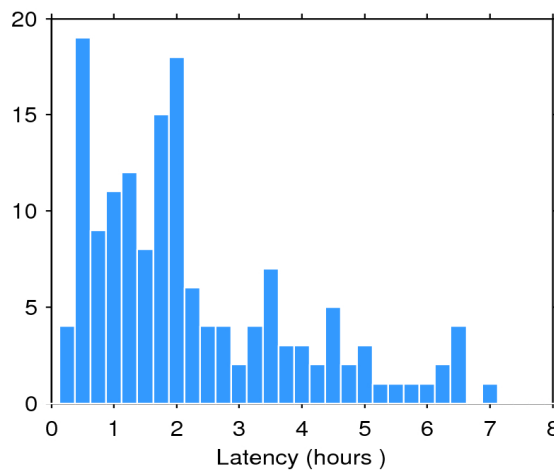
Figure 2. Histogram of the data latency for 22/10/2017. The y-axis denotes the number of files that are made available with a delay of x-hours with respect to the mean time of the records stored in the file.
