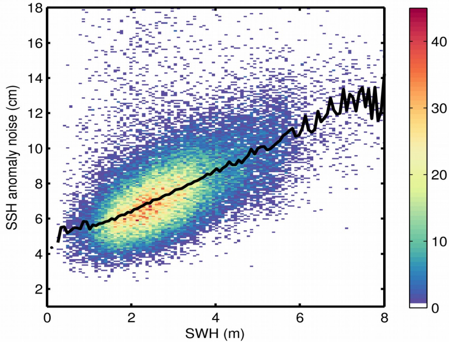
Figure 9. 2D histogram showing flag-valid SSH anomaly noise as a function of SWH for 20/10/2017. The black line denotes the median SSH anomaly noise as a function of SWH.
