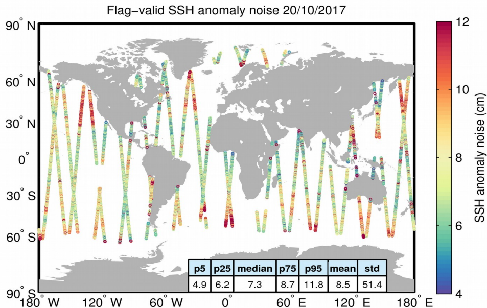
Figure 8. Geographical distribution of flag-valid 20-Hz SSH anomaly measurement noise over oceans and lakes for 20/10/2017. The statistical values shown in the table refer to the SSH anomaly noise and are calculated over all measurements shown in the figure.
