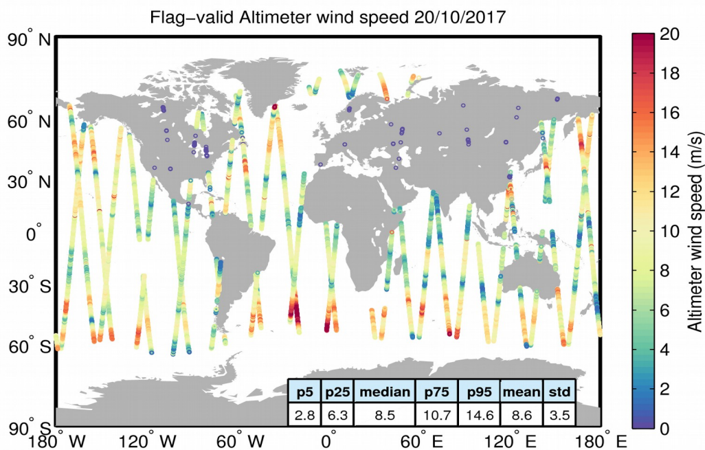
Figure 31. Geographical distribution of flag-valid wind data over oceans and lakes for 20/10/2017. The statistical values shown in the table refer to the wind in m/s and are calculated over all measurements shown in the figure.
