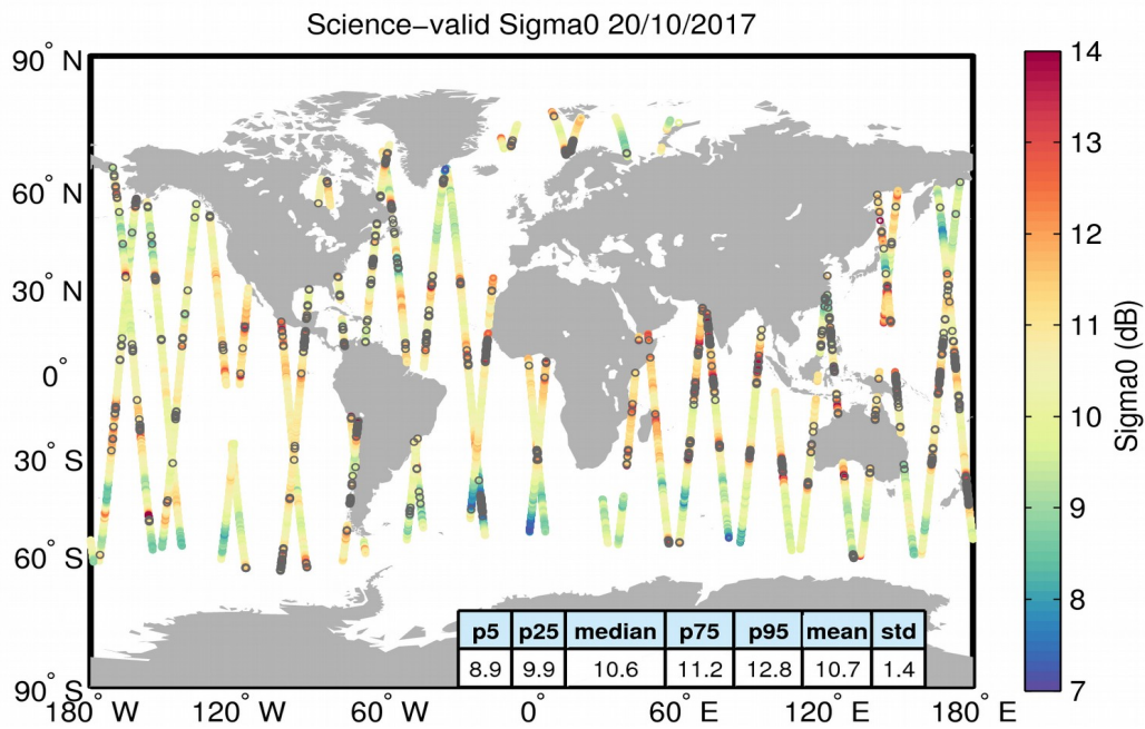
Figure 27. Geographical distribution of science-valid sigma0 data over oceans and lakes for 20/10/2017. The statistical values shown in the table refer to the sigma0 in dB and are calculated over all measurements shown in the figure. Gray circles denote records that have been rejected based on the editing criteria described in Table 4.
