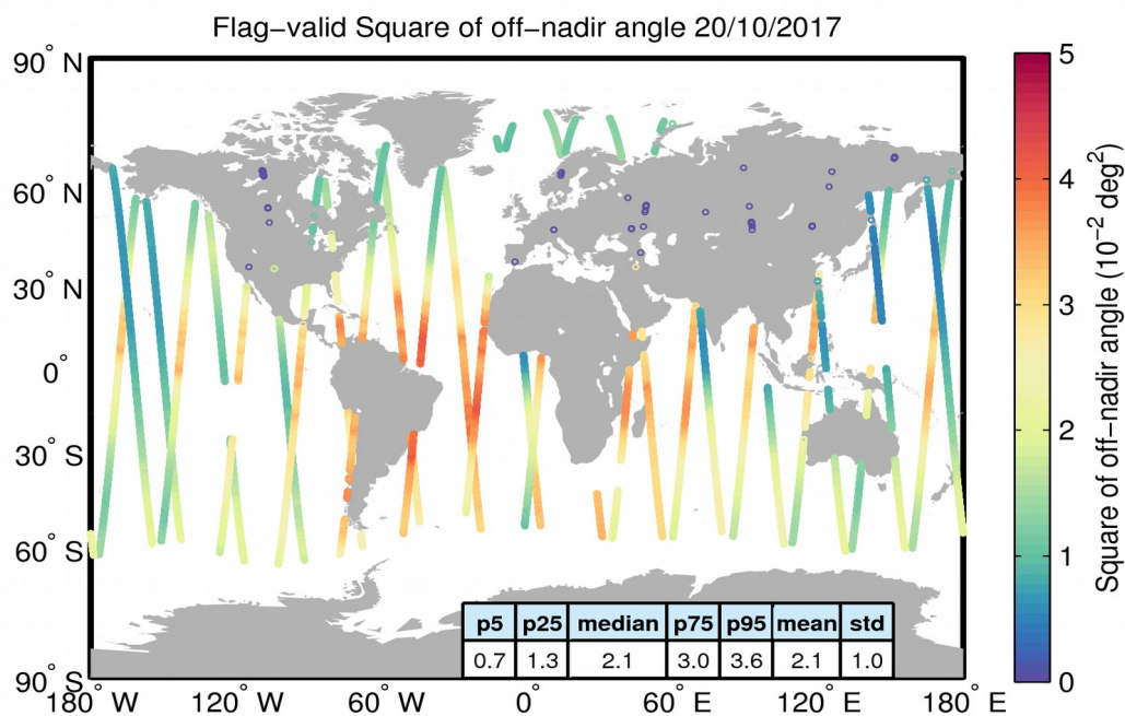
Figure 37. Geographical distribution of flag-valid mispointing data over oceans and lakes for 20/10/2017. The statistical values shown in the table refer to the mispointing in 10^{-2} deg 2 and are calculated over all measurements shown in the figure.
