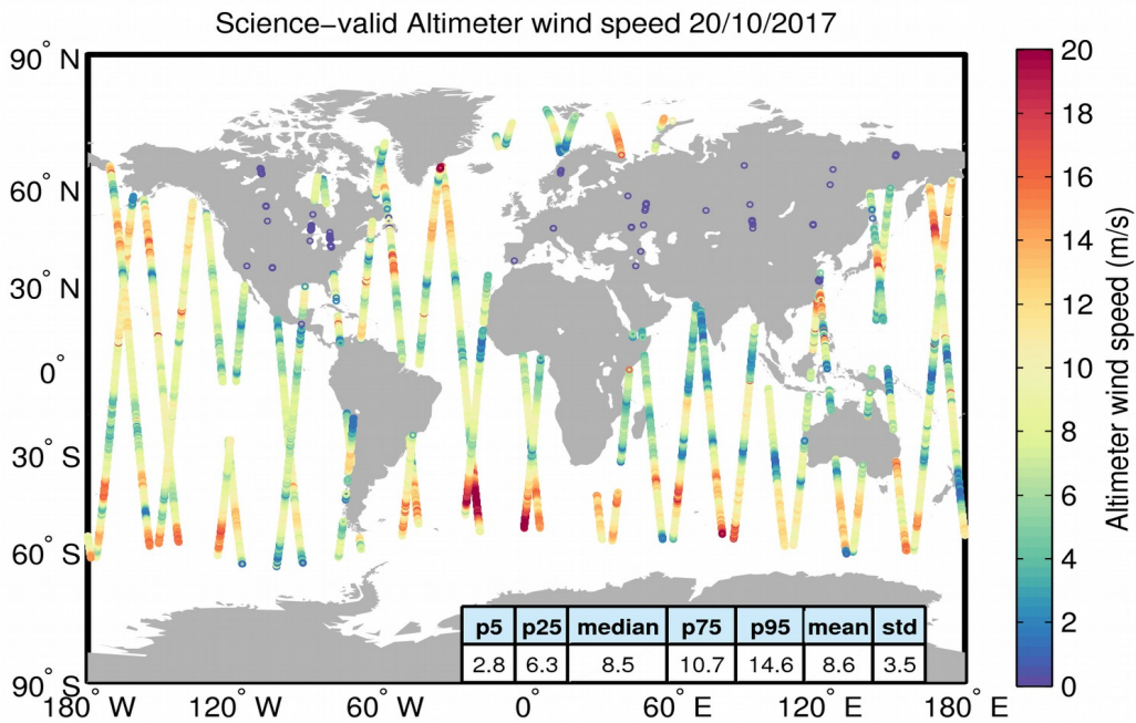
Figure 34. Geographical distribution of science-valid wind data over oceans and lakes for 20/10/2017. The statistical values shown in the table refer to the wind in m/s and are calculated over all measurements shown in the figure. Gray circles denote records that have been rejected based on the editing criteria described in Table 5.
