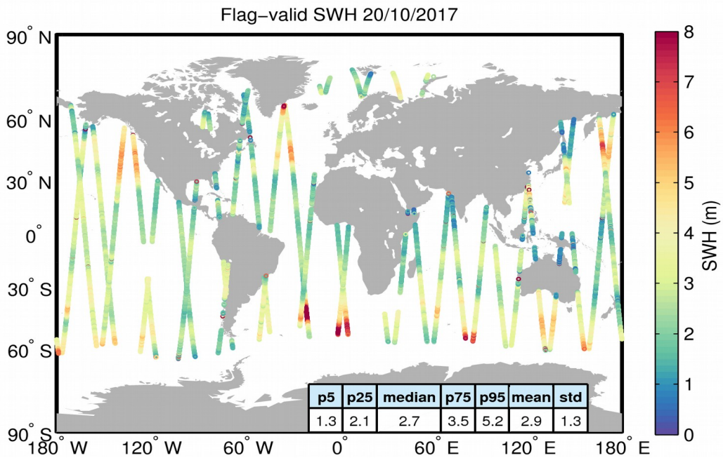
Figure 15. Geographical distribution of flag-valid SWH data over oceans and lakes for 20/10/2017. The statistical values shown in the table refer to the SWH in m and are calculated over all measurements shown in the figure.
