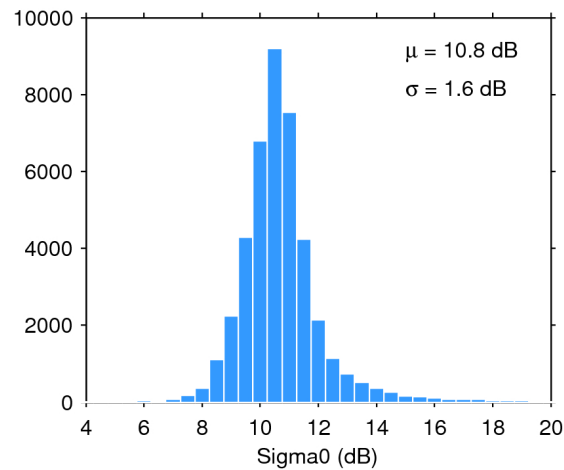
Figure 25. Histogram of flag-valid sigma0 over oceans and lakes for 20/10/2017. The mean ( \mu ) and standard deviation ( \sigma ) are also shown. Note that values outside [4 20] dB are excluded from the histogram for the sake of readability but not from the computation of \mu and \sigma .
