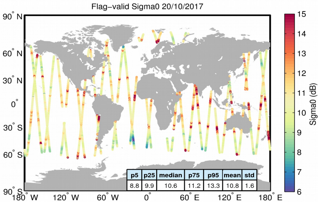
Figure 23. Geographical distribution of flag-valid sigma0 data over oceans and lakes for 20/10/2017. The statistical values shown in the table refer to the sigma0 in dB and are calculated over all measurements shown in the figure.
