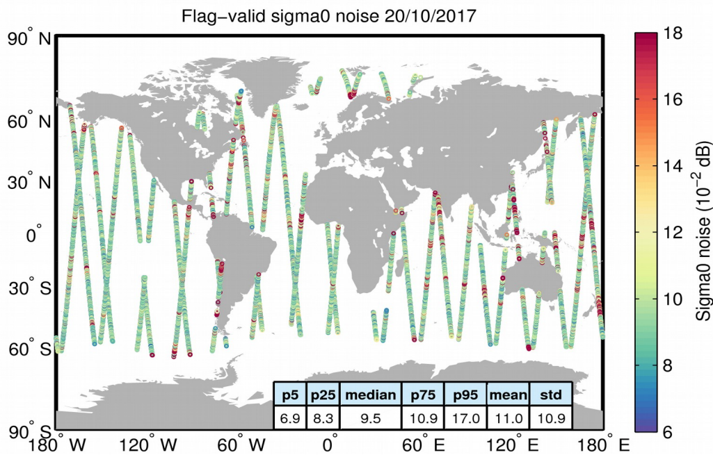
Figure 26. Geographical distribution of flag-valid 20-Hz sigma0 measurement noise over oceans and lakes for 20/10/2017. The statistical values shown in the table refer to the sigma0 noise and are calculated over all measurements shown in the figure.
