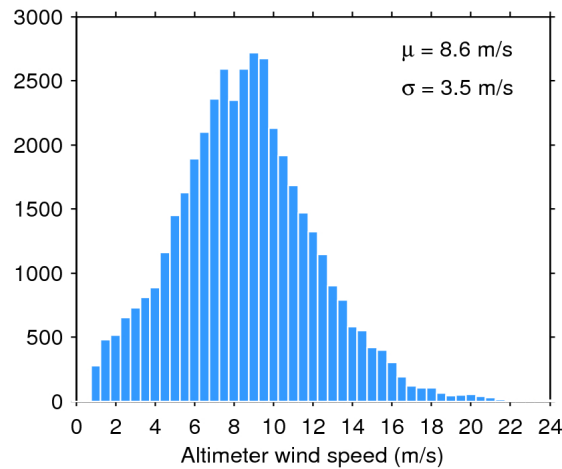
Figure 33. Histogram of flag-valid wind over oceans and lakes for 20/10/2017. The mean ( \mu ) and standard deviation ( \sigma ) are also shown. Note that values larger than 24 m/s are excluded from the histogram for the sake of readability but not from the computation of \mu and \sigma .
