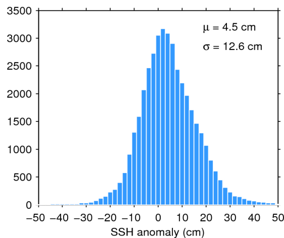
Figure 11. Histogram of science-valid SSH anomaly over oceans and lakes for 20/10/2017. The mean ( \mu ) and standard deviation ( \sigma ) are also shown. Note that values outside [-50 50] cm are excluded from the histogram for the sake of readability but not from the computation of \mu and \sigma .
