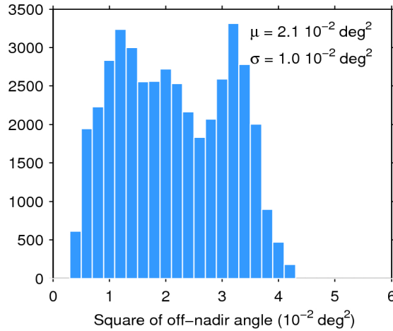
Figure 39. Histogram of flag-valid mispointing over oceans and lakes for 20/10/2017. The mean ( \mu ) and standard deviation ( \sigma ) are also shown. Note that values larger than 6 \cdot 10^{-2} \text{ deg}^2 are excluded from the histogram for the sake of readability but not from the computation of \mu and \sigma .
