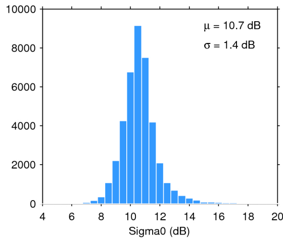
Figure 28. Histogram of science-valid sigma0 over oceans and lakes for 20/10/2017. The mean ( \mu ) and standard deviation ( \sigma ) are also shown. Note that values outside [4 20] dB are excluded from the histogram for the sake of readability but not from the computation of \mu and \sigma .
