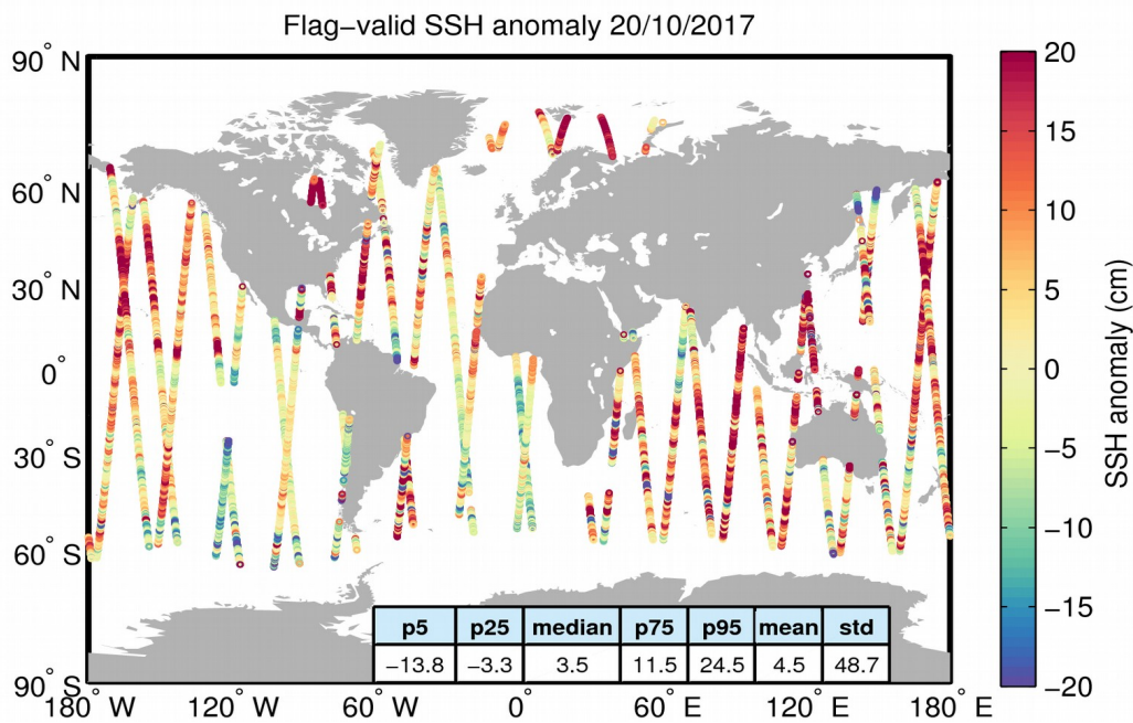
Figure 5. Geographical distribution of flag-valid 1-Hz SSH anomaly data over oceans and lakes for 20/10/2017. The statistical values shown in the table refer to the SSH anomaly in cm and are calculated over all measurements shown in the figure.
