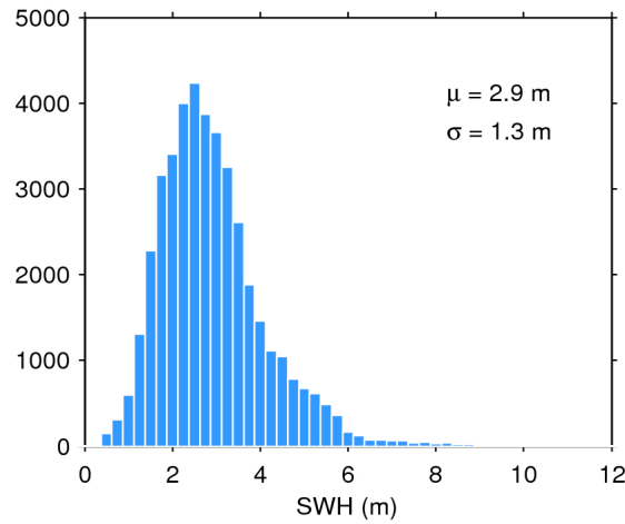
Figure 17. Histogram of flag-valid SWH over oceans and lakes for 20/10/2017. The mean ( \mu ) and standard deviation ( \sigma ) are also shown. Note that values larger than 12 m are excluded from the histogram for the sake of readability but not from the computation of \mu and \sigma .
