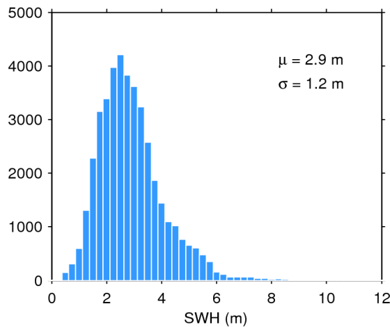
Figure 20. Histogram of science-valid SWH over oceans and lakes for 20/10/2017. The mean ( \mu ) and standard deviation ( \sigma ) are also shown. Note that values larger than 12 m are excluded from the histogram for the sake of readability but not from the computation of \mu and \sigma .
