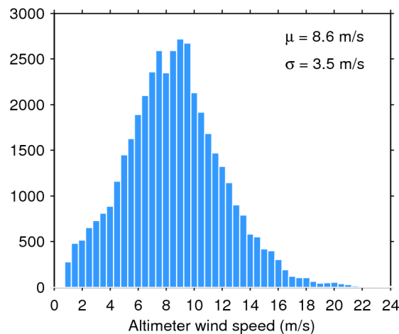
Figure 35. Histogram of science-valid wind over oceans and lakes for 20/10/2017. The mean ( \mu ) and standard deviation ( \sigma ) are also shown. Note that values larger than 24 m/s are excluded from the histogram for the sake of readability but not from the computation of \mu and \sigma .
