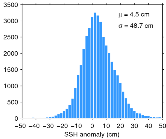
Figure 7. Histogram of flag-valid SSH anomaly over oceans and lakes for 20/10/2017. The mean ( \mu ) and standard deviation ( \sigma ) are also shown. Note that values outside [-50 50] cm are excluded from the histogram for the sake of readability but not from the computation of \mu and \sigma .
