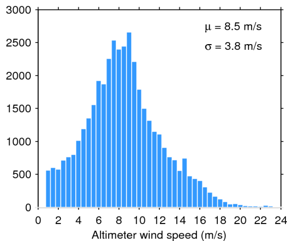
Figure 35. Histogram of science-valid wind over oceans and lakes for 19/10/2017. The mean ( \mu ) and standard deviation ( \sigma ) are also shown. Note that values larger than 24 m/s are excluded from the histogram for the sake of readability but not from the computation of \mu and \sigma .
