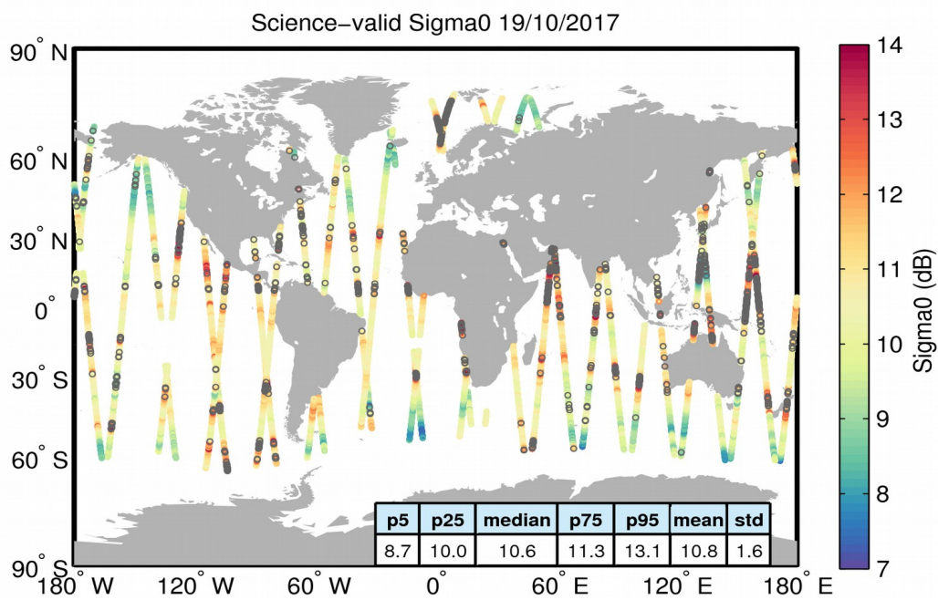
Figure 27. Geographical distribution of science-valid sigma0 data over oceans and lakes for 19/10/2017. The statistical values shown in the table refer to the sigma0 in dB and are calculated over all measurements shown in the figure. Gray circles denote records that have been rejected based on the editing criteria described in Table 4.
