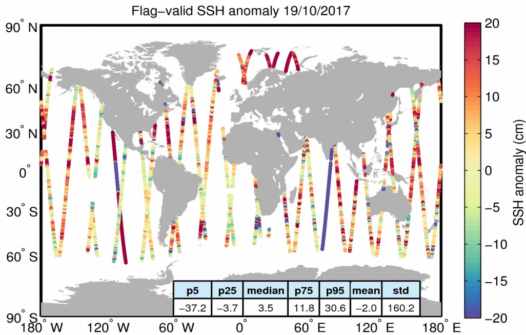
Figure 5. Geographical distribution of flag-valid 1-Hz SSH anomaly data over oceans and lakes for 19/10/2017. The statistical values shown in the table refer to the SSH anomaly in cm and are calculated over all measurements shown in the figure.
