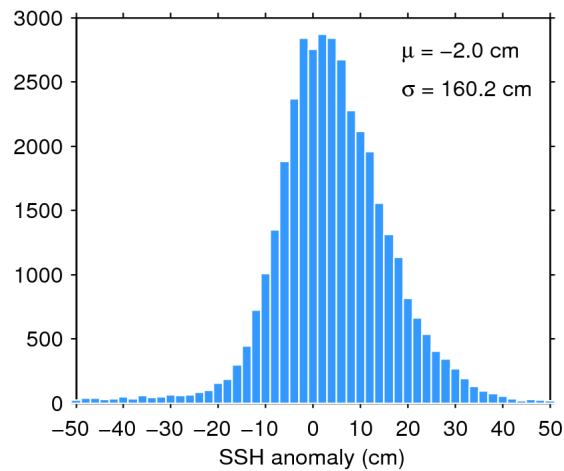
Figure 7. Histogram of flag-valid SSH anomaly over oceans and lakes for 19/10/2017. The mean ( \mu ) and standard deviation ( \sigma ) are also shown. Note that values outside [-50 50] cm are excluded from the histogram for the sake of readability but not from the computation of \mu and \sigma .
