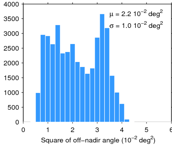
Figure 39. Histogram of flag-valid mispointing over oceans and lakes for 19/10/2017. The mean ( \mu ) and standard deviation ( \sigma ) are also shown. Note that values larger than 6 \cdot 10^{-2} \text{ deg}^2 are excluded from the histogram for the sake of readability but not from the computation of \mu and \sigma .
