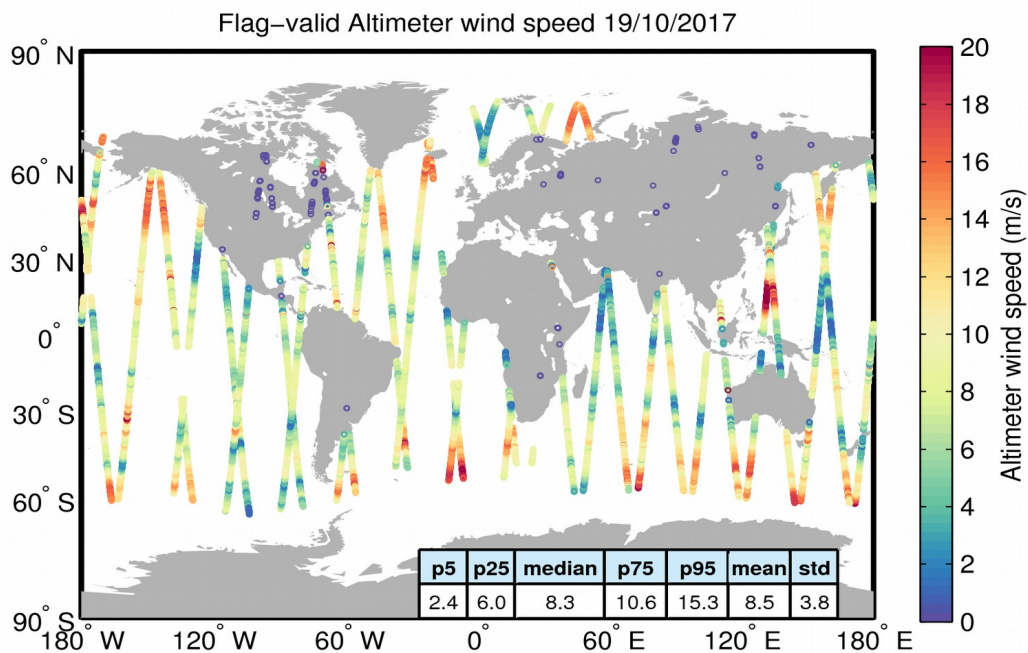
Figure 31. Geographical distribution of flag-valid wind data over oceans and lakes for 19/10/2017. The statistical values shown in the table refer to the wind in m/s and are calculated over all measurements shown in the figure.
