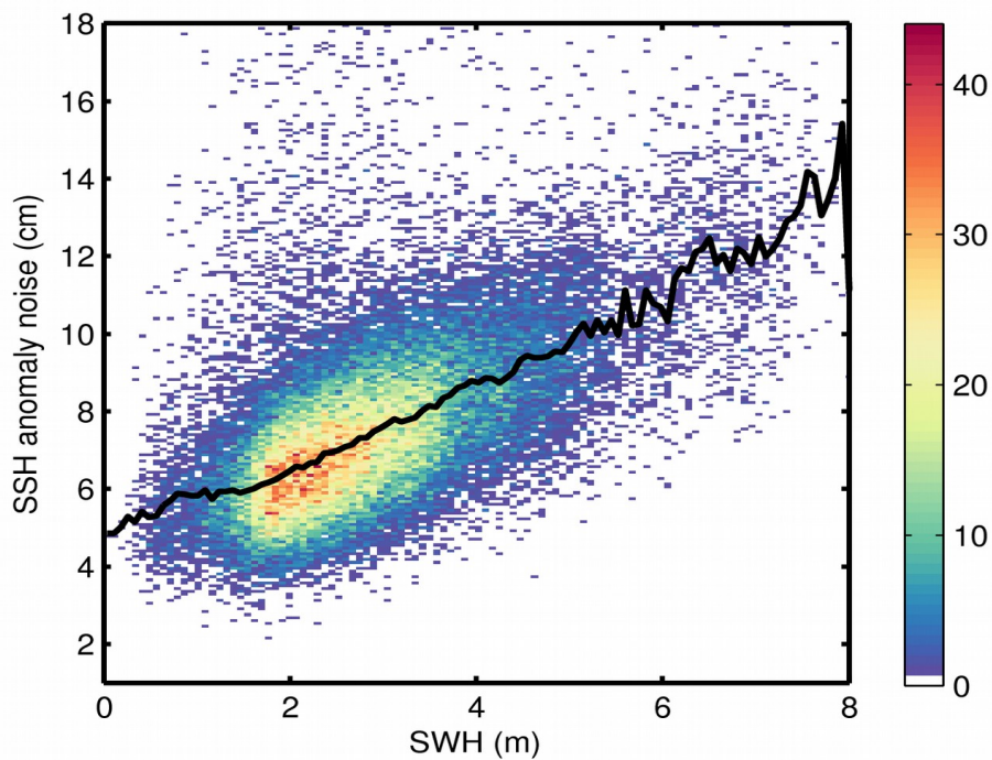
Figure 9. 2D histogram showing flag-valid SSH anomaly noise as a function of SWH for 19/10/2017. The black line denotes the median SSH anomaly noise as a function of SWH.
