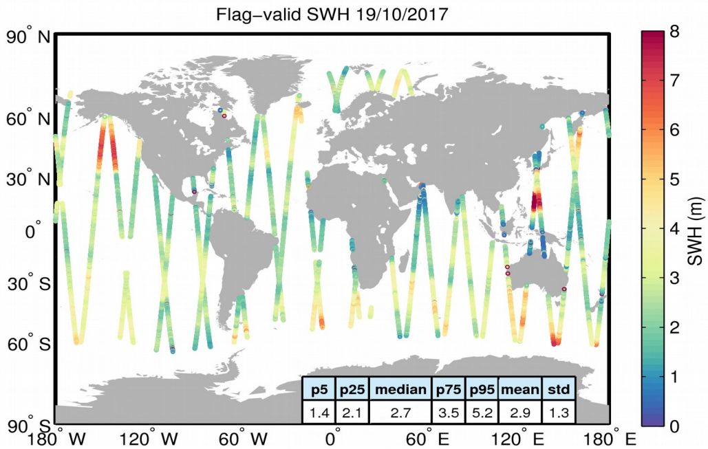
Figure 15. Geographical distribution of flag-valid SWH data over oceans and lakes for 19/10/2017. The statistical values shown in the table refer to the SWH in m and are calculated over all measurements shown in the figure.
