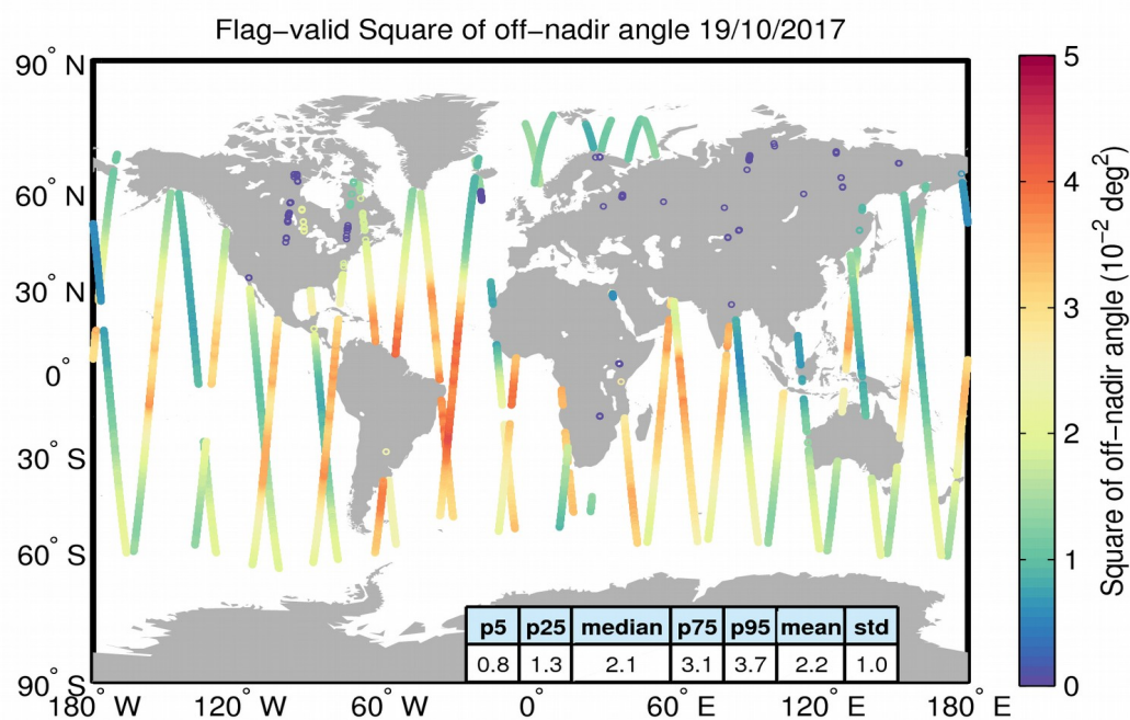
Figure 37. Geographical distribution of flag-valid mispointing data over oceans and lakes for 19/10/2017. The statistical values shown in the table refer to the mispointing in 10^{-2} deg 2 and are calculated over all measurements shown in the figure.
