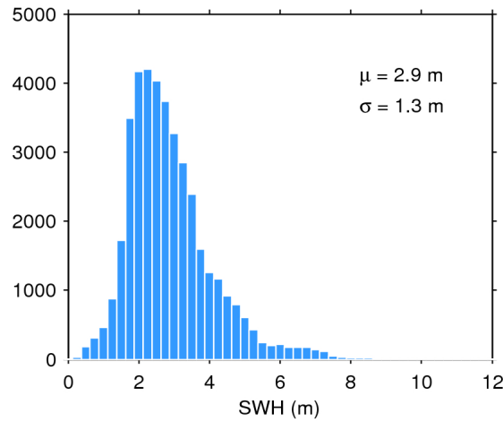
Figure 17. Histogram of flag-valid SWH over oceans and lakes for 19/10/2017. The mean ( \mu ) and standard deviation ( \sigma ) are also shown. Note that values larger than 12 m are excluded from the histogram for the sake of readability but not from the computation of \mu and \sigma .
