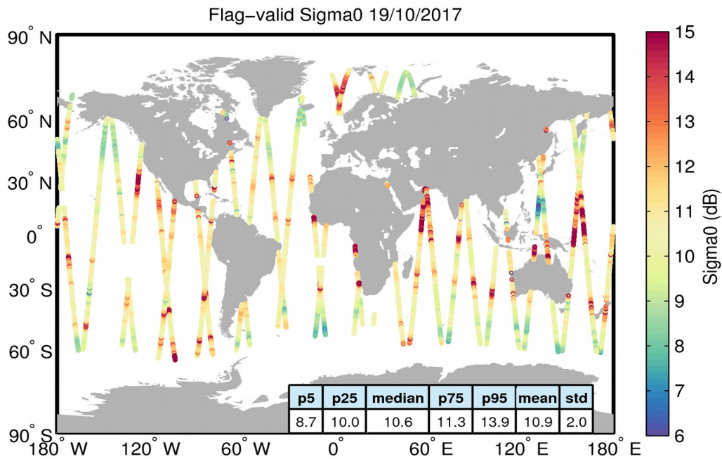
Figure 23. Geographical distribution of flag-valid sigma0 data over oceans and lakes for 19/10/2017. The statistical values shown in the table refer to the sigma0 in dB and are calculated over all measurements shown in the figure.
