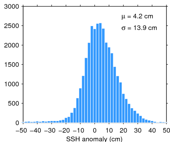
Figure 11. Histogram of science-valid SSH anomaly over oceans and lakes for 19/10/2017. The mean ( \mu ) and standard deviation ( \sigma ) are also shown. Note that values outside [-50 50] cm are excluded from the histogram for the sake of readability but not from the computation of \mu and \sigma .
