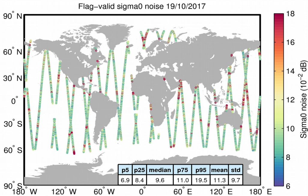
Figure 26. Geographical distribution of flag-valid 20-Hz sigma0 measurement noise over oceans and lakes for 19/10/2017. The statistical values shown in the table refer to the sigma0 noise and are calculated over all measurements shown in the figure.
