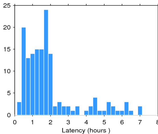
Figure 2. Histogram of the data latency for 19/10/2017. The y-axis denotes the number of files that are made available with a delay of x-hours with respect to the mean time of the records stored in the file.
