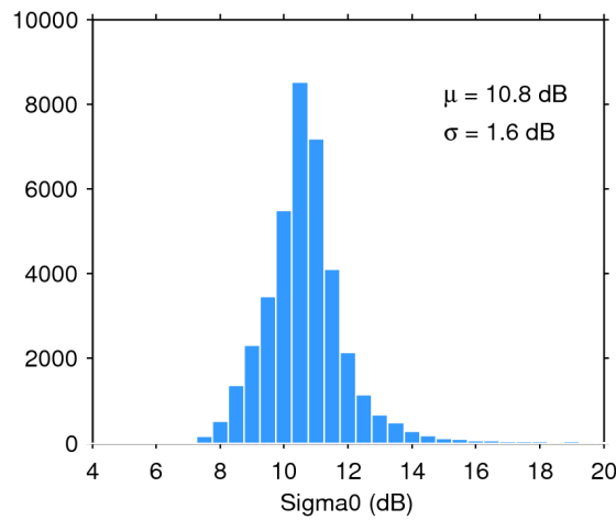
Figure 28. Histogram of science-valid sigma0 over oceans and lakes for 19/10/2017. The mean ( \mu ) and standard deviation ( \sigma ) are also shown. Note that values outside [4 20] dB are excluded from the histogram for the sake of readability but not from the computation of \mu and \sigma .
