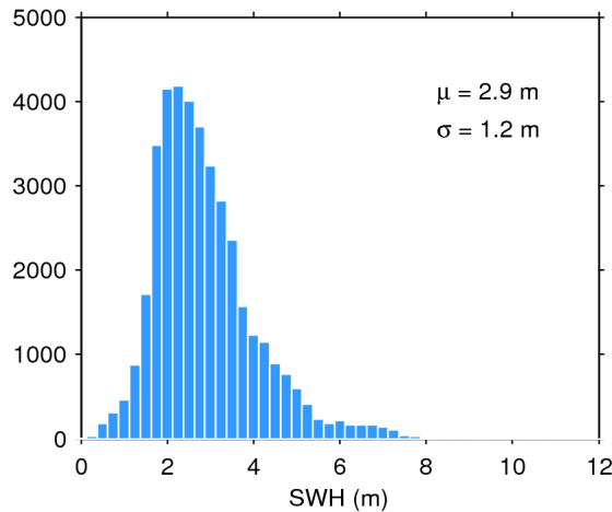
Figure 20. Histogram of science-valid SWH over oceans and lakes for 19/10/2017. The mean ( \mu ) and standard deviation ( \sigma ) are also shown. Note that values larger than 12 m are excluded from the histogram for the sake of readability but not from the computation of \mu and \sigma .
