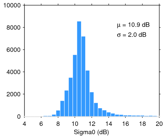
Figure 25. Histogram of flag-valid sigma0 over oceans and lakes for 19/10/2017. The mean ( \mu ) and standard deviation ( \sigma ) are also shown. Note that values outside [4 20] dB are excluded from the histogram for the sake of readability but not from the computation of \mu and \sigma .
