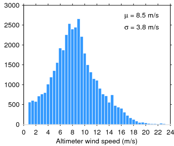
Figure 33. Histogram of flag-valid wind over oceans and lakes for 19/10/2017. The mean ( \mu ) and standard deviation ( \sigma ) are also shown. Note that values larger than 24 m/s are excluded from the histogram for the sake of readability but not from the computation of \mu and \sigma .
