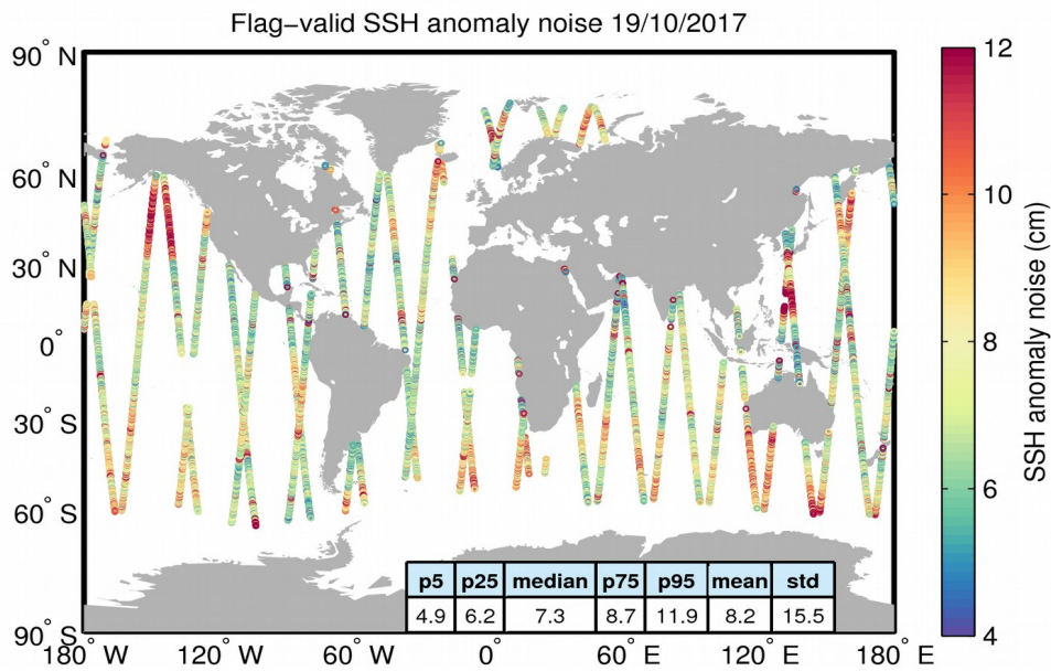
Figure 8. Geographical distribution of flag-valid 20-Hz SSH anomaly measurement noise over oceans and lakes for 19/10/2017. The statistical values shown in the table refer to the SSH anomaly noise and are calculated over all measurements shown in the figure.
