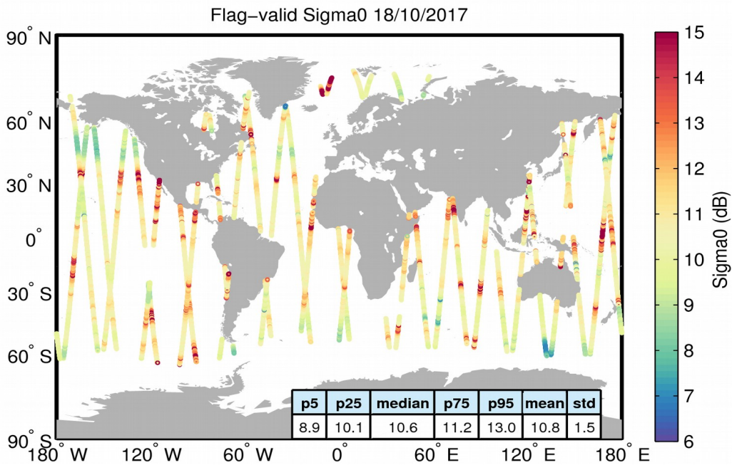
Figure 23. Geographical distribution of flag-valid sigma0 data over oceans and lakes for 18/10/2017. The statistical values shown in the table refer to the sigma0 in dB and are calculated over all measurements shown in the figure.
