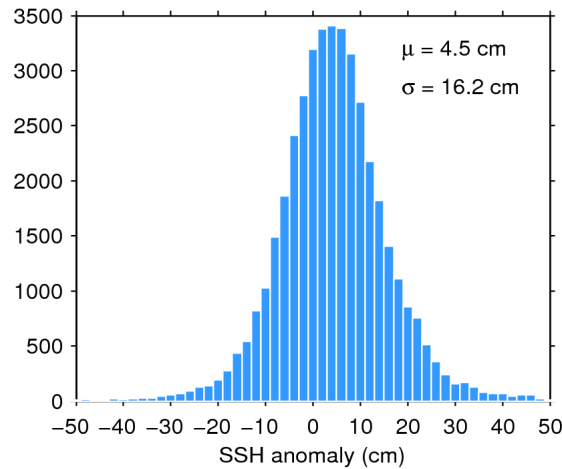
Figure 7. Histogram of flag-valid SSH anomaly over oceans and lakes for 18/10/2017. The mean ( \mu ) and standard deviation ( \sigma ) are also shown. Note that values outside [-50 50] cm are excluded from the histogram for the sake of readability but not from the computation of \mu and \sigma .
