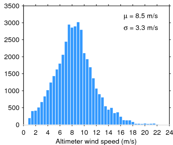
Figure 35. Histogram of science-valid wind over oceans and lakes for 18/10/2017. The mean ( \mu ) and standard deviation ( \sigma ) are also shown. Note that values larger than 24 m/s are excluded from the histogram for the sake of readability but not from the computation of \mu and \sigma .
