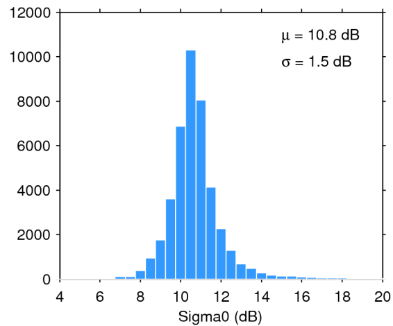
Figure 25. Histogram of flag-valid sigma0 over oceans and lakes for 18/10/2017. The mean ( \mu ) and standard deviation ( \sigma ) are also shown. Note that values outside [4 20] dB are excluded from the histogram for the sake of readability but not from the computation of \mu and \sigma .
