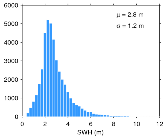
Figure 20. Histogram of science-valid SWH over oceans and lakes for 18/10/2017. The mean ( \mu ) and standard deviation ( \sigma ) are also shown. Note that values larger than 12 m are excluded from the histogram for the sake of readability but not from the computation of \mu and \sigma .
