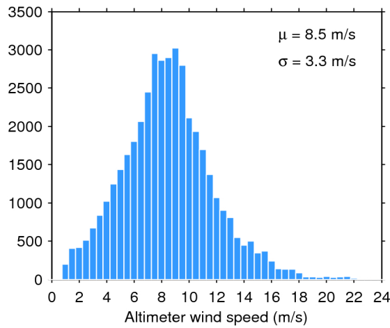
Figure 33. Histogram of flag-valid wind over oceans and lakes for 18/10/2017. The mean ( \mu ) and standard deviation ( \sigma ) are also shown. Note that values larger than 24 m/s are excluded from the histogram for the sake of readability but not from the computation of \mu and \sigma .
