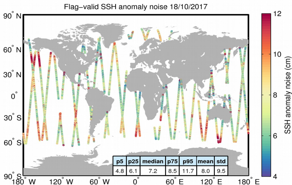
Figure 8. Geographical distribution of flag-valid 20-Hz SSH anomaly measurement noise over oceans and lakes for 18/10/2017. The statistical values shown in the table refer to the SSH anomaly noise and are calculated over all measurements shown in the figure.
