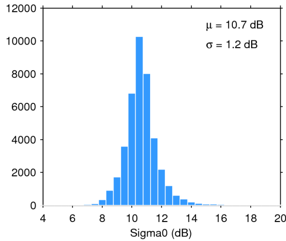
Figure 28. Histogram of science-valid sigma0 over oceans and lakes for 18/10/2017. The mean ( \mu ) and standard deviation ( \sigma ) are also shown. Note that values outside [4 20] dB are excluded from the histogram for the sake of readability but not from the computation of \mu and \sigma .
