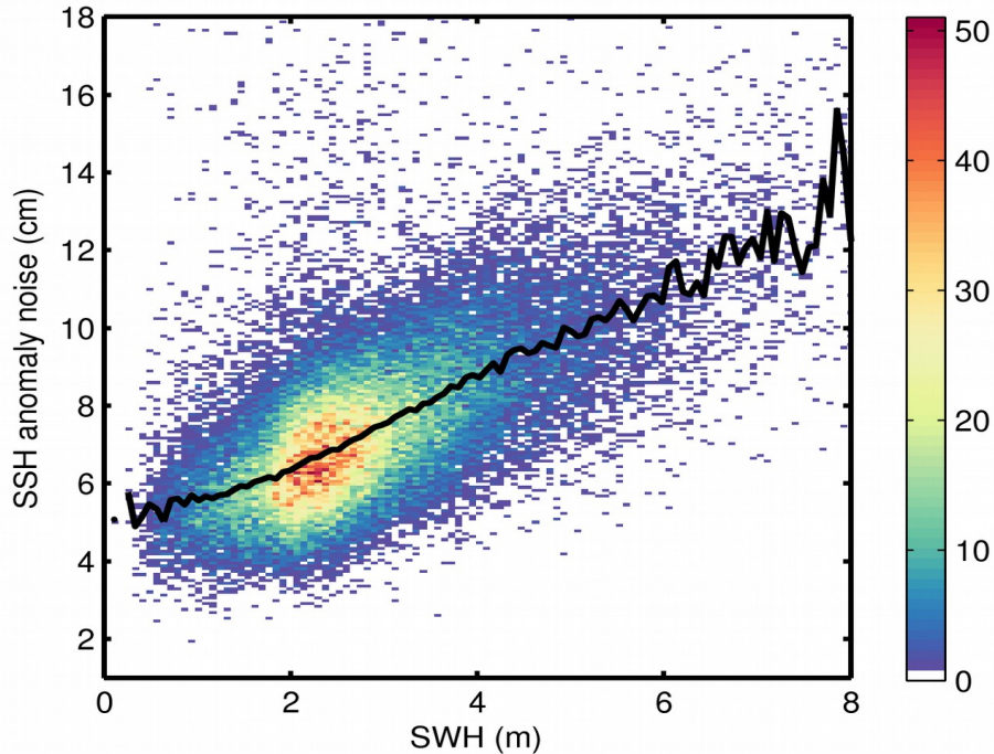
Figure 9. 2D histogram showing flag-valid SSH anomaly noise as a function of SWH for 18/10/2017. The black line denotes the median SSH anomaly noise as a function of SWH.
