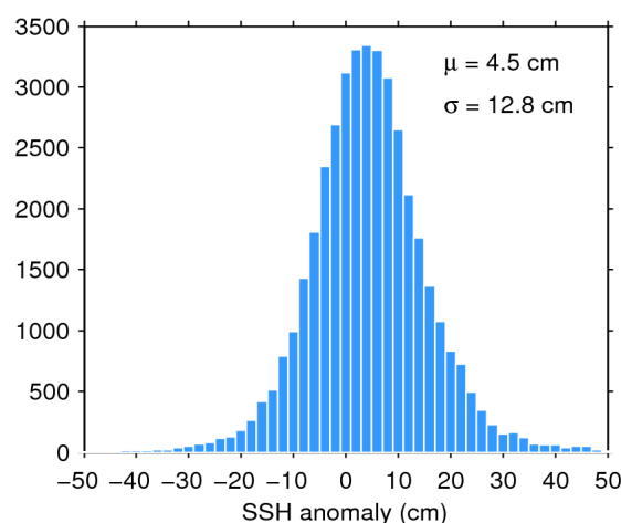
Figure 11. Histogram of science-valid SSH anomaly over oceans and lakes for 18/10/2017. The mean ( \mu ) and standard deviation ( \sigma ) are also shown. Note that values outside [-50 50] cm are excluded from the histogram for the sake of readability but not from the computation of \mu and \sigma .
