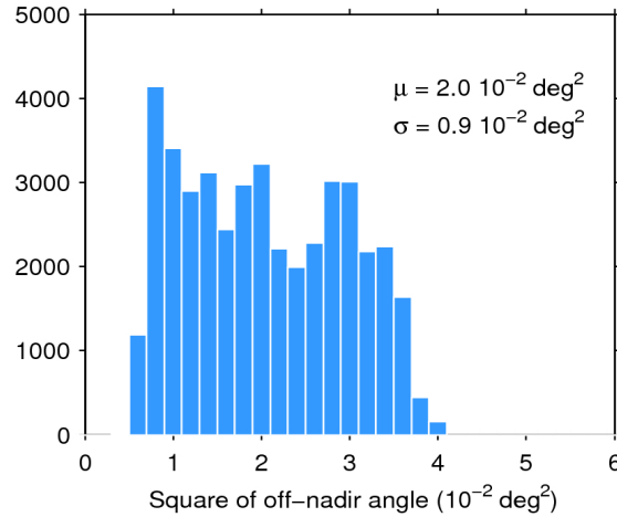
Figure 39. Histogram of flag-valid mispointing over oceans and lakes for 18/10/2017. The mean ( \mu ) and standard deviation ( \sigma ) are also shown. Note that values larger than 6 \cdot 10^{-2} \text{ deg}^2 are excluded from the histogram for the sake of readability but not from the computation of \mu and \sigma .
