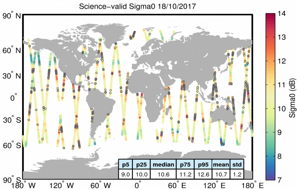
Figure 27. Geographical distribution of science-valid sigma0 data over oceans and lakes for 18/10/2017. The statistical values shown in the table refer to the sigma0 in dB and are calculated over all measurements shown in the figure. Gray circles denote records that have been rejected based on the editing criteria described in Table 4.
