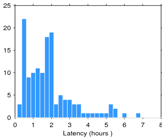
Figure 2. Histogram of the data latency for 18/10/2017. The y-axis denotes the number of files that are made available with a delay of x-hours with respect to the mean time of the records stored in the file.
