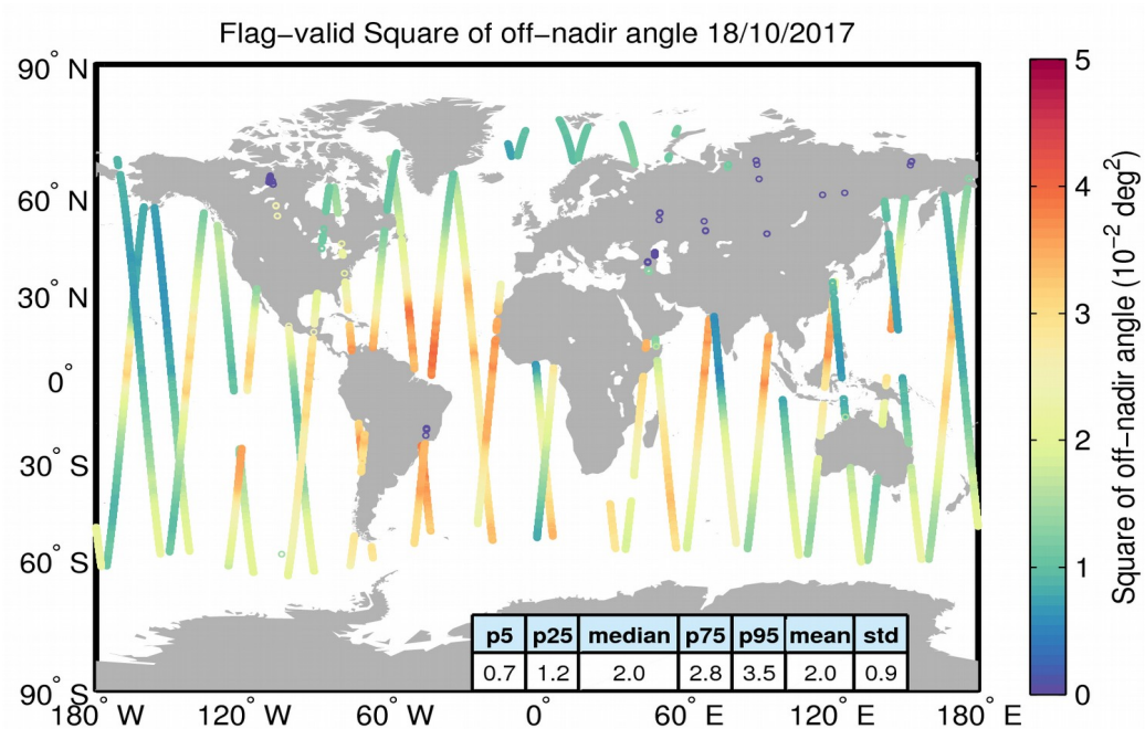
Figure 37. Geographical distribution of flag-valid mispointing data over oceans and lakes for 18/10/2017. The statistical values shown in the table refer to the mispointing in 10^{-2} deg 2 and are calculated over all measurements shown in the figure.
