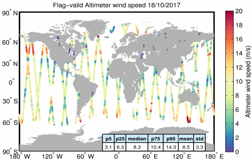
Figure 31. Geographical distribution of flag-valid wind data over oceans and lakes for 18/10/2017. The statistical values shown in the table refer to the wind in m/s and are calculated over all measurements shown in the figure.
