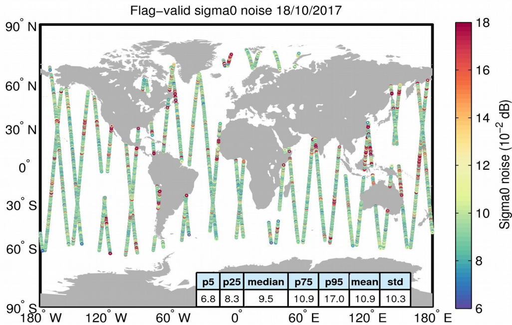
Figure 26. Geographical distribution of flag-valid 20-Hz sigma0 measurement noise over oceans and lakes for 18/10/2017. The statistical values shown in the table refer to the sigma0 noise and are calculated over all measurements shown in the figure.
