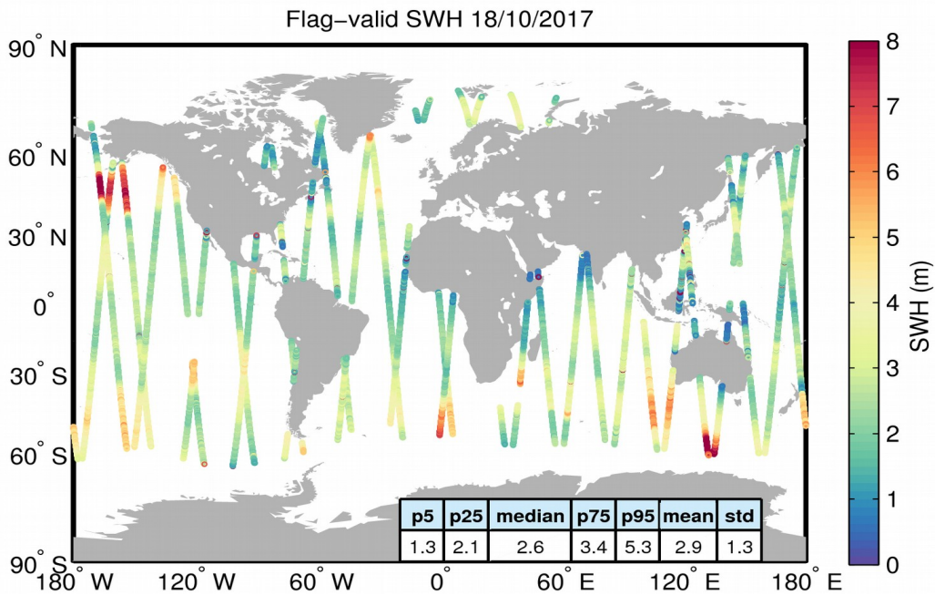
Figure 15. Geographical distribution of flag-valid SWH data over oceans and lakes for 18/10/2017. The statistical values shown in the table refer to the SWH in m and are calculated over all measurements shown in the figure.
