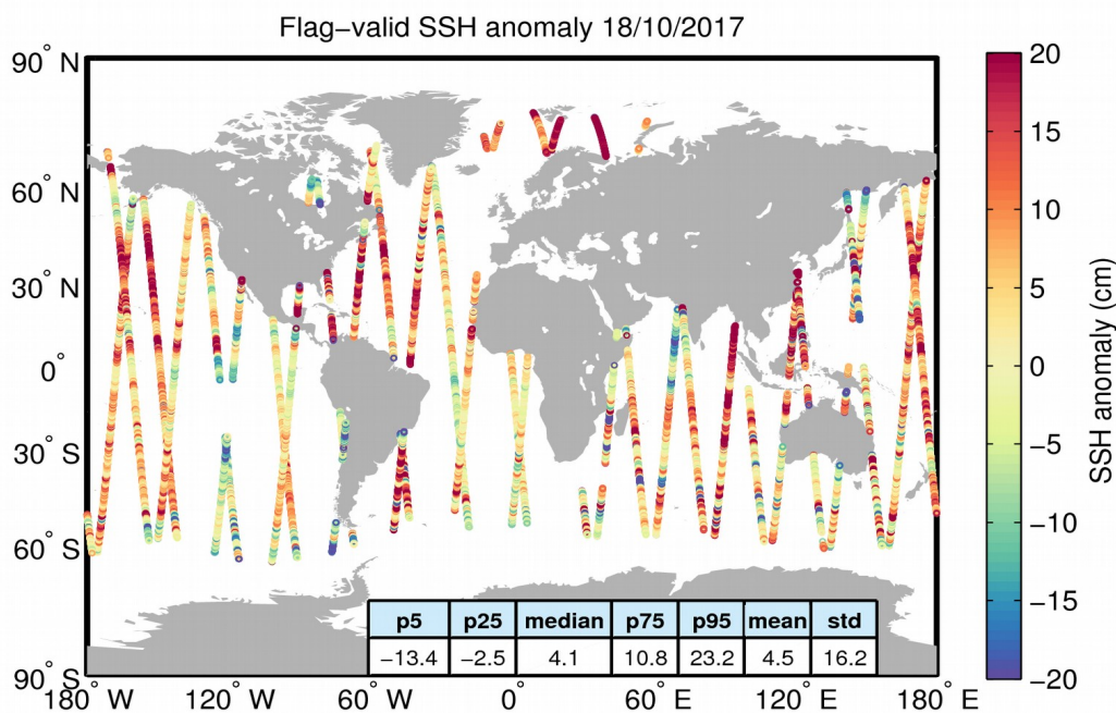
Figure 5. Geographical distribution of flag-valid 1-Hz SSH anomaly data over oceans and lakes for 18/10/2017. The statistical values shown in the table refer to the SSH anomaly in cm and are calculated over all measurements shown in the figure.
