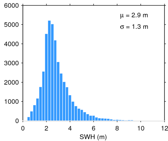
Figure 17. Histogram of flag-valid SWH over oceans and lakes for 18/10/2017. The mean ( \mu ) and standard deviation ( \sigma ) are also shown. Note that values larger than 12 m are excluded from the histogram for the sake of readability but not from the computation of \mu and \sigma .
