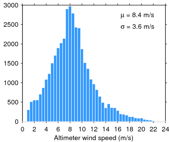
Figure 33. Histogram of flag-valid wind over oceans and lakes for 17/10/2017. The mean ( \mu ) and standard deviation ( \sigma ) are also shown. Note that values larger than 24 m/s are excluded from the histogram for the sake of readability but not from the computation of \mu and \sigma .
