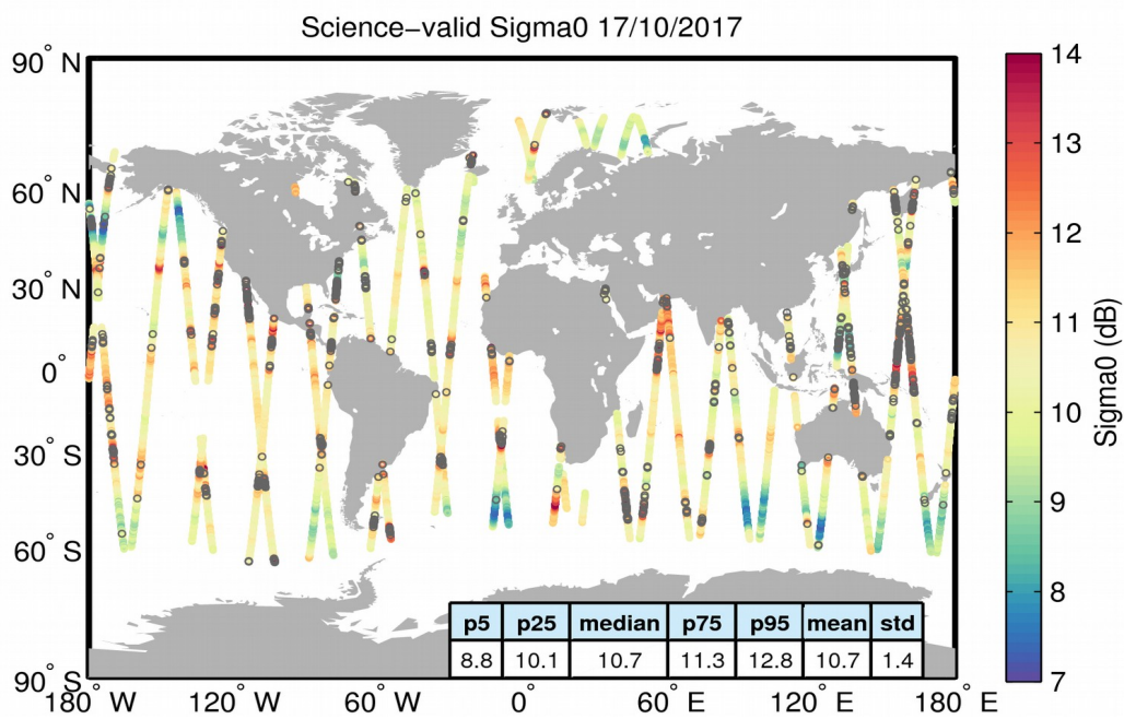
Figure 27. Geographical distribution of science-valid sigma0 data over oceans and lakes for 17/10/2017. The statistical values shown in the table refer to the sigma0 in dB and are calculated over all measurements shown in the figure. Gray circles denote records that have been rejected based on the editing criteria described in Table 4.
