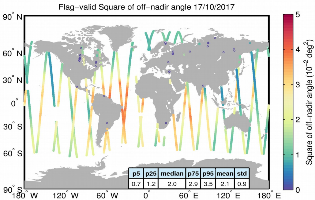
Figure 37. Geographical distribution of flag-valid mispointing data over oceans and lakes for 17/10/2017. The statistical values shown in the table refer to the mispointing in 10^{-2} deg 2 and are calculated over all measurements shown in the figure.
