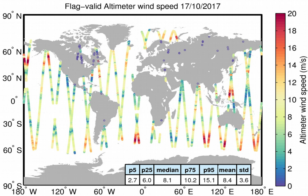
Figure 31. Geographical distribution of flag-valid wind data over oceans and lakes for 17/10/2017. The statistical values shown in the table refer to the wind in m/s and are calculated over all measurements shown in the figure.
