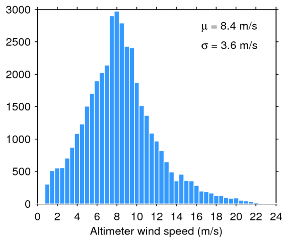
Figure 35. Histogram of science-valid wind over oceans and lakes for 17/10/2017. The mean ( \mu ) and standard deviation ( \sigma ) are also shown. Note that values larger than 24 m/s are excluded from the histogram for the sake of readability but not from the computation of \mu and \sigma .
