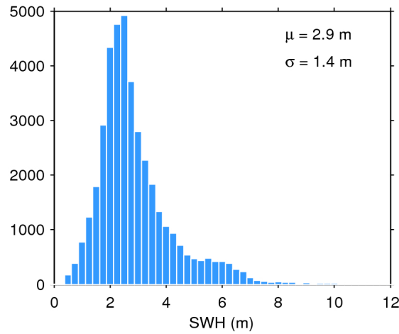
Figure 17. Histogram of flag-valid SWH over oceans and lakes for 17/10/2017. The mean ( \mu ) and standard deviation ( \sigma ) are also shown. Note that values larger than 12 m are excluded from the histogram for the sake of readability but not from the computation of \mu and \sigma .
