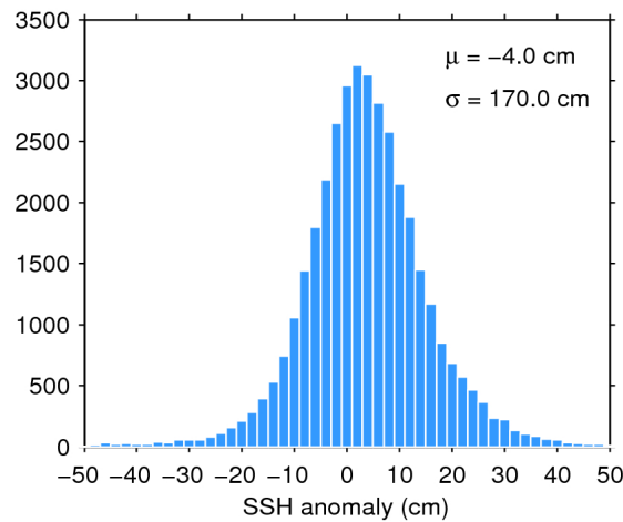
Figure 7. Histogram of flag-valid SSH anomaly over oceans and lakes for 17/10/2017. The mean ( \mu ) and standard deviation ( \sigma ) are also shown. Note that values outside [-50 50] cm are excluded from the histogram for the sake of readability but not from the computation of \mu and \sigma .
