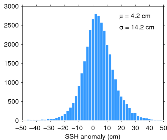
Figure 11. Histogram of science-valid SSH anomaly over oceans and lakes for 17/10/2017. The mean ( \mu ) and standard deviation ( \sigma ) are also shown. Note that values outside [-50 50] cm are excluded from the histogram for the sake of readability but not from the computation of \mu and \sigma .
