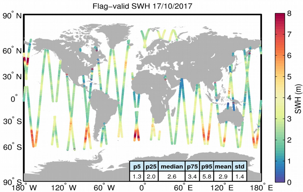
Figure 15. Geographical distribution of flag-valid SWH data over oceans and lakes for 17/10/2017. The statistical values shown in the table refer to the SWH in m and are calculated over all measurements shown in the figure.
