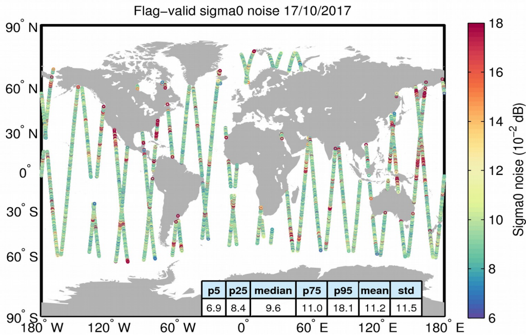
Figure 26. Geographical distribution of flag-valid 20-Hz sigma0 measurement noise over oceans and lakes for 17/10/2017. The statistical values shown in the table refer to the sigma0 noise and are calculated over all measurements shown in the figure.
