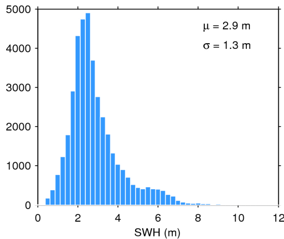
Figure 20. Histogram of science-valid SWH over oceans and lakes for 17/10/2017. The mean ( \mu ) and standard deviation ( \sigma ) are also shown. Note that values larger than 12 m are excluded from the histogram for the sake of readability but not from the computation of \mu and \sigma .
