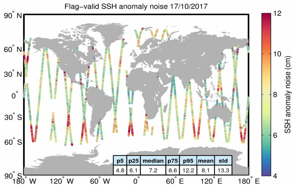
Figure 8. Geographical distribution of flag-valid 20-Hz SSH anomaly measurement noise over oceans and lakes for 17/10/2017. The statistical values shown in the table refer to the SSH anomaly noise and are calculated over all measurements shown in the figure.
