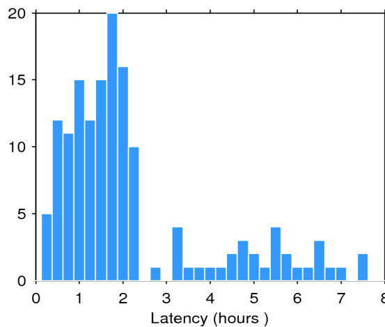
Figure 2. Histogram of the data latency for 17/10/2017. The y-axis denotes the number of files that are made available with a delay of x-hours with respect to the mean time of the records stored in the file.
