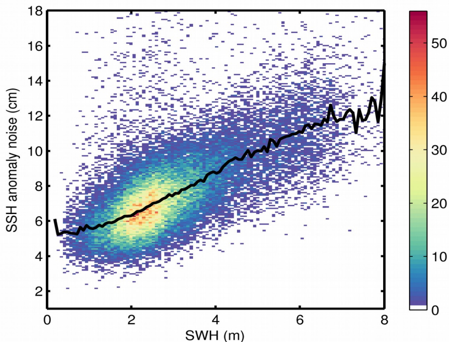
Figure 9. 2D histogram showing flag-valid SSH anomaly noise as a function of SWH for 17/10/2017. The black line denotes the median SSH anomaly noise as a function of SWH.
