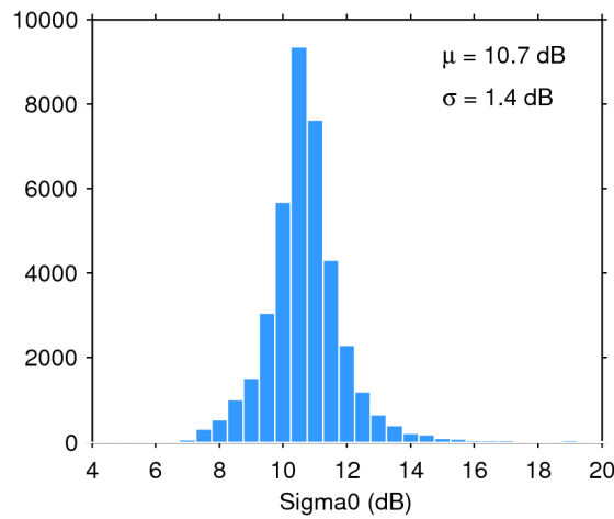
Figure 28. Histogram of science-valid sigma0 over oceans and lakes for 17/10/2017. The mean ( \mu ) and standard deviation ( \sigma ) are also shown. Note that values outside [4 20] dB are excluded from the histogram for the sake of readability but not from the computation of \mu and \sigma .
