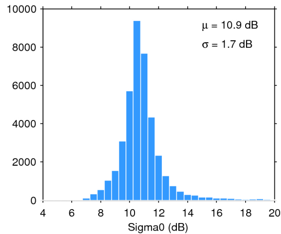
Figure 25. Histogram of flag-valid sigma0 over oceans and lakes for 17/10/2017. The mean ( \mu ) and standard deviation ( \sigma ) are also shown. Note that values outside [4 20] dB are excluded from the histogram for the sake of readability but not from the computation of \mu and \sigma .
