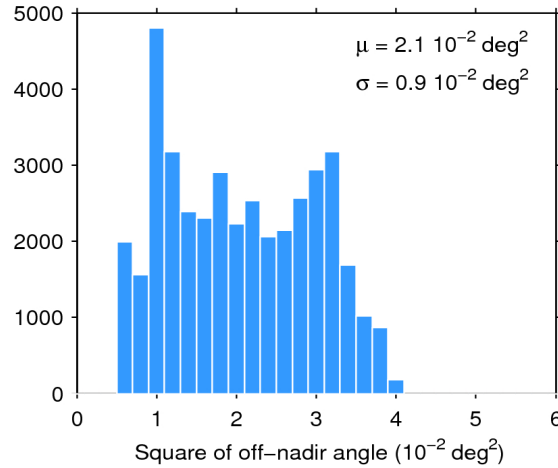
Figure 39. Histogram of flag-valid mispointing over oceans and lakes for 17/10/2017. The mean ( \mu ) and standard deviation ( \sigma ) are also shown. Note that values larger than 6 \cdot 10^{-2} \text{ deg}^2 are excluded from the histogram for the sake of readability but not from the computation of \mu and \sigma .
