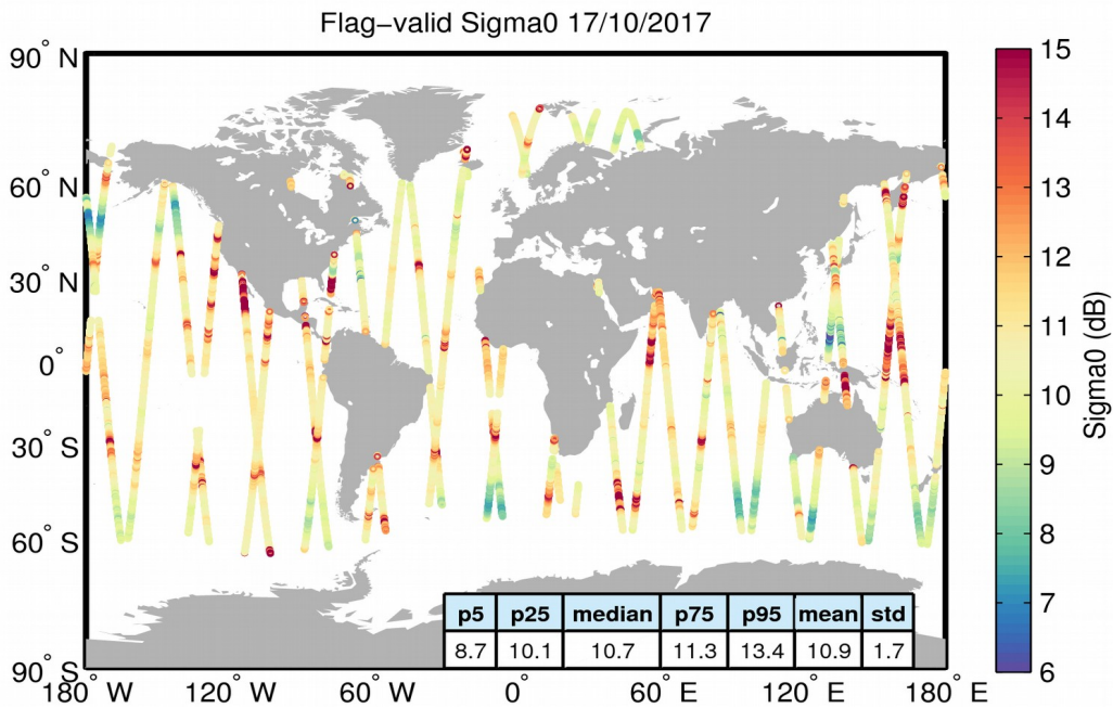
Figure 23. Geographical distribution of flag-valid sigma0 data over oceans and lakes for 17/10/2017. The statistical values shown in the table refer to the sigma0 in dB and are calculated over all measurements shown in the figure.
