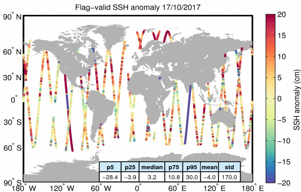
Figure 5. Geographical distribution of flag-valid 1-Hz SSH anomaly data over oceans and lakes for 17/10/2017. The statistical values shown in the table refer to the SSH anomaly in cm and are calculated over all measurements shown in the figure.
