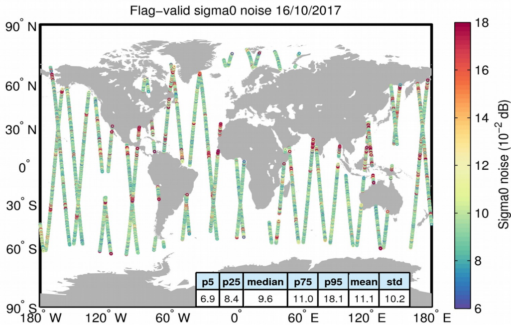
Figure 26. Geographical distribution of flag-valid 20-Hz sigma0 measurement noise over oceans and lakes for 16/10/2017. The statistical values shown in the table refer to the sigma0 noise and are calculated over all measurements shown in the figure.
