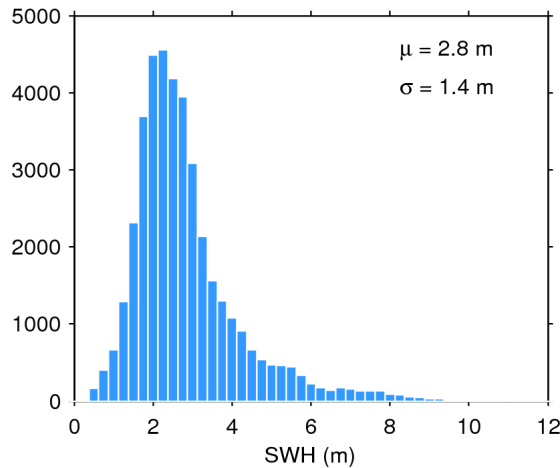
Figure 20. Histogram of science-valid SWH over oceans and lakes for 16/10/2017. The mean ( \mu ) and standard deviation ( \sigma ) are also shown. Note that values larger than 12 m are excluded from the histogram for the sake of readability but not from the computation of \mu and \sigma .
