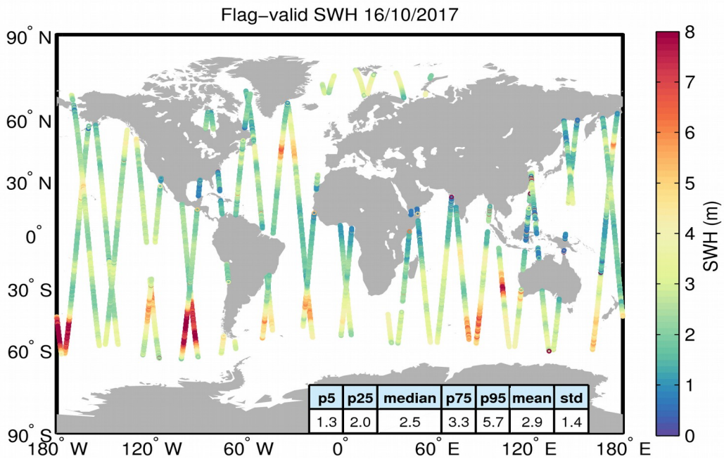
Figure 15. Geographical distribution of flag-valid SWH data over oceans and lakes for 16/10/2017. The statistical values shown in the table refer to the SWH in m and are calculated over all measurements shown in the figure.
