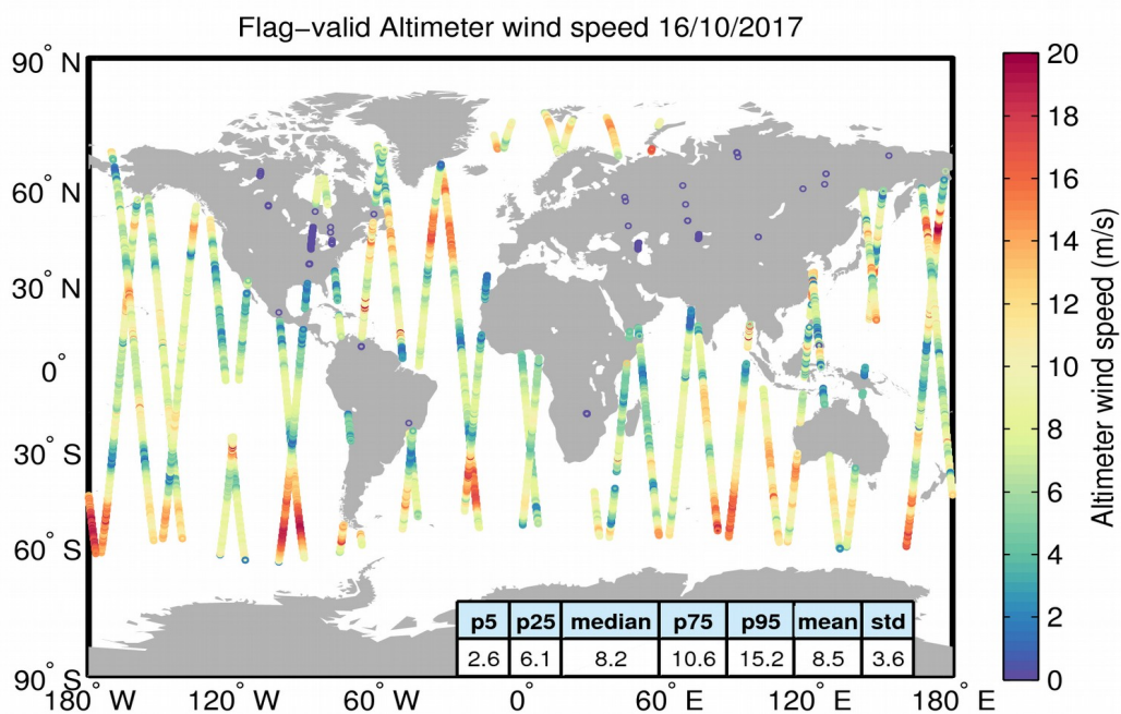
Figure 31. Geographical distribution of flag-valid wind data over oceans and lakes for 16/10/2017. The statistical values shown in the table refer to the wind in m/s and are calculated over all measurements shown in the figure.
