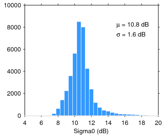
Figure 25. Histogram of flag-valid sigma0 over oceans and lakes for 16/10/2017. The mean ( \mu ) and standard deviation ( \sigma ) are also shown. Note that values outside [4 20] dB are excluded from the histogram for the sake of readability but not from the computation of \mu and \sigma .
