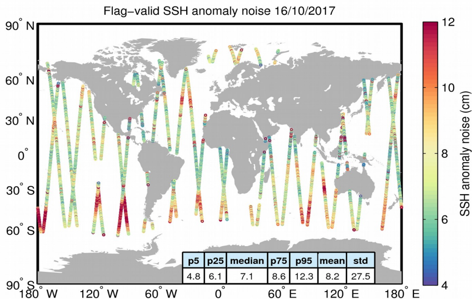
Figure 8. Geographical distribution of flag-valid 20-Hz SSH anomaly measurement noise over oceans and lakes for 16/10/2017. The statistical values shown in the table refer to the SSH anomaly noise and are calculated over all measurements shown in the figure.
