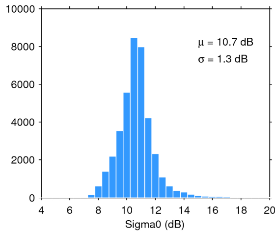
Figure 28. Histogram of science-valid sigma0 over oceans and lakes for 16/10/2017. The mean ( \mu ) and standard deviation ( \sigma ) are also shown. Note that values outside [4 20] dB are excluded from the histogram for the sake of readability but not from the computation of \mu and \sigma .
