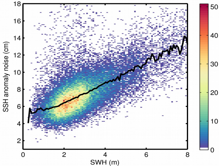
Figure 9. 2D histogram showing flag-valid SSH anomaly noise as a function of SWH for 16/10/2017. The black line denotes the median SSH anomaly noise as a function of SWH.
