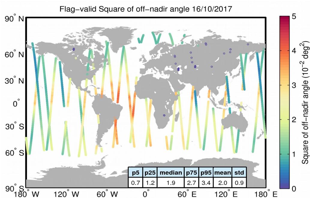
Figure 37. Geographical distribution of flag-valid mispointing data over oceans and lakes for 16/10/2017. The statistical values shown in the table refer to the mispointing in 10^{-2} deg 2 and are calculated over all measurements shown in the figure.
