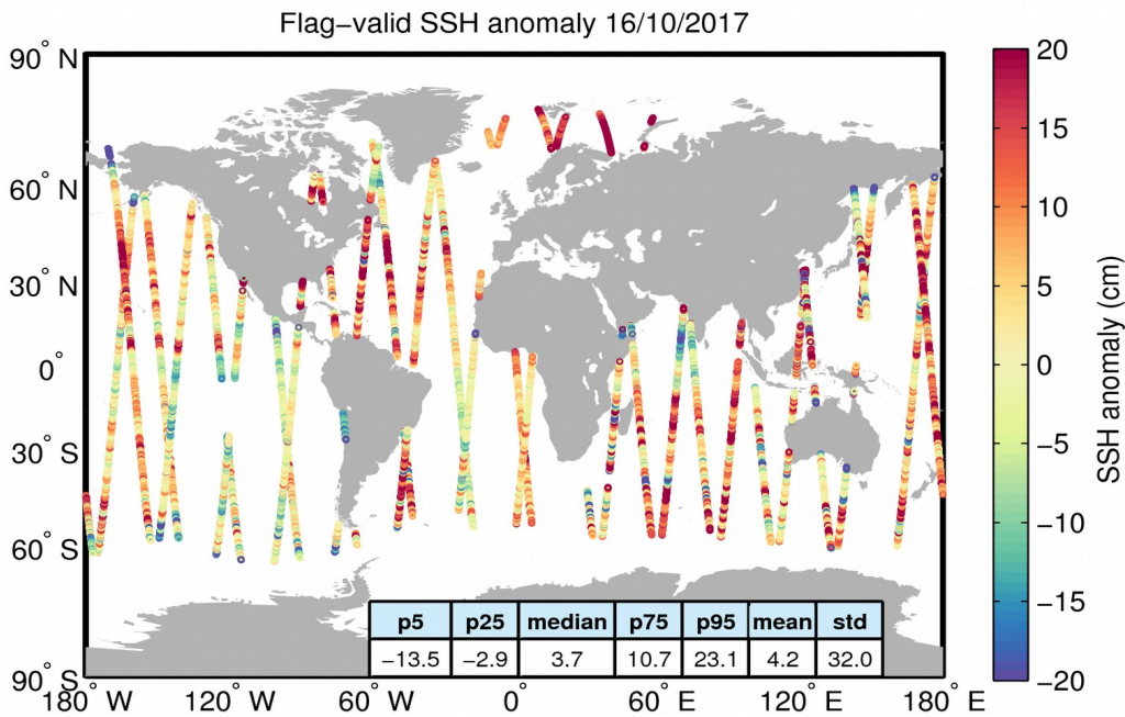
Figure 5. Geographical distribution of flag-valid 1-Hz SSH anomaly data over oceans and lakes for 16/10/2017. The statistical values shown in the table refer to the SSH anomaly in cm and are calculated over all measurements shown in the figure.
