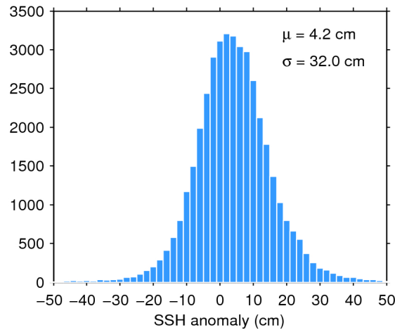
Figure 7. Histogram of flag-valid SSH anomaly over oceans and lakes for 16/10/2017. The mean ( \mu ) and standard deviation ( \sigma ) are also shown. Note that values outside [-50 50] cm are excluded from the histogram for the sake of readability but not from the computation of \mu and \sigma .
