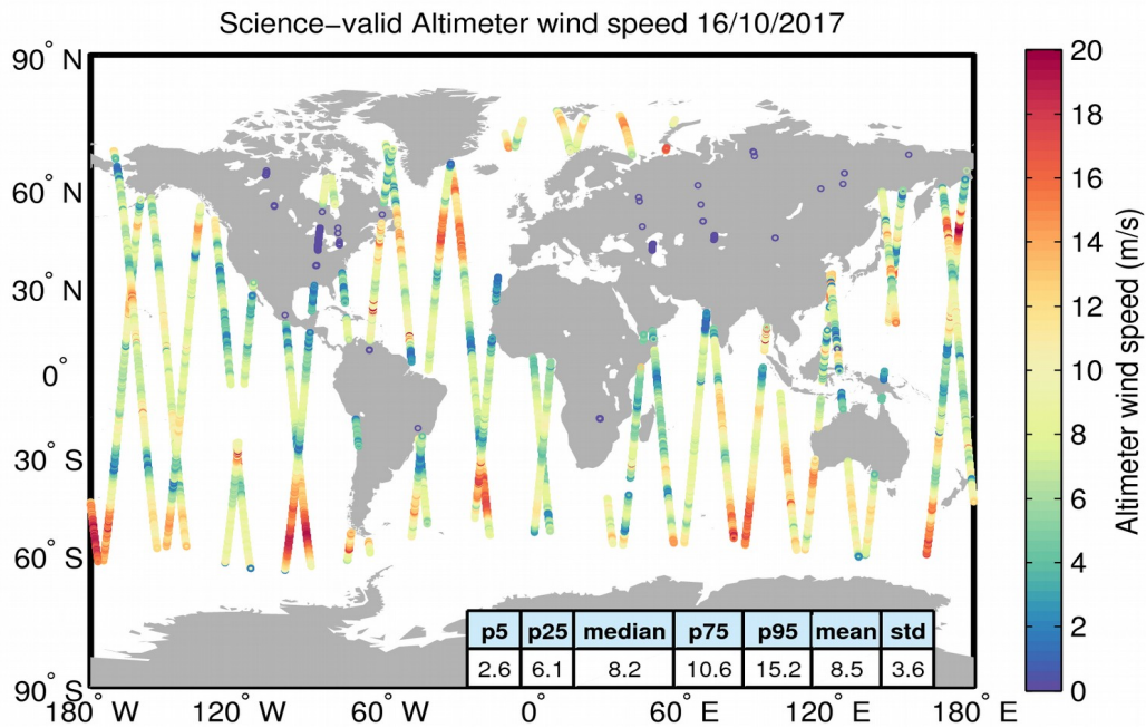
Figure 34. Geographical distribution of science-valid wind data over oceans and lakes for 16/10/2017. The statistical values shown in the table refer to the wind in m/s and are calculated over all measurements shown in the figure. Gray circles denote records that have been rejected based on the editing criteria described in Table 5.
