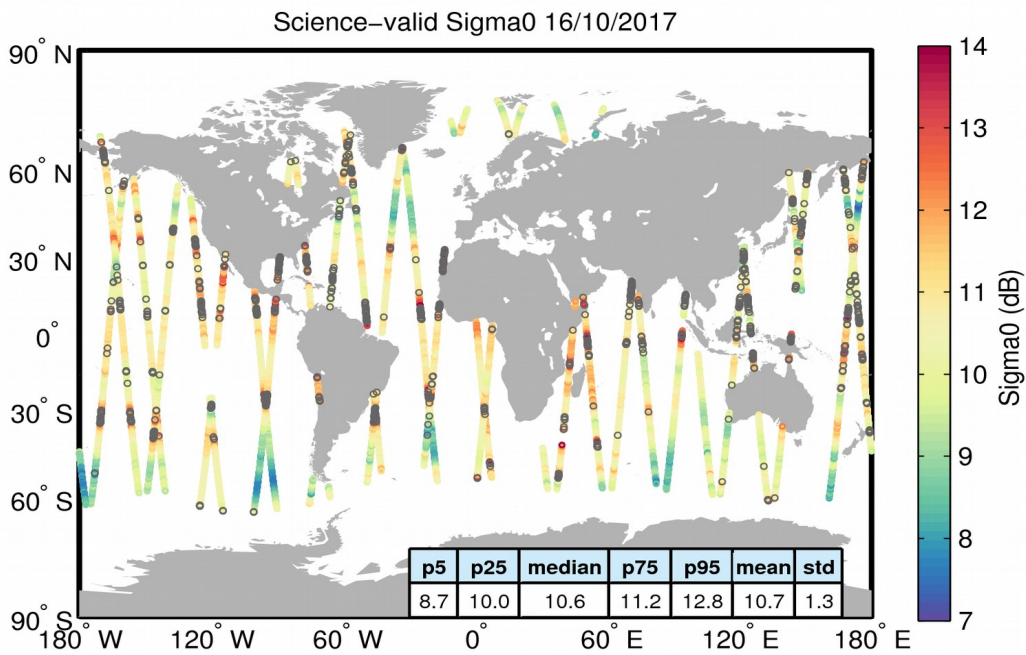
Figure 27. Geographical distribution of science-valid sigma0 data over oceans and lakes for 16/10/2017. The statistical values shown in the table refer to the sigma0 in dB and are calculated over all measurements shown in the figure. Gray circles denote records that have been rejected based on the editing criteria described in Table 4.
