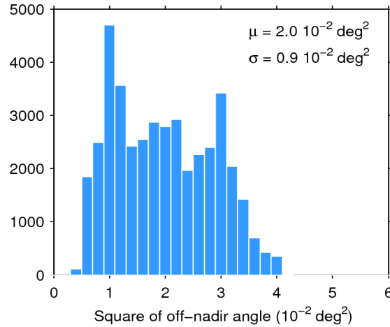
Figure 39. Histogram of flag-valid mispointing over oceans and lakes for 16/10/2017. The mean ( \mu ) and standard deviation ( \sigma ) are also shown. Note that values larger than 6 \cdot 10^{-2} \text{ deg}^2 are excluded from the histogram for the sake of readability but not from the computation of \mu and \sigma .
