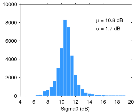
Figure 25. Histogram of flag-valid sigma0 over oceans and lakes for 15/10/2017. The mean ( \mu ) and standard deviation ( \sigma ) are also shown. Note that values outside [4 20] dB are excluded from the histogram for the sake of readability but not from the computation of \mu and \sigma .
