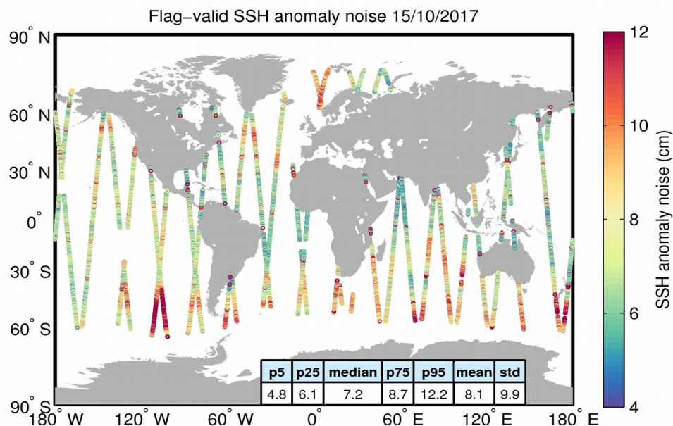
Figure 8. Geographical distribution of flag-valid 20-Hz SSH anomaly measurement noise over oceans and lakes for 15/10/2017. The statistical values shown in the table refer to the SSH anomaly noise and are calculated over all measurements shown in the figure.
