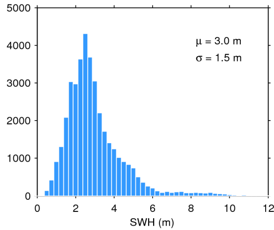
Figure 17. Histogram of flag-valid SWH over oceans and lakes for 15/10/2017. The mean ( \mu ) and standard deviation ( \sigma ) are also shown. Note that values larger than 12 m are excluded from the histogram for the sake of readability but not from the computation of \mu and \sigma .
