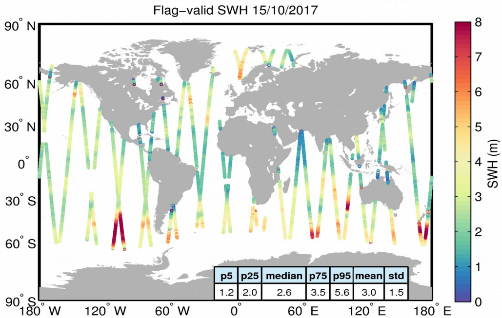
Figure 15. Geographical distribution of flag-valid SWH data over oceans and lakes for 15/10/2017. The statistical values shown in the table refer to the SWH in m and are calculated over all measurements shown in the figure.
