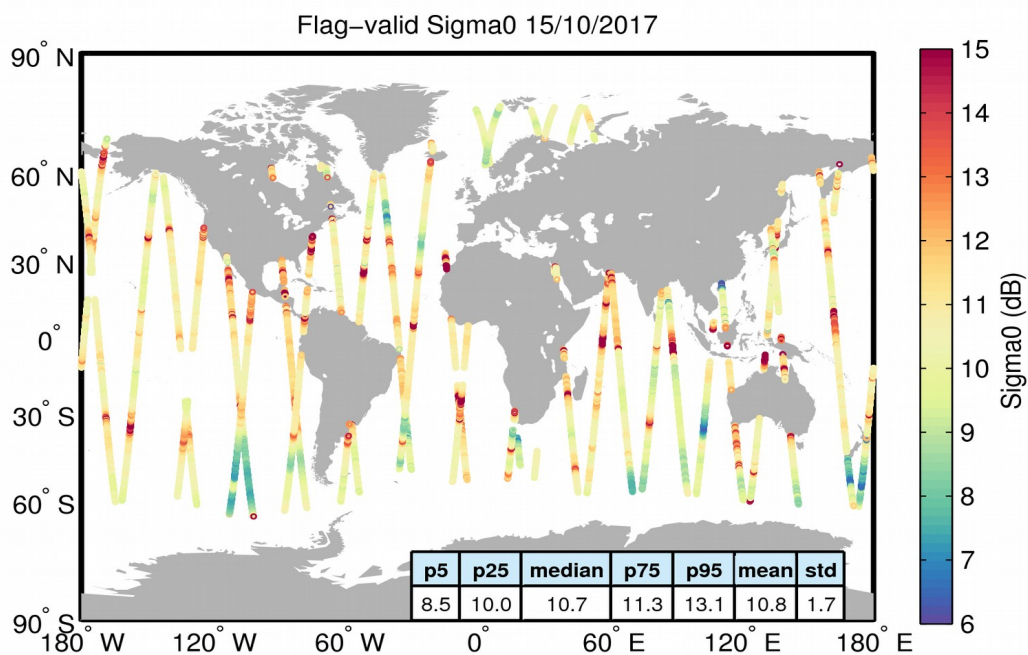
Figure 23. Geographical distribution of flag-valid sigma0 data over oceans and lakes for 15/10/2017. The statistical values shown in the table refer to the sigma0 in dB and are calculated over all measurements shown in the figure.
