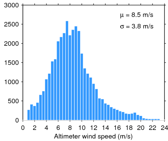
Figure 33. Histogram of flag-valid wind over oceans and lakes for 15/10/2017. The mean ( \mu ) and standard deviation ( \sigma ) are also shown. Note that values larger than 24 m/s are excluded from the histogram for the sake of readability but not from the computation of \mu and \sigma .
