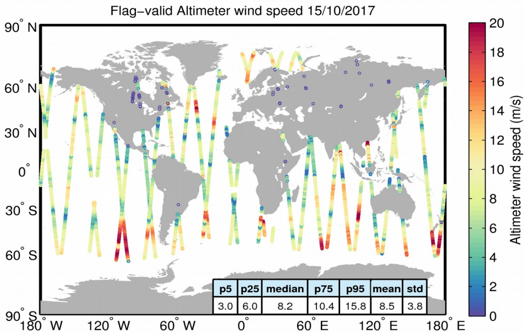
Figure 31. Geographical distribution of flag-valid wind data over oceans and lakes for 15/10/2017. The statistical values shown in the table refer to the wind in m/s and are calculated over all measurements shown in the figure.
