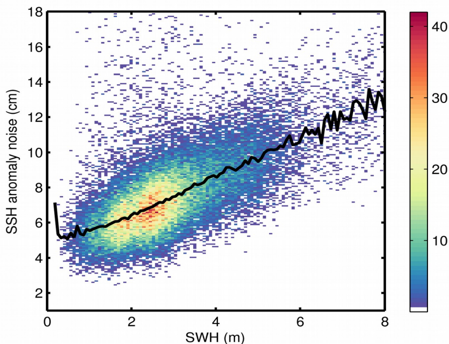
Figure 9. 2D histogram showing flag-valid SSH anomaly noise as a function of SWH for 15/10/2017. The black line denotes the median SSH anomaly noise as a function of SWH.
