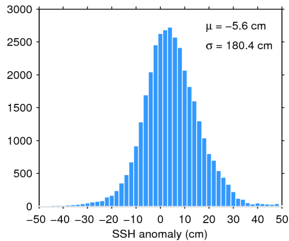
Figure 7. Histogram of flag-valid SSH anomaly over oceans and lakes for 15/10/2017. The mean ( \mu ) and standard deviation ( \sigma ) are also shown. Note that values outside [-50 50] cm are excluded from the histogram for the sake of readability but not from the computation of \mu and \sigma .
