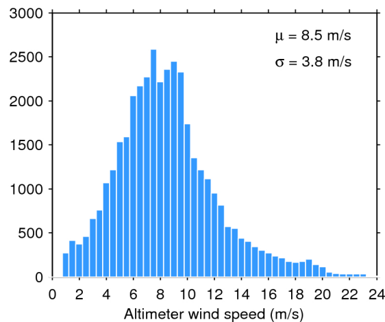
Figure 35. Histogram of science-valid wind over oceans and lakes for 15/10/2017. The mean ( \mu ) and standard deviation ( \sigma ) are also shown. Note that values larger than 24 m/s are excluded from the histogram for the sake of readability but not from the computation of \mu and \sigma .
