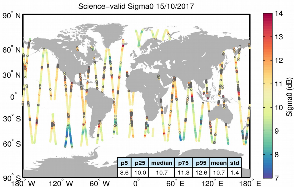
Figure 27. Geographical distribution of science-valid sigma0 data over oceans and lakes for 15/10/2017. The statistical values shown in the table refer to the sigma0 in dB and are calculated over all measurements shown in the figure. Gray circles denote records that have been rejected based on the editing criteria described in Table 4.
