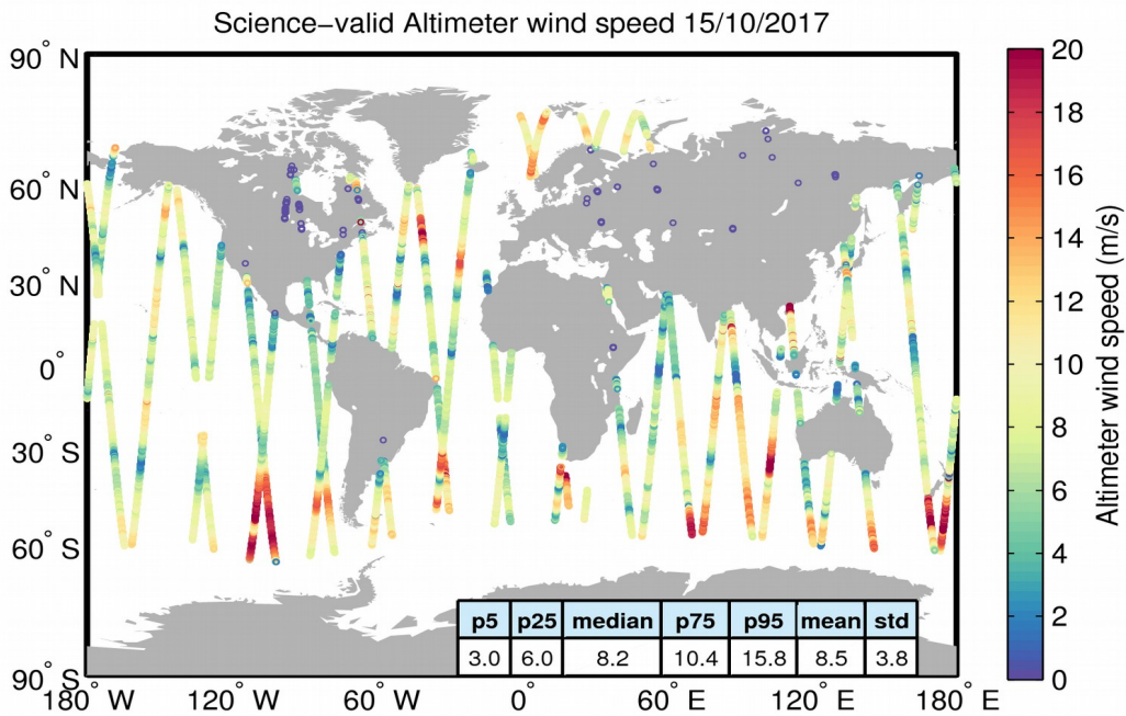
Figure 34. Geographical distribution of science-valid wind data over oceans and lakes for 15/10/2017. The statistical values shown in the table refer to the wind in m/s and are calculated over all measurements shown in the figure. Gray circles denote records that have been rejected based on the editing criteria described in Table 5.
