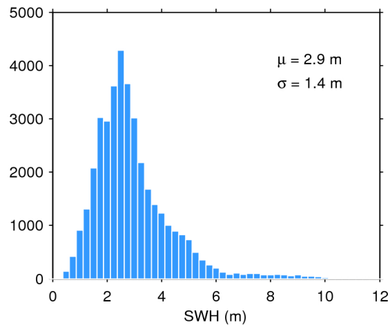
Figure 20. Histogram of science-valid SWH over oceans and lakes for 15/10/2017. The mean ( \mu ) and standard deviation ( \sigma ) are also shown. Note that values larger than 12 m are excluded from the histogram for the sake of readability but not from the computation of \mu and \sigma .
