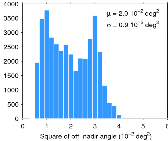
Figure 39. Histogram of flag-valid mispointing over oceans and lakes for 15/10/2017. The mean ( \mu ) and standard deviation ( \sigma ) are also shown. Note that values larger than 6 \cdot 10^{-2} \text{ deg}^2 are excluded from the histogram for the sake of readability but not from the computation of \mu and \sigma .
