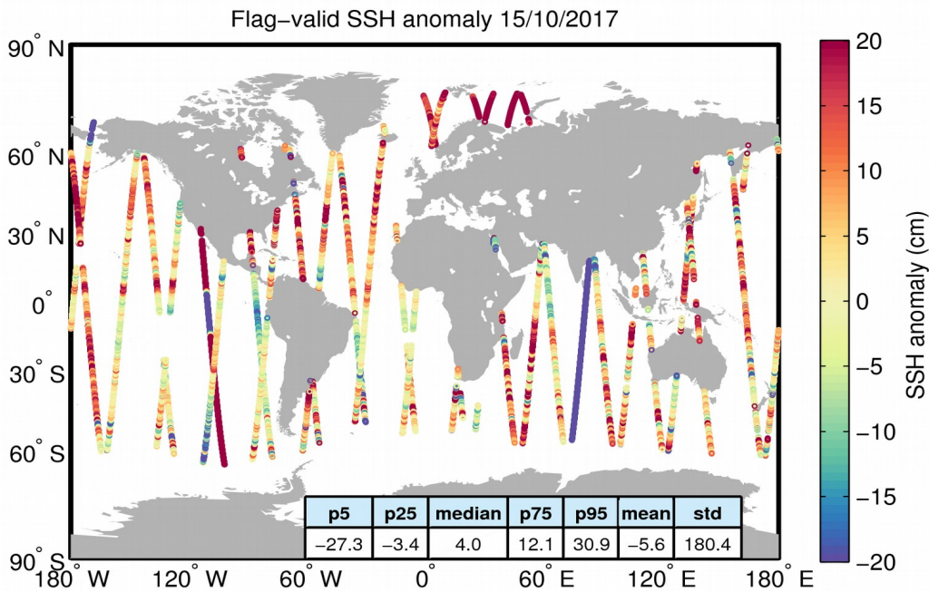
Figure 5. Geographical distribution of flag-valid 1-Hz SSH anomaly data over oceans and lakes for 15/10/2017. The statistical values shown in the table refer to the SSH anomaly in cm and are calculated over all measurements shown in the figure.
