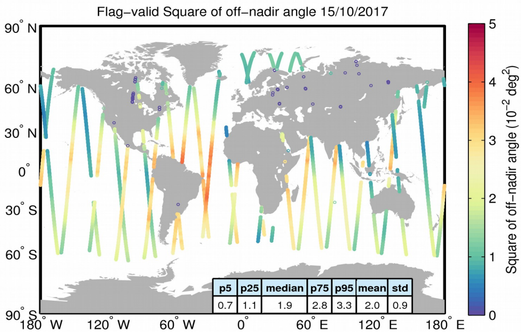
Figure 37. Geographical distribution of flag-valid mispointing data over oceans and lakes for 15/10/2017. The statistical values shown in the table refer to the mispointing in 10^{-2} deg 2 and are calculated over all measurements shown in the figure.
