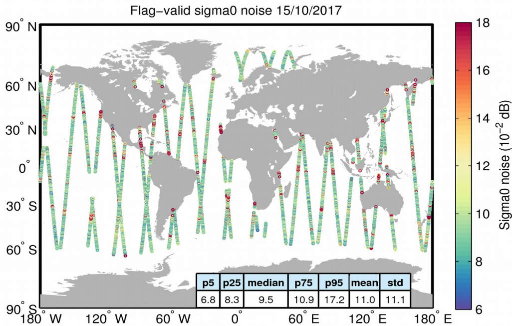
Figure 26. Geographical distribution of flag-valid 20-Hz sigma0 measurement noise over oceans and lakes for 15/10/2017. The statistical values shown in the table refer to the sigma0 noise and are calculated over all measurements shown in the figure.
