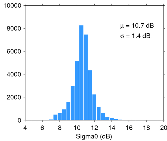
Figure 28. Histogram of science-valid sigma0 over oceans and lakes for 15/10/2017. The mean ( \mu ) and standard deviation ( \sigma ) are also shown. Note that values outside [4 20] dB are excluded from the histogram for the sake of readability but not from the computation of \mu and \sigma .
