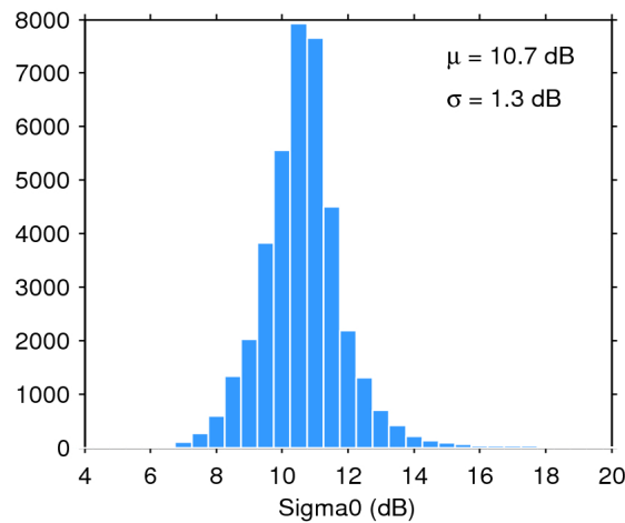
Figure 28. Histogram of science-valid sigma0 over oceans and lakes for 13/10/2017. The mean ( \mu ) and standard deviation ( \sigma ) are also shown. Note that values outside [4 20] dB are excluded from the histogram for the sake of readability but not from the computation of \mu and \sigma .
