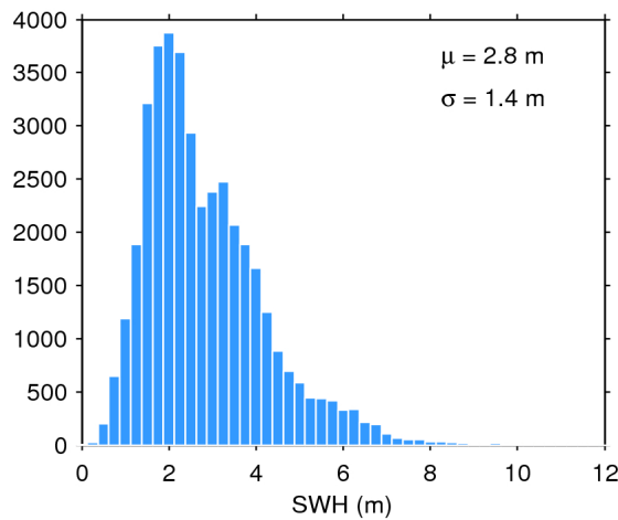
Figure 17. Histogram of flag-valid SWH over oceans and lakes for 13/10/2017. The mean ( \mu ) and standard deviation ( \sigma ) are also shown. Note that values larger than 12 m are excluded from the histogram for the sake of readability but not from the computation of \mu and \sigma .
