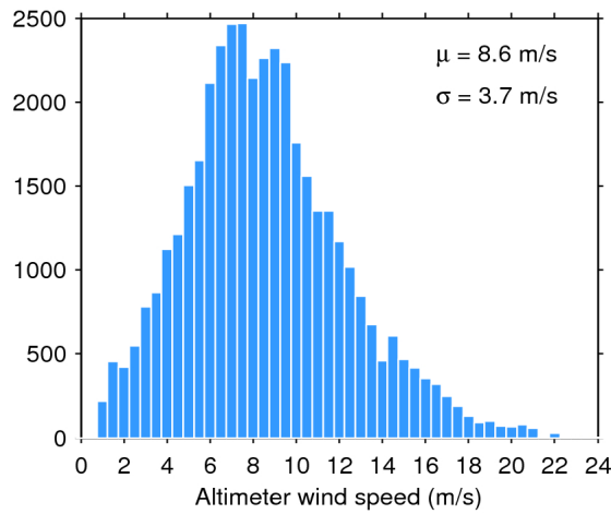
Figure 33. Histogram of flag-valid wind over oceans and lakes for 13/10/2017. The mean ( \mu ) and standard deviation ( \sigma ) are also shown. Note that values larger than 24 m/s are excluded from the histogram for the sake of readability but not from the computation of \mu and \sigma .
