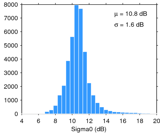
Figure 25. Histogram of flag-valid sigma0 over oceans and lakes for 13/10/2017. The mean ( \mu ) and standard deviation ( \sigma ) are also shown. Note that values outside [4 20] dB are excluded from the histogram for the sake of readability but not from the computation of \mu and \sigma .
