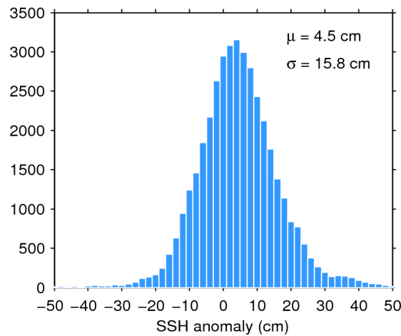
Figure 7. Histogram of flag-valid SSH anomaly over oceans and lakes for 13/10/2017. The mean ( \mu ) and standard deviation ( \sigma ) are also shown. Note that values outside [-50\ 50] cm are excluded from the histogram for the sake of readability but not from the computation of \mu and \sigma .
