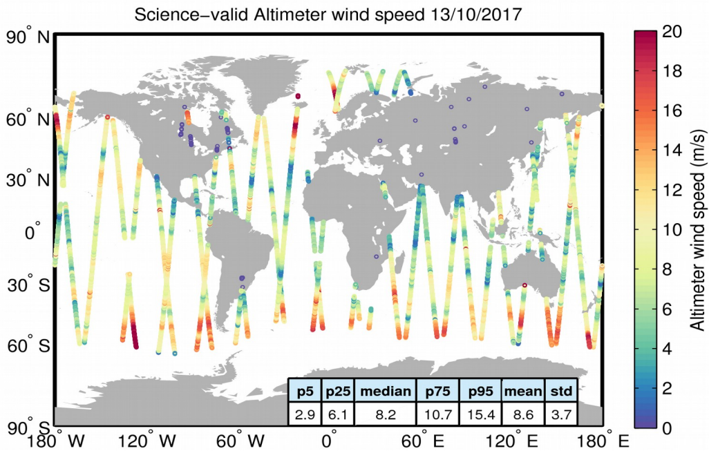
Figure 34. Geographical distribution of science-valid wind data over oceans and lakes for 13/10/2017. The statistical values shown in the table refer to the wind in m/s and are calculated over all measurements shown in the figure. Gray circles denote records that have been rejected based on the editing criteria described in Table 5.
