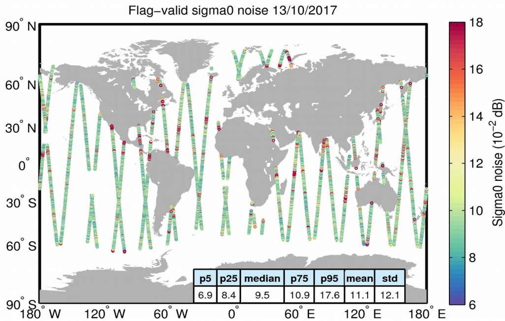
Figure 26. Geographical distribution of flag-valid 20-Hz sigma0 measurement noise over oceans and lakes for 13/10/2017. The statistical values shown in the table refer to the sigma0 noise and are calculated over all measurements shown in the figure.
