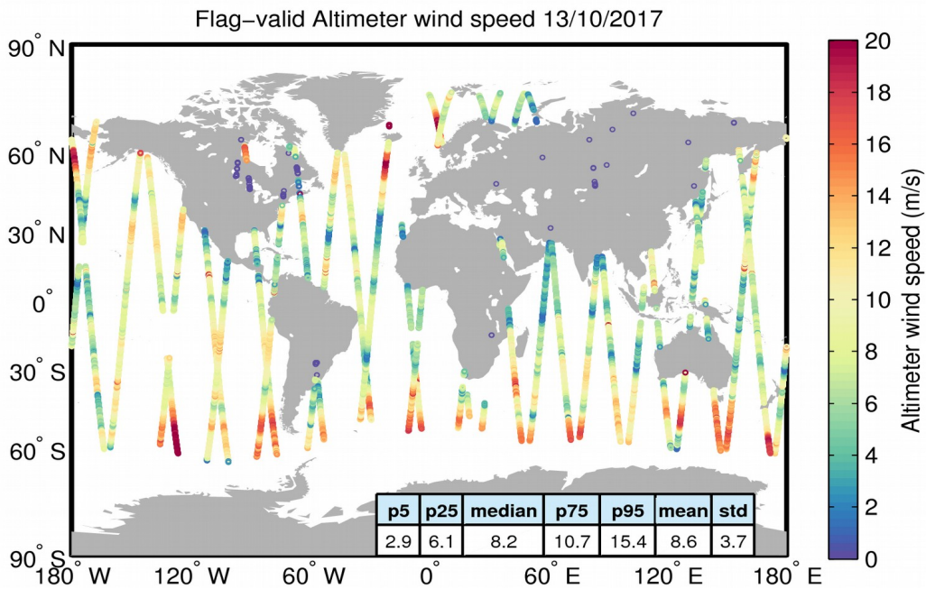
Figure 31. Geographical distribution of flag-valid wind data over oceans and lakes for 13/10/2017. The statistical values shown in the table refer to the wind in m/s and are calculated over all measurements shown in the figure.
