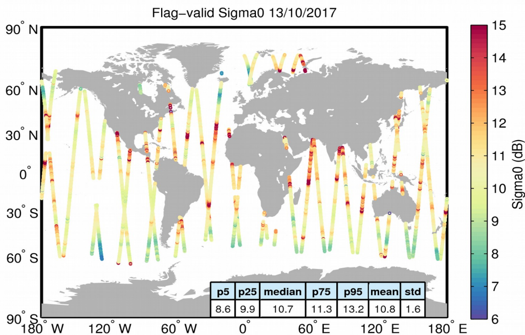
Figure 23. Geographical distribution of flag-valid sigma0 data over oceans and lakes for 13/10/2017. The statistical values shown in the table refer to the sigma0 in dB and are calculated over all measurements shown in the figure.
