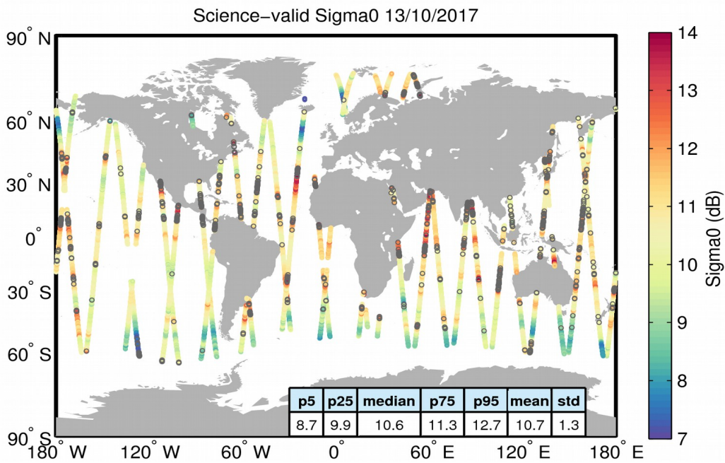
Figure 27. Geographical distribution of science-valid sigma0 data over oceans and lakes for 13/10/2017. The statistical values shown in the table refer to the sigma0 in dB and are calculated over all measurements shown in the figure. Gray circles denote records that have been rejected based on the editing criteria described in Table 4.
