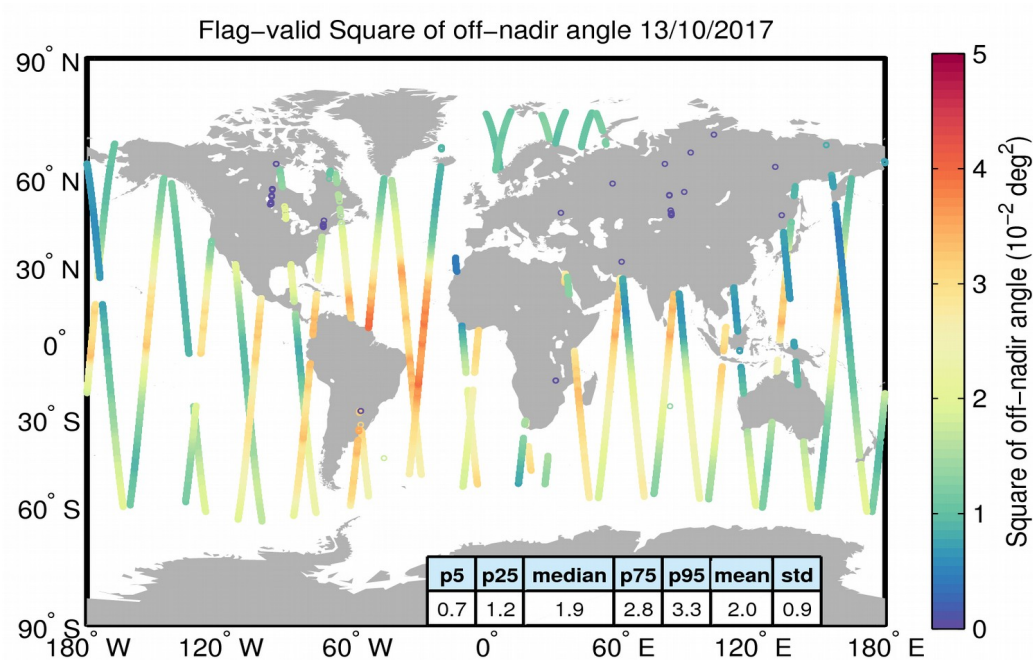
Figure 37. Geographical distribution of flag-valid mispointing data over oceans and lakes for 13/10/2017. The statistical values shown in the table refer to the mispointing in 10^{-2} deg 2 and are calculated over all measurements shown in the figure.
