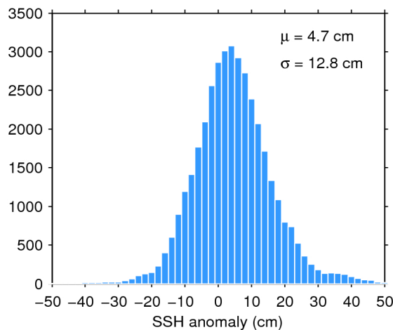
Figure 11. Histogram of science-valid SSH anomaly over oceans and lakes for 13/10/2017. The mean ( \mu ) and standard deviation ( \sigma ) are also shown. Note that values outside [-50 50] cm are excluded from the histogram for the sake of readability but not from the computation of \mu and \sigma .
