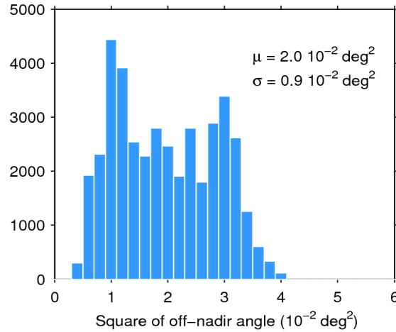
Figure 39. Histogram of flag-valid mispointing over oceans and lakes for 13/10/2017. The mean ( \mu ) and standard deviation ( \sigma ) are also shown. Note that values larger than 6 \cdot 10^{-2} \text{ deg}^2 are excluded from the histogram for the sake of readability but not from the computation of \mu and \sigma .
