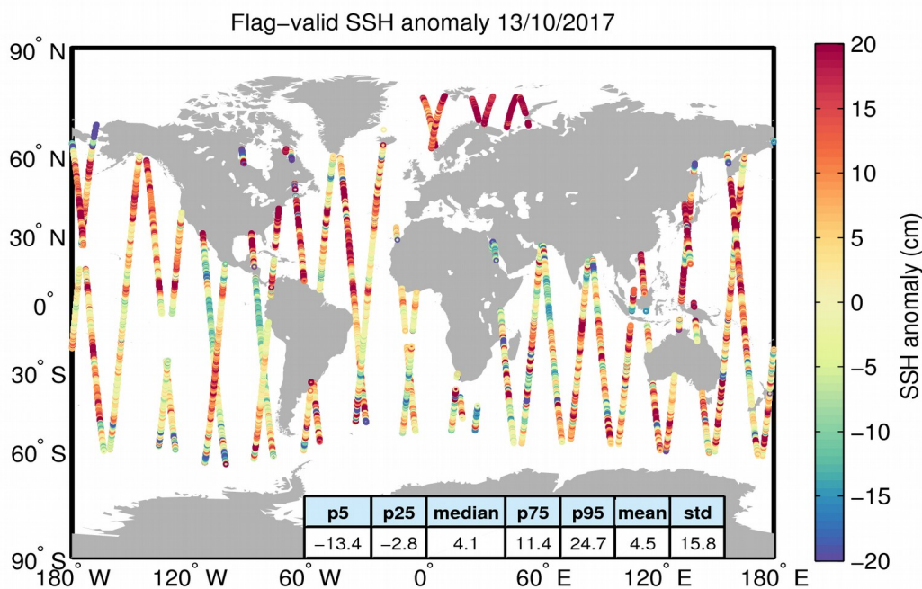
Figure 5. Geographical distribution of flag-valid 1-Hz SSH anomaly data over oceans and lakes for 13/10/2017. The statistical values shown in the table refer to the SSH anomaly in cm and are calculated over all measurements shown in the figure.
