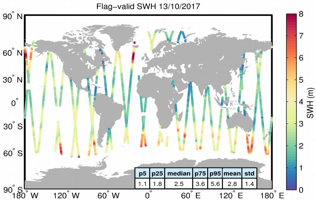
Figure 15. Geographical distribution of flag-valid SWH data over oceans and lakes for 13/10/2017. The statistical values shown in the table refer to the SWH in m and are calculated over all measurements shown in the figure.
