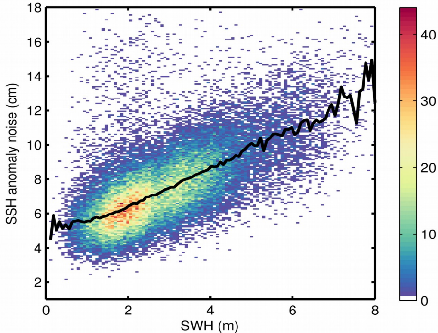
Figure 9. 2D histogram showing flag-valid SSH anomaly noise as a function of SWH for 13/10/2017. The black line denotes the median SSH anomaly noise as a function of SWH.
