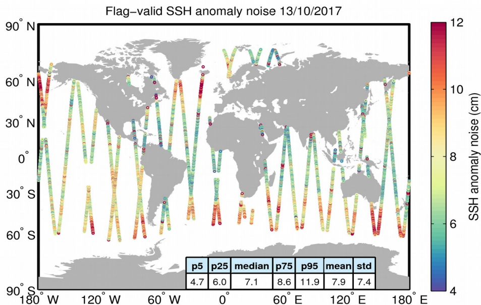
Figure 8. Geographical distribution of flag-valid 20-Hz SSH anomaly measurement noise over oceans and lakes for 13/10/2017. The statistical values shown in the table refer to the SSH anomaly noise and are calculated over all measurements shown in the figure.
