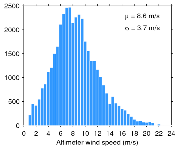
Figure 35. Histogram of science-valid wind over oceans and lakes for 13/10/2017. The mean ( \mu ) and standard deviation ( \sigma ) are also shown. Note that values larger than 24 m/s are excluded from the histogram for the sake of readability but not from the computation of \mu and \sigma .
