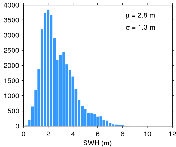
Figure 20. Histogram of science-valid SWH over oceans and lakes for 13/10/2017. The mean ( \mu ) and standard deviation ( \sigma ) are also shown. Note that values larger than 12 m are excluded from the histogram for the sake of readability but not from the computation of \mu and \sigma .
