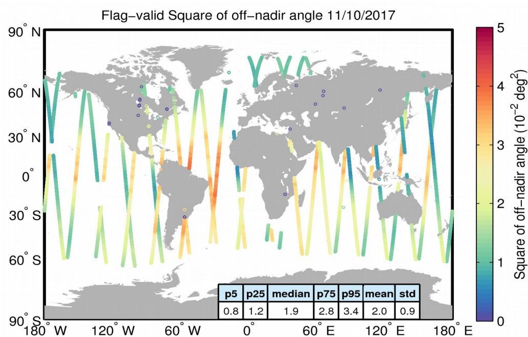
Figure 37. Geographical distribution of flag-valid mispointing data over oceans and lakes for 11/10/2017. The statistical values shown in the table refer to the mispointing in 10^{-2} deg 2 and are calculated over all measurements shown in the figure.
