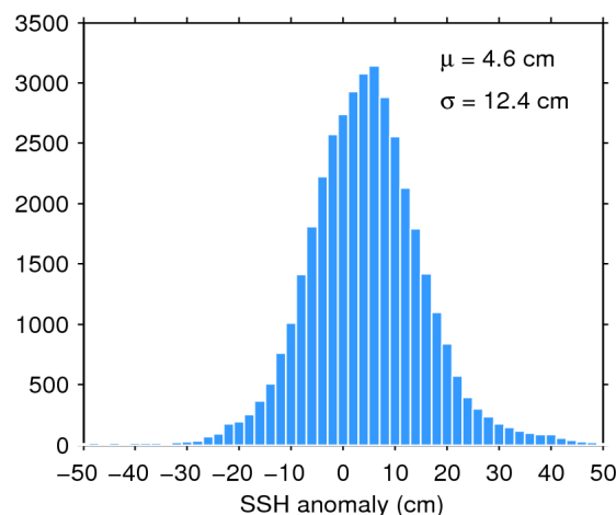
Figure 11. Histogram of science-valid SSH anomaly over oceans and lakes for 11/10/2017. The mean ( \mu ) and standard deviation ( \sigma ) are also shown. Note that values outside [-50 50] cm are excluded from the histogram for the sake of readability but not from the computation of \mu and \sigma .
