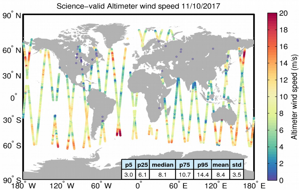
Figure 34. Geographical distribution of science-valid wind data over oceans and lakes for 11/10/2017. The statistical values shown in the table refer to the wind in m/s and are calculated over all measurements shown in the figure. Gray circles denote records that have been rejected based on the editing criteria described in Table 5.
