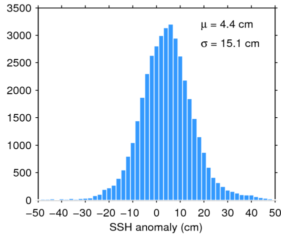
Figure 7. Histogram of flag-valid SSH anomaly over oceans and lakes for 11/10/2017. The mean ( \mu ) and standard deviation ( \sigma ) are also shown. Note that values outside [-50\ 50] cm are excluded from the histogram for the sake of readability but not from the computation of \mu and \sigma .
