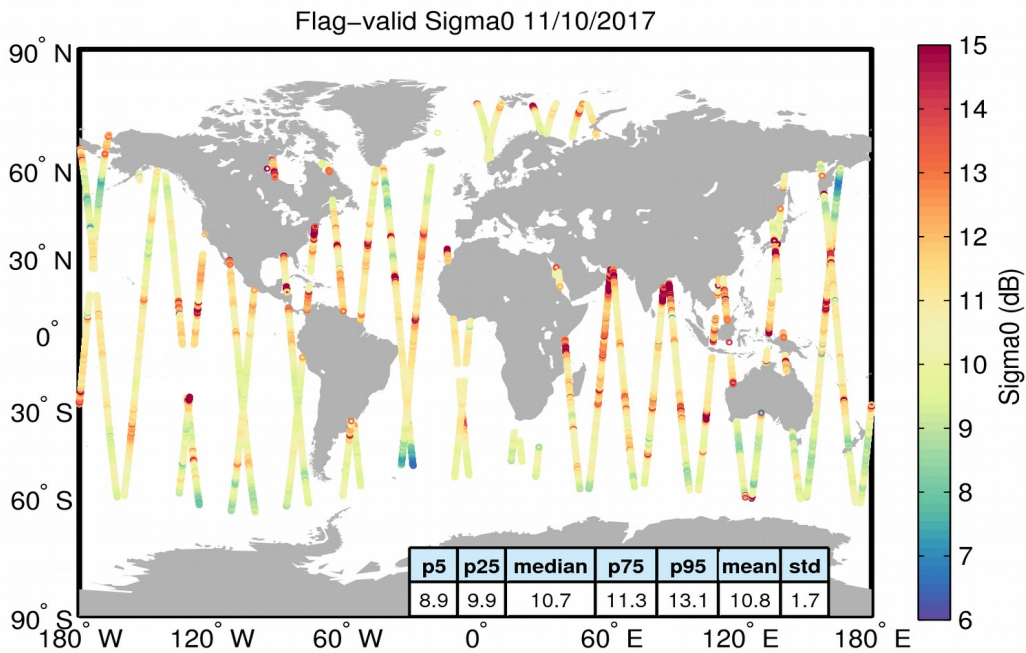
Figure 23. Geographical distribution of flag-valid sigma0 data over oceans and lakes for 11/10/2017. The statistical values shown in the table refer to the sigma0 in dB and are calculated over all measurements shown in the figure.
