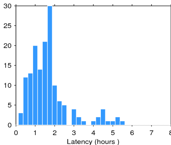
Figure 2. Histogram of the data latency for 11/10/2017. The y-axis denotes the number of files that are made available with a delay of x-hours with respect to the mean time of the records stored in the file.
