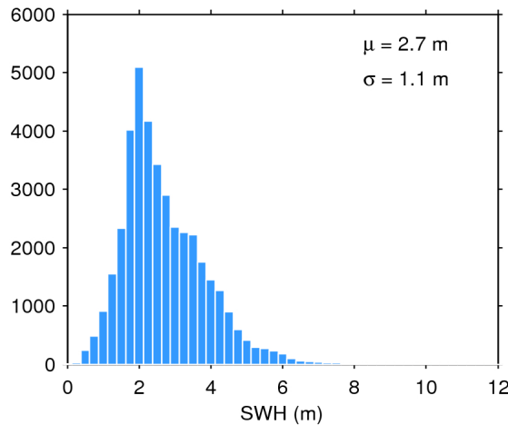
Figure 20. Histogram of science-valid SWH over oceans and lakes for 11/10/2017. The mean ( \mu ) and standard deviation ( \sigma ) are also shown. Note that values larger than 12 m are excluded from the histogram for the sake of readability but not from the computation of \mu and \sigma .
