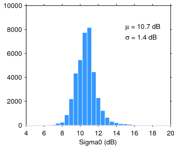
Figure 28. Histogram of science-valid sigma0 over oceans and lakes for 11/10/2017. The mean ( \mu ) and standard deviation ( \sigma ) are also shown. Note that values outside [4 20] dB are excluded from the histogram for the sake of readability but not from the computation of \mu and \sigma .
