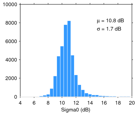
Figure 25. Histogram of flag-valid sigma0 over oceans and lakes for 11/10/2017. The mean ( \mu ) and standard deviation ( \sigma ) are also shown. Note that values outside [4 20] dB are excluded from the histogram for the sake of readability but not from the computation of \mu and \sigma .
