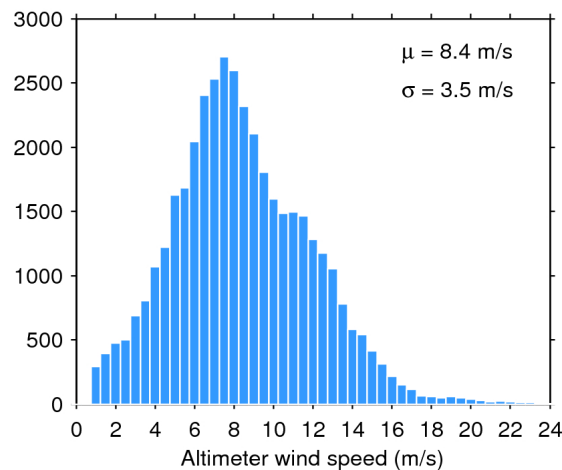
Figure 35. Histogram of science-valid wind over oceans and lakes for 11/10/2017. The mean ( \mu ) and standard deviation ( \sigma ) are also shown. Note that values larger than 24 m/s are excluded from the histogram for the sake of readability but not from the computation of \mu and \sigma .
