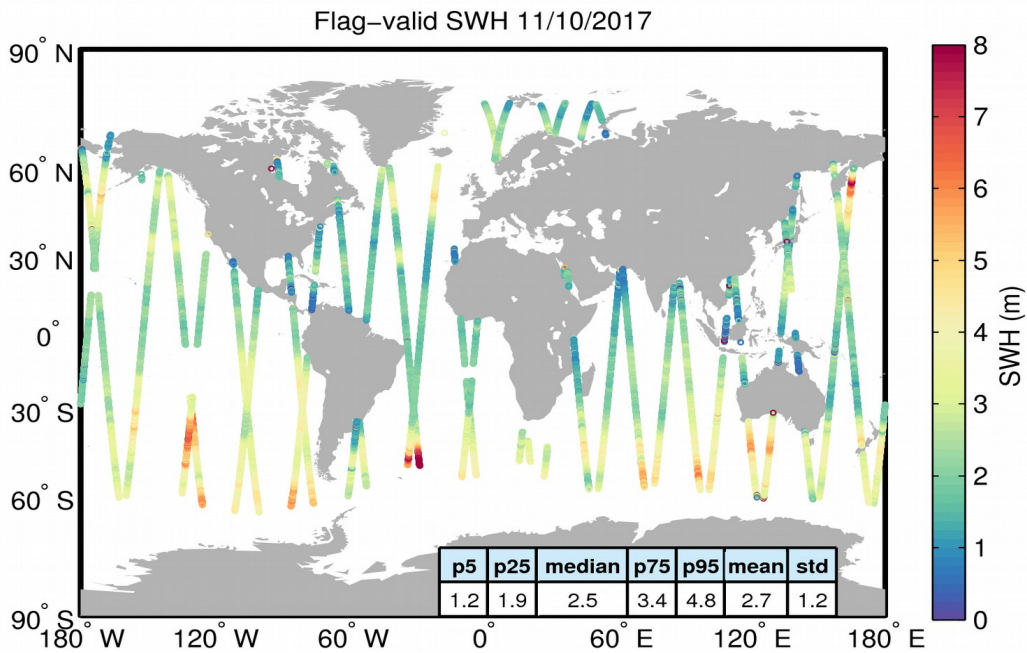
Figure 15. Geographical distribution of flag-valid SWH data over oceans and lakes for 11/10/2017. The statistical values shown in the table refer to the SWH in m and are calculated over all measurements shown in the figure.
