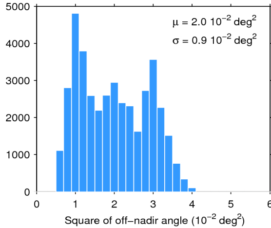
Figure 39. Histogram of flag-valid mispointing over oceans and lakes for 11/10/2017. The mean ( \mu ) and standard deviation ( \sigma ) are also shown. Note that values larger than 6 \cdot 10^{-2} \text{ deg}^2 are excluded from the histogram for the sake of readability but not from the computation of \mu and \sigma .
