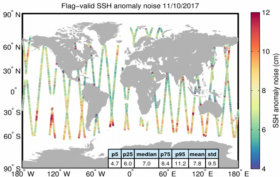
Figure 8. Geographical distribution of flag-valid 20-Hz SSH anomaly measurement noise over oceans and lakes for 11/10/2017. The statistical values shown in the table refer to the SSH anomaly noise and are calculated over all measurements shown in the figure.
