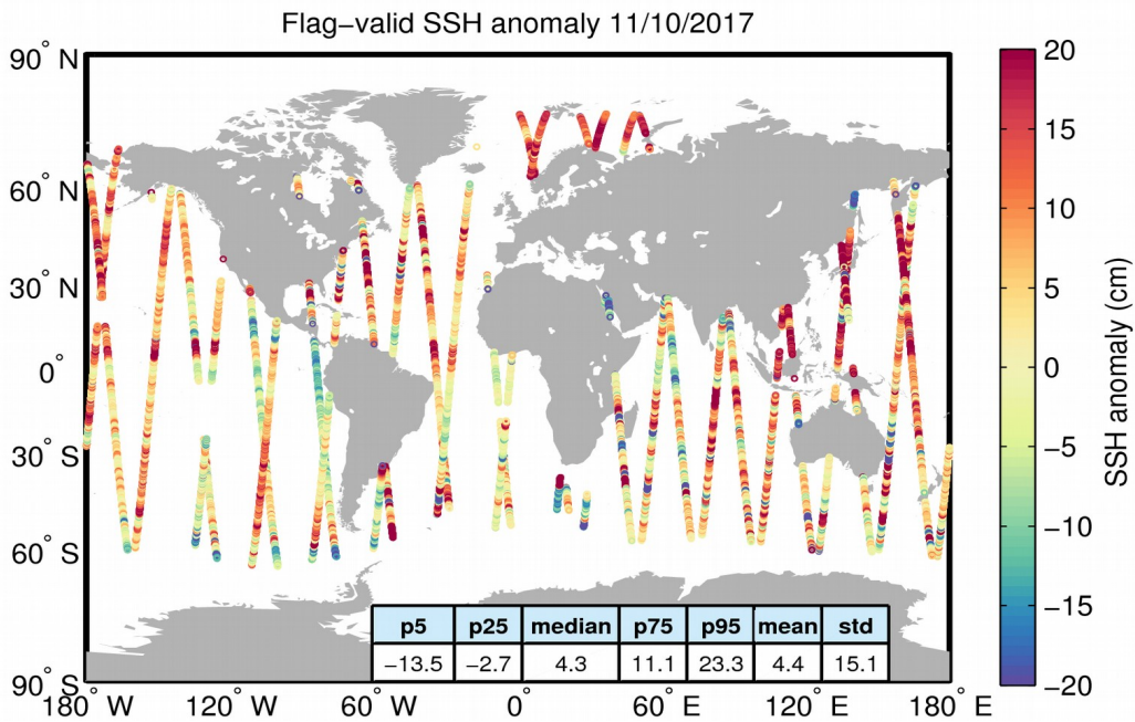
Figure 5. Geographical distribution of flag-valid 1-Hz SSH anomaly data over oceans and lakes for 11/10/2017. The statistical values shown in the table refer to the SSH anomaly in cm and are calculated over all measurements shown in the figure.
