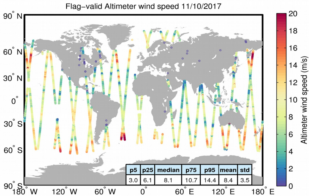
Figure 31. Geographical distribution of flag-valid wind data over oceans and lakes for 11/10/2017. The statistical values shown in the table refer to the wind in m/s and are calculated over all measurements shown in the figure.
