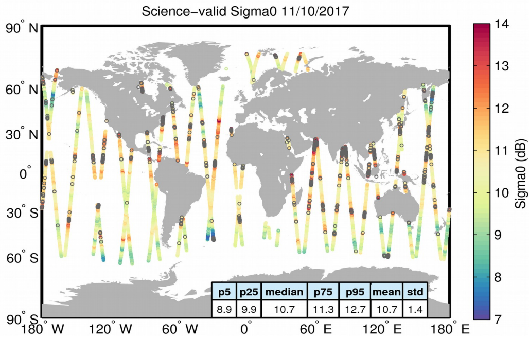
Figure 27. Geographical distribution of science-valid sigma0 data over oceans and lakes for 11/10/2017. The statistical values shown in the table refer to the sigma0 in dB and are calculated over all measurements shown in the figure. Gray circles denote records that have been rejected based on the editing criteria described in Table 4.
