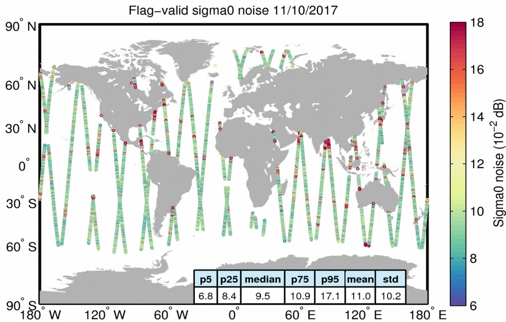
Figure 26. Geographical distribution of flag-valid 20-Hz sigma0 measurement noise over oceans and lakes for 11/10/2017. The statistical values shown in the table refer to the sigma0 noise and are calculated over all measurements shown in the figure.
