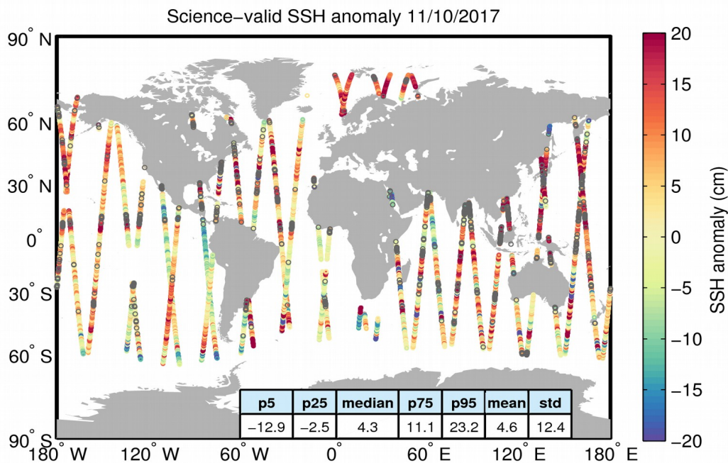
Figure 10. Geographical distribution of science-valid SSH anomaly data over oceans and lakes for 11/10/2017. The statistical values shown in the table refer to the SSH anomaly in cm and are calculated over all measurements shown in the figure. Gray circles denote records that have been rejected based on the editing criteria described in Table 2.
