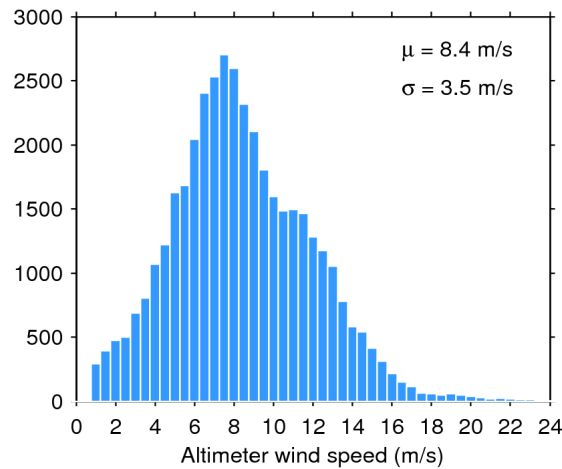
Figure 33. Histogram of flag-valid wind over oceans and lakes for 11/10/2017. The mean ( \mu ) and standard deviation ( \sigma ) are also shown. Note that values larger than 24 m/s are excluded from the histogram for the sake of readability but not from the computation of \mu and \sigma .
