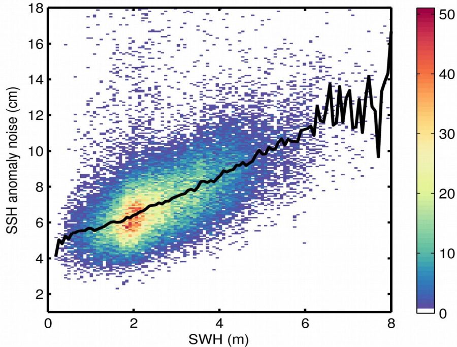
Figure 9. 2D histogram showing flag-valid SSH anomaly noise as a function of SWH for 11/10/2017. The black line denotes the median SSH anomaly noise as a function of SWH.
