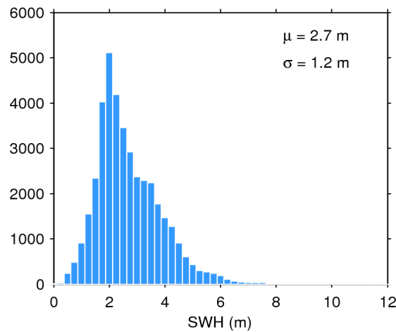
Figure 17. Histogram of flag-valid SWH over oceans and lakes for 11/10/2017. The mean ( \mu ) and standard deviation ( \sigma ) are also shown. Note that values larger than 12 m are excluded from the histogram for the sake of readability but not from the computation of \mu and \sigma .
