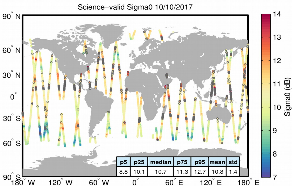
Figure 27. Geographical distribution of science-valid sigma0 data over oceans and lakes for 10/10/2017. The statistical values shown in the table refer to the sigma0 in dB and are calculated over all measurements shown in the figure. Gray circles denote records that have been rejected based on the editing criteria described in Table 4.
