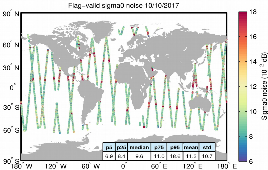
Figure 26. Geographical distribution of flag-valid 20-Hz sigma0 measurement noise over oceans and lakes for 10/10/2017. The statistical values shown in the table refer to the sigma0 noise and are calculated over all measurements shown in the figure.
