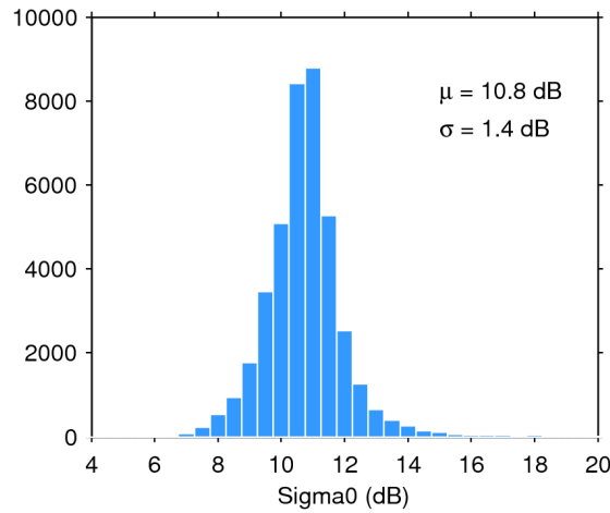
Figure 28. Histogram of science-valid sigma0 over oceans and lakes for 10/10/2017. The mean ( \mu ) and standard deviation ( \sigma ) are also shown. Note that values outside [4 20] dB are excluded from the histogram for the sake of readability but not from the computation of \mu and \sigma .
