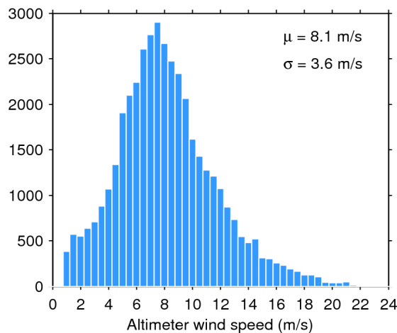
Figure 35. Histogram of science-valid wind over oceans and lakes for 10/10/2017. The mean ( \mu ) and standard deviation ( \sigma ) are also shown. Note that values larger than 24 m/s are excluded from the histogram for the sake of readability but not from the computation of \mu and \sigma .
