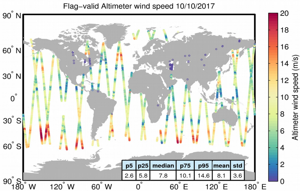
Figure 31. Geographical distribution of flag-valid wind data over oceans and lakes for 10/10/2017. The statistical values shown in the table refer to the wind in m/s and are calculated over all measurements shown in the figure.
