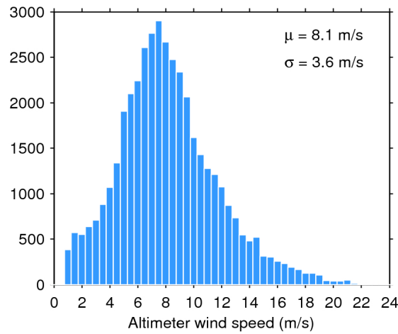
Figure 33. Histogram of flag-valid wind over oceans and lakes for 10/10/2017. The mean ( \mu ) and standard deviation ( \sigma ) are also shown. Note that values larger than 24 m/s are excluded from the histogram for the sake of readability but not from the computation of \mu and \sigma .
