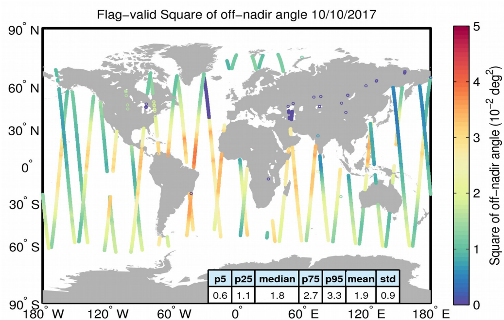
Figure 37. Geographical distribution of flag-valid mispointing data over oceans and lakes for 10/10/2017. The statistical values shown in the table refer to the mispointing in 10^{-2} deg 2 and are calculated over all measurements shown in the figure.
