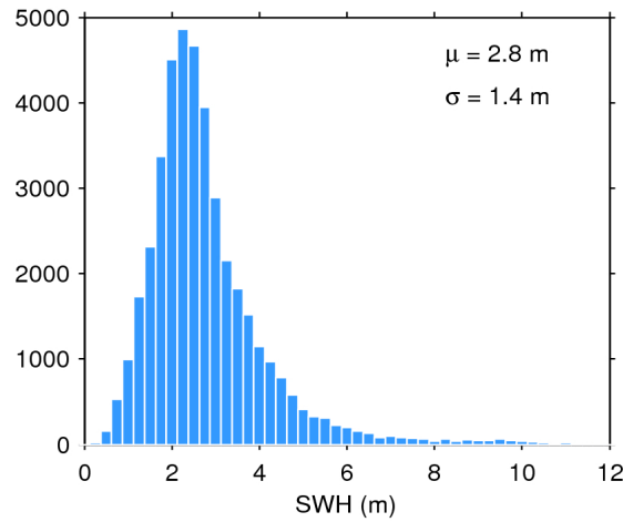
Figure 17. Histogram of flag-valid SWH over oceans and lakes for 10/10/2017. The mean ( \mu ) and standard deviation ( \sigma ) are also shown. Note that values larger than 12 m are excluded from the histogram for the sake of readability but not from the computation of \mu and \sigma .
