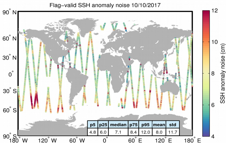
Figure 8. Geographical distribution of flag-valid 20-Hz SSH anomaly measurement noise over oceans and lakes for 10/10/2017. The statistical values shown in the table refer to the SSH anomaly noise and are calculated over all measurements shown in the figure.
