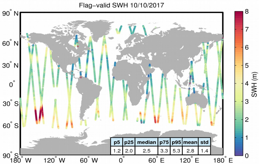
Figure 15. Geographical distribution of flag-valid SWH data over oceans and lakes for 10/10/2017. The statistical values shown in the table refer to the SWH in m and are calculated over all measurements shown in the figure.
