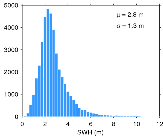
Figure 20. Histogram of science-valid SWH over oceans and lakes for 10/10/2017. The mean ( \mu ) and standard deviation ( \sigma ) are also shown. Note that values larger than 12 m are excluded from the histogram for the sake of readability but not from the computation of \mu and \sigma .
