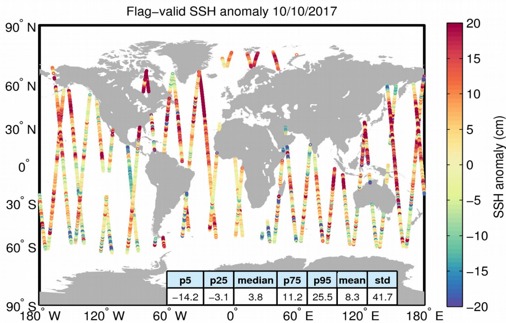
Figure 5. Geographical distribution of flag-valid 1-Hz SSH anomaly data over oceans and lakes for 10/10/2017. The statistical values shown in the table refer to the SSH anomaly in cm and are calculated over all measurements shown in the figure.
