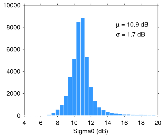
Figure 25. Histogram of flag-valid sigma0 over oceans and lakes for 10/10/2017. The mean ( \mu ) and standard deviation ( \sigma ) are also shown. Note that values outside [4 20] dB are excluded from the histogram for the sake of readability but not from the computation of \mu and \sigma .
