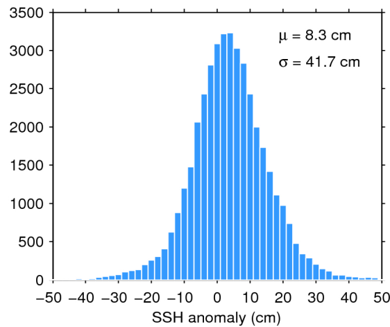
Figure 7. Histogram of flag-valid SSH anomaly over oceans and lakes for 10/10/2017. The mean ( \mu ) and standard deviation ( \sigma ) are also shown. Note that values outside [-50 50] cm are excluded from the histogram for the sake of readability but not from the computation of \mu and \sigma .
