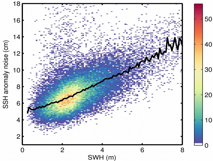
Figure 9. 2D histogram showing flag-valid SSH anomaly noise as a function of SWH for 10/10/2017. The black line denotes the median SSH anomaly noise as a function of SWH.
