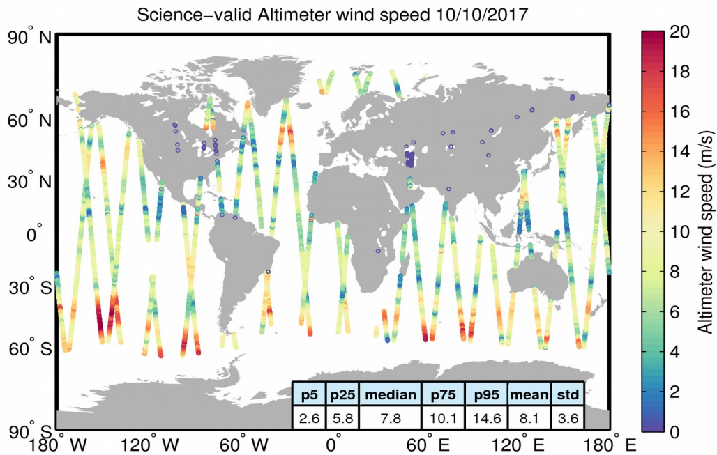
Figure 34. Geographical distribution of science-valid wind data over oceans and lakes for 10/10/2017. The statistical values shown in the table refer to the wind in m/s and are calculated over all measurements shown in the figure. Gray circles denote records that have been rejected based on the editing criteria described in Table 5.
