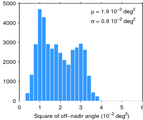
Figure 39. Histogram of flag-valid mispointing over oceans and lakes for 10/10/2017. The mean ( \mu ) and standard deviation ( \sigma ) are also shown. Note that values larger than 6 \cdot 10^{-2} \text{ deg}^2 are excluded from the histogram for the sake of readability but not from the computation of \mu and \sigma .
