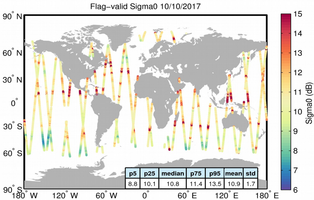
Figure 23. Geographical distribution of flag-valid sigma0 data over oceans and lakes for 10/10/2017. The statistical values shown in the table refer to the sigma0 in dB and are calculated over all measurements shown in the figure.
