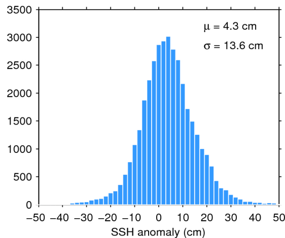
Figure 11. Histogram of science-valid SSH anomaly over oceans and lakes for 10/10/2017. The mean ( \mu ) and standard deviation ( \sigma ) are also shown. Note that values outside [-50 50] cm are excluded from the histogram for the sake of readability but not from the computation of \mu and \sigma .
