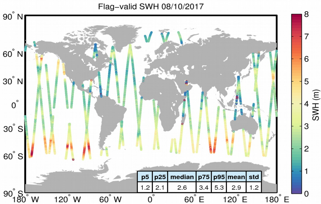
Figure 15. Geographical distribution of flag-valid SWH data over oceans and lakes for 08/10/2017. The statistical values shown in the table refer to the SWH in m and are calculated over all measurements shown in the figure.
