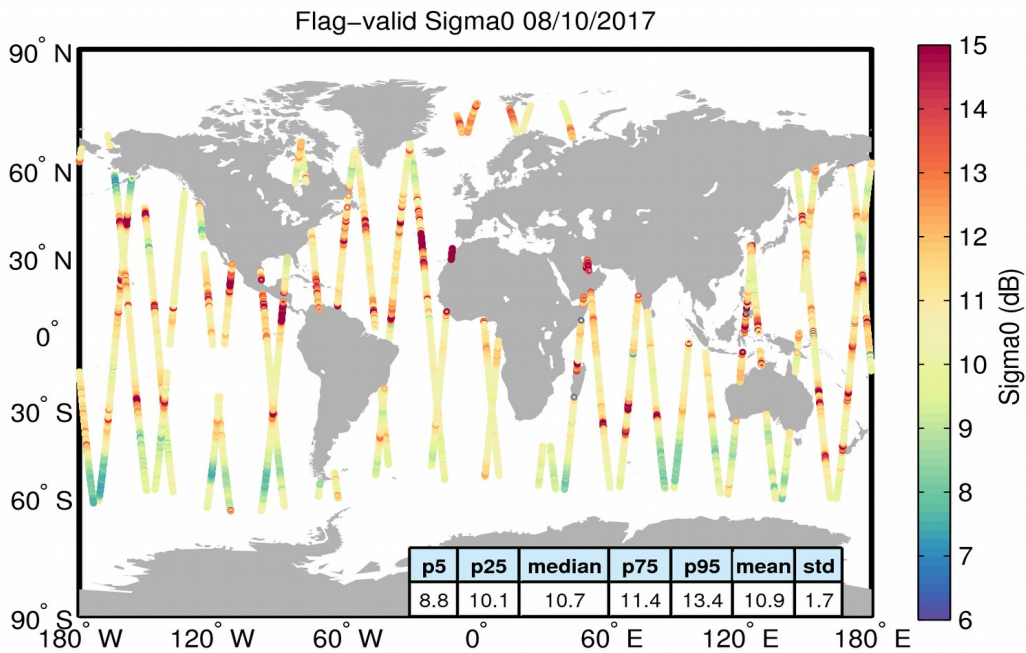
Figure 23. Geographical distribution of flag-valid sigma0 data over oceans and lakes for 08/10/2017. The statistical values shown in the table refer to the sigma0 in dB and are calculated over all measurements shown in the figure.
