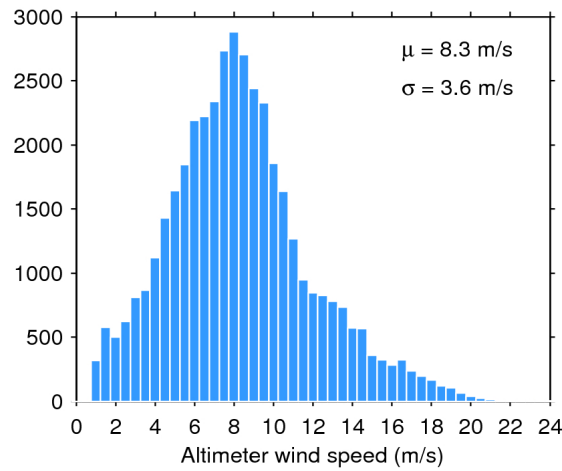
Figure 33. Histogram of flag-valid wind over oceans and lakes for 08/10/2017. The mean ( \mu ) and standard deviation ( \sigma ) are also shown. Note that values larger than 24 m/s are excluded from the histogram for the sake of readability but not from the computation of \mu and \sigma .
