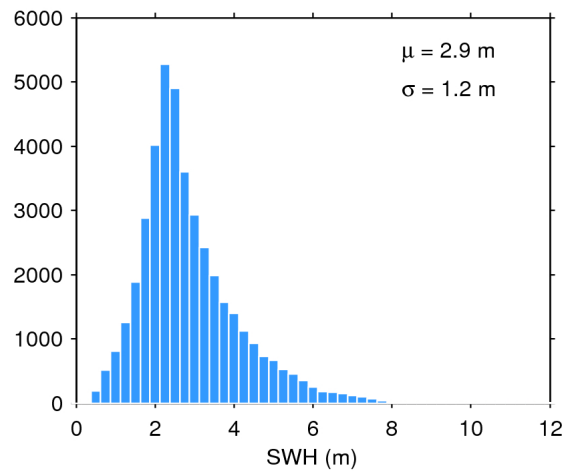
Figure 17. Histogram of flag-valid SWH over oceans and lakes for 08/10/2017. The mean ( \mu ) and standard deviation ( \sigma ) are also shown. Note that values larger than 12 m are excluded from the histogram for the sake of readability but not from the computation of \mu and \sigma .
