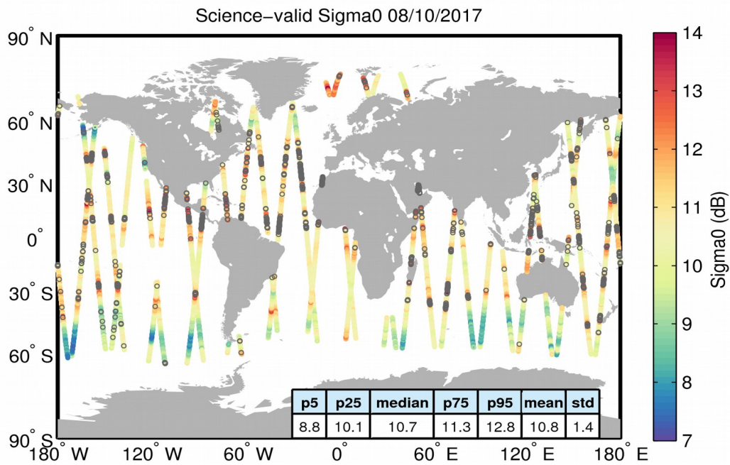
Figure 27. Geographical distribution of science-valid sigma0 data over oceans and lakes for 08/10/2017. The statistical values shown in the table refer to the sigma0 in dB and are calculated over all measurements shown in the figure. Gray circles denote records that have been rejected based on the editing criteria described in Table 4.
