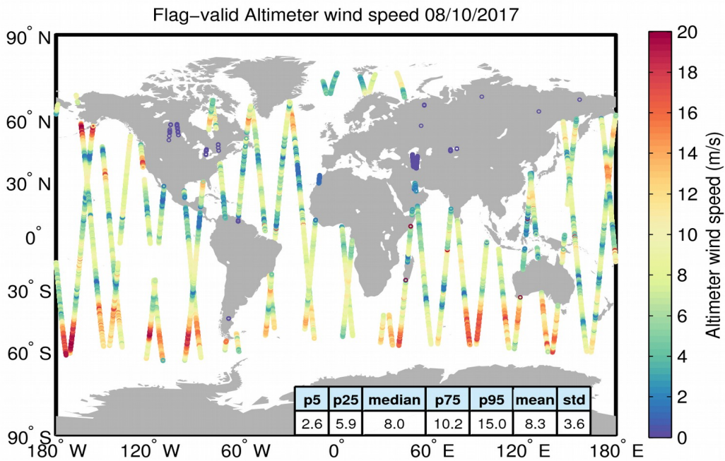
Figure 31. Geographical distribution of flag-valid wind data over oceans and lakes for 08/10/2017. The statistical values shown in the table refer to the wind in m/s and are calculated over all measurements shown in the figure.
