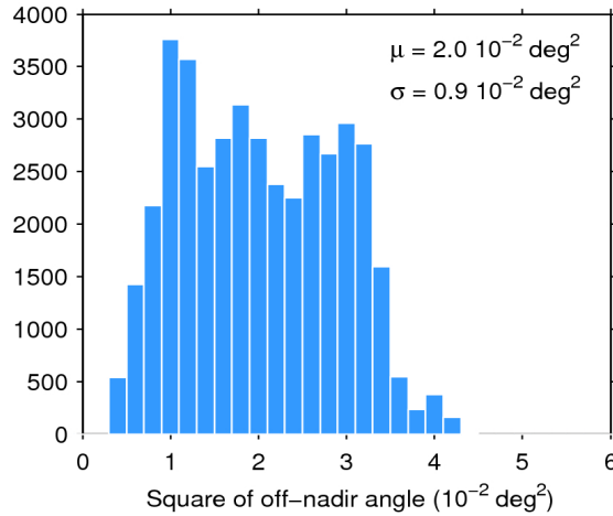
Figure 39. Histogram of flag-valid mispointing over oceans and lakes for 08/10/2017. The mean ( \mu ) and standard deviation ( \sigma ) are also shown. Note that values larger than 6 \cdot 10^{-2} \text{ deg}^2 are excluded from the histogram for the sake of readability but not from the computation of \mu and \sigma .
