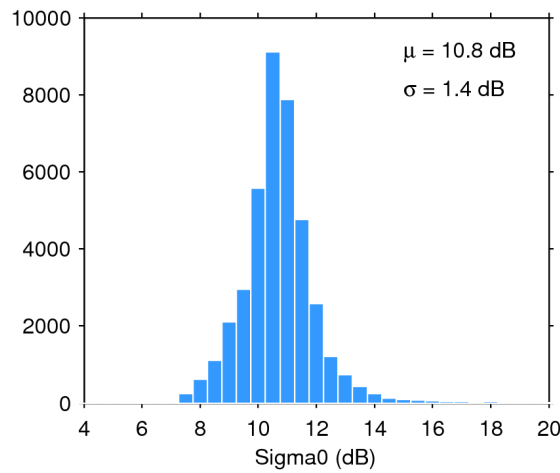
Figure 28. Histogram of science-valid sigma0 over oceans and lakes for 08/10/2017. The mean ( \mu ) and standard deviation ( \sigma ) are also shown. Note that values outside [4 20] dB are excluded from the histogram for the sake of readability but not from the computation of \mu and \sigma .
