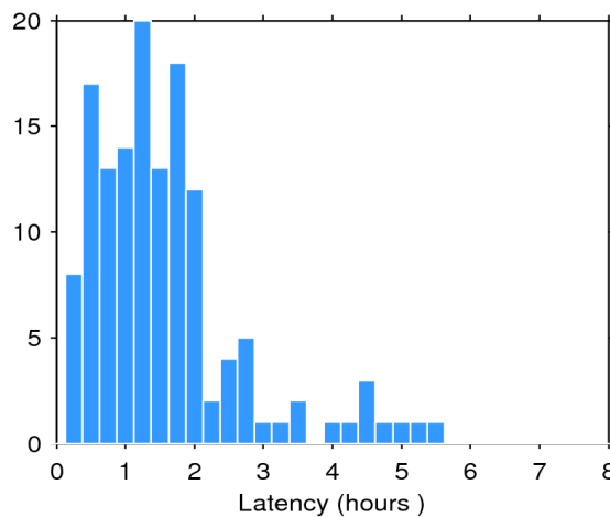
Figure 2. Histogram of the data latency for 08/10/2017. The y-axis denotes the number of files that are made available with a delay of x-hours with respect to the mean time of the records stored in the file.
