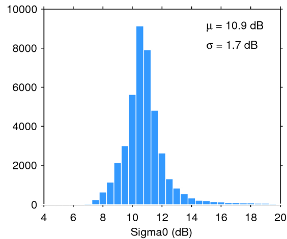
Figure 25. Histogram of flag-valid sigma0 over oceans and lakes for 08/10/2017. The mean ( \mu ) and standard deviation ( \sigma ) are also shown. Note that values outside [4 20] dB are excluded from the histogram for the sake of readability but not from the computation of \mu and \sigma .
