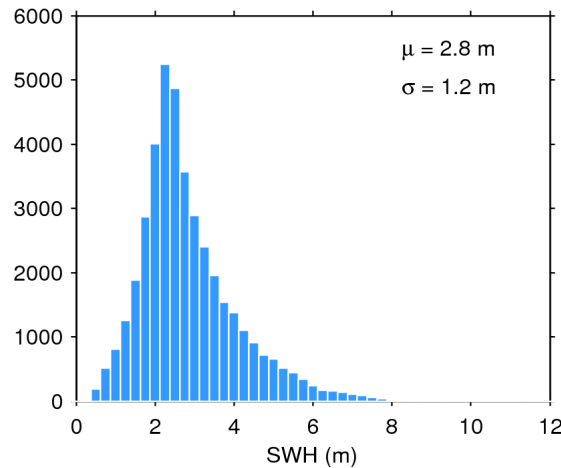
Figure 20. Histogram of science-valid SWH over oceans and lakes for 08/10/2017. The mean ( \mu ) and standard deviation ( \sigma ) are also shown. Note that values larger than 12 m are excluded from the histogram for the sake of readability but not from the computation of \mu and \sigma .
