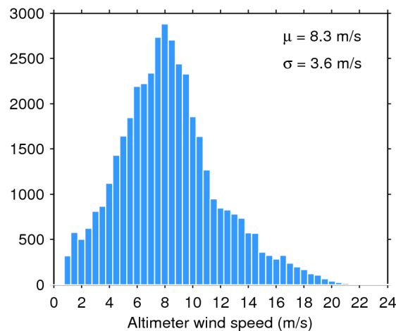
Figure 35. Histogram of science-valid wind over oceans and lakes for 08/10/2017. The mean ( \mu ) and standard deviation ( \sigma ) are also shown. Note that values larger than 24 m/s are excluded from the histogram for the sake of readability but not from the computation of \mu and \sigma .
