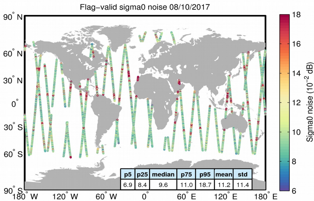
Figure 26. Geographical distribution of flag-valid 20-Hz sigma0 measurement noise over oceans and lakes for 08/10/2017. The statistical values shown in the table refer to the sigma0 noise and are calculated over all measurements shown in the figure.
