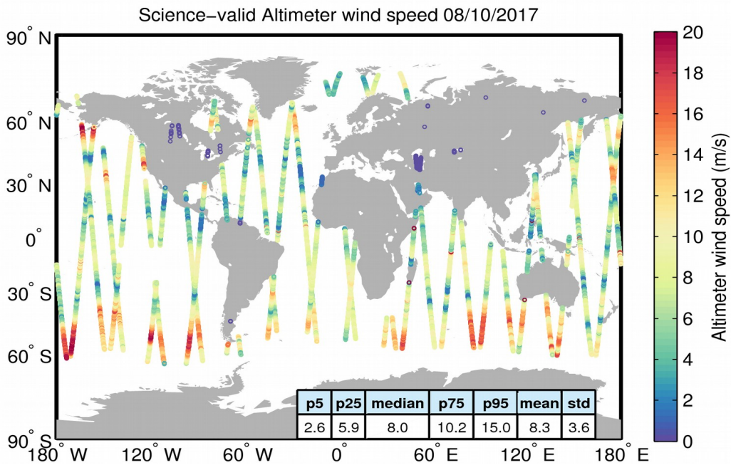
Figure 34. Geographical distribution of science-valid wind data over oceans and lakes for 08/10/2017. The statistical values shown in the table refer to the wind in m/s and are calculated over all measurements shown in the figure. Gray circles denote records that have been rejected based on the editing criteria described in Table 5.
