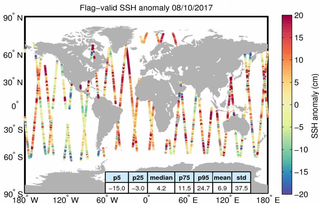
Figure 5. Geographical distribution of flag-valid 1-Hz SSH anomaly data over oceans and lakes for 08/10/2017. The statistical values shown in the table refer to the SSH anomaly in cm and are calculated over all measurements shown in the figure.
