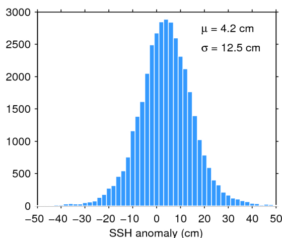
Figure 11. Histogram of science-valid SSH anomaly over oceans and lakes for 08/10/2017. The mean ( \mu ) and standard deviation ( \sigma ) are also shown. Note that values outside [-50 50] cm are excluded from the histogram for the sake of readability but not from the computation of \mu and \sigma .
