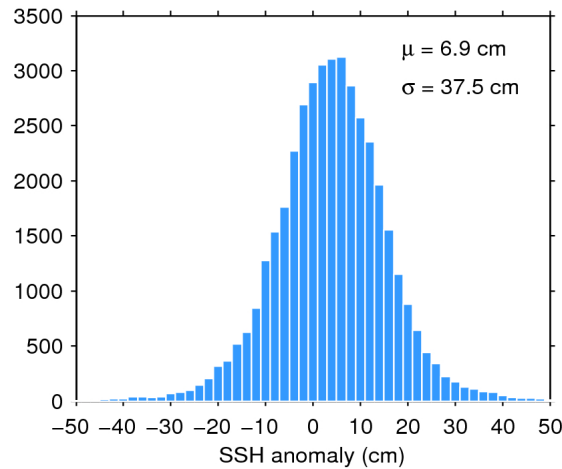
Figure 7. Histogram of flag-valid SSH anomaly over oceans and lakes for 08/10/2017. The mean ( \mu ) and standard deviation ( \sigma ) are also shown. Note that values outside [-50\ 50] cm are excluded from the histogram for the sake of readability but not from the computation of \mu and \sigma .
