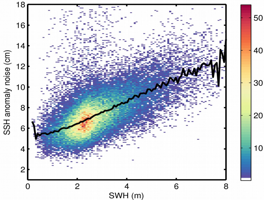
Figure 9. 2D histogram showing flag-valid SSH anomaly noise as a function of SWH for 08/10/2017. The black line denotes the median SSH anomaly noise as a function of SWH.
