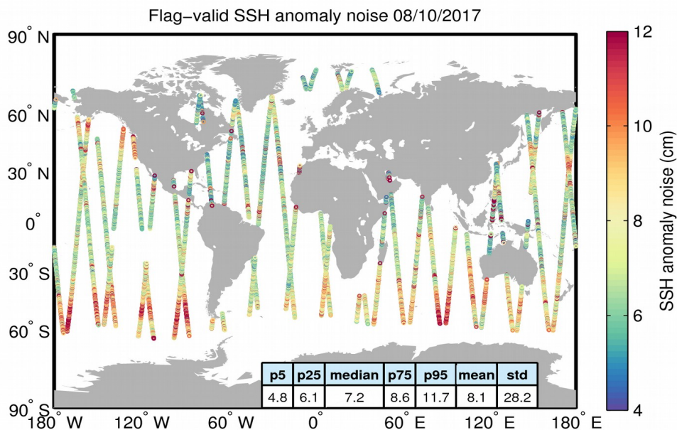
Figure 8. Geographical distribution of flag-valid 20-Hz SSH anomaly measurement noise over oceans and lakes for 08/10/2017. The statistical values shown in the table refer to the SSH anomaly noise and are calculated over all measurements shown in the figure.
