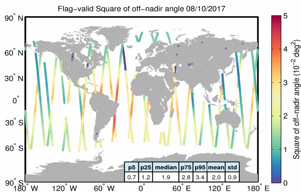
Figure 37. Geographical distribution of flag-valid mispointing data over oceans and lakes for 08/10/2017. The statistical values shown in the table refer to the mispointing in 10^{-2} \text{deg}^2 and are calculated over all measurements shown in the figure.
