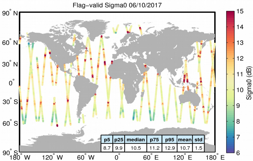
Figure 23. Geographical distribution of flag-valid sigma0 data over oceans and lakes for 06/10/2017. The statistical values shown in the table refer to the sigma0 in dB and are calculated over all measurements shown in the figure.
