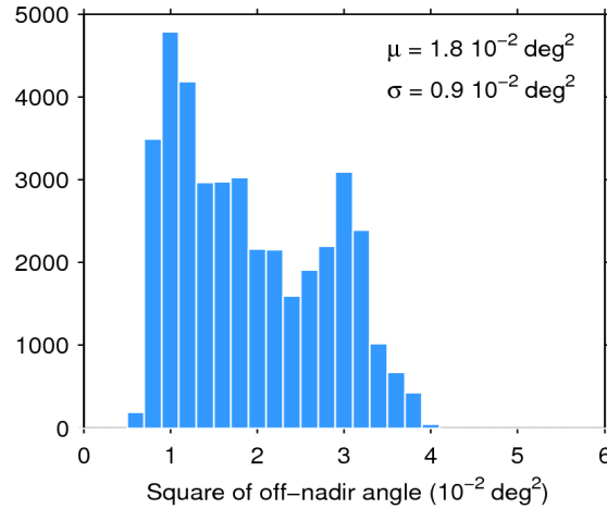
Figure 39. Histogram of flag-valid mispointing over oceans and lakes for 06/10/2017. The mean ( \mu ) and standard deviation ( \sigma ) are also shown. Note that values larger than 6 \cdot 10^{-2} \text{ deg}^2 are excluded from the histogram for the sake of readability but not from the computation of \mu and \sigma .
