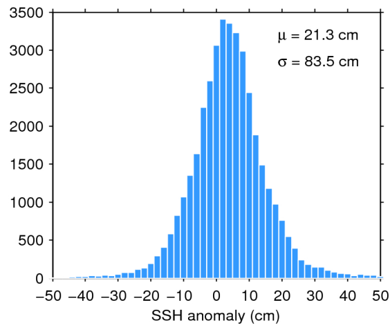
Figure 7. Histogram of flag-valid SSH anomaly over oceans and lakes for 06/10/2017. The mean ( \mu ) and standard deviation ( \sigma ) are also shown. Note that values outside [-50 50] cm are excluded from the histogram for the sake of readability but not from the computation of \mu and \sigma .
