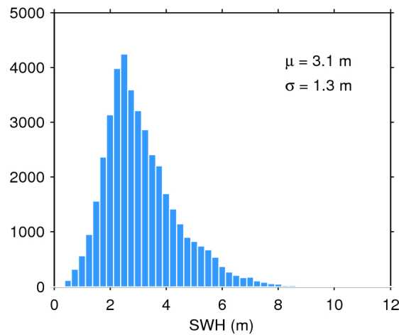
Figure 17. Histogram of flag-valid SWH over oceans and lakes for 06/10/2017. The mean ( \mu ) and standard deviation ( \sigma ) are also shown. Note that values larger than 12 m are excluded from the histogram for the sake of readability but not from the computation of \mu and \sigma .
