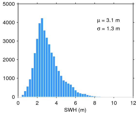
Figure 20. Histogram of science-valid SWH over oceans and lakes for 06/10/2017. The mean ( \mu ) and standard deviation ( \sigma ) are also shown. Note that values larger than 12 m are excluded from the histogram for the sake of readability but not from the computation of \mu and \sigma .
