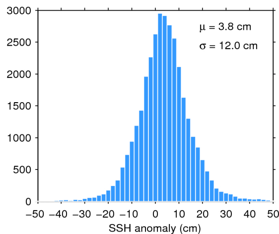
Figure 11. Histogram of science-valid SSH anomaly over oceans and lakes for 06/10/2017. The mean ( \mu ) and standard deviation ( \sigma ) are also shown. Note that values outside [-50 50] cm are excluded from the histogram for the sake of readability but not from the computation of \mu and \sigma .
