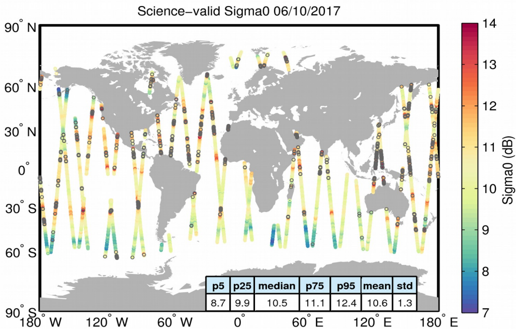
Figure 27. Geographical distribution of science-valid sigma0 data over oceans and lakes for 06/10/2017. The statistical values shown in the table refer to the sigma0 in dB and are calculated over all measurements shown in the figure. Gray circles denote records that have been rejected based on the editing criteria described in Table 4.
