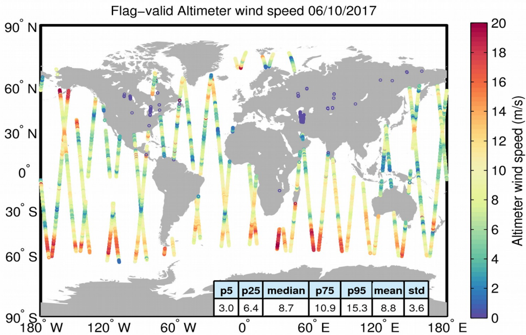
Figure 31. Geographical distribution of flag-valid wind data over oceans and lakes for 06/10/2017. The statistical values shown in the table refer to the wind in m/s and are calculated over all measurements shown in the figure.
