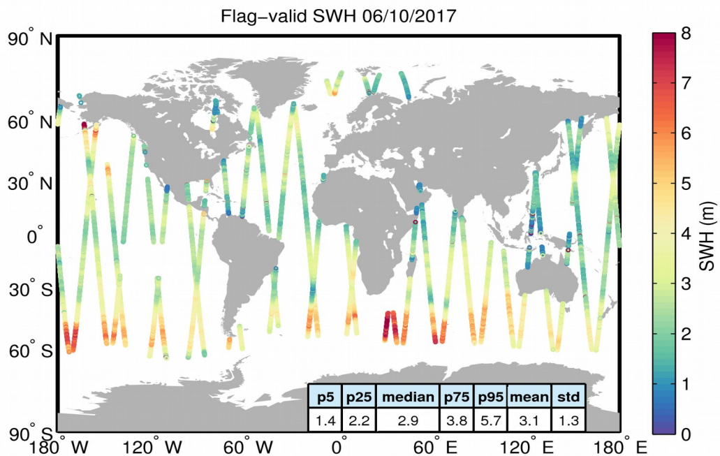
Figure 15. Geographical distribution of flag-valid SWH data over oceans and lakes for 06/10/2017. The statistical values shown in the table refer to the SWH in m and are calculated over all measurements shown in the figure.
