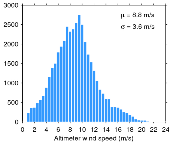
Figure 33. Histogram of flag-valid wind over oceans and lakes for 06/10/2017. The mean ( \mu ) and standard deviation ( \sigma ) are also shown. Note that values larger than 24 m/s are excluded from the histogram for the sake of readability but not from the computation of \mu and \sigma .
