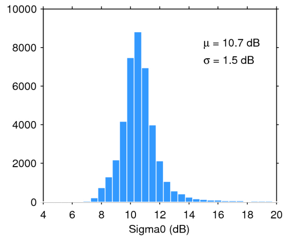
Figure 25. Histogram of flag-valid sigma0 over oceans and lakes for 06/10/2017. The mean ( \mu ) and standard deviation ( \sigma ) are also shown. Note that values outside [4 20] dB are excluded from the histogram for the sake of readability but not from the computation of \mu and \sigma .
