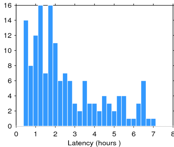
Figure 2. Histogram of the data latency for 06/10/2017. The y-axis denotes the number of files that are made available with a delay of x-hours with respect to the mean time of the records stored in the file.
