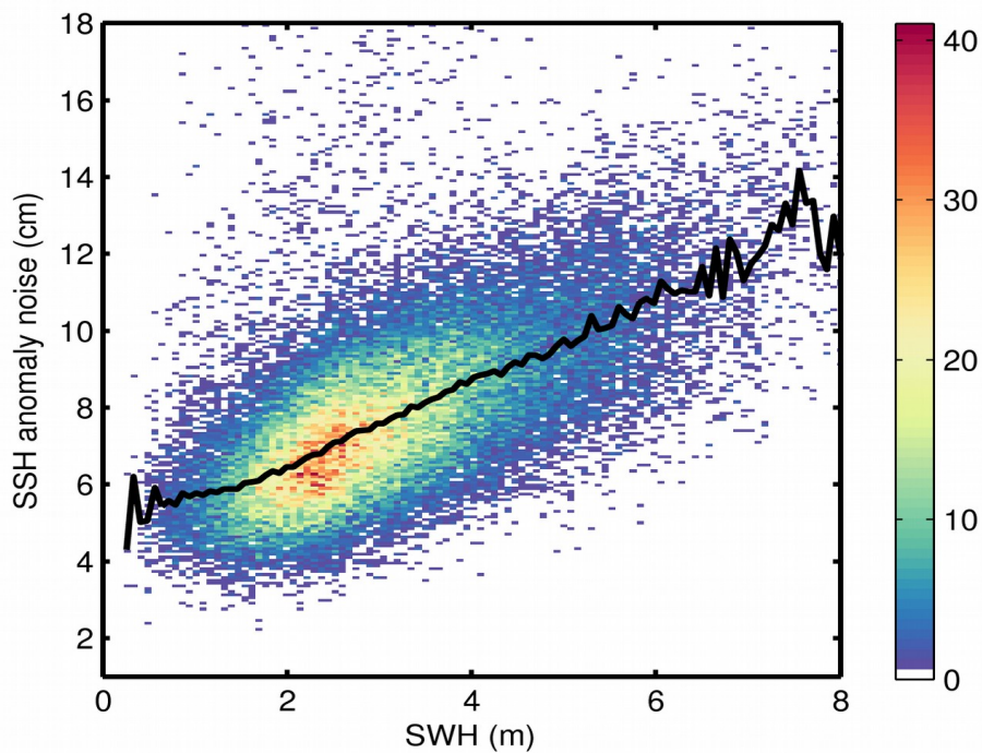
Figure 9. 2D histogram showing flag-valid SSH anomaly noise as a function of SWH for 06/10/2017. The black line denotes the median SSH anomaly noise as a function of SWH.
