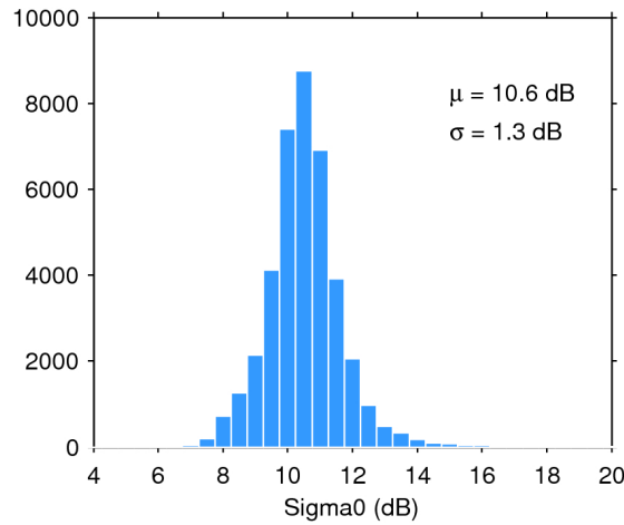
Figure 28. Histogram of science-valid sigma0 over oceans and lakes for 06/10/2017. The mean ( \mu ) and standard deviation ( \sigma ) are also shown. Note that values outside [4 20] dB are excluded from the histogram for the sake of readability but not from the computation of \mu and \sigma .
