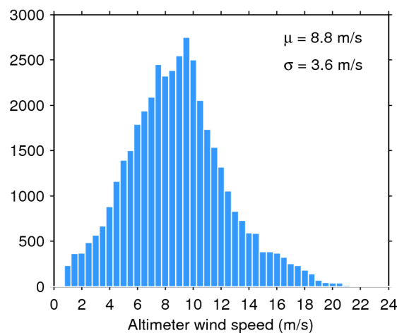
Figure 35. Histogram of science-valid wind over oceans and lakes for 06/10/2017. The mean ( \mu ) and standard deviation ( \sigma ) are also shown. Note that values larger than 24 m/s are excluded from the histogram for the sake of readability but not from the computation of \mu and \sigma .
