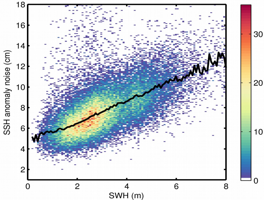
Figure 9. 2D histogram showing flag-valid SSH anomaly noise as a function of SWH for 05/10/2017. The black line denotes the median SSH anomaly noise as a function of SWH.
