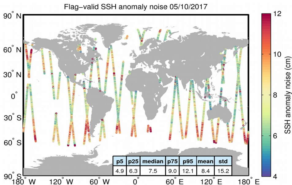
Figure 8. Geographical distribution of flag-valid 20-Hz SSH anomaly measurement noise over oceans and lakes for 05/10/2017. The statistical values shown in the table refer to the SSH anomaly noise and are calculated over all measurements shown in the figure.
