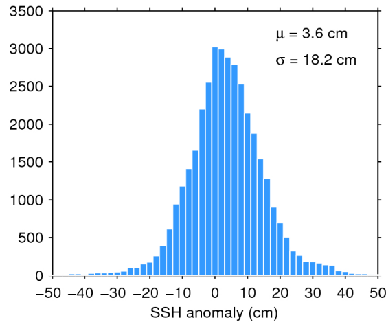
Figure 7. Histogram of flag-valid SSH anomaly over oceans and lakes for 05/10/2017. The mean ( \mu ) and standard deviation ( \sigma ) are also shown. Note that values outside [-50\ 50] cm are excluded from the histogram for the sake of readability but not from the computation of \mu and \sigma .
