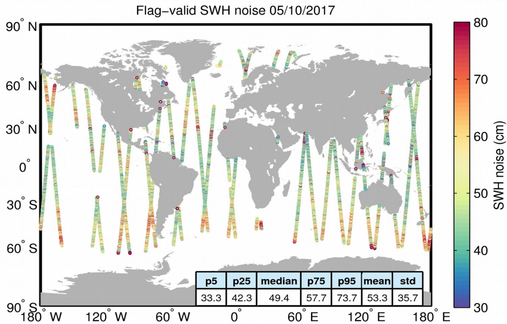
Figure 18. Geographical distribution of flag-valid 20-Hz SWH measurement noise over oceans and lakes for 05/10/2017. The statistical values shown in the table refer to the SWH noise and are calculated over all measurements shown in the figure.
