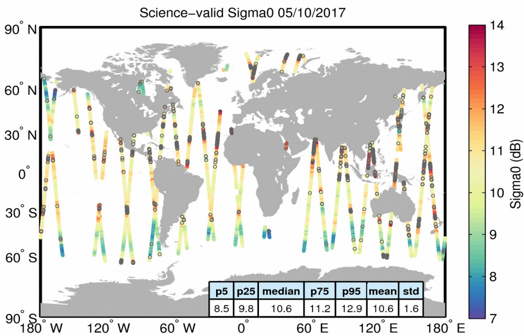
Figure 27. Geographical distribution of science-valid sigma0 data over oceans and lakes for 05/10/2017. The statistical values shown in the table refer to the sigma0 in dB and are calculated over all measurements shown in the figure. Gray circles denote records that have been rejected based on the editing criteria described in Table 4.
