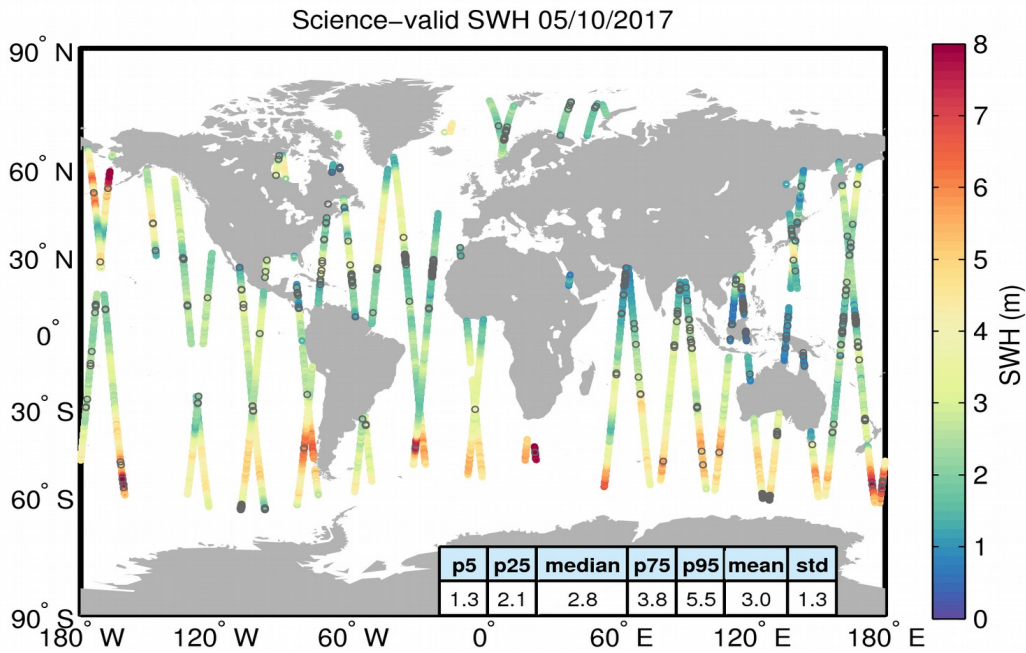
Figure 19. Geographical distribution of science-valid SWH data over oceans and lakes for 05/10/2017. The statistical values shown in the table refer to the SWH in m and are calculated over all measurements shown in the figure. Gray circles denote records that have been rejected based on the editing criteria described in Table 3.
