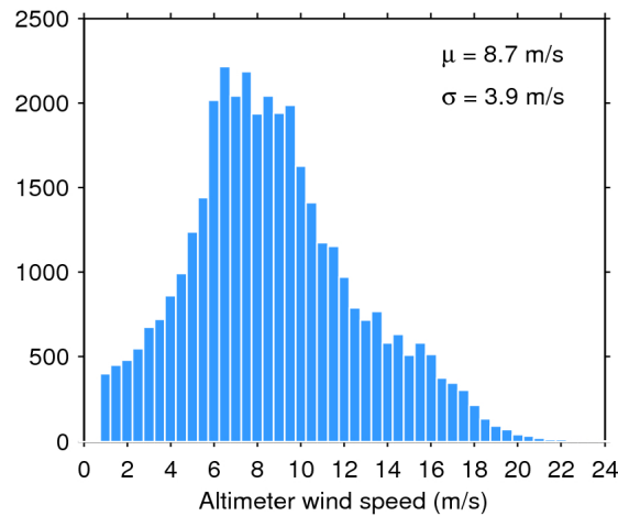
Figure 33. Histogram of flag-valid wind over oceans and lakes for 05/10/2017. The mean ( \mu ) and standard deviation ( \sigma ) are also shown. Note that values larger than 24 m/s are excluded from the histogram for the sake of readability but not from the computation of \mu and \sigma .
