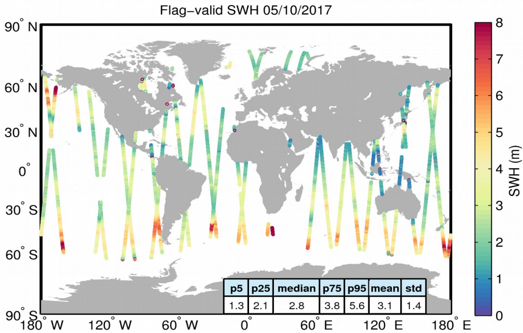
Figure 15. Geographical distribution of flag-valid SWH data over oceans and lakes for 05/10/2017. The statistical values shown in the table refer to the SWH in m and are calculated over all measurements shown in the figure.
