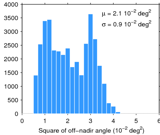
Figure 39. Histogram of flag-valid mispointing over oceans and lakes for 05/10/2017. The mean ( \mu ) and standard deviation ( \sigma ) are also shown. Note that values larger than 6 \cdot 10^{-2} \text{ deg}^2 are excluded from the histogram for the sake of readability but not from the computation of \mu and \sigma .
