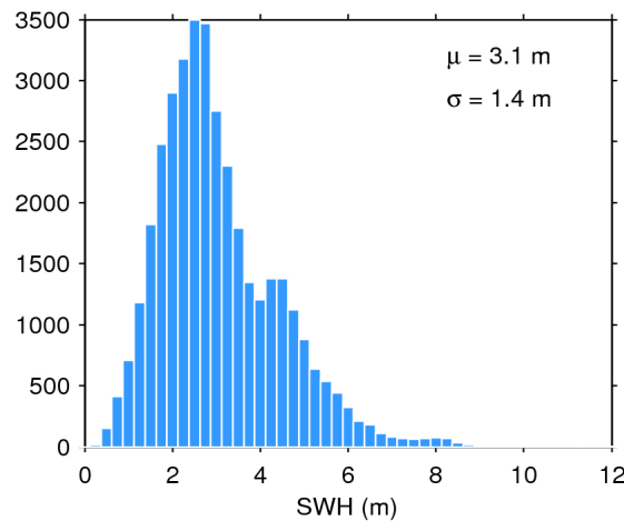
Figure 17. Histogram of flag-valid SWH over oceans and lakes for 05/10/2017. The mean ( \mu ) and standard deviation ( \sigma ) are also shown. Note that values larger than 12 m are excluded from the histogram for the sake of readability but not from the computation of \mu and \sigma .
