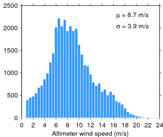
Figure 35. Histogram of science-valid wind over oceans and lakes for 05/10/2017. The mean ( \mu ) and standard deviation ( \sigma ) are also shown. Note that values larger than 24 m/s are excluded from the histogram for the sake of readability but not from the computation of \mu and \sigma .
