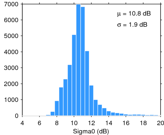
Figure 25. Histogram of flag-valid sigma0 over oceans and lakes for 05/10/2017. The mean ( \mu ) and standard deviation ( \sigma ) are also shown. Note that values outside [4 20] dB are excluded from the histogram for the sake of readability but not from the computation of \mu and \sigma .
