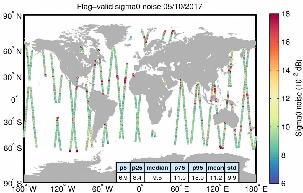
Figure 26. Geographical distribution of flag-valid 20-Hz sigma0 measurement noise over oceans and lakes for 05/10/2017. The statistical values shown in the table refer to the sigma0 noise and are calculated over all measurements shown in the figure.
