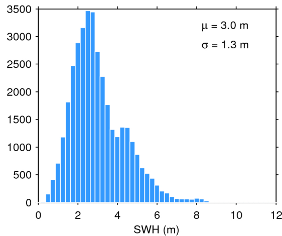
Figure 20. Histogram of science-valid SWH over oceans and lakes for 05/10/2017. The mean ( \mu ) and standard deviation ( \sigma ) are also shown. Note that values larger than 12 m are excluded from the histogram for the sake of readability but not from the computation of \mu and \sigma .
