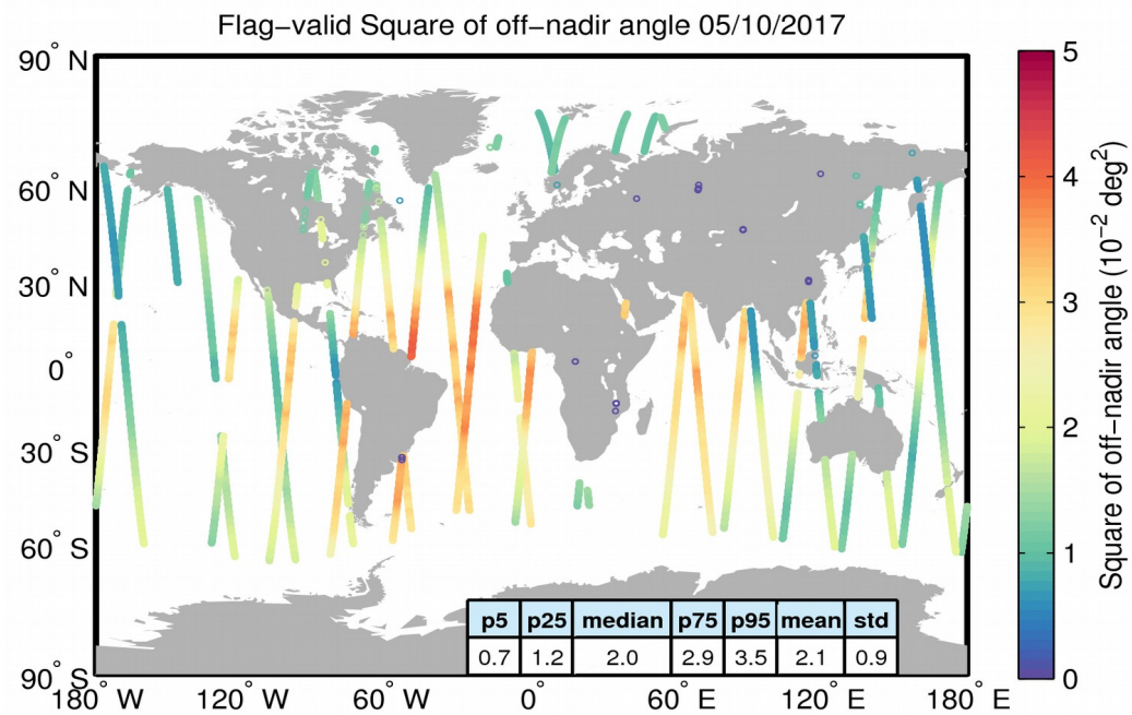
Figure 37. Geographical distribution of flag-valid mispointing data over oceans and lakes for 05/10/2017. The statistical values shown in the table refer to the mispointing in 10^{-2} deg 2 and are calculated over all measurements shown in the figure.
