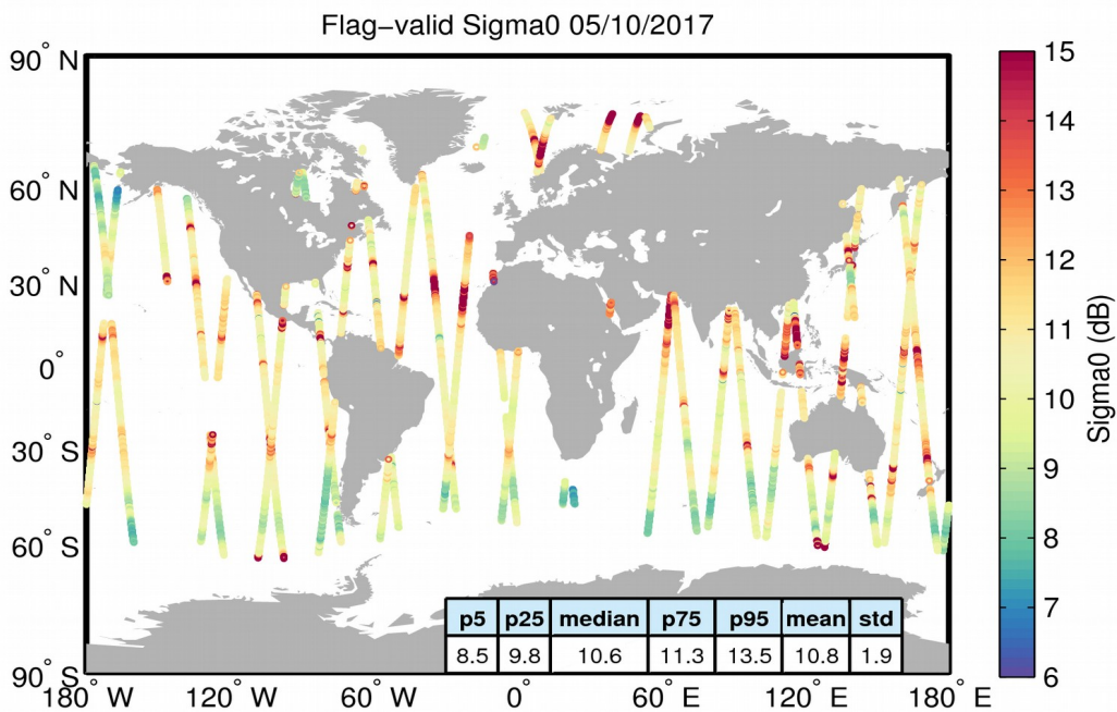
Figure 23. Geographical distribution of flag-valid sigma0 data over oceans and lakes for 05/10/2017. The statistical values shown in the table refer to the sigma0 in dB and are calculated over all measurements shown in the figure.
