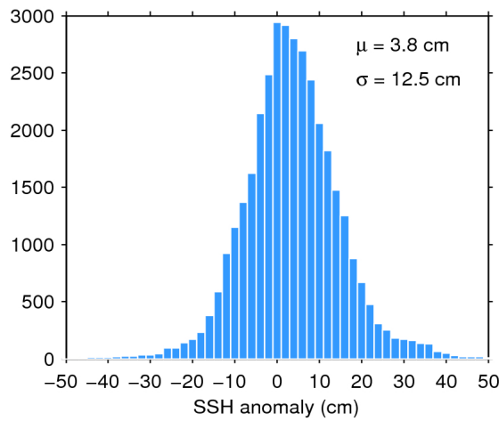
Figure 11. Histogram of science-valid SSH anomaly over oceans and lakes for 05/10/2017. The mean ( \mu ) and standard deviation ( \sigma ) are also shown. Note that values outside [-50 50] cm are excluded from the histogram for the sake of readability but not from the computation of \mu and \sigma .
