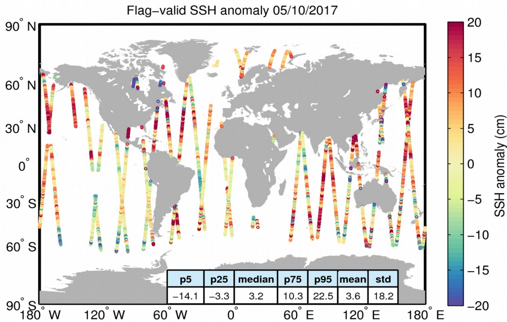
Figure 5. Geographical distribution of flag-valid 1-Hz SSH anomaly data over oceans and lakes for 05/10/2017. The statistical values shown in the table refer to the SSH anomaly in cm and are calculated over all measurements shown in the figure.
